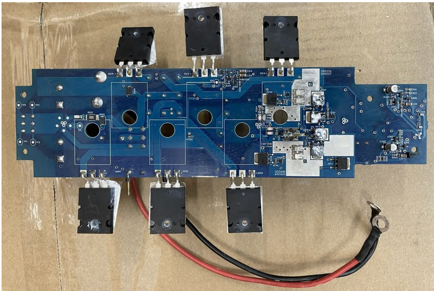
ZCAS4GHEATSINK - Caspian 4G Power Amplifier PCB BOTTOM.JPG
