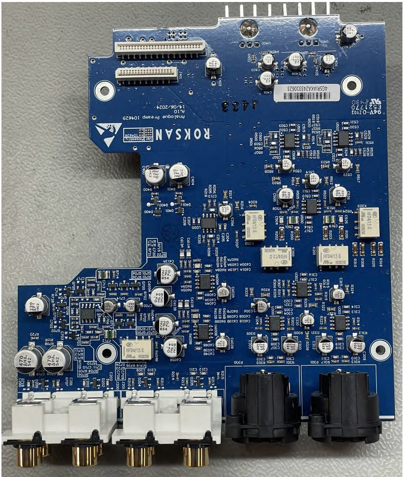
ZCAS4GPREPCB - Caspian 4G PRE-RIAA Assembly TOP.JPEG
