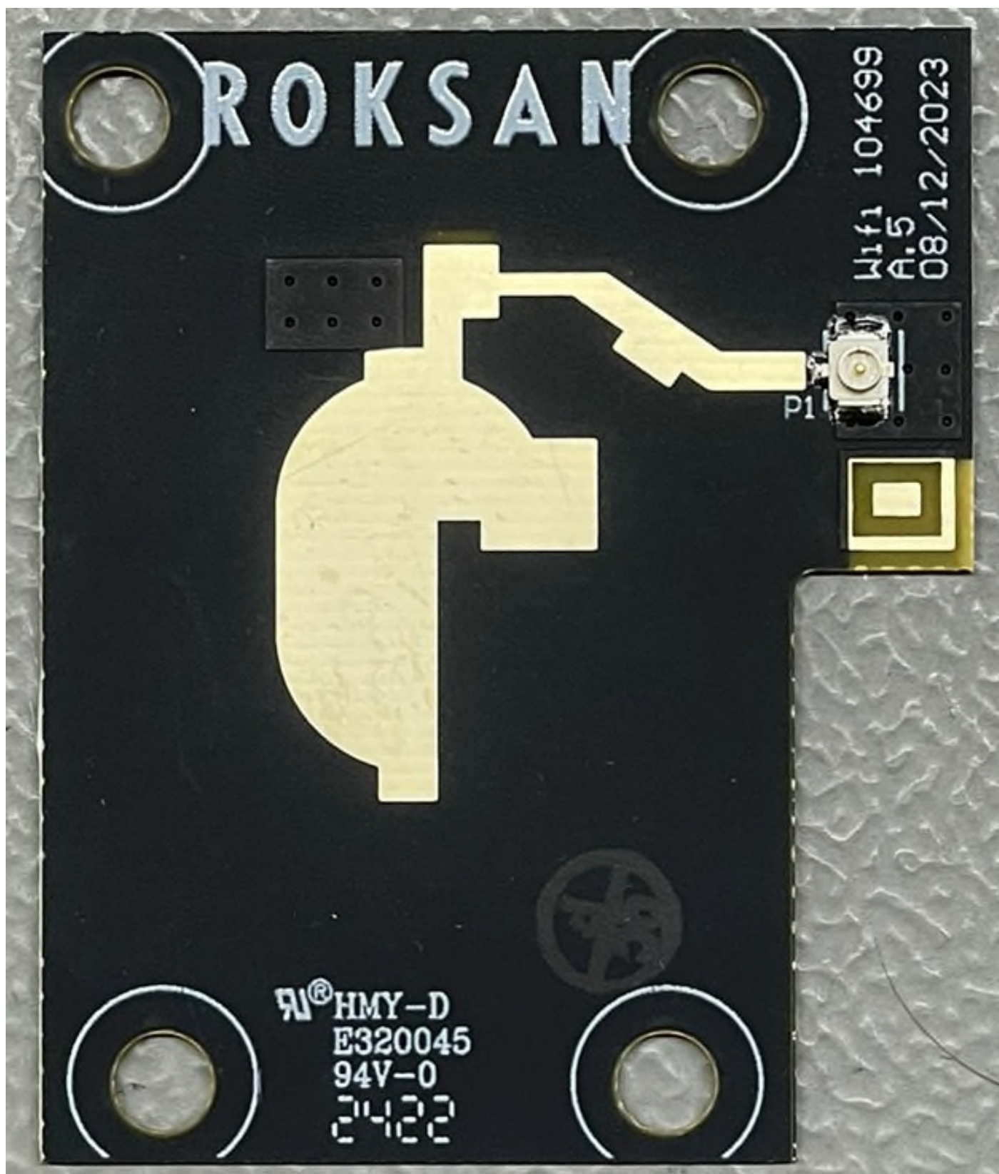
ZCAS4GWIFIPCB - Caspian 4G Dual Band WiFi/BT ANT PCB TOP.JPEG
