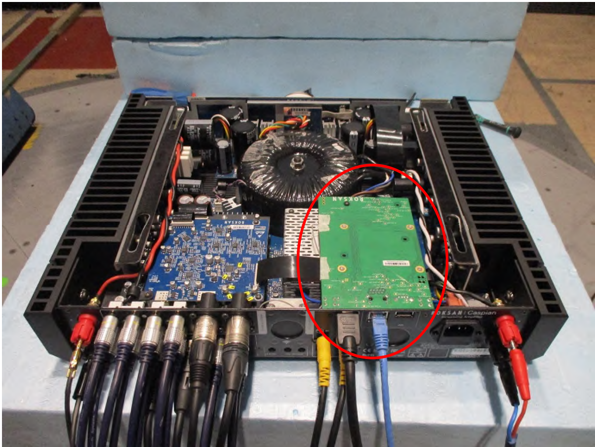
WLAN Module board in place circled
