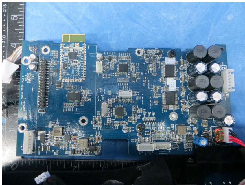
PCB Board
