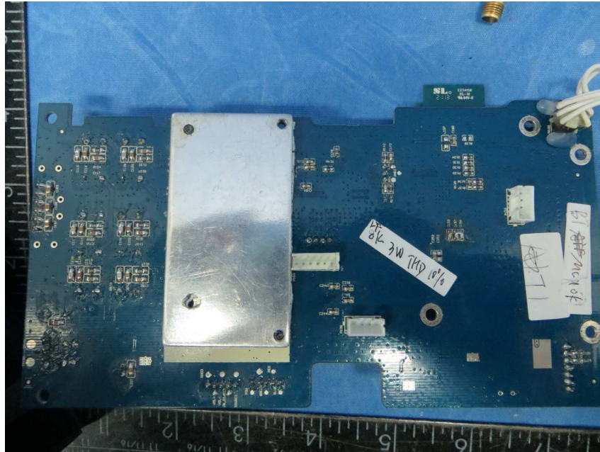
Internal PCB antenna
