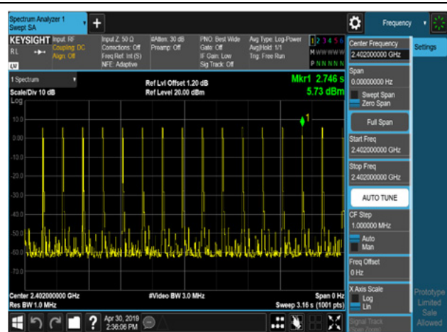
GFSK,2402,DH5,Transmission Number
