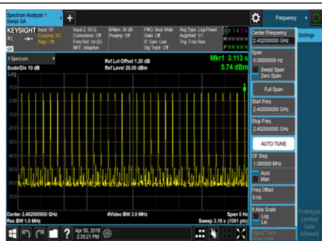
GFSK,2402,DH3,Transmission Number
