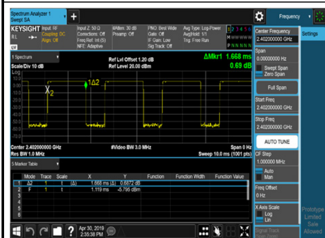
GFSK,2402,DH5,Transmission Time
