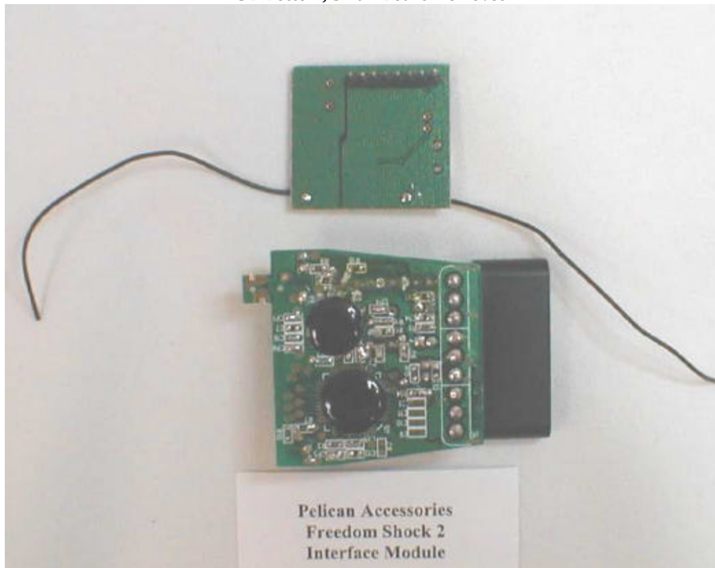
PCB Bottom, Small Board Removed
