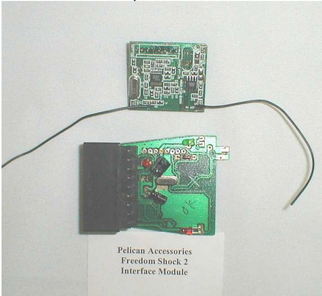
PCB Bottom, Small Board Removed
