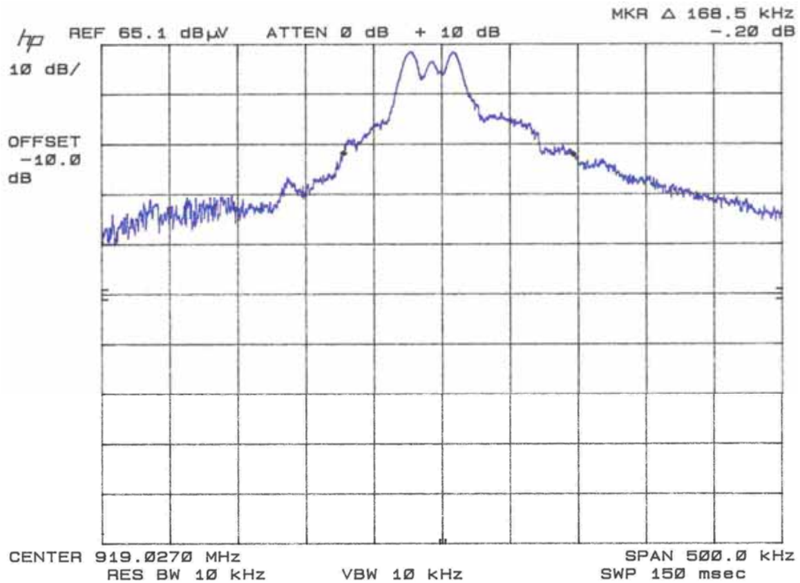
Figure 4-5. Occupied Bandwidth, Channel 3
