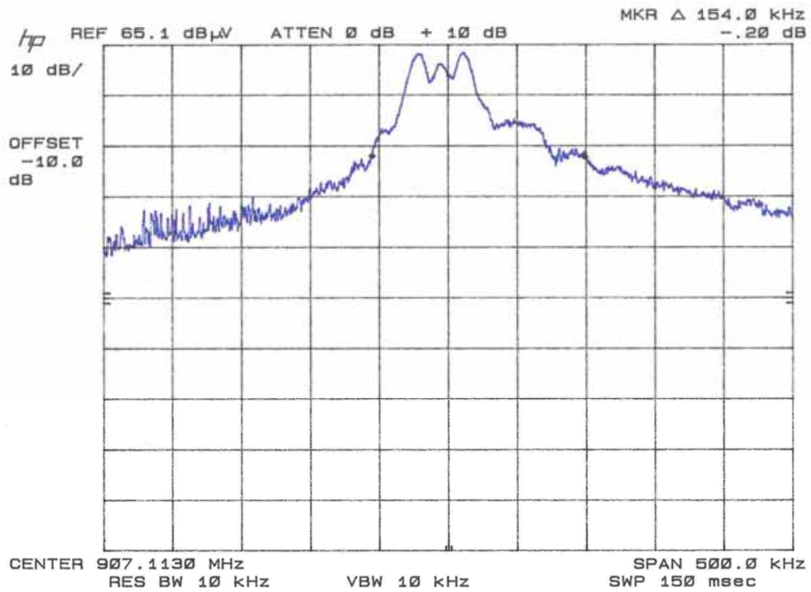
Figure 4-3. Occupied Bandwidth, Channel 1
