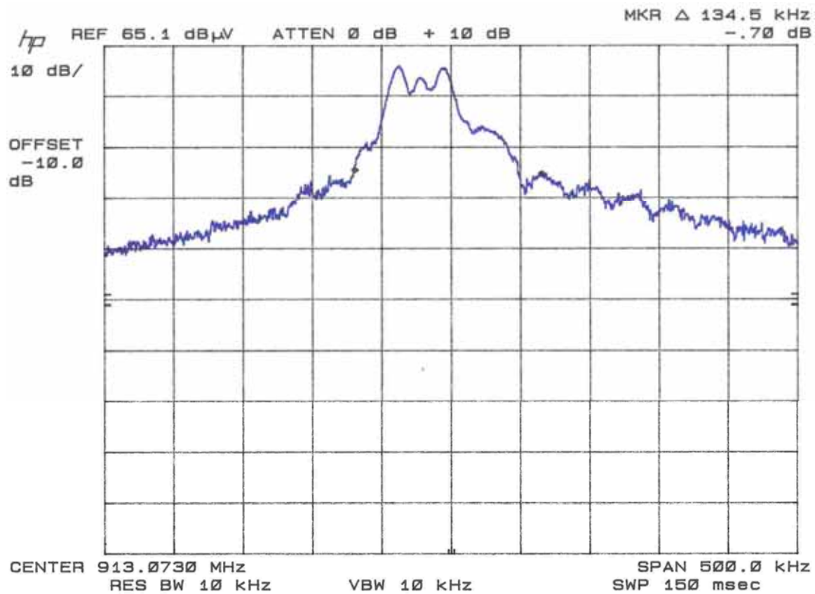
Figure 4-4. Occupied Bandwidth, Channel 2
