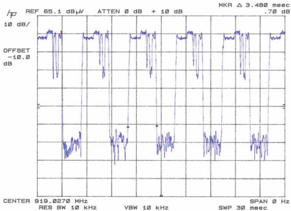
Figure 4-2. Duty Cycle Plot, Pulse Width
