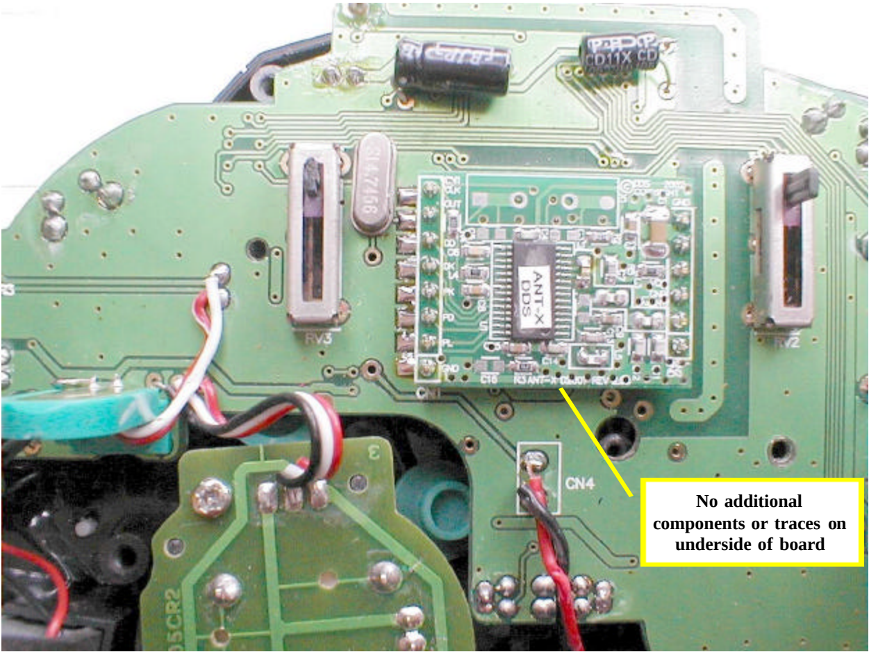
Functional Board, Top Detail
