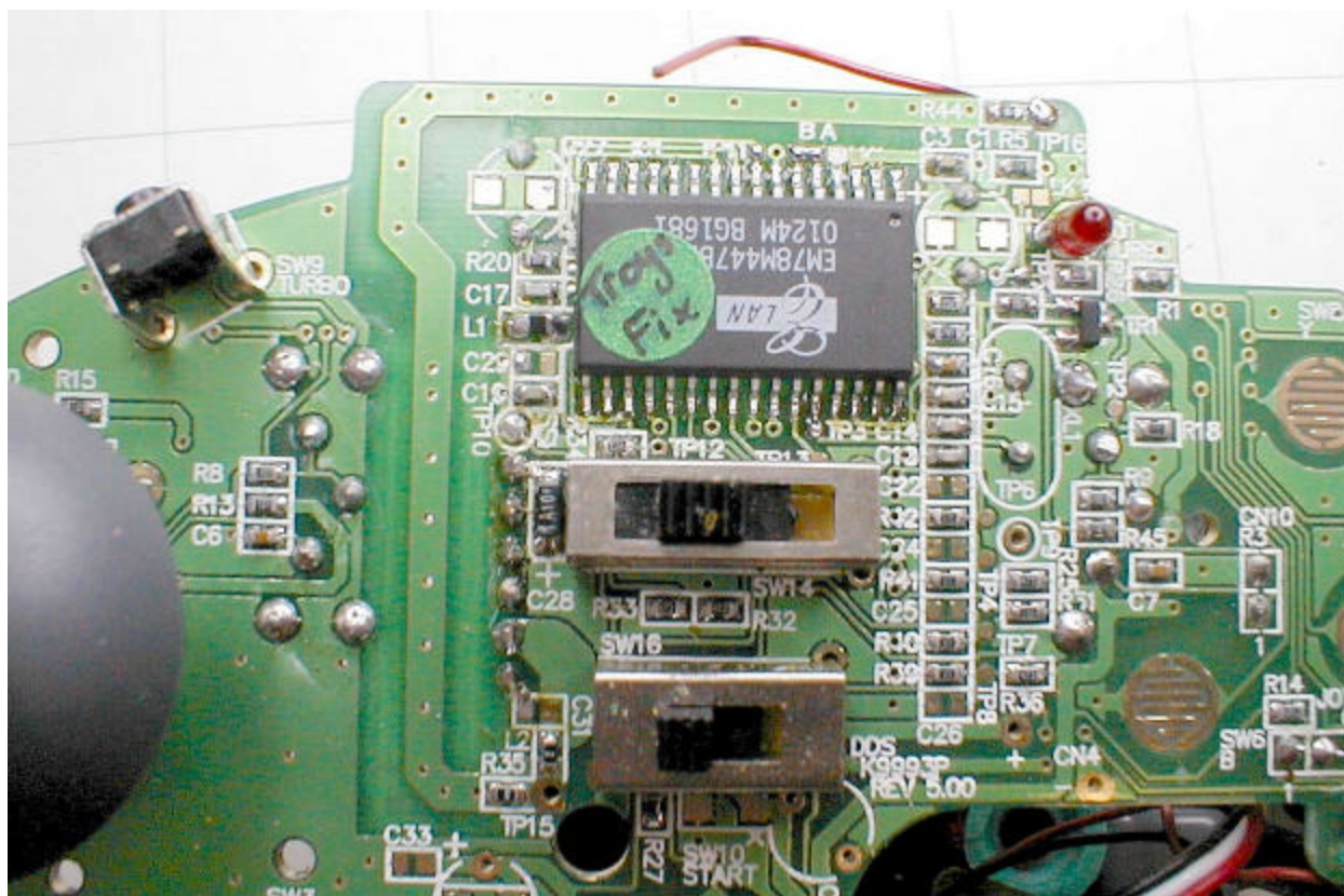
Functional Board, Bottom Detail
