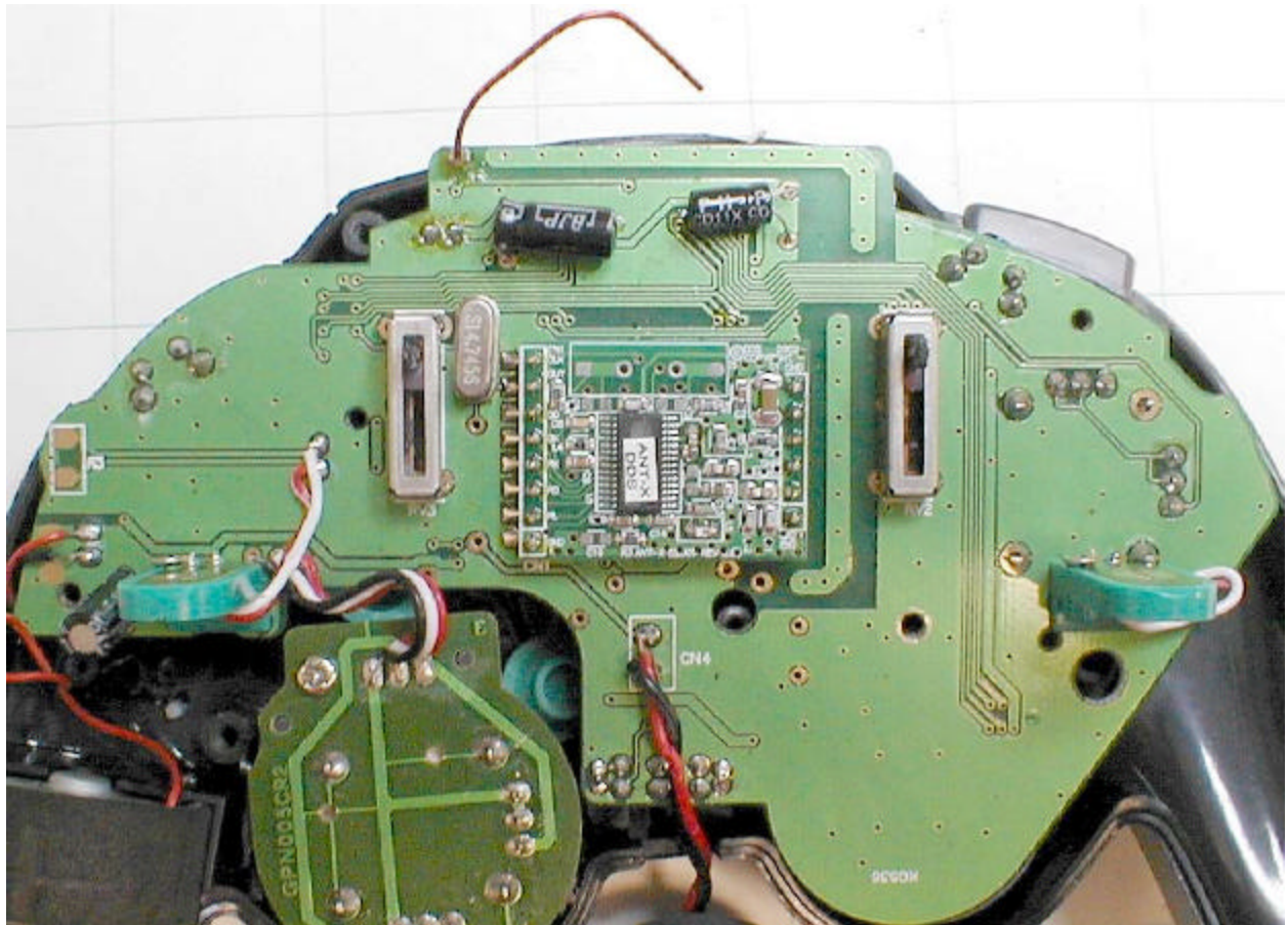
Functional Board, Top
