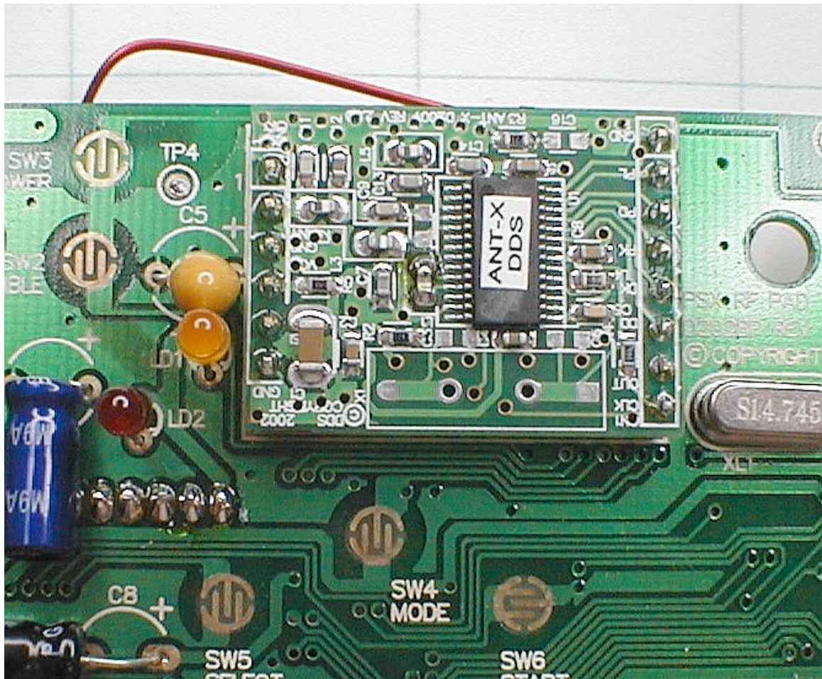
Radio Board in Place on Function Board
