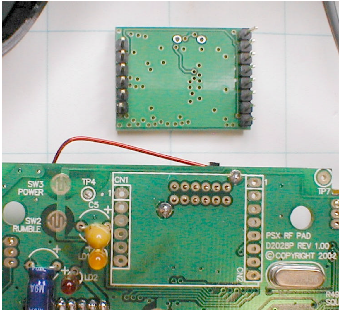
Radio Board Removed from Function Board
