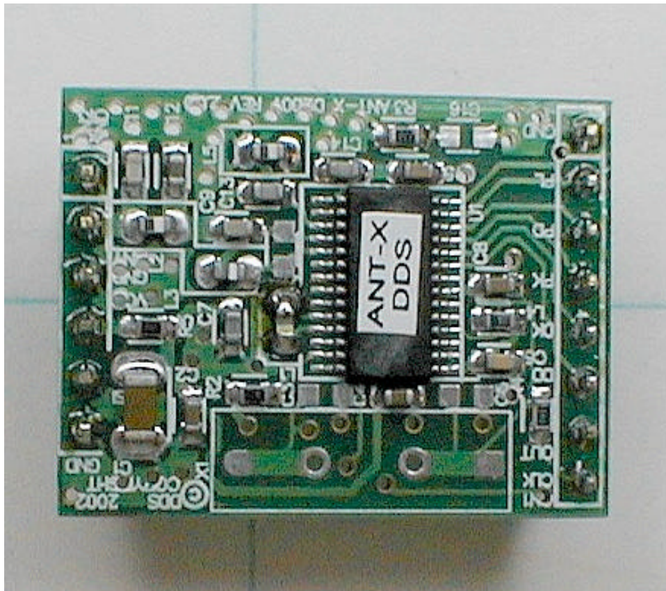
Radio Board Top
