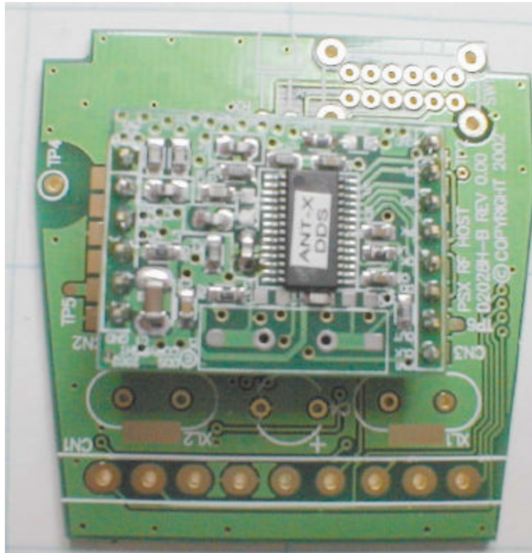
Radio Board in place on Main Board
