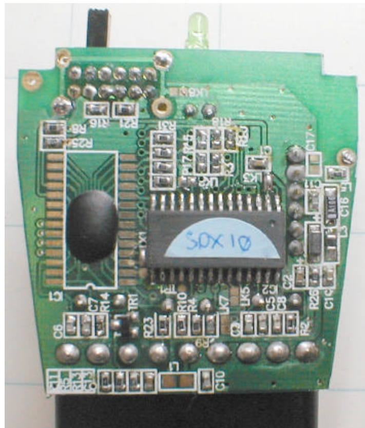
Bottom View of Function Board
