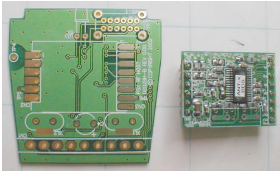
Radio Board Removed
