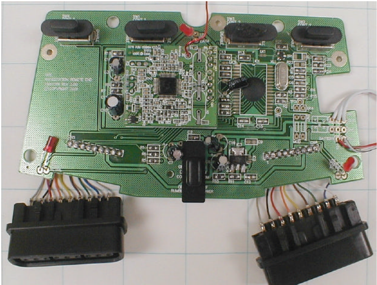
Top View of PC Board with Radio Module
