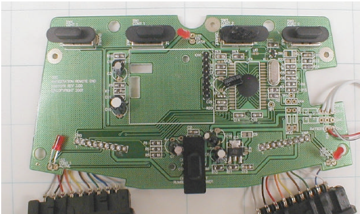
Top View of PC Board Without Radio Module
