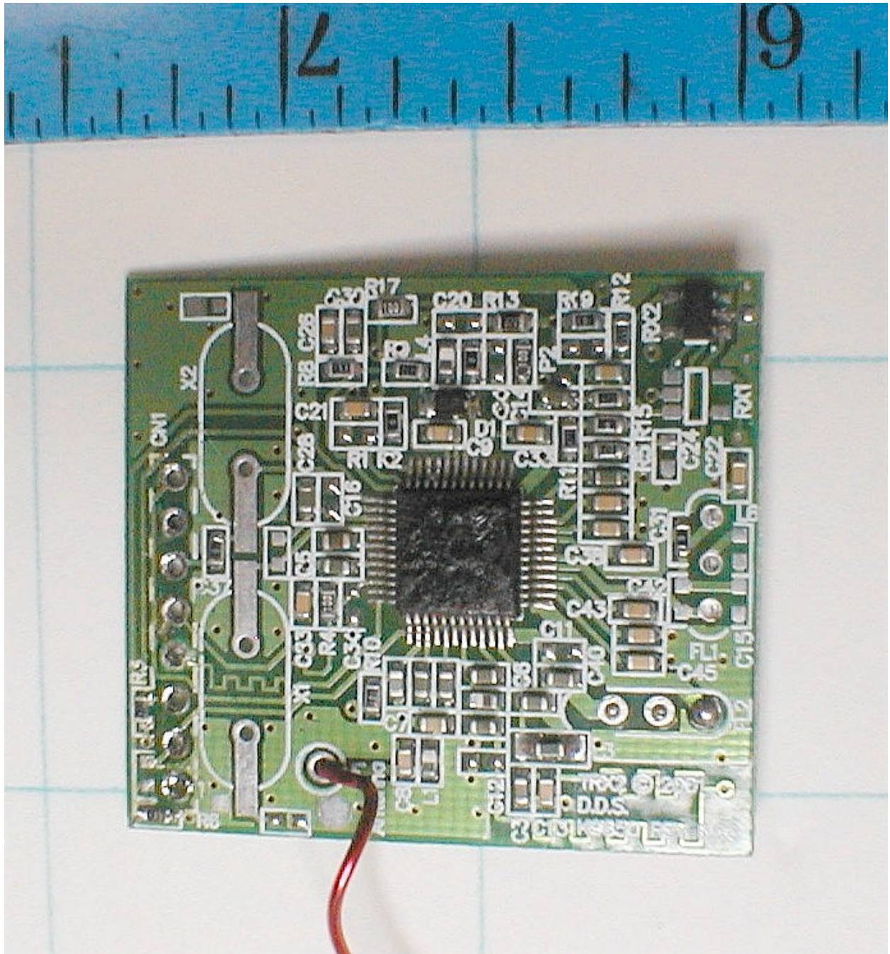
Radio Module Top View
