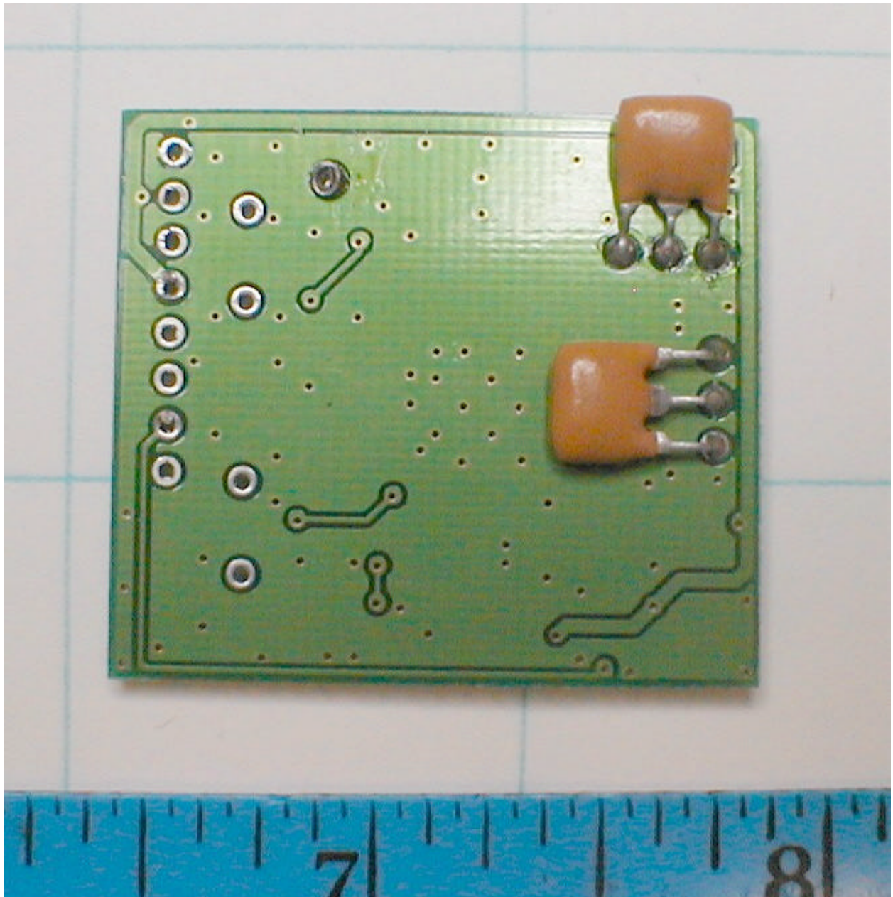
Radio Module Bottom View
