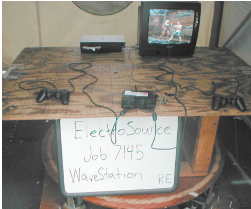
Emissions Testing, Rear View
