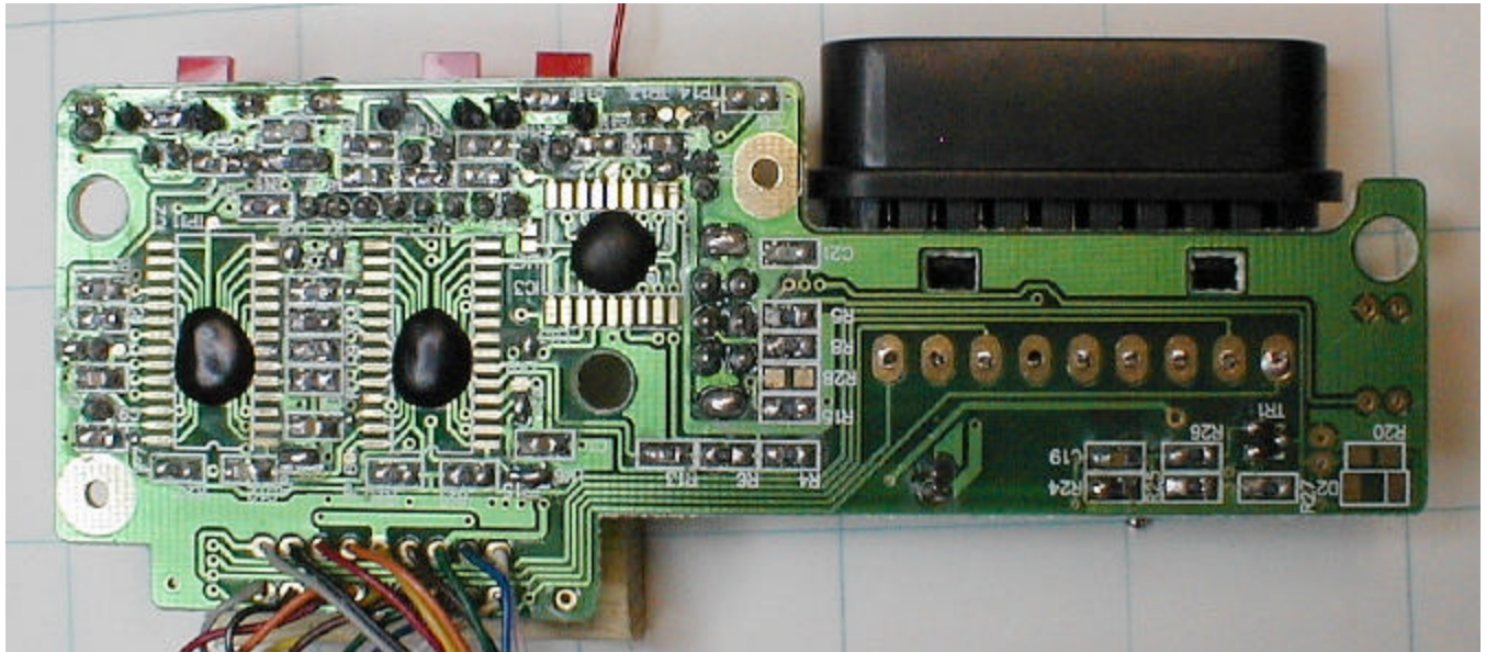
PCB Bottom View
