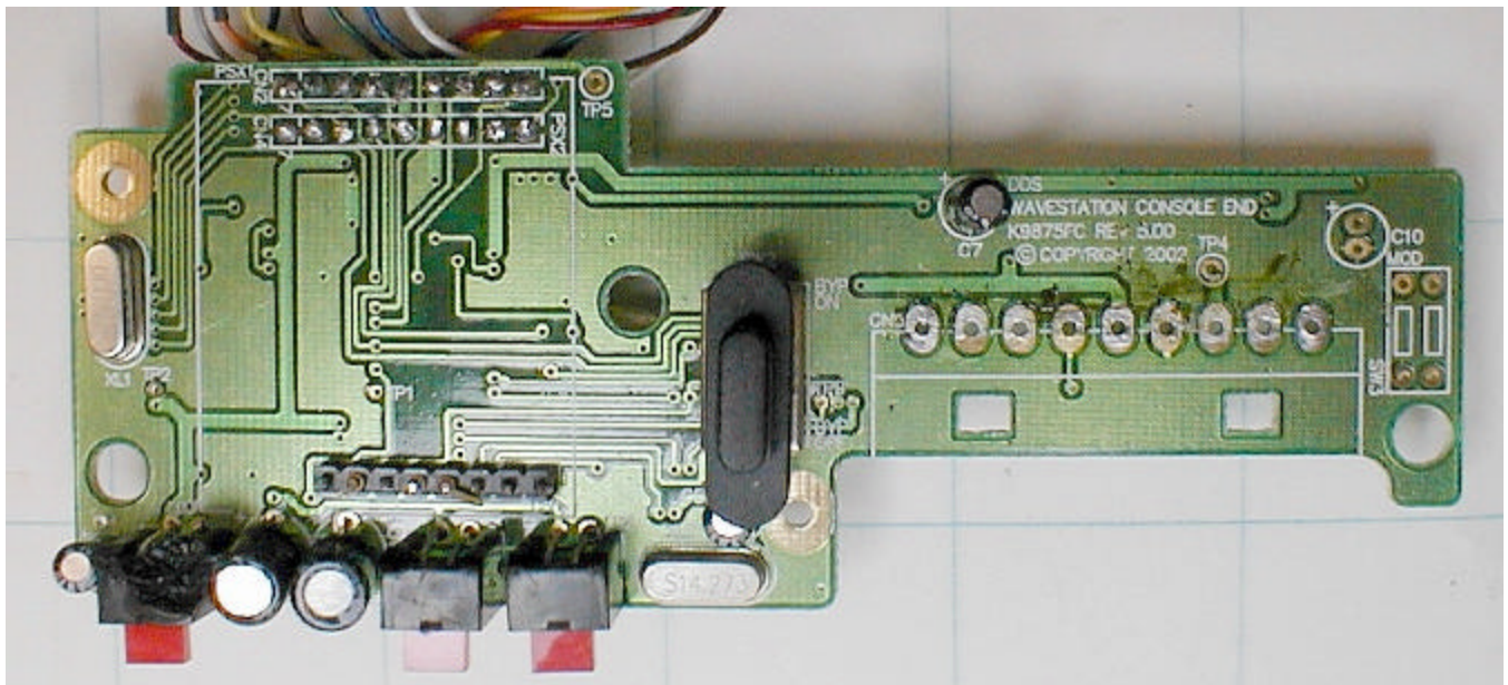
Main PCB without Radio Module and Port Connector
