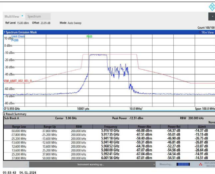
11AX20MIMO Ant1_5955_26Tone_RU0
