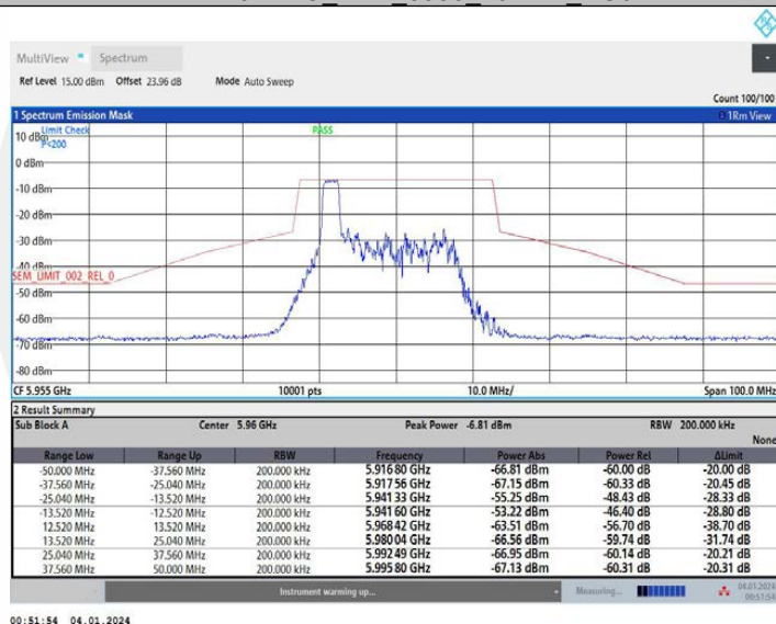
11AX20MIMO Ant1_5955_52Tone_RU37
