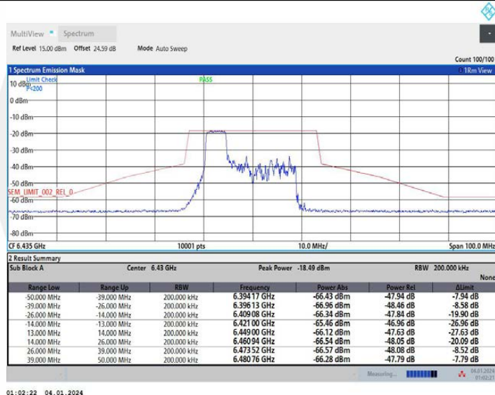
11AX20MIMO Ant2 6435 106Tone RU53
