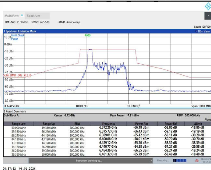
11AX20MIMO Ant1_6415_52Tone_RU37
