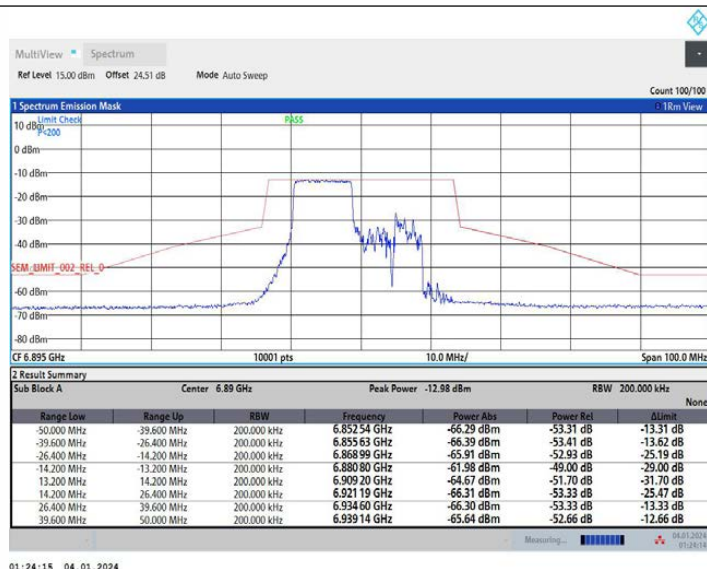
11AX20MIMO Ant1_6895_26Tone_RU0
