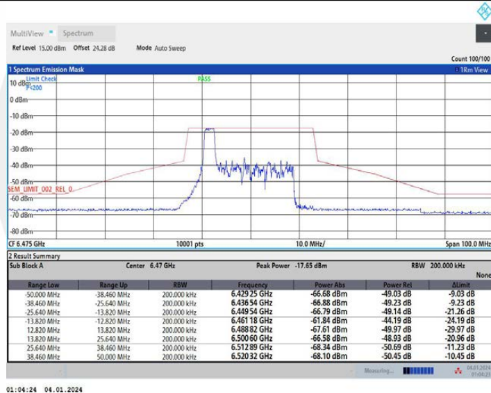
11AX20MIMO Ant1_6475_52Tone_RU37
