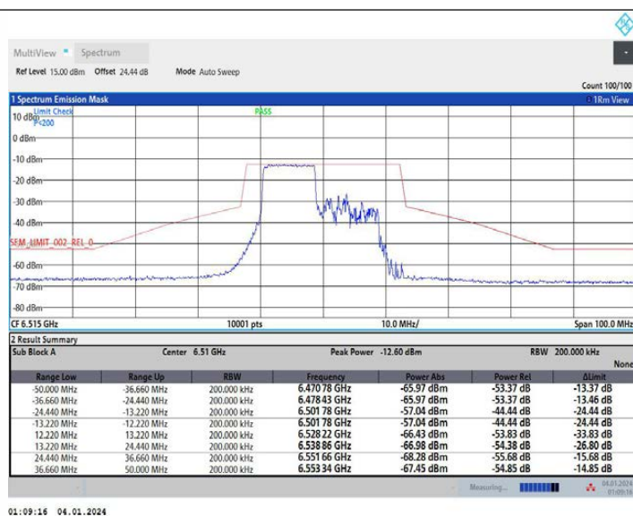
11AX20MIMO Ant1_6515_26Tone_RU0
