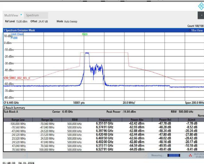
11AX40MIMO Ant2 6445 106Tone RU53
