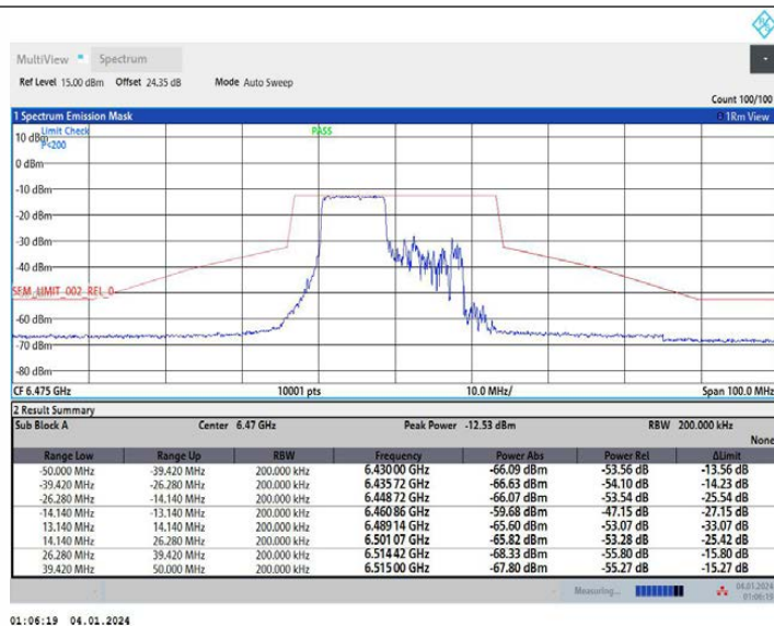
11AX20MIMO Ant1_6475_26Tone_RU0
