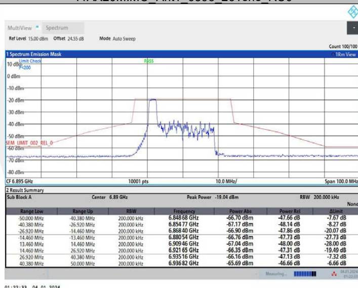
11AX20MIMO Ant1_6895_52Tone_RU37
