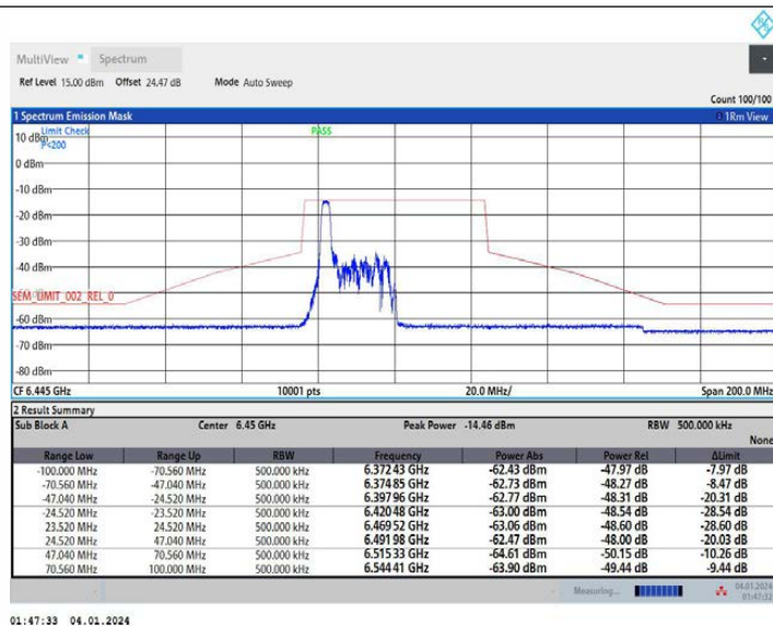
11AX40MIMO Ant2 6445 52Tone RU37
