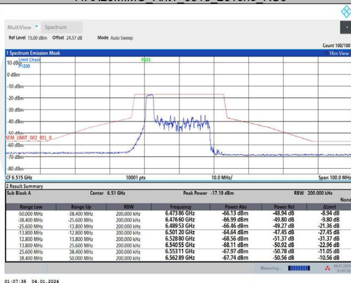
11AX20MIMO Ant1_6515_52Tone_RU37
