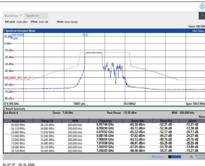
11AX20MIMO Ant1_6995_26Tone_RU0
