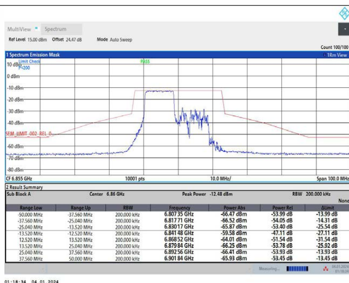
11AX20MIMO Ant1 6855_26Tone RU0
