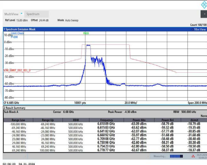
11AX40MIMO Ant2 6685 106Tone RU53
