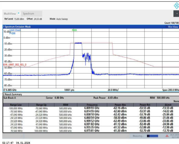
11AX40MIMO Ant2_6885_242Tone_RU61
