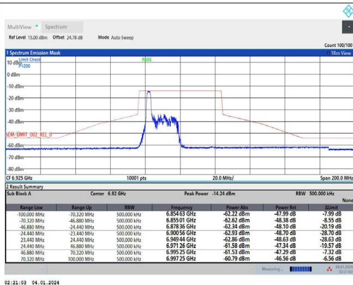
11AX40MIMO Ant2 6925 52Tone RU37
