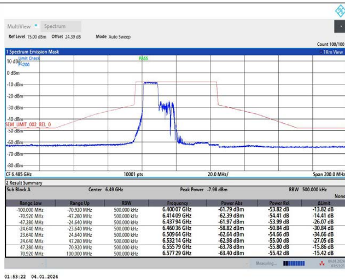
11AX40MIMO Ant2 6485_242Tone RU61
