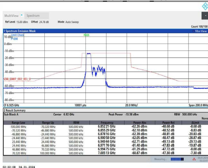
11AX40MIMO Ant2 6925 106Tone RU53
