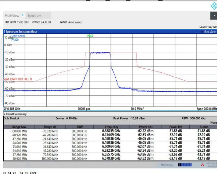
11AX40MIMO Ant1 6485_26Tone RU0
