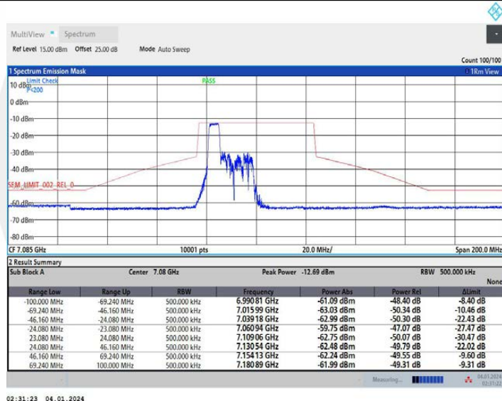
11AX40MIMO Ant2 7085 106Tone RU53
