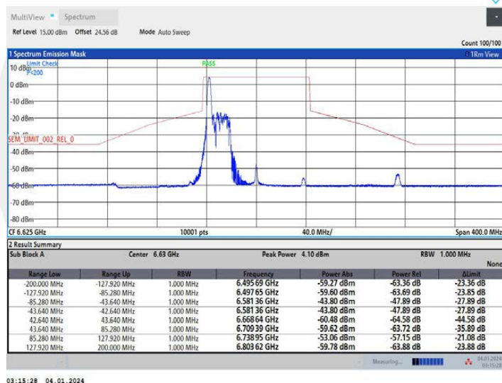
11AX80MIMO Ant1_6625_52Tone_RU37
