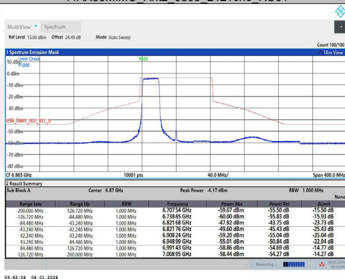
11AX80MIMO Ant2_6865_484Tone_RU65
