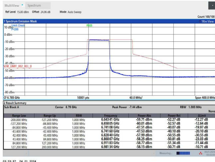
11AX80MIMO Ant1_6785_26Tone_RU0
