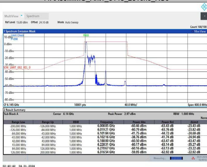
11AX80MIMO Ant1_6145_52Tone_RU37
