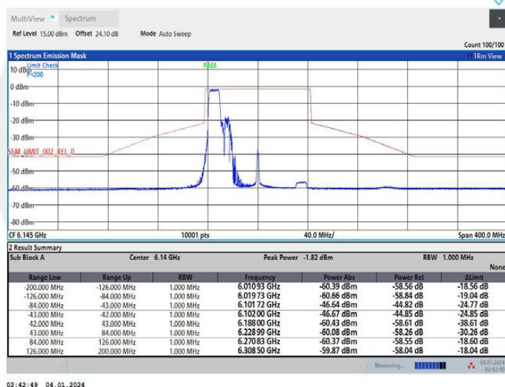
11AX80MIMO_Ant1_6145_242Tone_RU61
