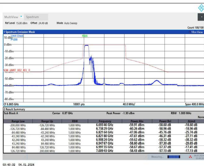
11AX80MIMO Ant2_6865_242Tone_RU61
