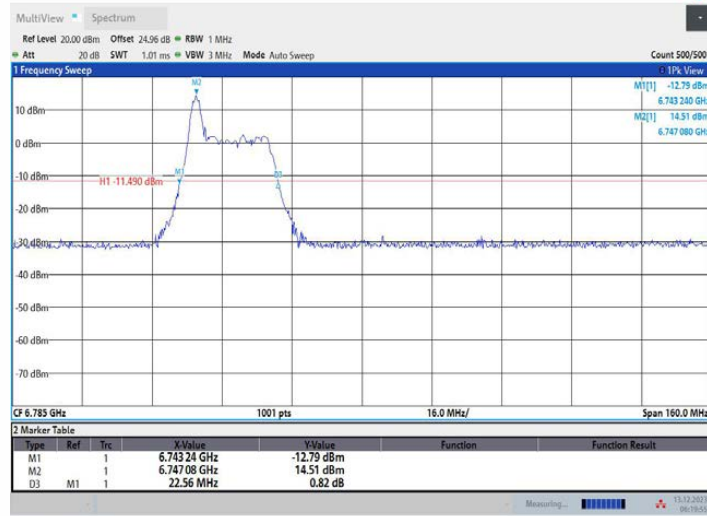
11AX80MIMO Ant2 6785 52Tone RU37
