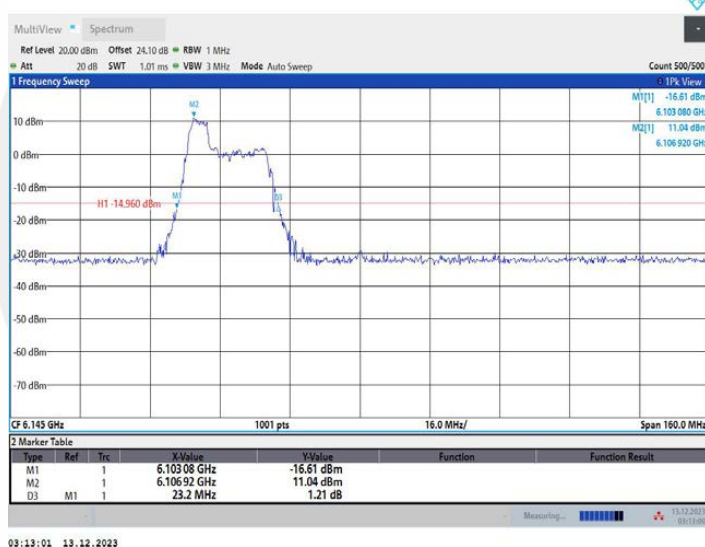
11AX80MIMO Ant2 6145 106Tone RU53
