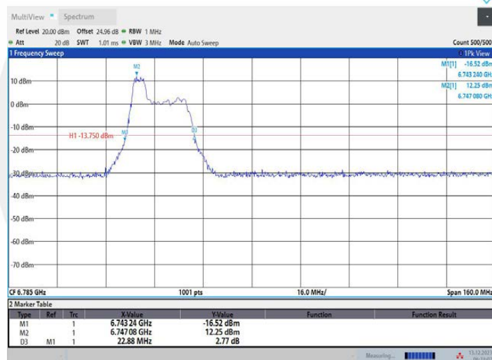
11AX80MIMO Ant2 6785 106Tone RU53
