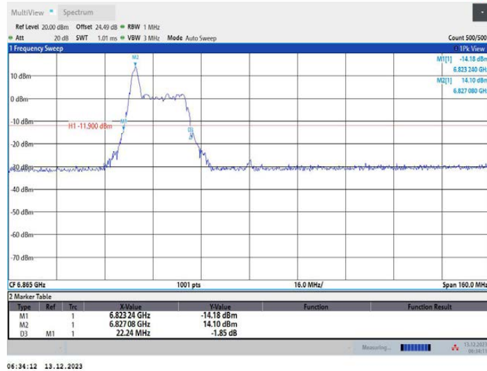
11AX80MIMO Ant2 6865 52Tone RU37
