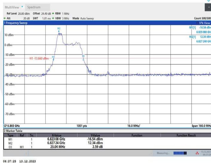
11AX80MIMO Ant2 6865 106Tone RU53
