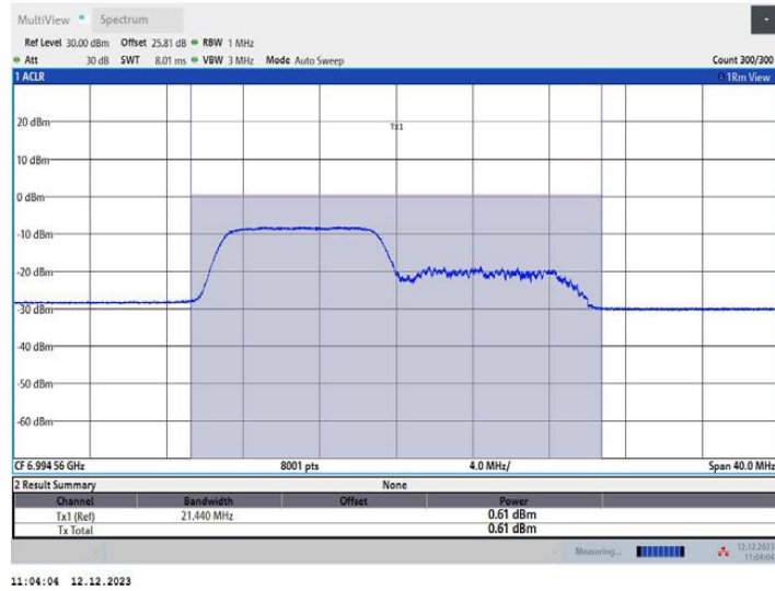
11AX20MIMO Ant1_6995_26Tone_RU0
