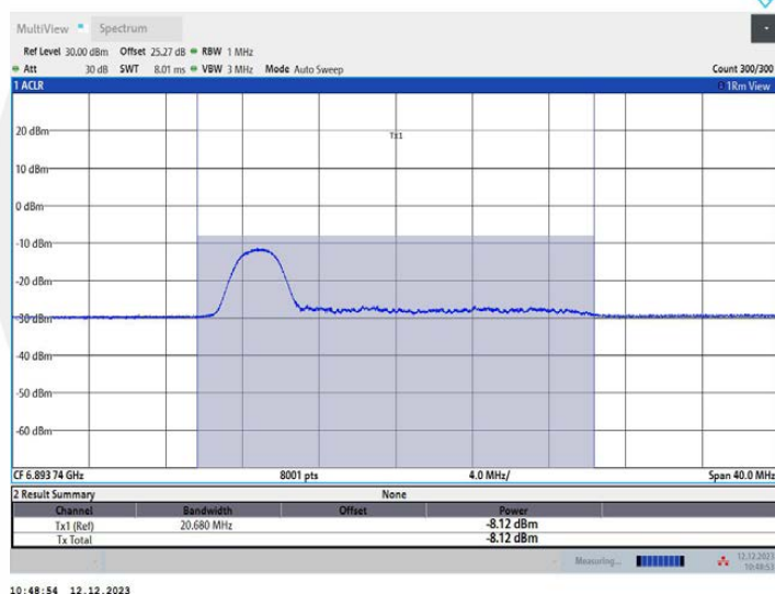
11AX20MIMO Ant1_6895_52Tone_RU37
