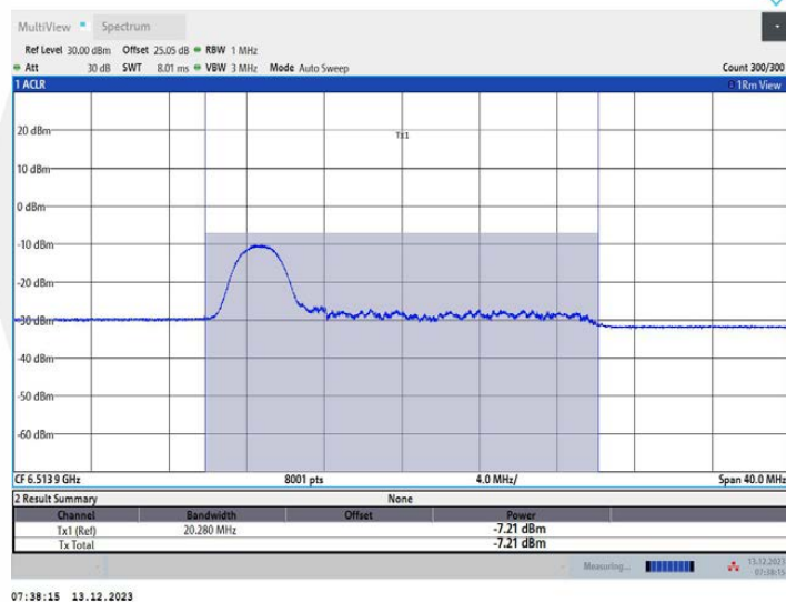
11AX20MIMO Ant1_6515_52Tone_RU37
