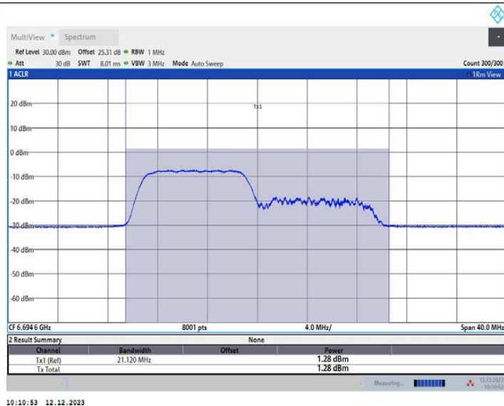
11AX20MIMO Ant1_6695_26Tone_RU0
