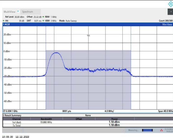
11AX20MIMO Ant1_6695_52Tone_RU37
