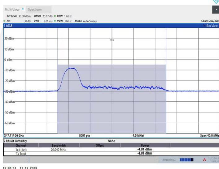
11AX20MIMO Ant1_7115_52Tone_RU37
