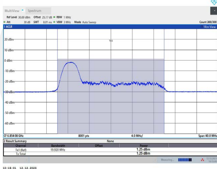
11AX20MIMO Ant1_6855_52Tone_RU37
