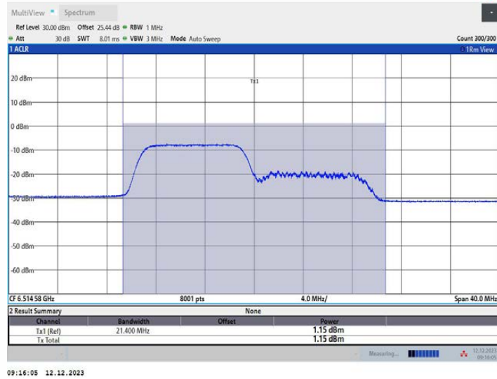
11AX20MIMO Ant1_6515_26Tone_RU0
