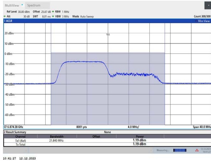
11AX20MIMO Ant1_6875_26Tone_RU0
