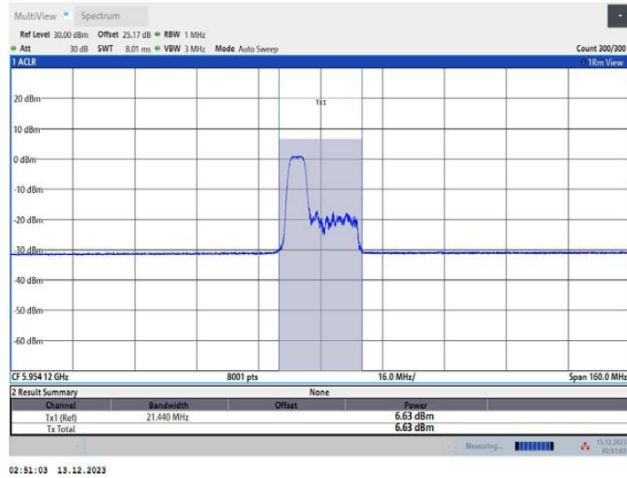
11AX80MIMO Ant1_5985_106Tone_RU53
