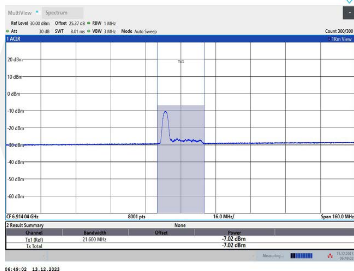
11AX80MIMO Ant1_6945_52Tone_RU37
