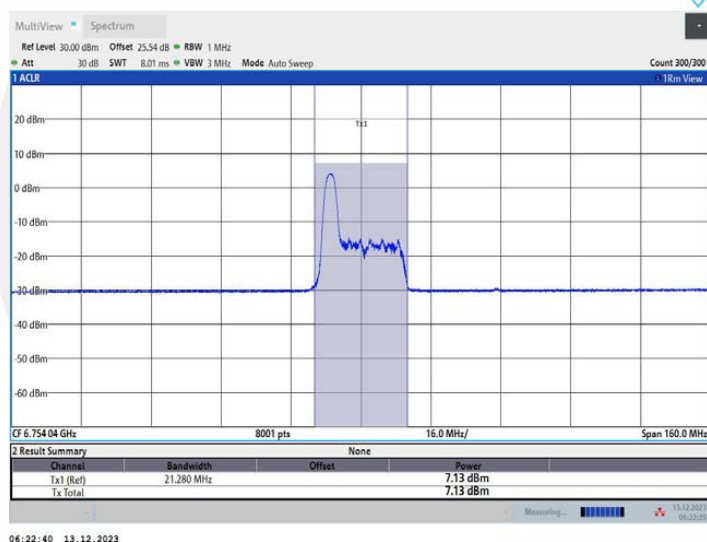
11AX80MIMO Ant1_6785_52Tone_RU37
