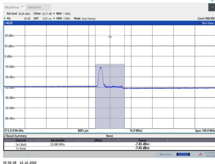
11AX80MIMO Ant1_6545_52Tone_RU37
