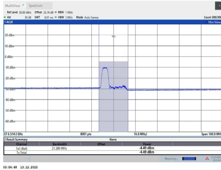
11AX80MIMO_Ant1_6545_106Tone_RU53
