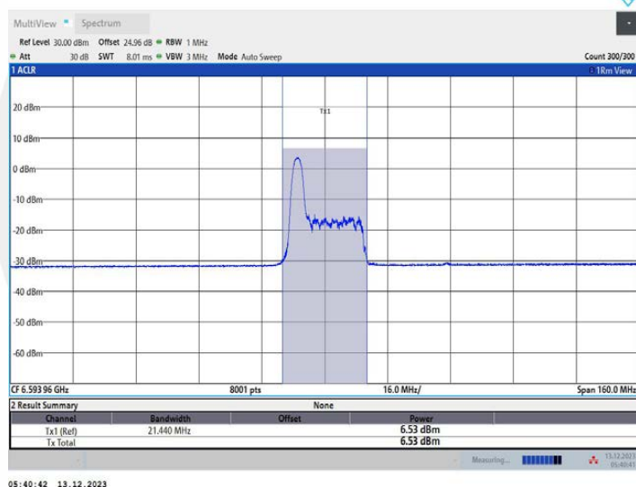
11AX80MIMO Ant1_6625_52Tone_RU37
