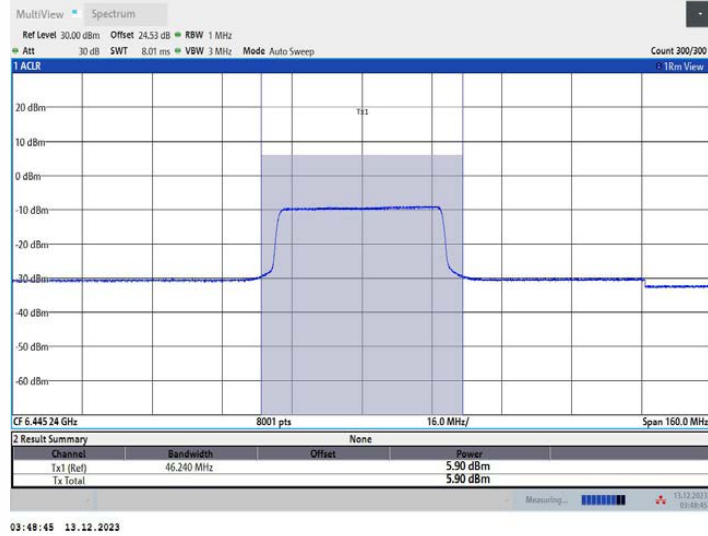
11AX80MIMO Ant1_6465_26Tone_RU0
