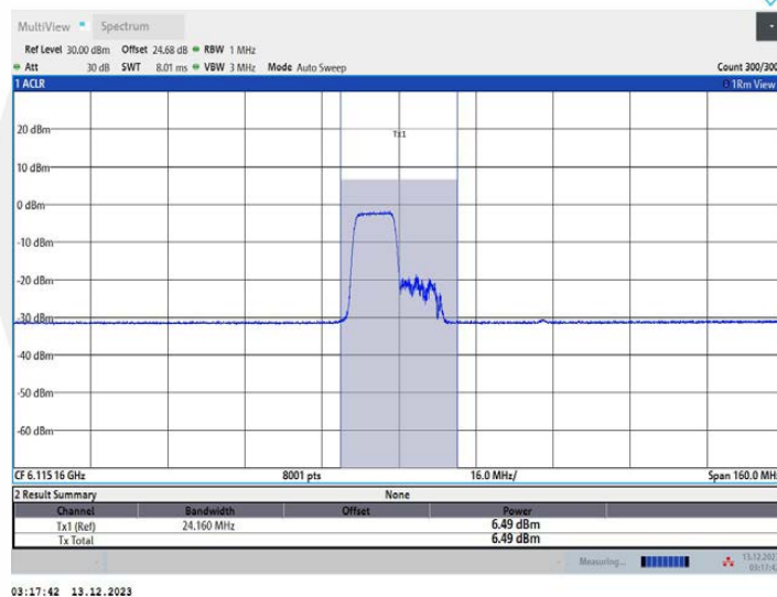
11AX80MIMO_Ant1_6145_242Tone_RU61
