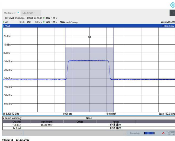
11AX80MIMO Ant1_6145_26Tone_RU0
