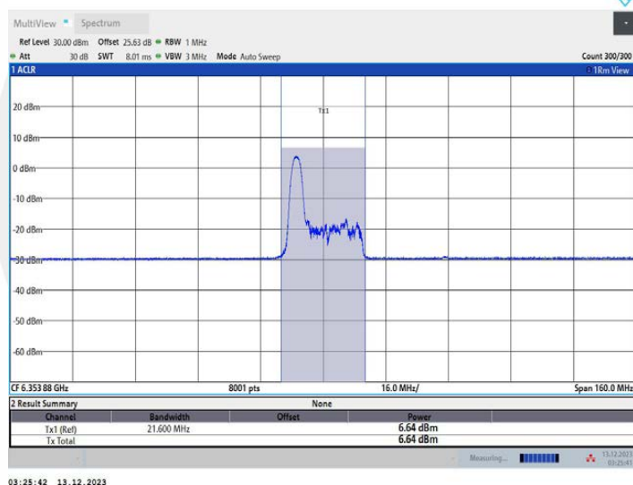
11AX80MIMO Ant1_6385_52Tone_RU37
