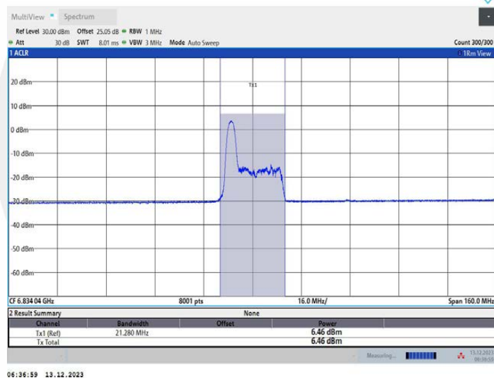
11AX80MIMO Ant1_6865_52Tone_RU37
