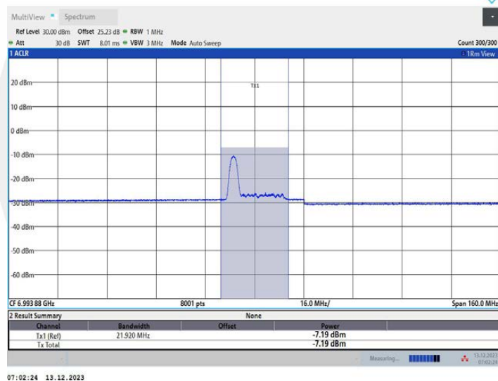
11AX80MIMO Ant1_7025_52Tone_RU37
