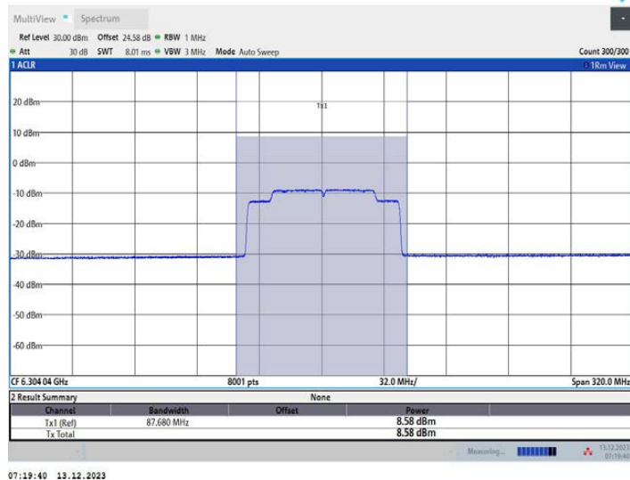
11AX160MIMO_Ant1_6345_996Tone_RU67
