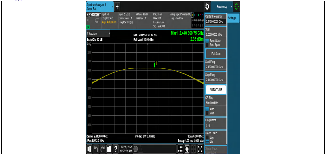
BLE_2M-2440-PASS
