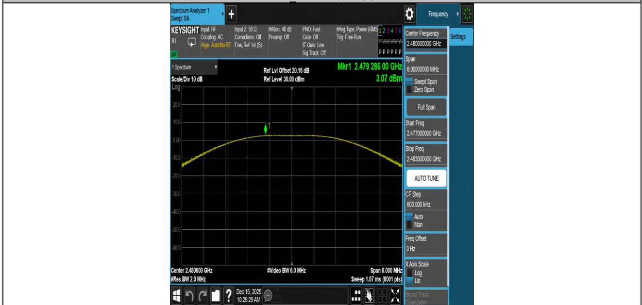
BLE_2M-2480-PASS
