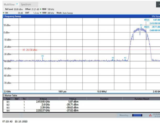
11B_Ant2_Low_2412
