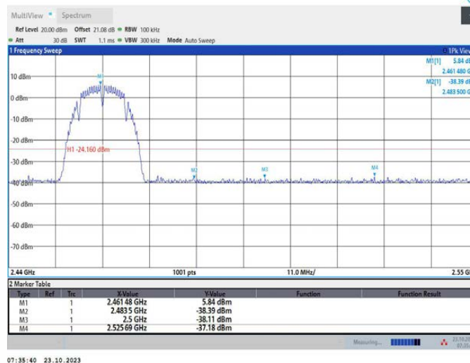
11B_Ant1_High_2462
