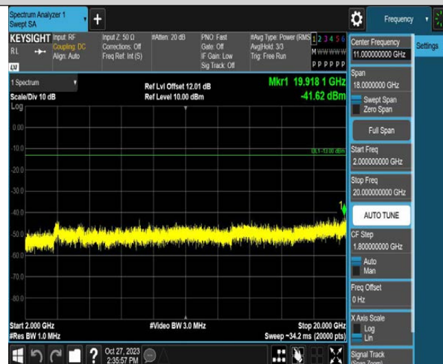
Band2-20MHz-64QAM-19100-1RB#0-Range3:2000~20000MHz
