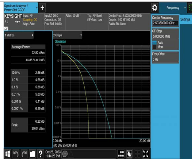
Band41-15MHz-QPSK-40620-75RB#0
