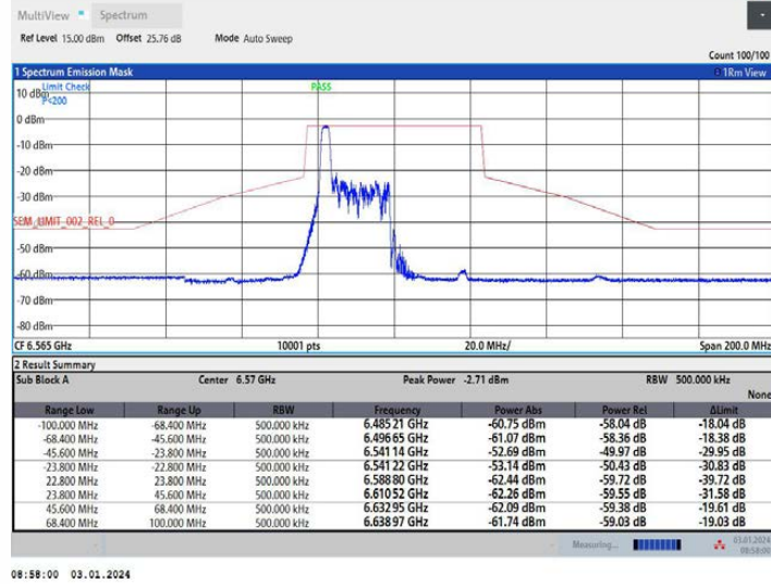
11AX40MIMO Ant2 6565 52Tone RU37
