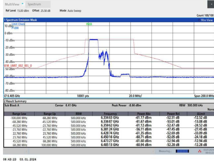
11AX40MIMO Ant2 6405 242Tone RU61
