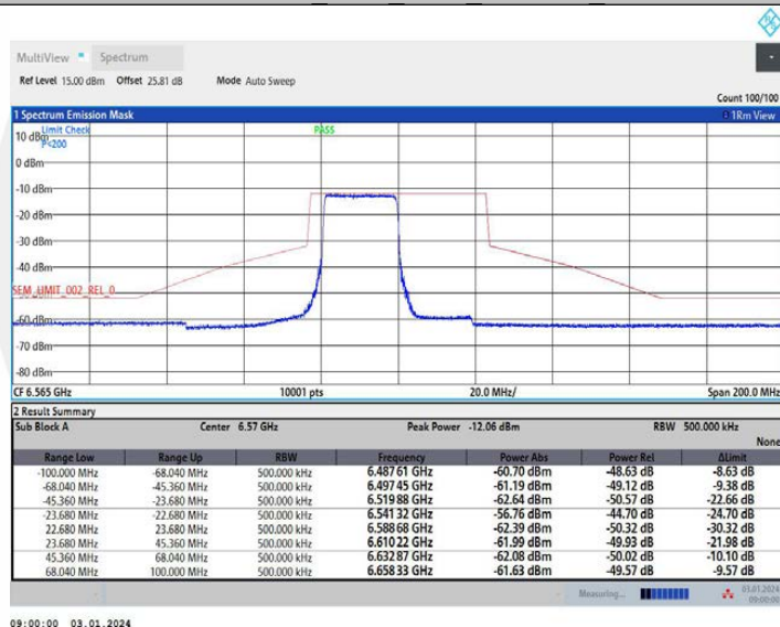
11AX40MIMO Ant2 6565 26Tone RU0
