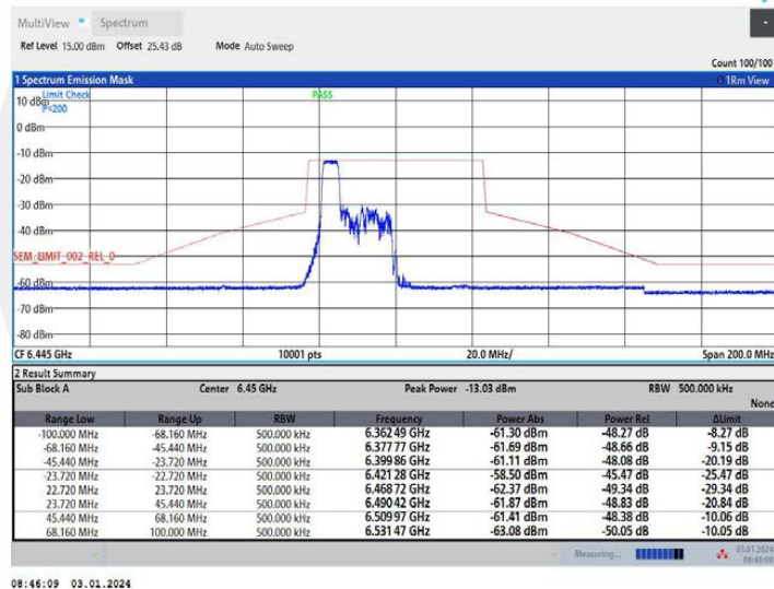
11AX40MIMO Ant2 6445 106Tone RU53
