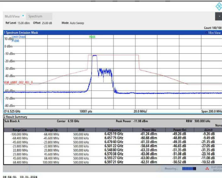
11AX40MIMO Ant2 6525 106Tone RU53
