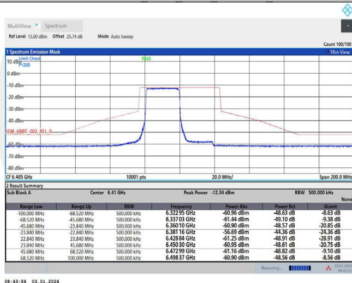
11AX40MIMO Ant2 6405 26Tone RU0
