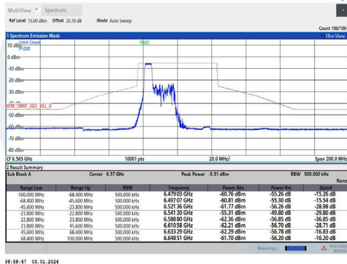
11AX40MIMO Ant2 6565 106Tone RU53
