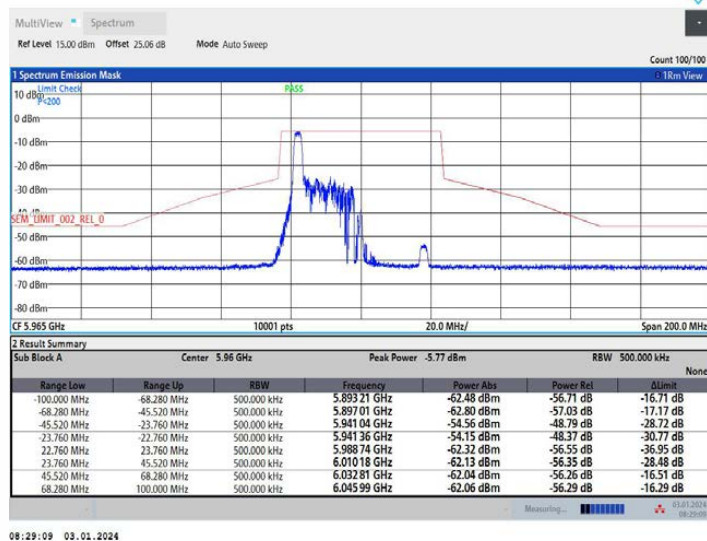
11AX40MIMO Ant2 5965 52Tone RU37
