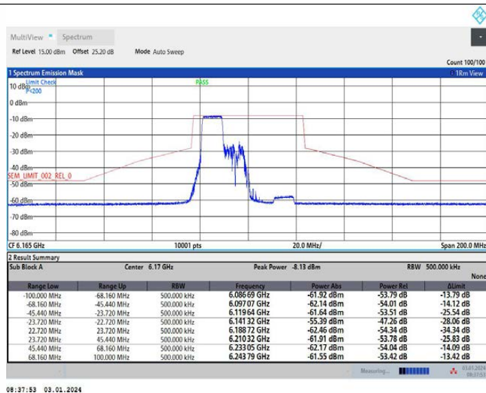
11AX40MIMO Ant2 6165 242Tone RU61
