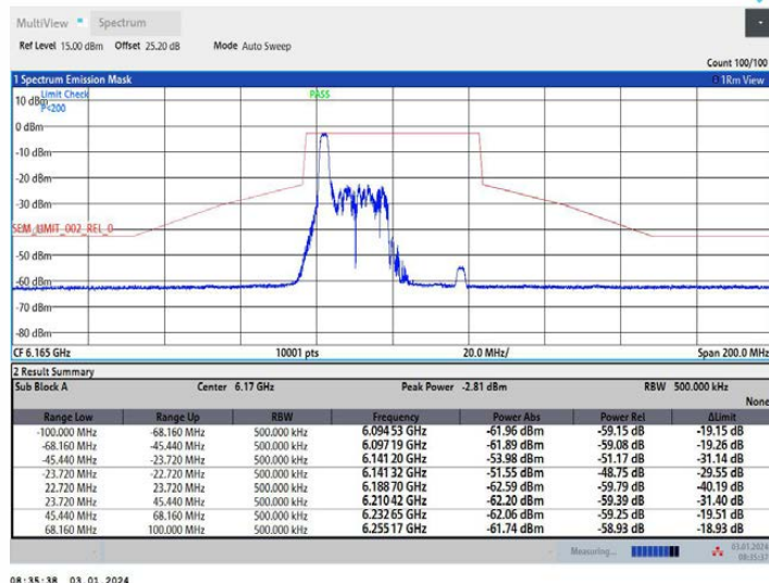
11AX40MIMO Ant2 6165 52Tone RU37
