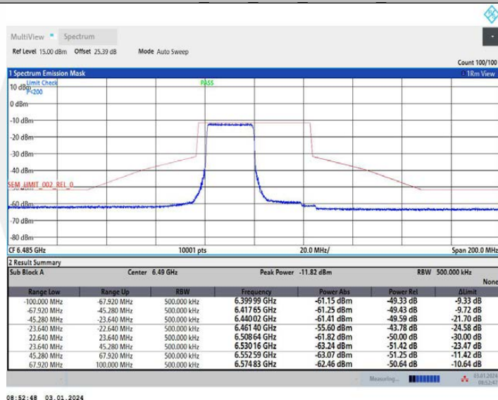
11AX40MIMO Ant2 6485 26Tone RU0
