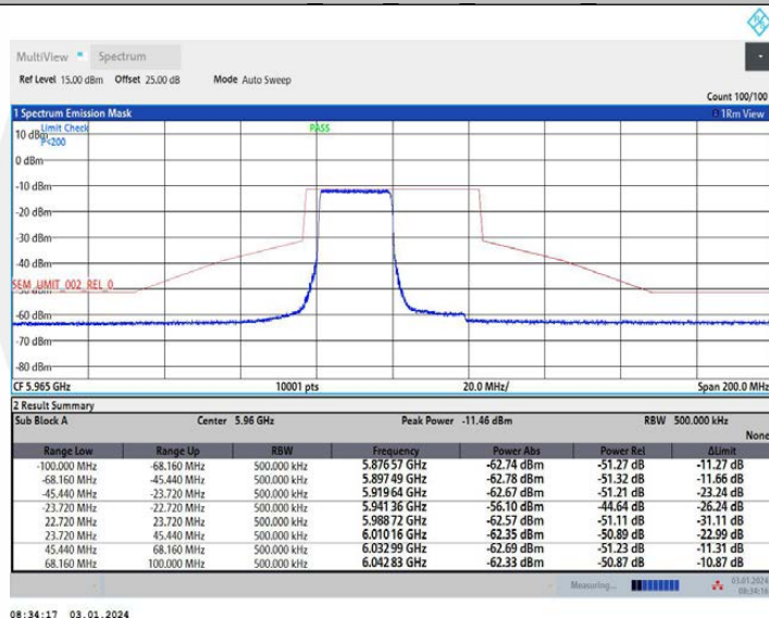
11AX40MIMO Ant2 5965 26Tone RU0
