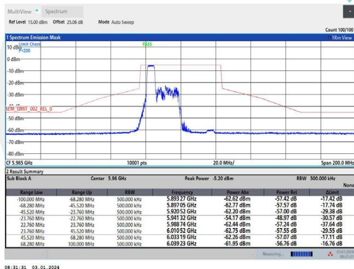
11AX40MIMO Ant2 5965 106Tone RU53
