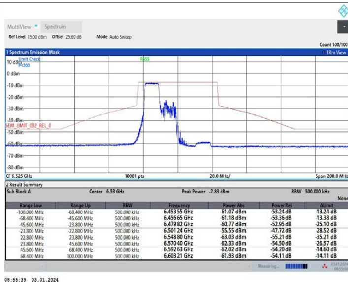
11AX40MIMO Ant2 6525 242Tone RU61
