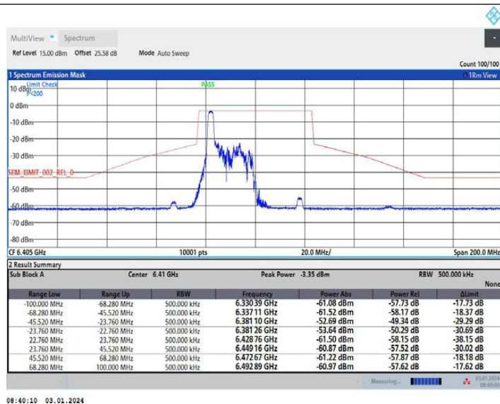
11AX40MIMO Ant2 6405 52Tone RU37
