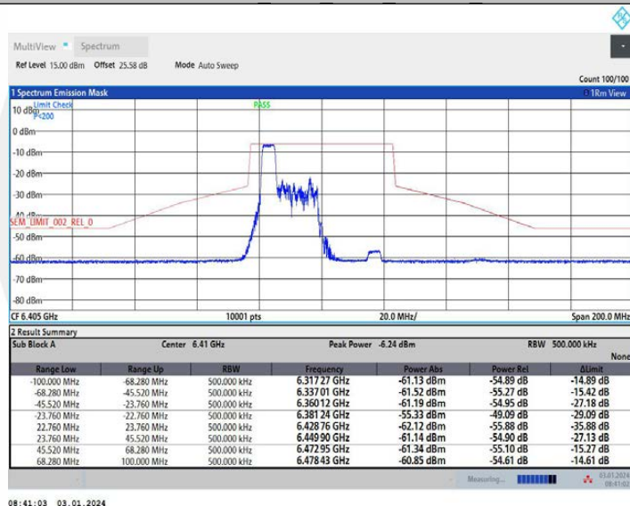
11AX40MIMO Ant2 6405 106Tone RU53
