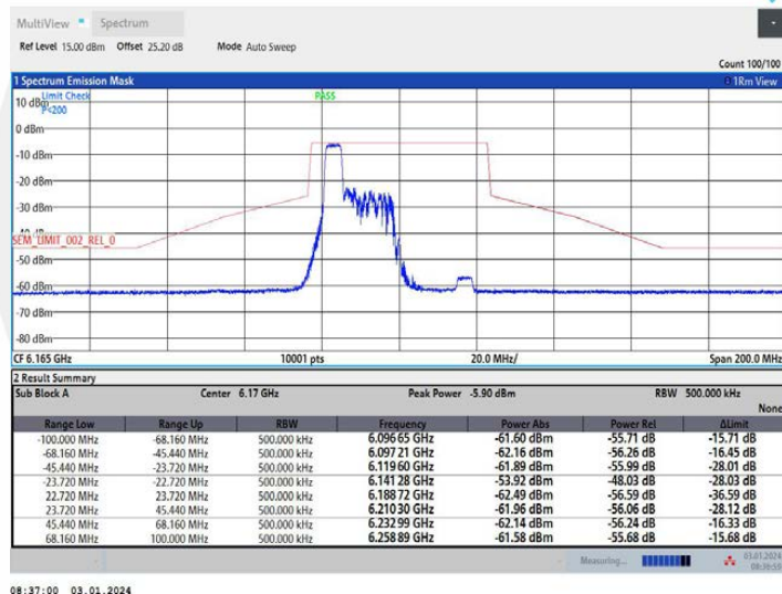
11AX40MIMO Ant2 6165 106Tone RU53
