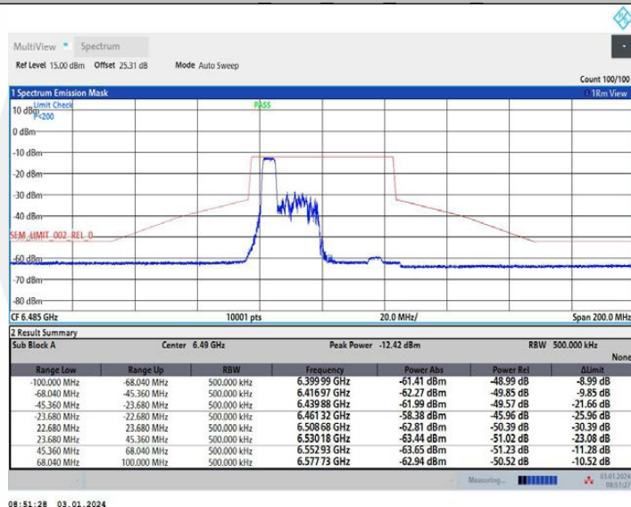
11AX40MIMO Ant2 6485 106Tone RU53
