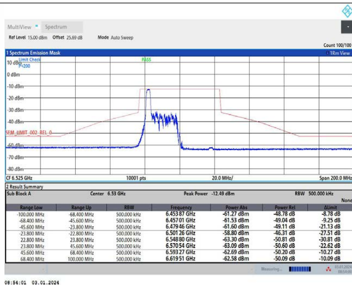
11AX40MIMO Ant2 6525 52Tone RU37
