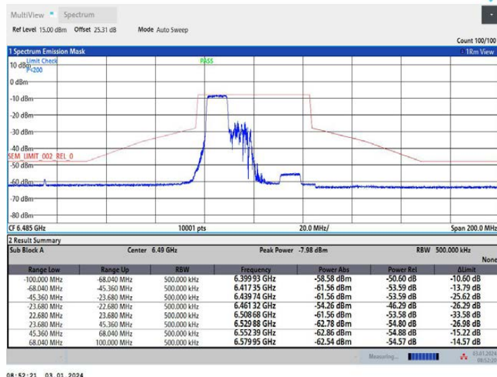
11AX40MIMO Ant2 6485 242Tone RU61
