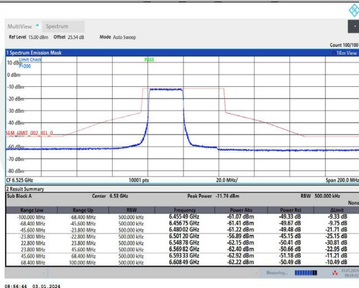
11AX40MIMO Ant2 6525 26Tone RU0
