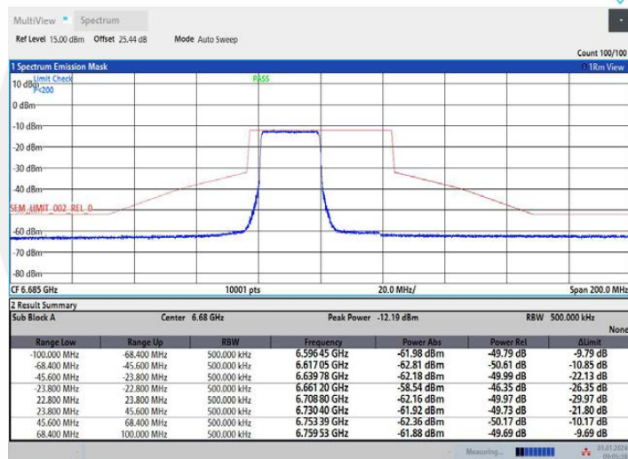
11AX40MIMO Ant2 6685 26Tone RU0
