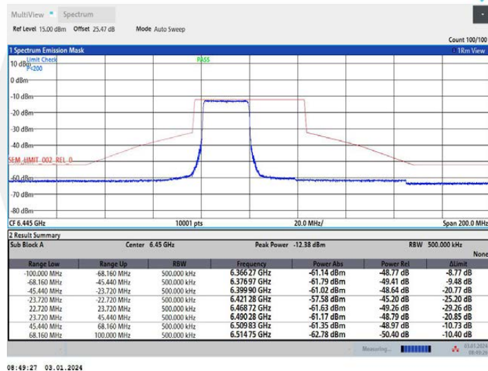
11AX40MIMO Ant2 6445 26Tone RU0
