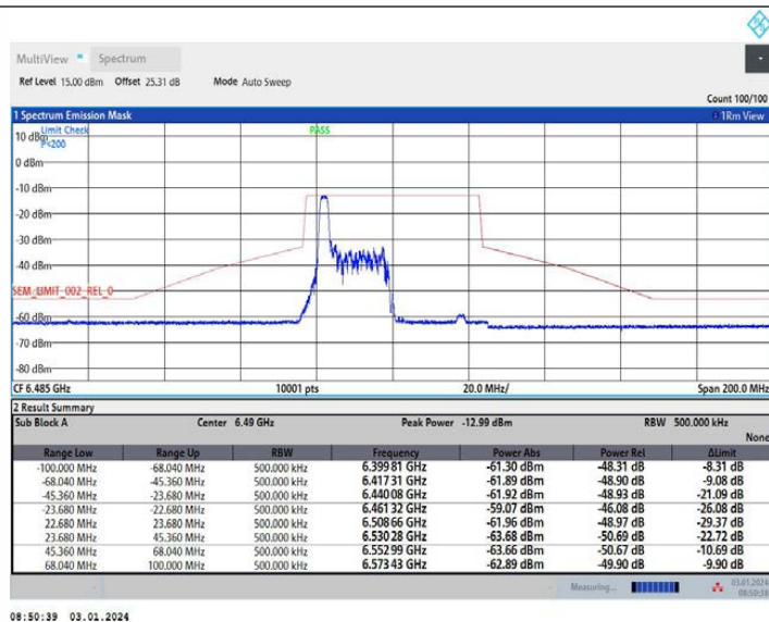
11AX40MIMO Ant2 6485 52Tone RU37
