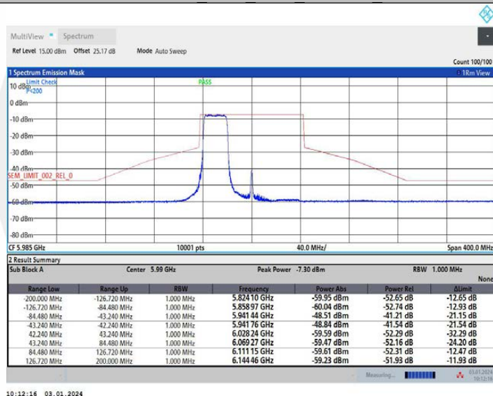
11AX80MIMO Ant1 5985 484Tone RU65
