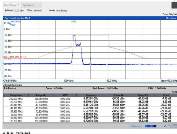
11AX80MIMO Ant1 6545 106Tone RU53
