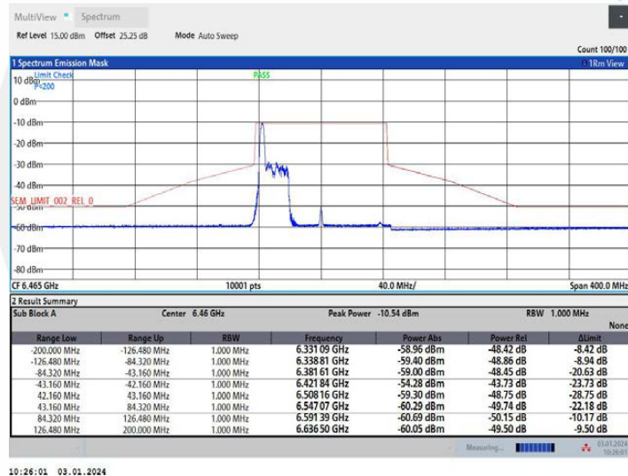
11AX80MIMO Ant2 6465 52Tone RU37
