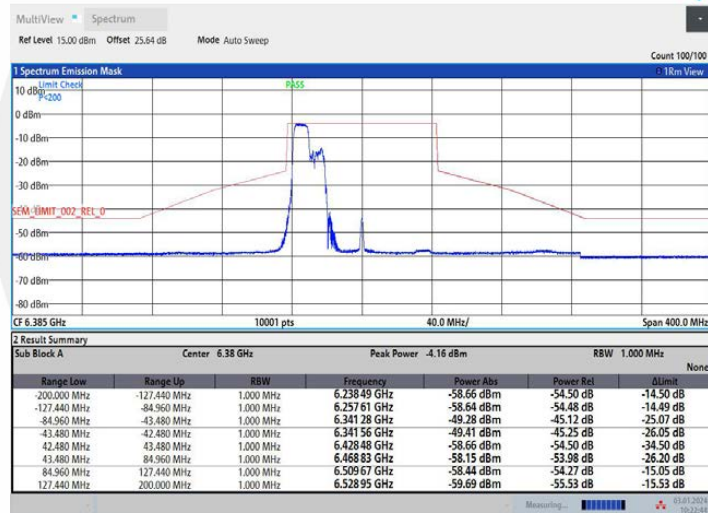
11AX80MIMO Ant2 6385 242Tone RU61
