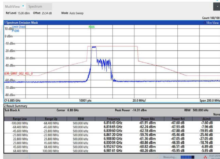
11AX40MIMO Ant2 6885 106Tone RU53
