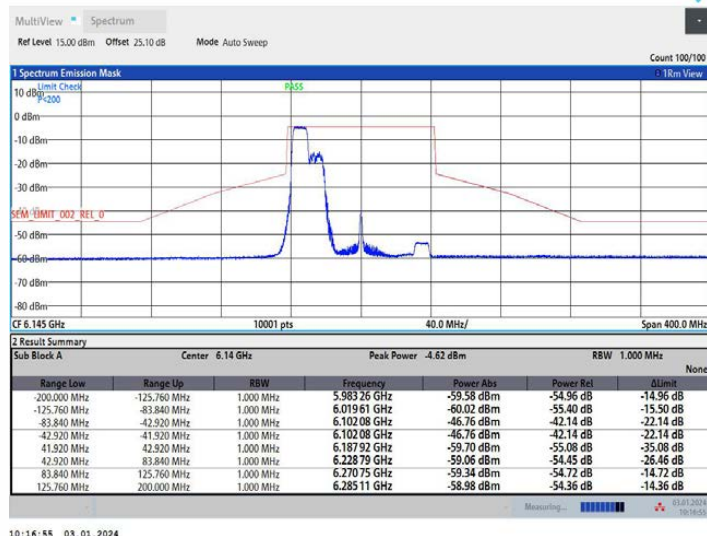
11AX80MIMO Ant1 6145 242Tone RU61
