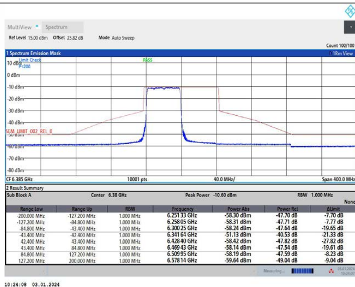
11AX80MIMO Ant2 6385 26Tone RU0
