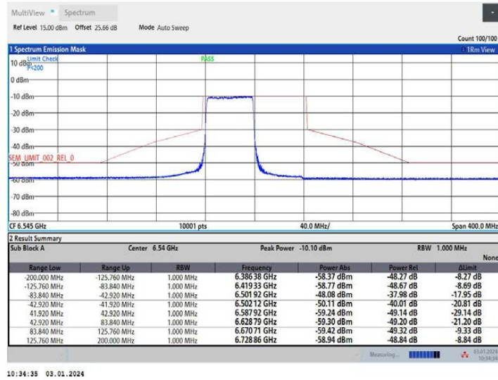
11AX80MIMO Ant2 6545 26Tone RU0
