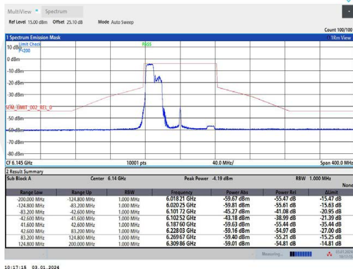
11AX80MIMO Ant2 6145 242Tone RU61
