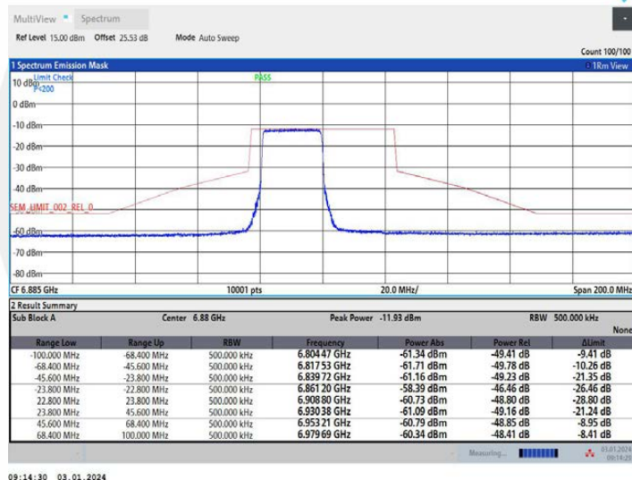
11AX40MIMO Ant2 6885 26Tone RU0
