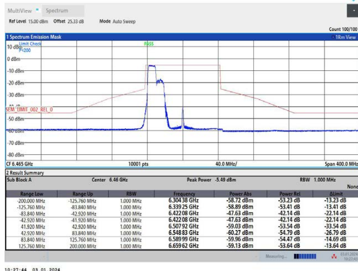
11AX80MIMO Ant1 6465 242Tone RU61
