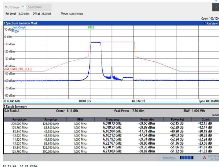
11AX80MIMO Ant1 6145 484Tone RU65
