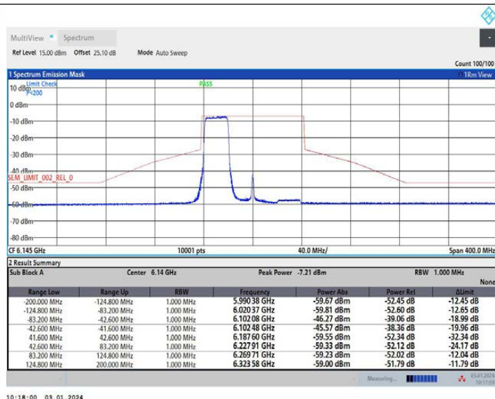
11AX80MIMO Ant2 6145 484Tone RU65
