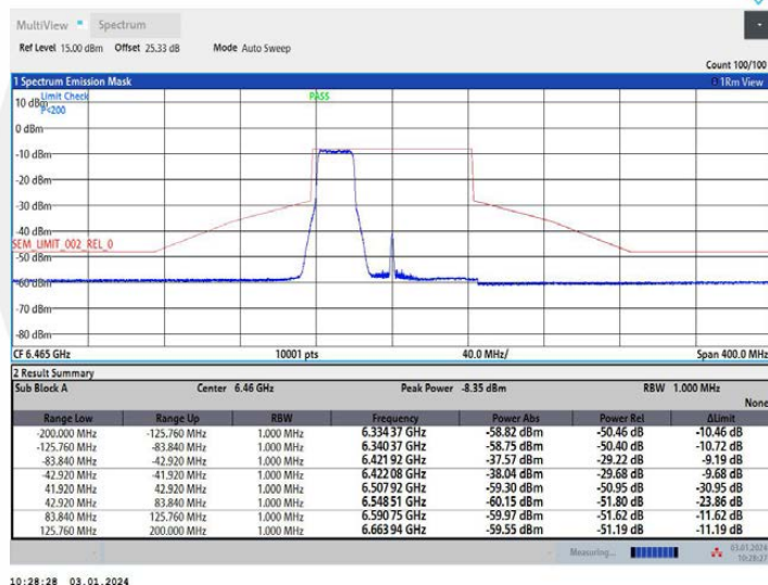
11AX80MIMO Ant1 6465 484Tone RU65
