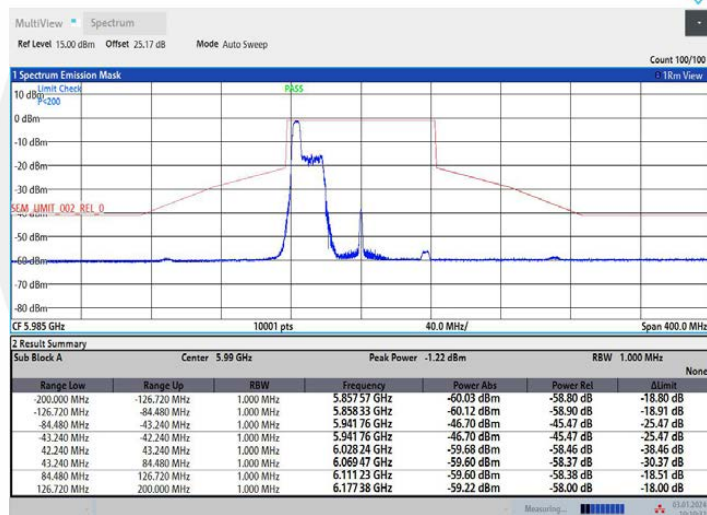
11AX80MIMO Ant1 5985 106Tone RU53
