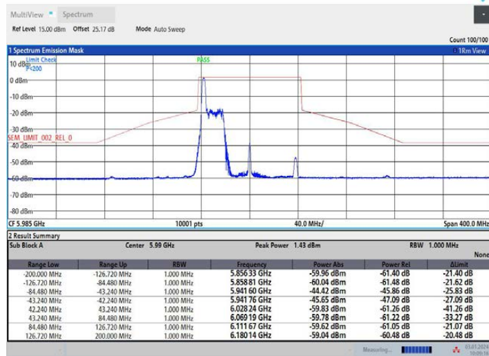
11AX80MIMO Ant1 5985 52Tone RU37
