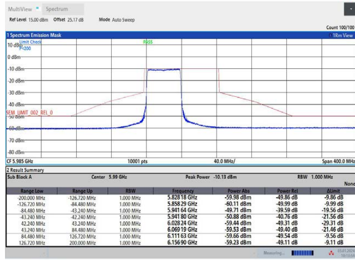
11AX80MIMO Ant2 5985 26Tone RU0
