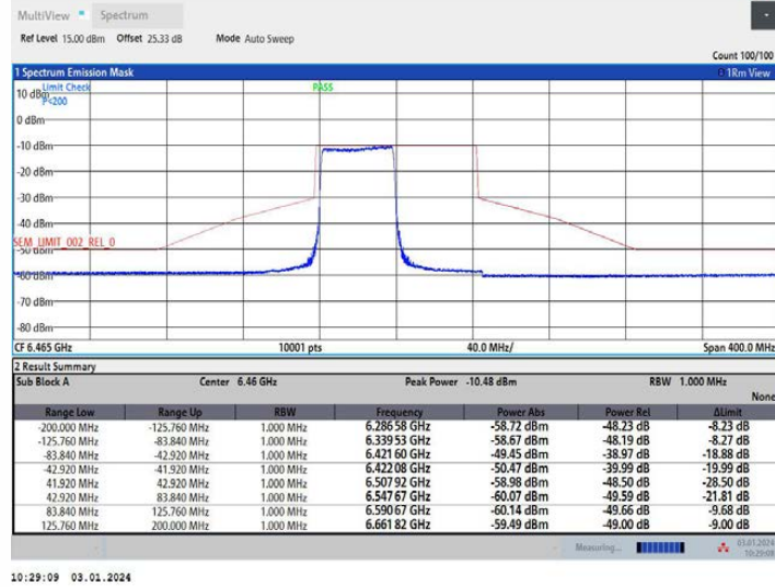
11AX80MIMO Ant2 6465 26Tone RU0
