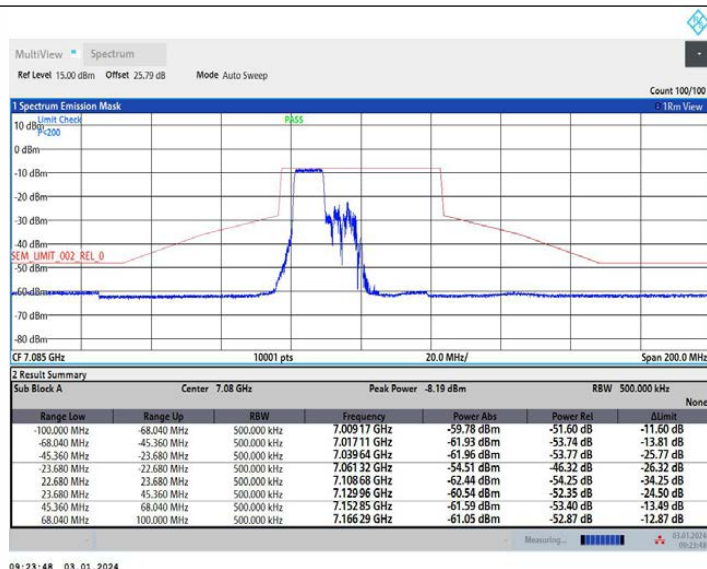
11AX40MIMO Ant2 7085 242Tone RU61
