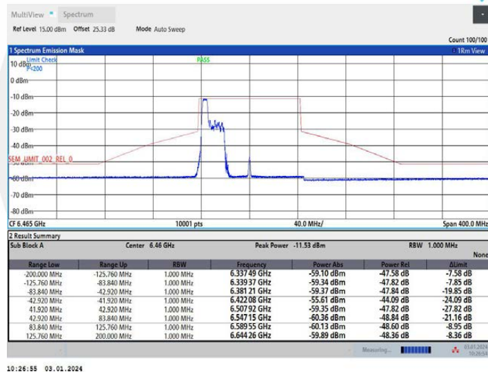
11AX80MIMO Ant1 6465 106Tone RU53
