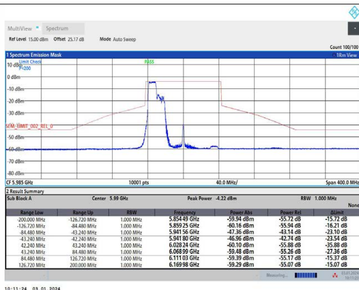
11AX80MIMO Ant1 5985 242Tone RU61
