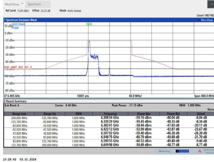
11AX80MIMO Ant1 6465 52Tone RU37
