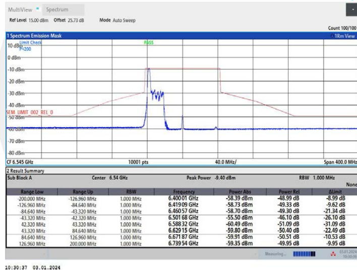
11AX80MIMO Ant2 6545 52Tone RU37
