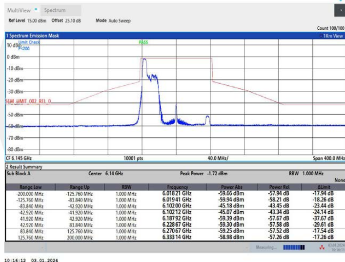
11AX80MIMO Ant1 6145 106Tone RU53
