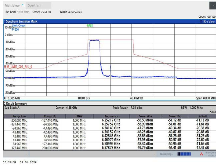
11AX80MIMO Ant2 6385 484Tone RU65
