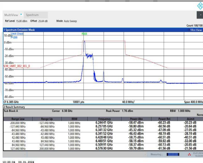
11AX80MIMO Ant2 6385 52Tone RU37
