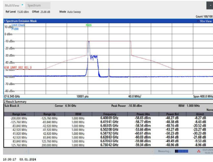
11AX80MIMO Ant1 6545 52Tone RU37
