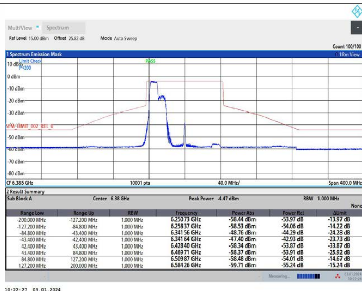
11AX80MIMO Ant1 6385 242Tone RU61
