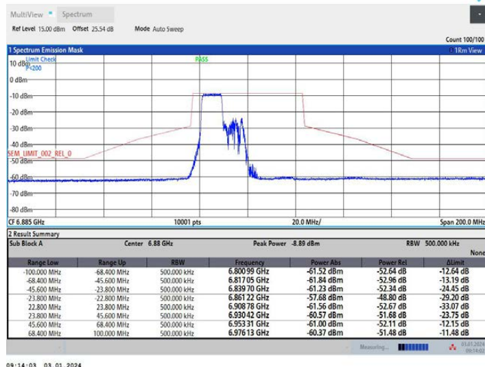
11AX40MIMO Ant2 6885 242Tone RU61
