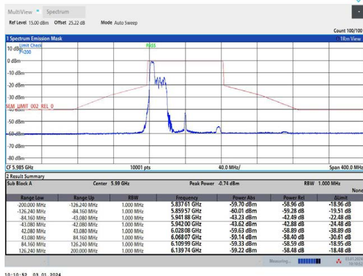
11AX80MIMO Ant2 5985 106Tone RU53
