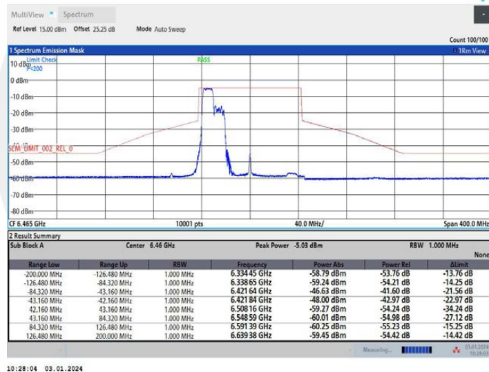
11AX80MIMO Ant2 6465 242Tone RU61
