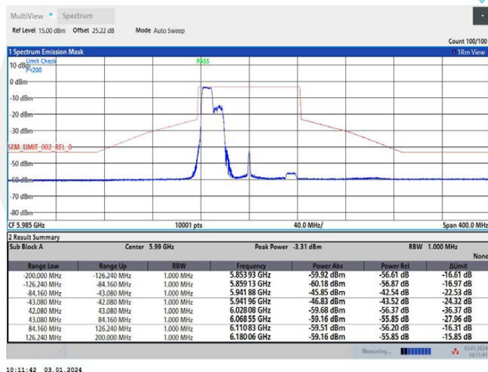
11AX80MIMO Ant2 5985 242Tone RU61
