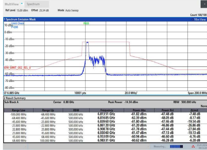
11AX40MIMO Ant2 6885 52Tone RU37
