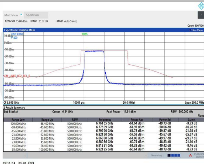
11AX40MIMO Ant2 6845 26Tone RU0
