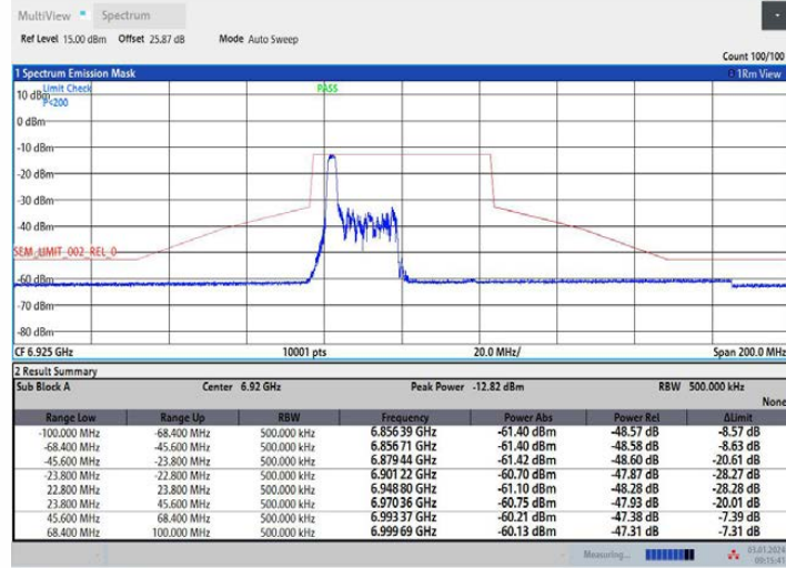
11AX40MIMO Ant2 6925 52Tone RU37
