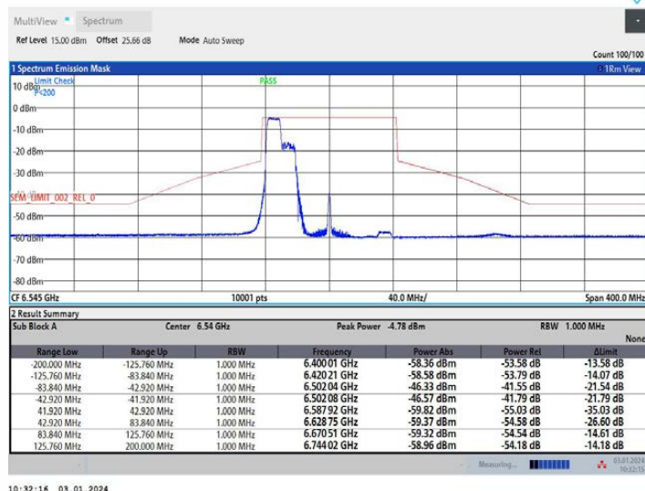
11AX80MIMO Ant1 6545 242Tone RU61
