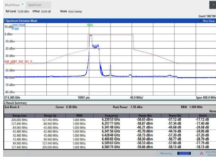
11AX80MIMO Ant2 6385 106Tone RU53
