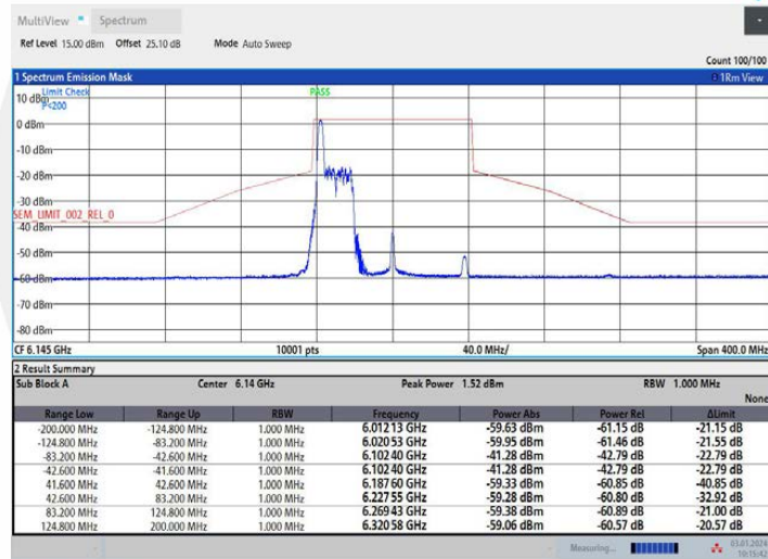
11AX80MIMO Ant2 6145 52Tone RU37
