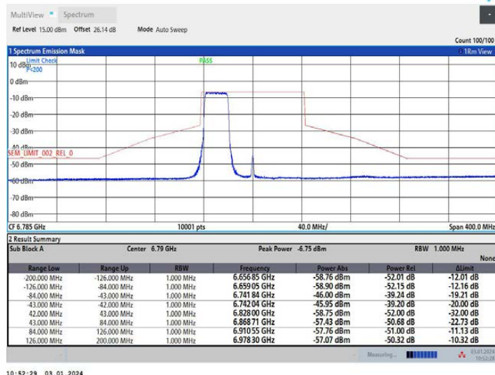
11AX80MIMO Ant2 6785 484Tone RU65
