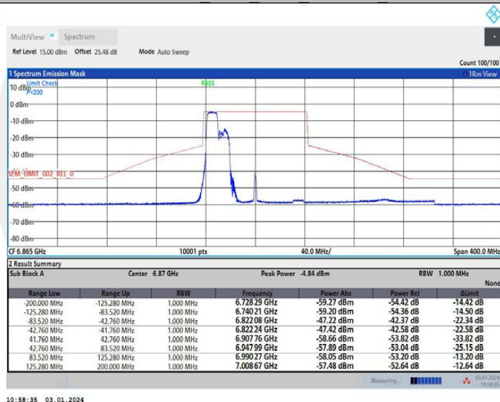
11AX80MIMO Ant2 6865 242Tone RU61
