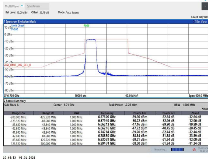
11AX80MIMO Ant1 6705 484Tone RU65
