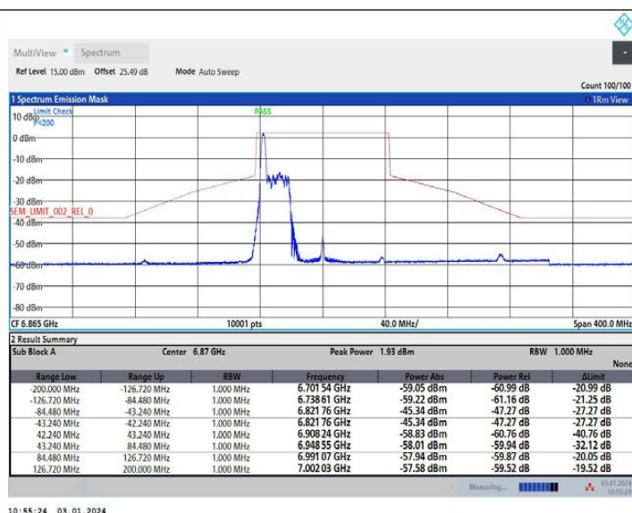
11AX80MIMO Ant1 6865 52Tone RU37
