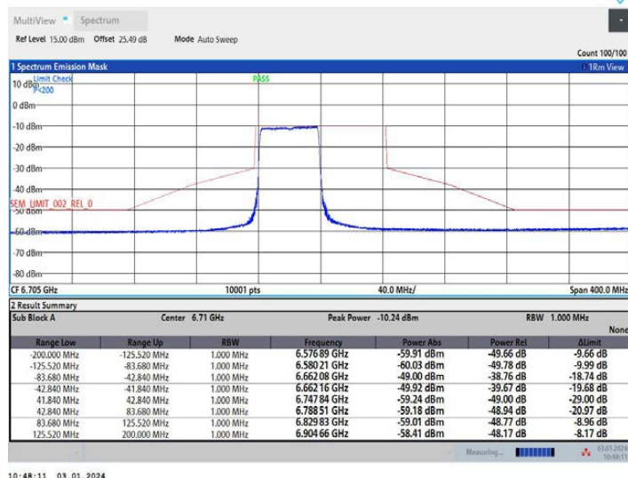
11AX80MIMO Ant2 6705 26Tone RU0
