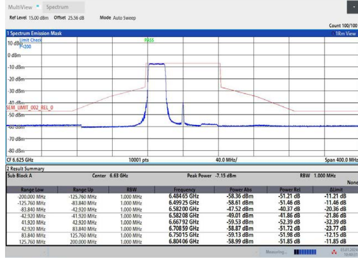
11AX80MIMO Ant2 6625 484Tone RU65
