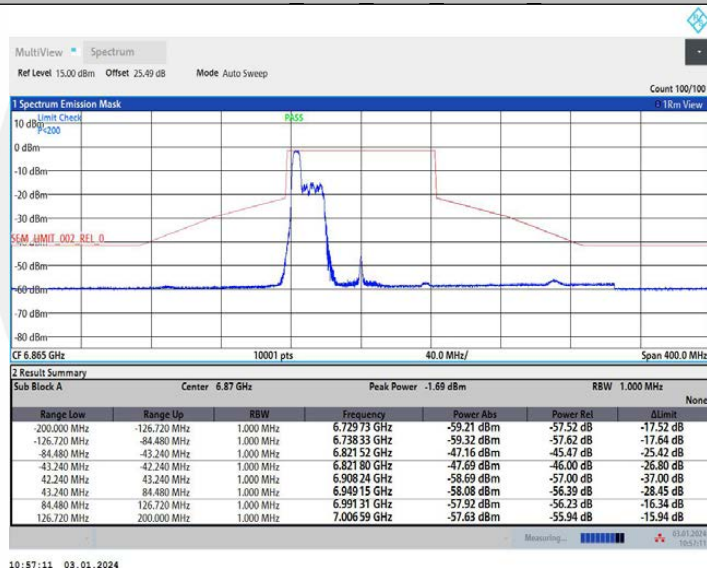
11AX80MIMO Ant1 6865 106Tone RU53
