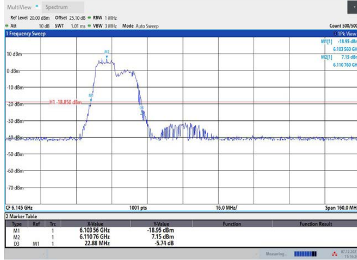
11AX80MIMO_Ant1_6145_242Tone_RU61
