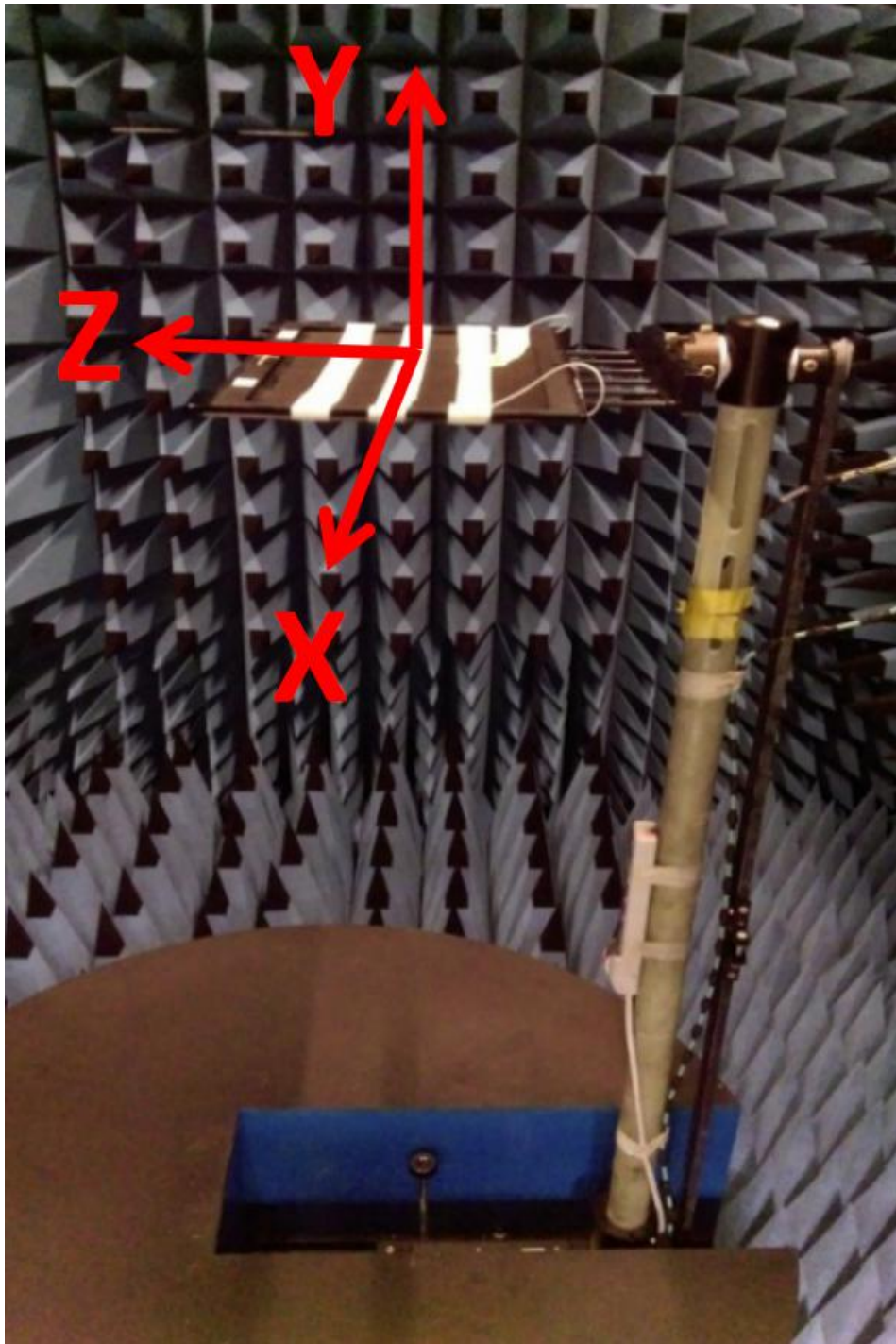
Antenna Test Setup Photos:
