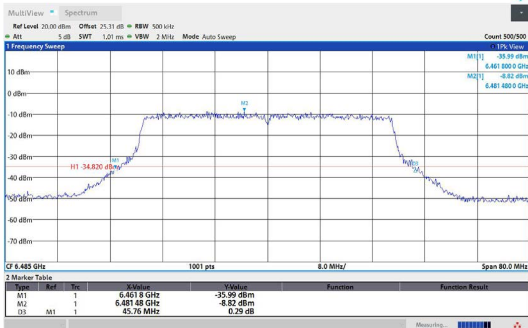
11AX40MIMO-Ant2-6485
