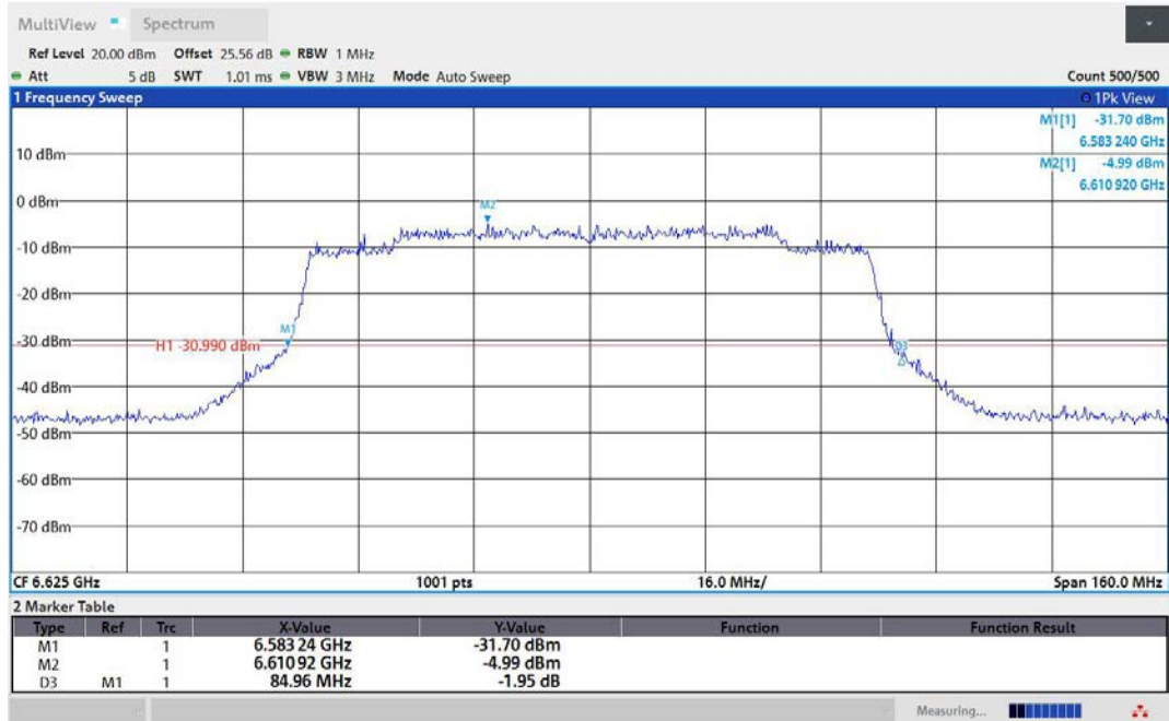
11AX80MIMO-Ant2-6625
