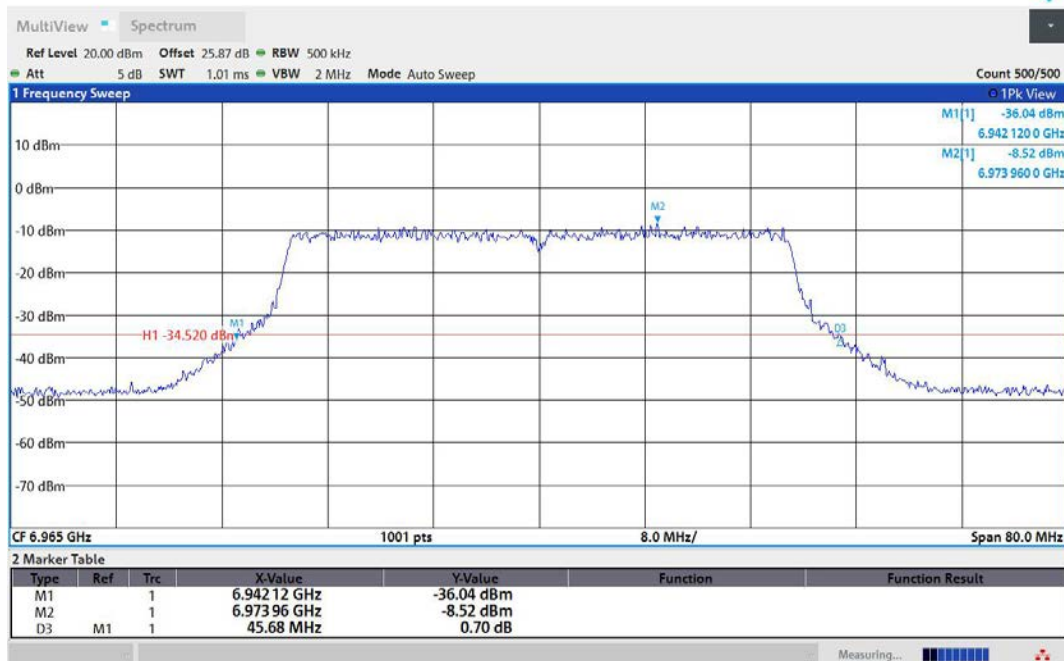
11AX40MIMO-Ant2-6965
