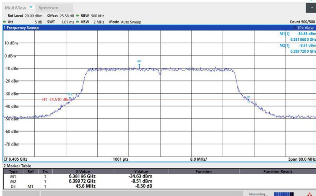
11AX40MIMO-Ant2-6405
