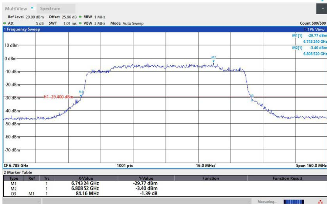
11AX80MIMO-Ant1-6785
