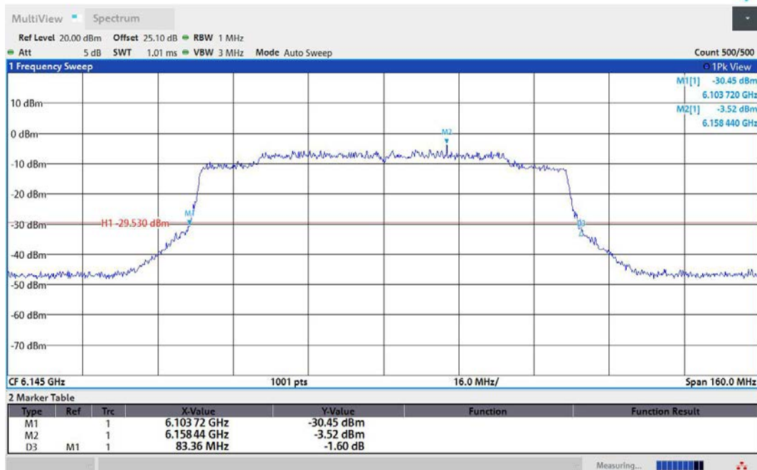
11AX80MIMO-Ant2-6145
