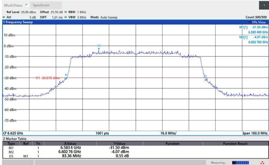
11AX80MIMO-Ant1-6625
