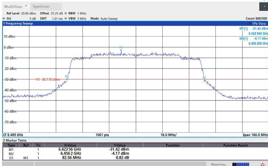
11AX80MIMO-Ant2-6465
