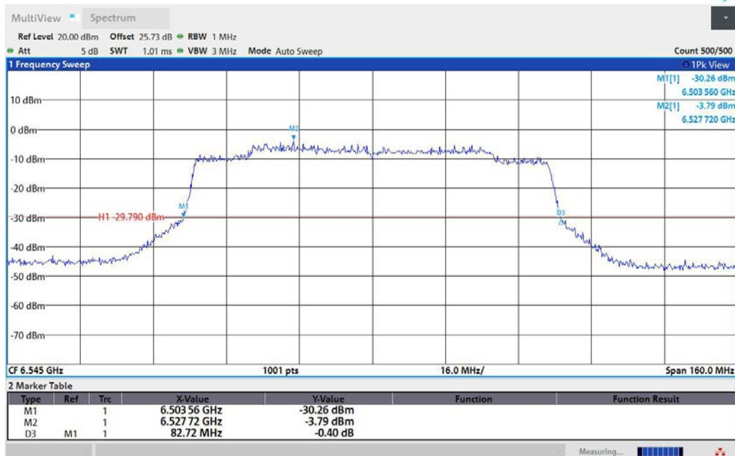
11AX80MIMO-Ant2-6545
