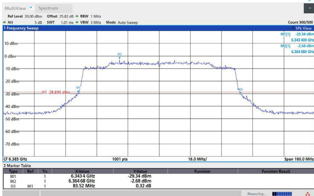
11AX80MIMO-Ant1-6385
