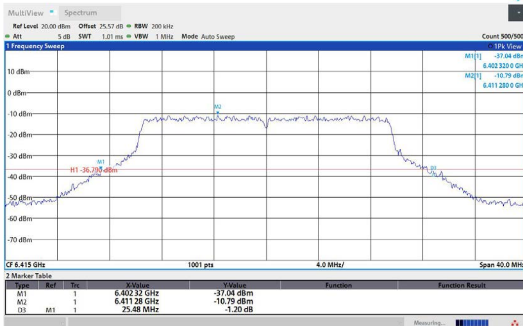
11AX20MIMO-Ant2-6415
