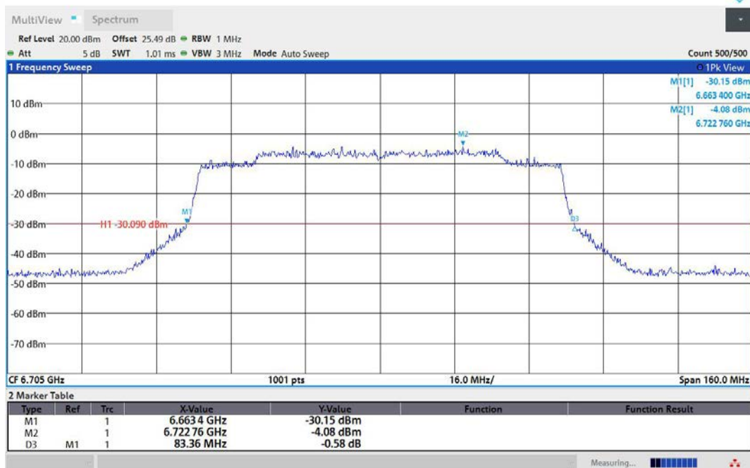
11AX80MIMO-Ant1-6705
