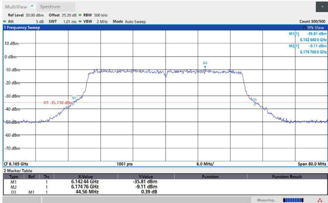
11AX40MIMO-Ant2-6165
