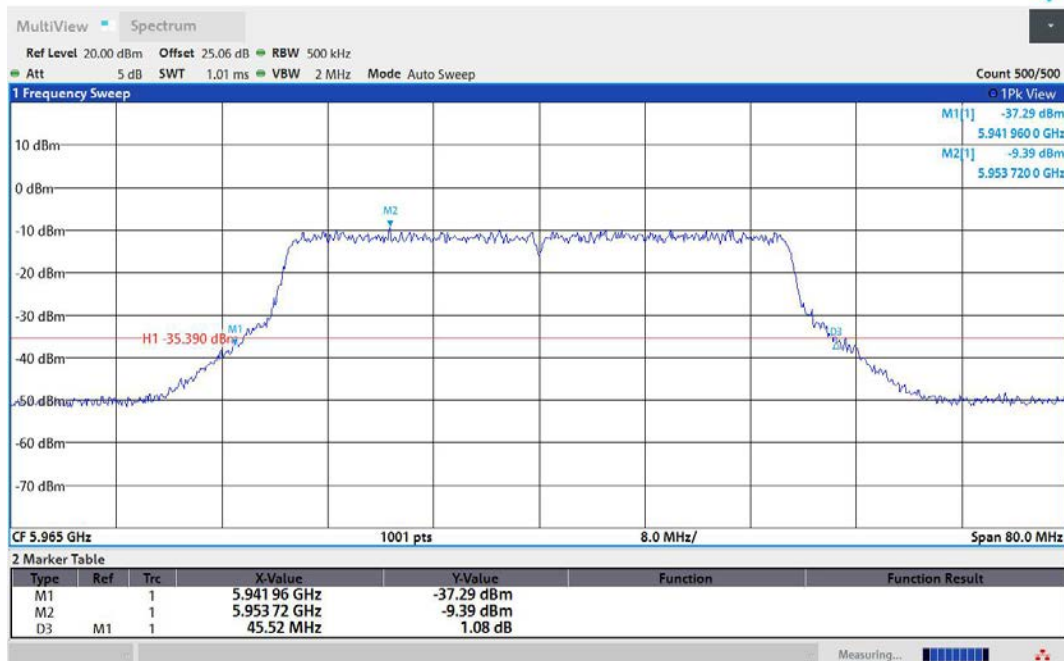
11AX40MIMO-Ant2-5965
