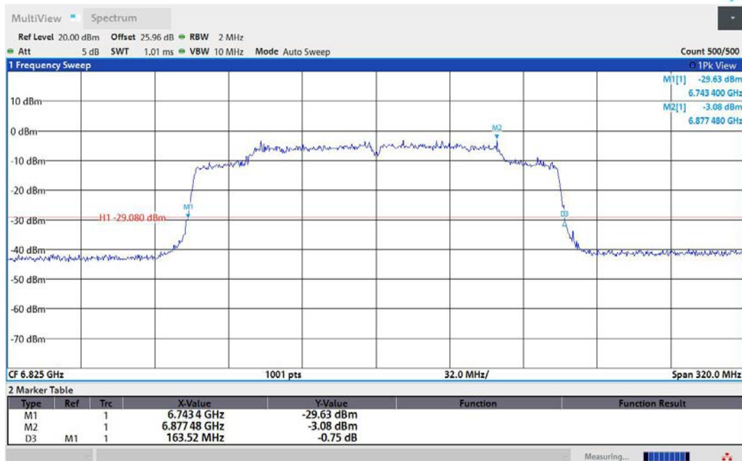
11AX160MIMO-Ant2-6825
