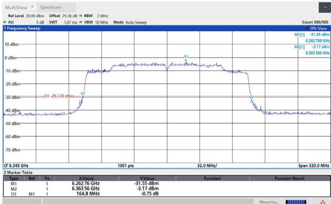
11AX160MIMO-Ant2-6345
