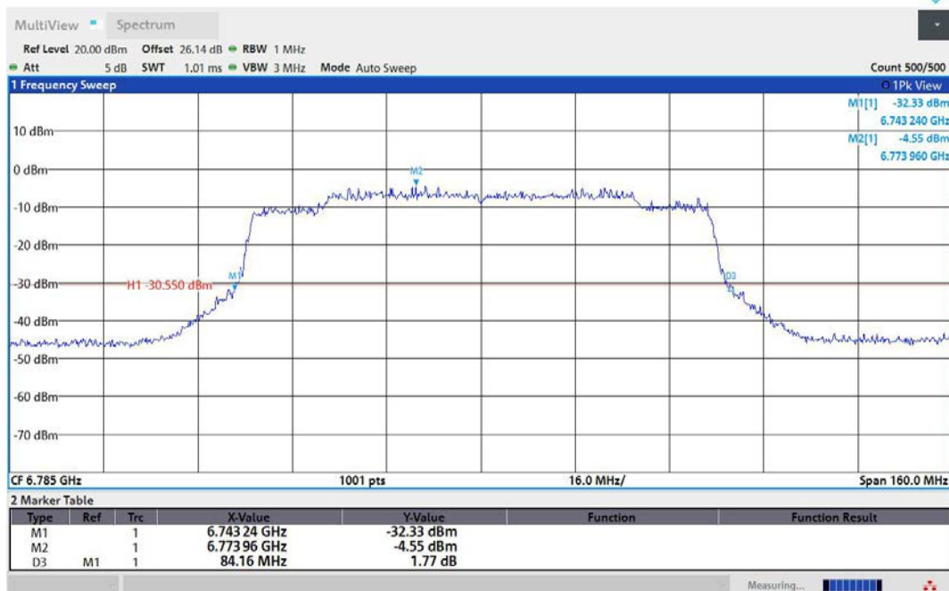
11AX80MIMO-Ant2-6785
