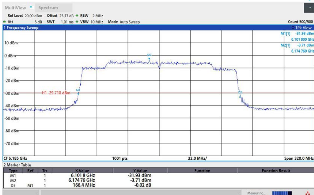
11AX160MIMO-Ant2-6185
