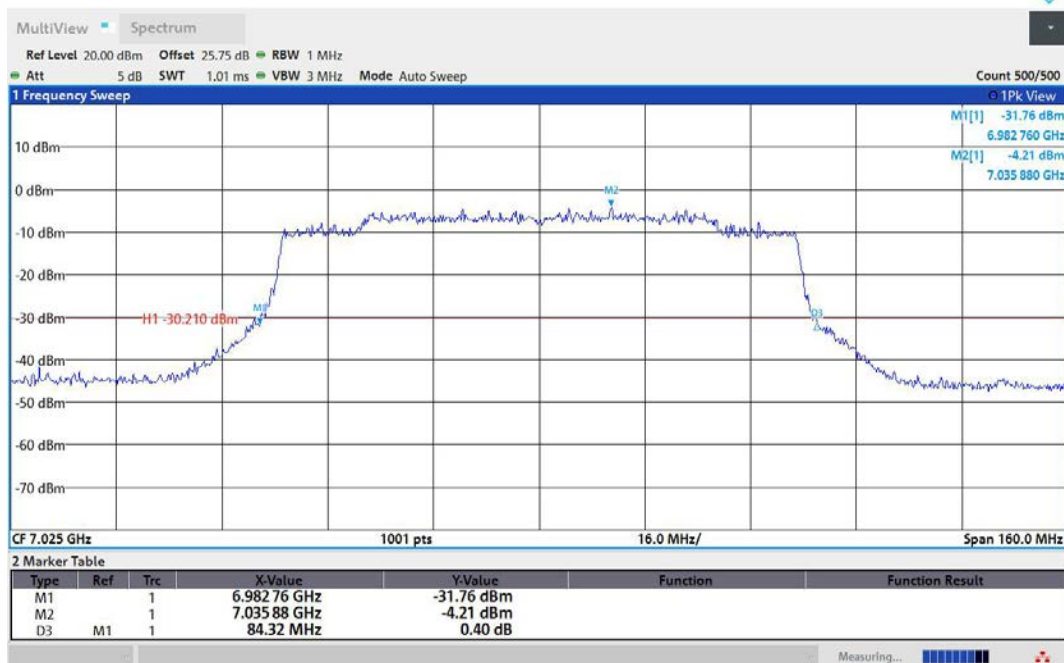
11AX80MIMO-Ant2-7025
