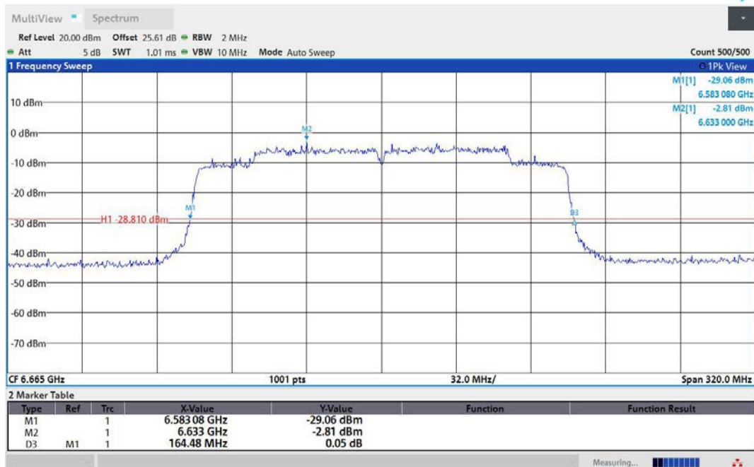
11AX160MIMO-Ant2-6665
