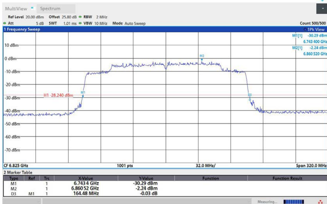
11AX160MIMO-Ant1-6825
