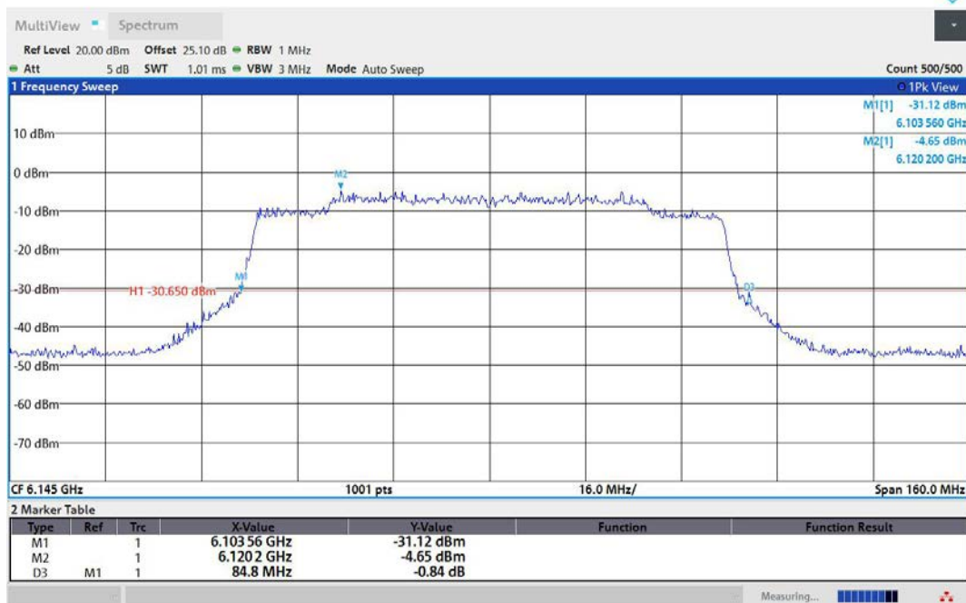
11AX80MIMO-Ant1-6145
