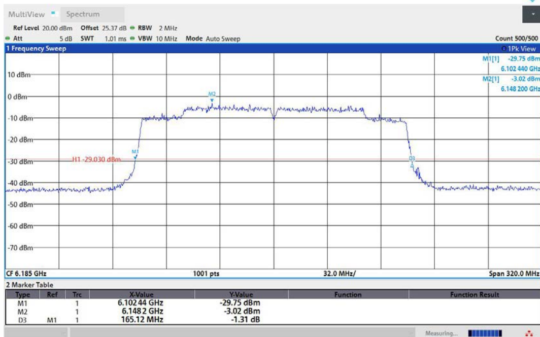
11AX160MIMO-Ant1-6185
