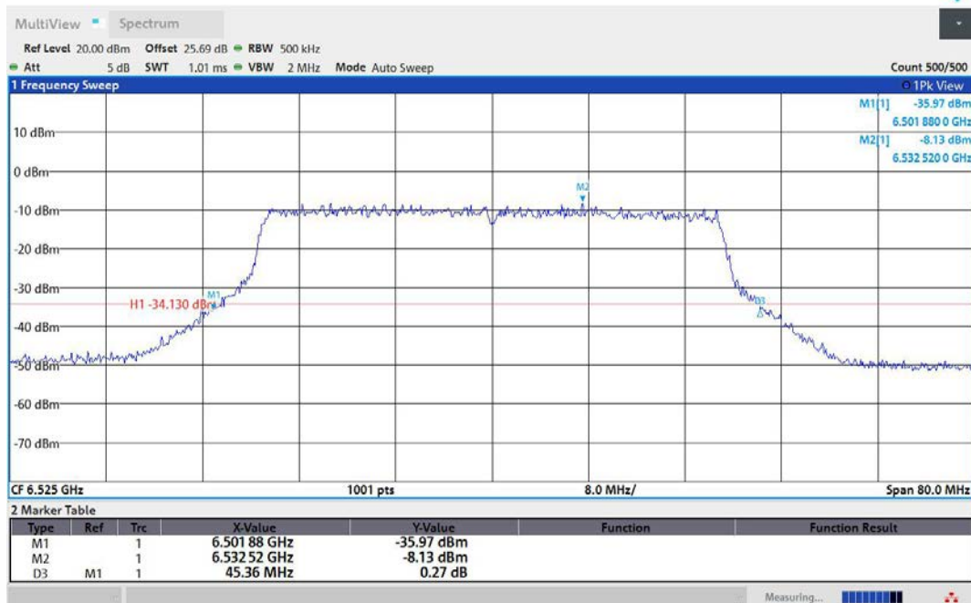
11AX40MIMO-Ant2-6525
