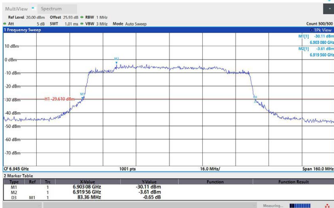
11AX80MIMO-Ant1-6945
