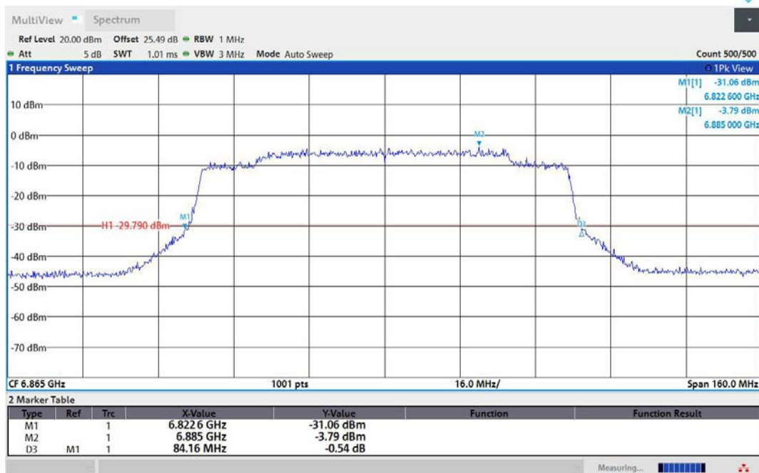
11AX80MIMO-Ant1-6865
