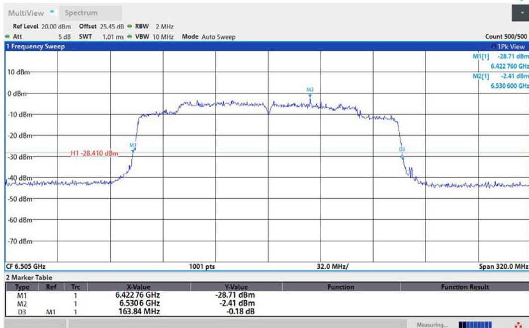
11AX160MIMO-Ant2-6505
