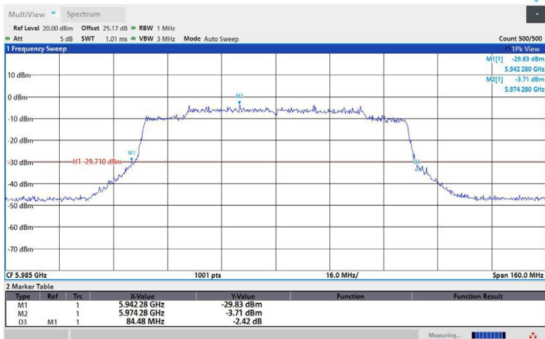
11AX80MIMO-Ant1-5985
