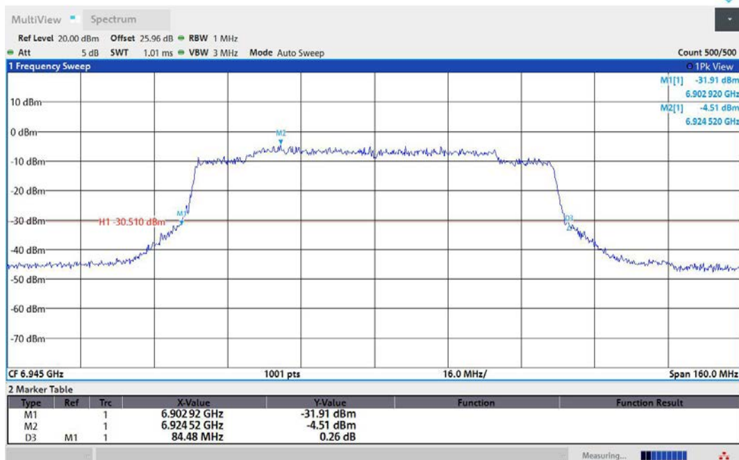
11AX80MIMO-Ant2-6945
