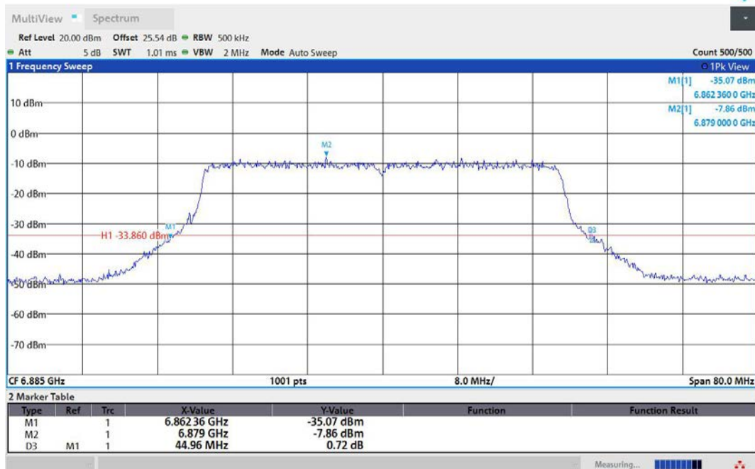
11AX40MIMO-Ant2-6885
