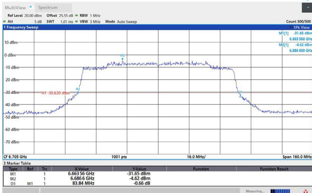
11AX80MIMO-Ant2-6705
