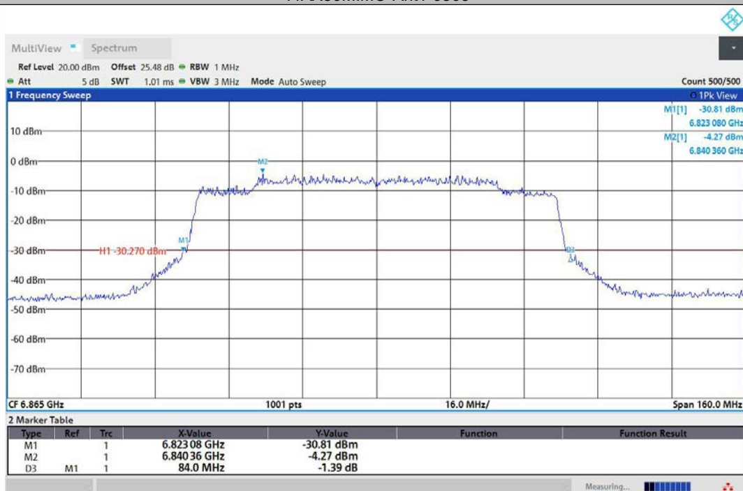
11AX80MIMO-Ant2-6865
