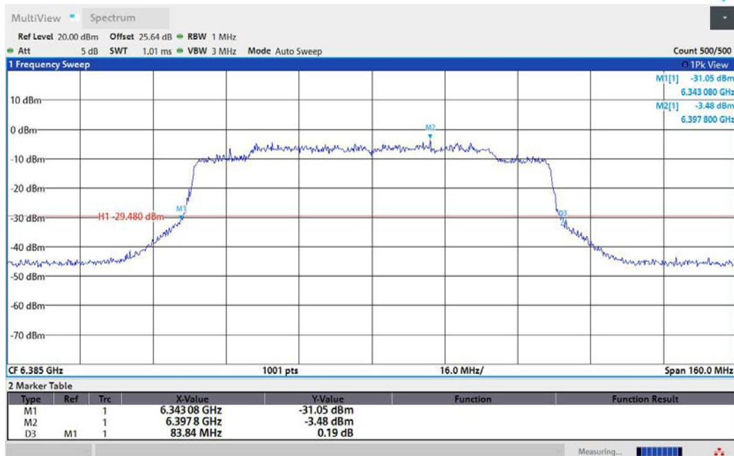
11AX80MIMO-Ant2-6385
