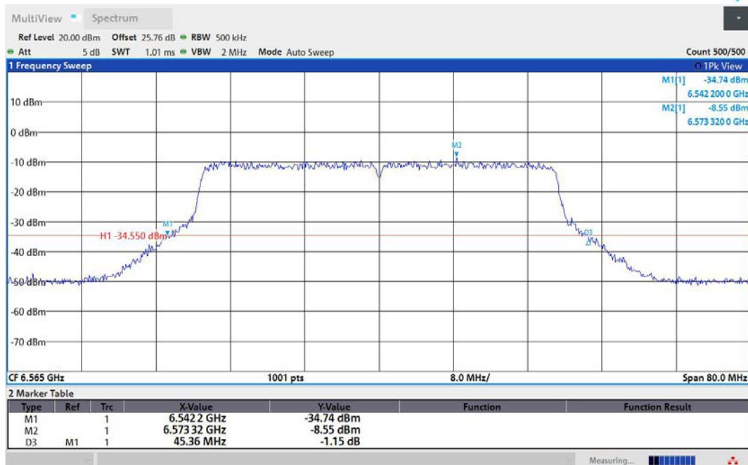
11AX40MIMO-Ant2-6565
