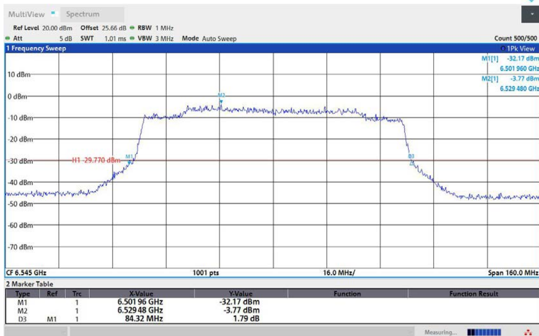
11AX80MIMO-Ant1-6545
