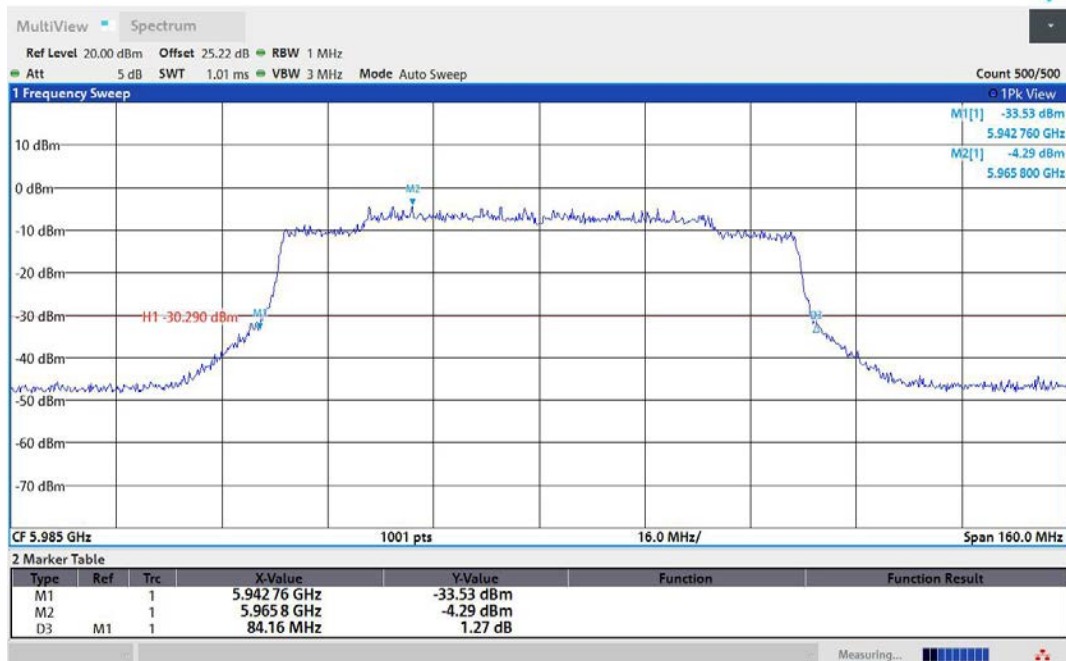
11AX80MIMO-Ant2-5985
