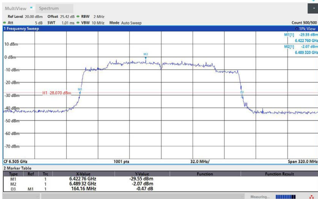
11AX160MIMO-Ant1-6505
