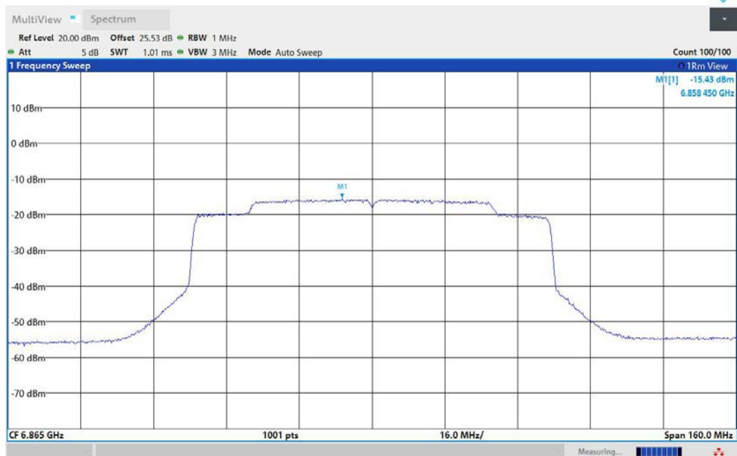
11AX80MIMO-Ant2-6865-PASS
