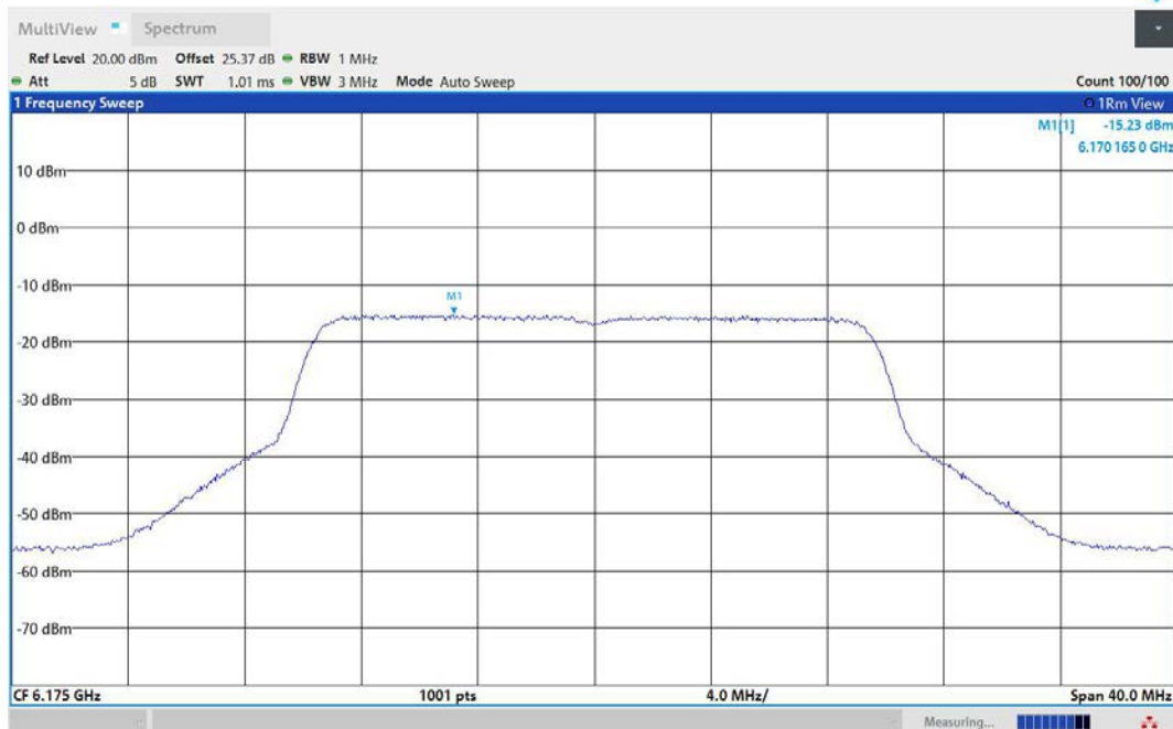
11AX20MIMO-Ant2-6175-PASS
