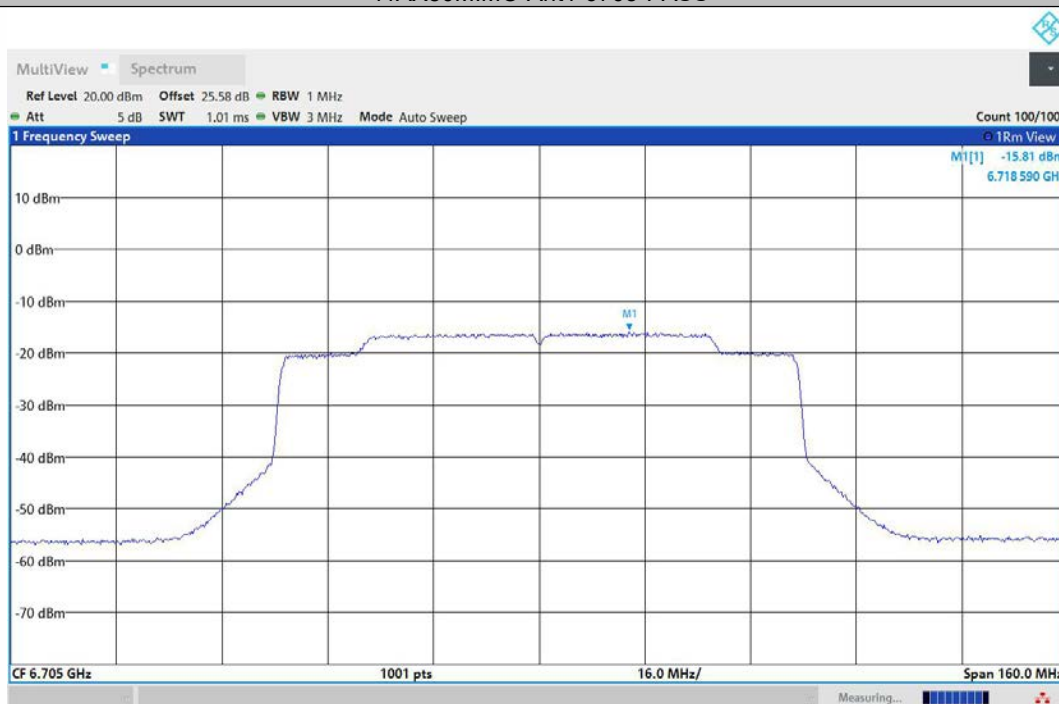
11AX80MIMO-Ant2-6705-PASS
