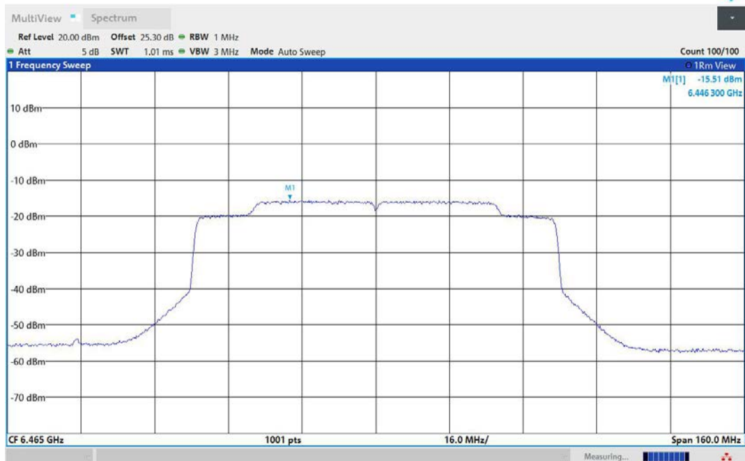
11AX80MIMO-Ant2-6465-PASS
