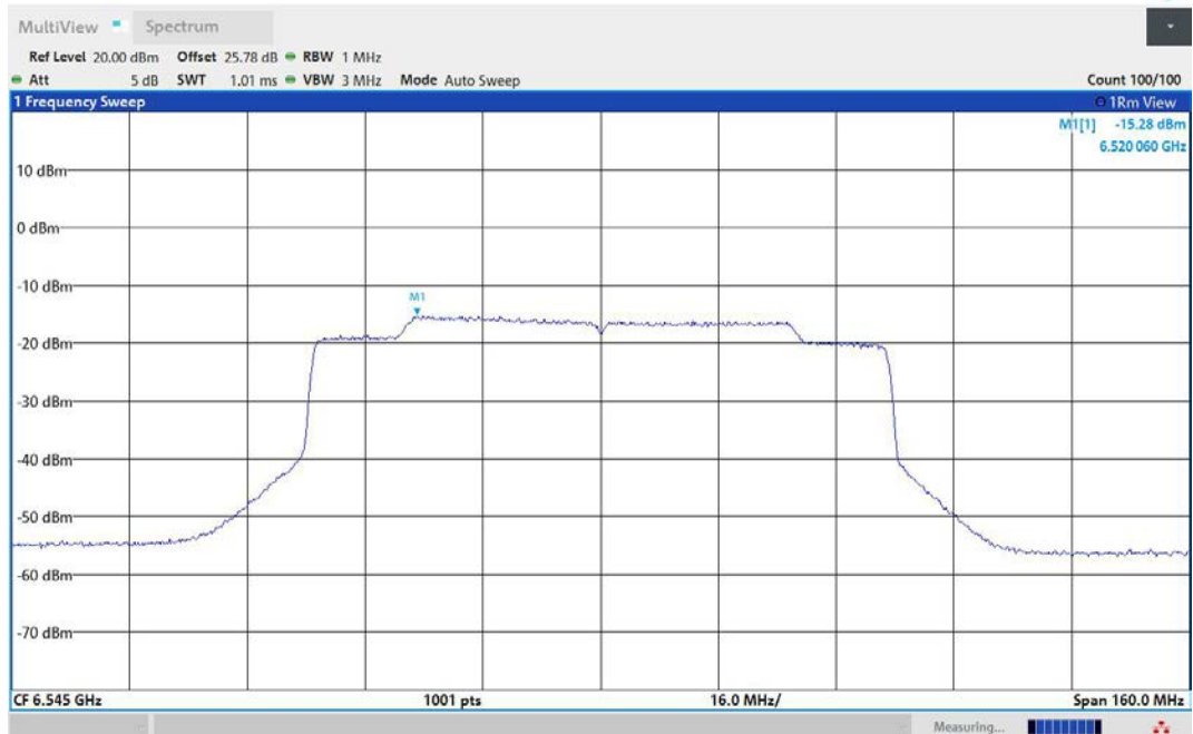
11AX80MIMO-Ant2-6545-PASS
