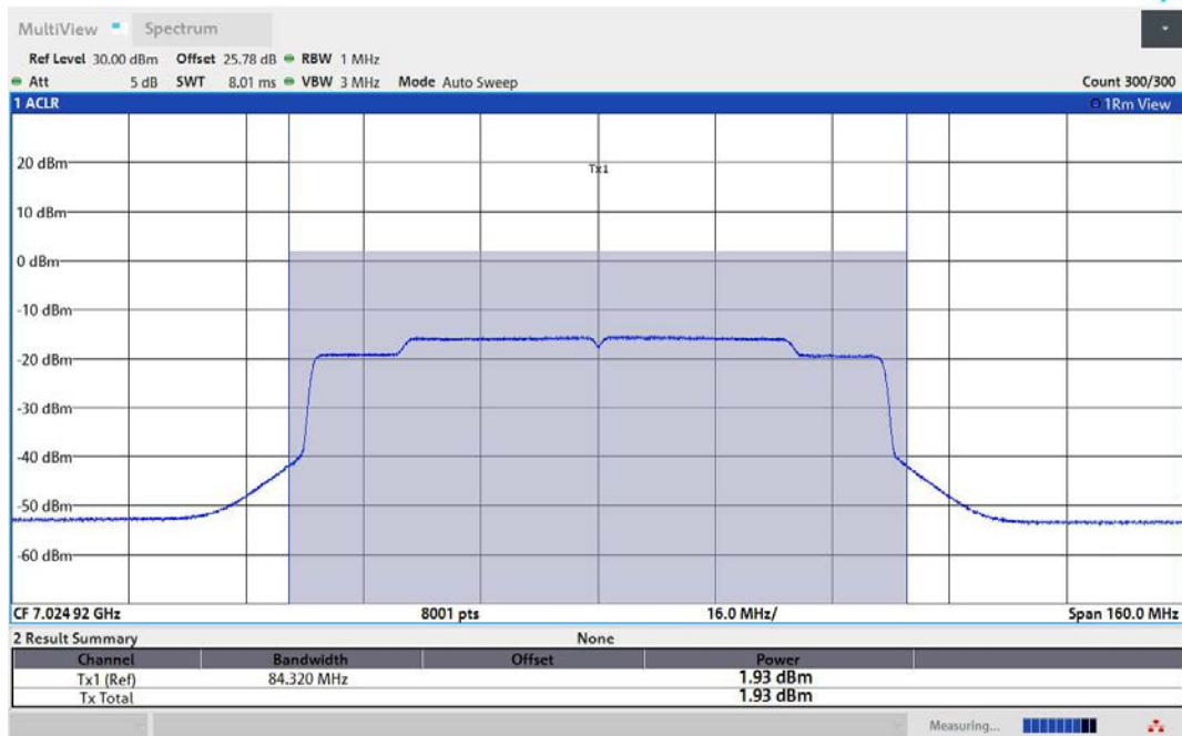
11AX80MIMO-Ant2-7025-PASS
