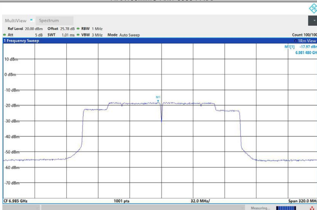
11AX160MIMO-Ant2-6985-PASS
