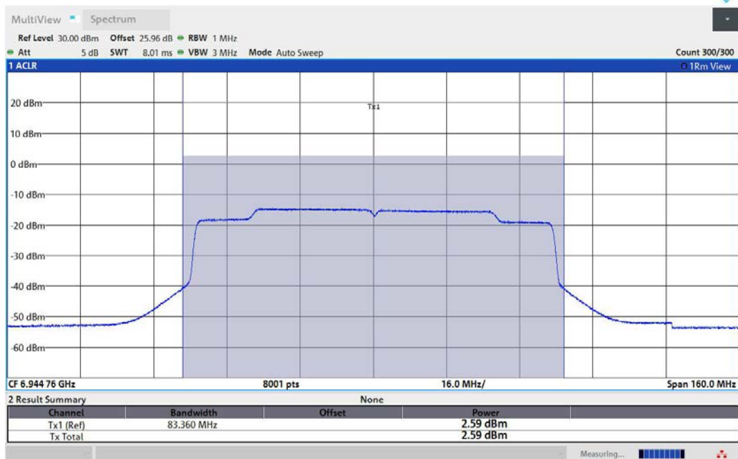
11AX80MIMO-Ant1-6945-PASS
