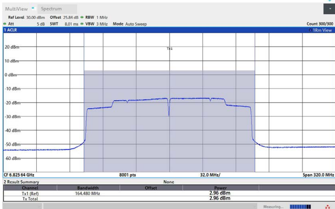
11AX160MIMO-Ant1-6825-PASS
