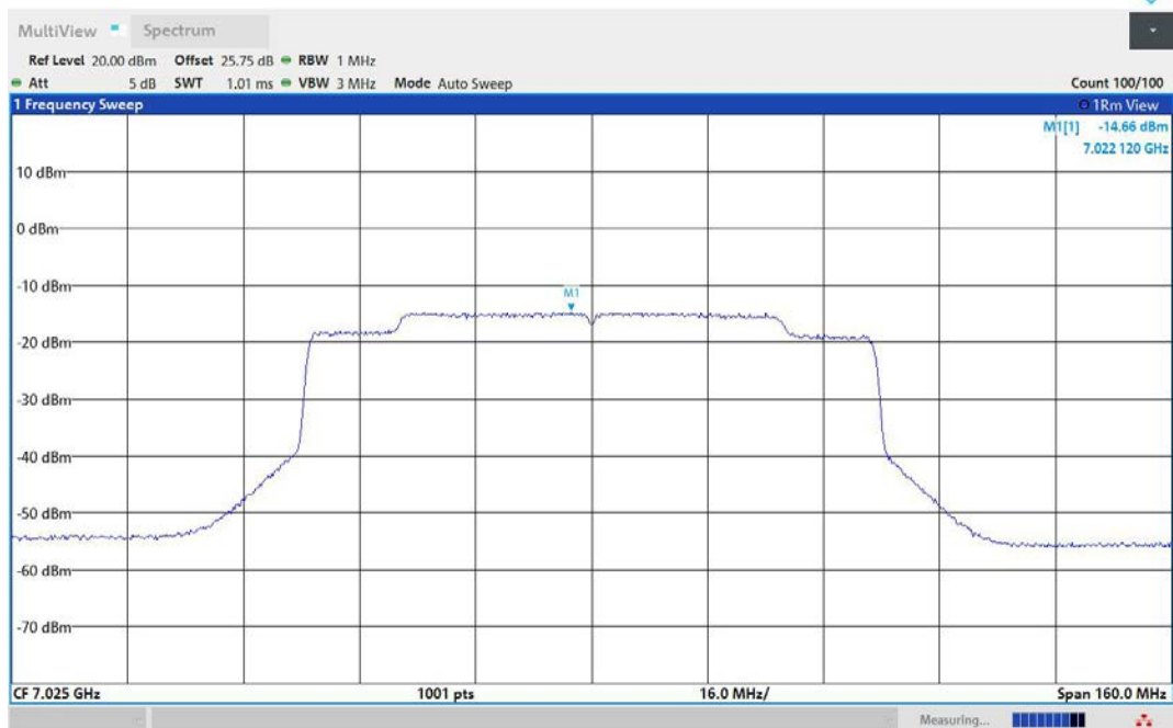
11AX80MIMO-Ant1-7025-PASS
