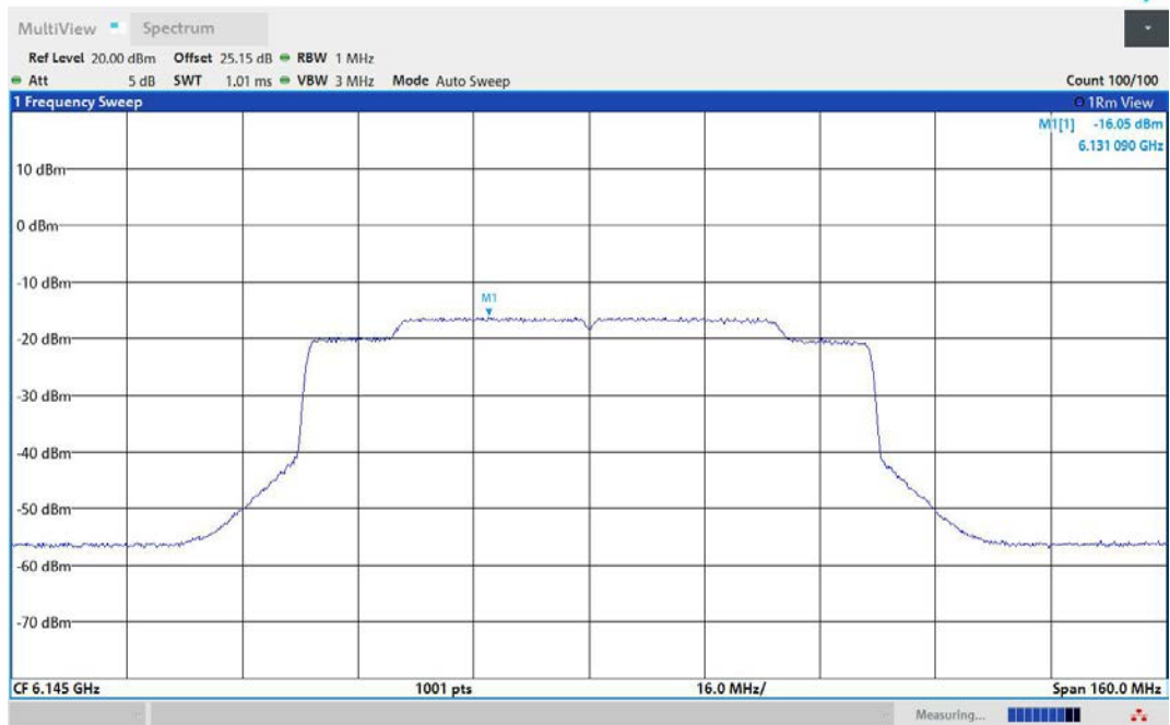
11AX80MIMO-Ant2-6145-PASS
