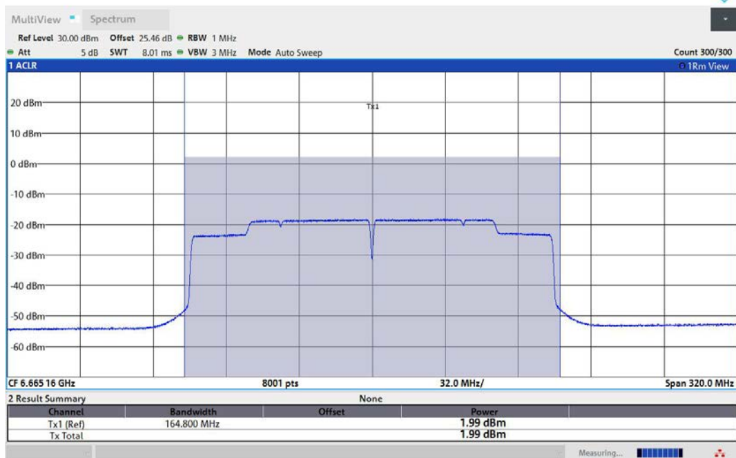
11AX160MIMO-Ant1-6665-PASS
