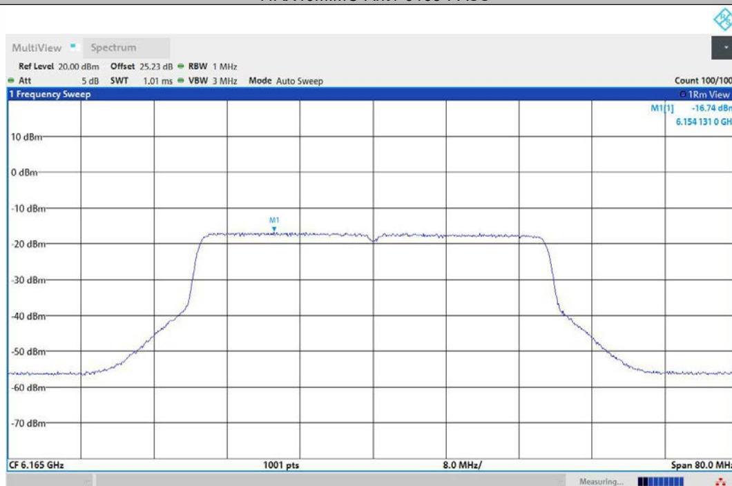
11AX40MIMO-Ant2-6165-PASS
