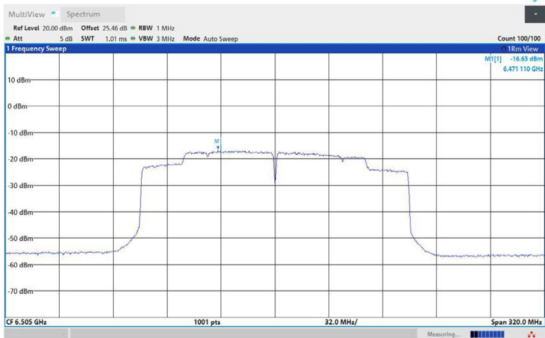
11AX160MIMO-Ant1-6505-PASS
