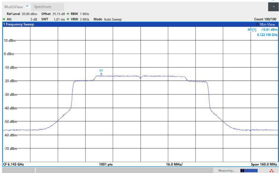
11AX80MIMO-Ant1-6145-PASS
