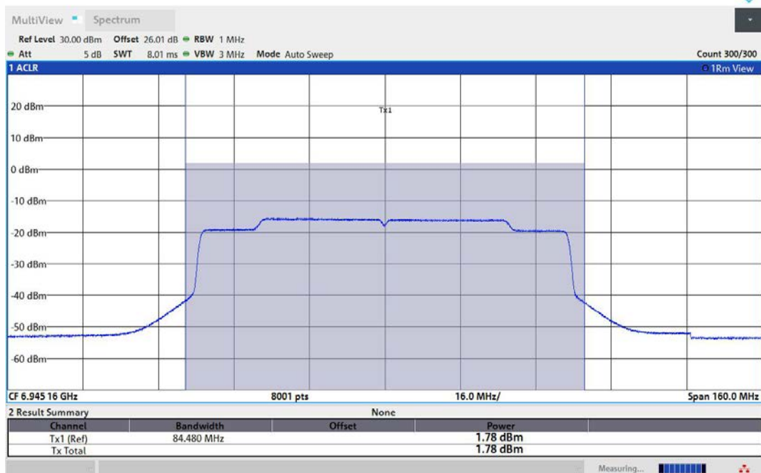
11AX80MIMO-Ant2-6945-PASS
