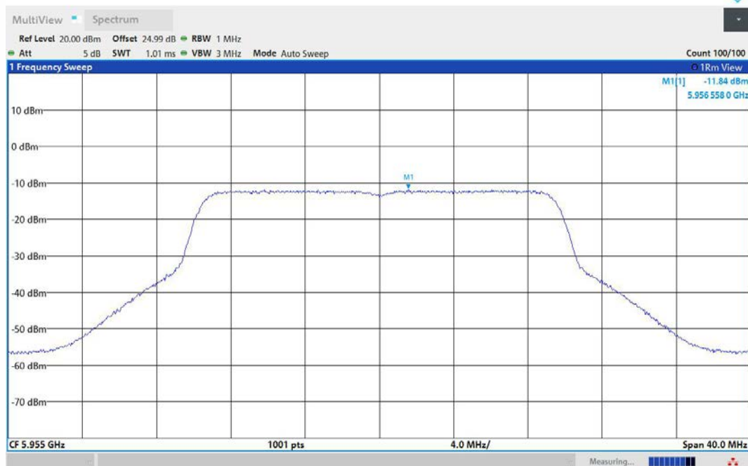
11AX20MIMO-Ant2-5955-PASS
