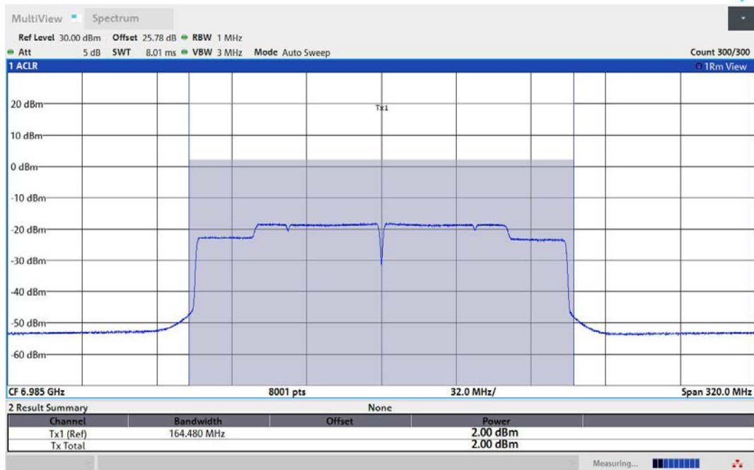
11AX160MIMO-Ant2-6985-PASS
