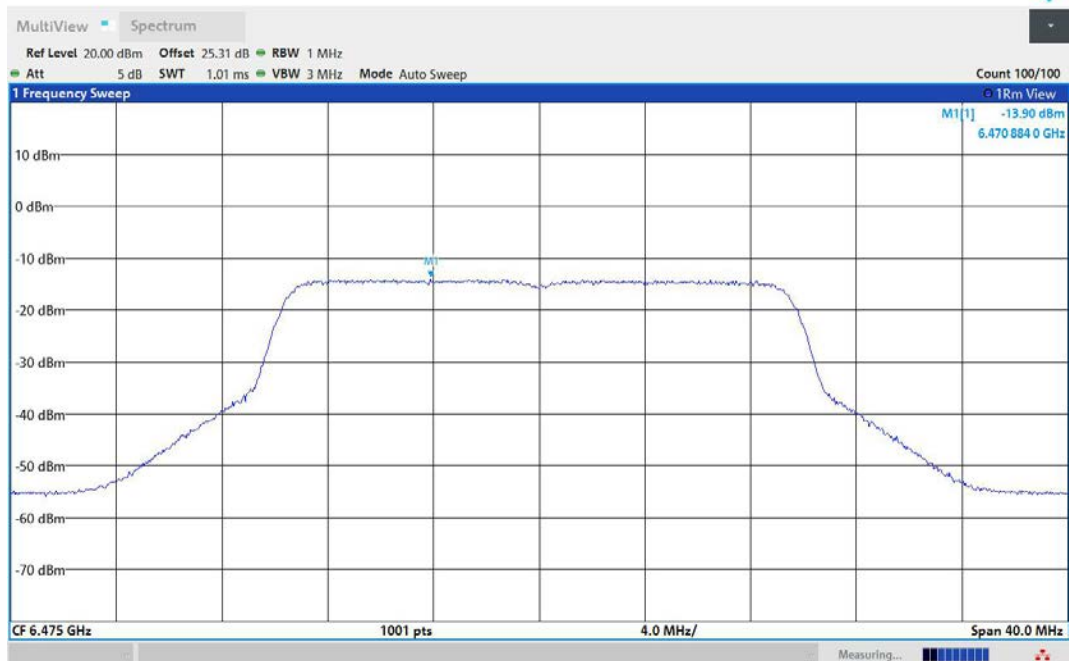
11AX20MIMO-Ant2-6475-PASS
