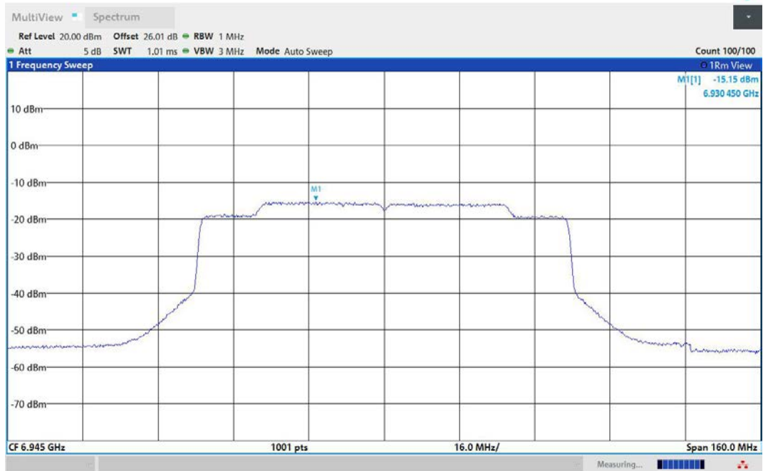
11AX80MIMO-Ant2-6945-PASS
