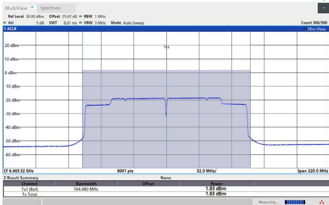
11AX160MIMO-Ant2-6665-PASS
