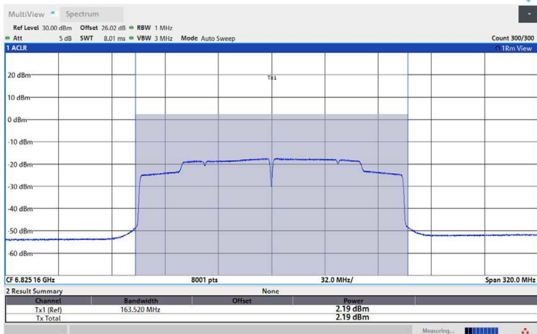
11AX160MIMO-Ant2-6825-PASS
