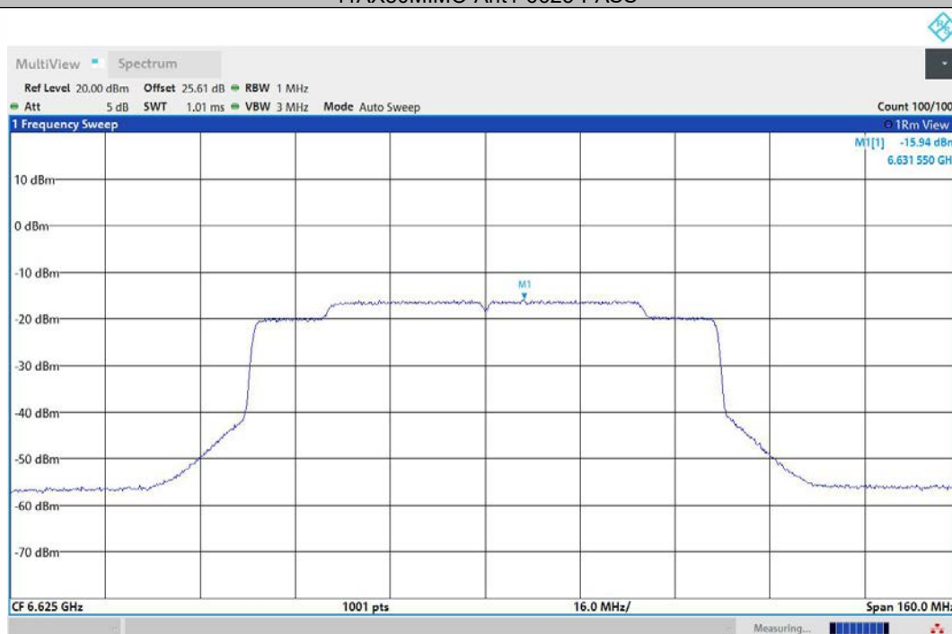
11AX80MIMO-Ant2-6625-PASS
