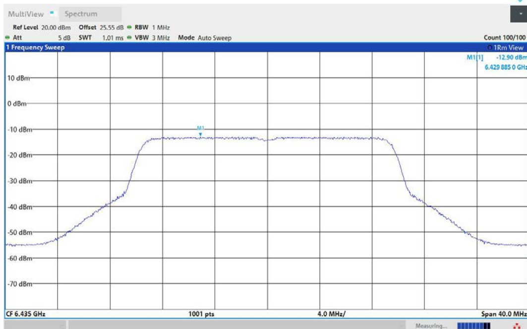
11AX20MIMO-Ant2-6435-PASS
