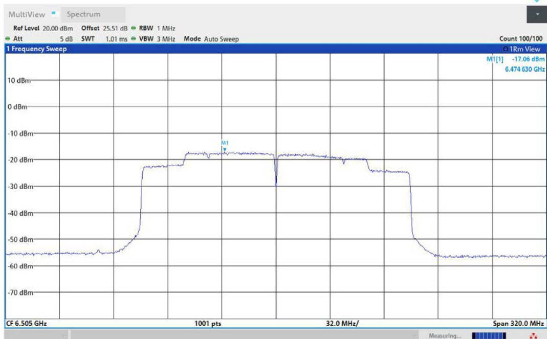
11AX160MIMO-Ant2-6505-PASS
