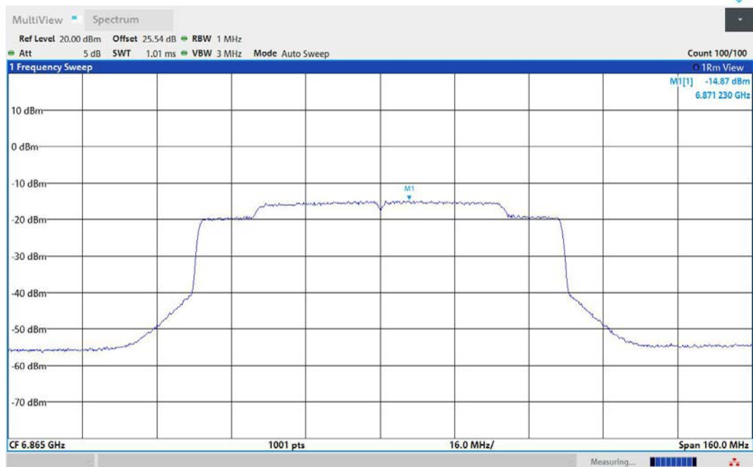
11AX80MIMO-Ant1-6865-PASS
