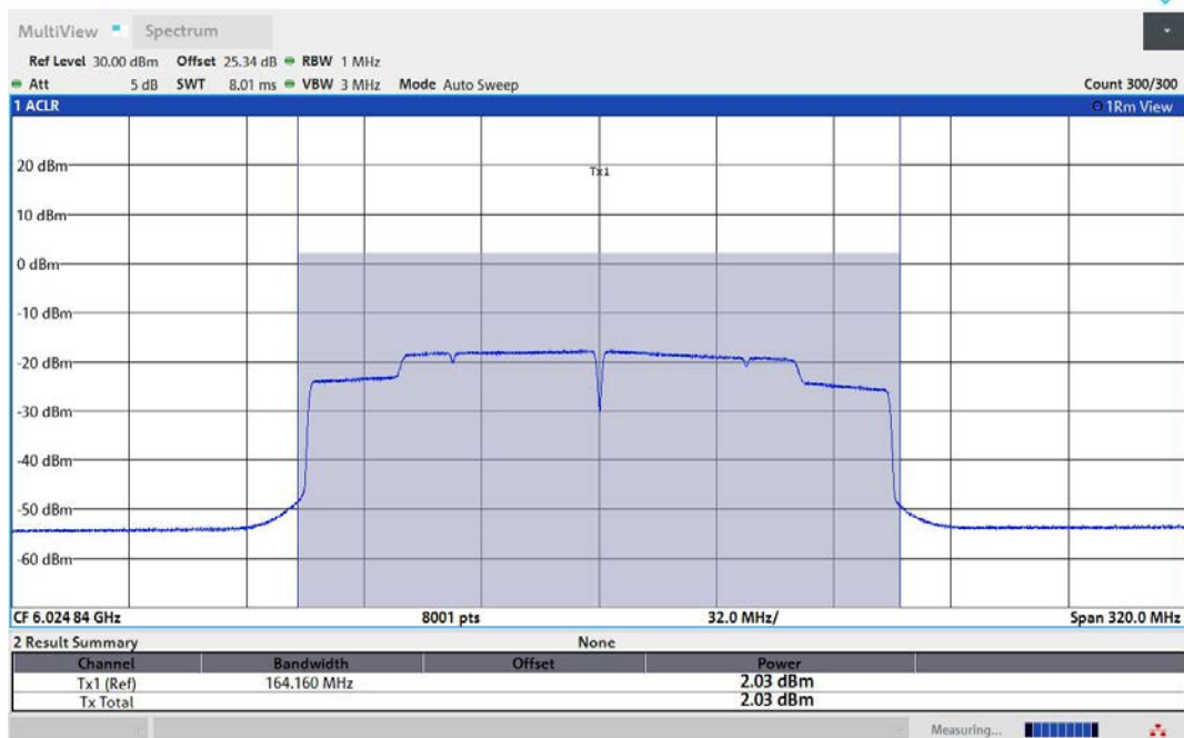
11AX160MIMO-Ant1-6025-PASS
