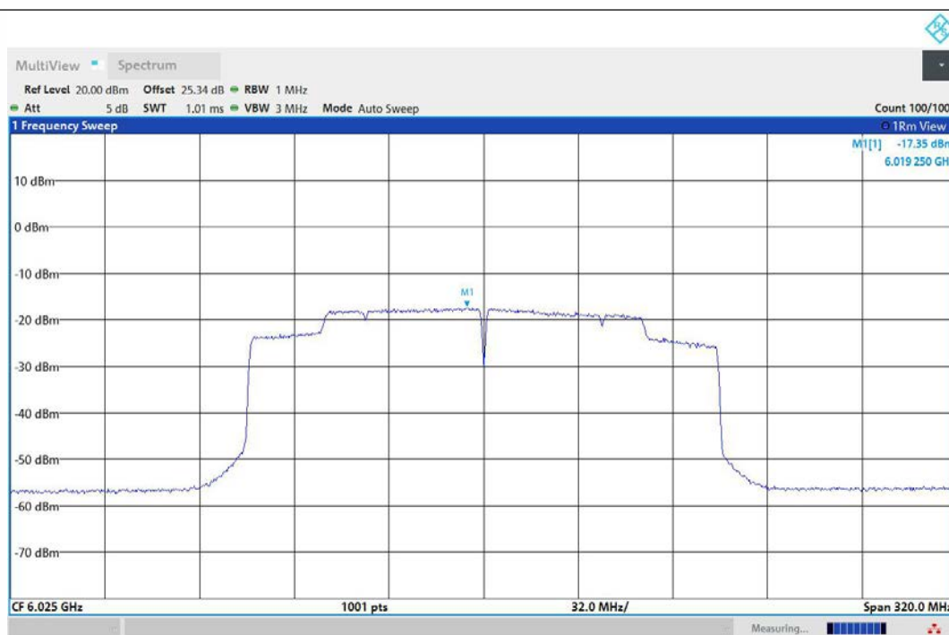
11AX160MIMO-Ant1-6025-PASS
