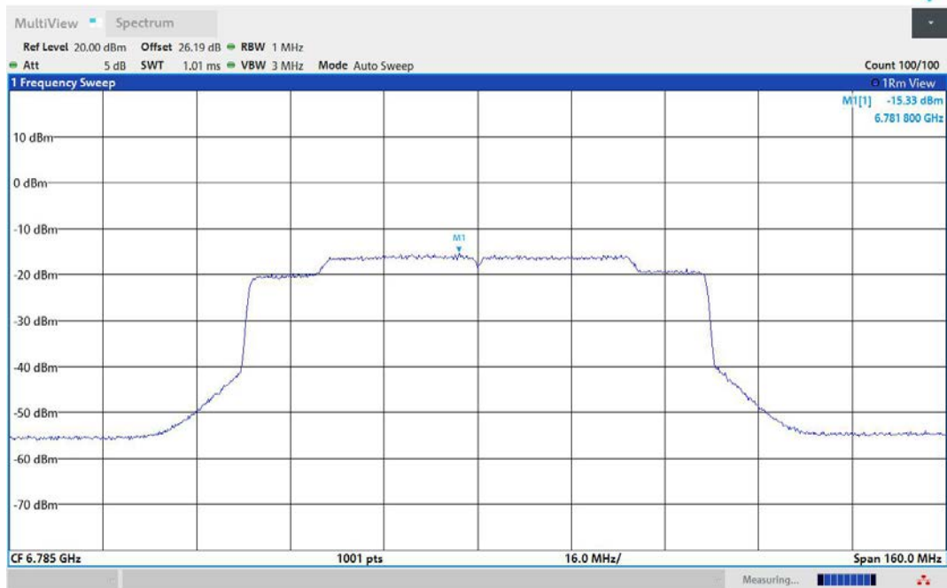
11AX80MIMO-Ant2-6785-PASS
