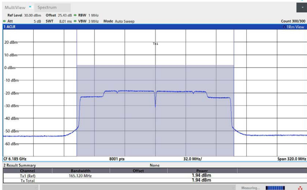
11AX160MIMO-Ant1-6185-PASS
