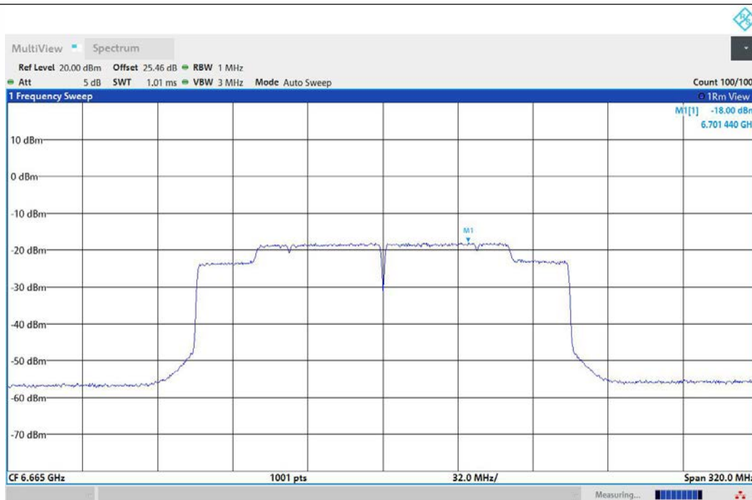
11AX160MIMO-Ant1-6665-PASS
