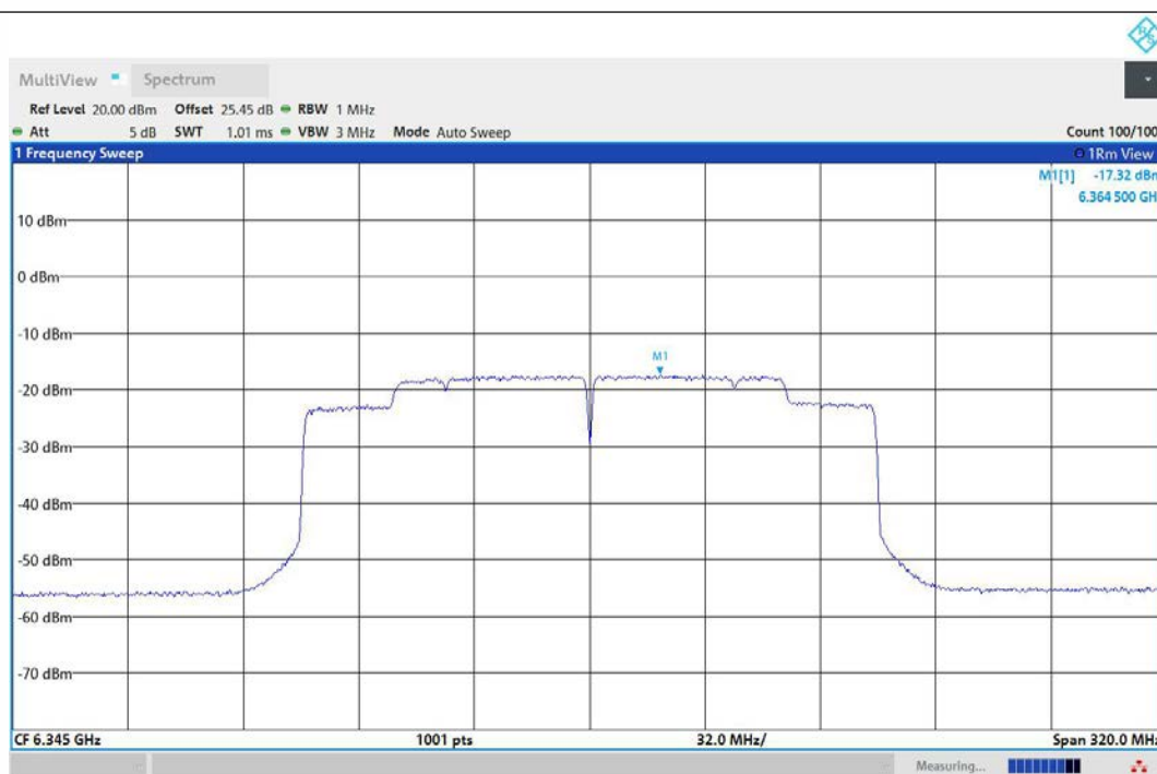
11AX160MIMO-Ant1-6345-PASS
