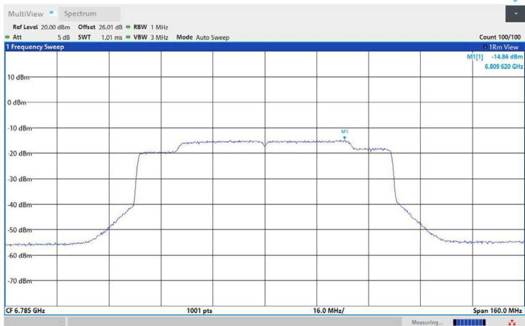
11AX80MIMO-Ant1-6785-PASS
