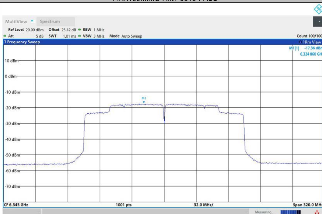
11AX160MIMO-Ant2-6345-PASS
