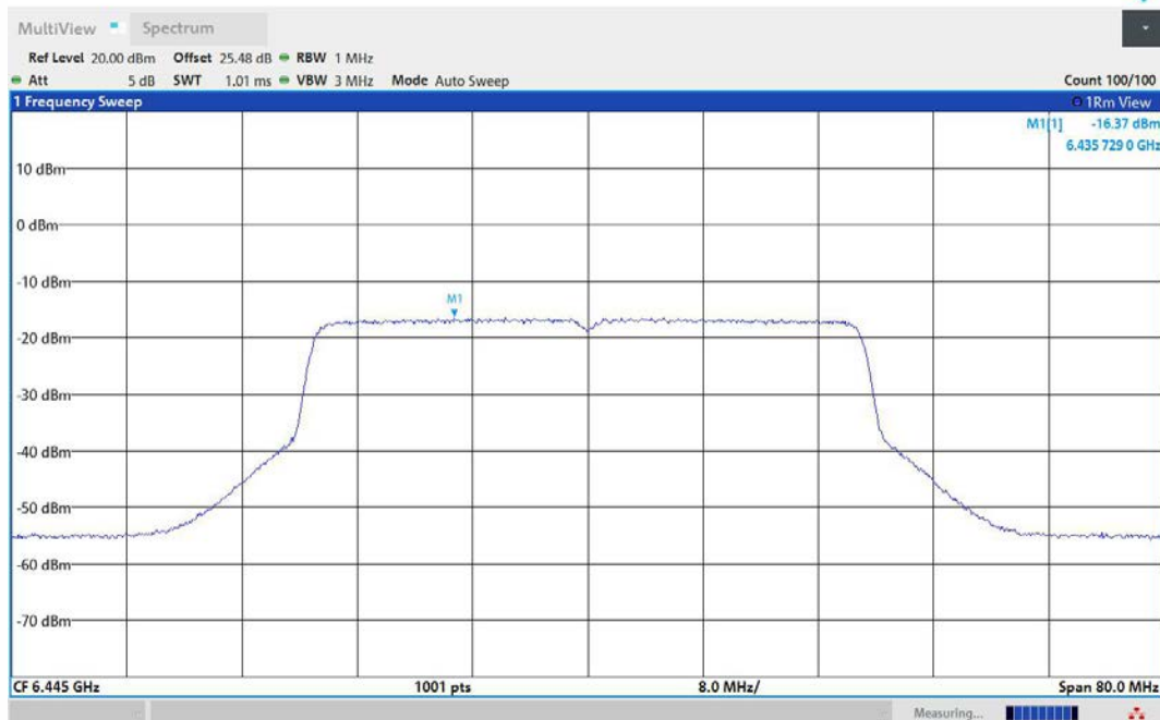
11AX40MIMO-Ant2-6445-PASS
