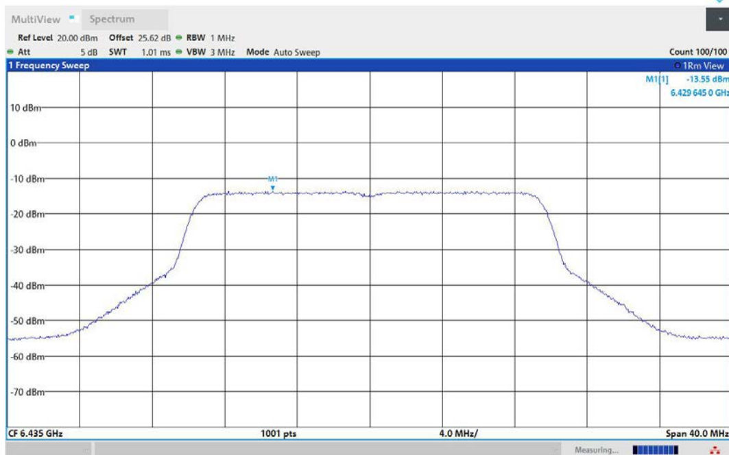
11AX20MIMO-Ant1-6435-PASS
