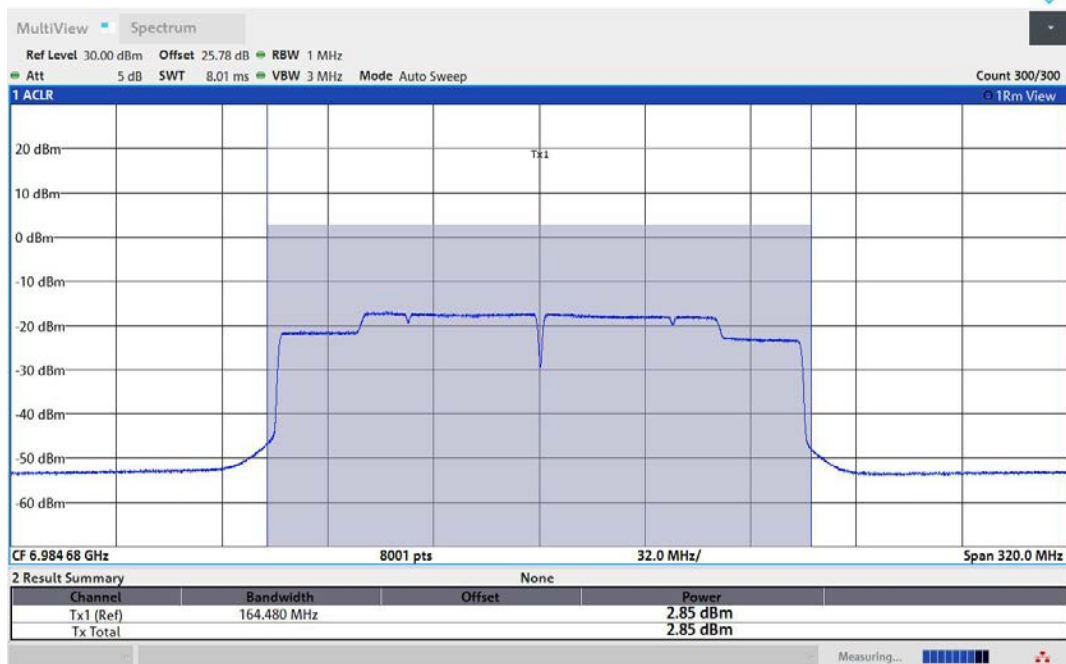
11AX160MIMO-Ant1-6985-PASS
