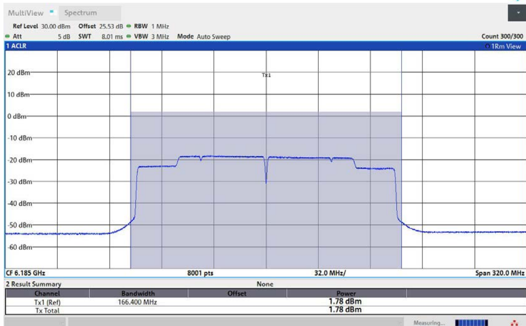
11AX160MIMO-Ant2-6185-PASS
