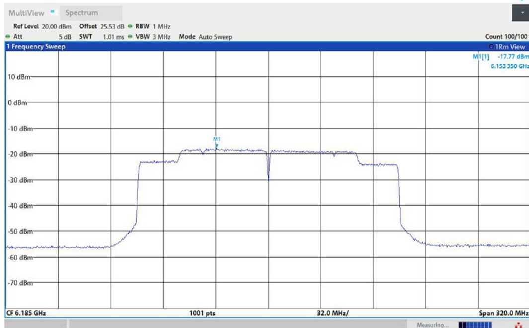
11AX160MIMO-Ant2-6185-PASS
