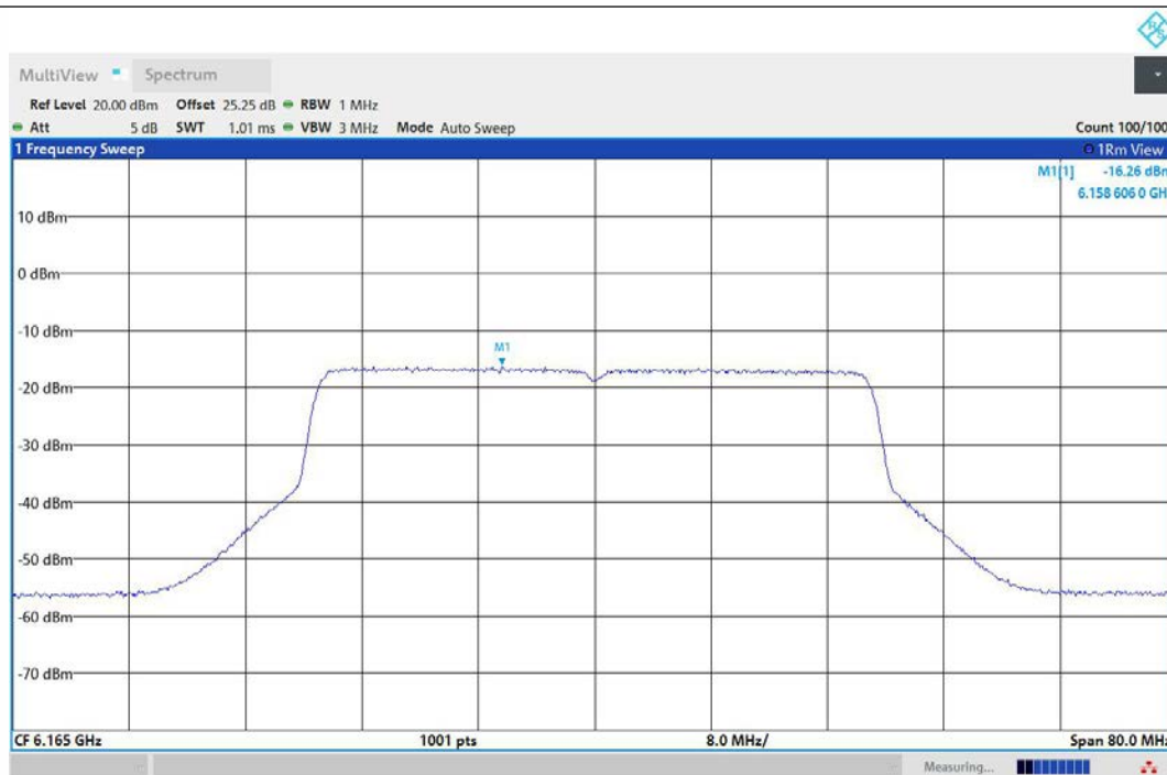
11AX40MIMO-Ant1-6165-PASS
