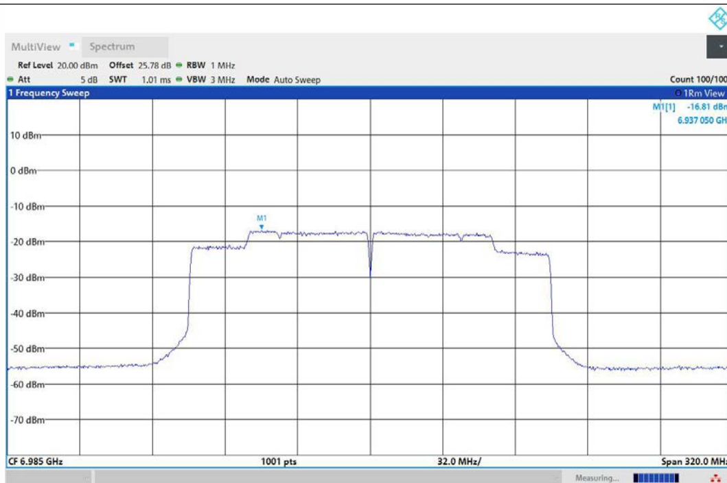
11AX160MIMO-Ant1-6985-PASS
