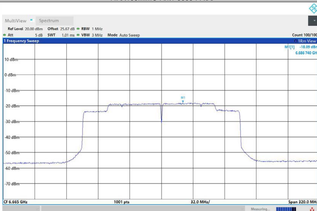
11AX160MIMO-Ant2-6665-PASS
