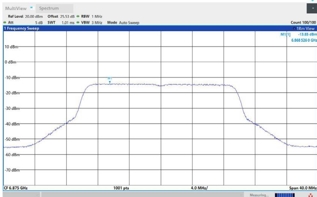
11AX20MIMO-Ant2-6875-PASS
