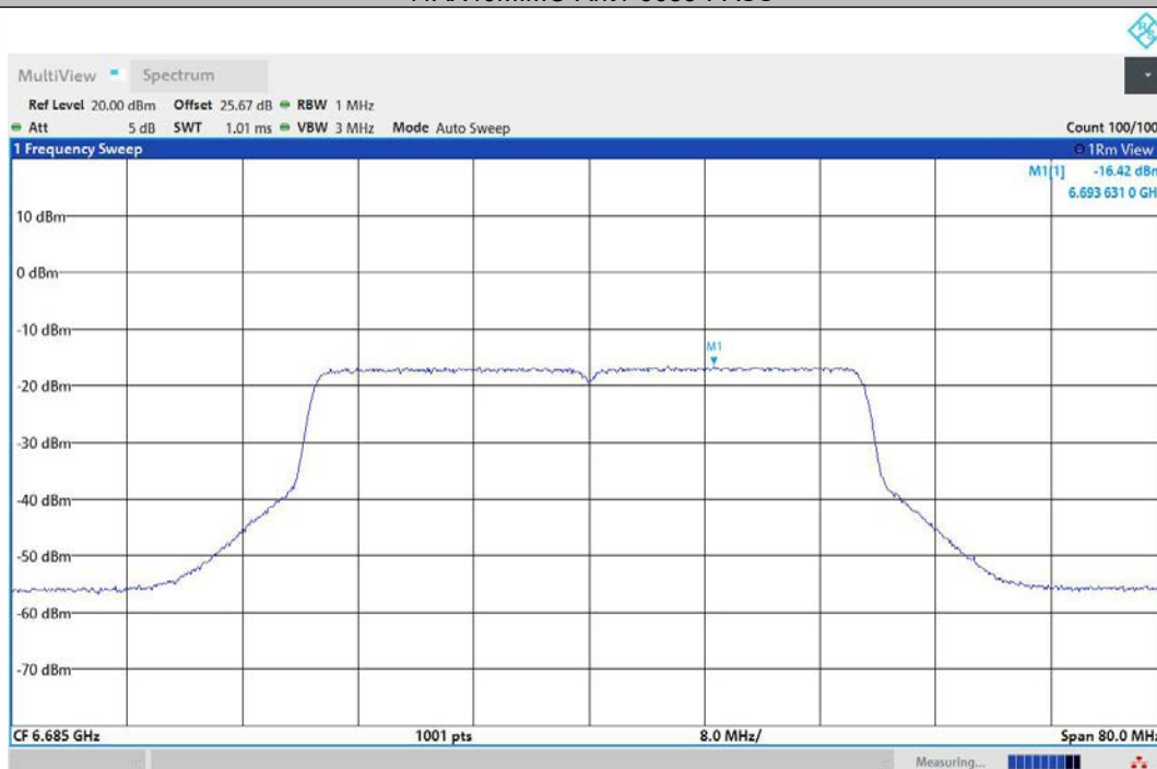
11AX40MIMO-Ant2-6685-PASS
