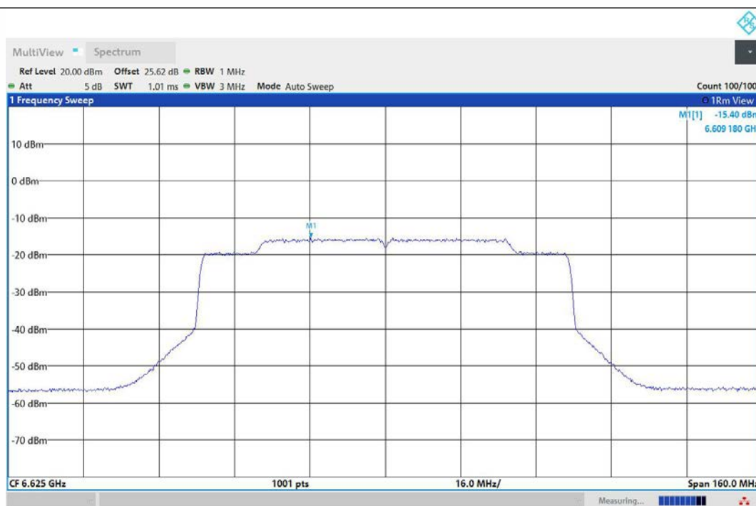
11AX80MIMO-Ant1-6625-PASS
