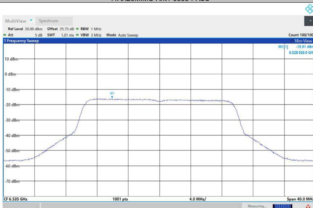
11AX20MIMO-Ant2-6535-PASS
