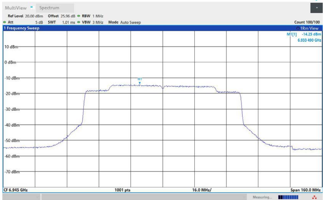
11AX80MIMO-Ant1-6945-PASS
