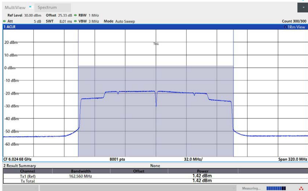
11AX160MIMO-Ant2-6025-PASS
