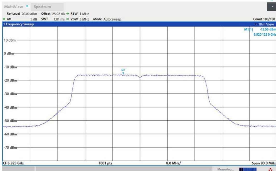
11AX40MIMO-Ant2-6925-PASS
