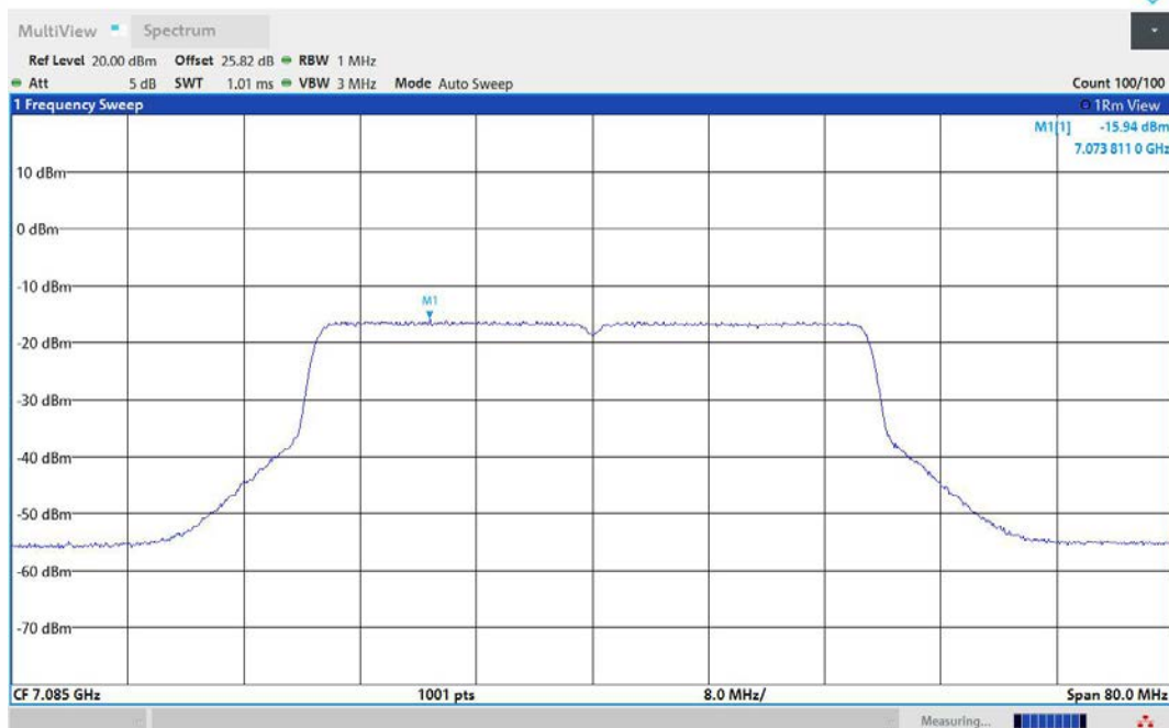
11AX40MIMO-Ant2-7085-PASS
