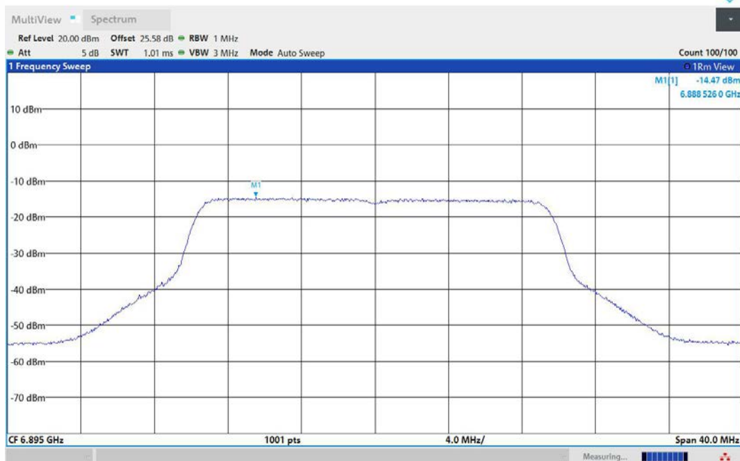
11AX20MIMO-Ant2-6895-PASS
