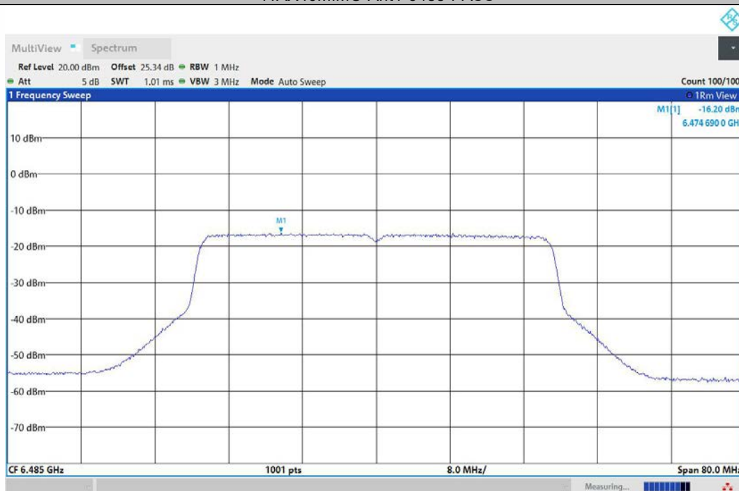
11AX40MIMO-Ant2-6485-PASS
