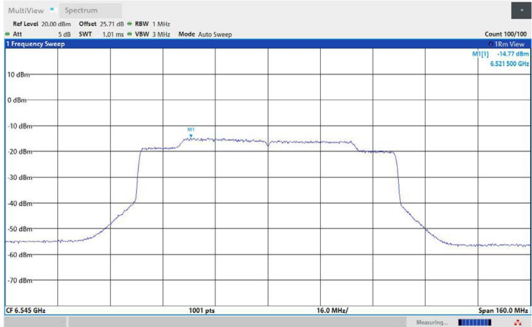
11AX80MIMO-Ant1-6545-PASS
