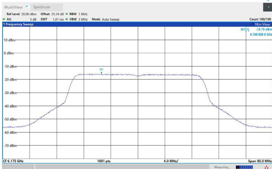
11AX20MIMO-Ant1-6175-PASS
