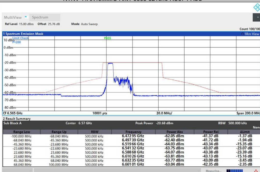
NTNV-11AX40MIMO-Ant2-6565-52Tone-RU37-PASS
