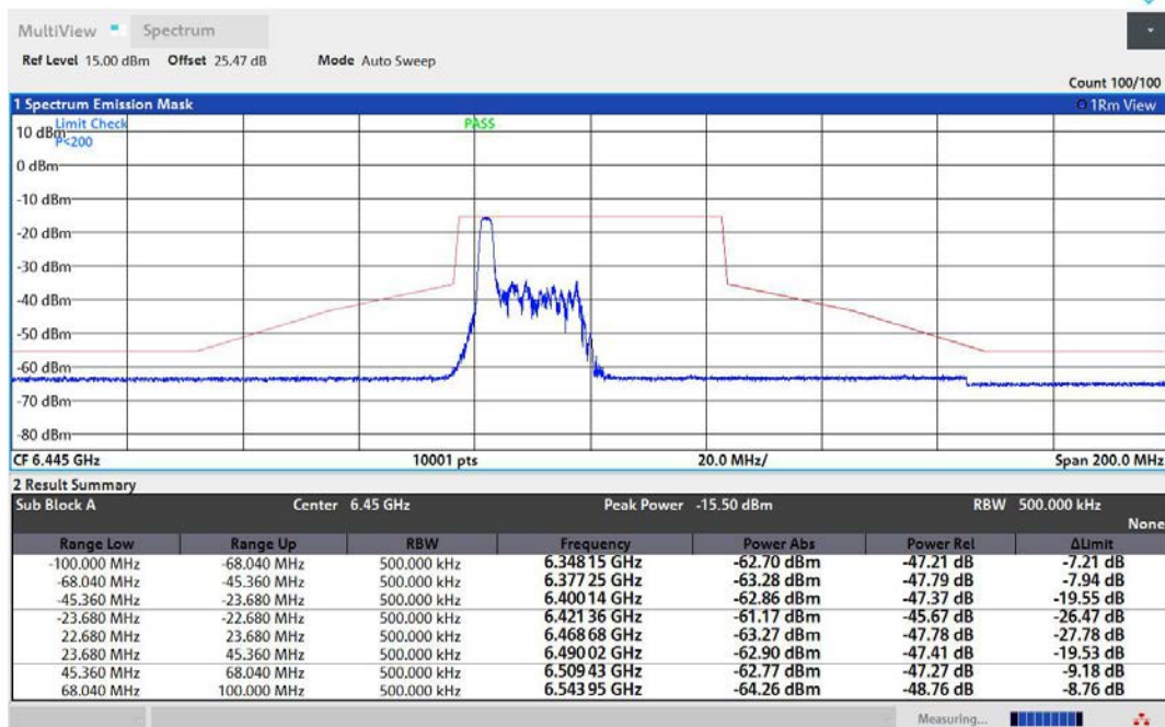
NTNV-11AX40MIMO-Ant1-6445-26Tone-RU0-PASS
