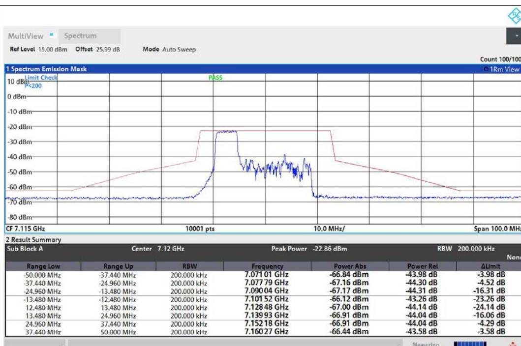
NTNV-11AX20MIMO-Ant1-7115-52Tone-RU37-PASS
