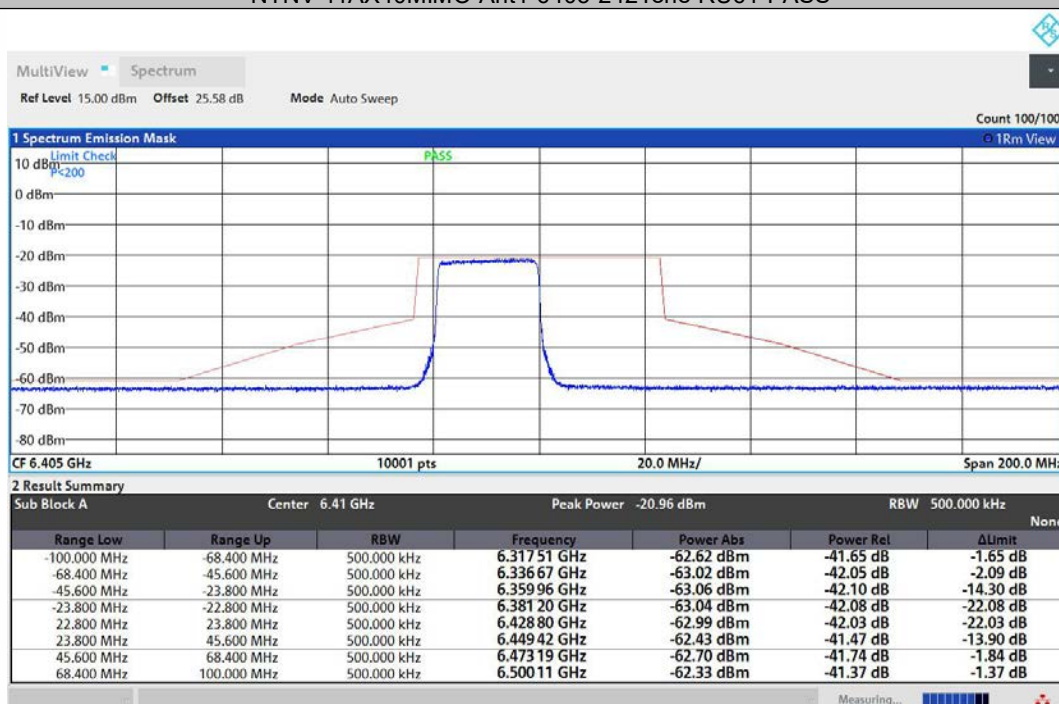
NTNV-11AX40MIMO-Ant2-6405-242Tone-RU61-PASS
