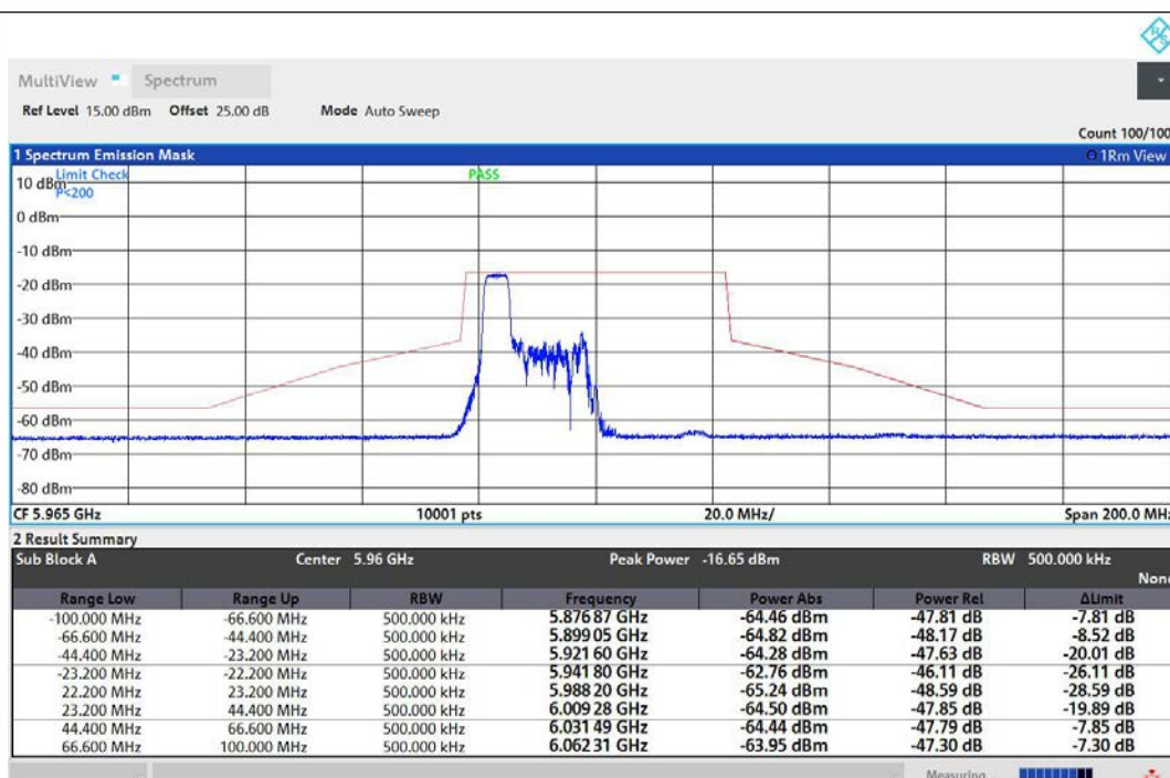
NTNV-11AX40MIMO-Ant1-5965-52Tone-RU37-PASS
