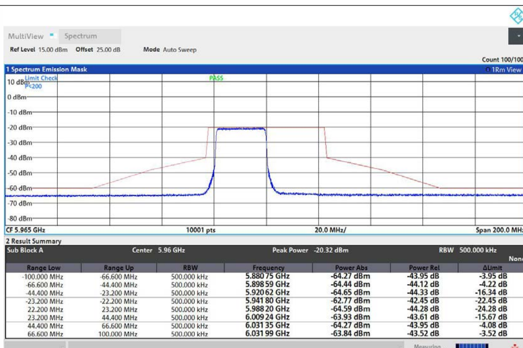
NTNV-11AX40MIMO-Ant1-5965-242Tone-RU61-PASS
