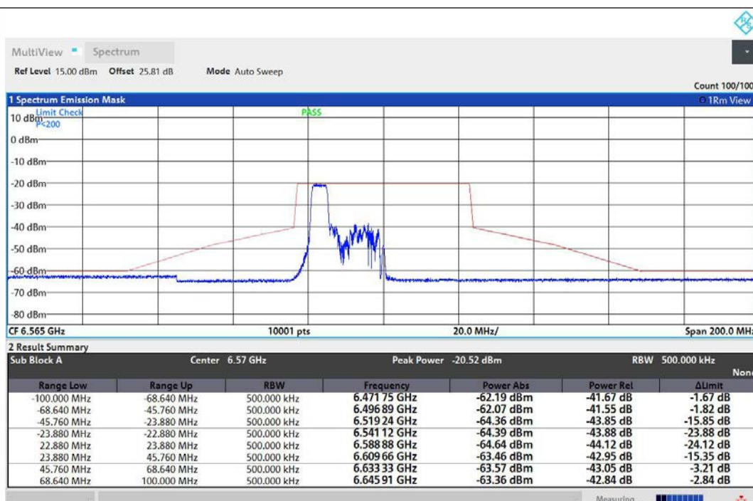
NTNV-11AX40MIMO-Ant1-6565-52Tone-RU37-PASS
