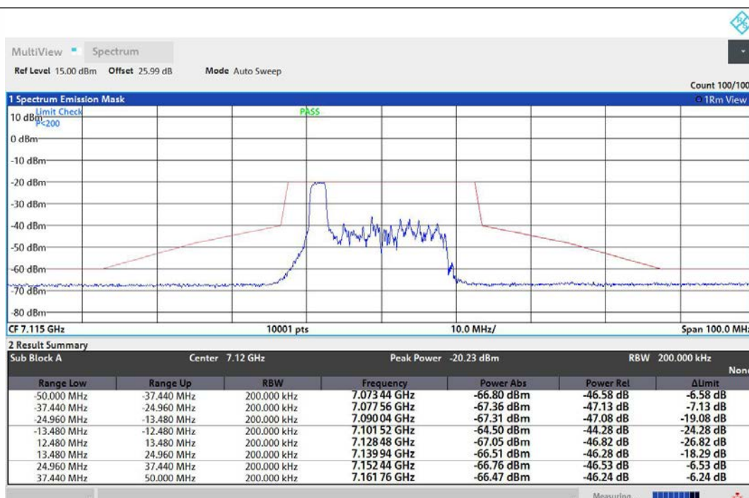
NTNV-11AX20MIMO-Ant1-7115-26Tone-RU0-PASS
