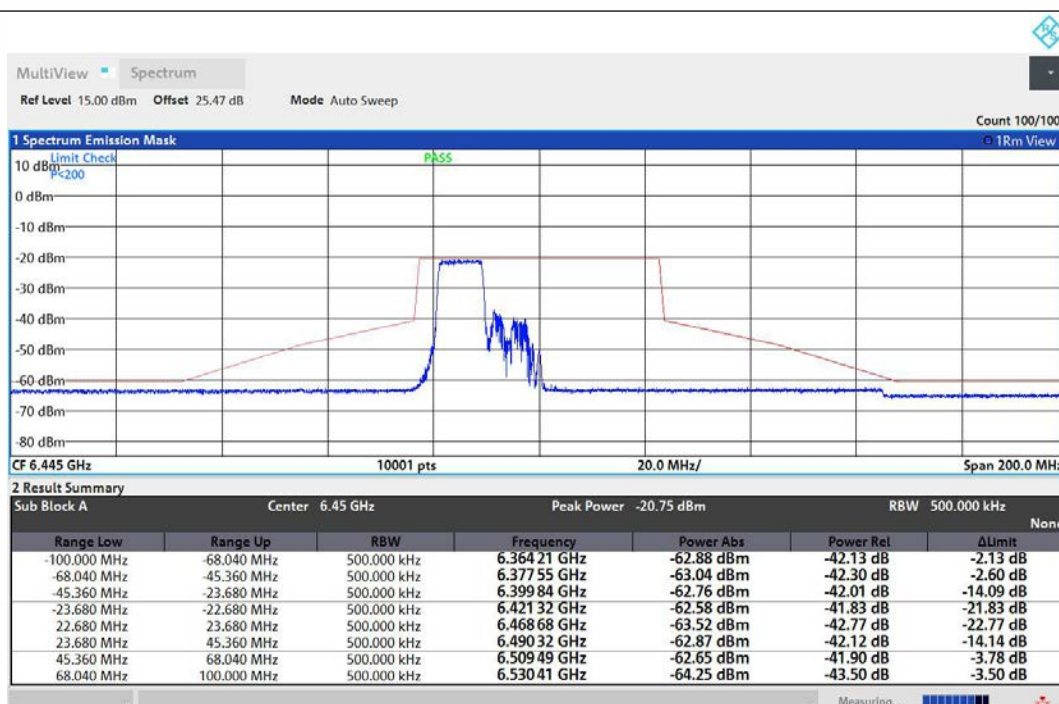
NTNV-11AX40MIMO-Ant1-6445-106Tone-RU53-PASS
