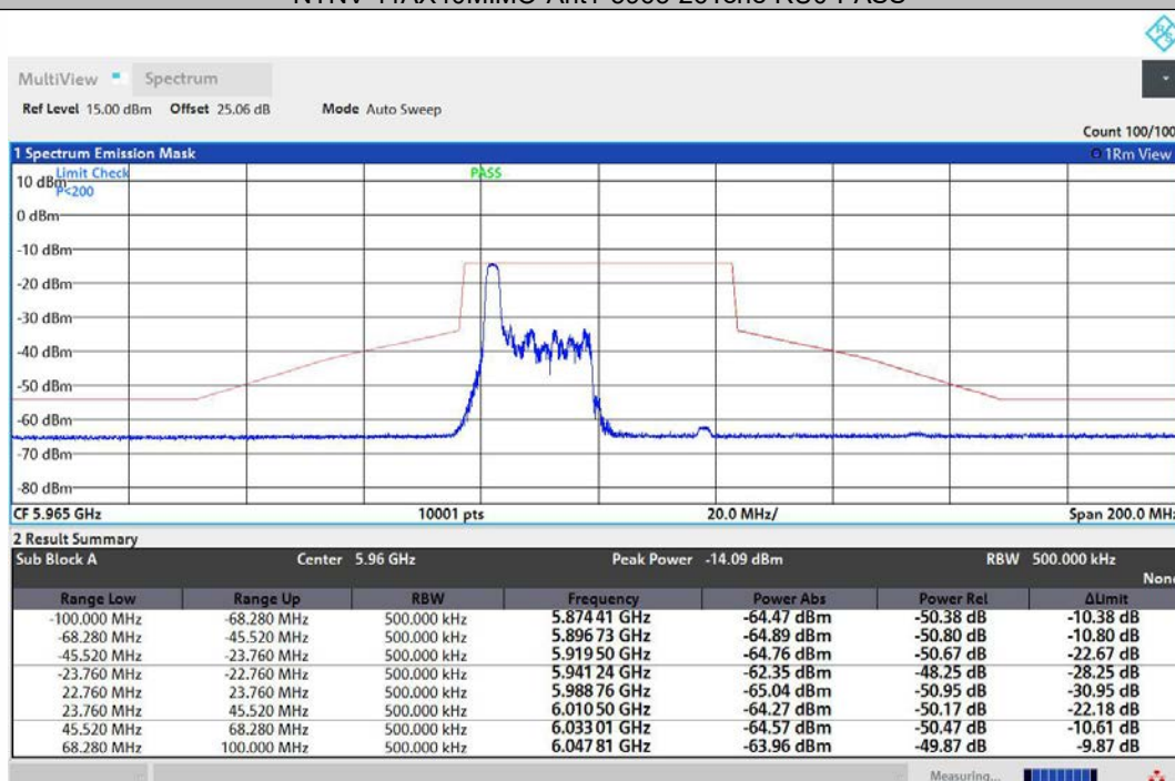
NTNV-11AX40MIMO-Ant2-5965-26Tone-RU0-PASS
