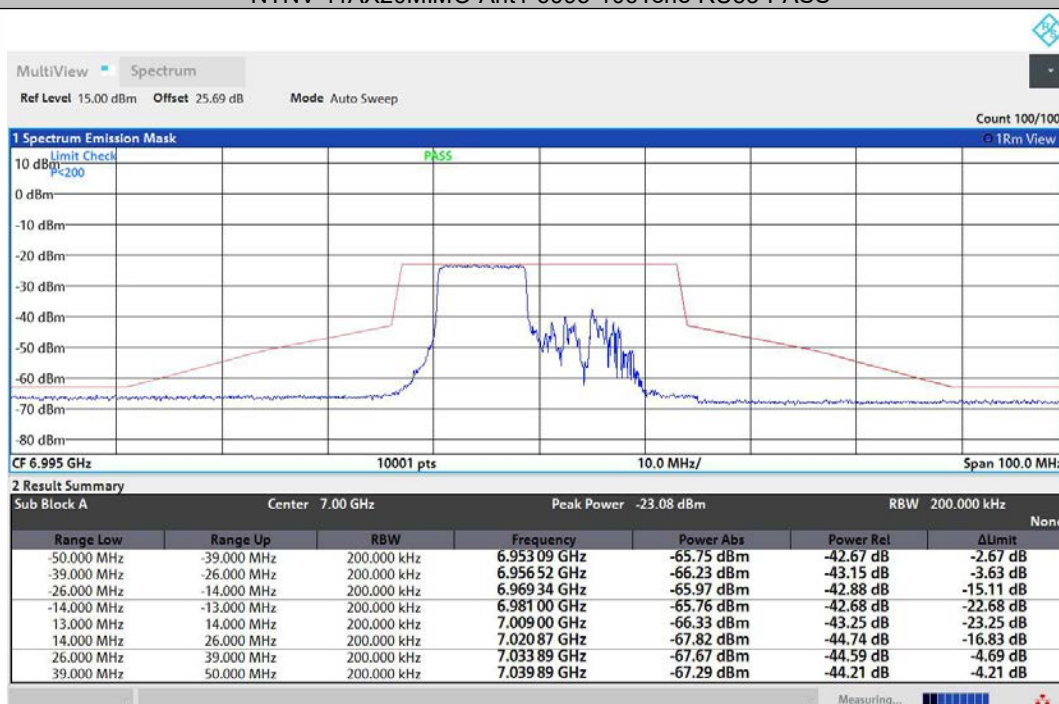
NTNV-11AX20MIMO-Ant2-6995-106Tone-RU53-PASS
