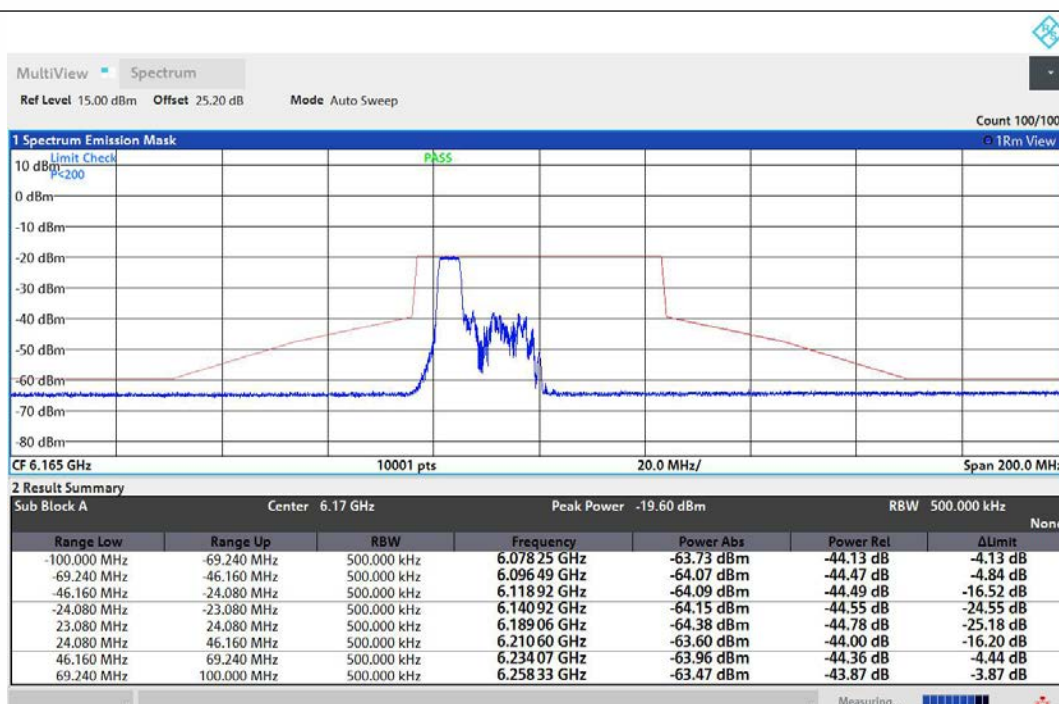
NTNV-11AX40MIMO-Ant1-6165-52Tone-RU37-PASS
