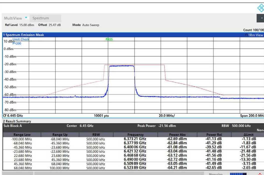
NTNV-11AX40MIMO-Ant1-6445-242Tone-RU61-PASS
