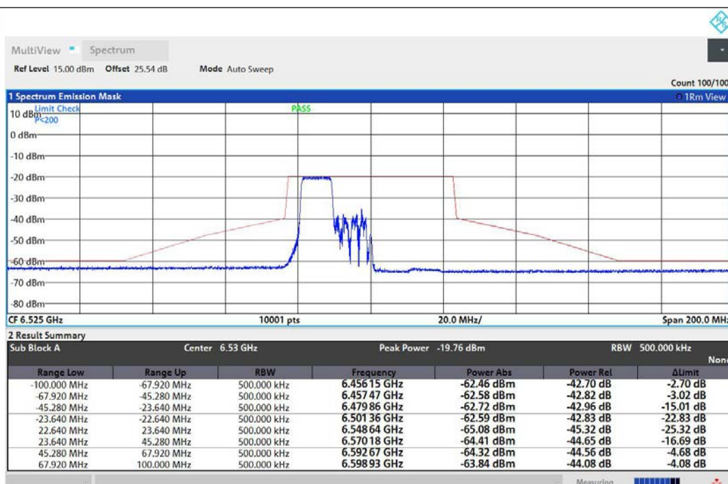
NTNV-11AX40MIMO-Ant1-6525-106Tone-RU53-PASS
