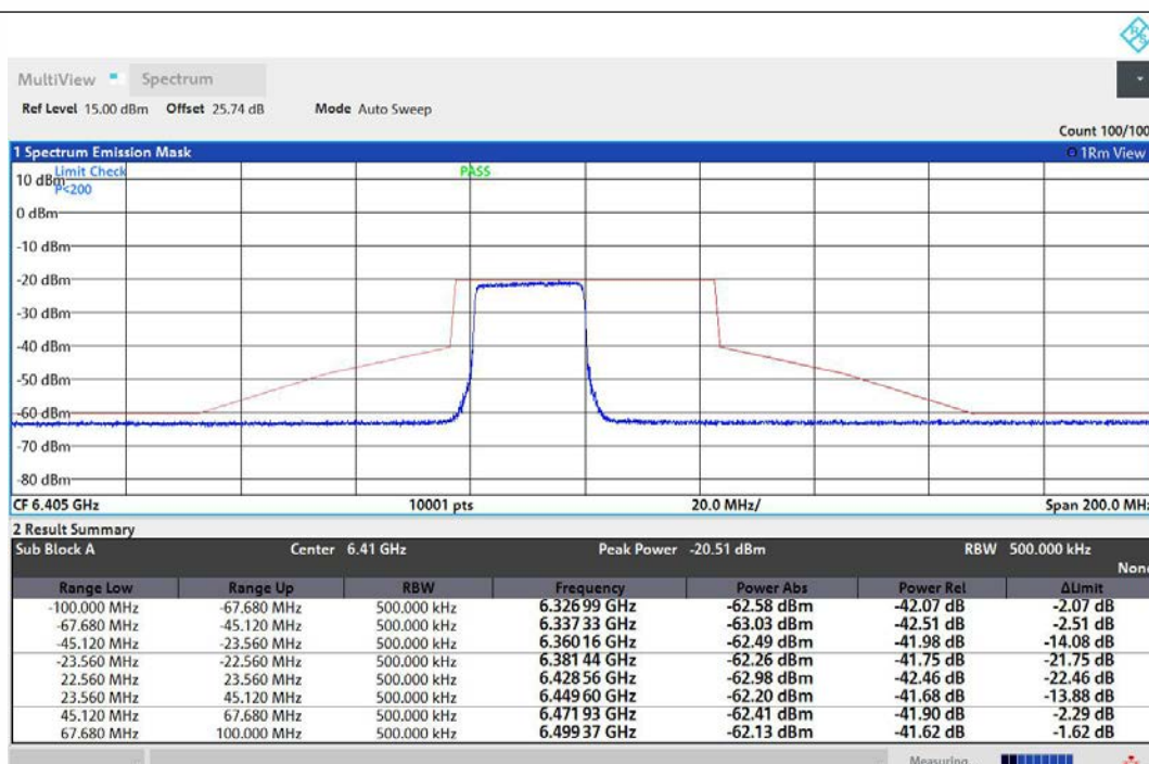
NTNV-11AX40MIMO-Ant1-6405-242Tone-RU61-PASS
