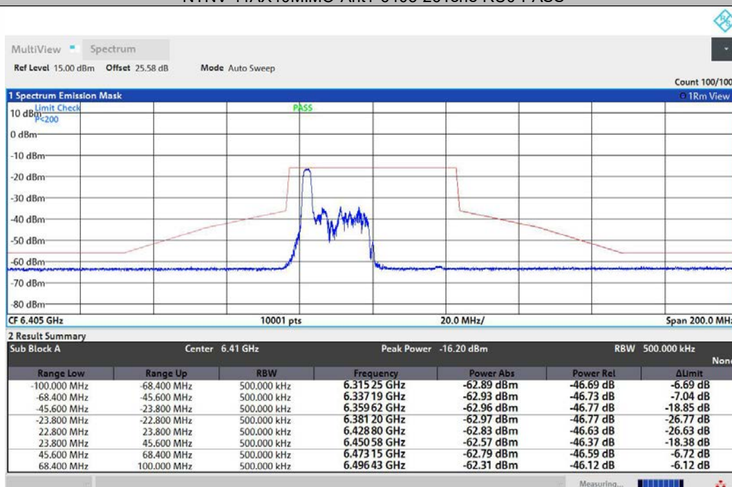
NTNV-11AX40MIMO-Ant2-6405-26Tone-RU0-PASS
