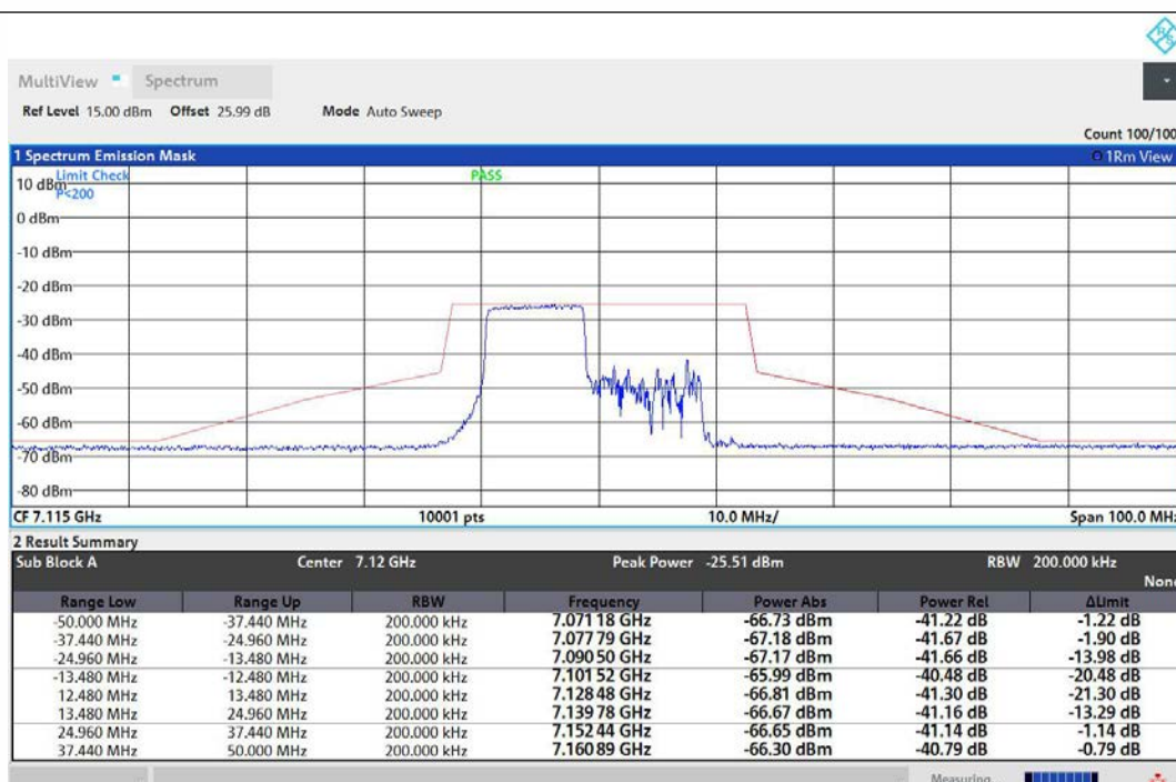
NTNV-11AX20MIMO-Ant1-7115-106Tone-RU53-PASS
