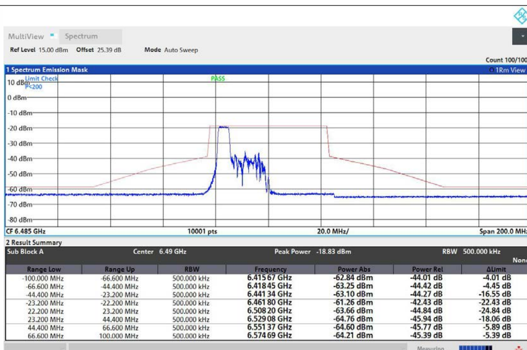
NTNV-11AX40MIMO-Ant1-6485-52Tone-RU37-PASS
