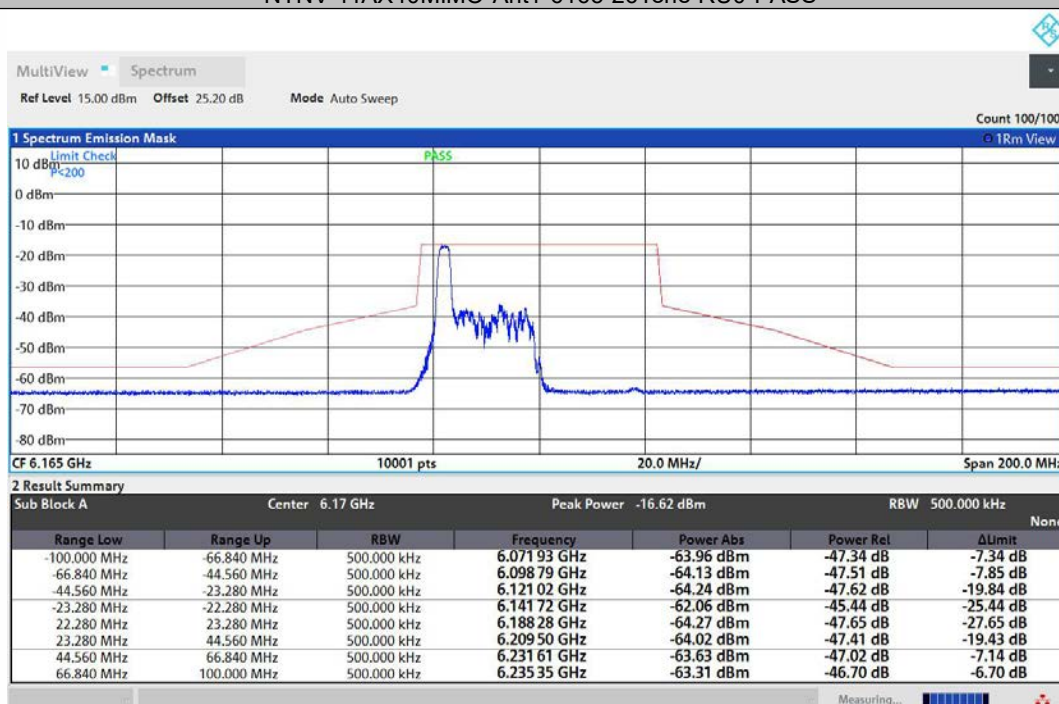
NTNV-11AX40MIMO-Ant2-6165-26Tone-RU0-PASS
