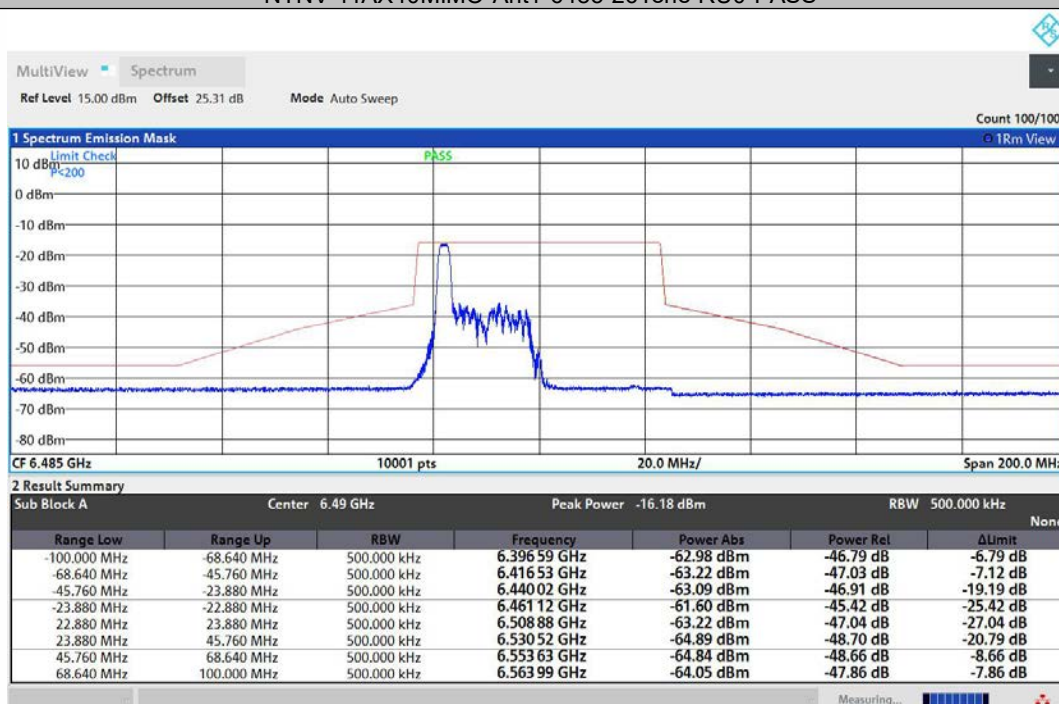
NTNV-11AX40MIMO-Ant2-6485-26Tone-RU0-PASS
