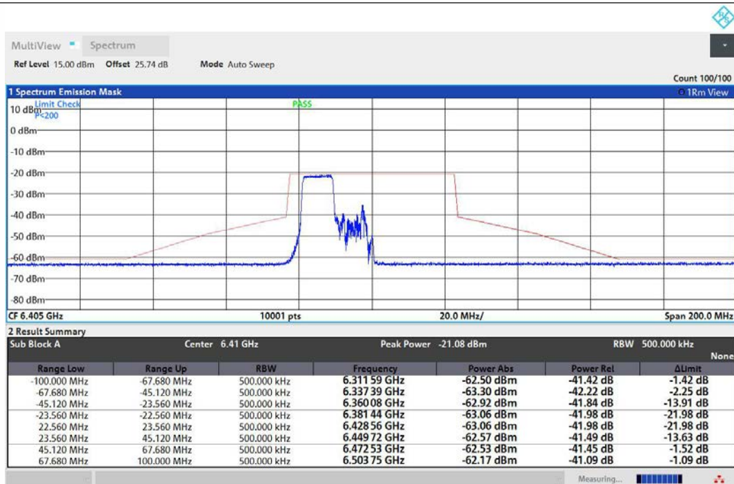
NTNV-11AX40MIMO-Ant1-6405-106Tone-RU53-PASS
