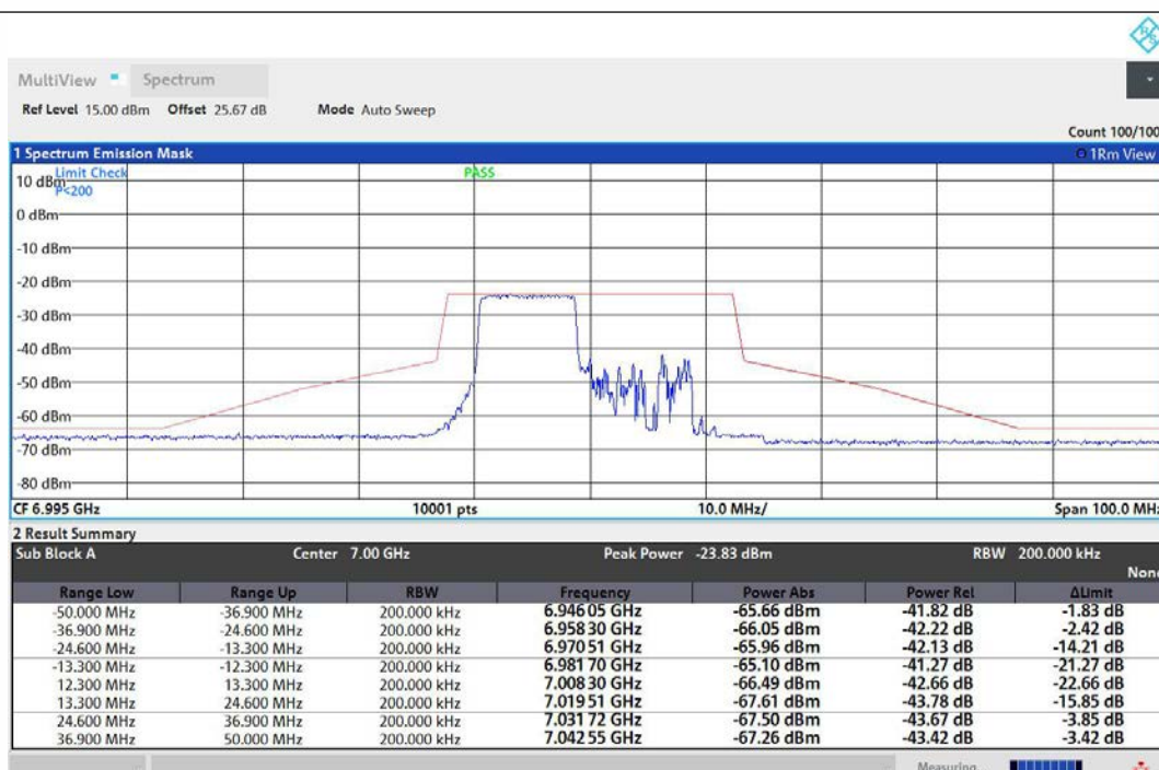
NTNV-11AX20MIMO-Ant1-6995-106Tone-RU53-PASS
