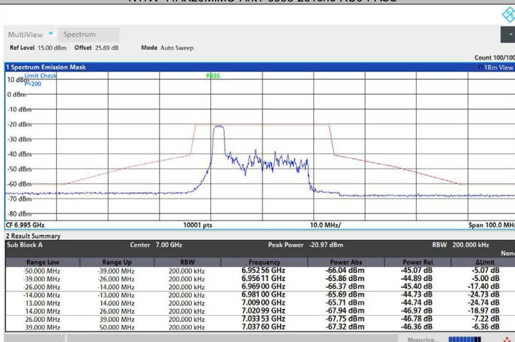
NTNV-11AX20MIMO-Ant2-6995-26Tone-RU0-PASS
