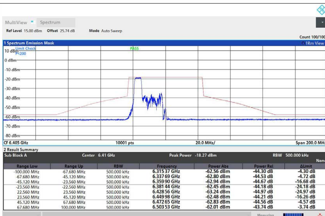
NTNV-11AX40MIMO-Ant1-6405-52Tone-RU37-PASS
