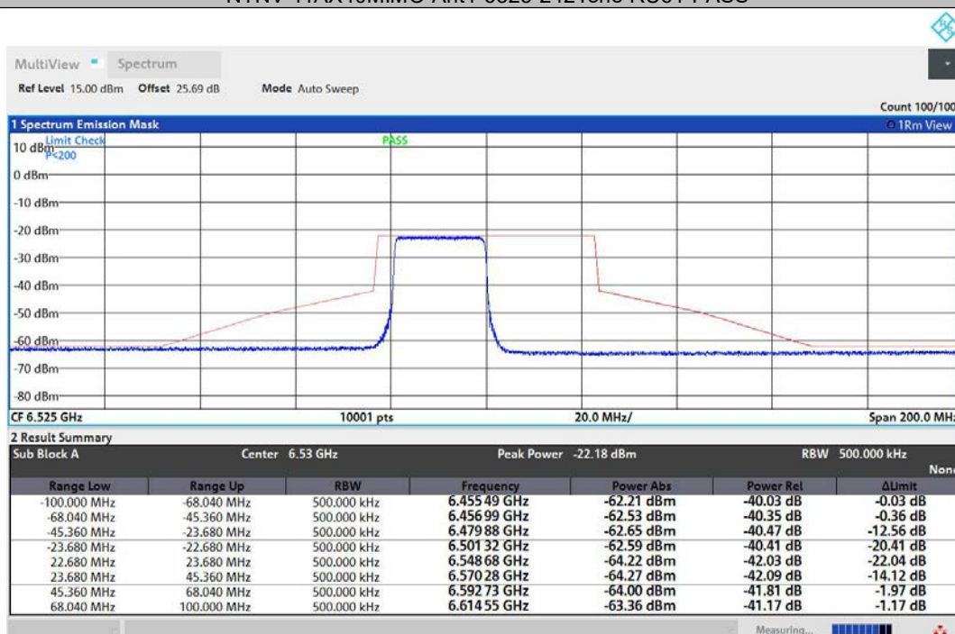
NTNV-11AX40MIMO-Ant2-6525-242Tone-RU61-PASS
