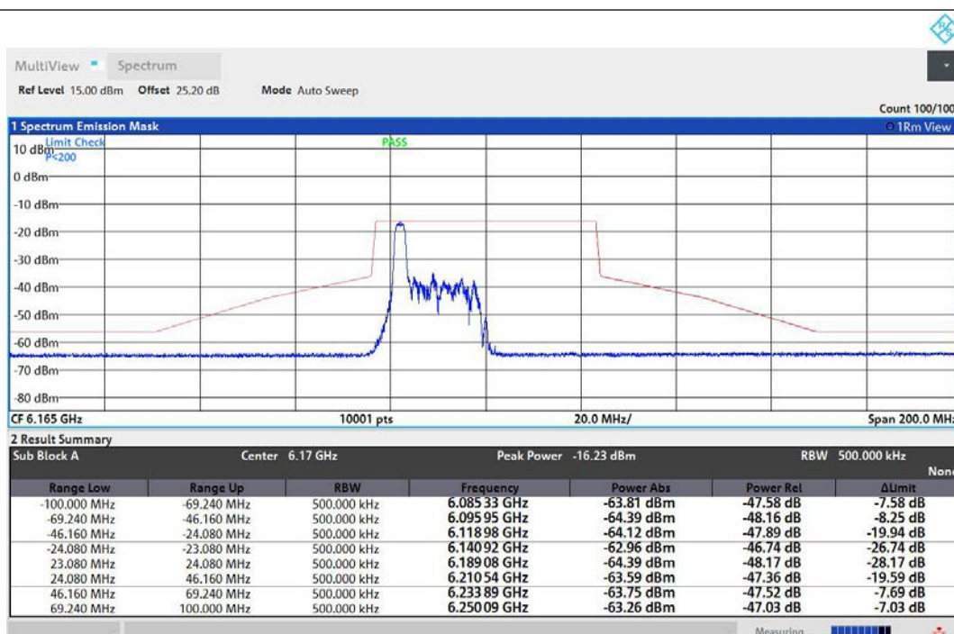
NTNV-11AX40MIMO-Ant1-6165-26Tone-RU0-PASS
