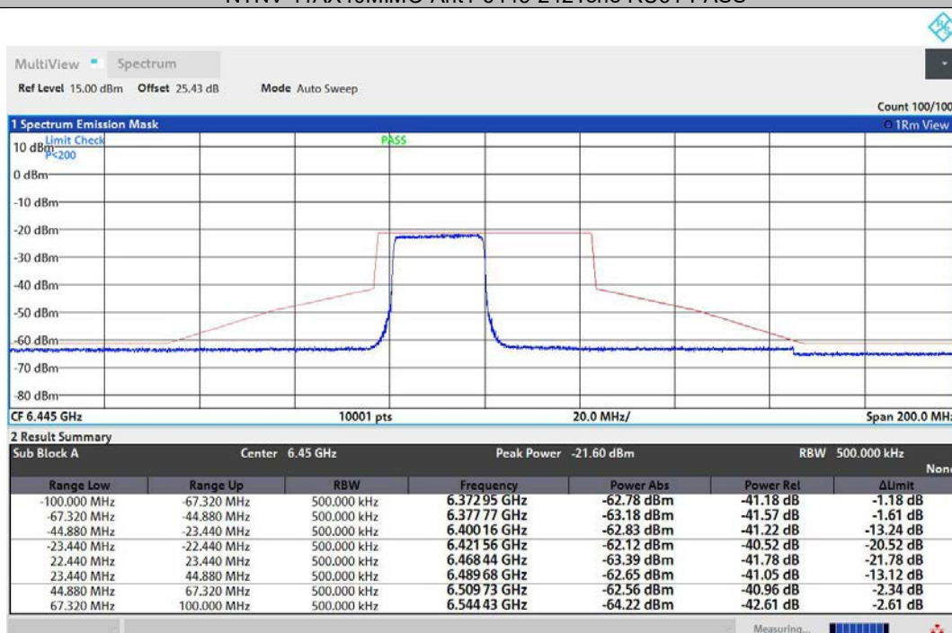
NTNV-11AX40MIMO-Ant2-6445-242Tone-RU61-PASS
