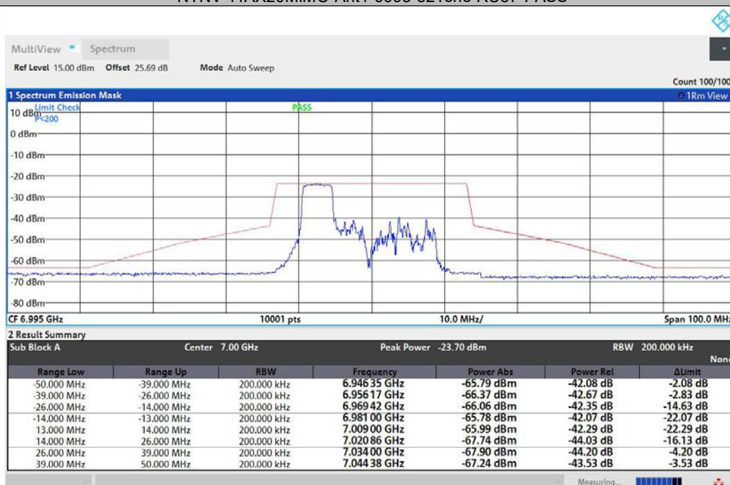
NTNV-11AX20MIMO-Ant2-6995-52Tone-RU37-PASS
