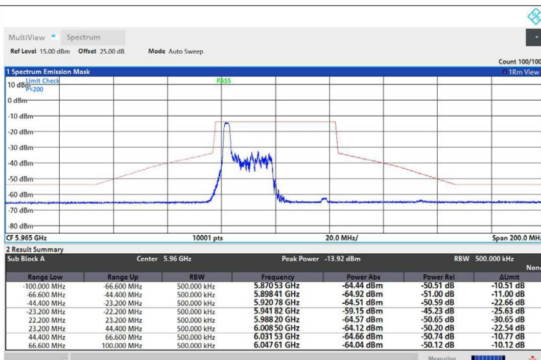
NTNV-11AX40MIMO-Ant1-5965-26Tone-RU0-PASS
