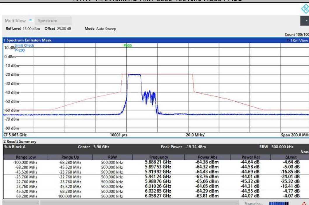
NTNV-11AX40MIMO-Ant2-5965-106Tone-RU53-PASS
