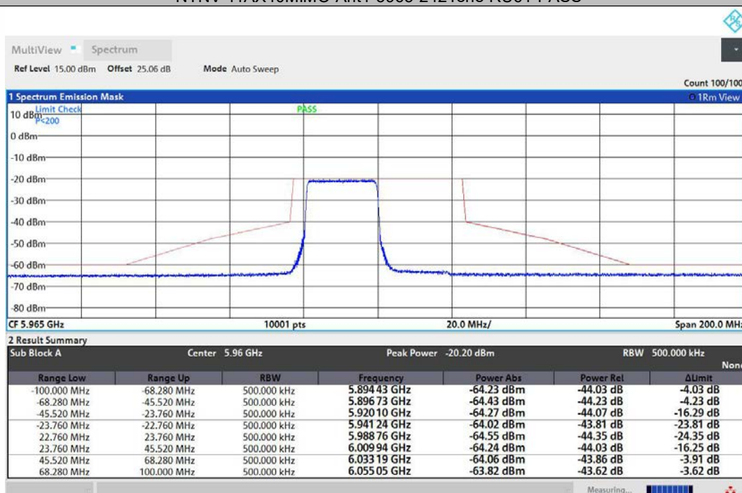
NTNV-11AX40MIMO-Ant2-5965-242Tone-RU61-PASS
