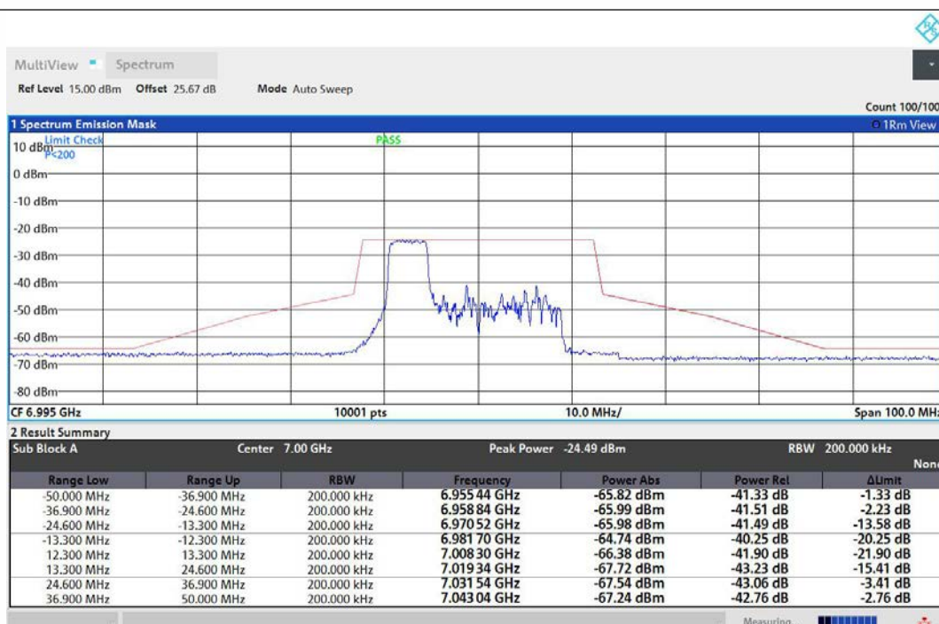
NTNV-11AX20MIMO-Ant1-6995-52Tone-RU37-PASS
