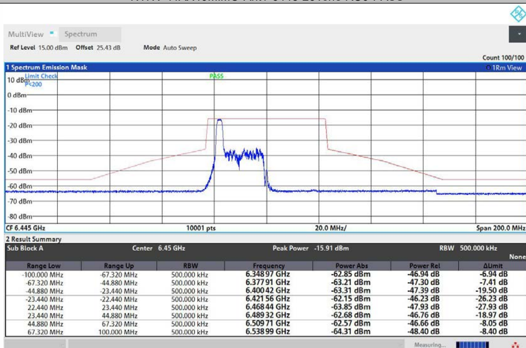
NTNV-11AX40MIMO-Ant2-6445-26Tone-RU0-PASS
