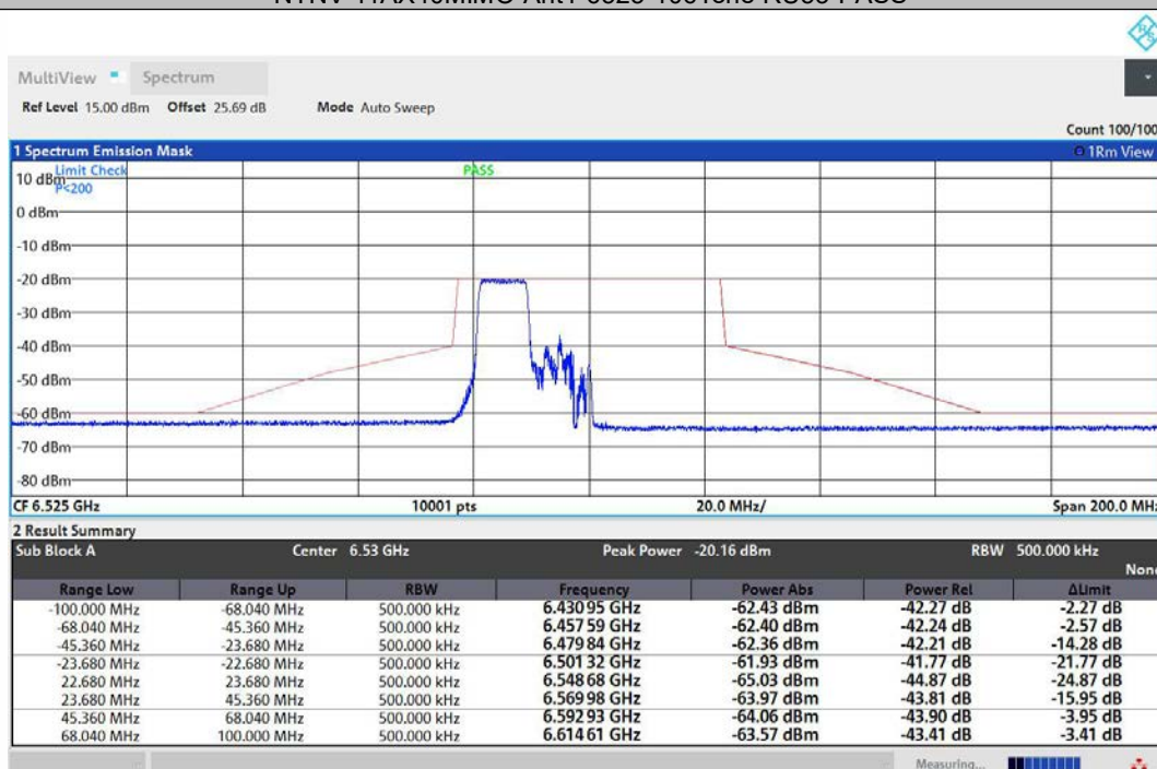
NTNV-11AX40MIMO-Ant2-6525-106Tone-RU53-PASS
