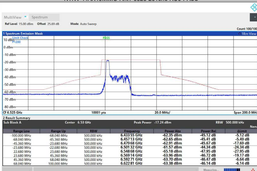
NTNV-11AX40MIMO-Ant2-6525-26Tone-RU0-PASS
