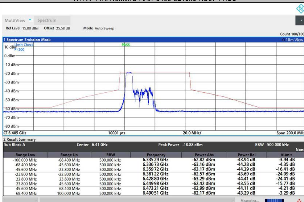
NTNV-11AX40MIMO-Ant2-6405-52Tone-RU37-PASS
