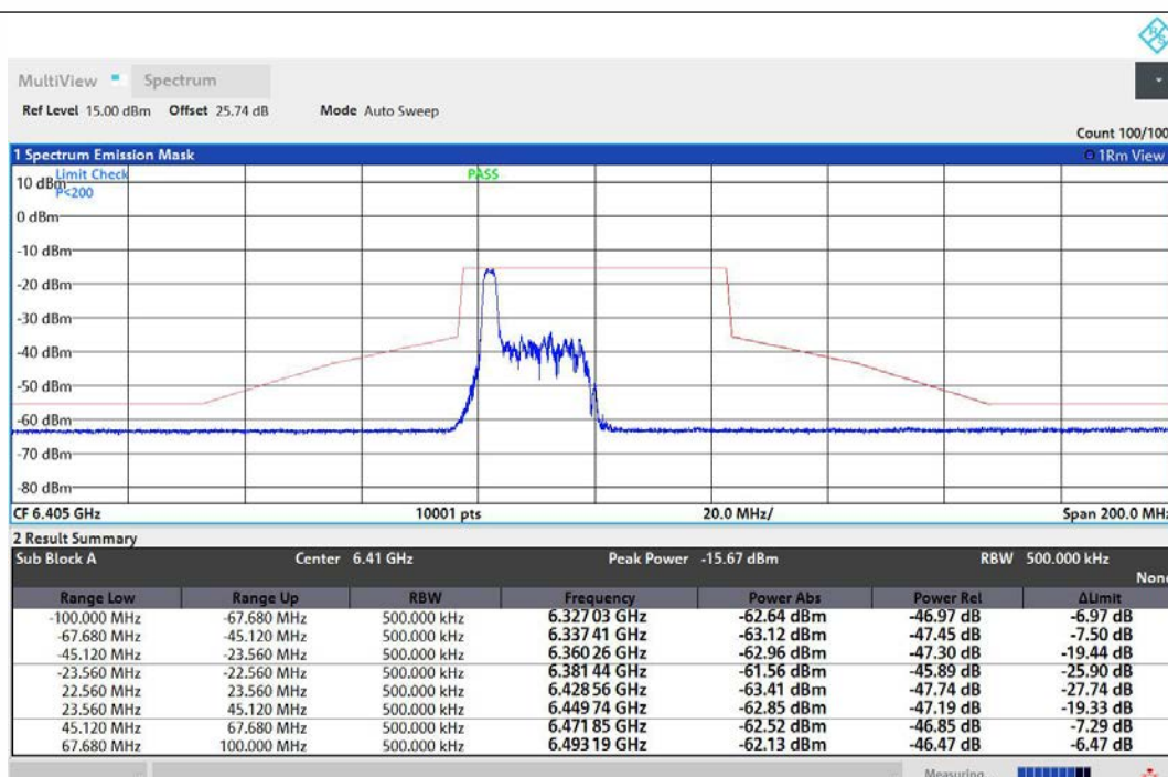
NTNV-11AX40MIMO-Ant1-6405-26Tone-RU0-PASS
