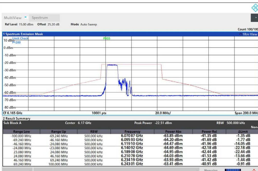
NTNV-11AX40MIMO-Ant1-6165-106Tone-RU53-PASS
