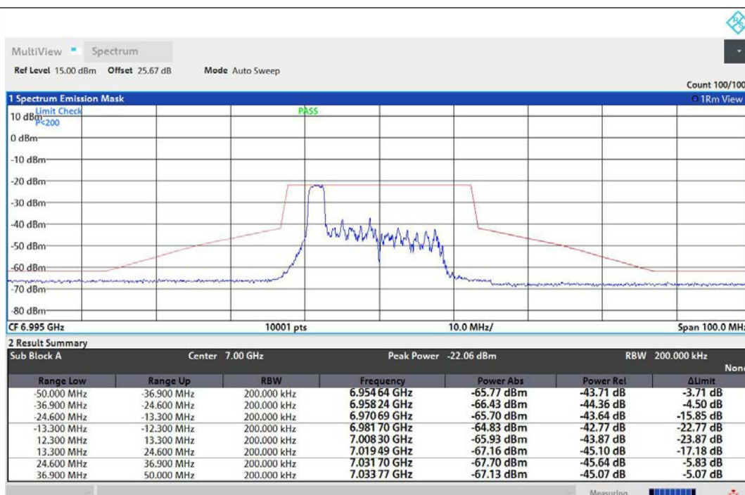
NTNV-11AX20MIMO-Ant1-6995-26Tone-RU0-PASS
