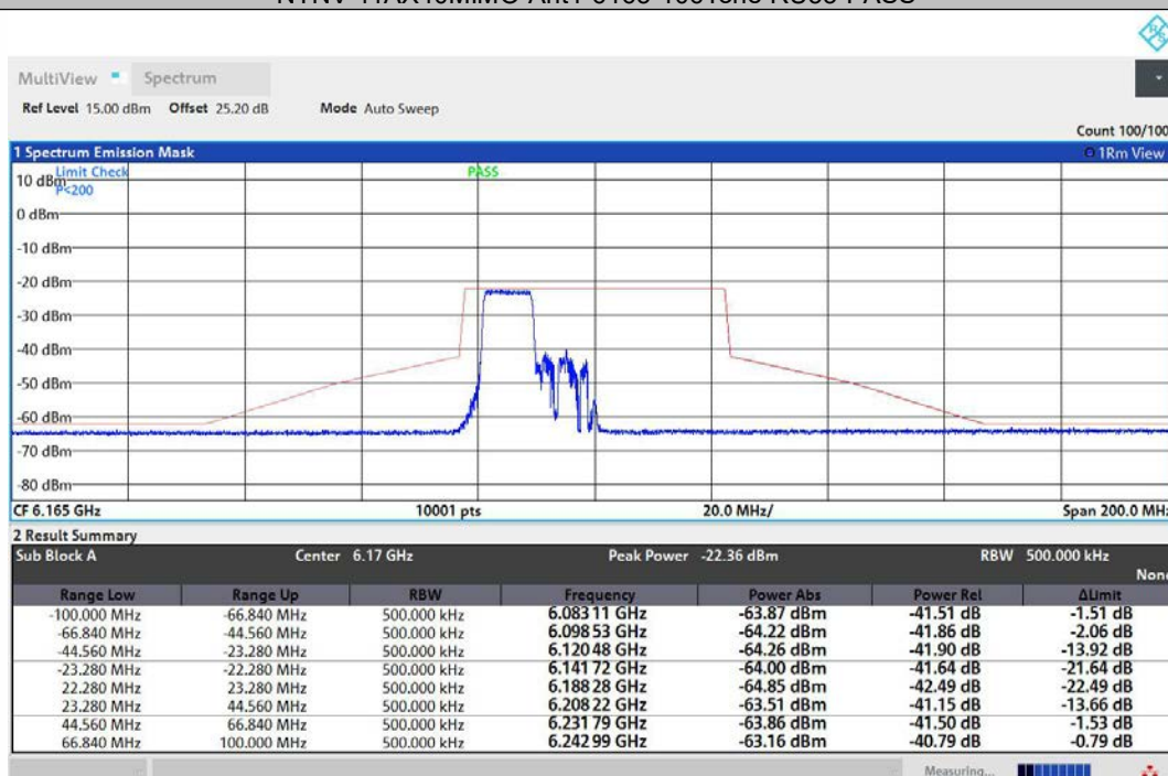
NTNV-11AX40MIMO-Ant2-6165-106Tone-RU53-PASS
