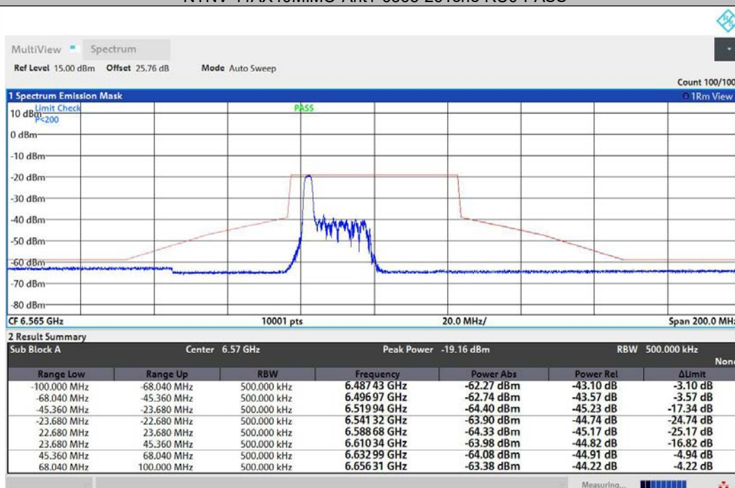
NTNV-11AX40MIMO-Ant2-6565-26Tone-RU0-PASS
