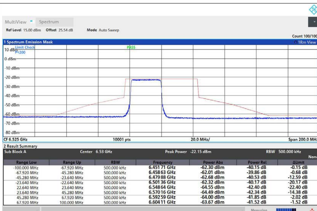
NTNV-11AX40MIMO-Ant1-6525-242Tone-RU61-PASS
