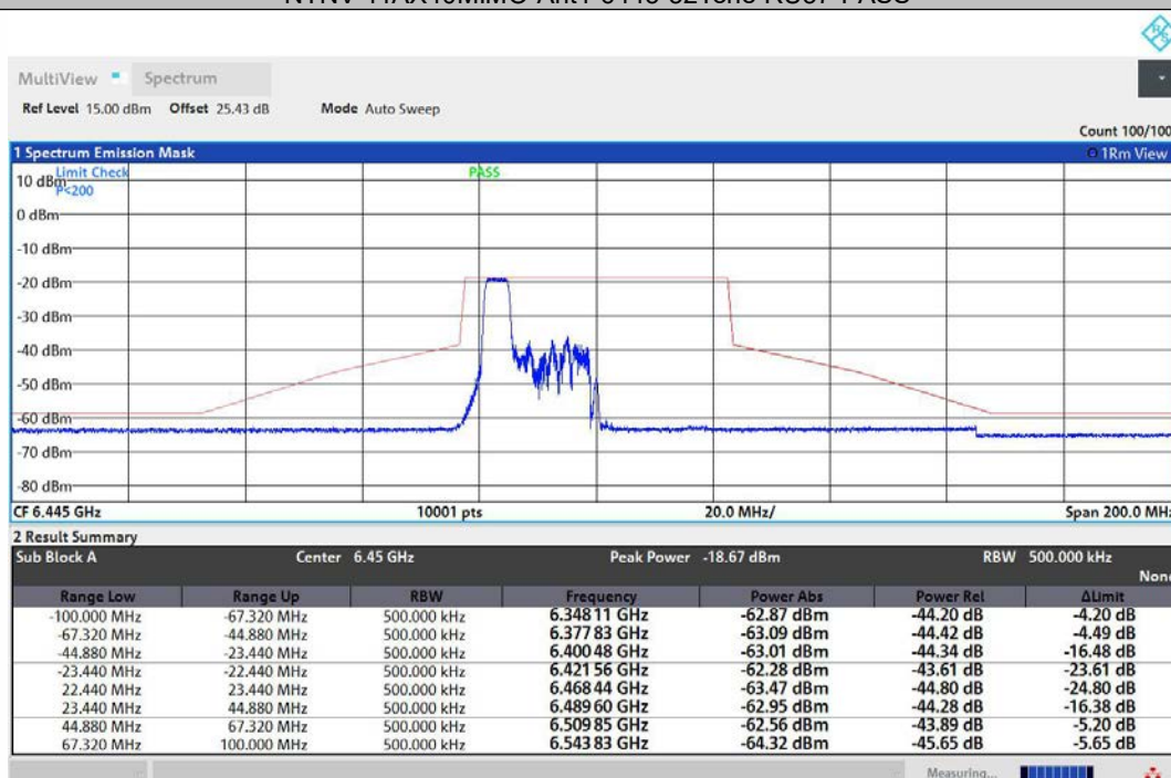
NTNV-11AX40MIMO-Ant2-6445-52Tone-RU37-PASS
