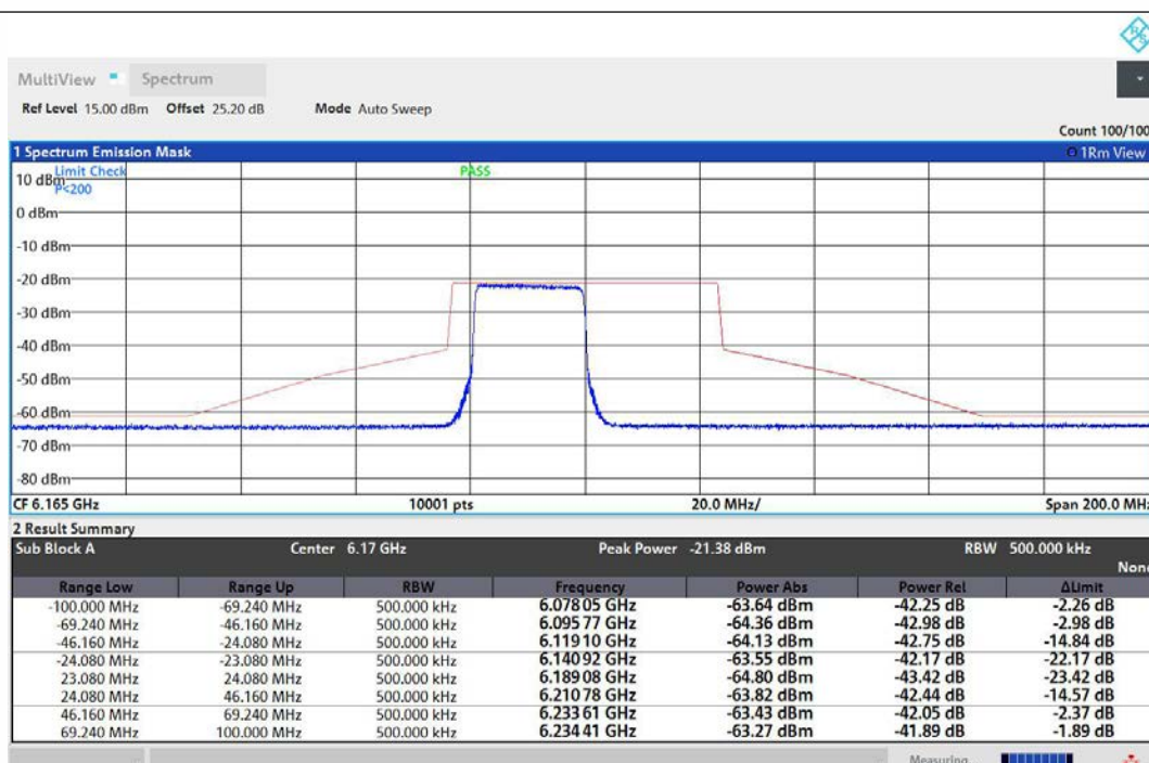
NTNV-11AX40MIMO-Ant1-6165-242Tone-RU61-PASS
