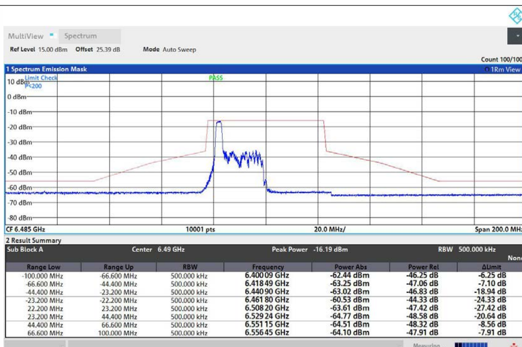
NTNV-11AX40MIMO-Ant1-6485-26Tone-RU0-PASS
