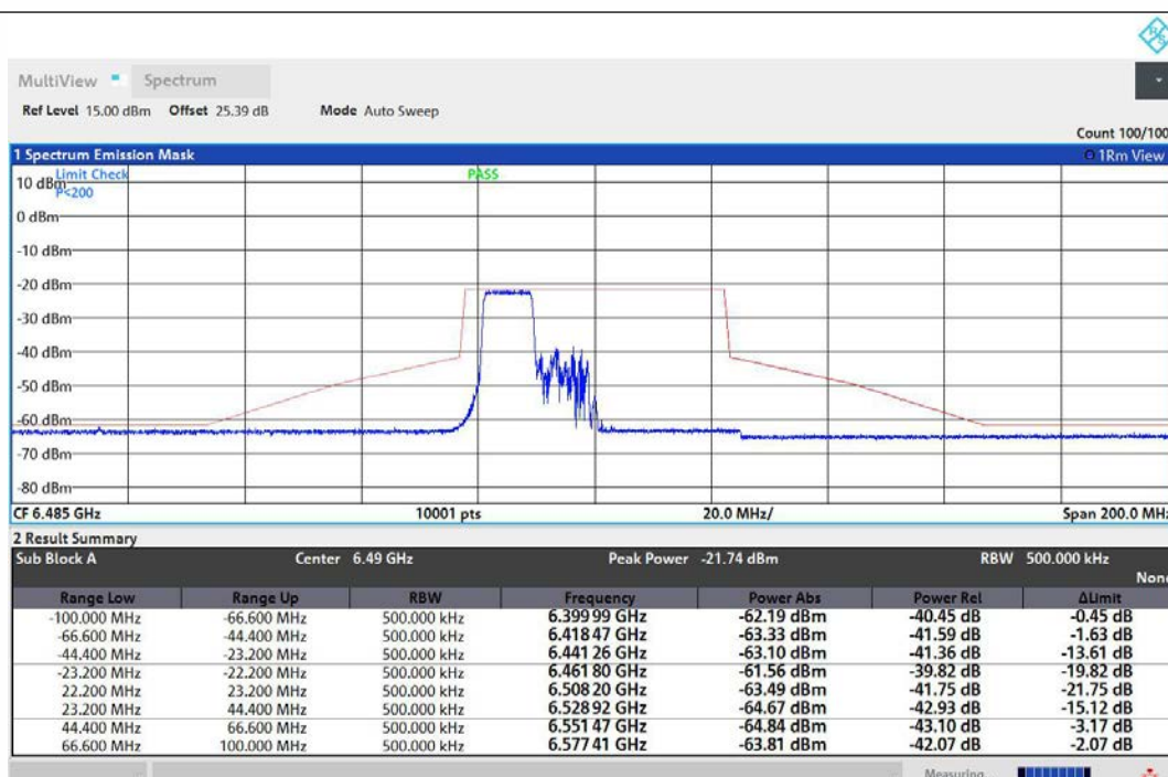
NTNV-11AX40MIMO-Ant1-6485-106Tone-RU53-PASS
