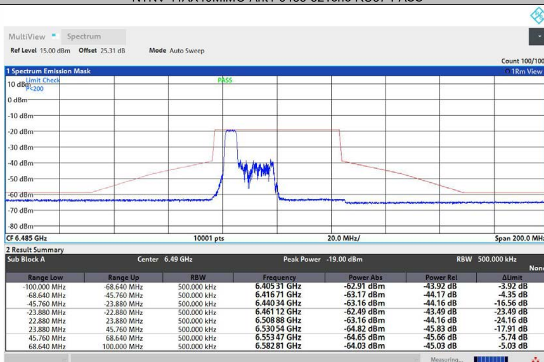
NTNV-11AX40MIMO-Ant2-6485-52Tone-RU37-PASS
