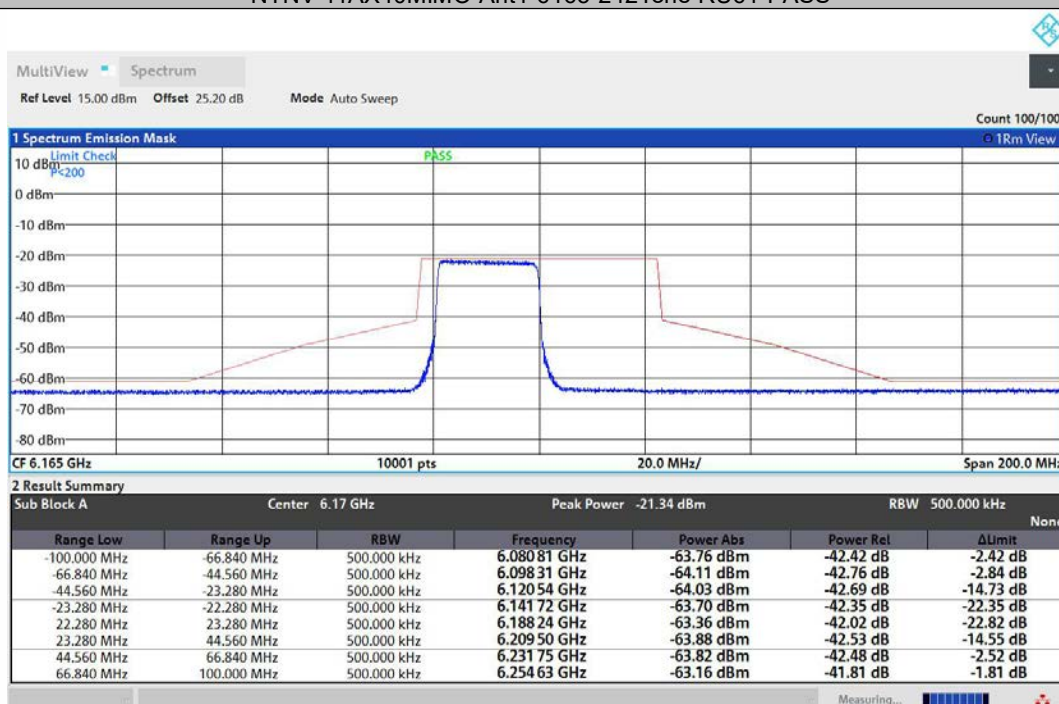
NTNV-11AX40MIMO-Ant2-6165-242Tone-RU61-PASS
