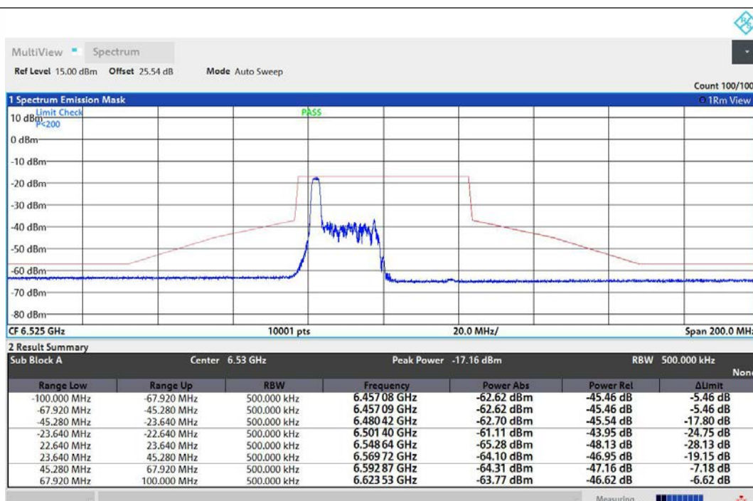
NTNV-11AX40MIMO-Ant1-6525-26Tone-RU0-PASS
