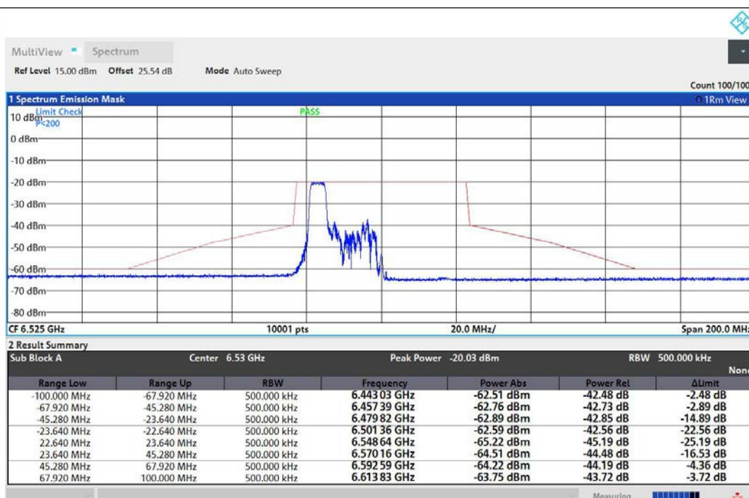
NTNV-11AX40MIMO-Ant1-6525-52Tone-RU37-PASS
