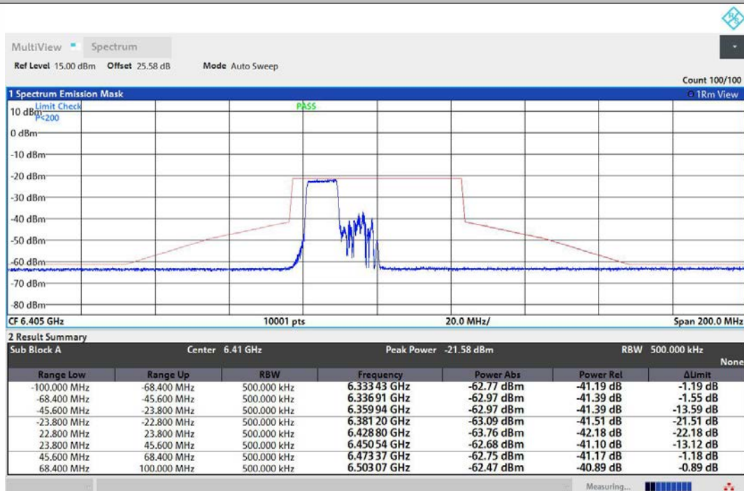
NTNV-11AX40MIMO-Ant2-6405-106Tone-RU53-PASS
