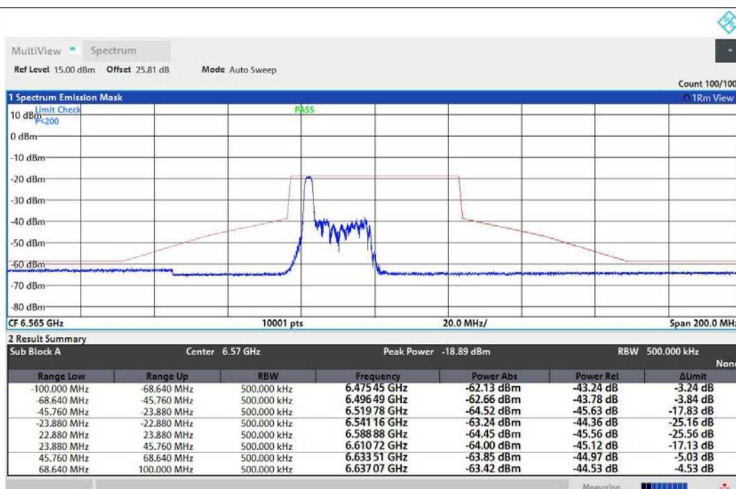
NTNV-11AX40MIMO-Ant1-6565-26Tone-RU0-PASS
