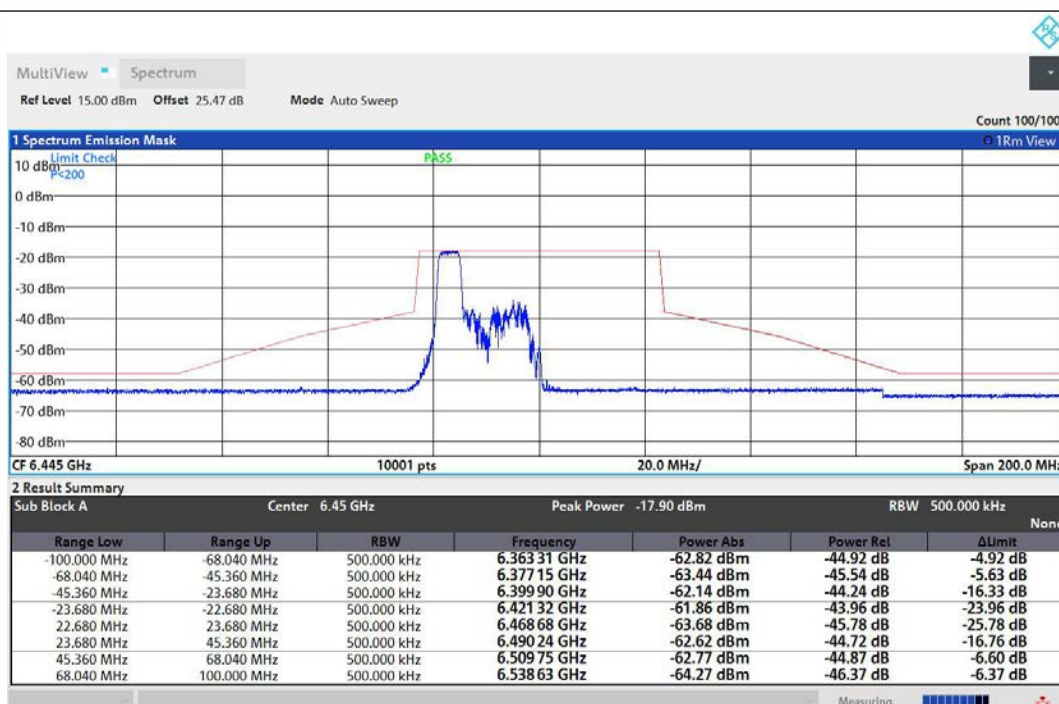
NTNV-11AX40MIMO-Ant1-6445-52Tone-RU37-PASS
