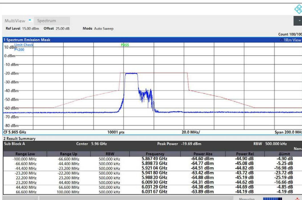
NTNV-11AX40MIMO-Ant1-5965-106Tone-RU53-PASS
