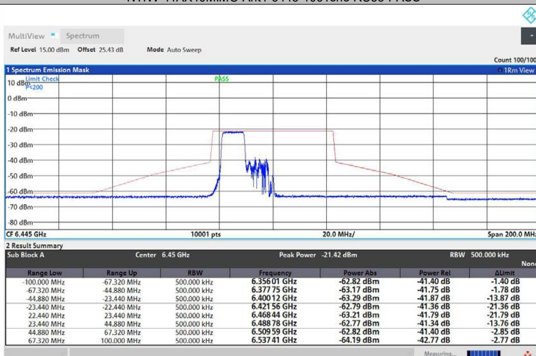
NTNV-11AX40MIMO-Ant2-6445-106Tone-RU53-PASS
