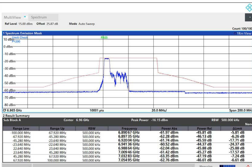
NTNV-11AX40MIMO-Ant1-6965-52Tone-RU37-PASS
