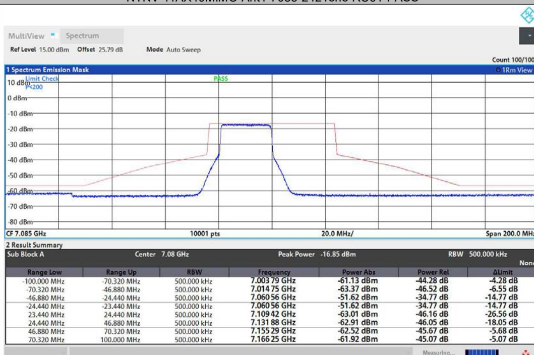
NTNV-11AX40MIMO-Ant2-7085-242Tone-RU61-PASS
