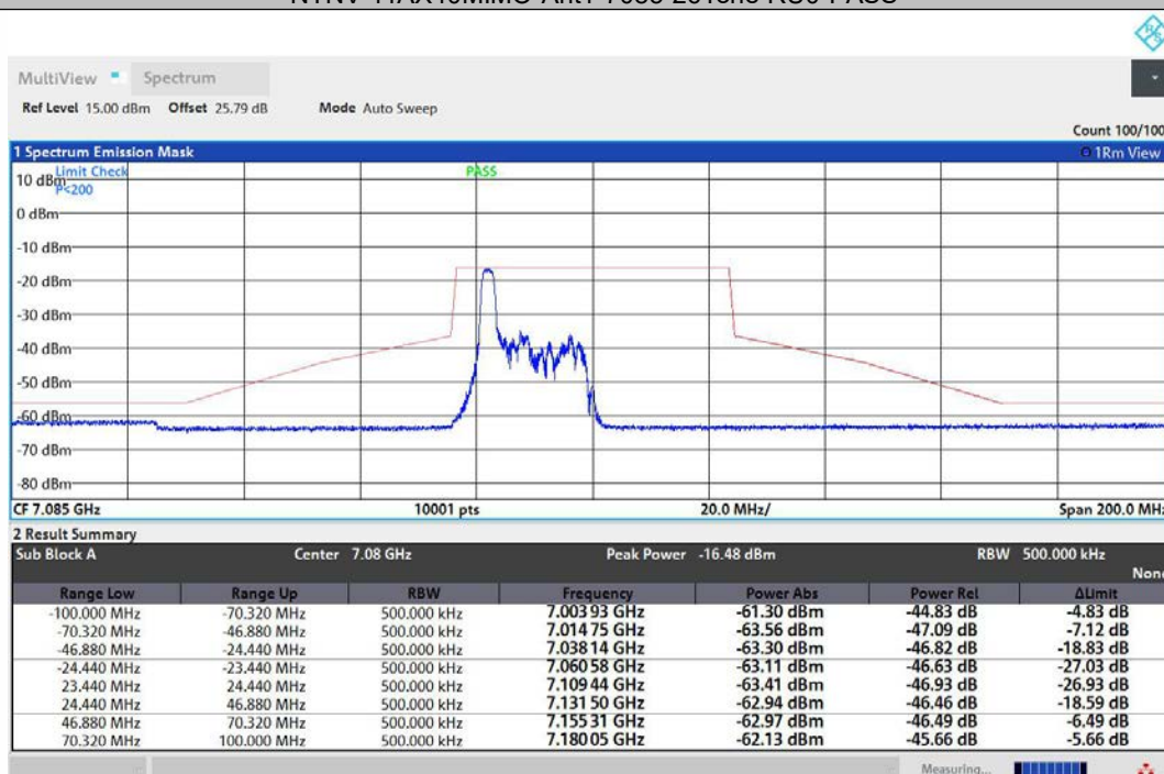
NTNV-11AX40MIMO-Ant2-7085-26Tone-RU0-PASS
