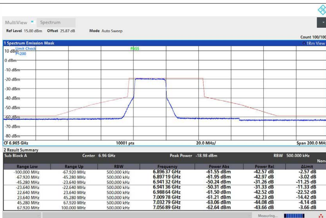
NTNV-11AX40MIMO-Ant1-6965-242Tone-RU61-PASS
