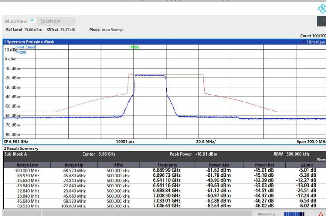
NTNV-11AX40MIMO-Ant2-6965-242Tone-RU61-PASS
