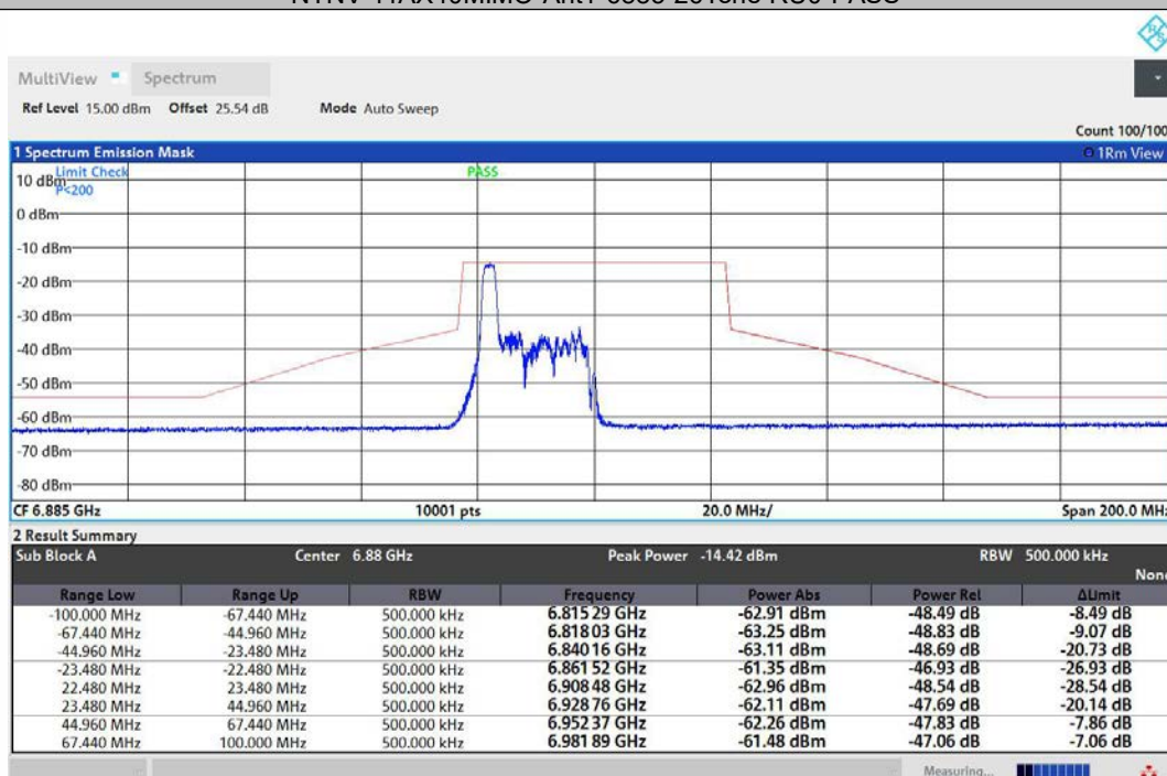
NTNV-11AX40MIMO-Ant2-6885-26Tone-RU0-PASS
