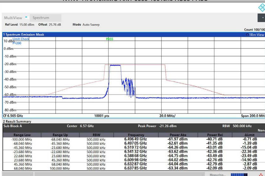
NTNV-11AX40MIMO-Ant2-6565-106Tone-RU53-PASS
