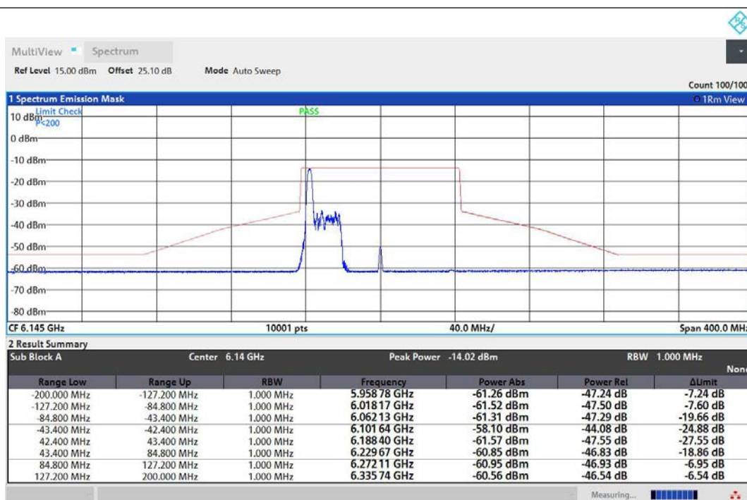
NTNV-11AX80MIMO-Ant1-6145-26Tone-RU0-PASS
