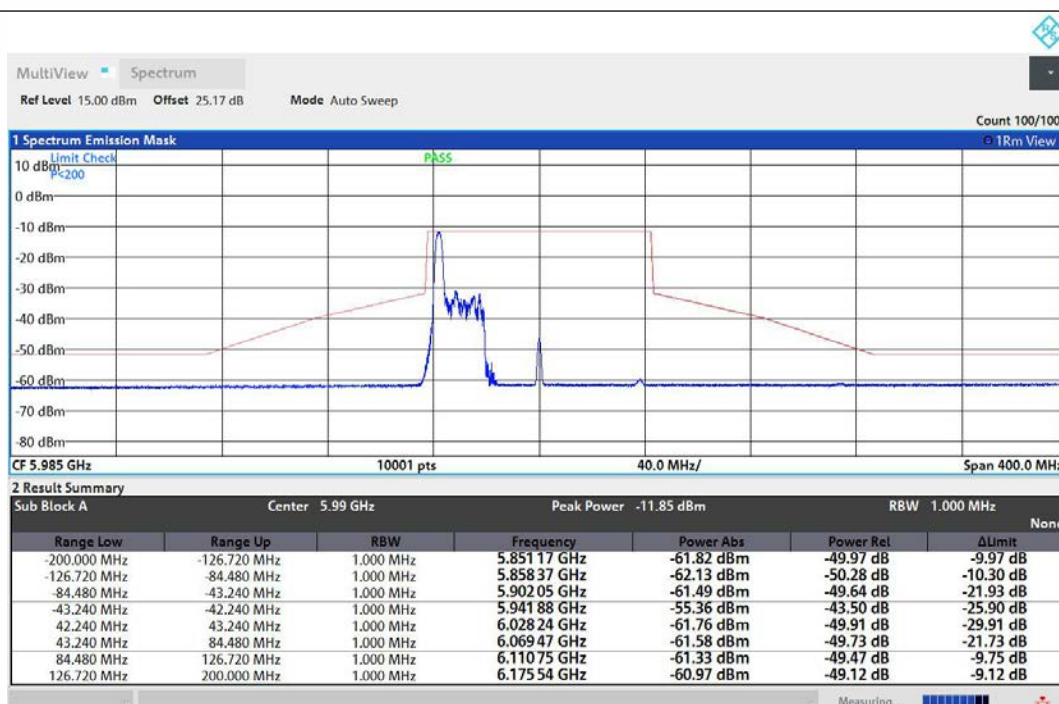
NTNV-11AX80MIMO-Ant1-5985-26Tone-RU0-PASS
