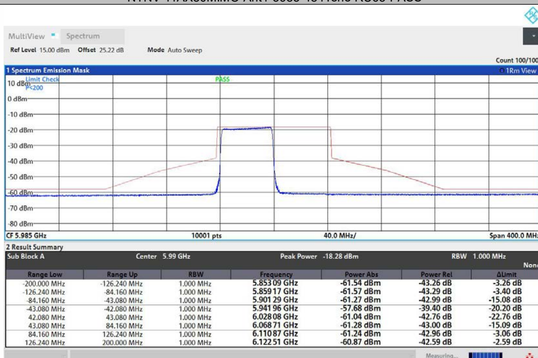
NTNV-11AX80MIMO-Ant2-5985-484Tone-RU65-PASS
