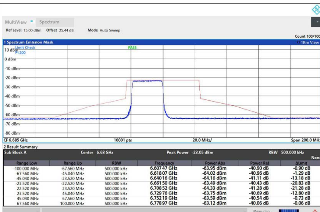
NTNV-11AX40MIMO-Ant1-6685-242Tone-RU61-PASS
