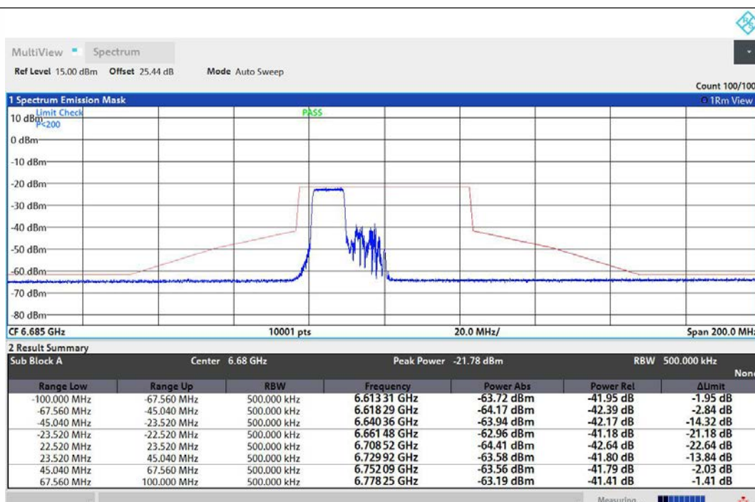
NTNV-11AX40MIMO-Ant1-6685-106Tone-RU53-PASS
