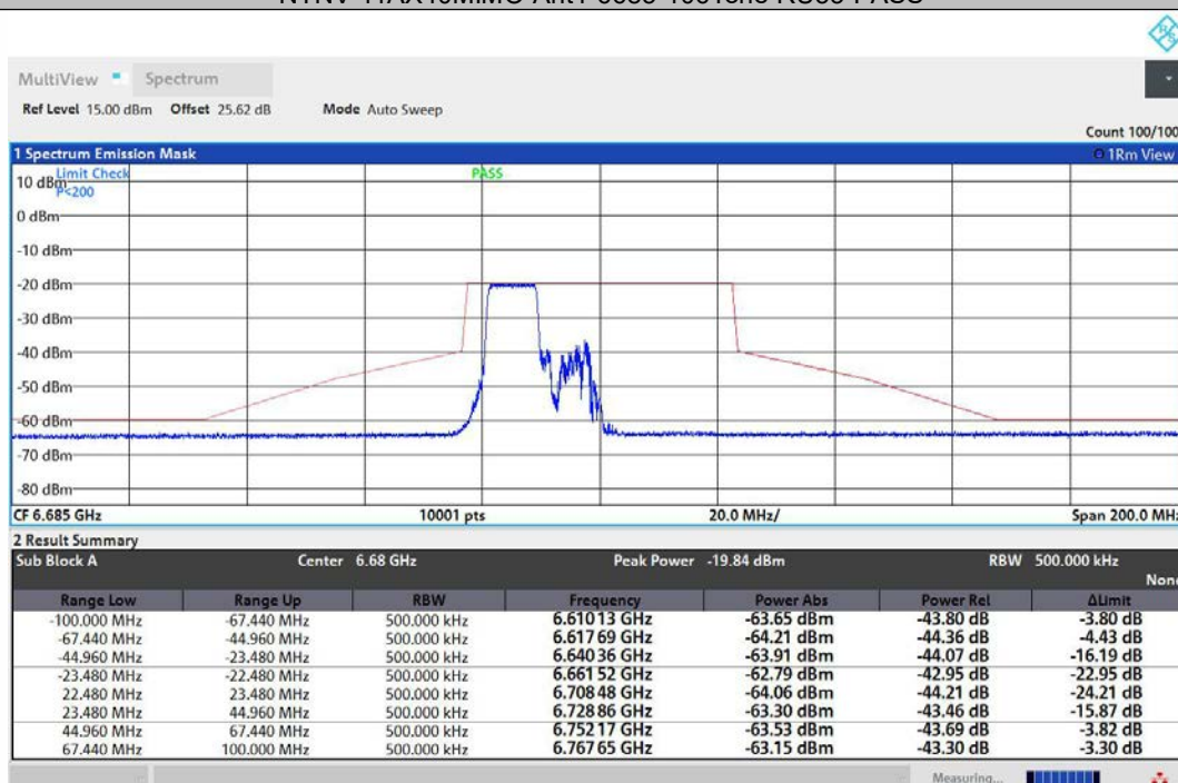
NTNV-11AX40MIMO-Ant2-6685-106Tone-RU53-PASS
