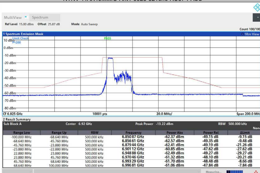
NTNV-11AX40MIMO-Ant2-6925-52Tone-RU37-PASS
