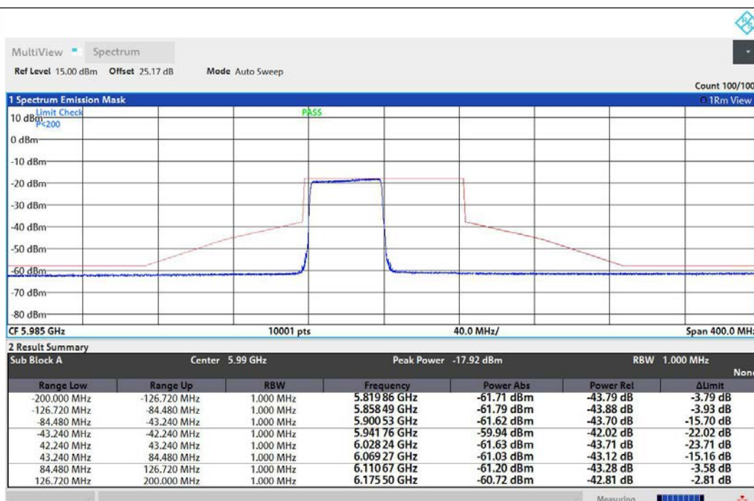
NTNV-11AX80MIMO-Ant1-5985-484Tone-RU65-PASS
