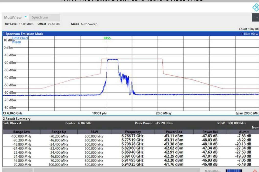
NTNV-11AX40MIMO-Ant2-6845-106Tone-RU53-PASS
