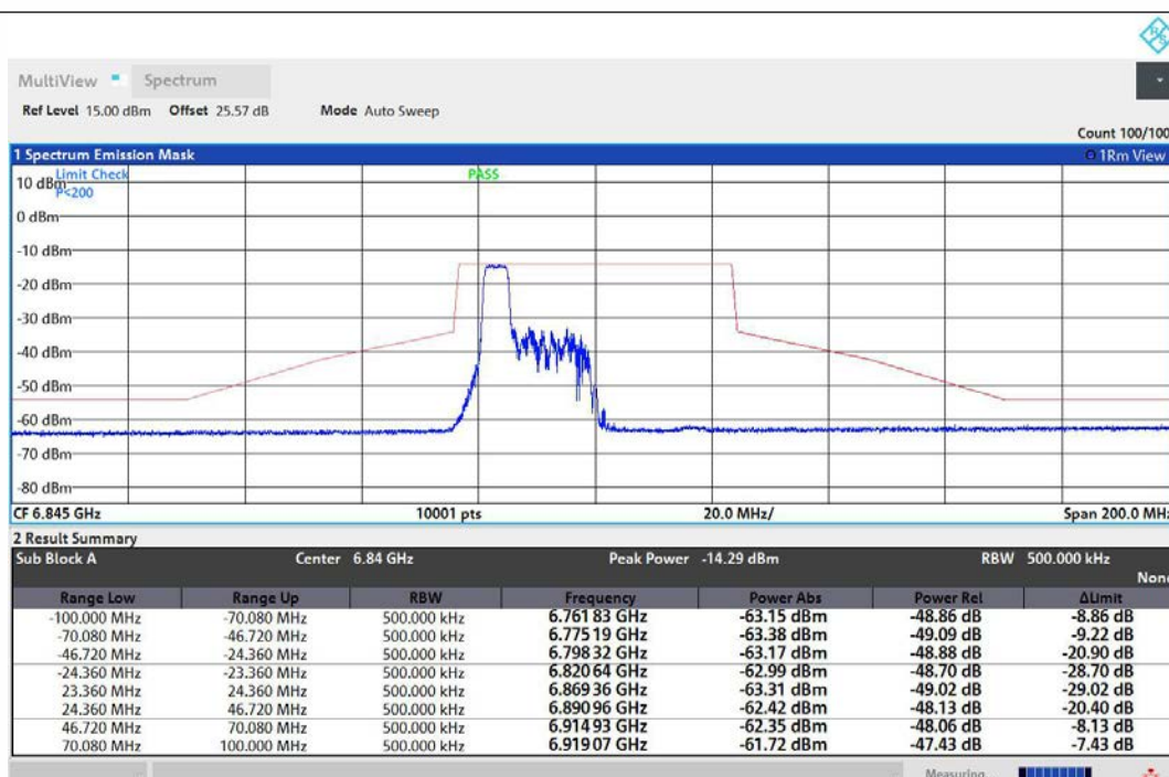
NTNV-11AX40MIMO-Ant1-6845-52Tone-RU37-PASS
