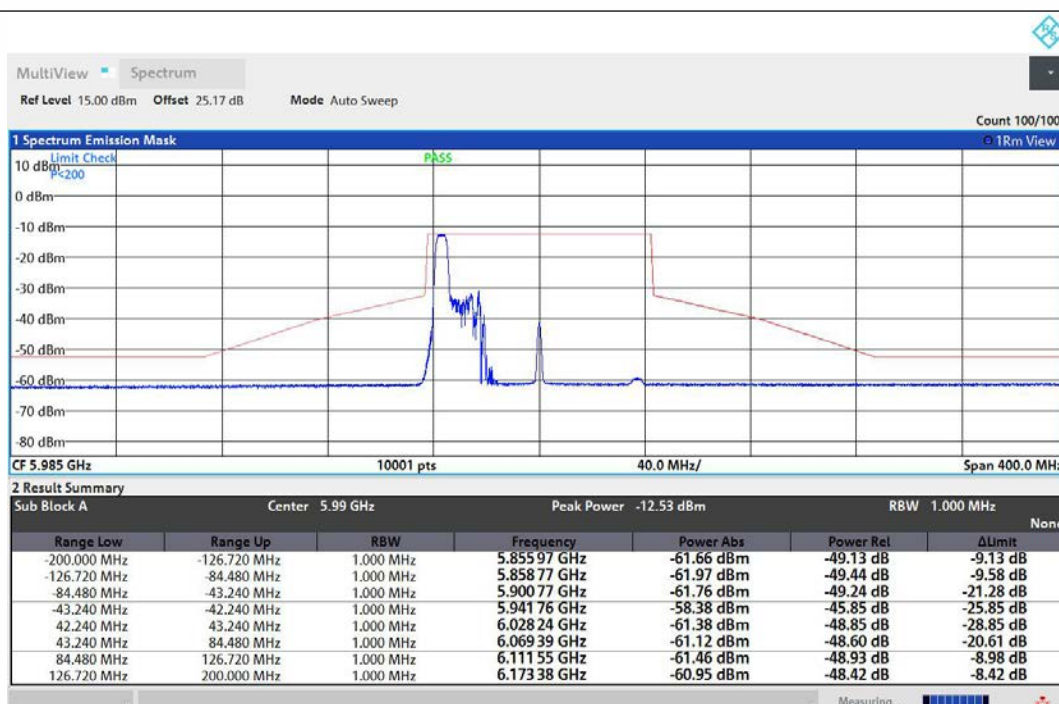
NTNV-11AX80MIMO-Ant1-5985-52Tone-RU37-PASS
