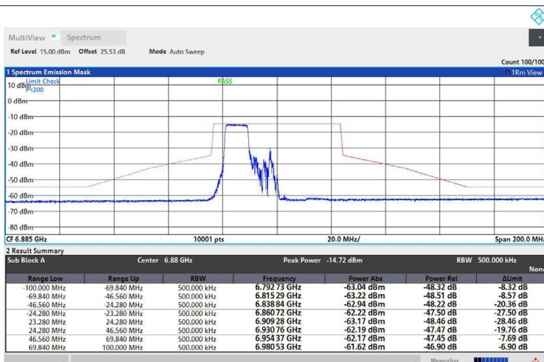
NTNV-11AX40MIMO-Ant1-6885-106Tone-RU53-PASS
