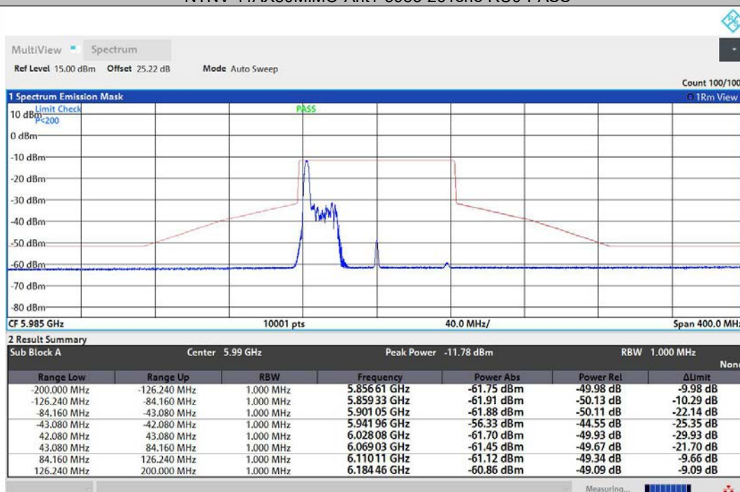
NTNV-11AX80MIMO-Ant2-5985-26Tone-RU0-PASS
