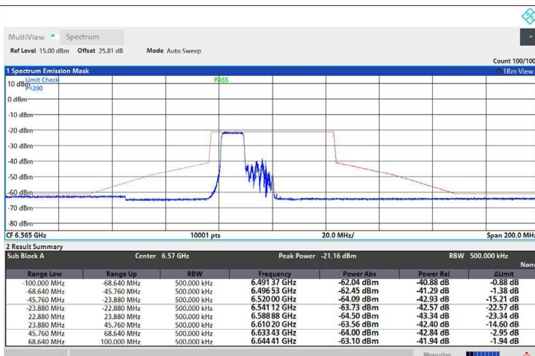
NTNV-11AX40MIMO-Ant1-6565-106Tone-RU53-PASS
