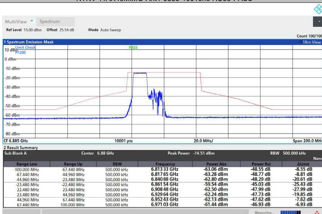
NTNV-11AX40MIMO-Ant2-6885-106Tone-RU53-PASS
