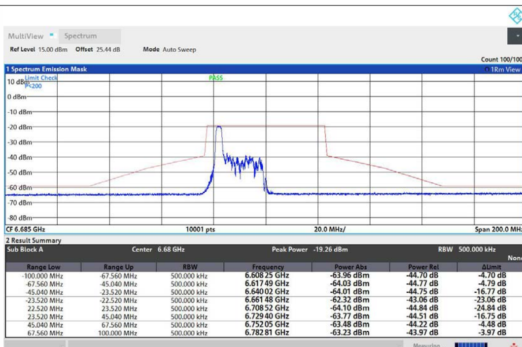
NTNV-11AX40MIMO-Ant1-6685-26Tone-RU0-PASS
