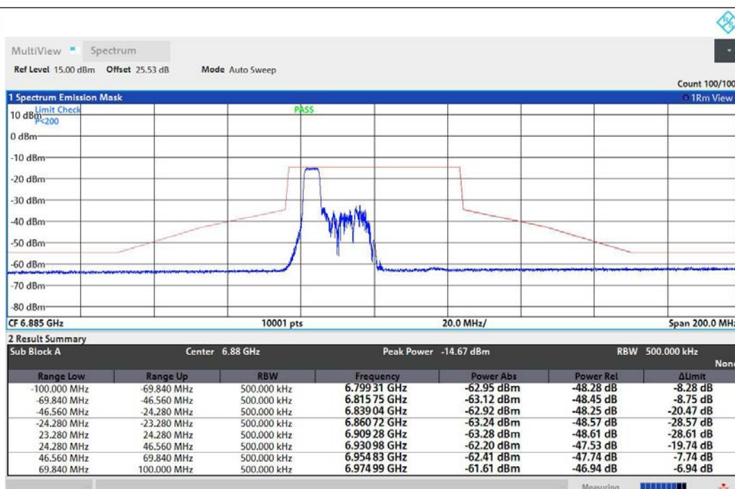
NTNV-11AX40MIMO-Ant1-6885-52Tone-RU37-PASS
