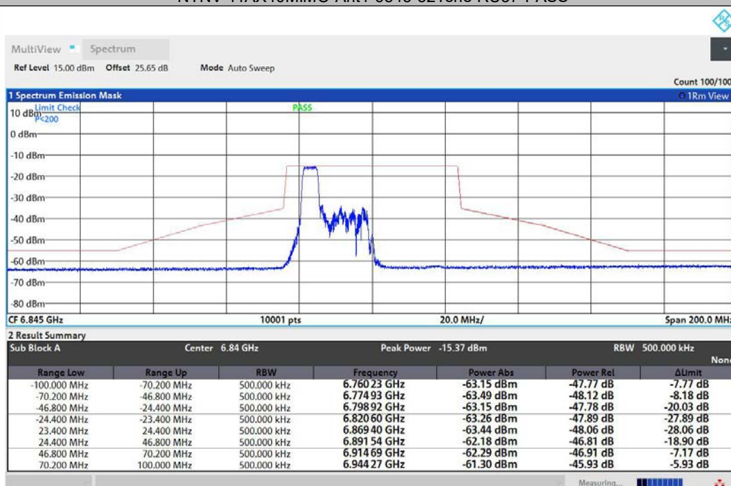
NTNV-11AX40MIMO-Ant2-6845-52Tone-RU37-PASS
