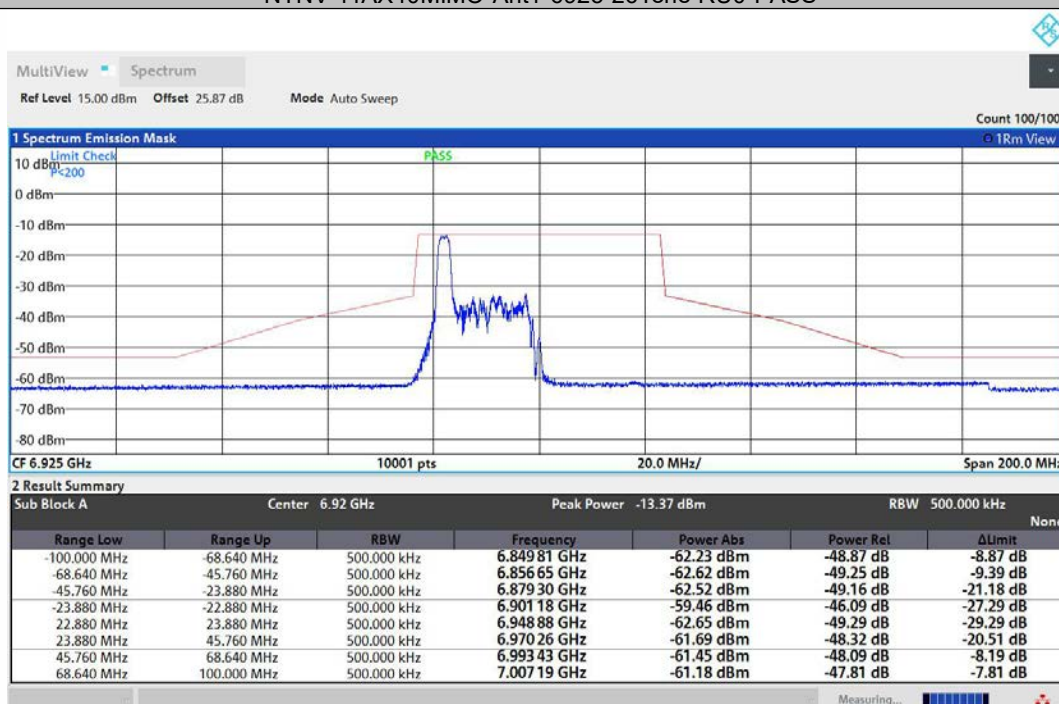
NTNV-11AX40MIMO-Ant2-6925-26Tone-RU0-PASS
