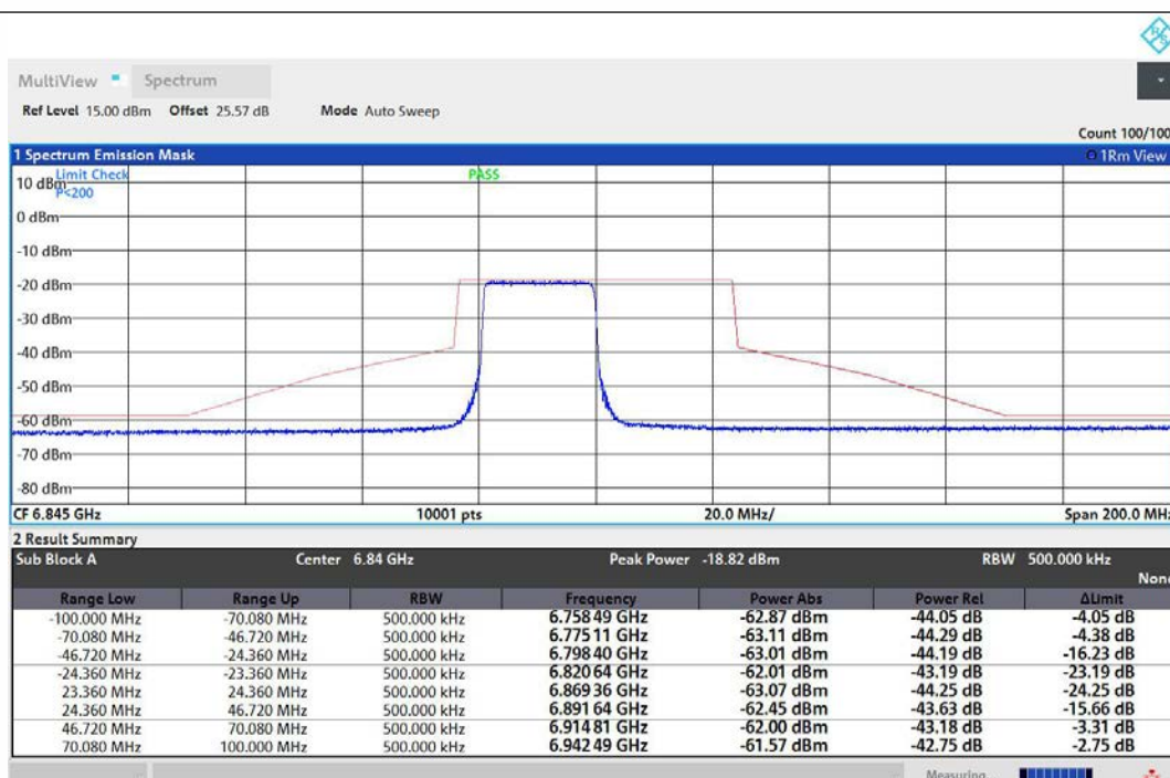
NTNV-11AX40MIMO-Ant1-6845-242Tone-RU61-PASS
