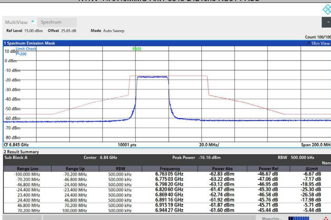
NTNV-11AX40MIMO-Ant2-6845-242Tone-RU61-PASS
