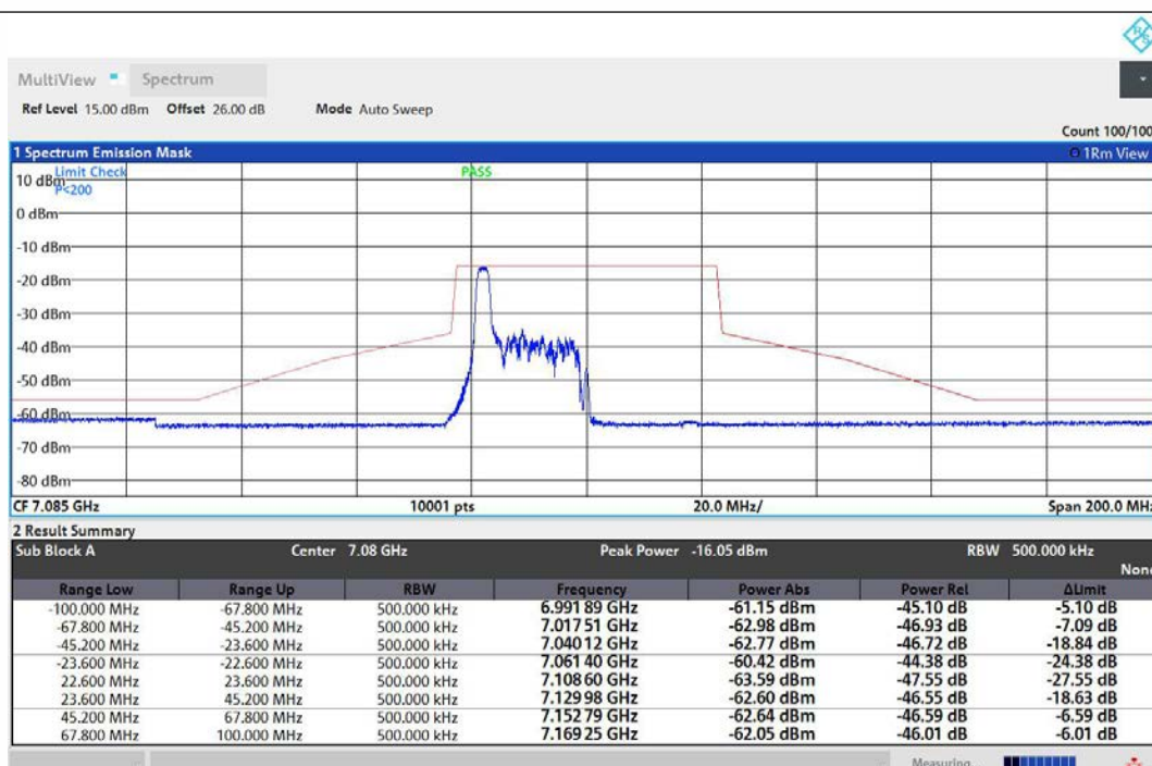
NTNV-11AX40MIMO-Ant1-7085-26Tone-RU0-PASS
