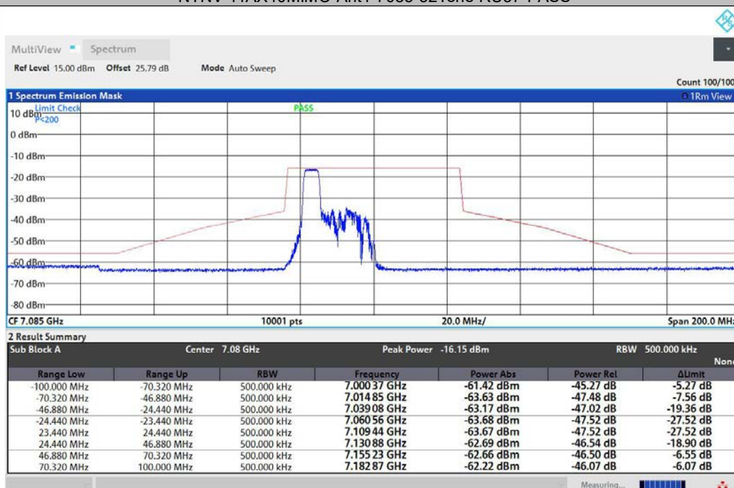
NTNV-11AX40MIMO-Ant2-7085-52Tone-RU37-PASS
