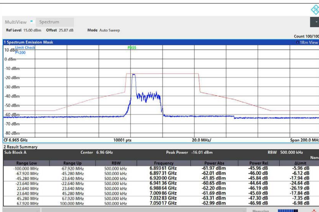
NTNV-11AX40MIMO-Ant1-6965-26Tone-RU0-PASS
