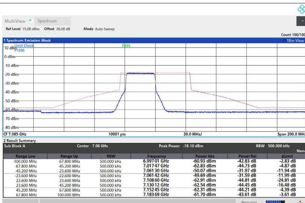
NTNV-11AX40MIMO-Ant1-7085-242Tone-RU61-PASS
