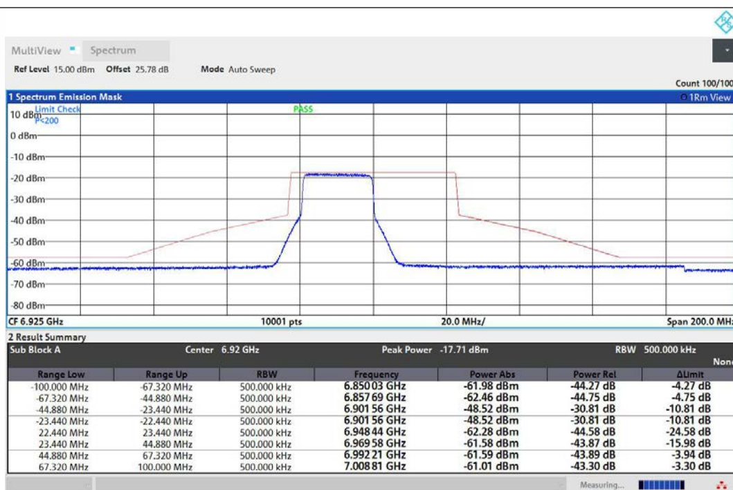
NTNV-11AX40MIMO-Ant1-6925-242Tone-RU61-PASS
