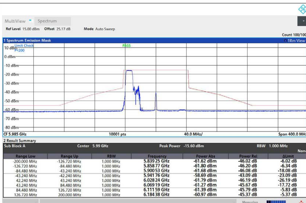
NTNV-11AX80MIMO-Ant1-5985-106Tone-RU53-PASS
