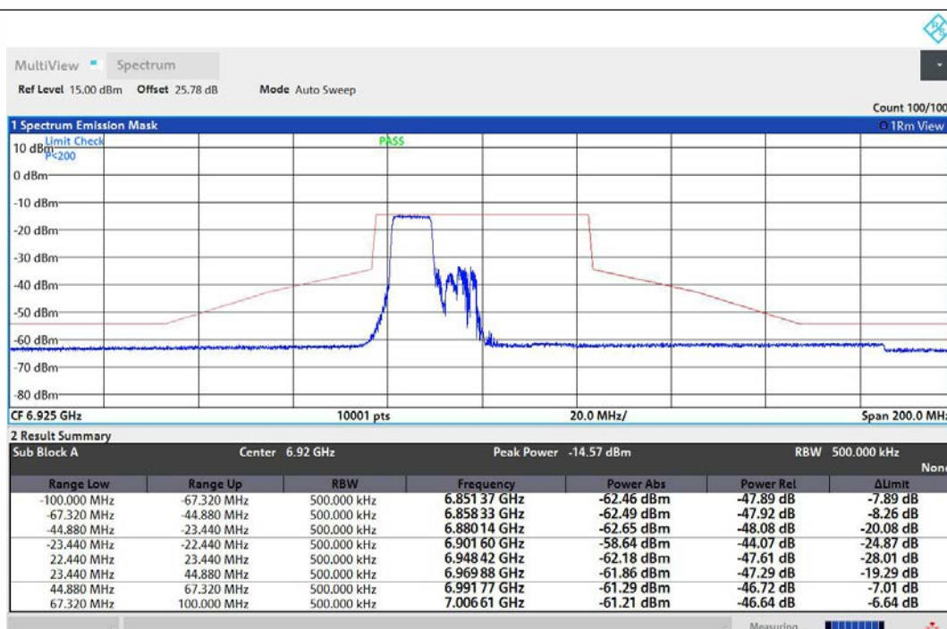
NTNV-11AX40MIMO-Ant1-6925-106Tone-RU53-PASS
