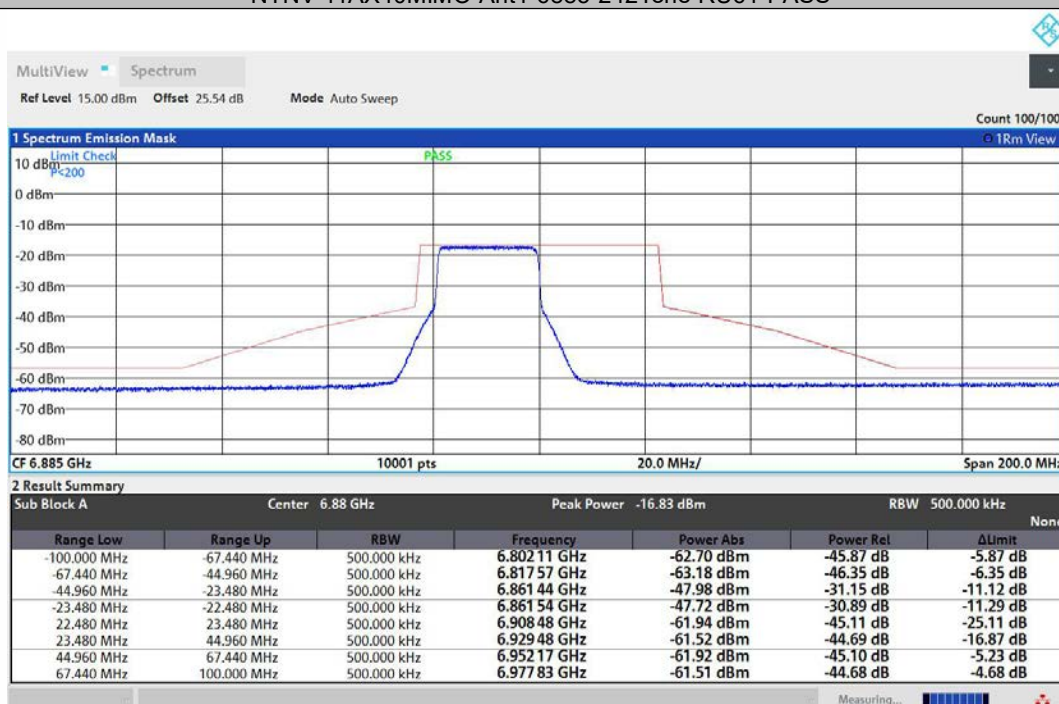
NTNV-11AX40MIMO-Ant2-6885-242Tone-RU61-PASS
