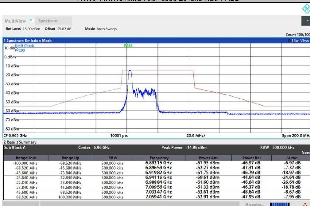
NTNV-11AX40MIMO-Ant2-6965-26Tone-RU0-PASS
