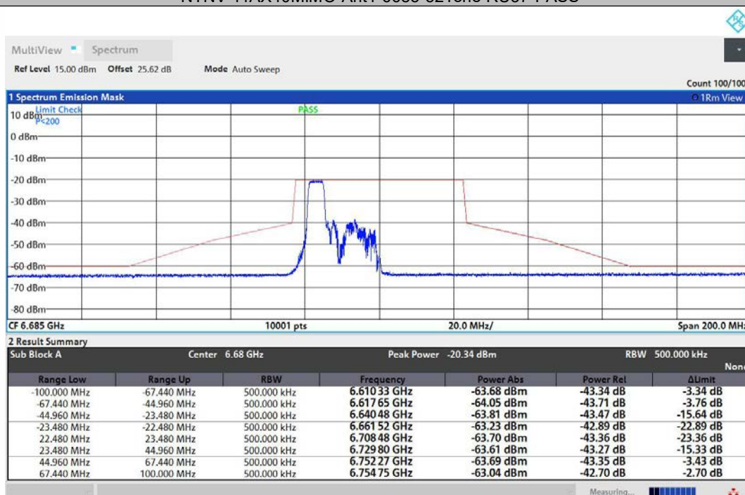
NTNV-11AX40MIMO-Ant2-6685-52Tone-RU37-PASS
