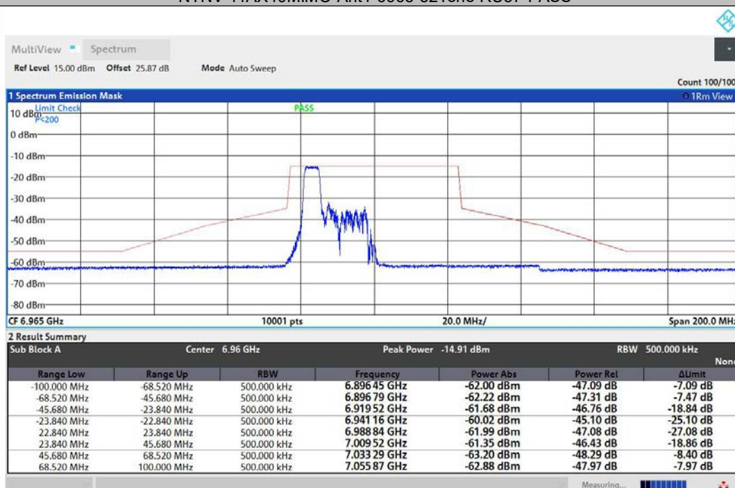
NTNV-11AX40MIMO-Ant2-6965-52Tone-RU37-PASS
