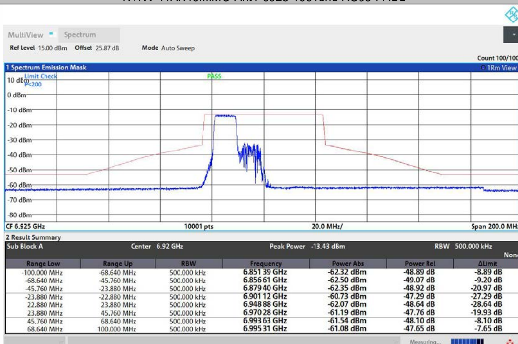
NTNV-11AX40MIMO-Ant2-6925-106Tone-RU53-PASS
