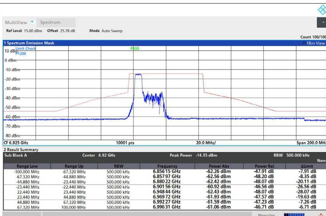
NTNV-11AX40MIMO-Ant1-6925-52Tone-RU37-PASS
