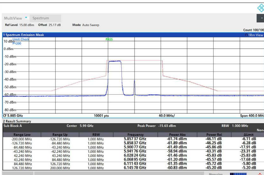
NTNV-11AX80MIMO-Ant1-5985-242Tone-RU61-PASS
