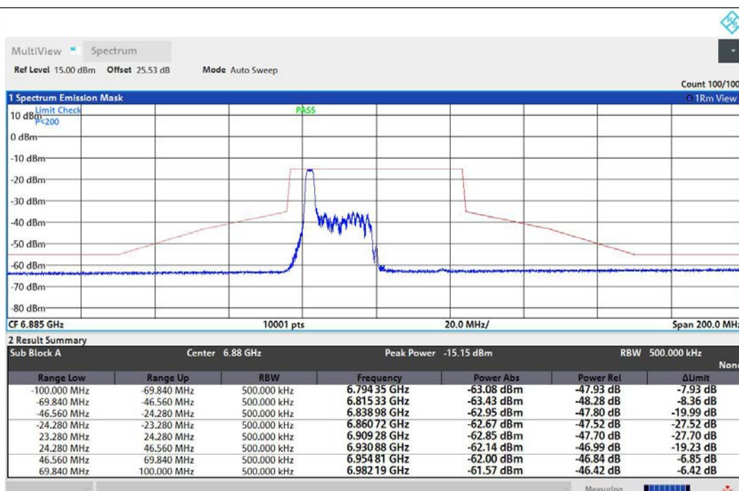
NTNV-11AX40MIMO-Ant1-6885-26Tone-RU0-PASS
