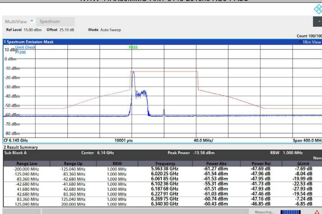
NTNV-11AX80MIMO-Ant2-6145-26Tone-RU0-PASS
