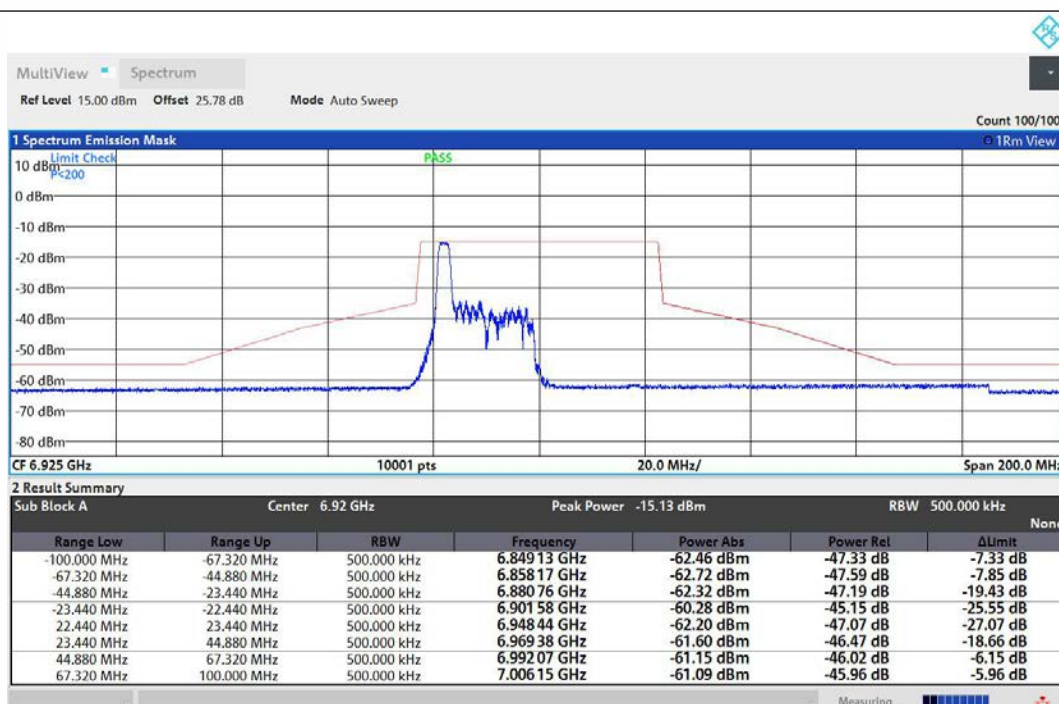
NTNV-11AX40MIMO-Ant1-6925-26Tone-RU0-PASS
