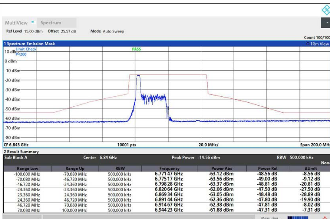
NTNV-11AX40MIMO-Ant1-6845-26Tone-RU0-PASS
