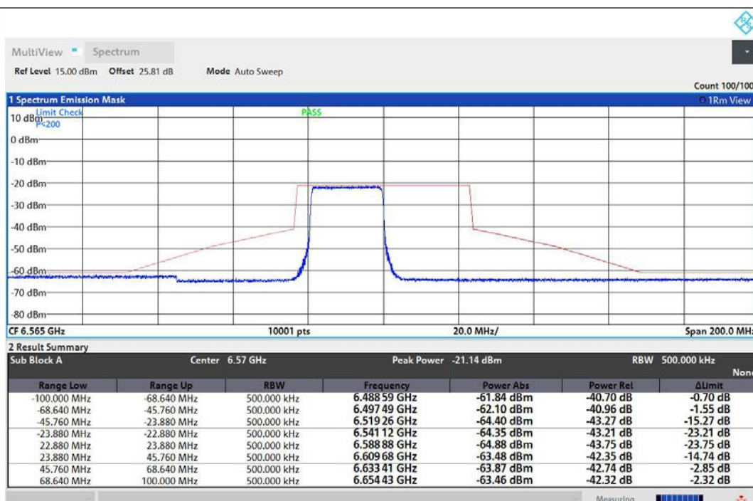
NTNV-11AX40MIMO-Ant1-6565-242Tone-RU61-PASS
