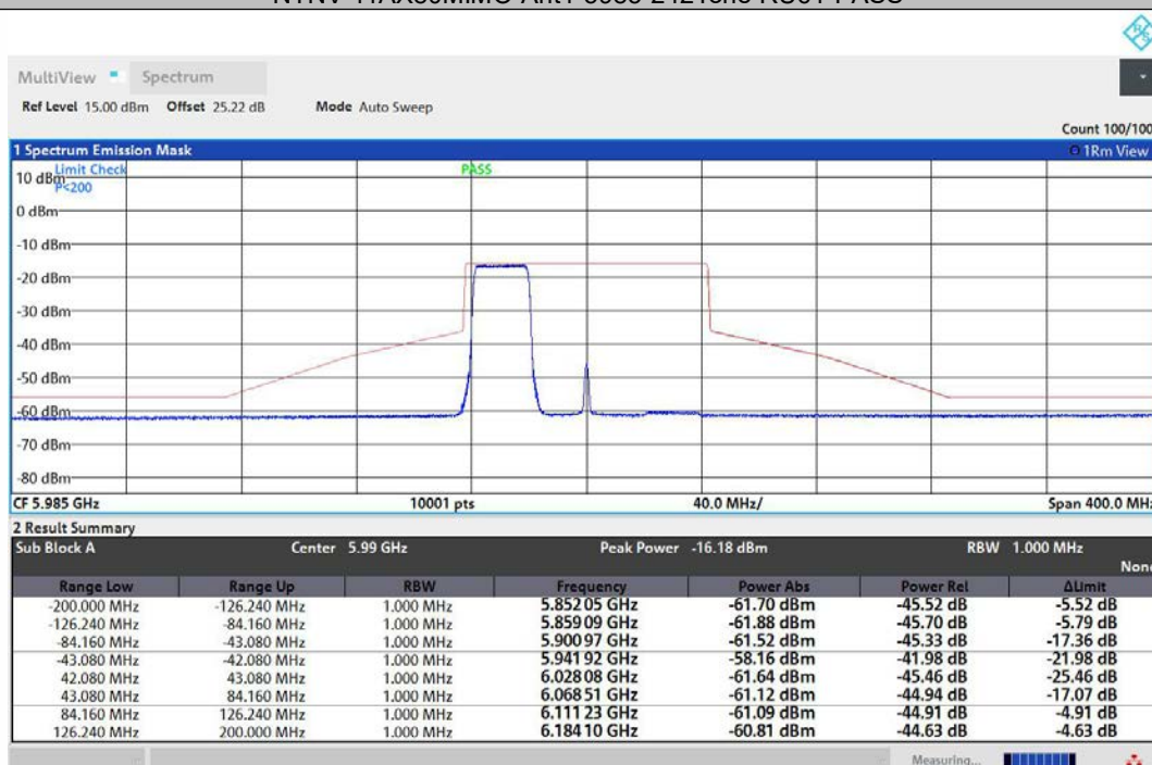
NTNV-11AX80MIMO-Ant2-5985-242Tone-RU61-PASS
