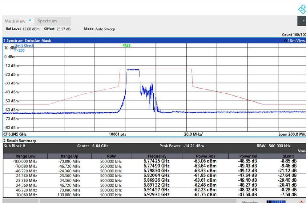
NTNV-11AX40MIMO-Ant1-6845-106Tone-RU53-PASS
