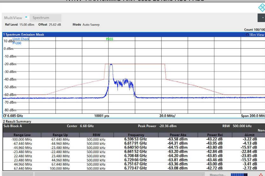
NTNV-11AX40MIMO-Ant2-6685-26Tone-RU0-PASS
