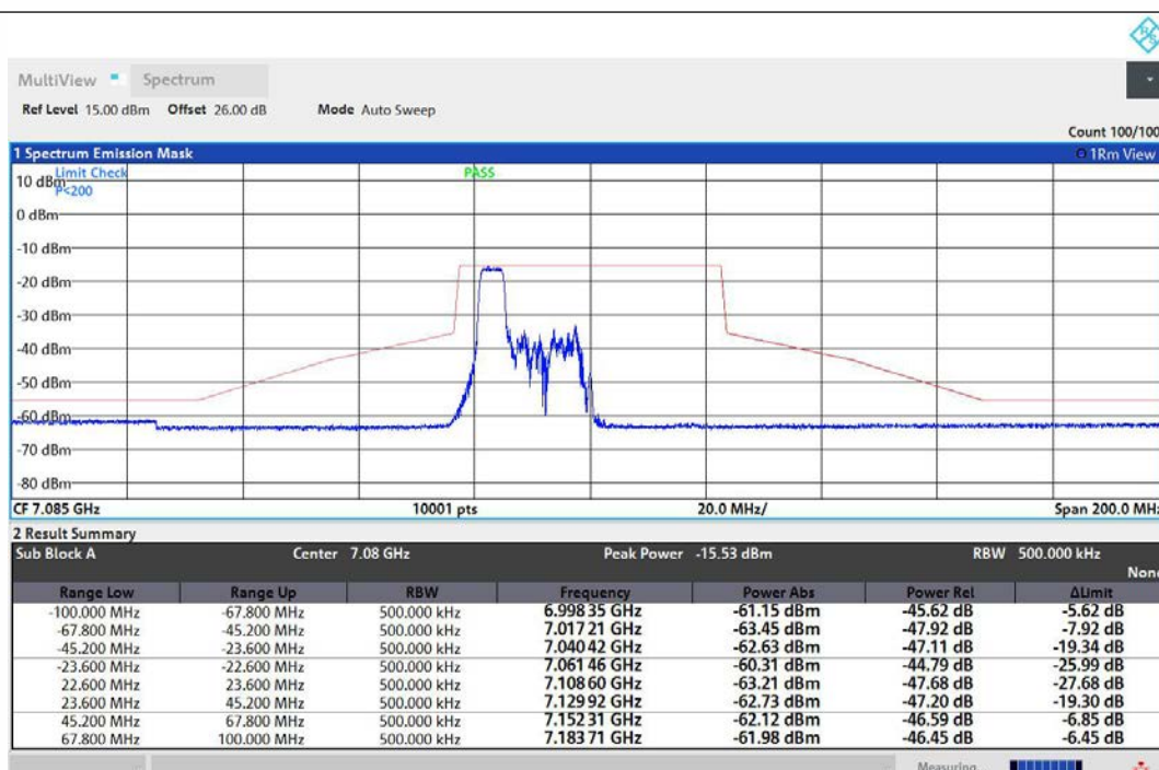
NTNV-11AX40MIMO-Ant1-7085-52Tone-RU37-PASS
