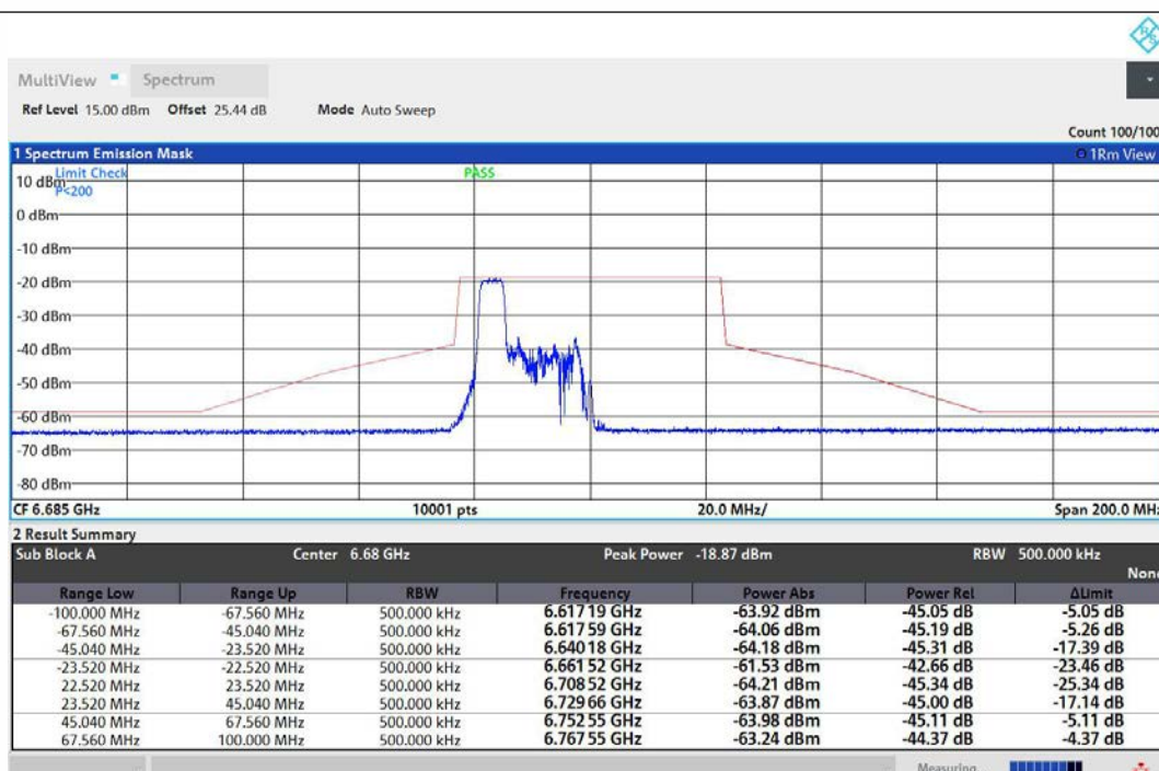
NTNV-11AX40MIMO-Ant1-6685-52Tone-RU37-PASS
