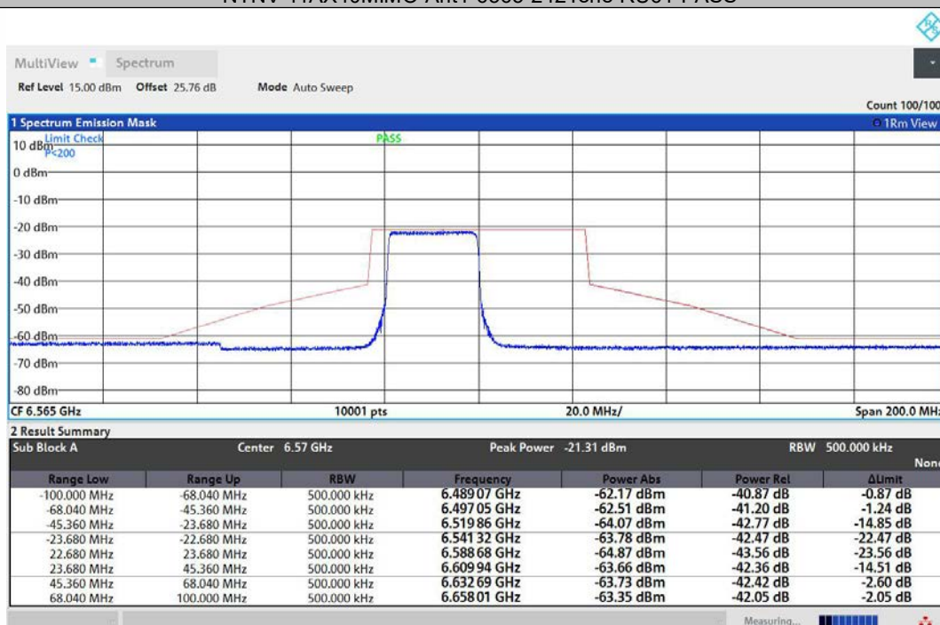
NTNV-11AX40MIMO-Ant2-6565-242Tone-RU61-PASS
