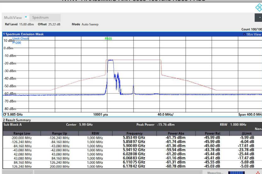
NTNV-11AX80MIMO-Ant2-5985-106Tone-RU53-PASS
