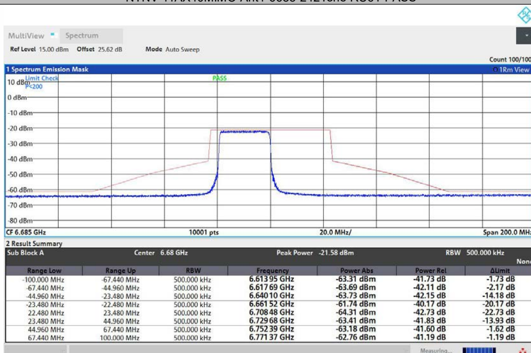
NTNV-11AX40MIMO-Ant2-6685-242Tone-RU61-PASS
