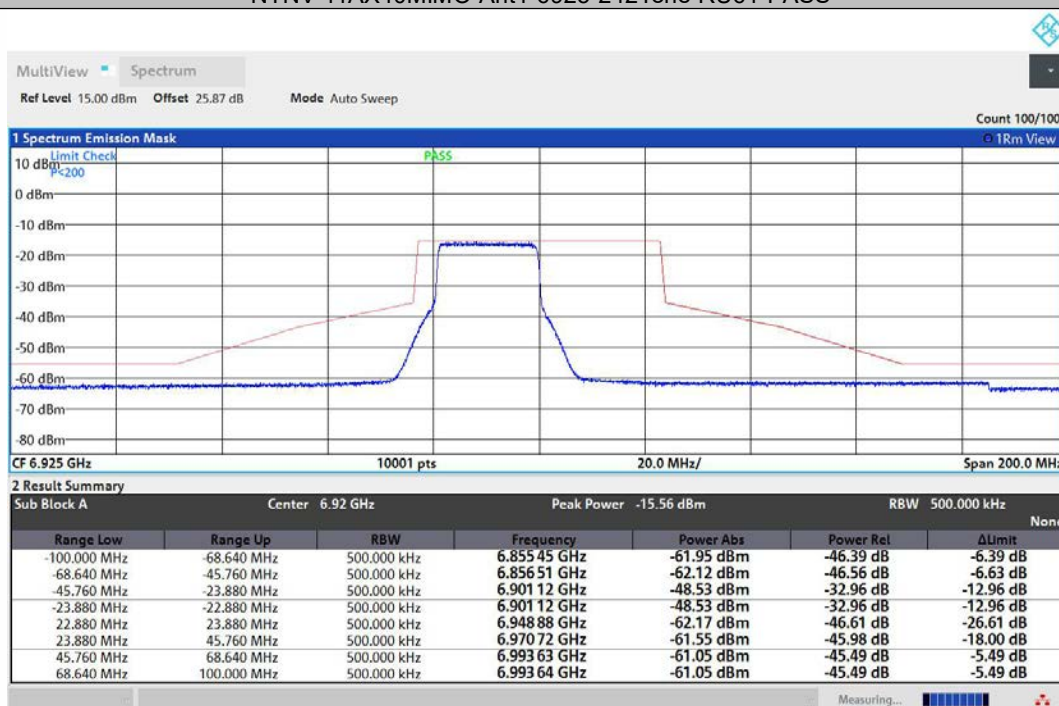
NTNV-11AX40MIMO-Ant2-6925-242Tone-RU61-PASS
