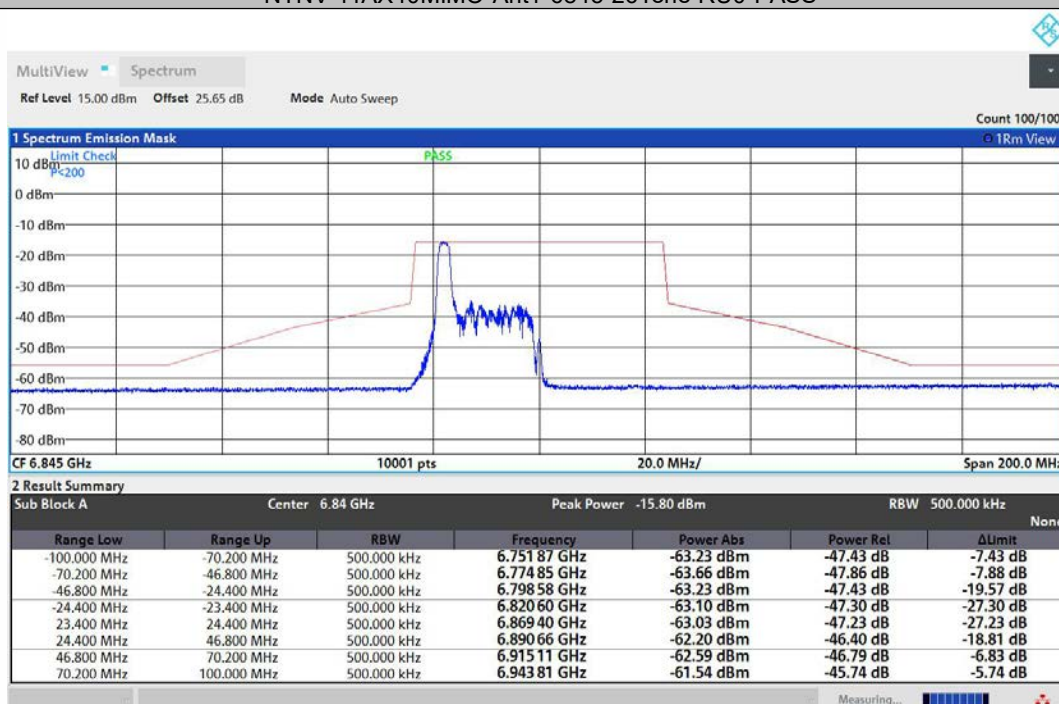
NTNV-11AX40MIMO-Ant2-6845-26Tone-RU0-PASS
