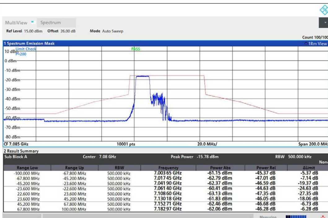
NTNV-11AX40MIMO-Ant1-7085-106Tone-RU53-PASS
