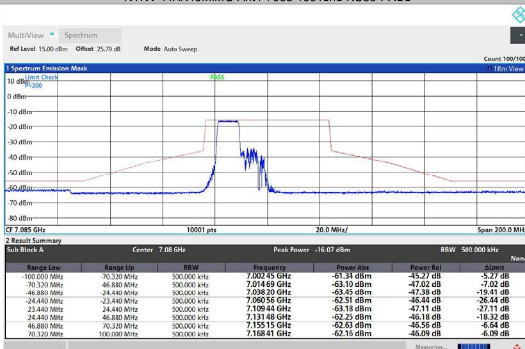
NTNV-11AX40MIMO-Ant2-7085-106Tone-RU53-PASS
