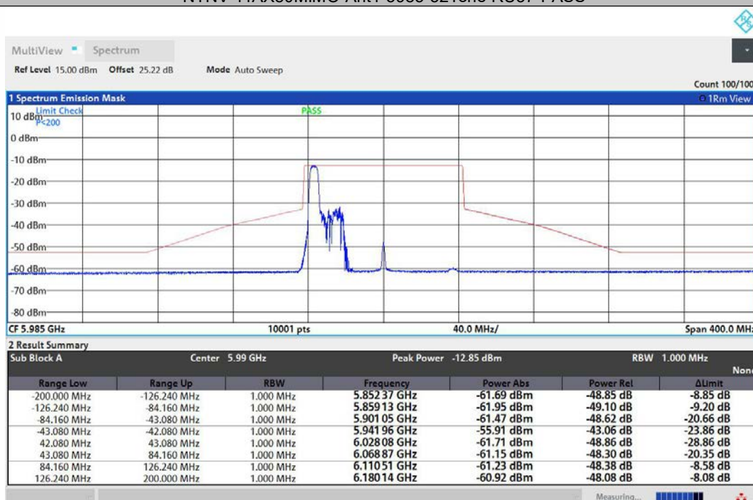
NTNV-11AX80MIMO-Ant2-5985-52Tone-RU37-PASS
