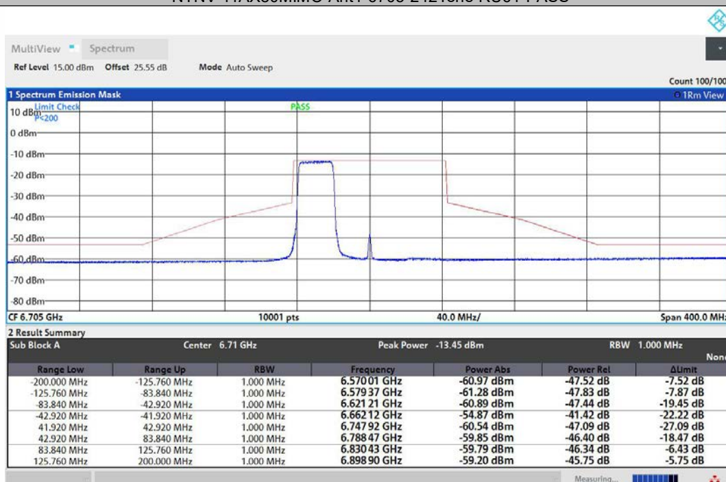
NTNV-11AX80MIMO-Ant2-6705-242Tone-RU61-PASS
