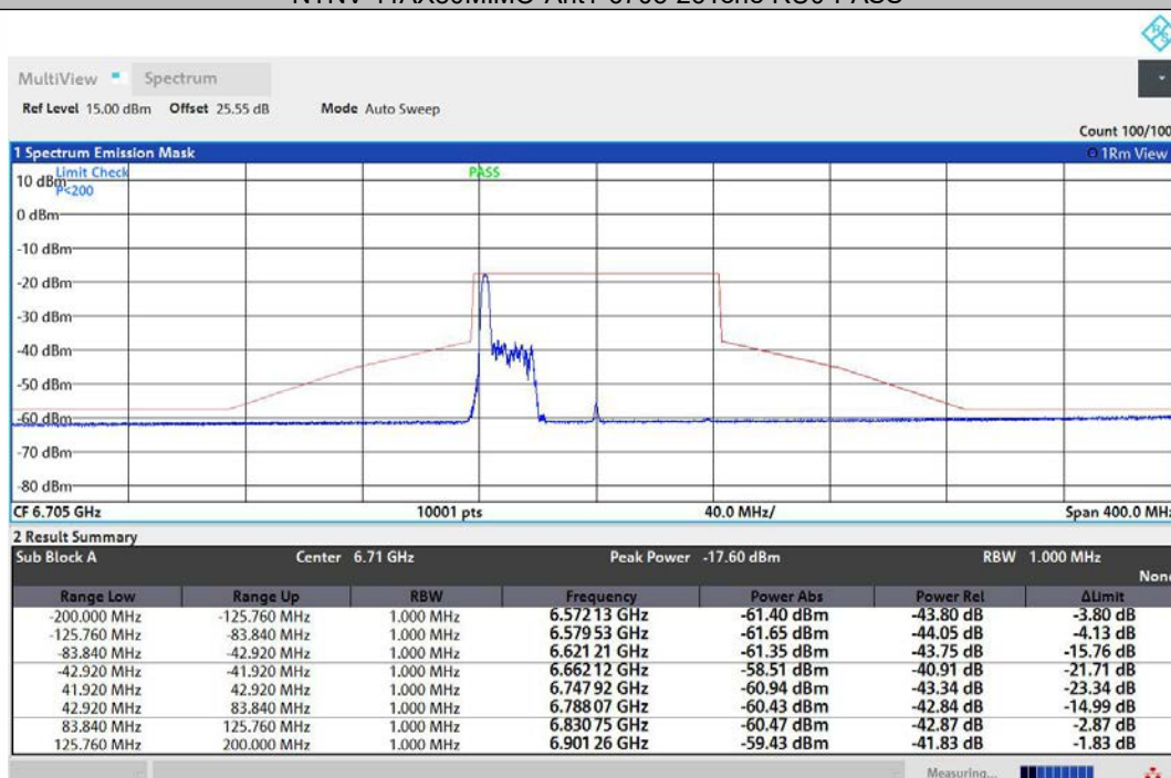
NTNV-11AX80MIMO-Ant2-6705-26Tone-RU0-PASS
