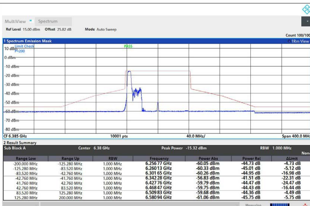
NTNV-11AX80MIMO-Ant1-6385-52Tone-RU37-PASS
