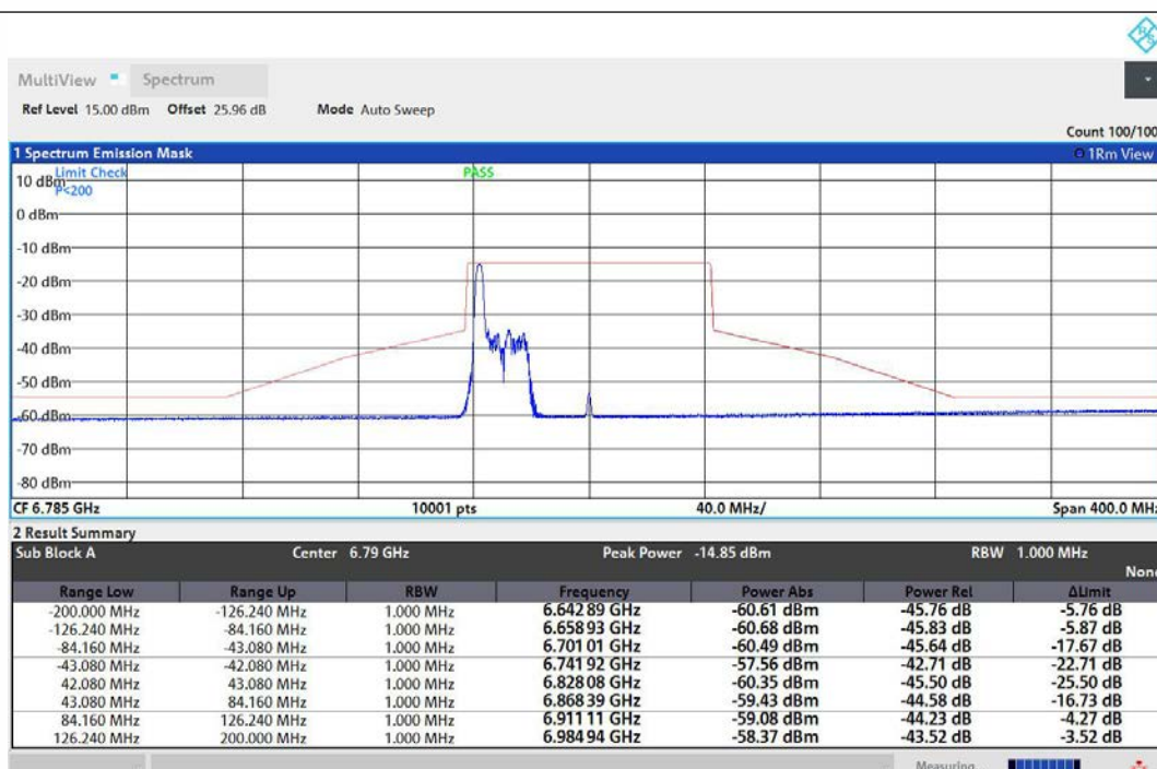
NTNV-11AX80MIMO-Ant1-6785-26Tone-RU0-PASS
