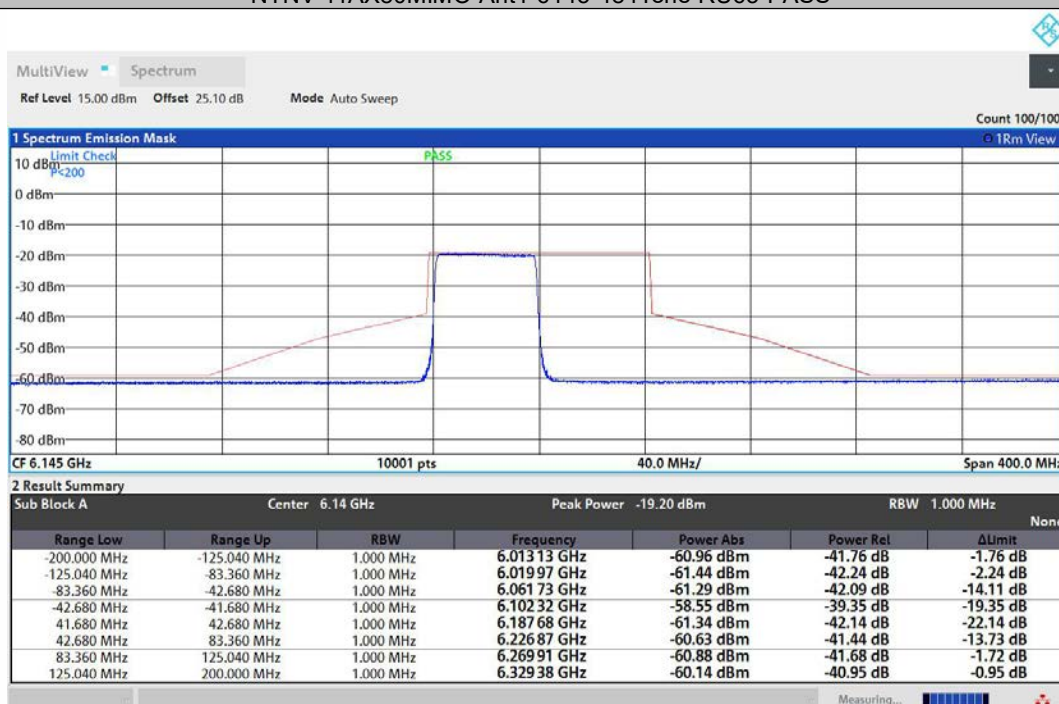
NTNV-11AX80MIMO-Ant2-6145-484Tone-RU65-PASS
