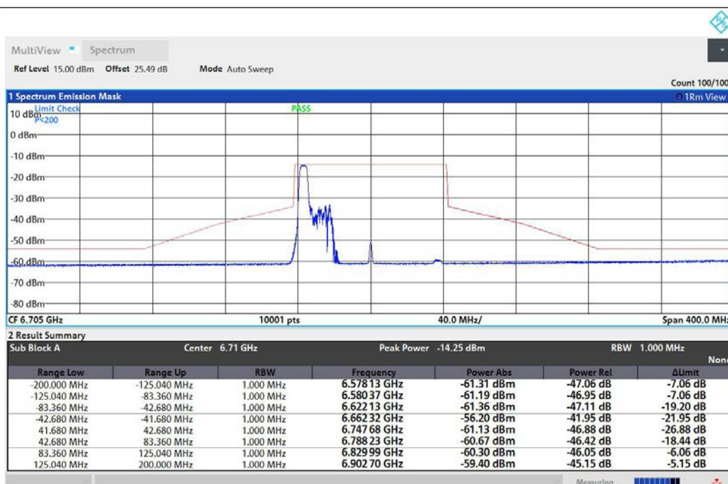
NTNV-11AX80MIMO-Ant1-6705-52Tone-RU37-PASS
