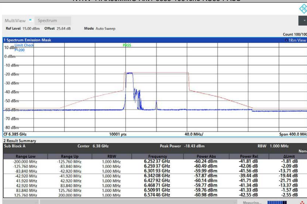
NTNV-11AX80MIMO-Ant2-6385-106Tone-RU53-PASS
