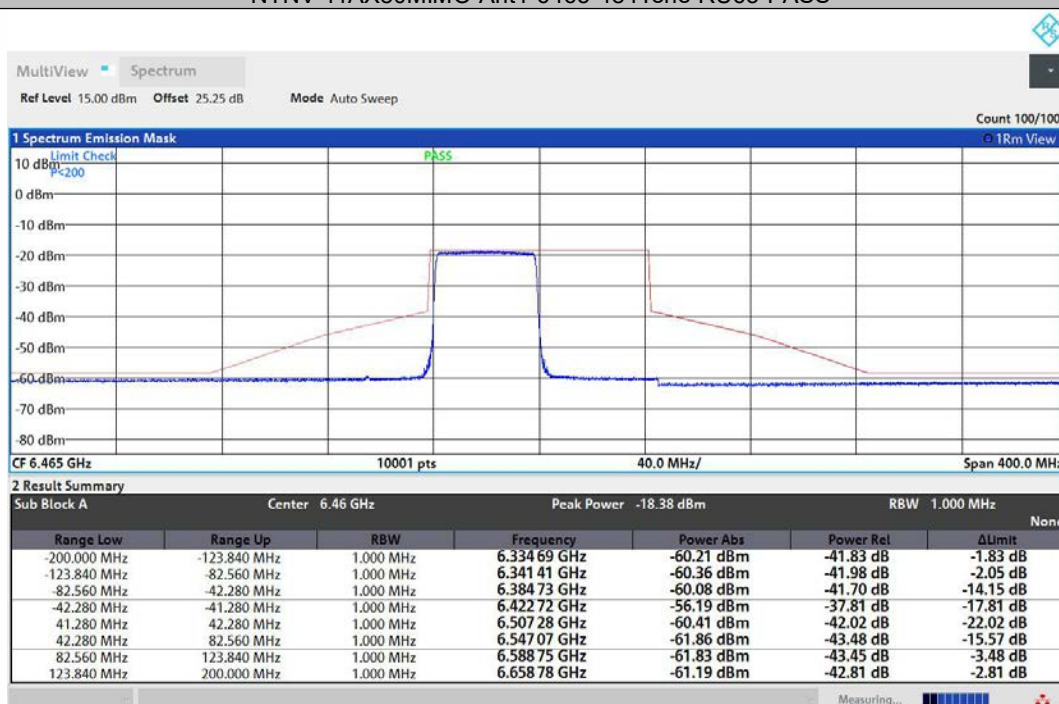
NTNV-11AX80MIMO-Ant2-6465-484Tone-RU65-PASS
