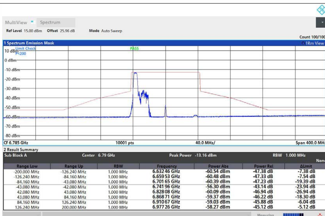
NTNV-11AX80MIMO-Ant1-6785-52Tone-RU37-PASS
