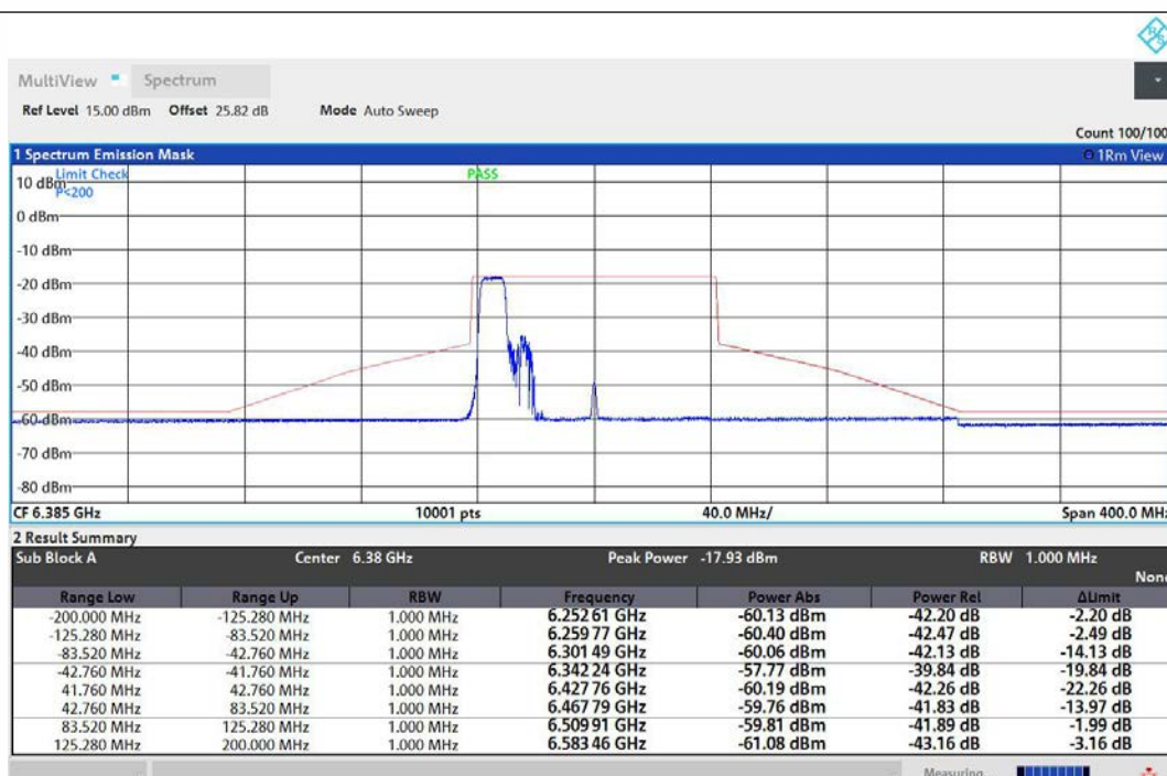
NTNV-11AX80MIMO-Ant1-6385-106Tone-RU53-PASS
