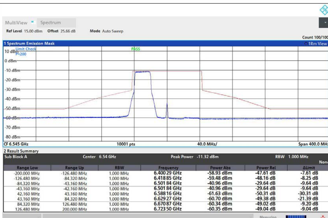
NTNV-11AX80MIMO-Ant1-6545-242Tone-RU61-PASS
