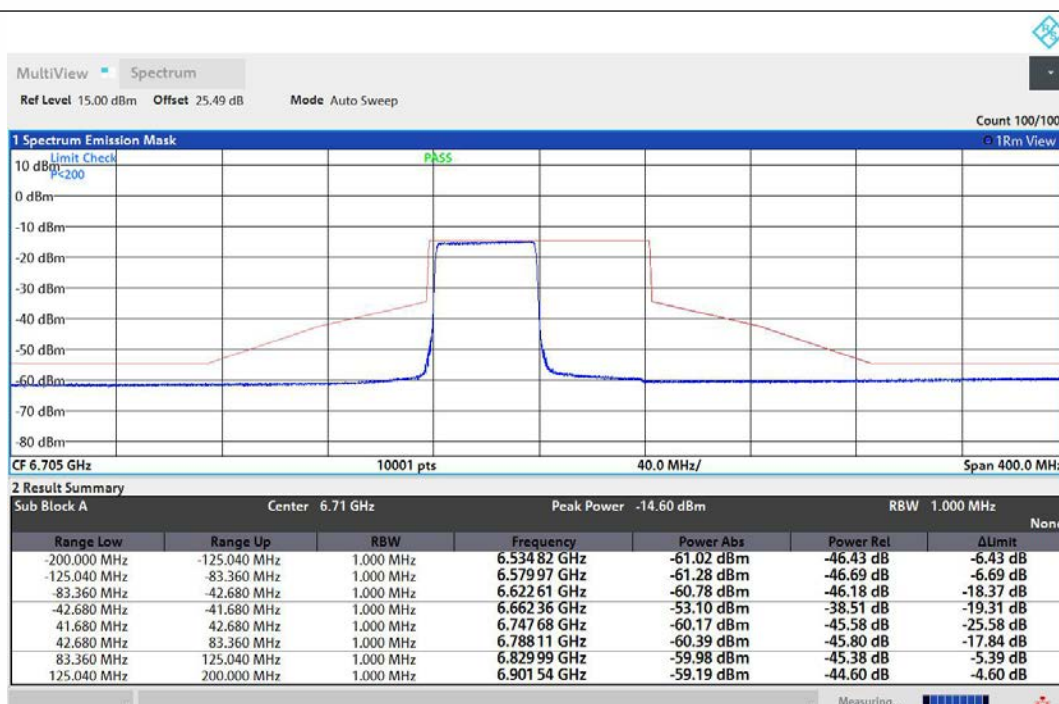
NTNV-11AX80MIMO-Ant1-6705-484Tone-RU65-PASS
