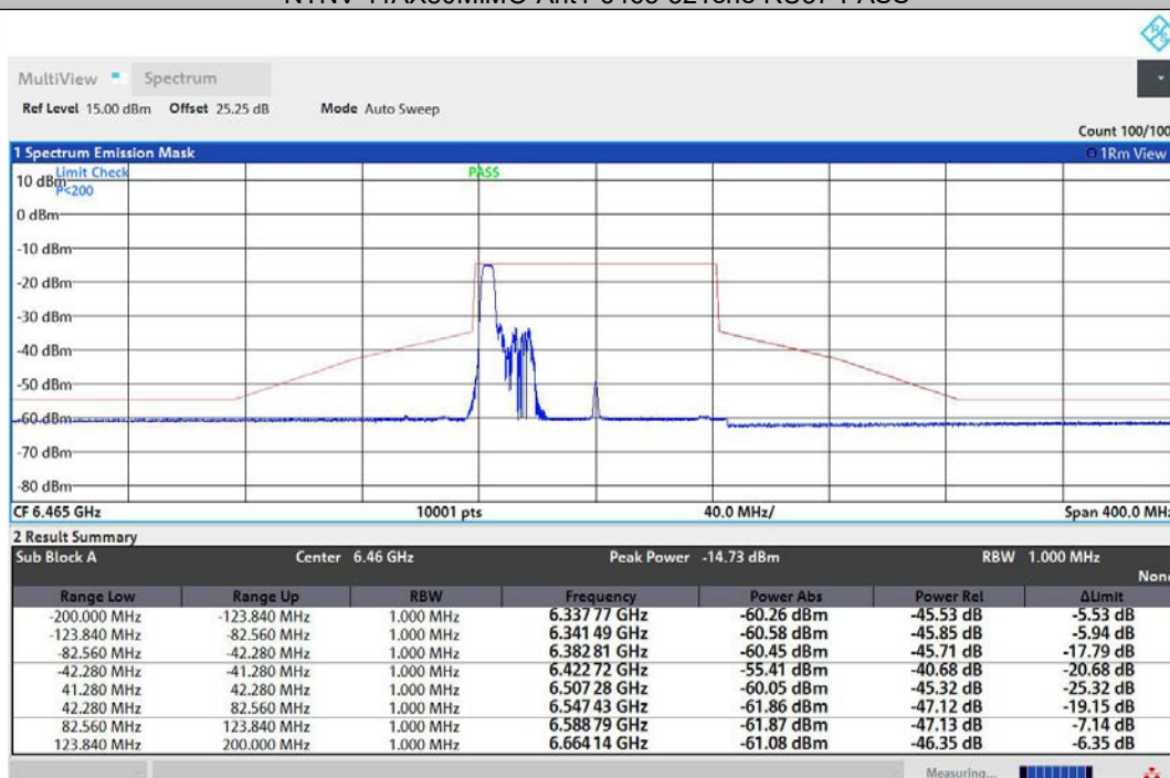
NTNV-11AX80MIMO-Ant2-6465-52Tone-RU37-PASS
