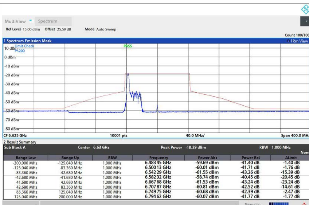
NTNV-11AX80MIMO-Ant1-6625-26Tone-RU0-PASS
