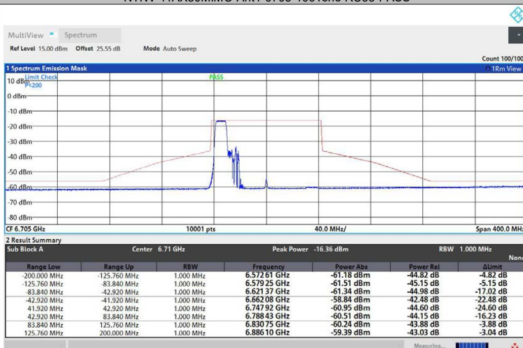
NTNV-11AX80MIMO-Ant2-6705-106Tone-RU53-PASS
