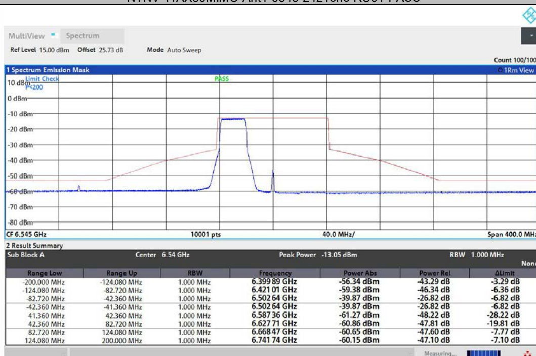
NTNV-11AX80MIMO-Ant2-6545-242Tone-RU61-PASS
