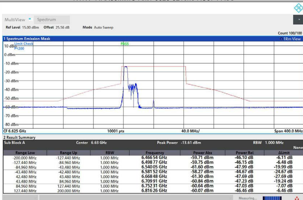
NTNV-11AX80MIMO-Ant2-6625-52Tone-RU37-PASS
