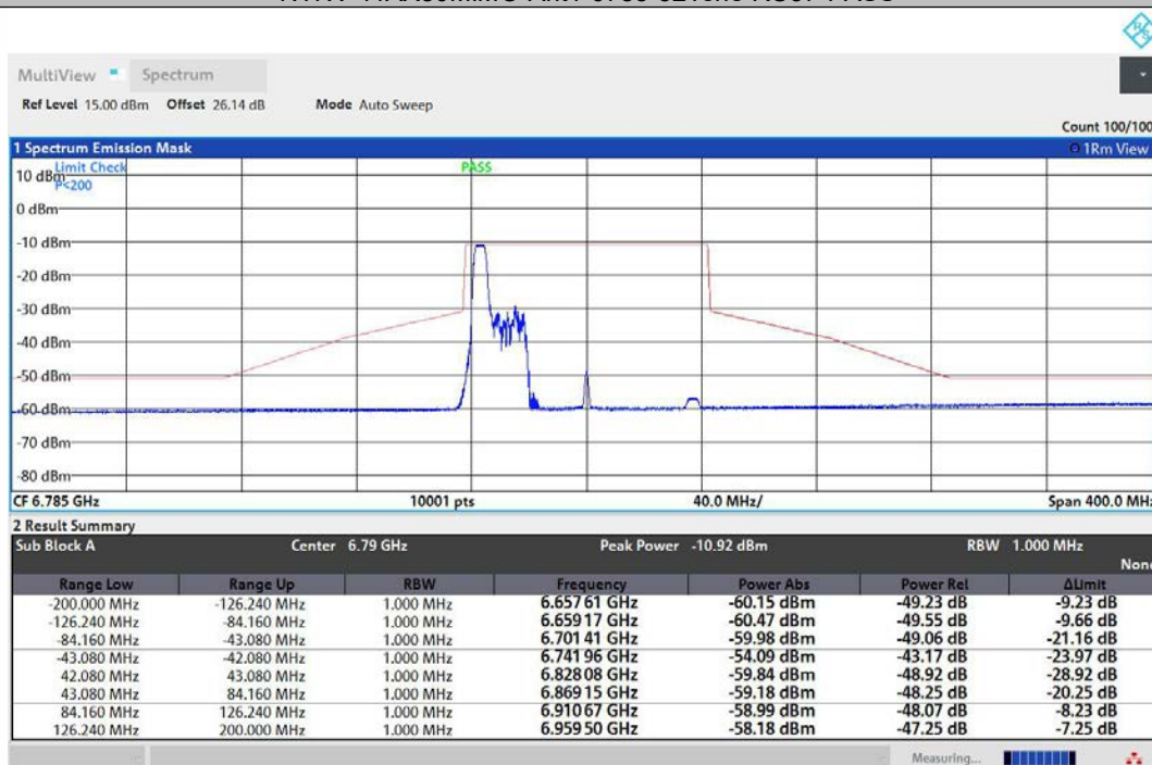
NTNV-11AX80MIMO-Ant2-6785-52Tone-RU37-PASS
