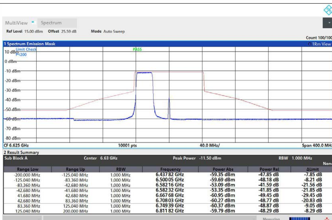
NTNV-11AX80MIMO-Ant1-6625-242Tone-RU61-PASS
