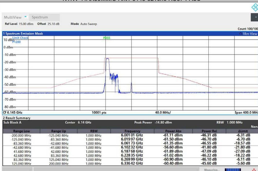
NTNV-11AX80MIMO-Ant2-6145-52Tone-RU37-PASS
