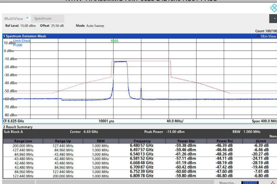
NTNV-11AX80MIMO-Ant2-6625-242Tone-RU61-PASS
