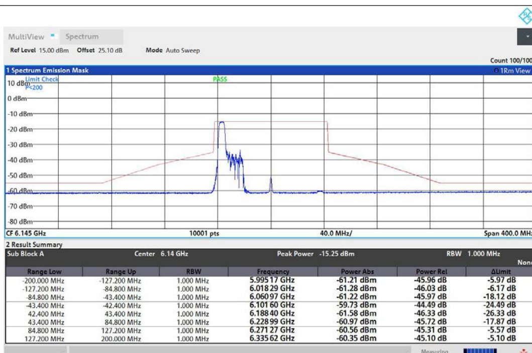
NTNV-11AX80MIMO-Ant1-6145-52Tone-RU37-PASS
