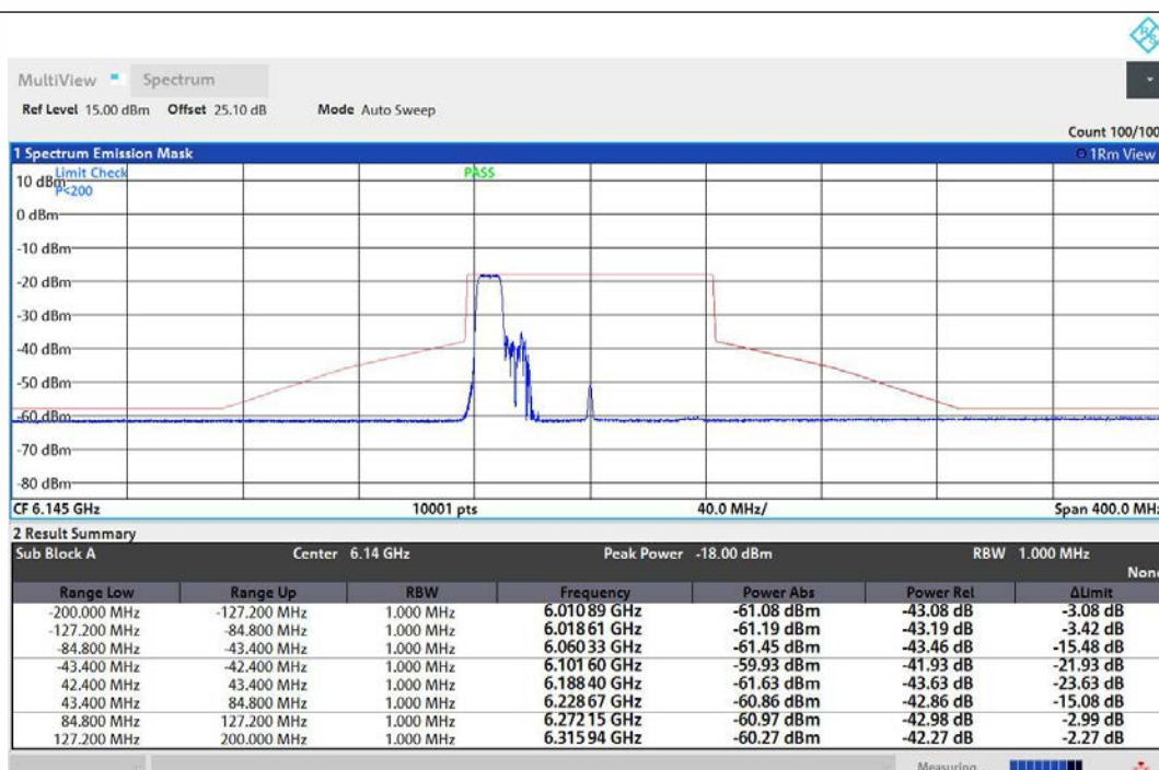
NTNV-11AX80MIMO-Ant1-6145-106Tone-RU53-PASS
