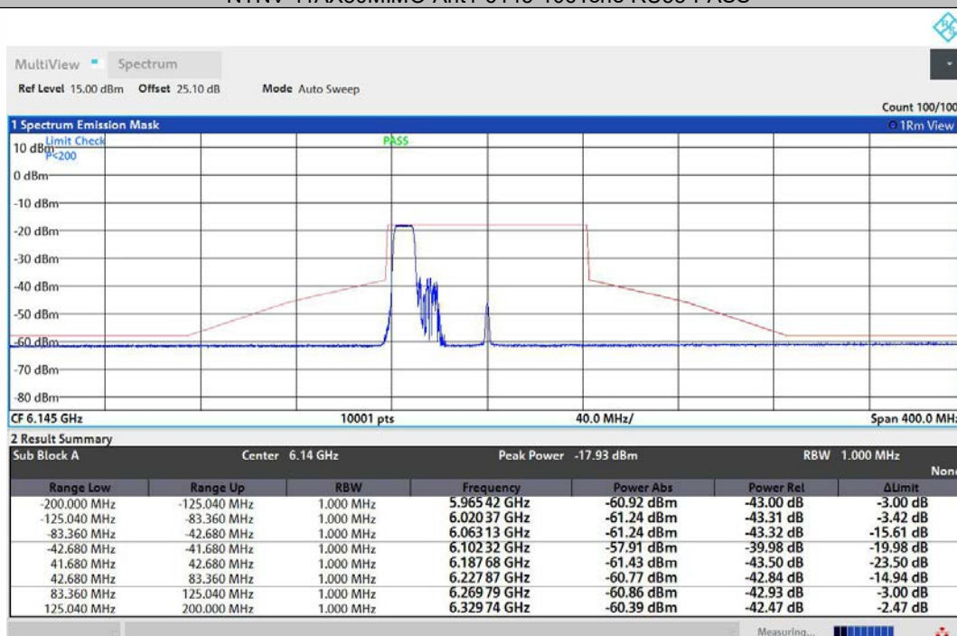
NTNV-11AX80MIMO-Ant2-6145-106Tone-RU53-PASS
