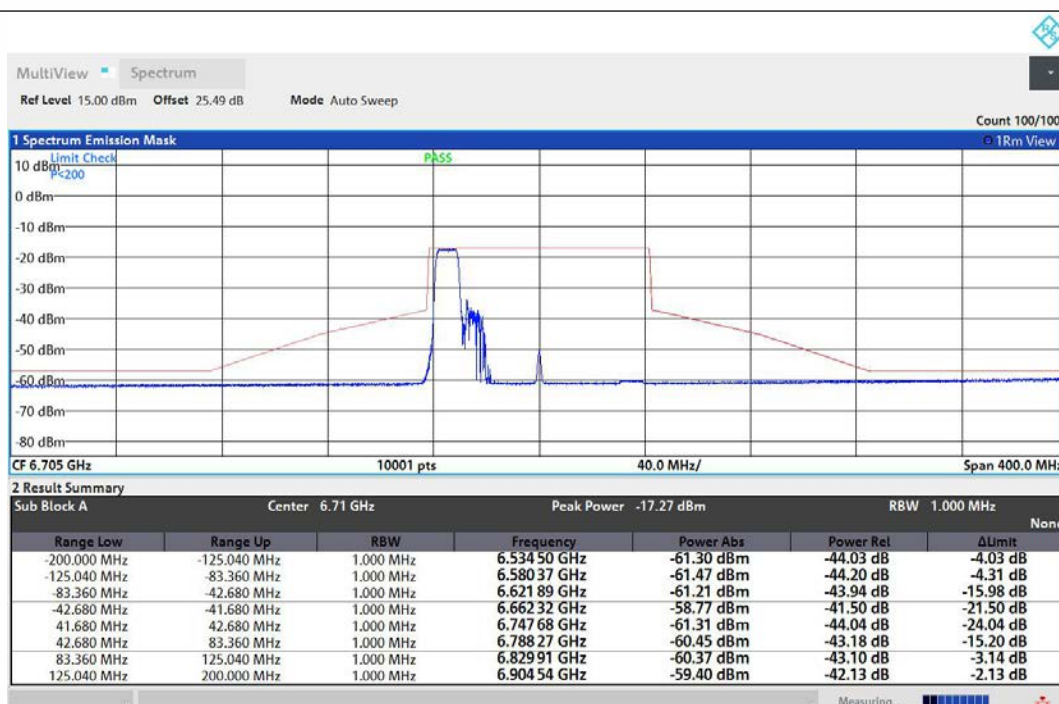
NTNV-11AX80MIMO-Ant1-6705-106Tone-RU53-PASS
