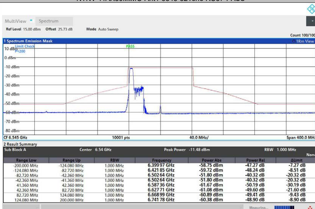
NTNV-11AX80MIMO-Ant2-6545-52Tone-RU37-PASS
