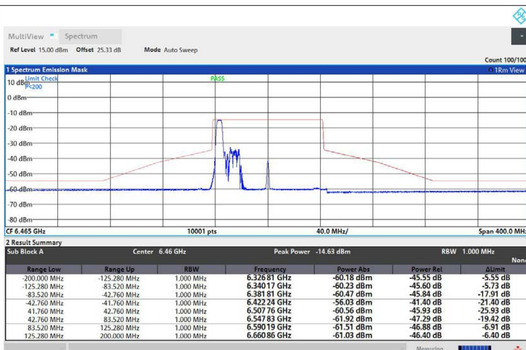
NTNV-11AX80MIMO-Ant1-6465-52Tone-RU37-PASS
