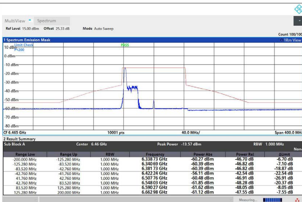
NTNV-11AX80MIMO-Ant1-6465-26Tone-RU0-PASS
