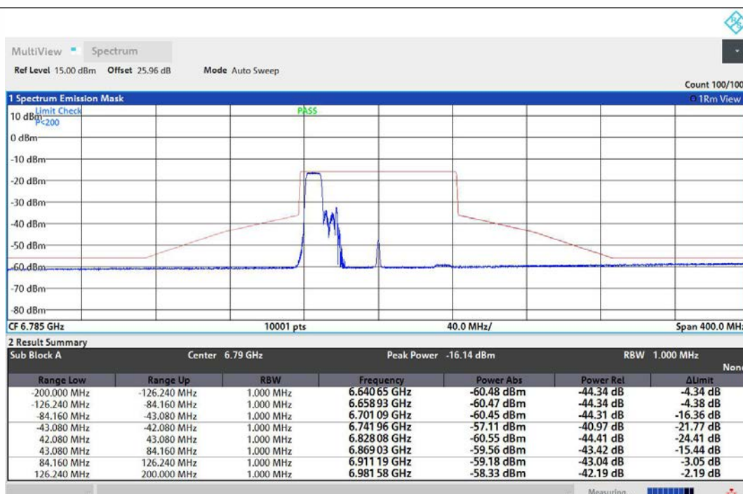
NTNV-11AX80MIMO-Ant1-6785-106Tone-RU53-PASS
