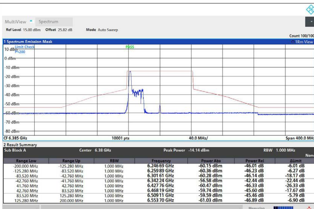
NTNV-11AX80MIMO-Ant1-6385-26Tone-RU0-PASS
