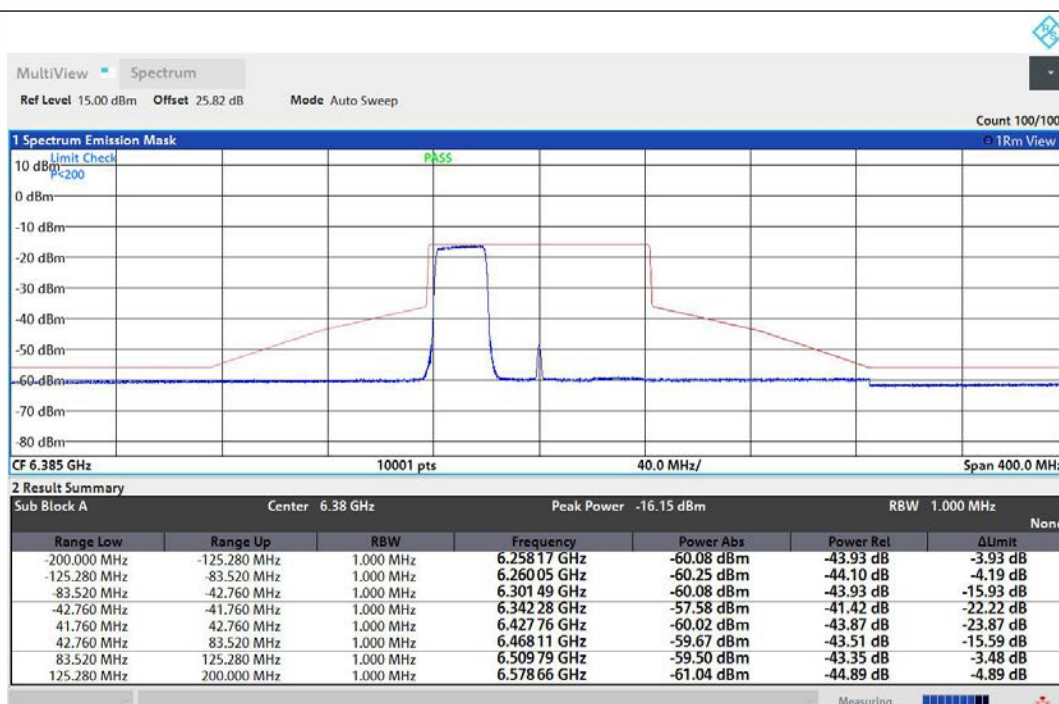
NTNV-11AX80MIMO-Ant1-6385-242Tone-RU61-PASS
