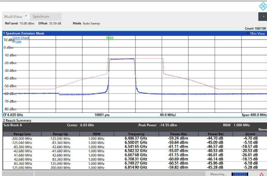
NTNV-11AX80MIMO-Ant1-6625-484Tone-RU65-PASS
