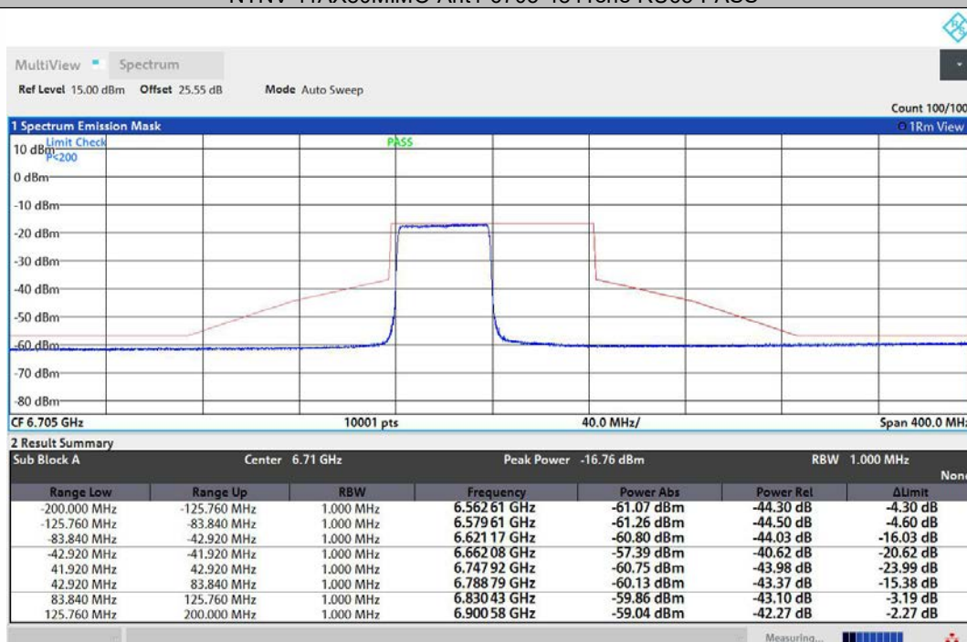
NTNV-11AX80MIMO-Ant2-6705-484Tone-RU65-PASS
