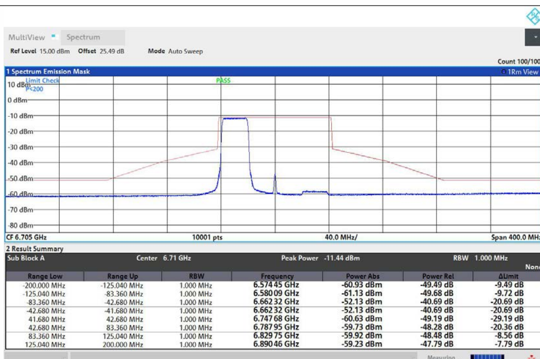
NTNV-11AX80MIMO-Ant1-6705-242Tone-RU61-PASS
