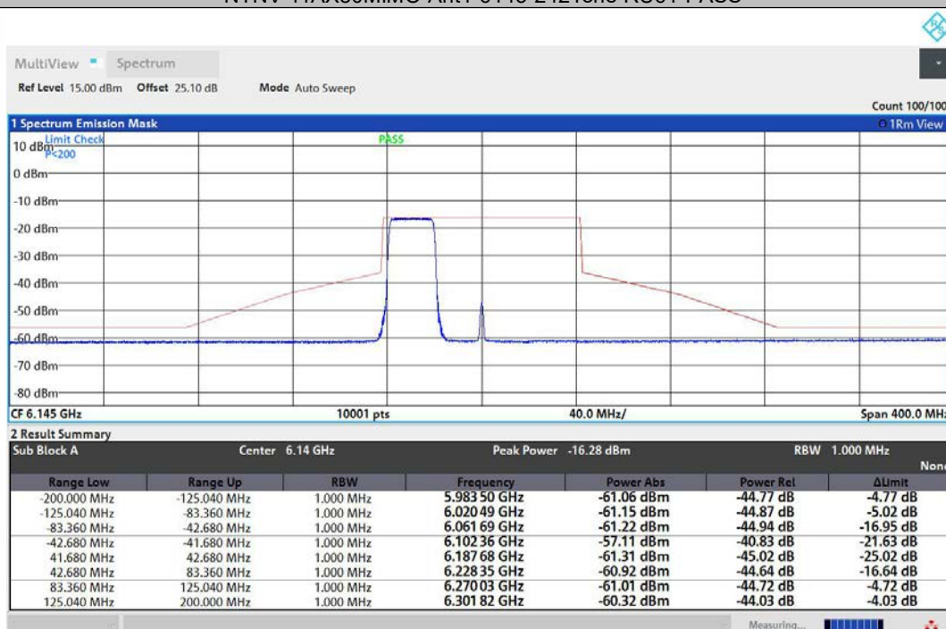
NTNV-11AX80MIMO-Ant2-6145-242Tone-RU61-PASS
