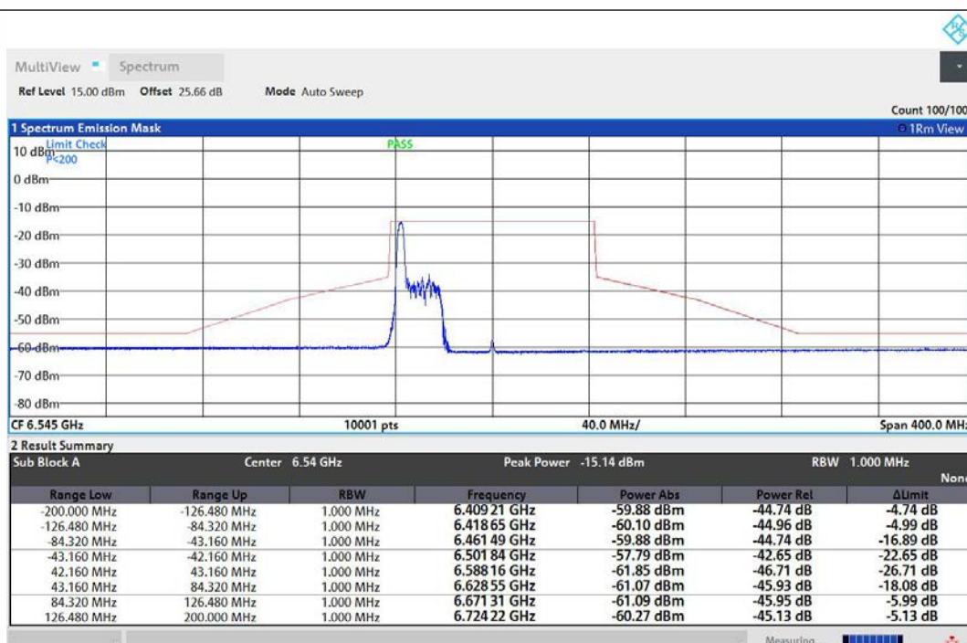
NTNV-11AX80MIMO-Ant1-6545-26Tone-RU0-PASS
