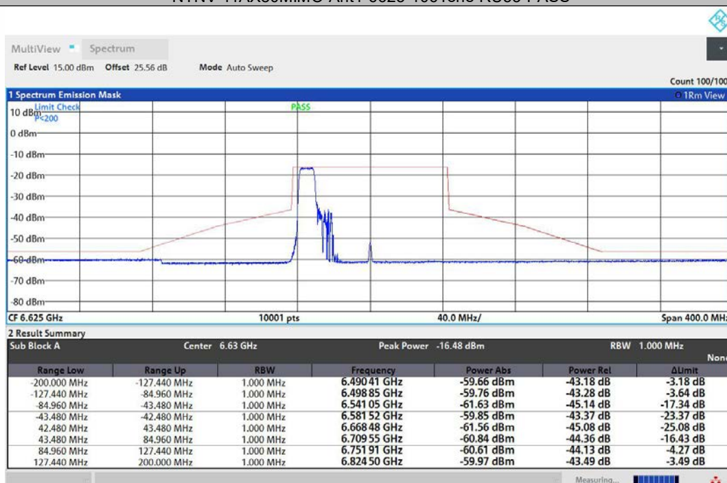
NTNV-11AX80MIMO-Ant2-6625-106Tone-RU53-PASS
