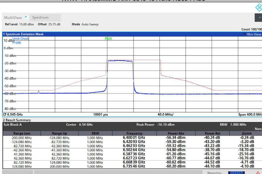
NTNV-11AX80MIMO-Ant2-6545-484Tone-RU65-PASS
