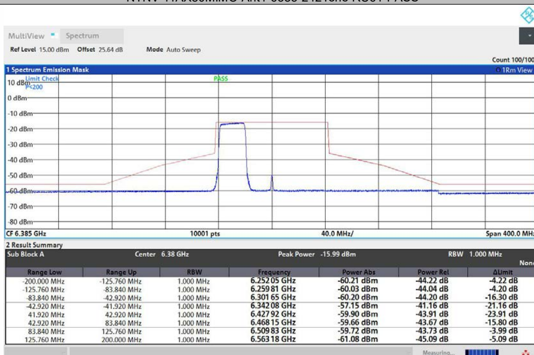
NTNV-11AX80MIMO-Ant2-6385-242Tone-RU61-PASS
