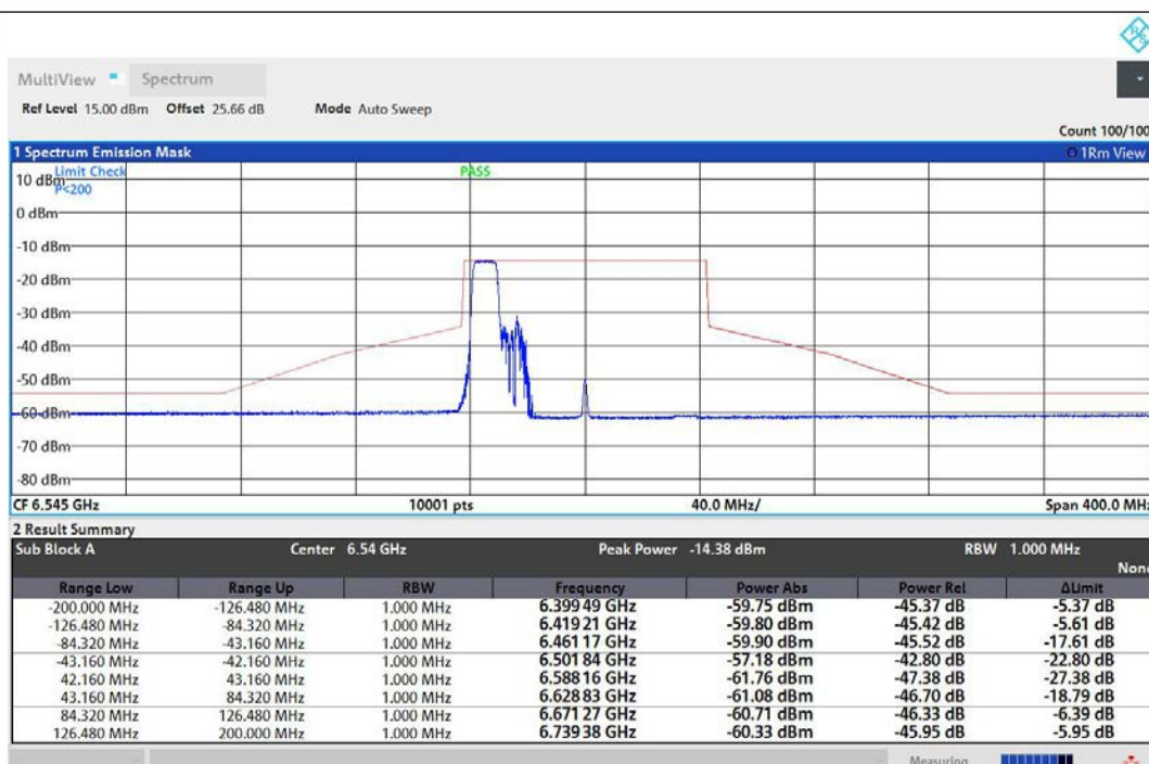
NTNV-11AX80MIMO-Ant1-6545-106Tone-RU53-PASS
