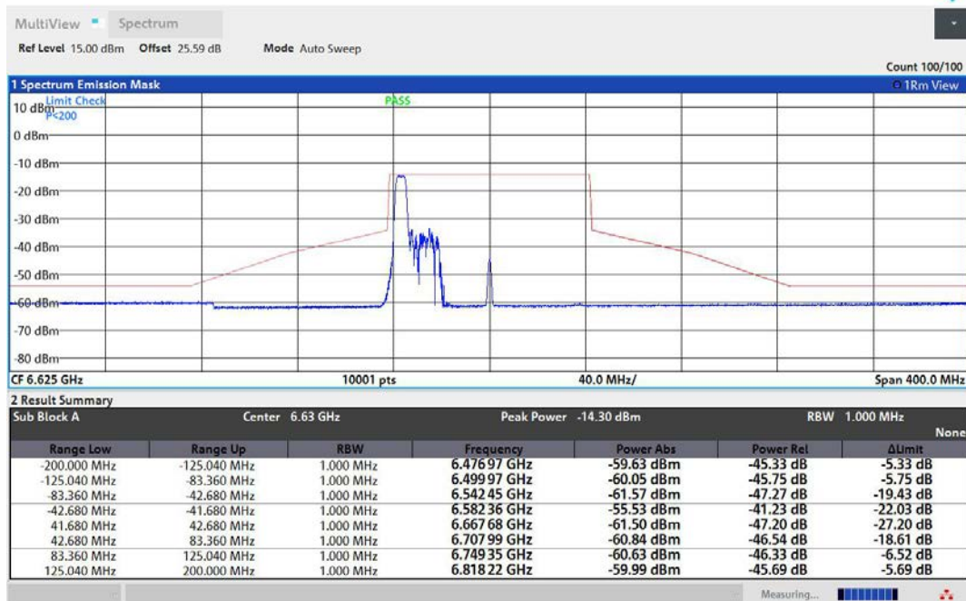
NTNV-11AX80MIMO-Ant1-6625-52Tone-RU37-PASS
