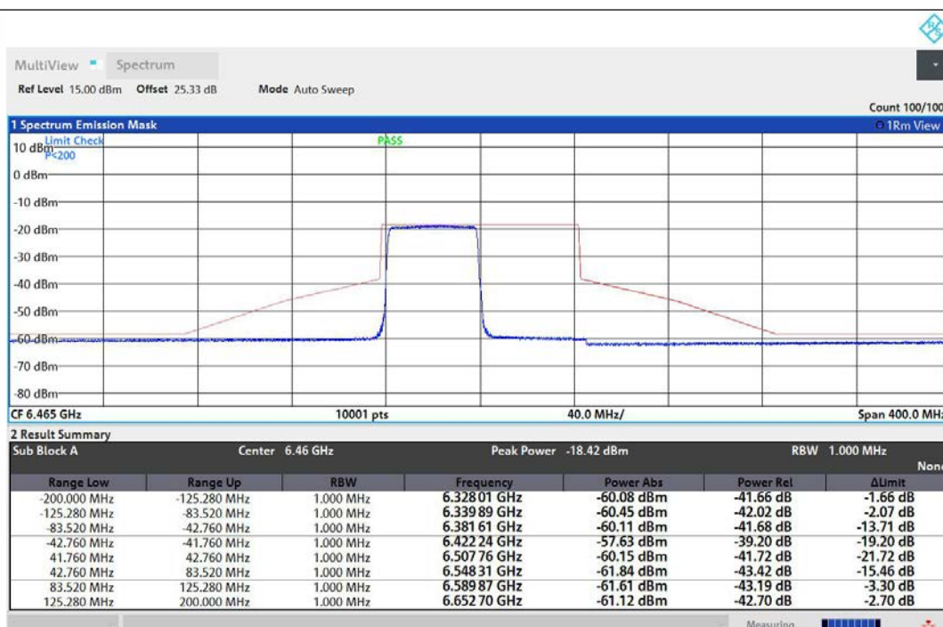
NTNV-11AX80MIMO-Ant1-6465-484Tone-RU65-PASS
