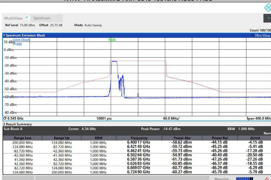
NTNV-11AX80MIMO-Ant2-6545-106Tone-RU53-PASS
