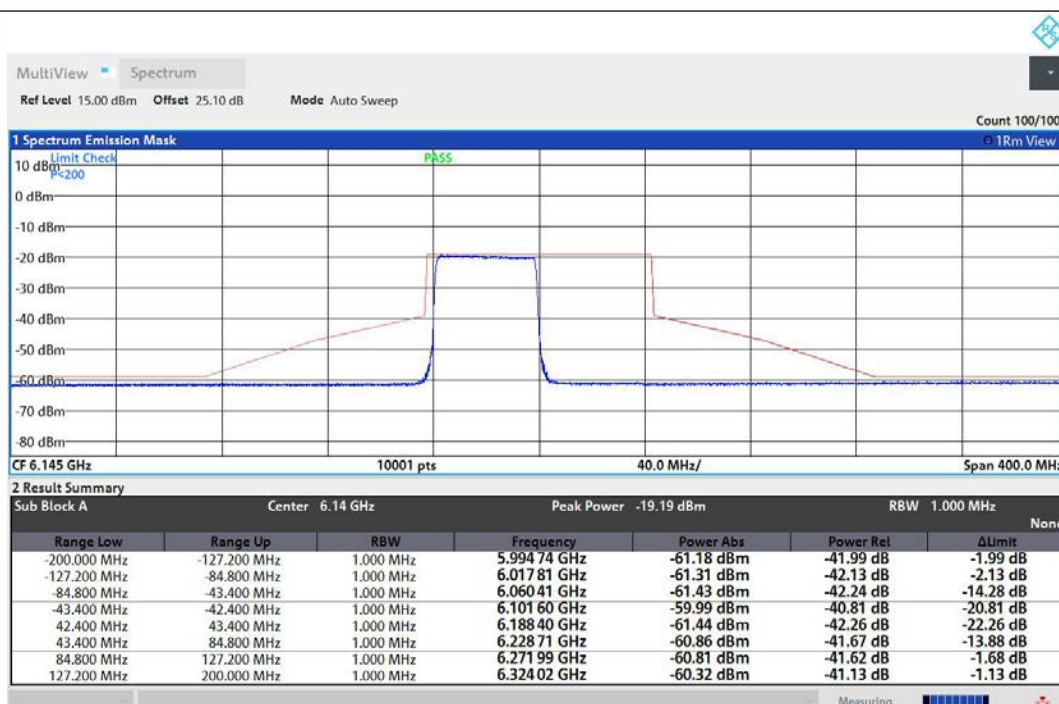
NTNV-11AX80MIMO-Ant1-6145-484Tone-RU65-PASS
