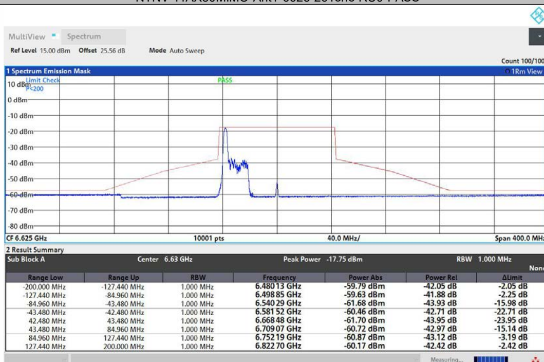
NTNV-11AX80MIMO-Ant2-6625-26Tone-RU0-PASS
