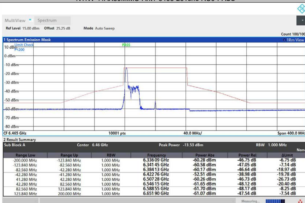
NTNV-11AX80MIMO-Ant2-6465-26Tone-RU0-PASS
