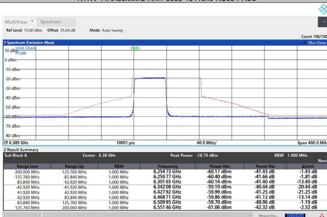
NTNV-11AX80MIMO-Ant2-6385-484Tone-RU65-PASS
