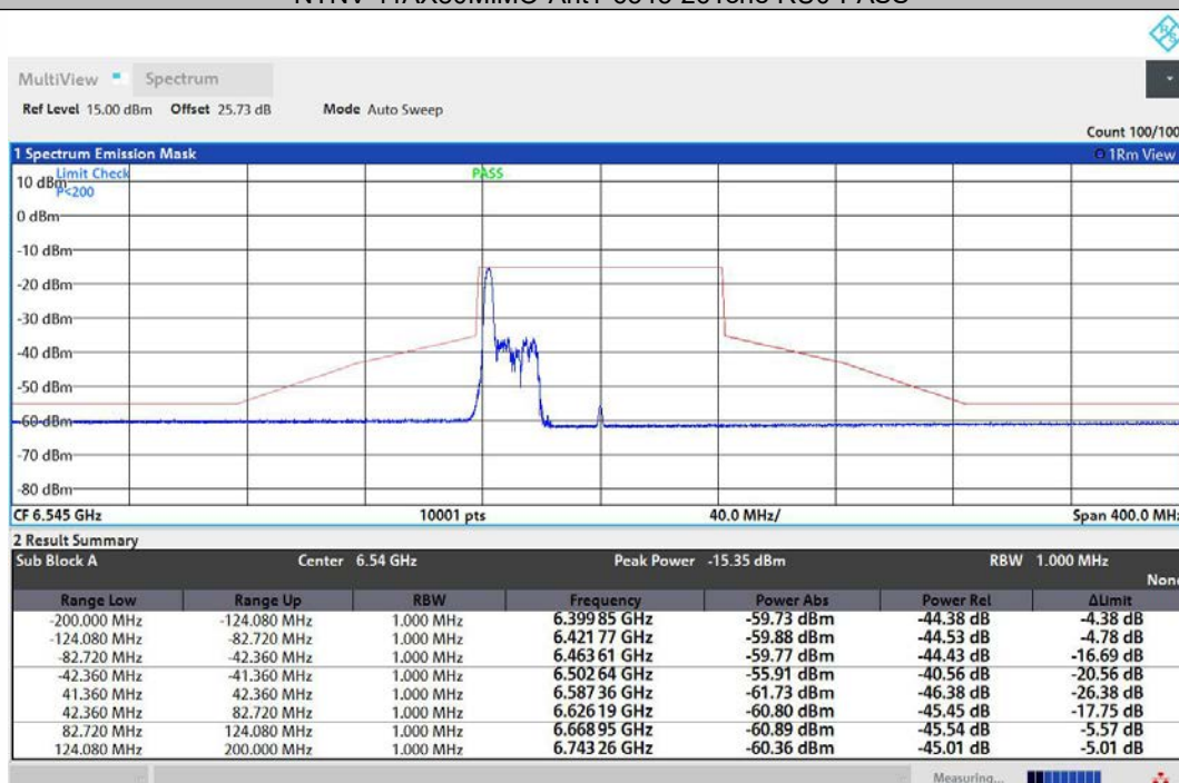
NTNV-11AX80MIMO-Ant2-6545-26Tone-RU0-PASS
