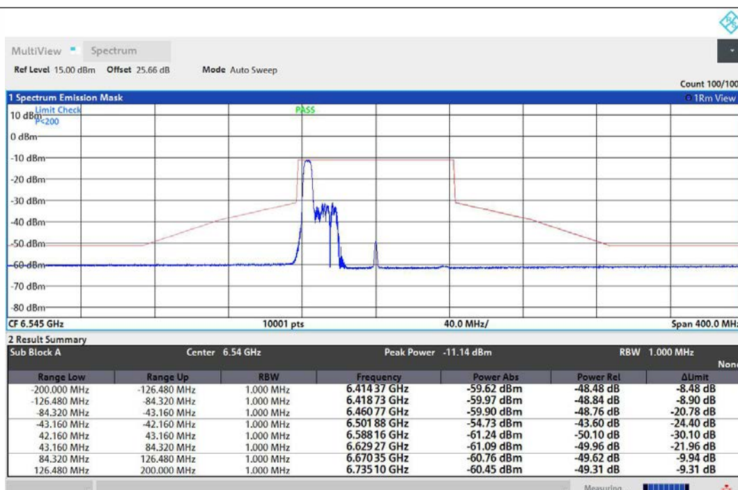
NTNV-11AX80MIMO-Ant1-6545-52Tone-RU37-PASS
