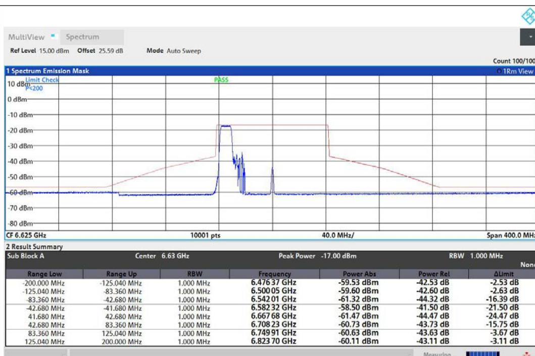
NTNV-11AX80MIMO-Ant1-6625-106Tone-RU53-PASS
