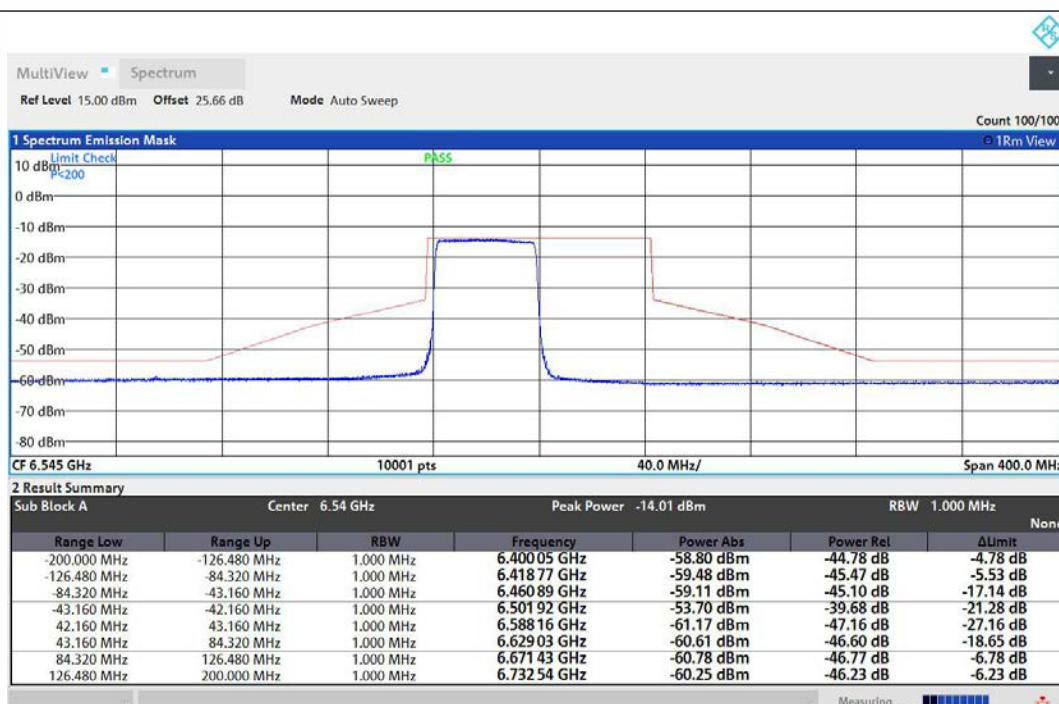
NTNV-11AX80MIMO-Ant1-6545-484Tone-RU65-PASS
