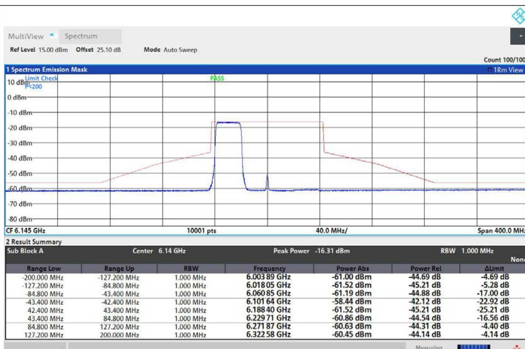
NTNV-11AX80MIMO-Ant1-6145-242Tone-RU61-PASS
