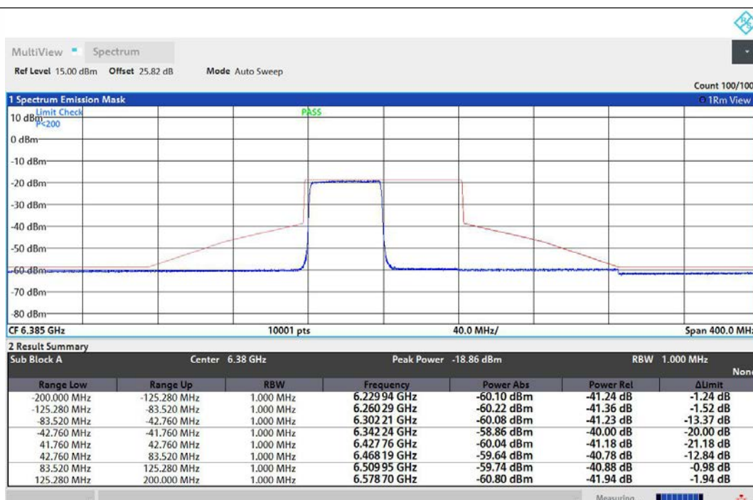
NTNV-11AX80MIMO-Ant1-6385-484Tone-RU65-PASS
