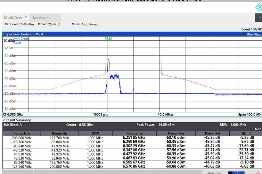
NTNV-11AX80MIMO-Ant2-6385-26Tone-RU0-PASS
