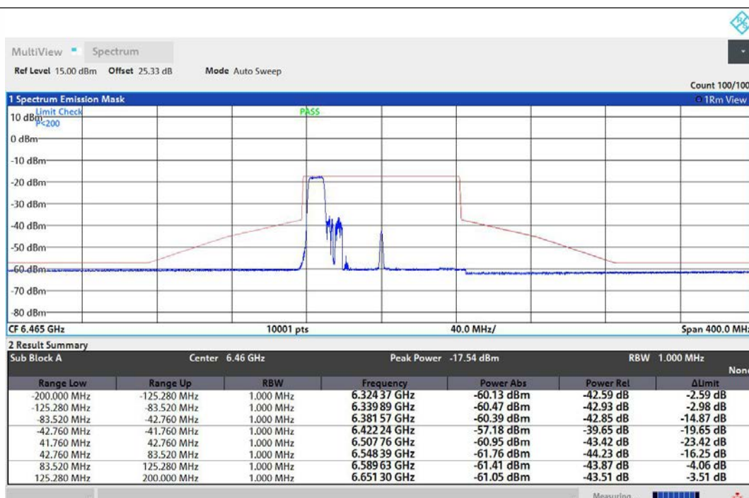
NTNV-11AX80MIMO-Ant1-6465-106Tone-RU53-PASS
