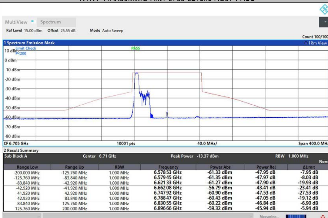
NTNV-11AX80MIMO-Ant2-6705-52Tone-RU37-PASS
