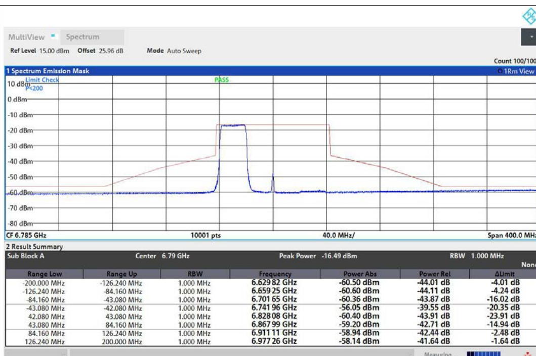
NTNV-11AX80MIMO-Ant1-6785-242Tone-RU61-PASS
