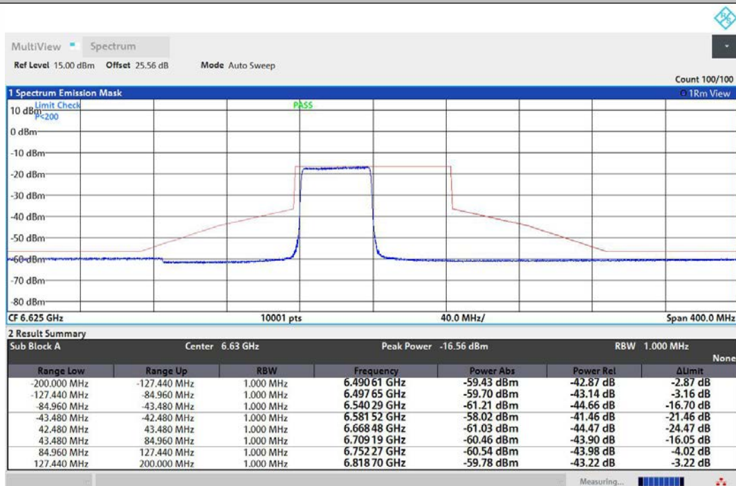
NTNV-11AX80MIMO-Ant2-6625-484Tone-RU65-PASS
