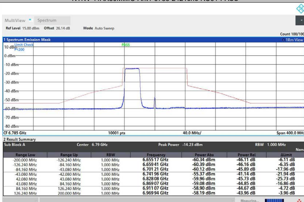
NTNV-11AX80MIMO-Ant2-6785-242Tone-RU61-PASS
