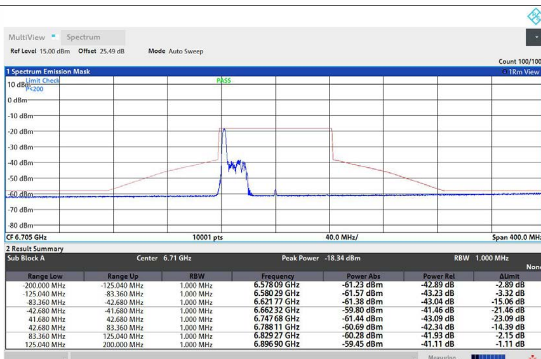
NTNV-11AX80MIMO-Ant1-6705-26Tone-RU0-PASS
