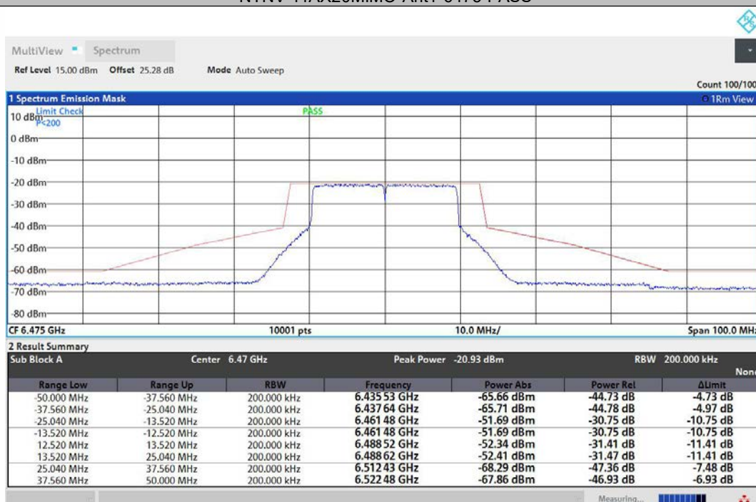
NTNV-11AX20MIMO-Ant2-6475-PASS
