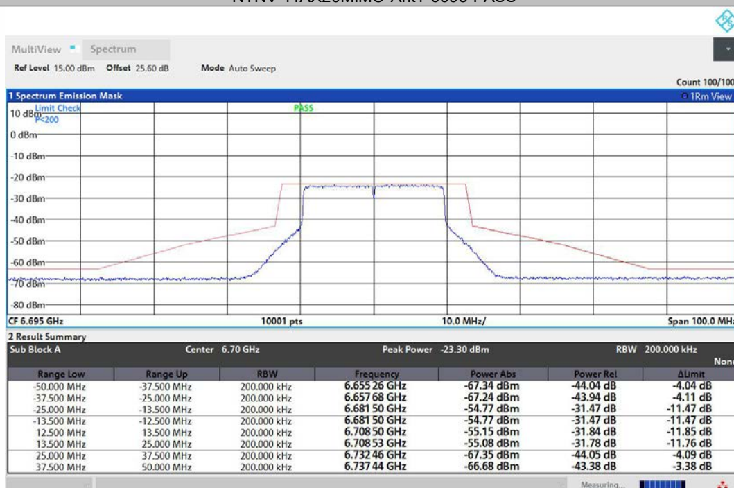
NTNV-11AX20MIMO-Ant2-6695-PASS
