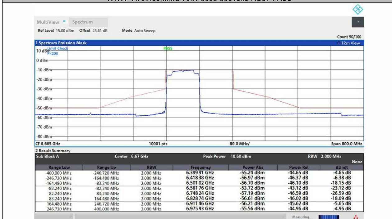
NTNV-11AX160MIMO-Ant2-6665-996Tone-RU67-PASS
