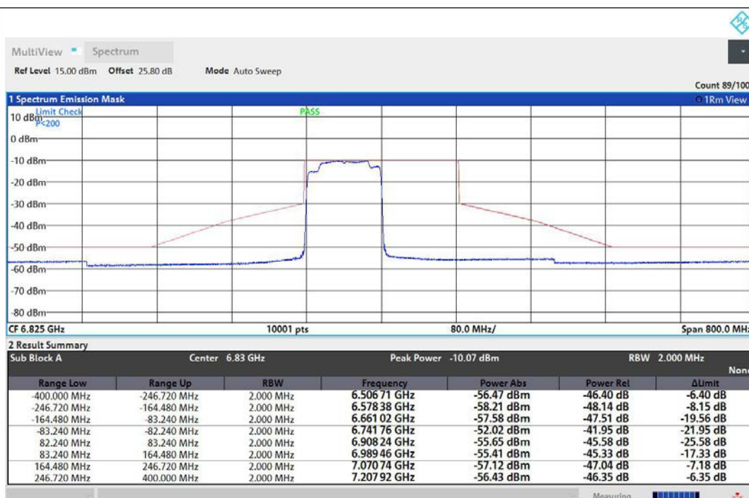
NTNV-11AX160MIMO-Ant1-6825-996Tone-RU67-PASS
