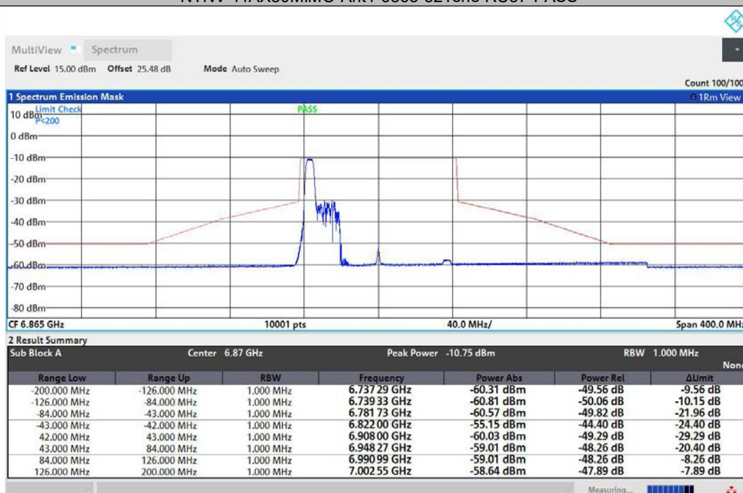
NTNV-11AX80MIMO-Ant2-6865-52Tone-RU37-PASS
