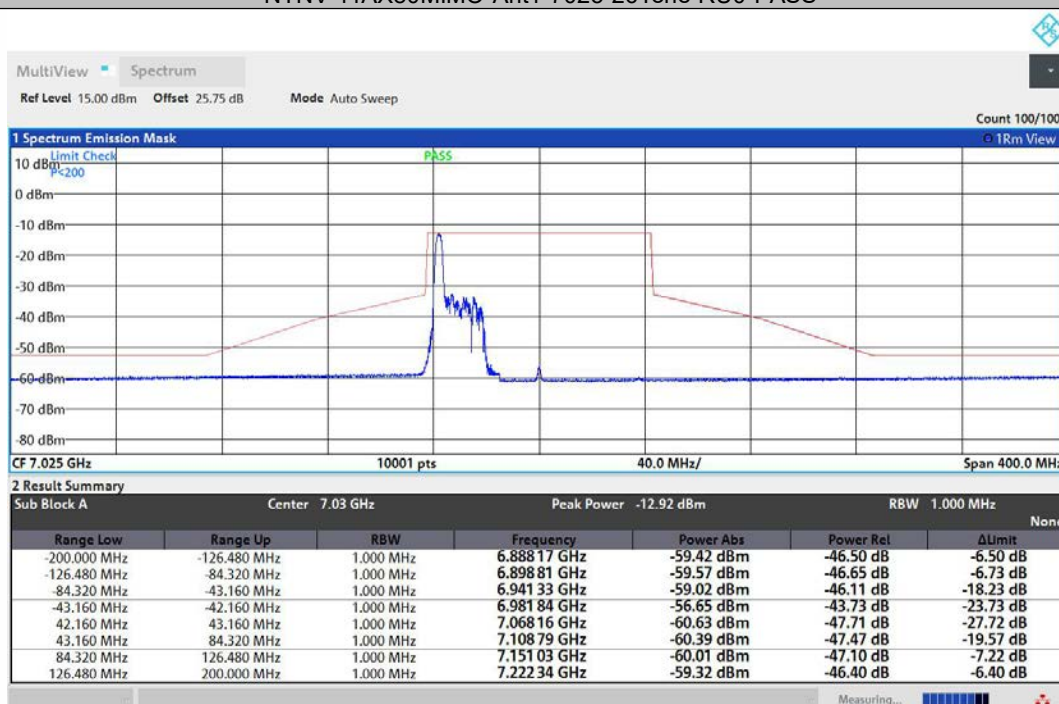
NTNV-11AX80MIMO-Ant2-7025-26Tone-RU0-PASS
