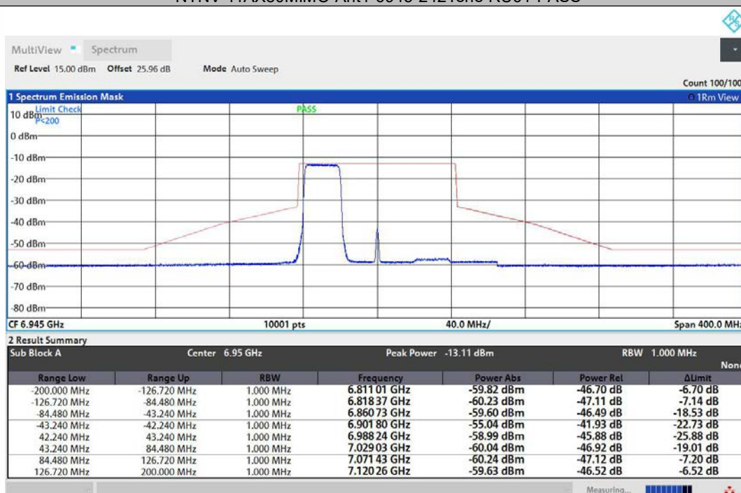
NTNV-11AX80MIMO-Ant2-6945-242Tone-RU61-PASS
