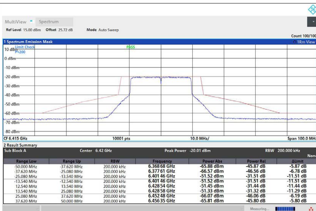
NTNV-11AX20MIMO-Ant1-6415-PASS
