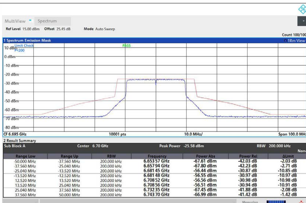
NTNV-11AX20MIMO-Ant1-6695-PASS
