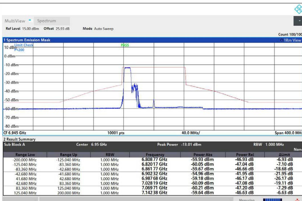
NTNV-11AX80MIMO-Ant1-6945-106Tone-RU53-PASS
