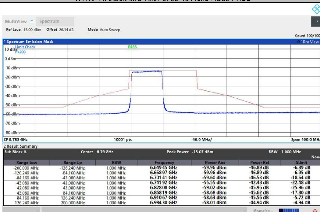
NTNV-11AX80MIMO-Ant2-6785-484Tone-RU65-PASS
