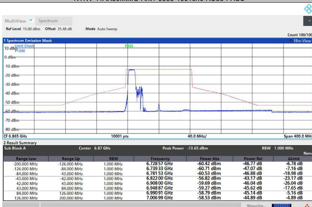
NTNV-11AX80MIMO-Ant2-6865-106Tone-RU53-PASS
