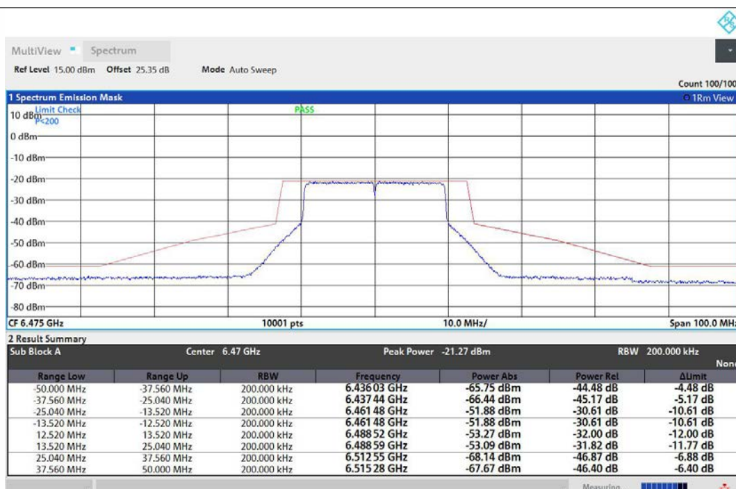
NTNV-11AX20MIMO-Ant1-6475-PASS
