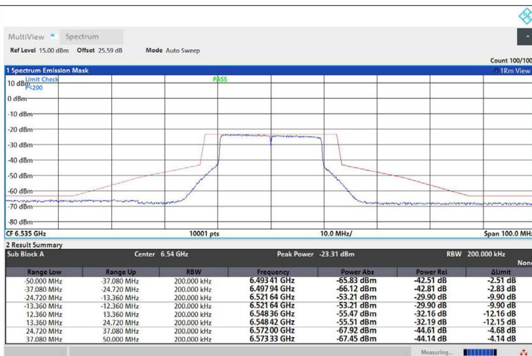
NTNV-11AX20MIMO-Ant1-6535-PASS
