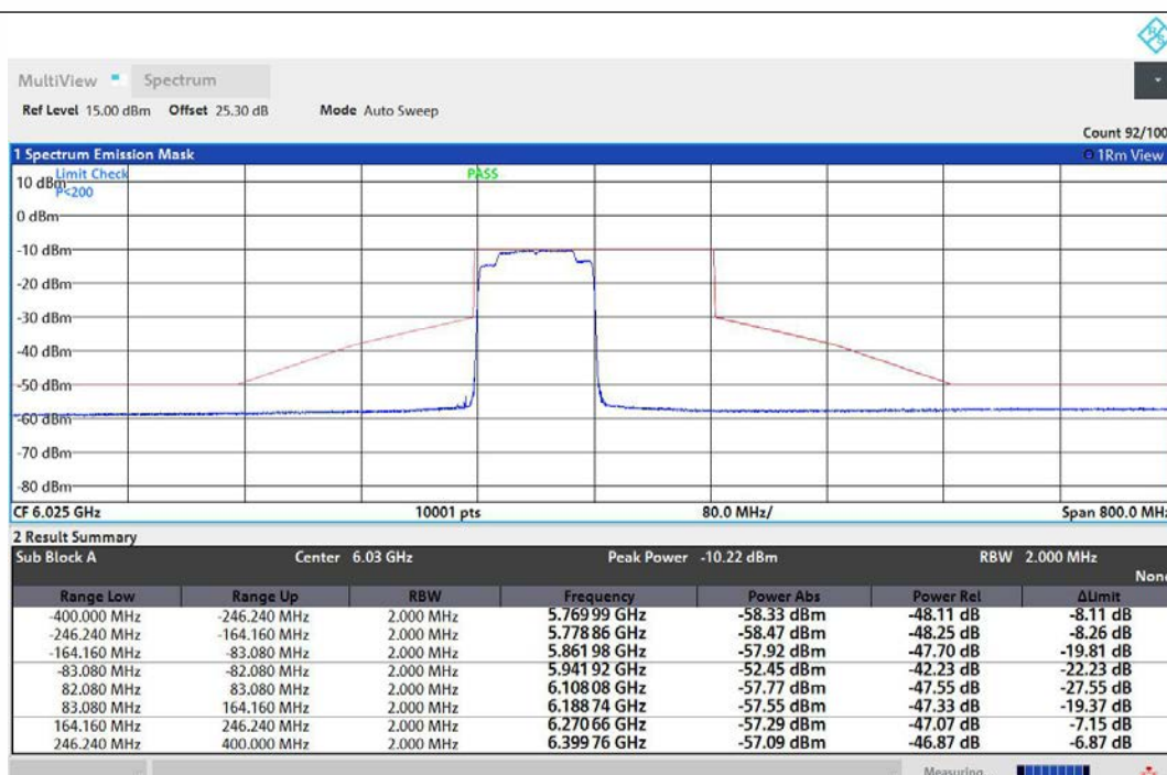
NTNV-11AX160MIMO-Ant1-6025-996Tone-RU67-PASS
