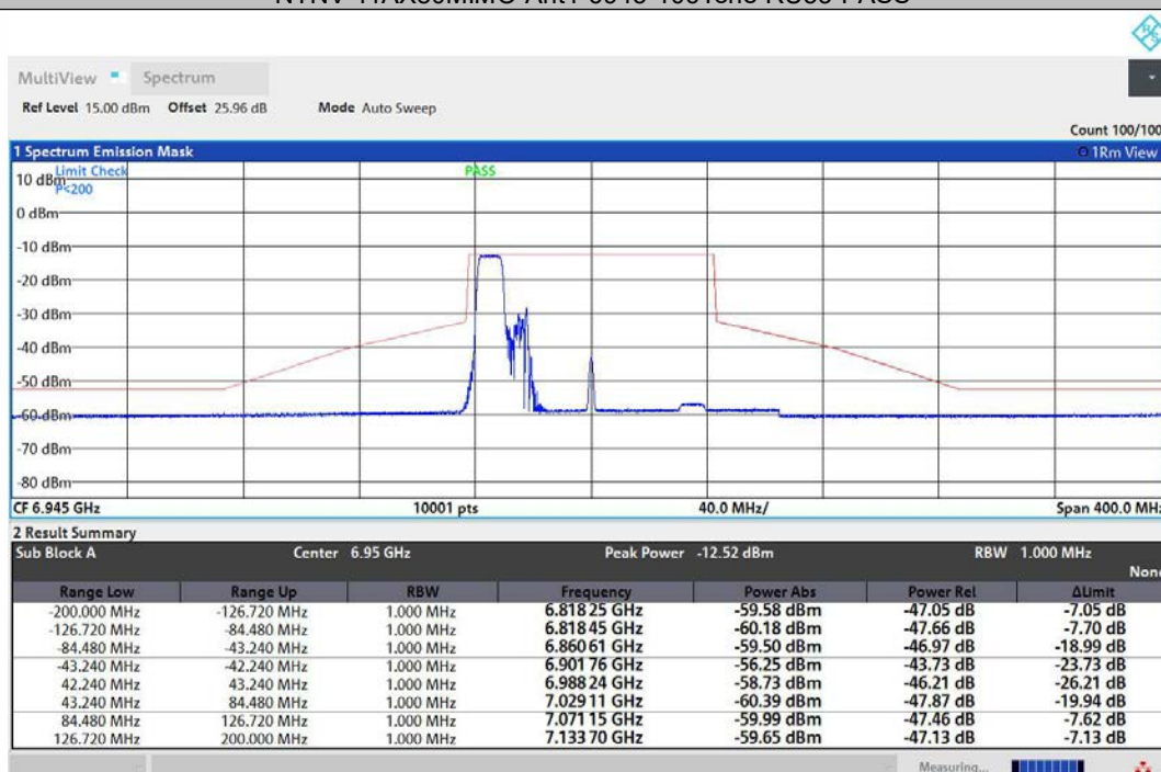
NTNV-11AX80MIMO-Ant2-6945-106Tone-RU53-PASS
