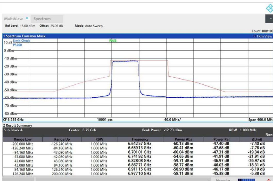
NTNV-11AX80MIMO-Ant1-6785-484Tone-RU65-PASS
