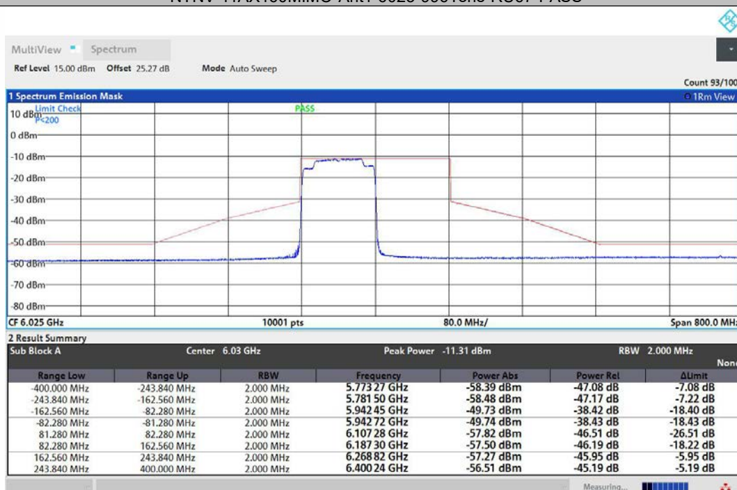
NTNV-11AX160MIMO-Ant2-6025-996Tone-RU67-PASS
