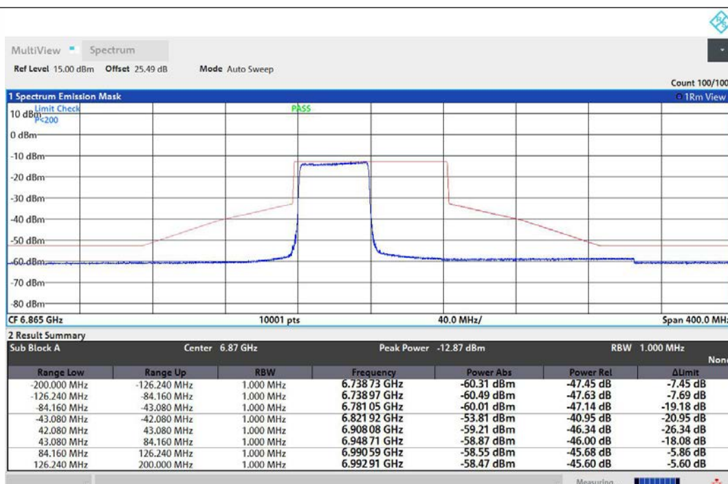
NTNV-11AX80MIMO-Ant1-6865-484Tone-RU65-PASS
