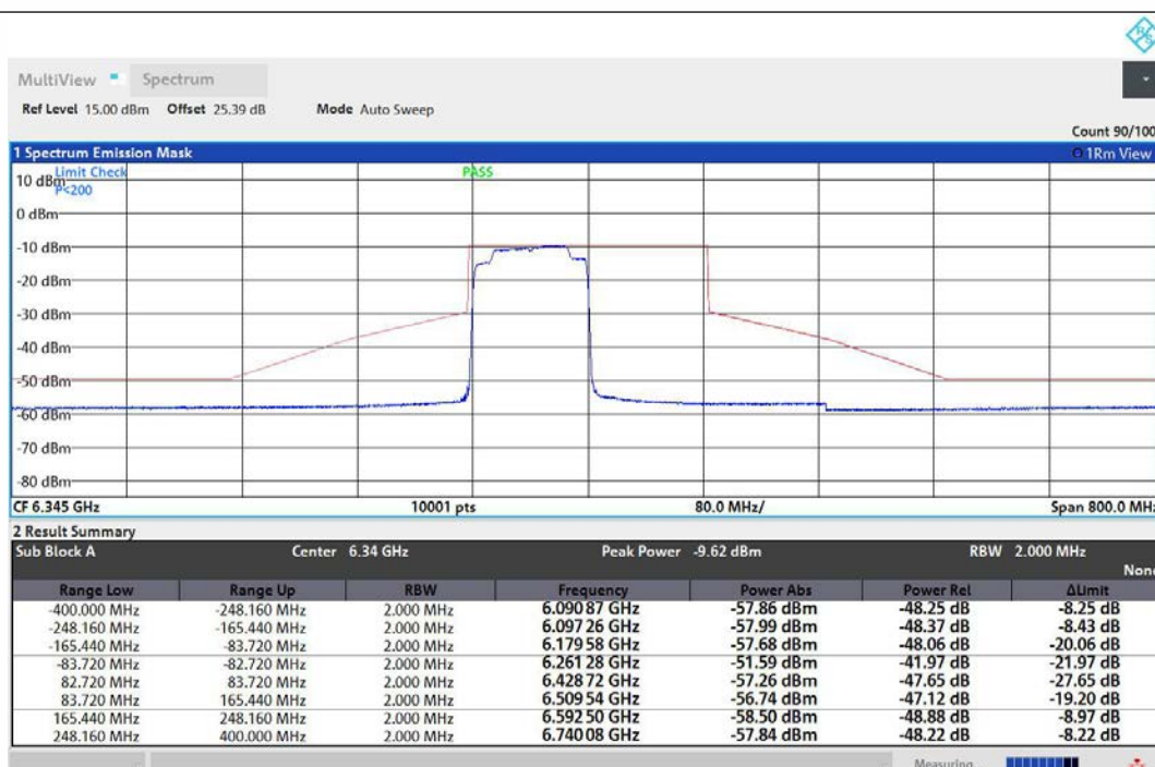
NTNV-11AX160MIMO-Ant1-6345-996Tone-RU67-PASS
