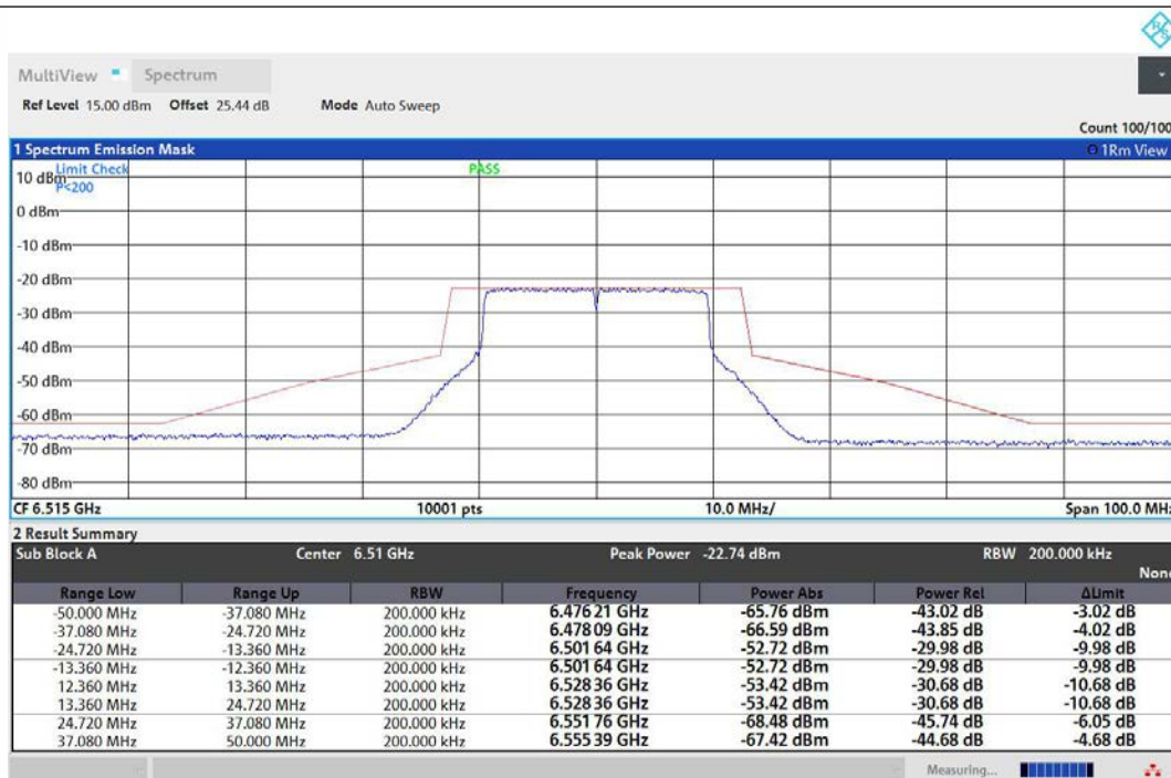
NTNV-11AX20MIMO-Ant1-6515-PASS
