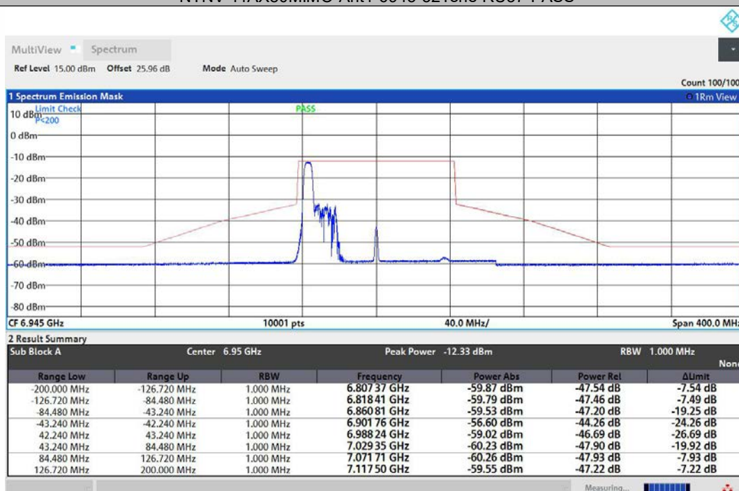
NTNV-11AX80MIMO-Ant2-6945-52Tone-RU37-PASS
