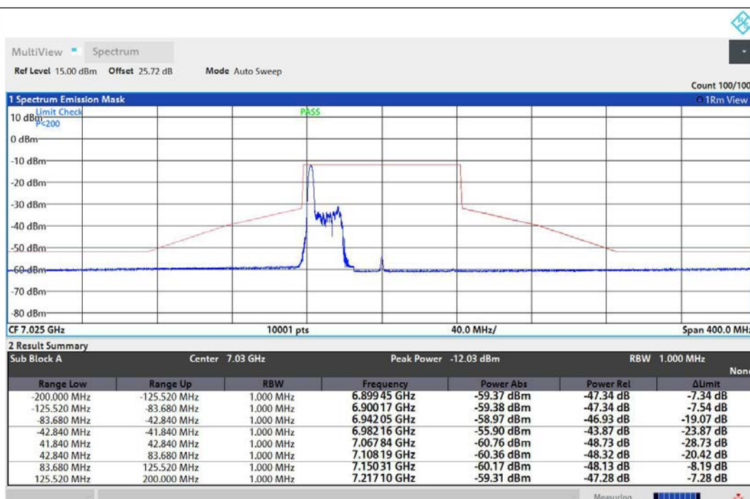
NTNV-11AX80MIMO-Ant1-7025-26Tone-RU0-PASS
