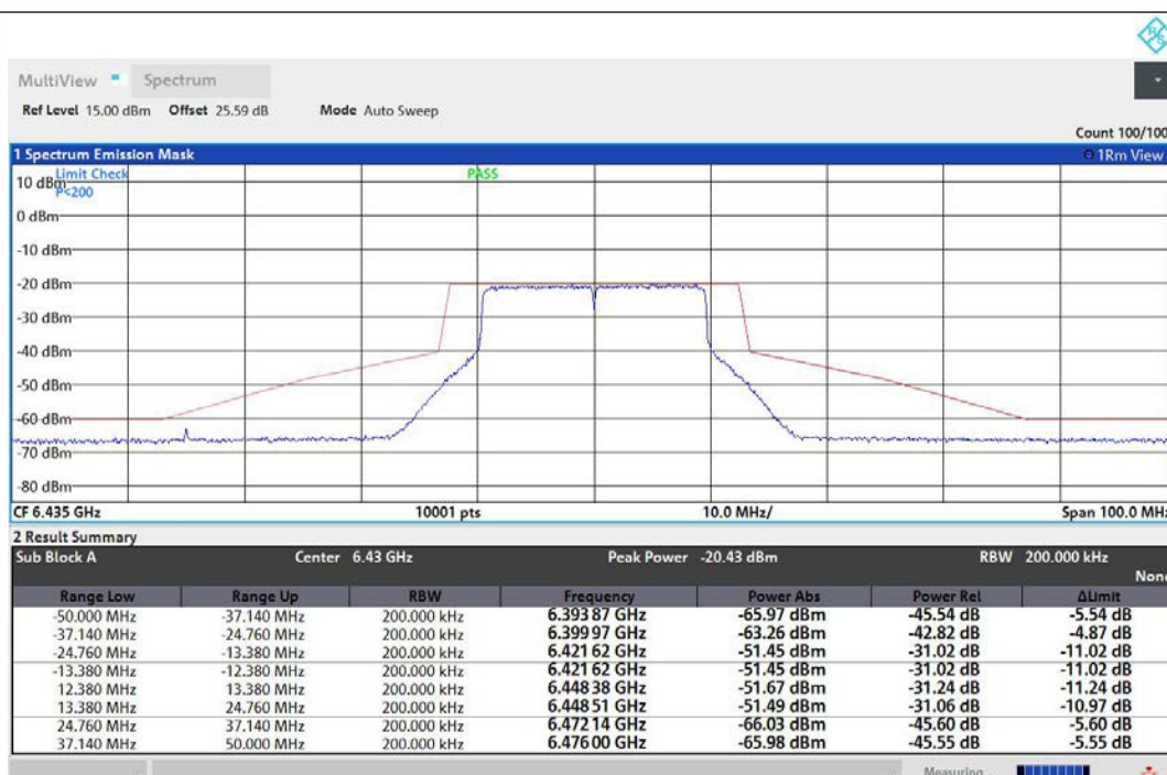
NTNV-11AX20MIMO-Ant1-6435-PASS
