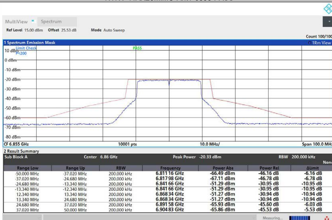
NTNV-11AX20MIMO-Ant2-6855-PASS
