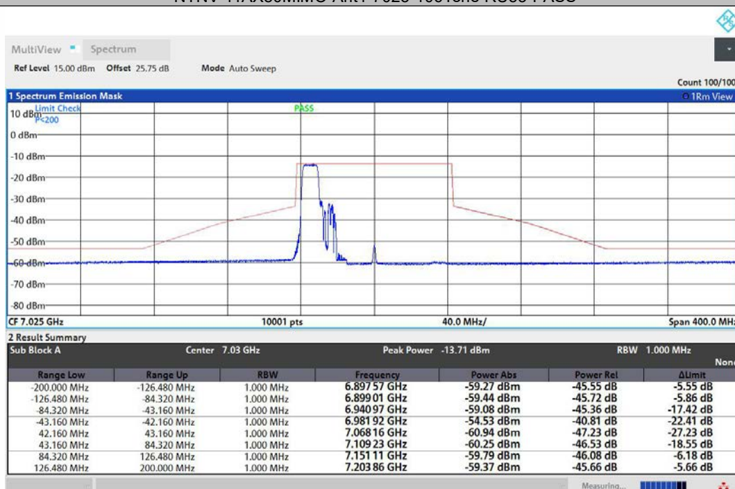
NTNV-11AX80MIMO-Ant2-7025-106Tone-RU53-PASS
