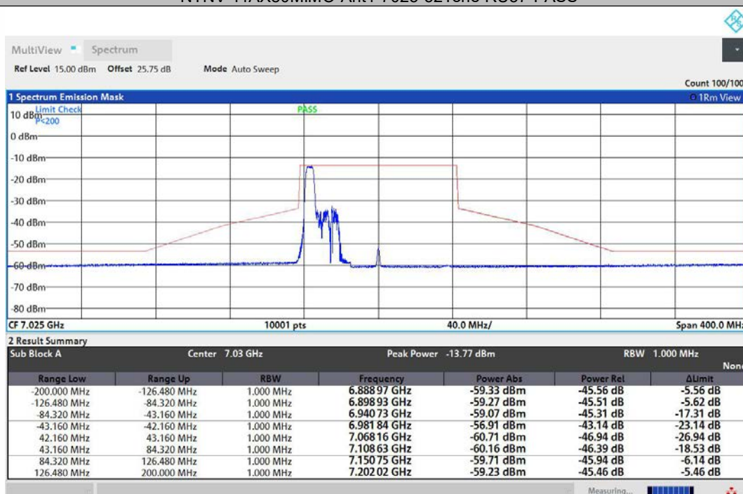
NTNV-11AX80MIMO-Ant2-7025-52Tone-RU37-PASS
