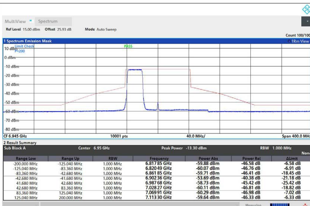
NTNV-11AX80MIMO-Ant1-6945-242Tone-RU61-PASS
