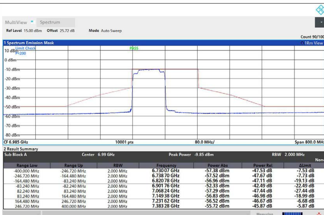
NTNV-11AX160MIMO-Ant1-6985-996Tone-RU67-PASS
