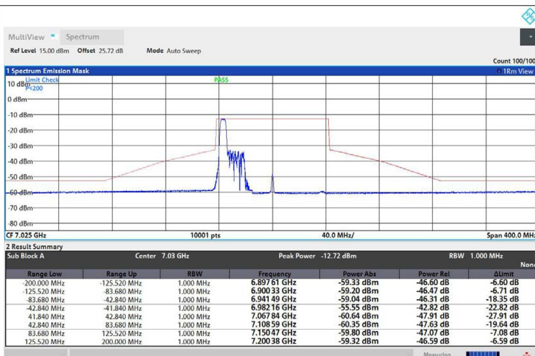
NTNV-11AX80MIMO-Ant1-7025-52Tone-RU37-PASS
