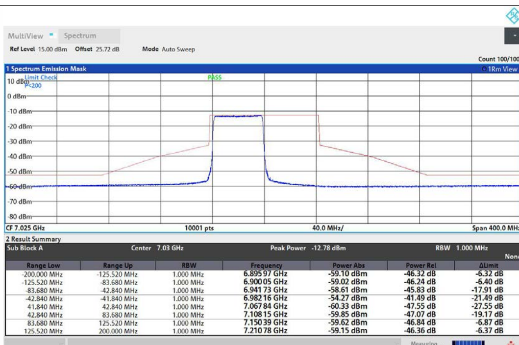
NTNV-11AX80MIMO-Ant1-7025-484Tone-RU65-PASS
