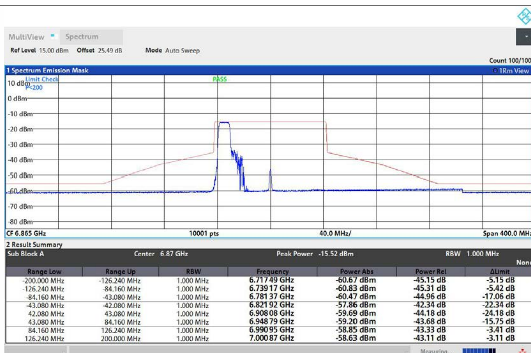
NTNV-11AX80MIMO-Ant1-6865-106Tone-RU53-PASS
