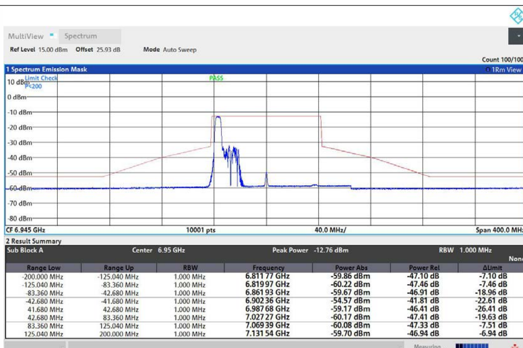
NTNV-11AX80MIMO-Ant1-6945-52Tone-RU37-PASS
