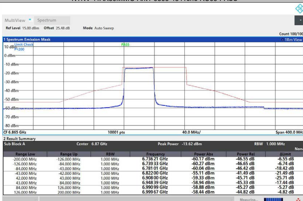
NTNV-11AX80MIMO-Ant2-6865-484Tone-RU65-PASS
