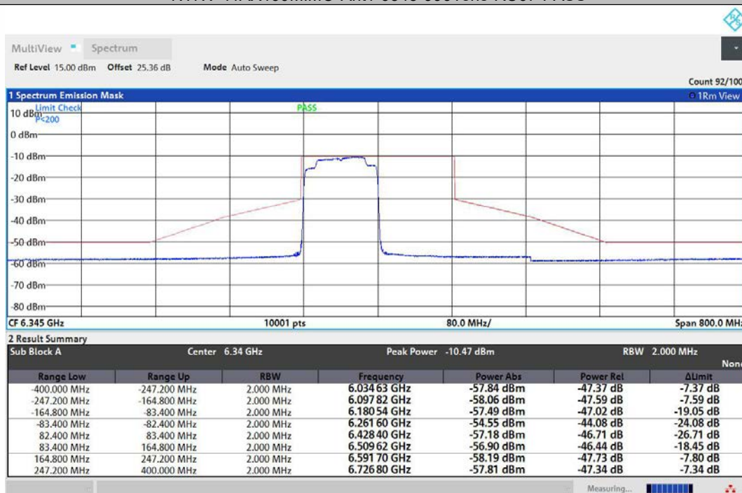
NTNV-11AX160MIMO-Ant2-6345-996Tone-RU67-PASS
