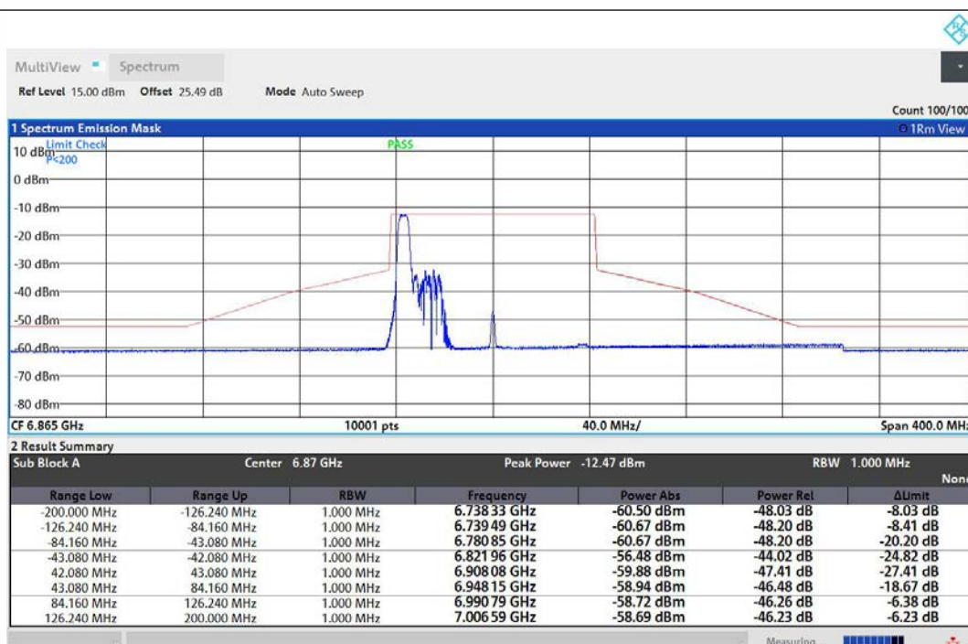
NTNV-11AX80MIMO-Ant1-6865-52Tone-RU37-PASS
