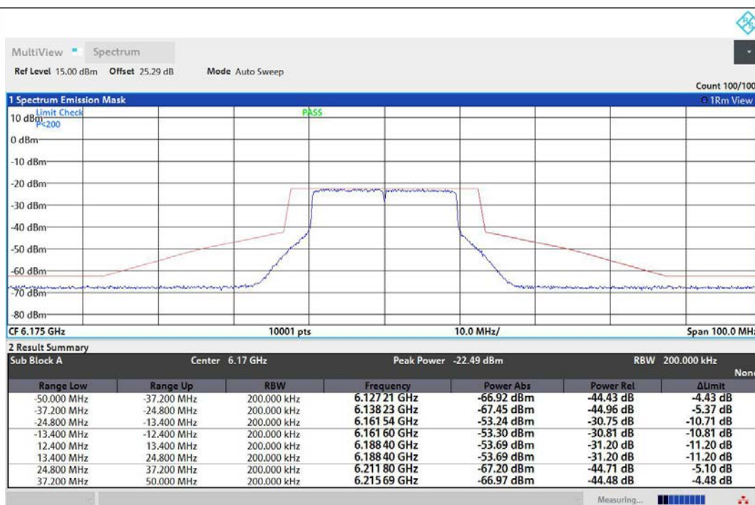
NTNV-11AX20MIMO-Ant1-6175-PASS
