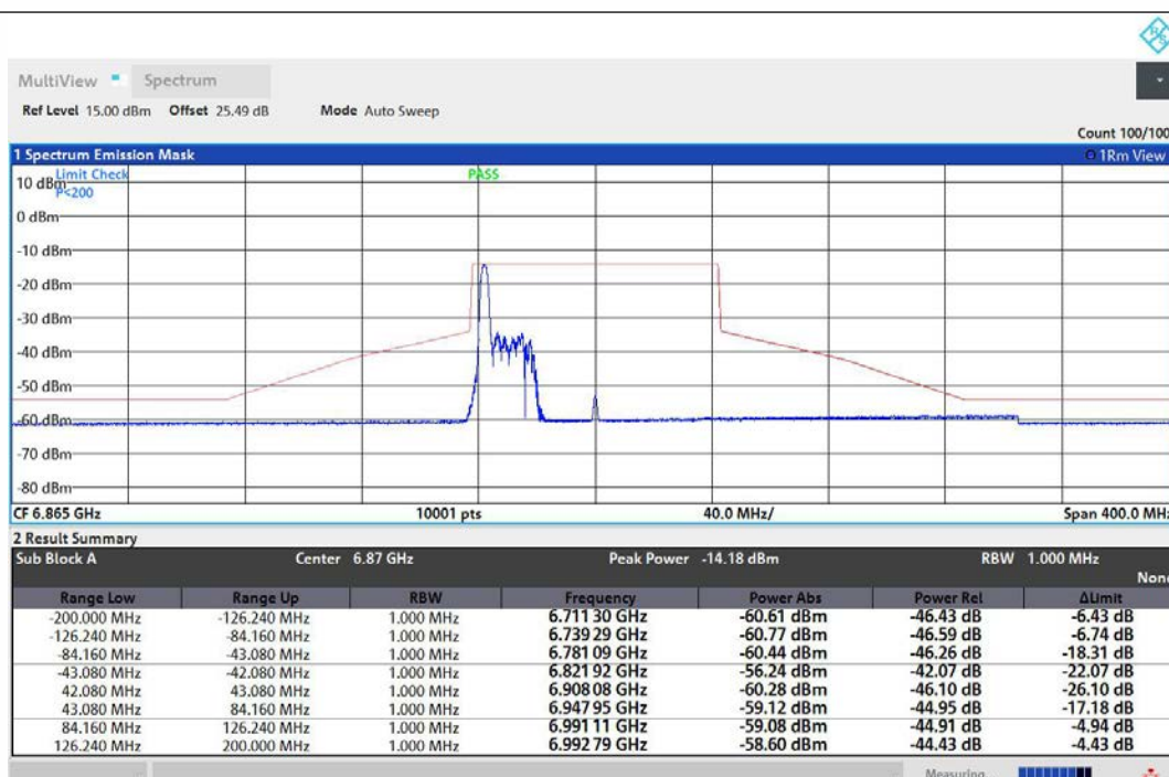
NTNV-11AX80MIMO-Ant1-6865-26Tone-RU0-PASS
