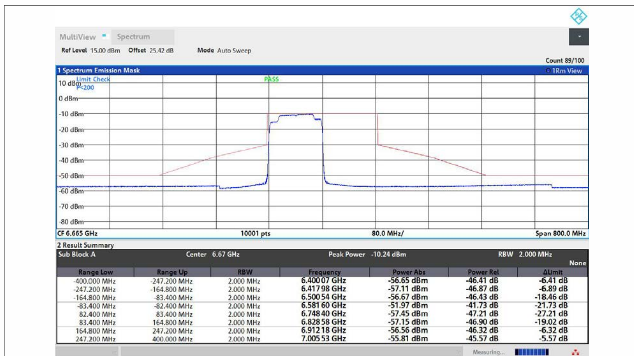
NTNV-11AX160MIMO-Ant1-6665-996Tone-RU67-PASS
