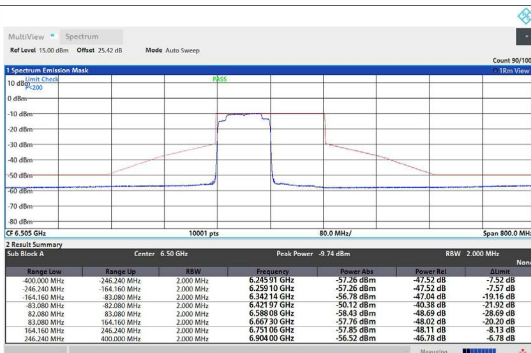
NTNV-11AX160MIMO-Ant1-6505-996Tone-RU67-PASS
