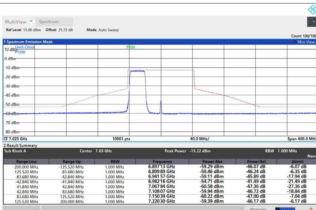
NTNV-11AX80MIMO-Ant1-7025-242Tone-RU61-PASS
