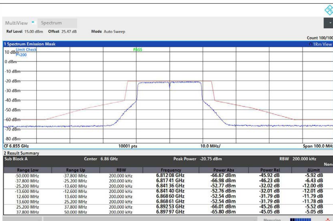
NTNV-11AX20MIMO-Ant1-6855-PASS
