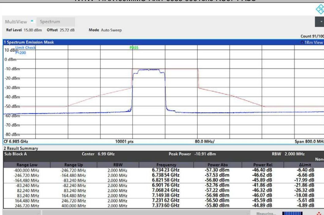
NTNV-11AX160MIMO-Ant2-6985-996Tone-RU67-PASS
