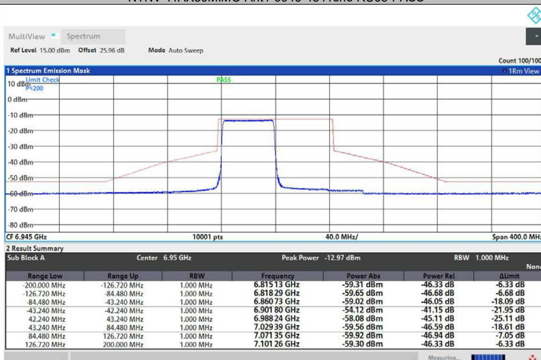
NTNV-11AX80MIMO-Ant2-6945-484Tone-RU65-PASS
