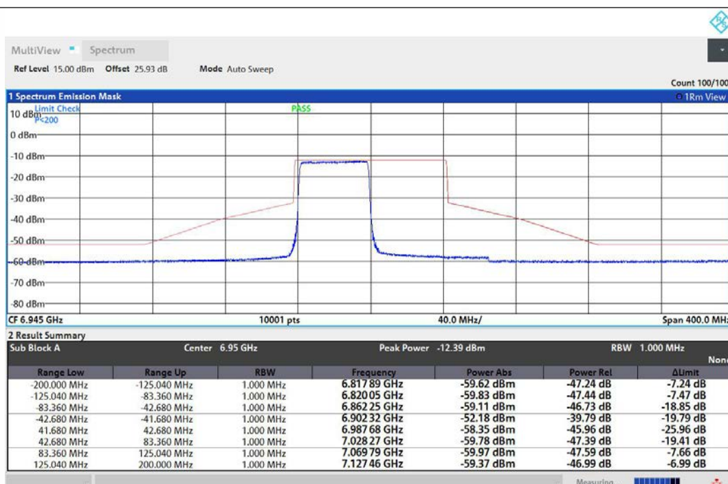
NTNV-11AX80MIMO-Ant1-6945-484Tone-RU65-PASS
