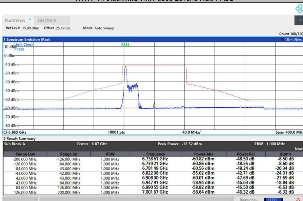
NTNV-11AX80MIMO-Ant2-6865-26Tone-RU0-PASS
