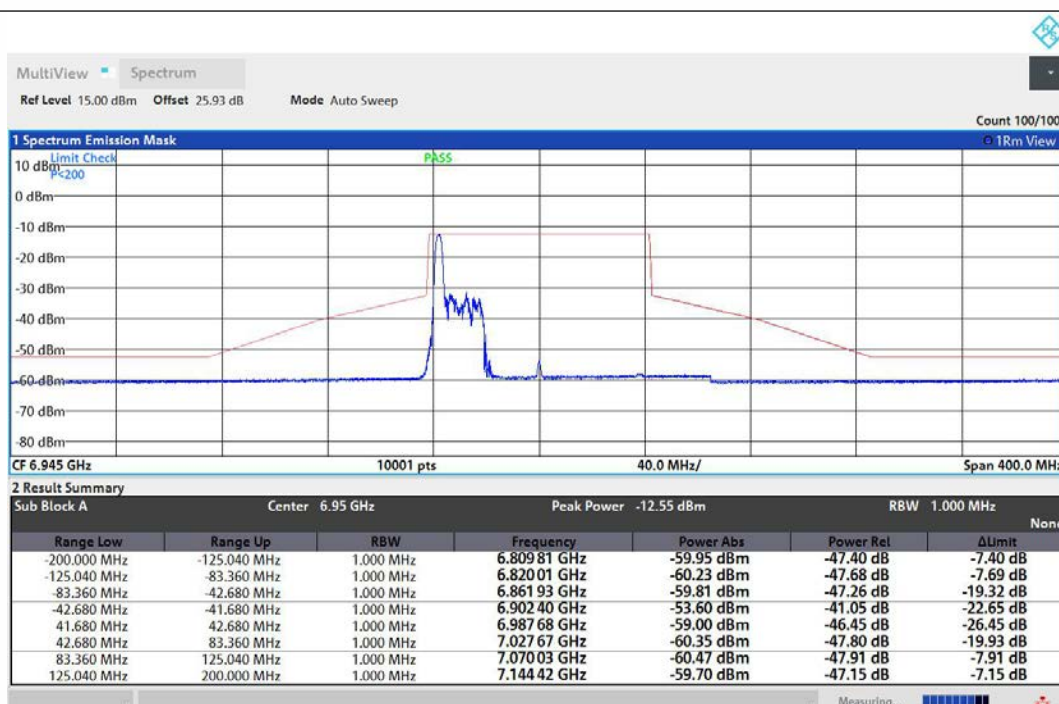
NTNV-11AX80MIMO-Ant1-6945-26Tone-RU0-PASS
