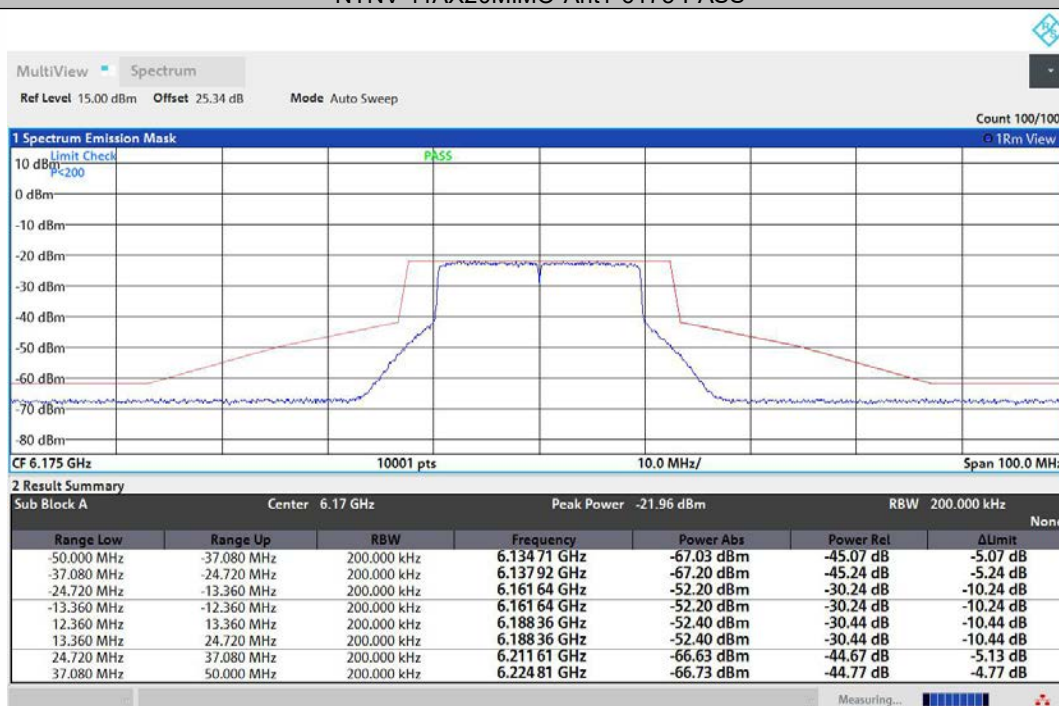
NTNV-11AX20MIMO-Ant2-6175-PASS
