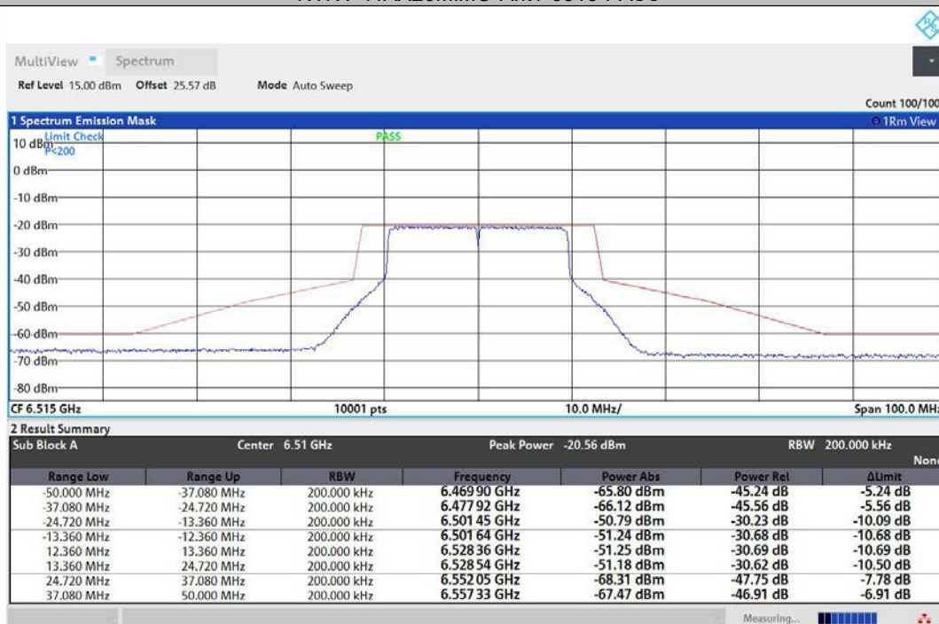
NTNV-11AX20MIMO-Ant2-6515-PASS
