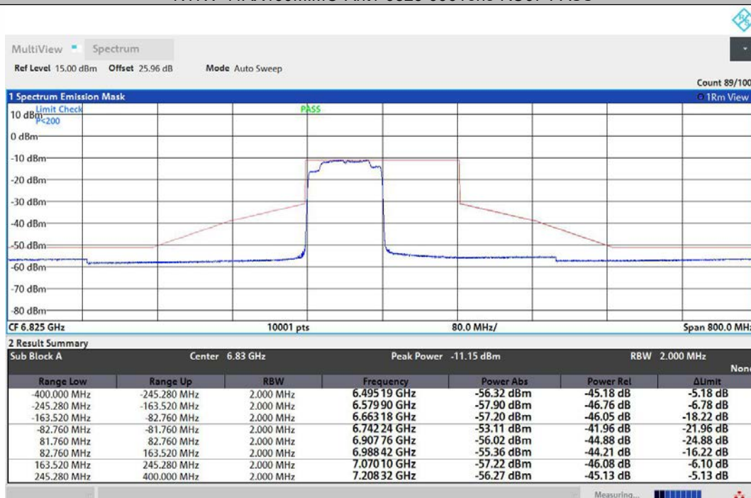
NTNV-11AX160MIMO-Ant2-6825-996Tone-RU67-PASS
