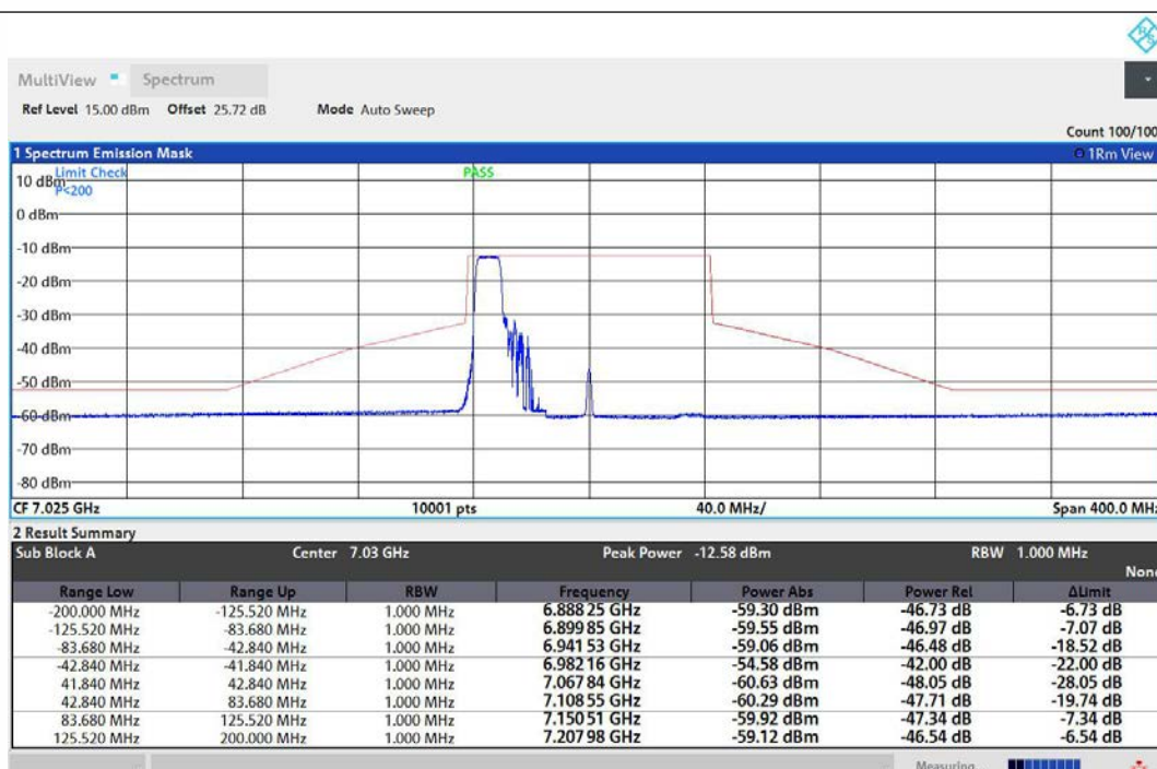
NTNV-11AX80MIMO-Ant1-7025-106Tone-RU53-PASS
