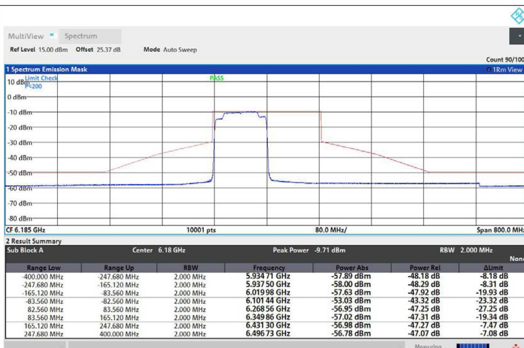
NTNV-11AX160MIMO-Ant1-6185-996Tone-RU67-PASS
