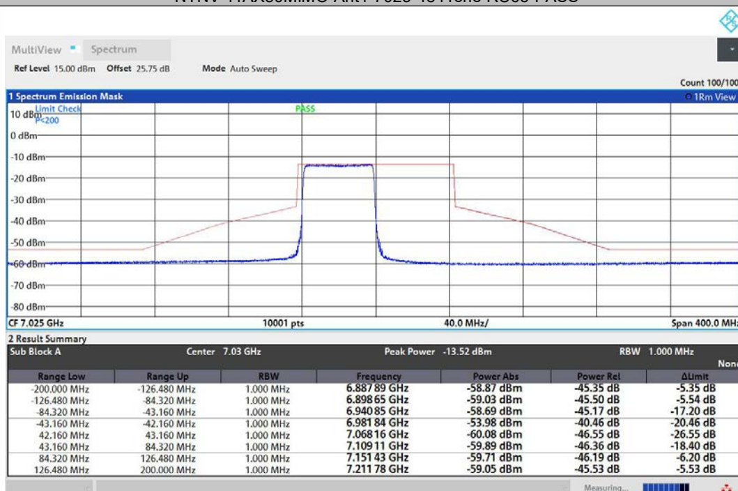
NTNV-11AX80MIMO-Ant2-7025-484Tone-RU65-PASS
