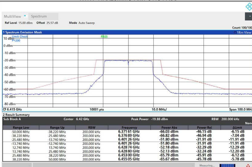
NTNV-11AX20MIMO-Ant2-6415-PASS
