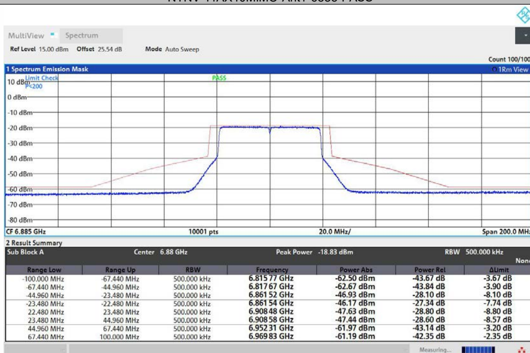
NTNV-11AX40MIMO-Ant2-6885-PASS
