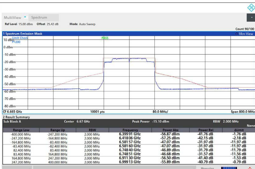
NTNV-11AX160MIMO-Ant1-6665-PASS
