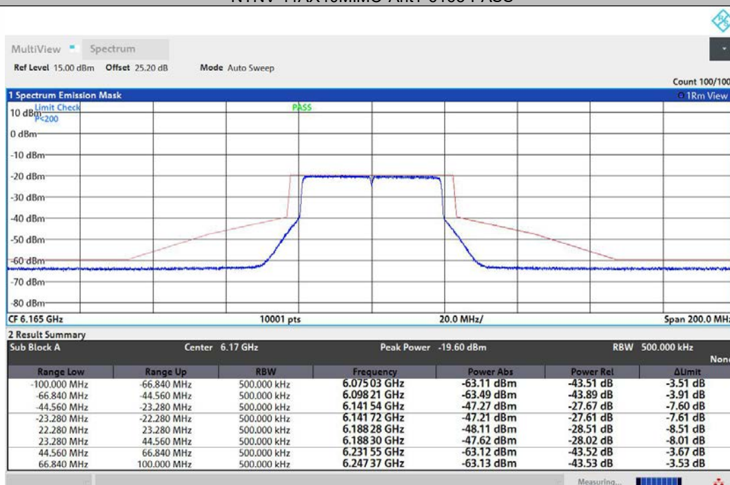
NTNV-11AX40MIMO-Ant2-6165-PASS
