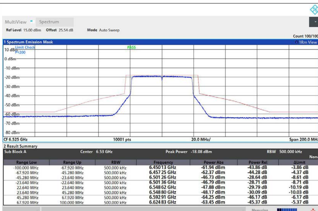
NTNV-11AX40MIMO-Ant1-6525-PASS
