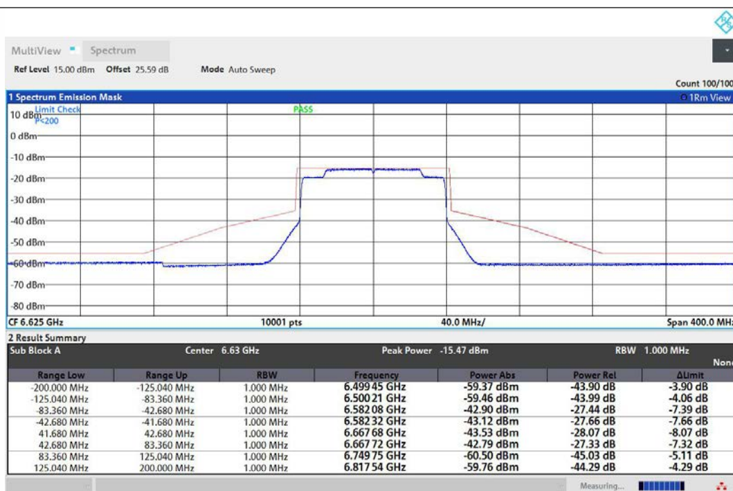
NTNV-11AX80MIMO-Ant1-6625-PASS
