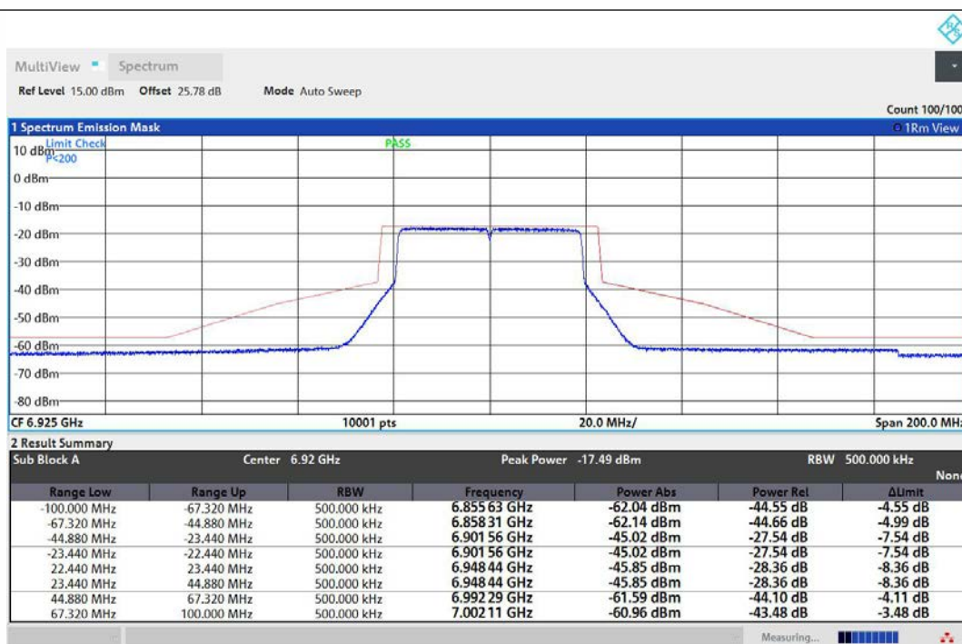
NTNV-11AX40MIMO-Ant1-6925-PASS
