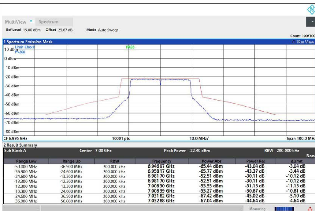
NTNV-11AX20MIMO-Ant1-6995-PASS
