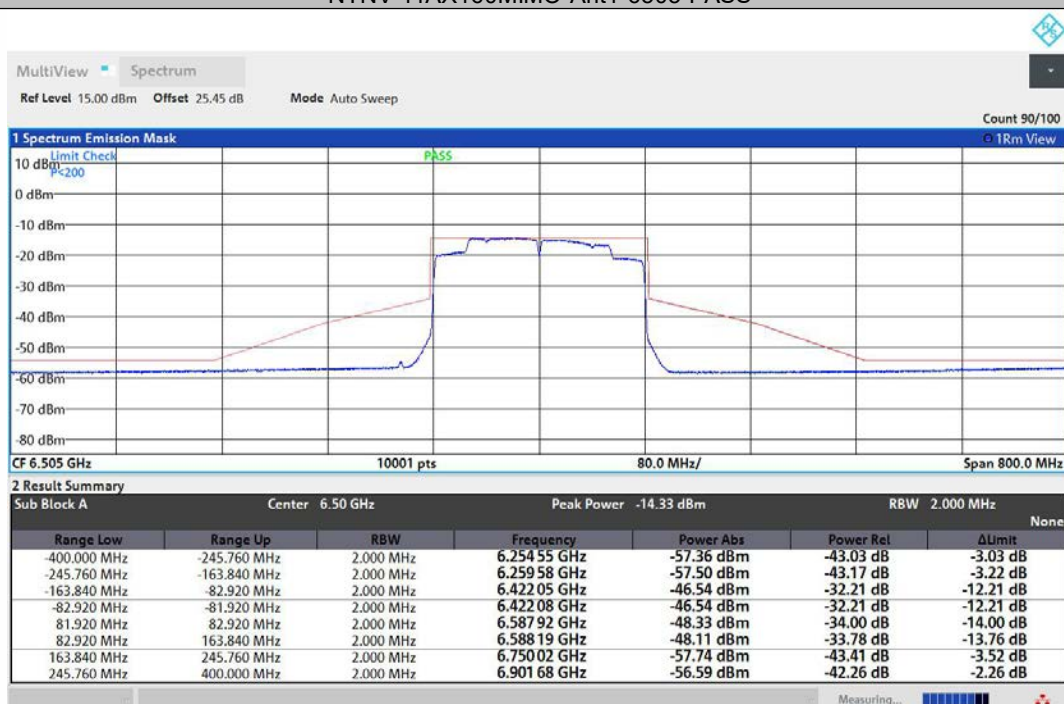
NTNV-11AX160MIMO-Ant2-6505-PASS
