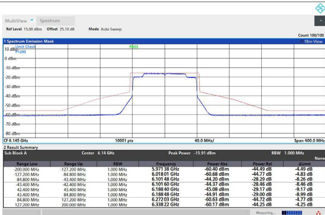
NTNV-11AX80MIMO-Ant1-6145-PASS
