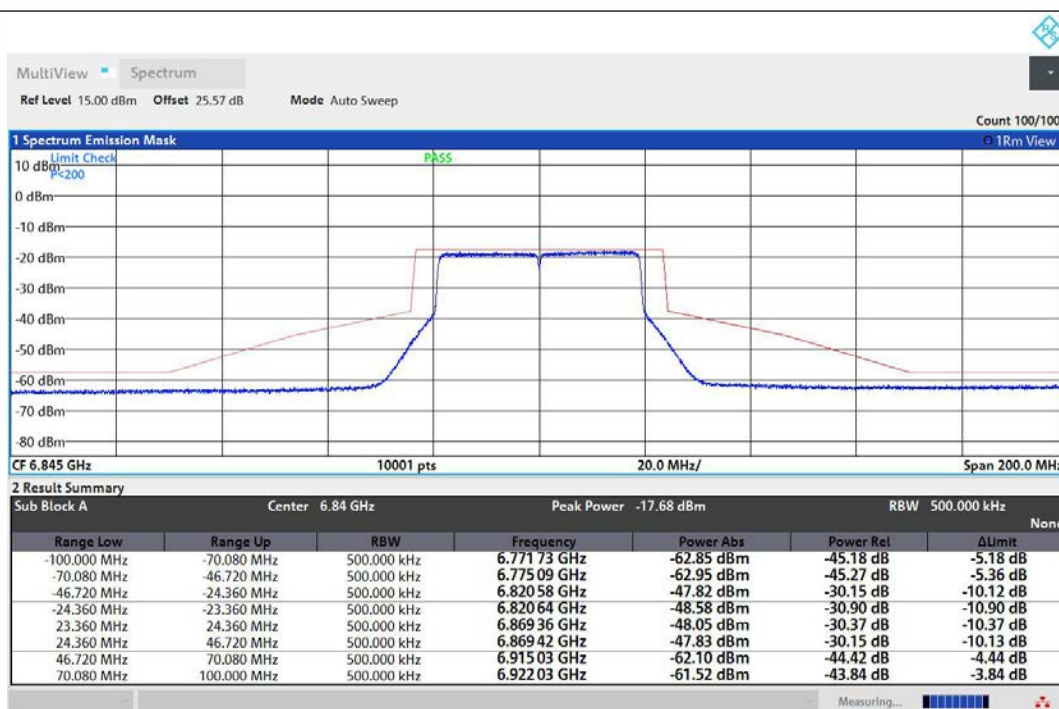
NTNV-11AX40MIMO-Ant1-6845-PASS
