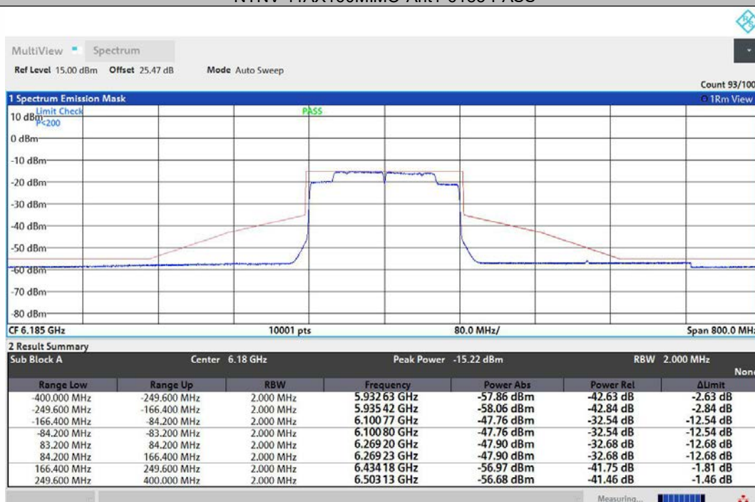
NTNV-11AX160MIMO-Ant2-6185-PASS
