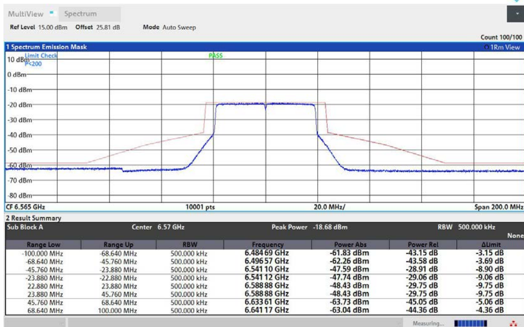
NTNV-11AX40MIMO-Ant1-6565-PASS
