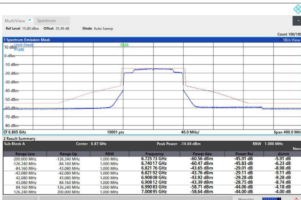
NTNV-11AX80MIMO-Ant1-6865-PASS
