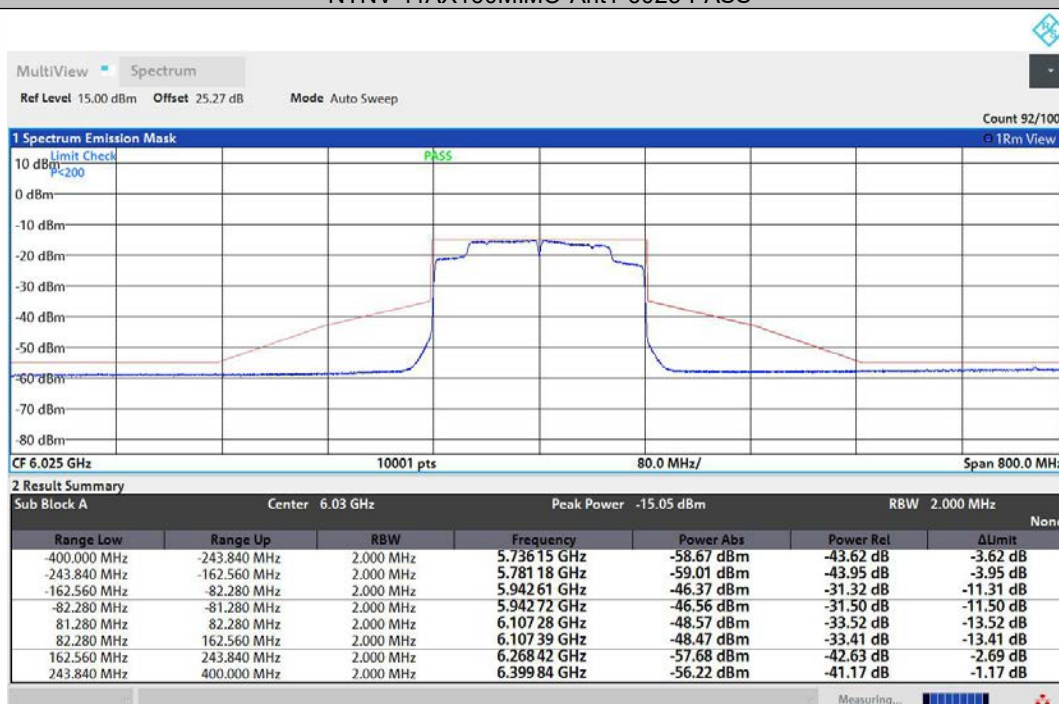
NTNV-11AX160MIMO-Ant2-6025-PASS
