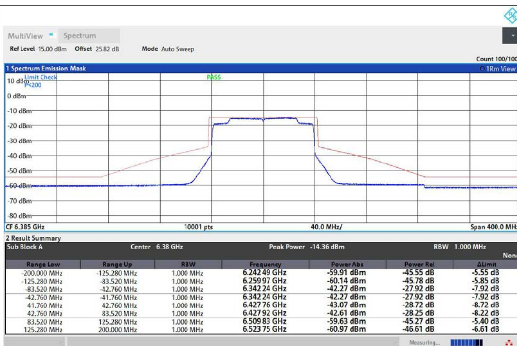
NTNV-11AX80MIMO-Ant1-6385-PASS
