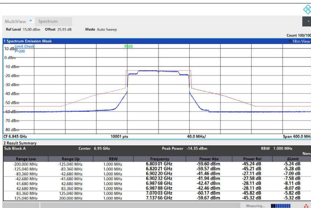
NTNV-11AX80MIMO-Ant1-6945-PASS
