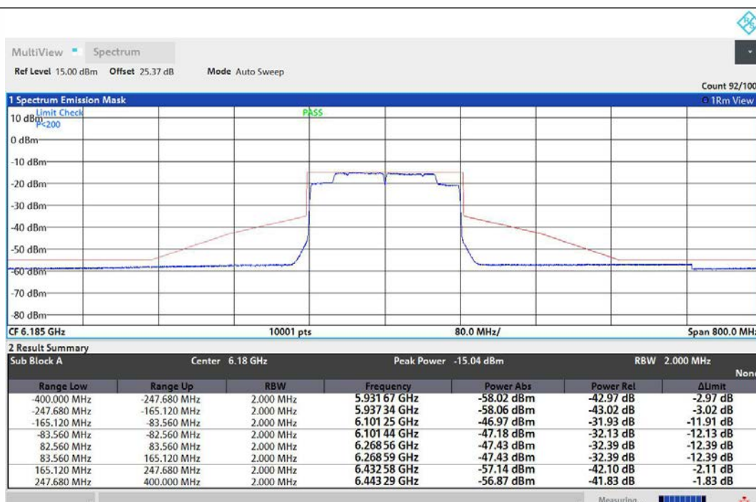
NTNV-11AX160MIMO-Ant1-6185-PASS
