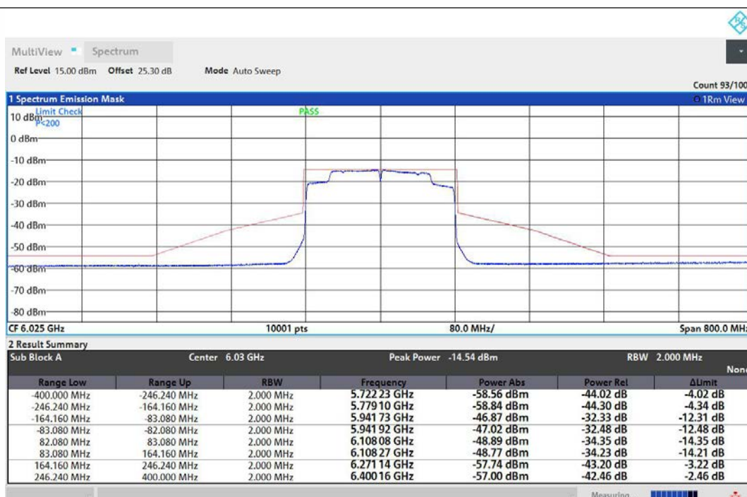
NTNV-11AX160MIMO-Ant1-6025-PASS
