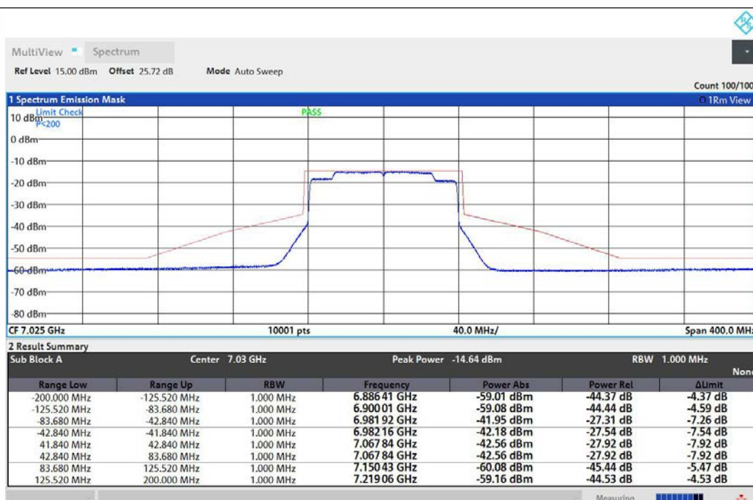
NTNV-11AX80MIMO-Ant1-7025-PASS
