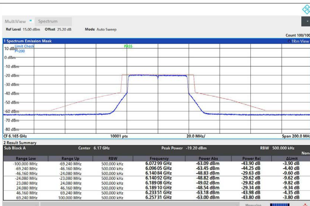
NTNV-11AX40MIMO-Ant1-6165-PASS
