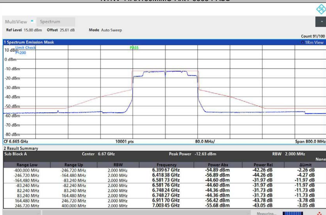
NTNV-11AX160MIMO-Ant2-6665-PASS
