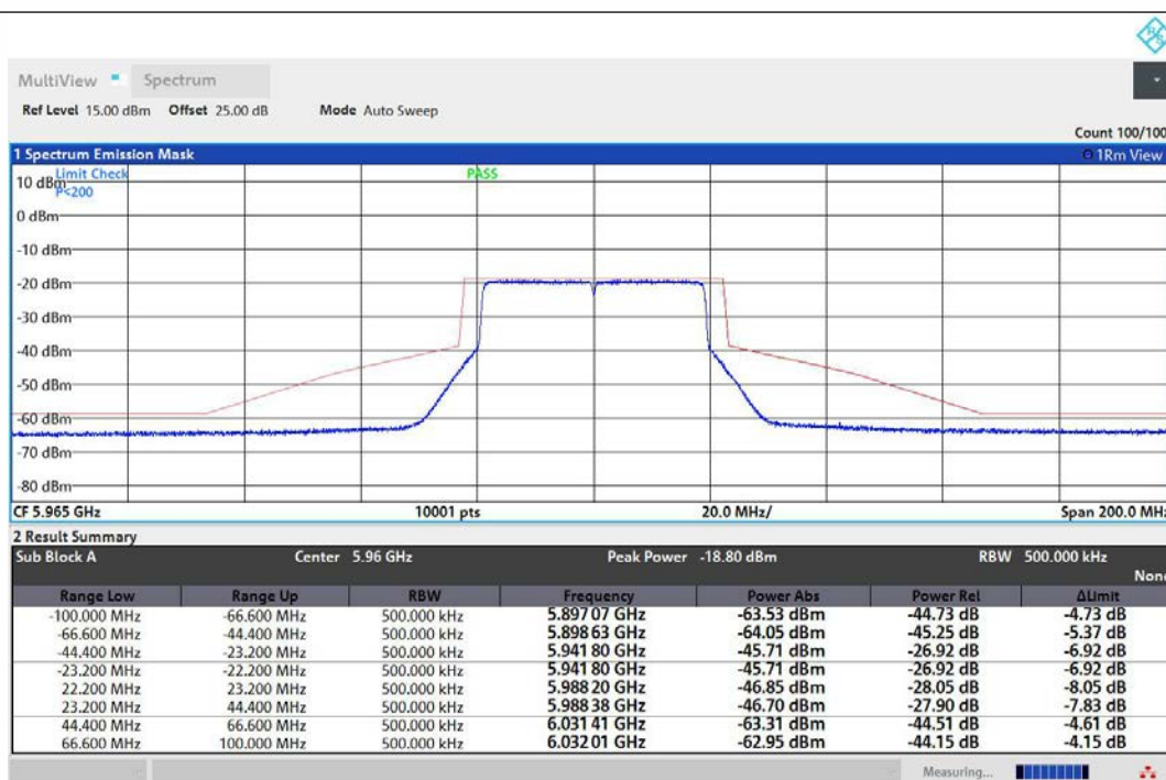
NTNV-11AX40MIMO-Ant1-5965-PASS
