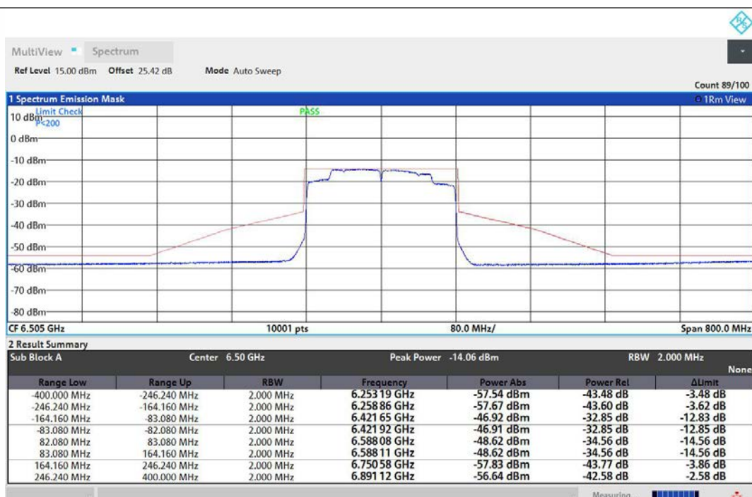
NTNV-11AX160MIMO-Ant1-6505-PASS
