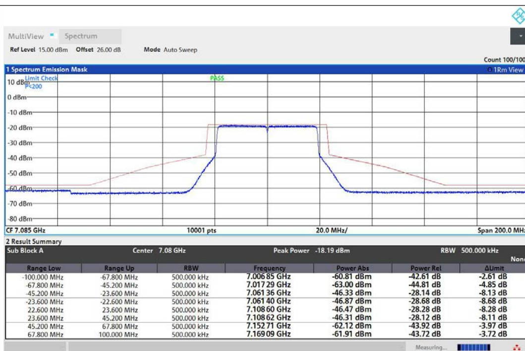
NTNV-11AX40MIMO-Ant1-7085-PASS
