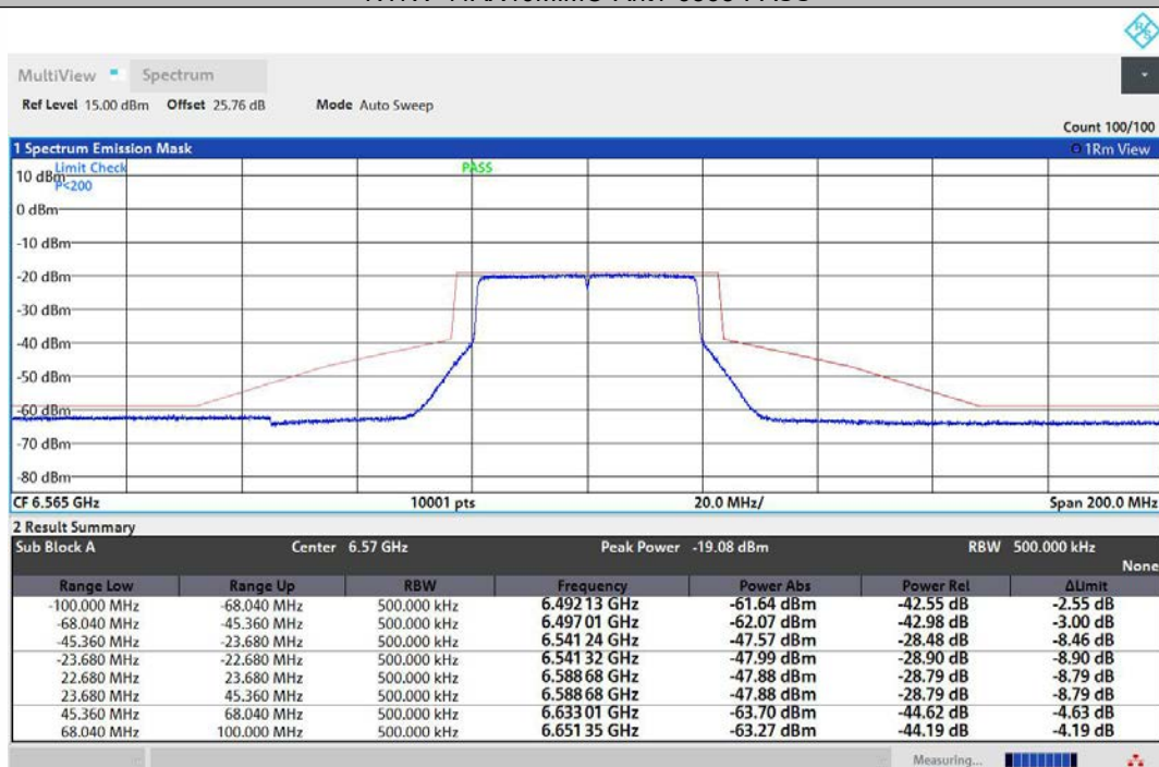
NTNV-11AX40MIMO-Ant2-6565-PASS
