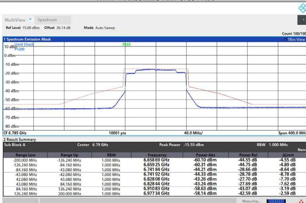
NTNV-11AX80MIMO-Ant2-6785-PASS
