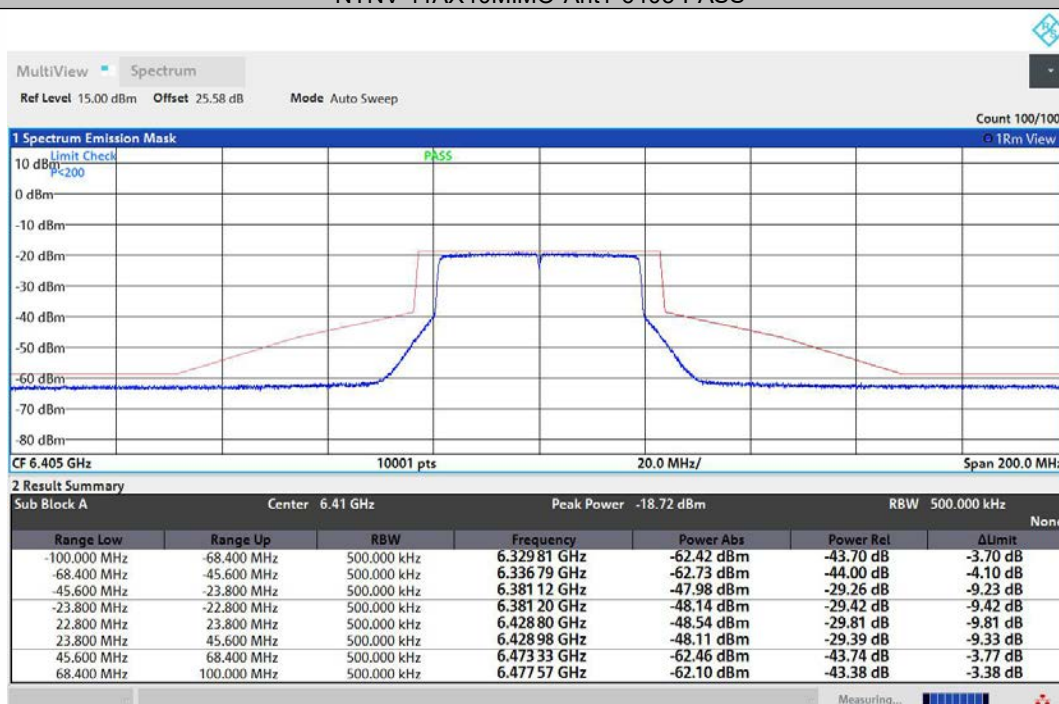
NTNV-11AX40MIMO-Ant2-6405-PASS
