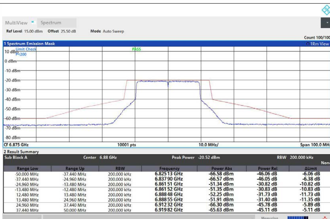
NTNV-11AX20MIMO-Ant1-6875-PASS
