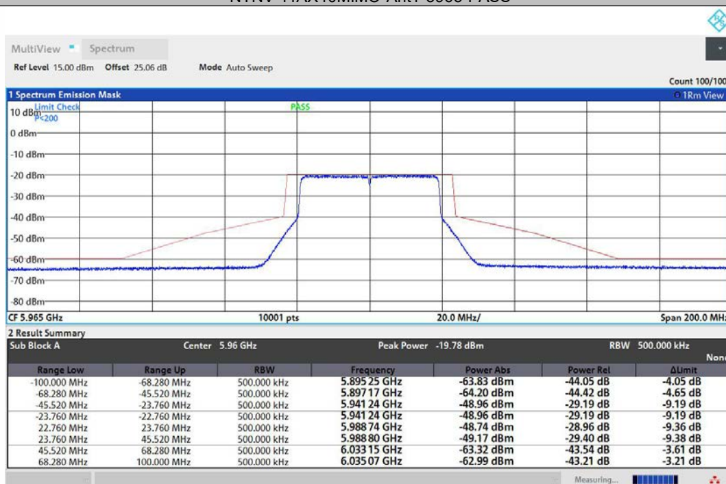
NTNV-11AX40MIMO-Ant2-5965-PASS
