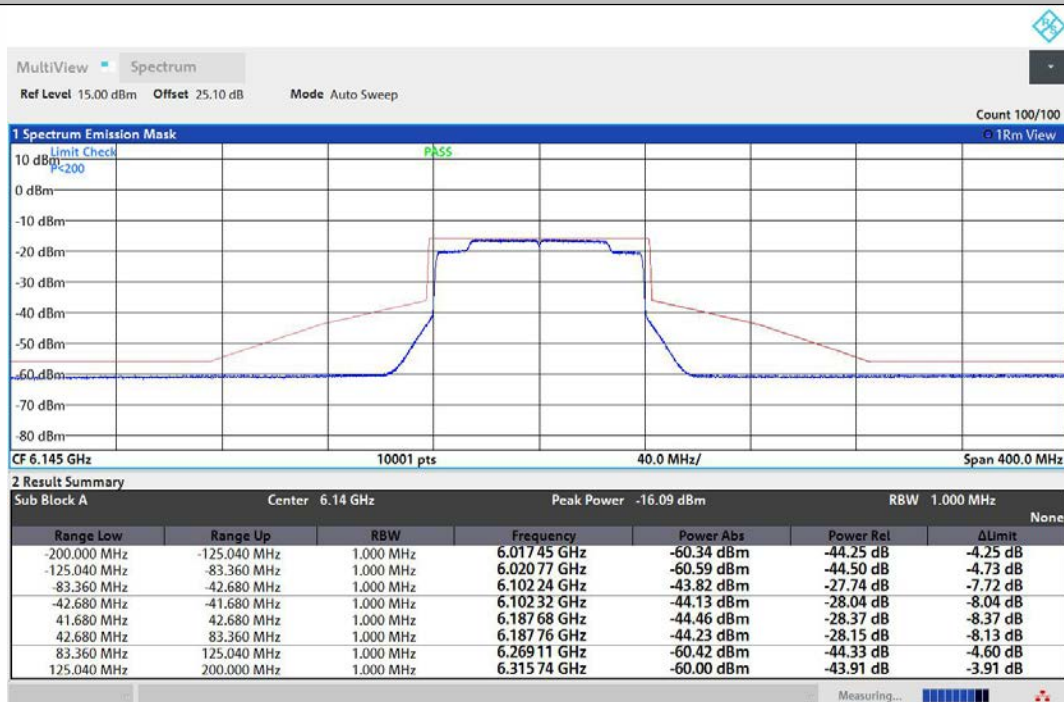
NTNV-11AX80MIMO-Ant2-6145-PASS
