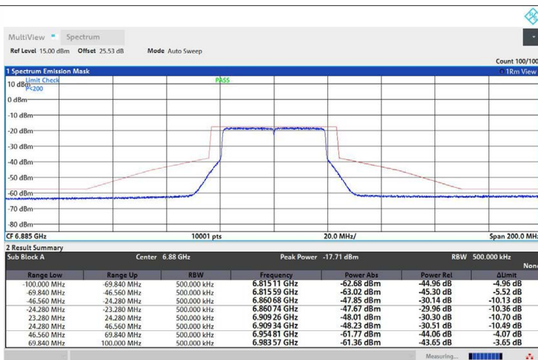
NTNV-11AX40MIMO-Ant1-6885-PASS
