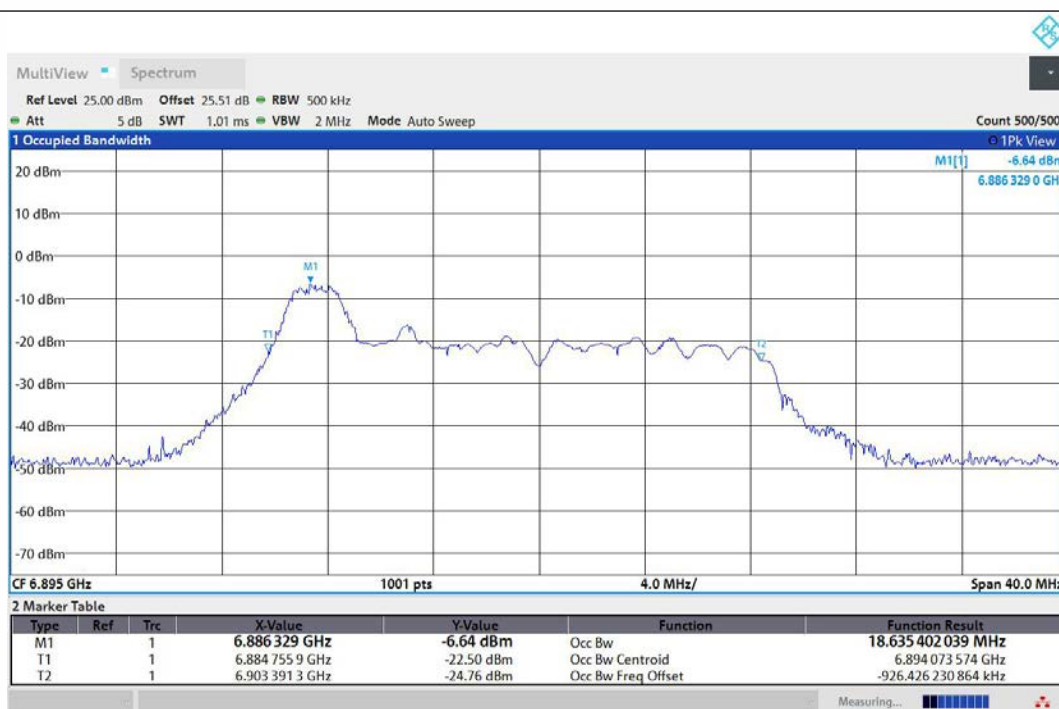
11AX20MIMO-Ant1-6895-26Tone-RU0-PASS
