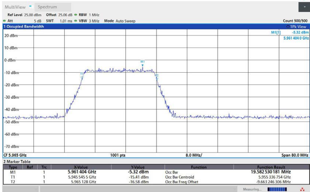
11AX40MIMO-Ant2-5965-242Tone-RU61-PASS
