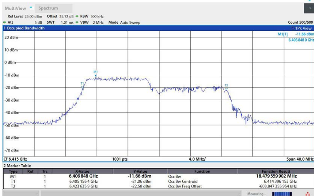
11AX20MIMO-Ant1-6415-106Tone-RU53-PASS
