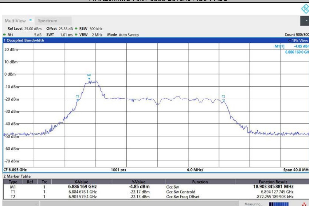
11AX20MIMO-Ant2-6895-26Tone-RU0-PASS
