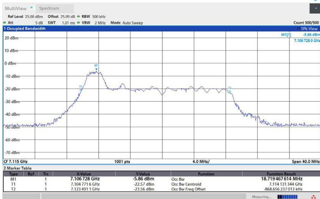
11AX20MIMO-Ant1-7115-26Tone-RU0-PASS
