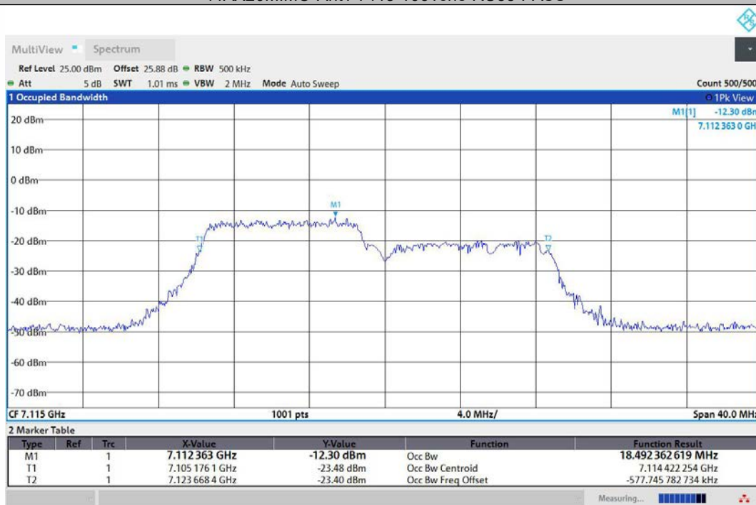
11AX20MIMO-Ant2-7115-106Tone-RU53-PASS
