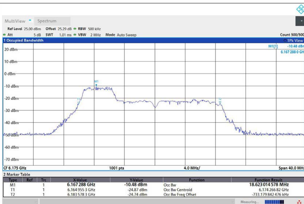
11AX20MIMO-Ant1-6175-52Tone-RU37-PASS
