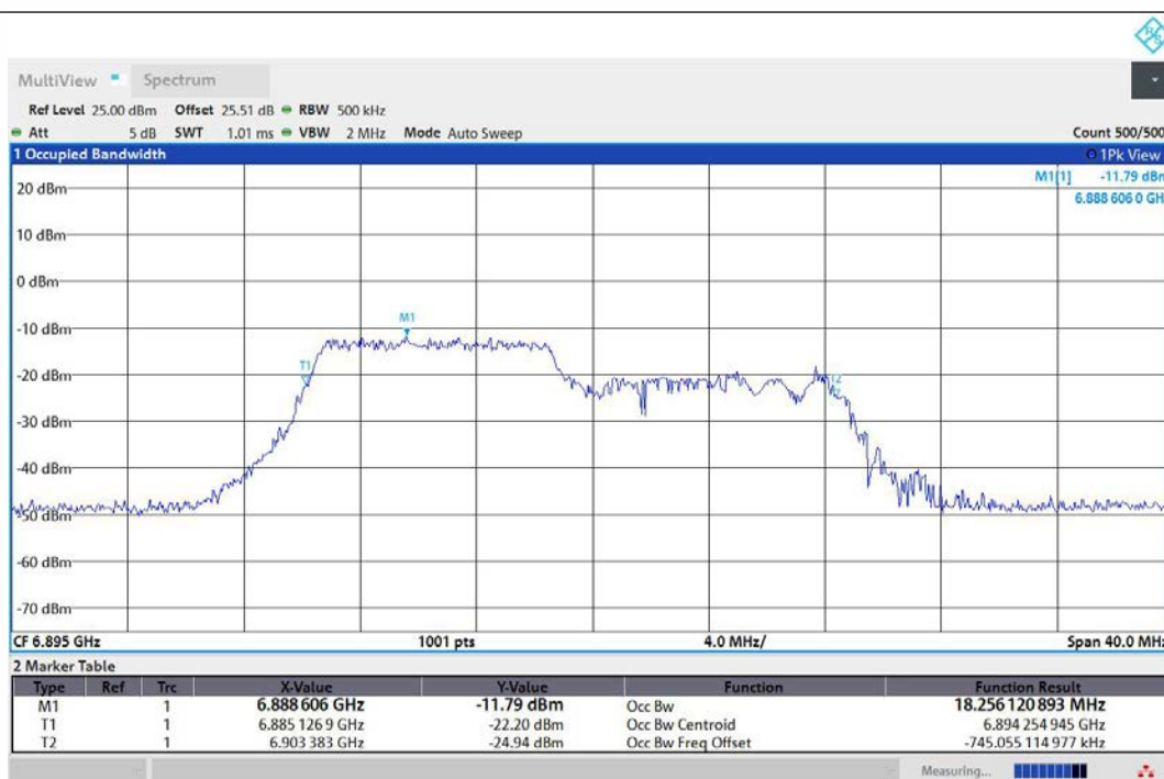
11AX20MIMO-Ant1-6895-106Tone-RU53-PASS
