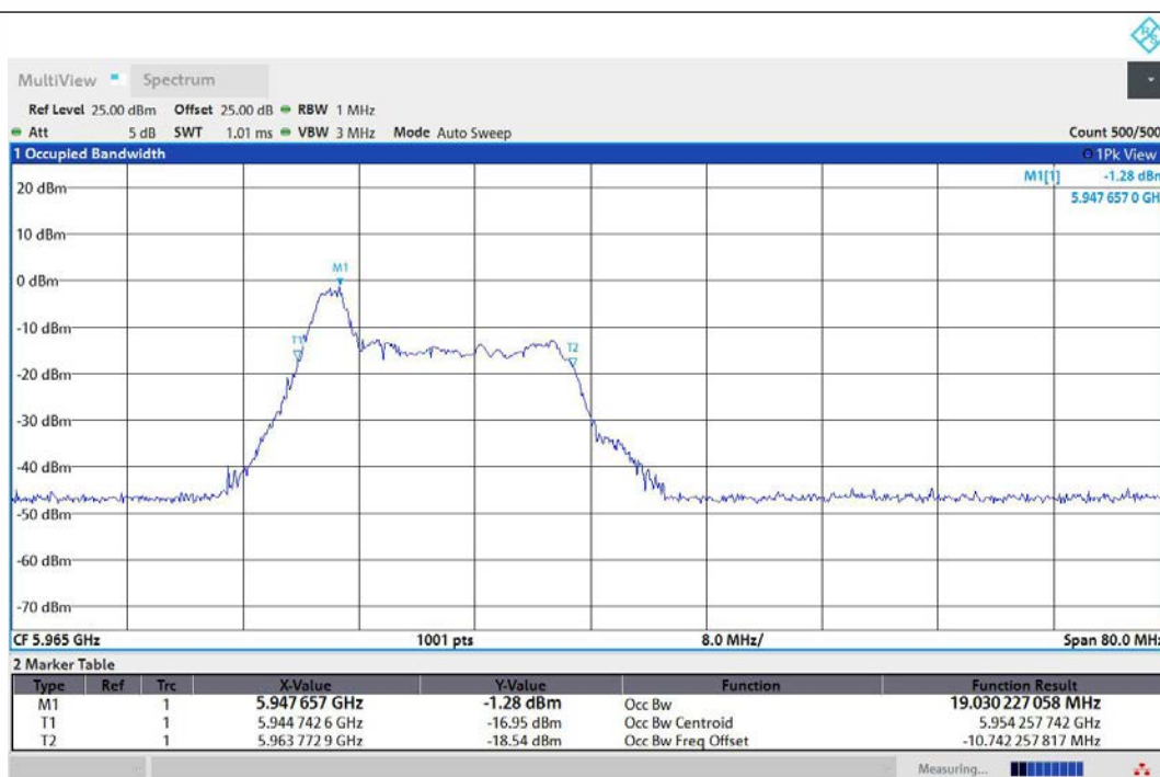
11AX40MIMO-Ant1-5965-26Tone-RU0-PASS
