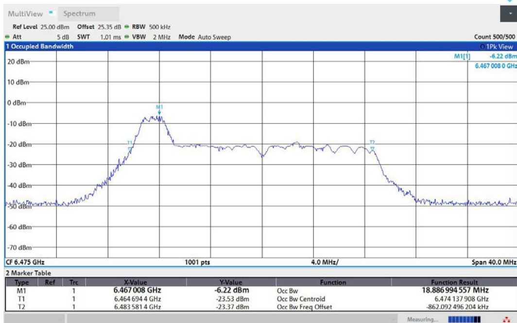
11AX20MIMO-Ant1-6475-26Tone-RU0-PASS
