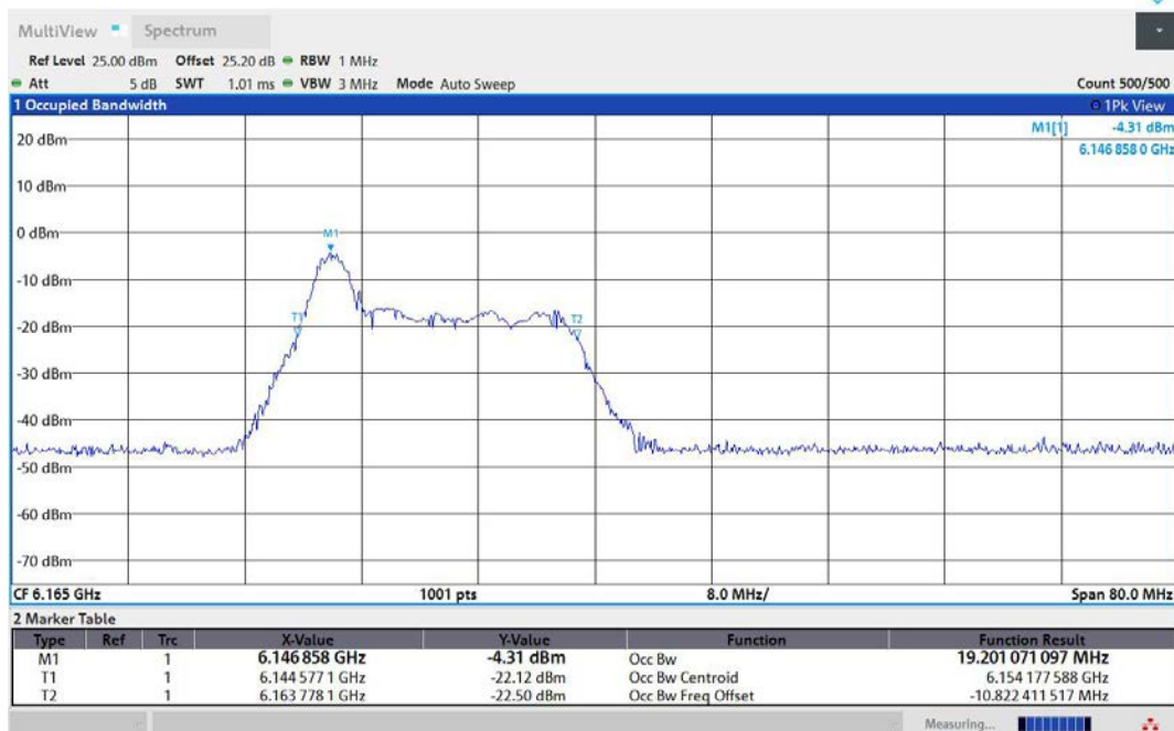
11AX40MIMO-Ant2-6165-26Tone-RU0-PASS
