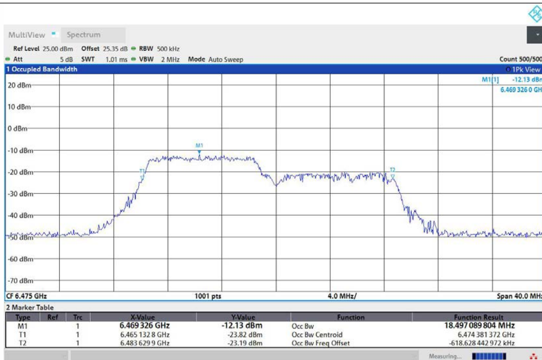
11AX20MIMO-Ant1-6475-106Tone-RU53-PASS
