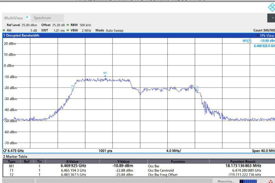
11AX20MIMO-Ant2-6475-106Tone-RU53-PASS
