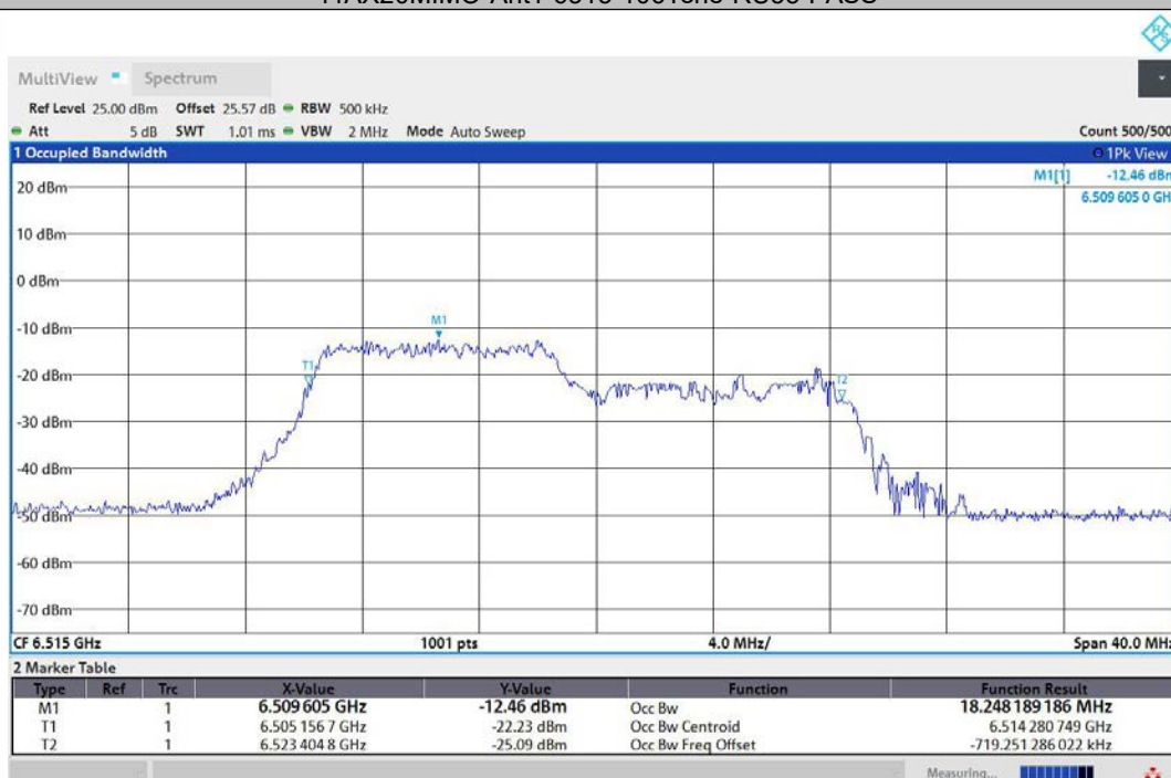
11AX20MIMO-Ant2-6515-106Tone-RU53-PASS
