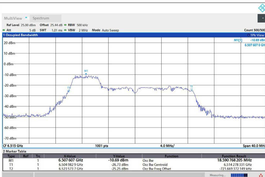
11AX20MIMO-Ant1-6515-52Tone-RU37-PASS
