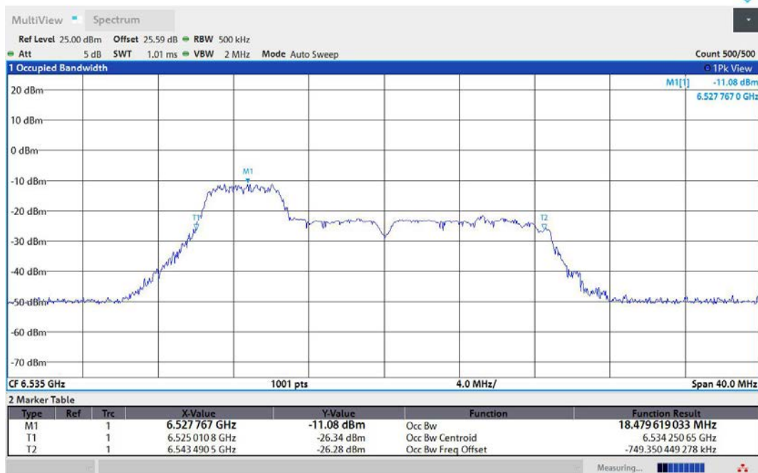
11AX20MIMO-Ant1-6535-52Tone-RU37-PASS
