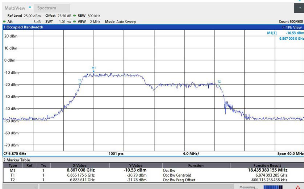
11AX20MIMO-Ant2-6875-106Tone-RU53-PASS
