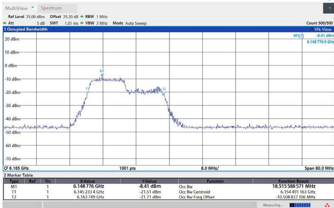
11AX40MIMO-Ant2-6165-106Tone-RU53-PASS
