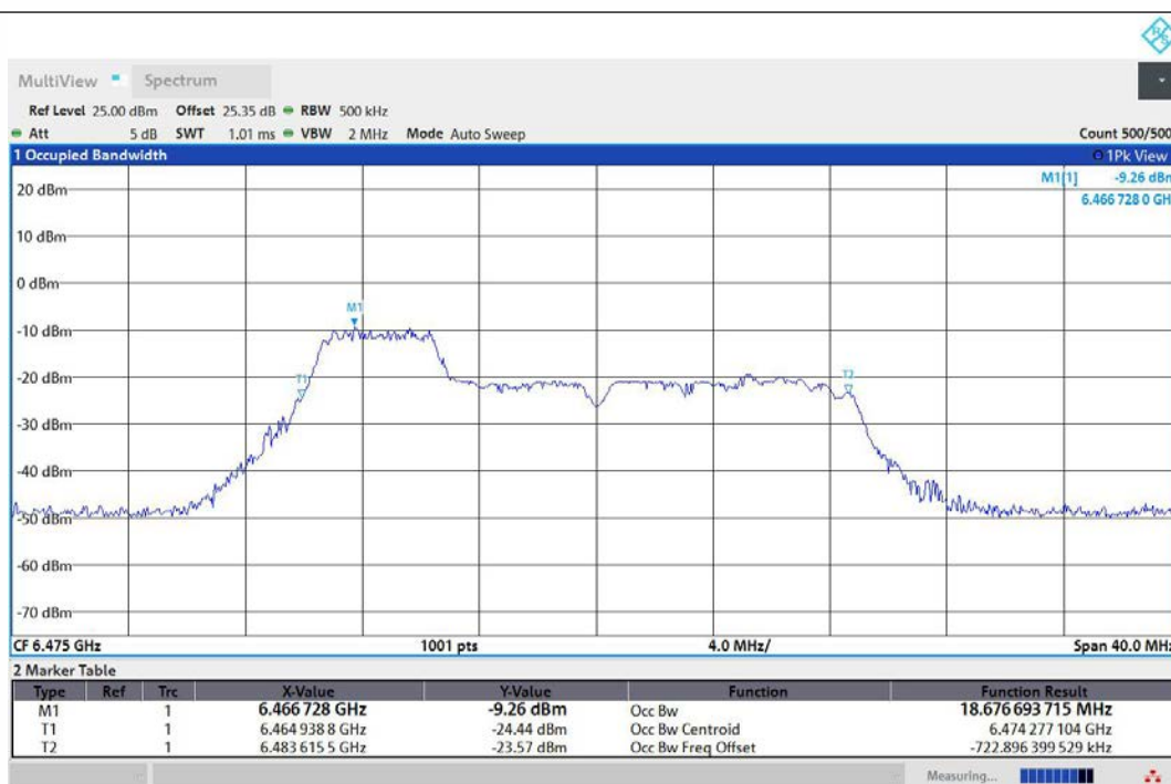
11AX20MIMO-Ant1-6475-52Tone-RU37-PASS
