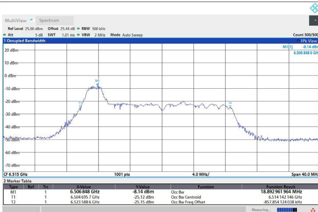
11AX20MIMO-Ant1-6515-26Tone-RU0-PASS
