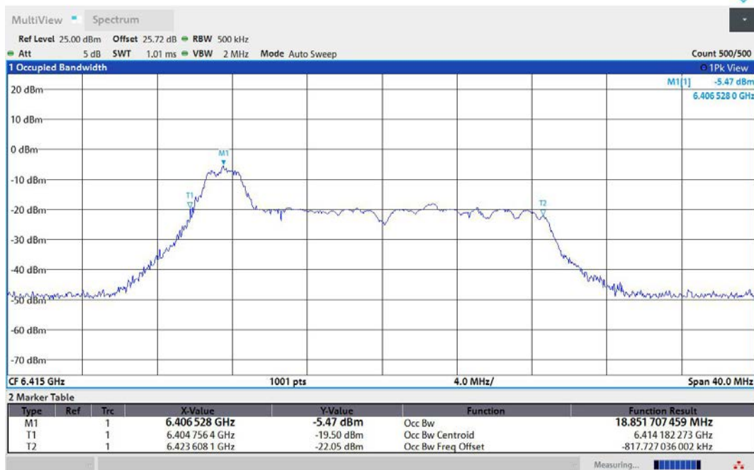
11AX20MIMO-Ant1-6415-26Tone-RU0-PASS
