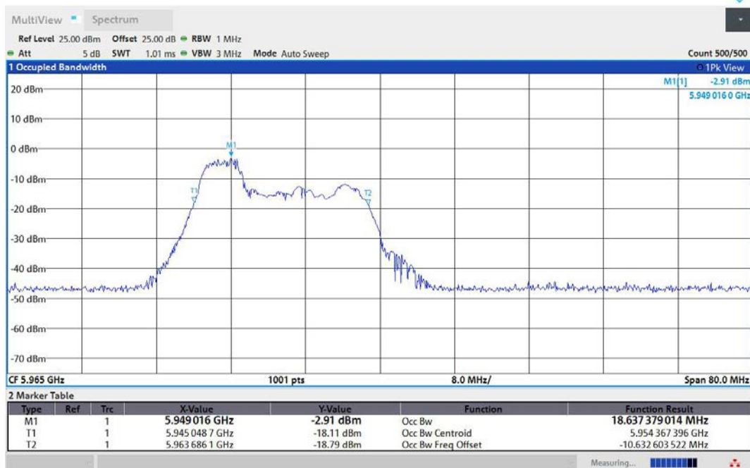
11AX40MIMO-Ant1-5965-52Tone-RU37-PASS
