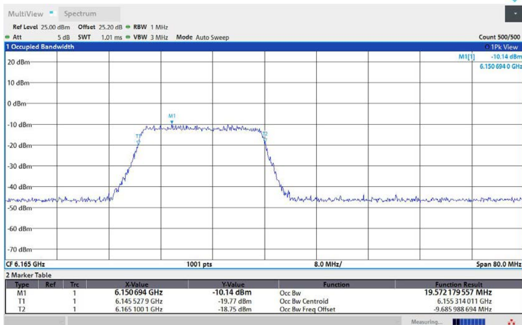
11AX40MIMO-Ant2-6165-242Tone-RU61-PASS
