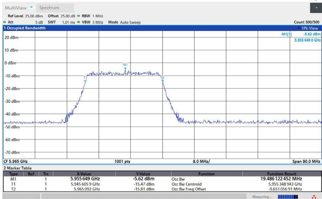
11AX40MIMO-Ant1-5965-242Tone-RU61-PASS
