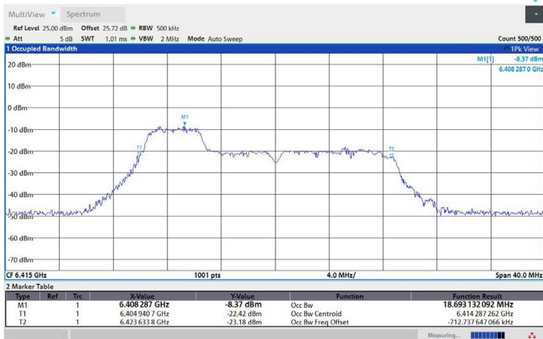
11AX20MIMO-Ant1-6415-52Tone-RU37-PASS
