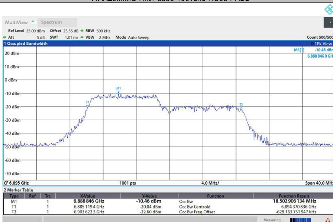
11AX20MIMO-Ant2-6895-106Tone-RU53-PASS
