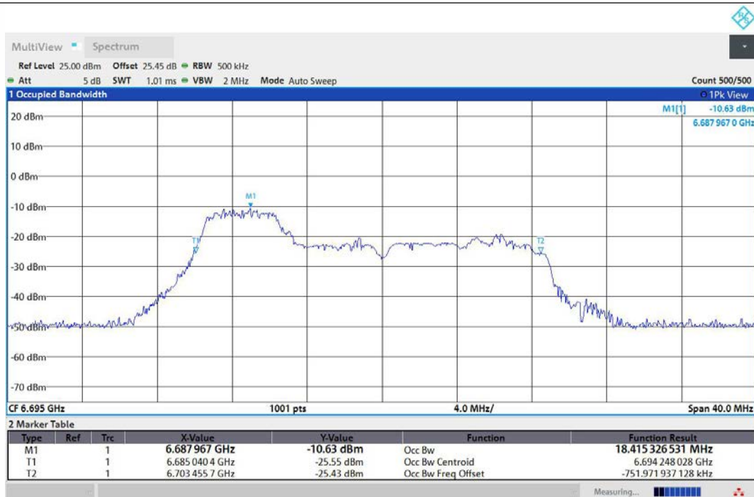
11AX20MIMO-Ant1-6695-52Tone-RU37-PASS
