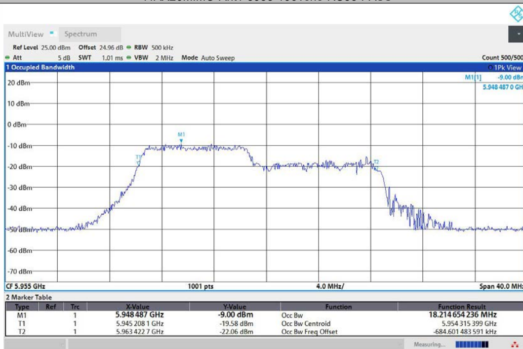
11AX20MIMO-Ant2-5955-106Tone-RU53-PASS
