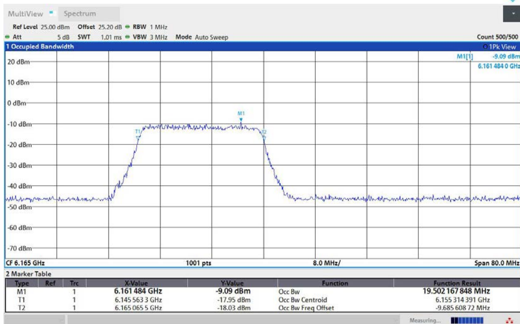
11AX40MIMO-Ant1-6165-242Tone-RU61-PASS
