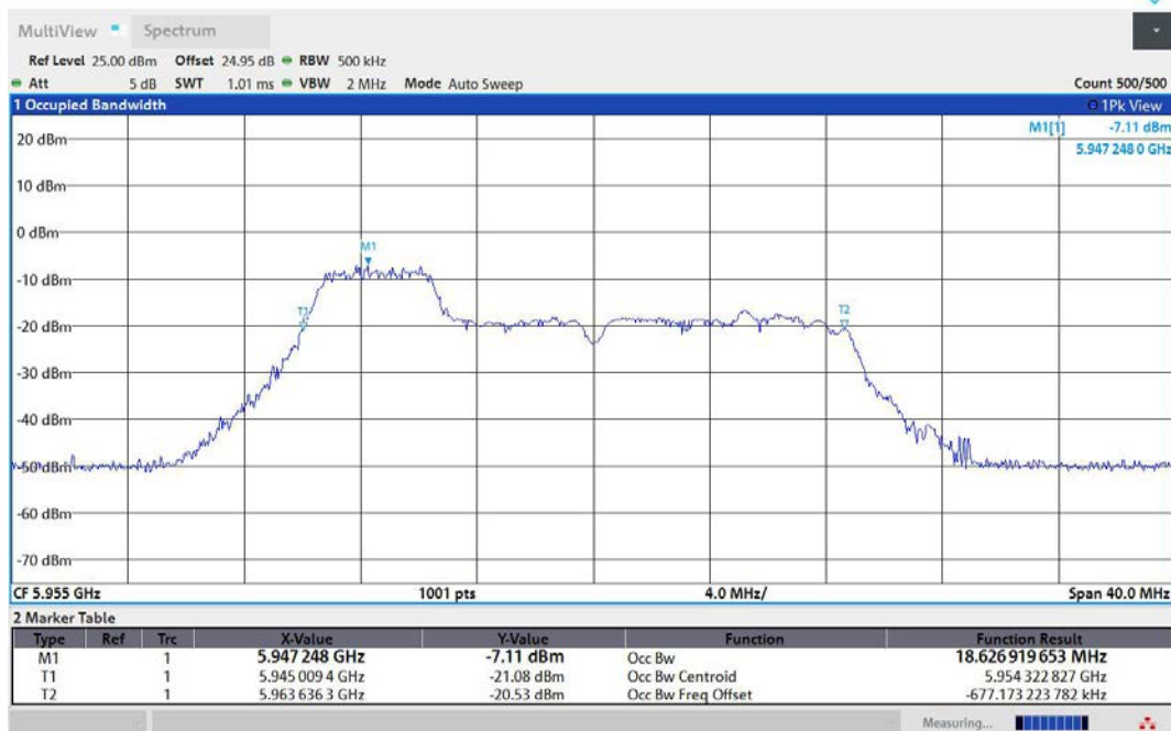
11AX20MIMO-Ant1-5955-52Tone-RU37-PASS
