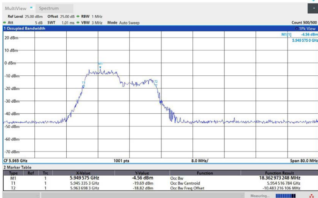
11AX40MIMO-Ant1-5965-106Tone-RU53-PASS
