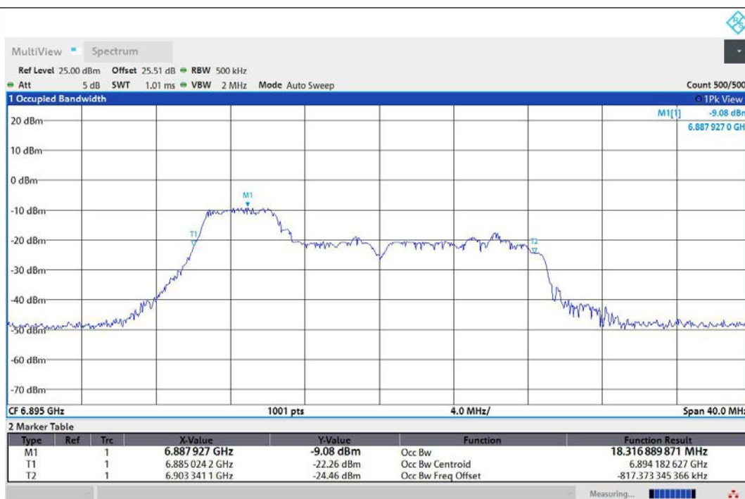
11AX20MIMO-Ant1-6895-52Tone-RU37-PASS
