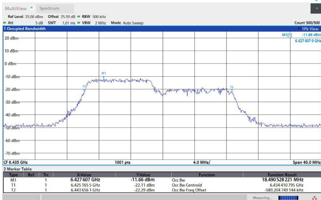
11AX20MIMO-Ant1-6435-106Tone-RU53-PASS
