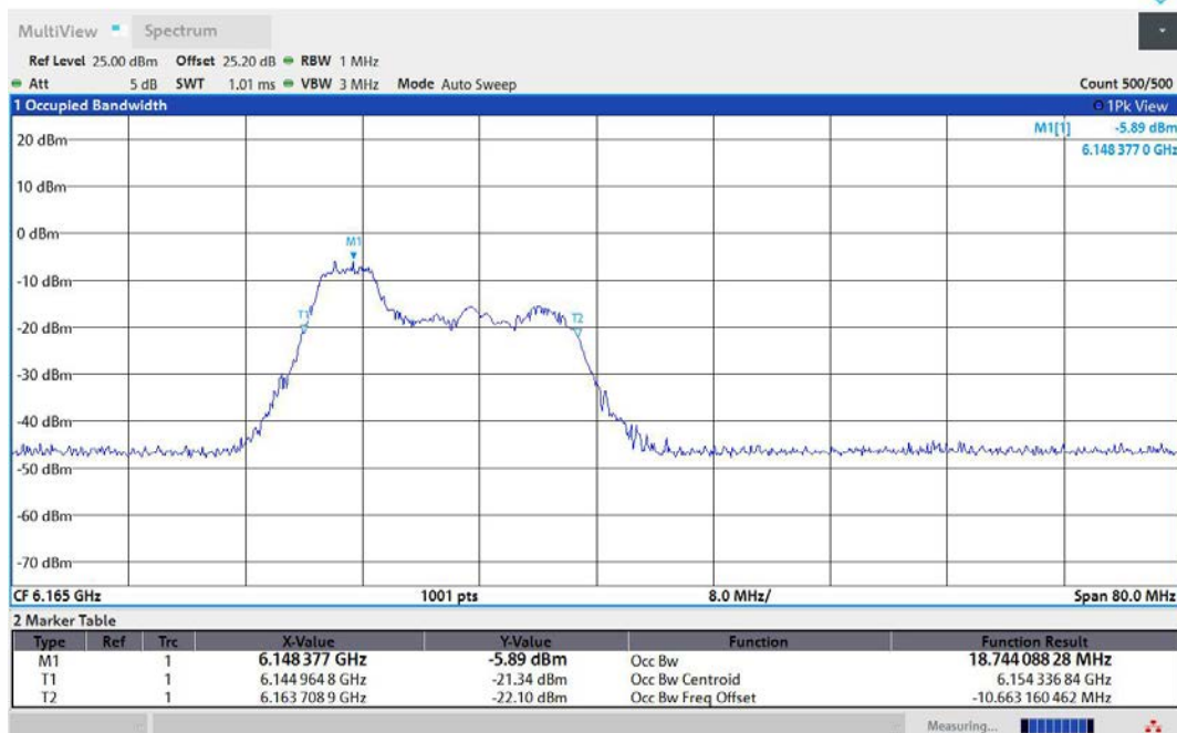
11AX40MIMO-Ant2-6165-52Tone-RU37-PASS
