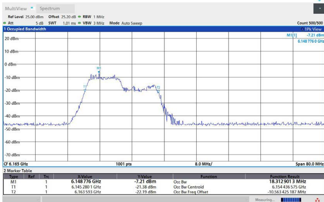
11AX40MIMO-Ant1-6165-106Tone-RU53-PASS
