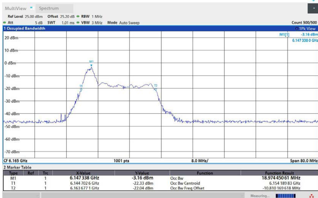
11AX40MIMO-Ant1-6165-26Tone-RU0-PASS
