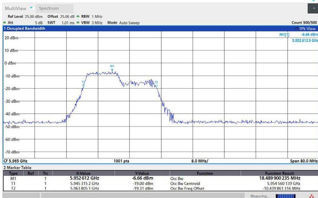
11AX40MIMO-Ant2-5965-106Tone-RU53-PASS
