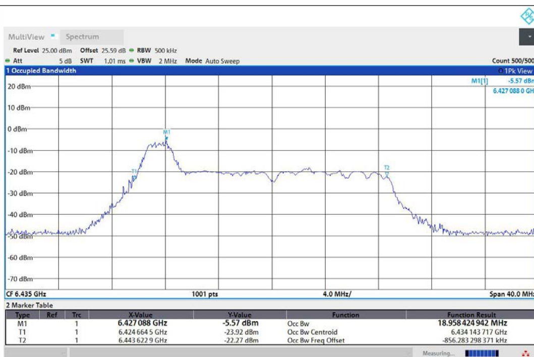
11AX20MIMO-Ant1-6435-26Tone-RU0-PASS
