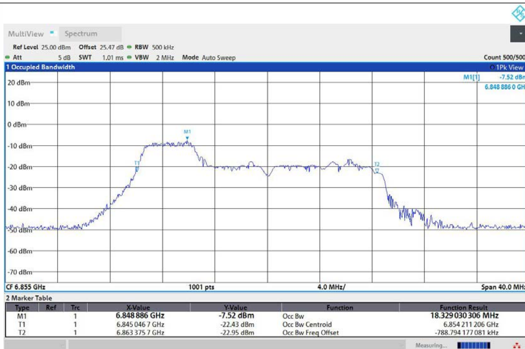
11AX20MIMO-Ant1-6855-52Tone-RU37-PASS
