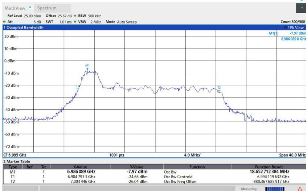
11AX20MIMO-Ant1-6995-26Tone-RU0-PASS
