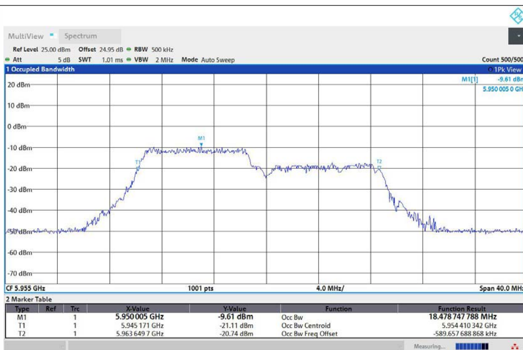
11AX20MIMO-Ant1-5955-106Tone-RU53-PASS
