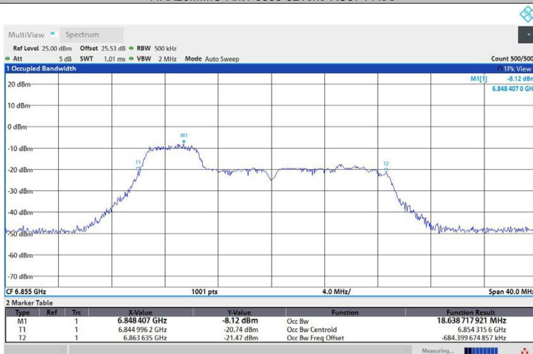
11AX20MIMO-Ant2-6855-52Tone-RU37-PASS
