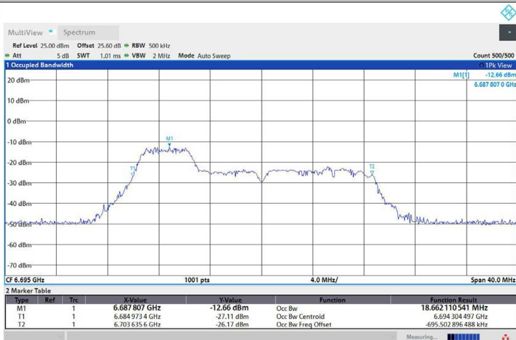
11AX20MIMO-Ant2-6695-52Tone-RU37-PASS
