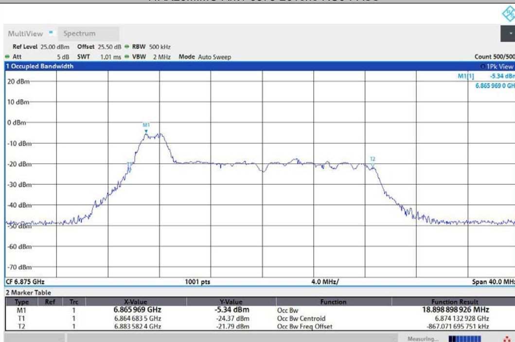
11AX20MIMO-Ant2-6875-26Tone-RU0-PASS
