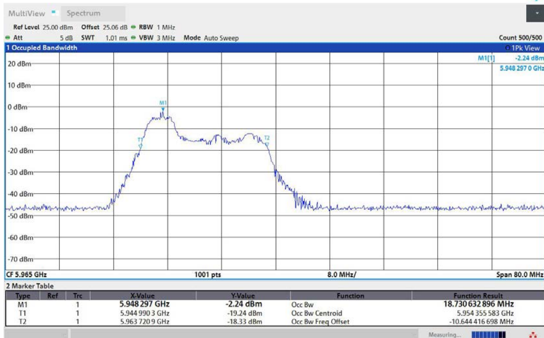
11AX40MIMO-Ant2-5965-52Tone-RU37-PASS
