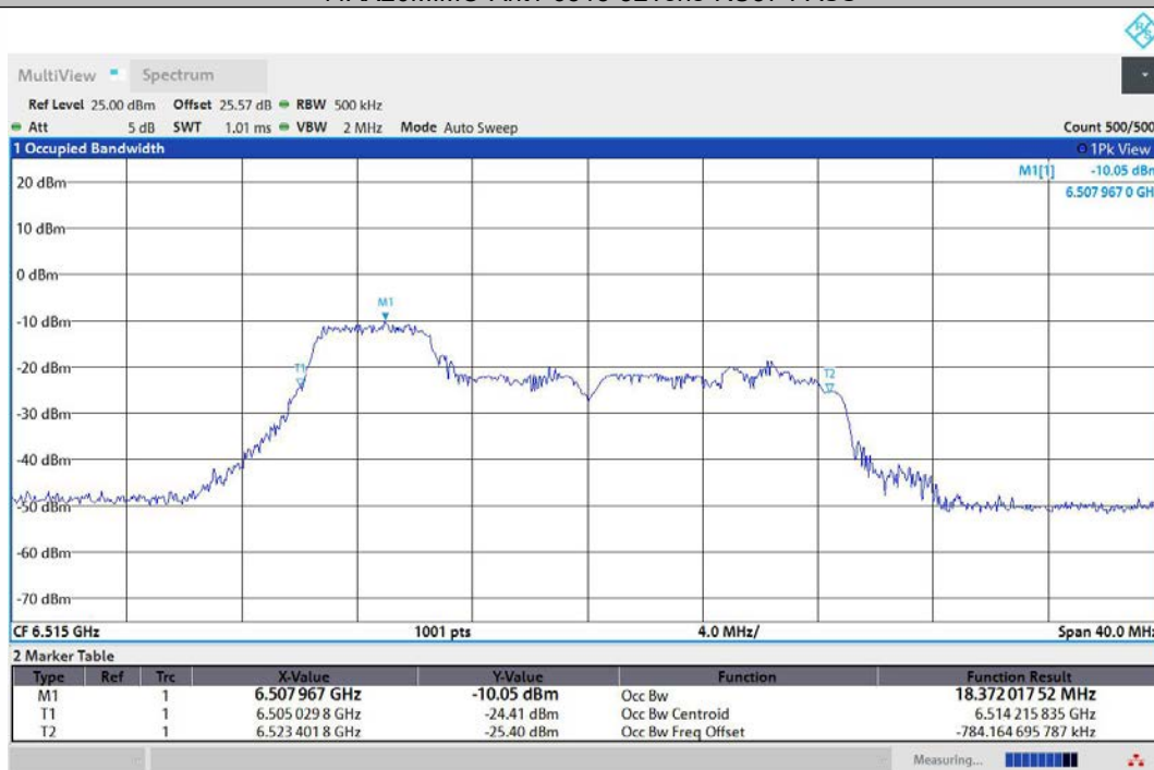
11AX20MIMO-Ant2-6515-52Tone-RU37-PASS
