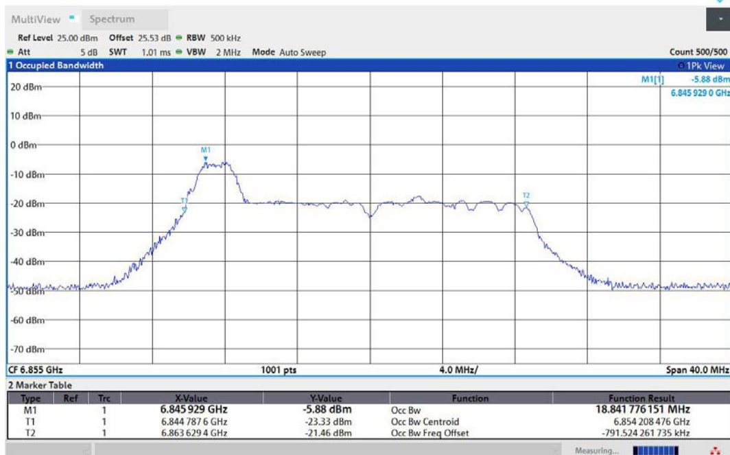
11AX20MIMO-Ant2-6855-26Tone-RU0-PASS
