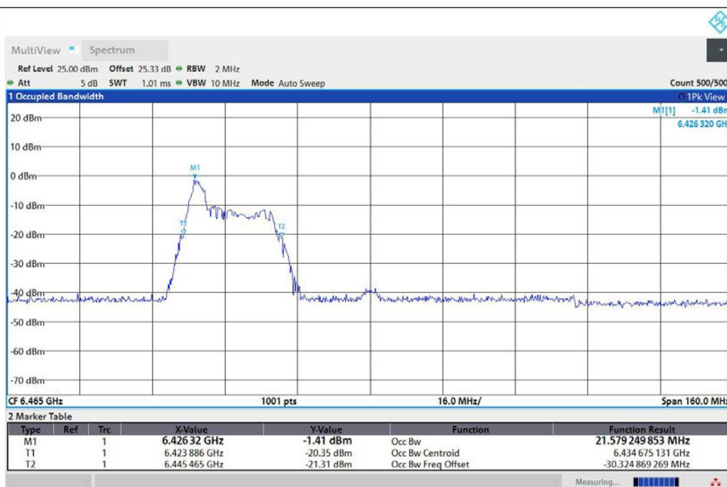
11AX80MIMO-Ant1-6465-26Tone-RU0-PASS
