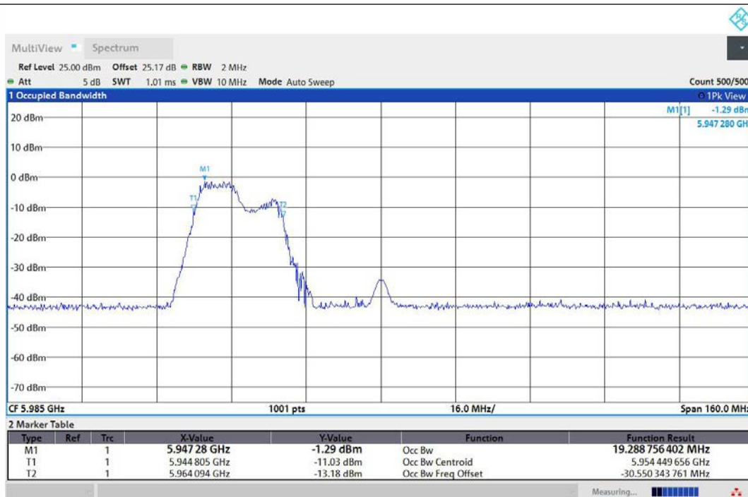
11AX80MIMO-Ant1-5985-106Tone-RU53-PASS
