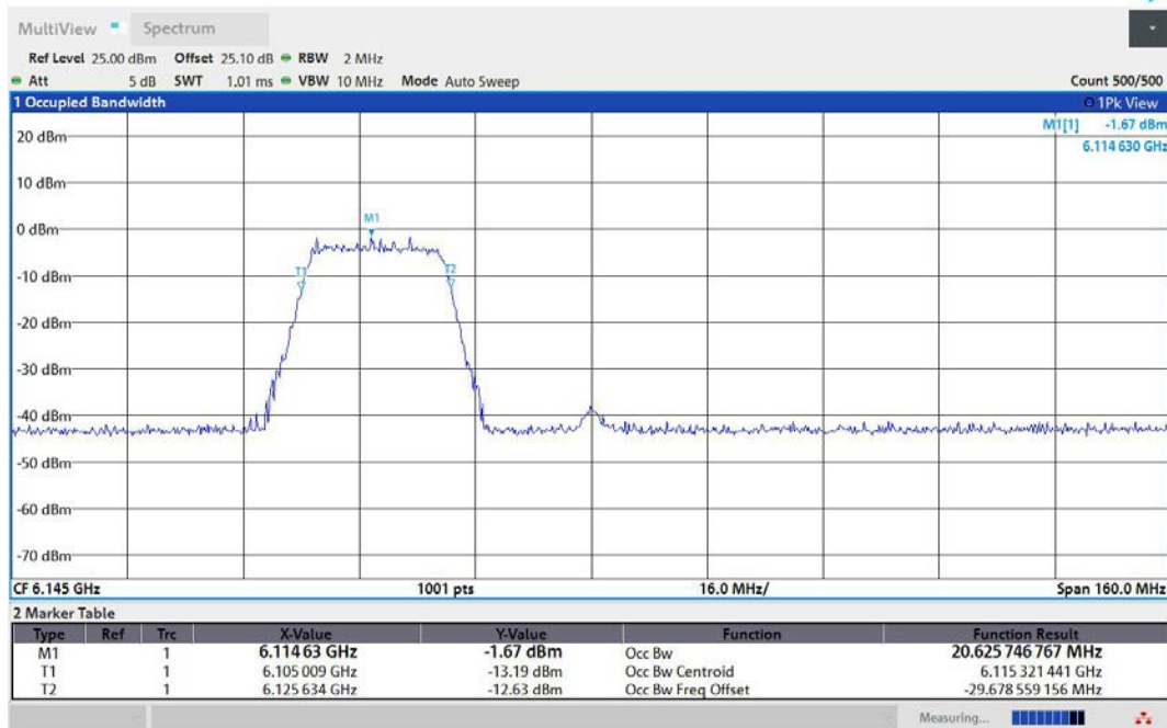
11AX80MIMO-Ant2-6145-242Tone-RU61-PASS
