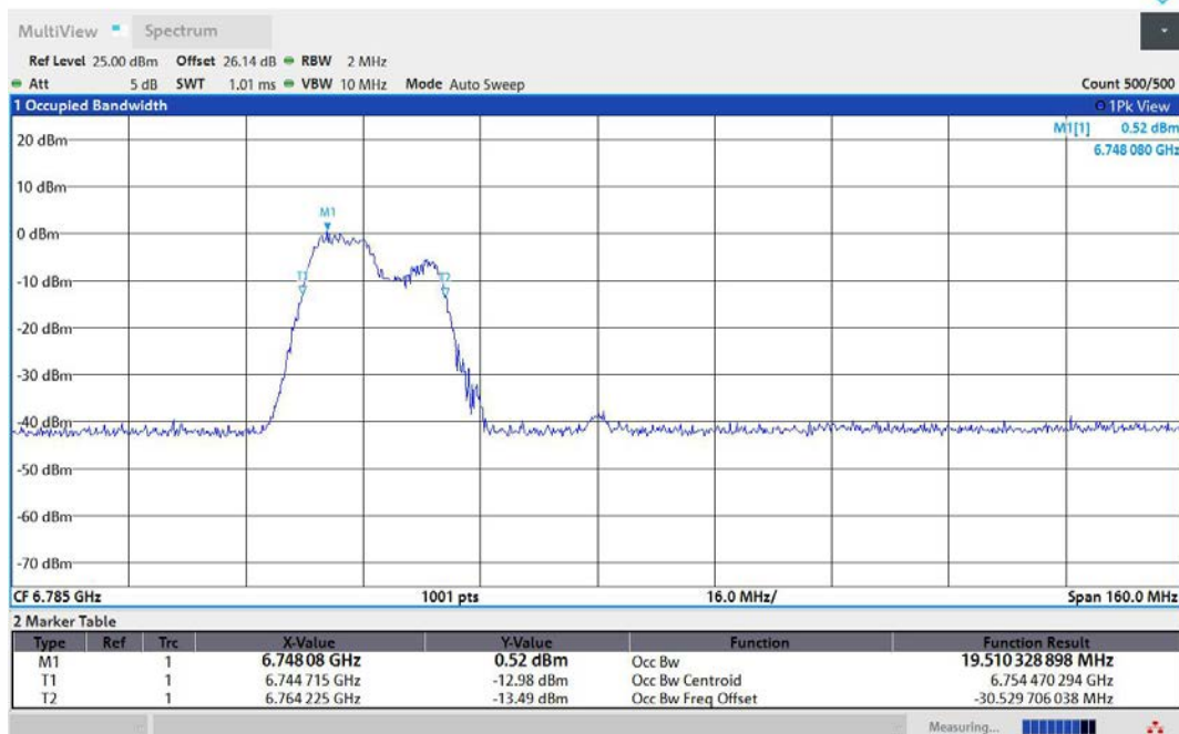
11AX80MIMO-Ant2-6785-106Tone-RU53-PASS
