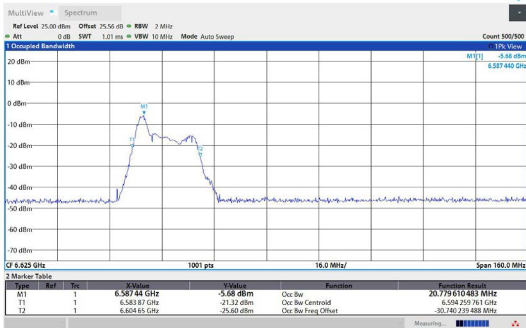
11AX80MIMO-Ant2-6625-26Tone-RU0-PASS
