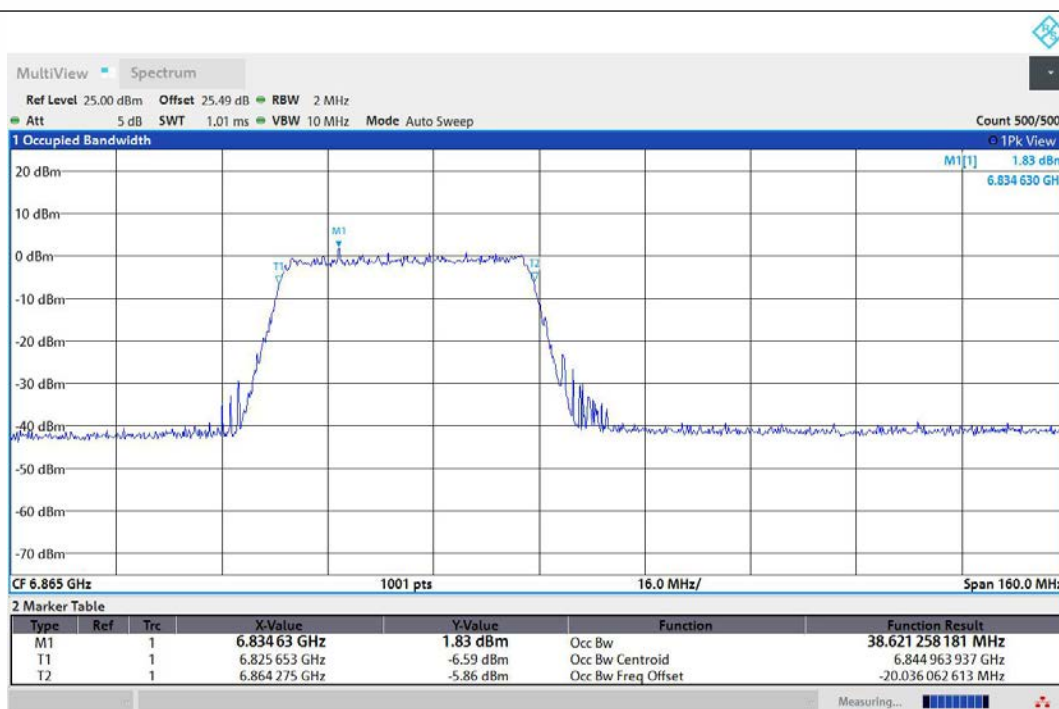
11AX80MIMO-Ant1-6865-484Tone-RU65-PASS
