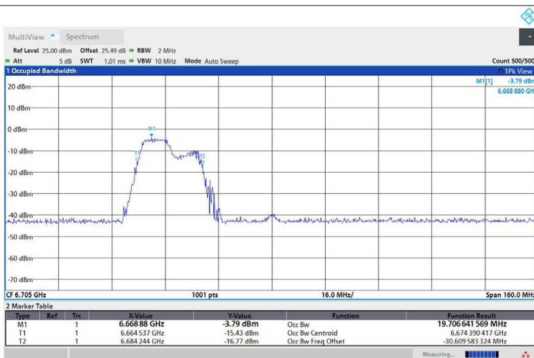
11AX80MIMO-Ant1-6705-106Tone-RU53-PASS
