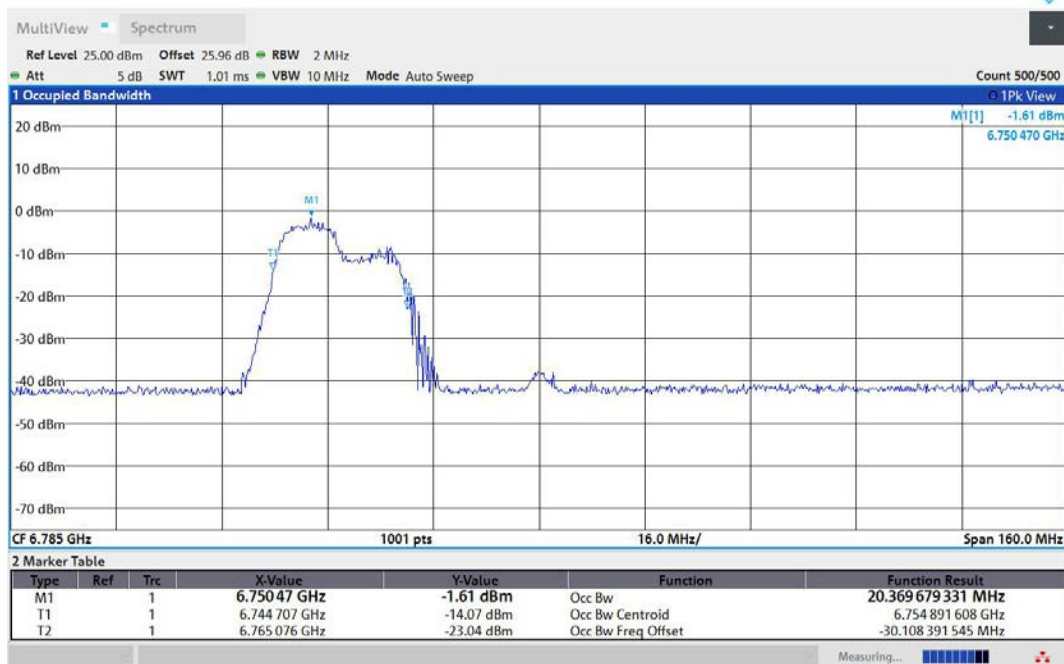
11AX80MIMO-Ant1-6785-106Tone-RU53-PASS
