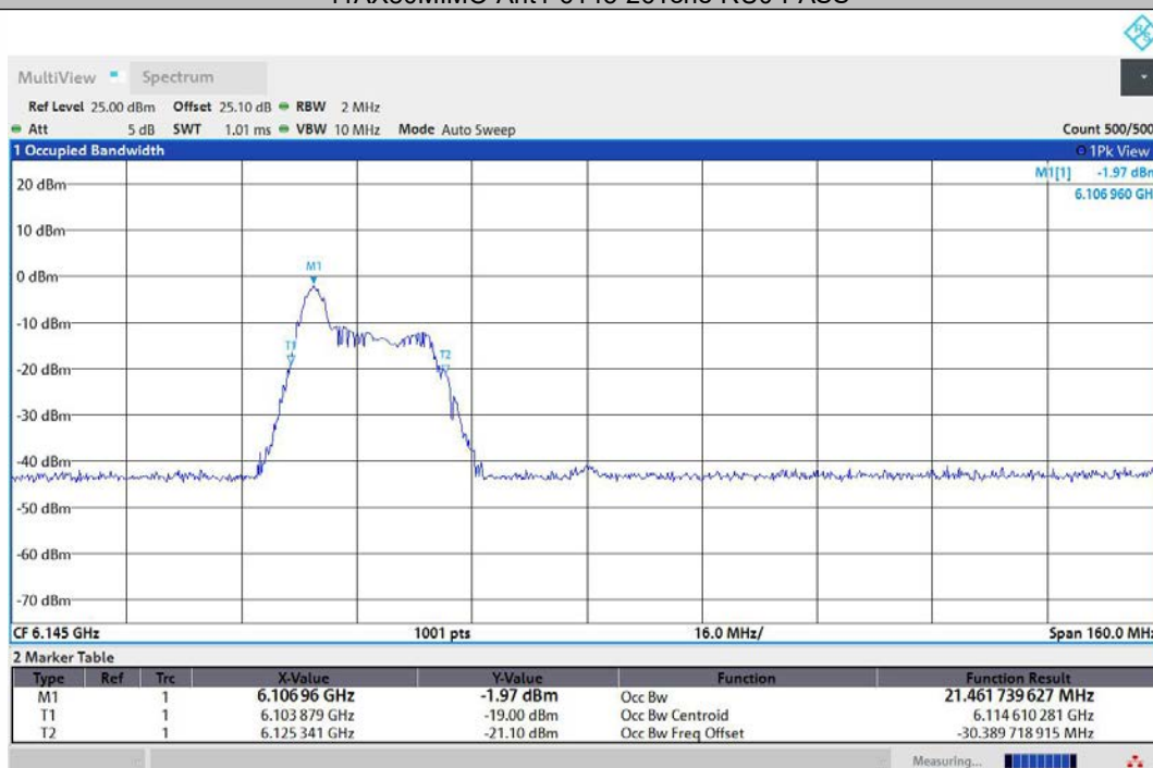
11AX80MIMO-Ant2-6145-26Tone-RU0-PASS
