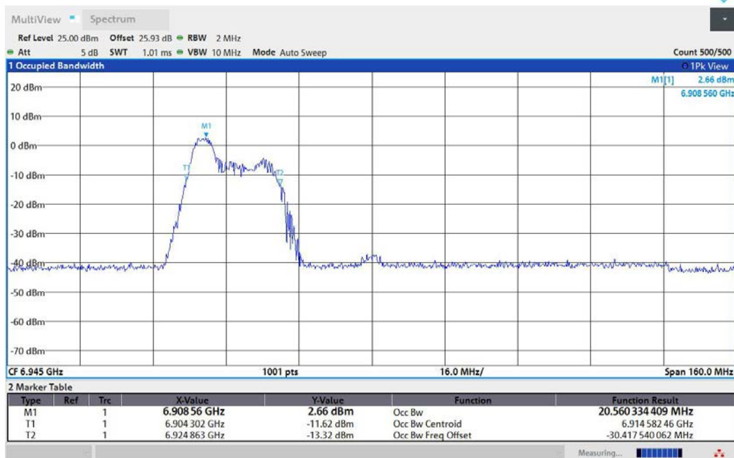
11AX80MIMO-Ant1-6945-52Tone-RU37-PASS
