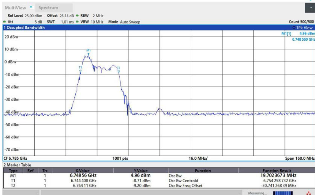
11AX80MIMO-Ant2-6785-52Tone-RU37-PASS
