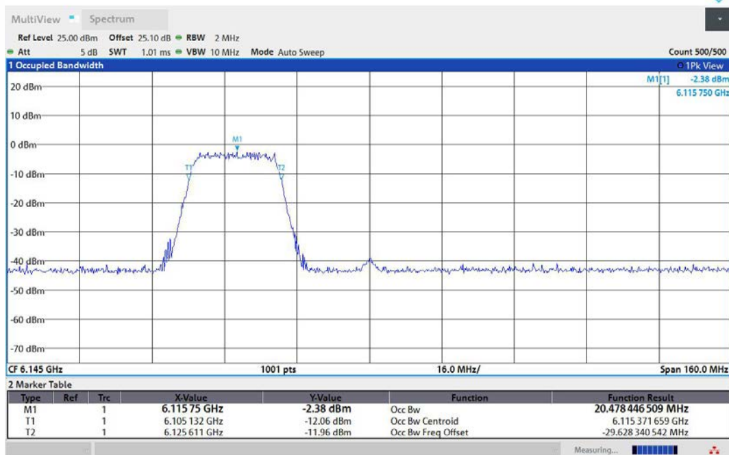
11AX80MIMO-Ant1-6145-242Tone-RU61-PASS
