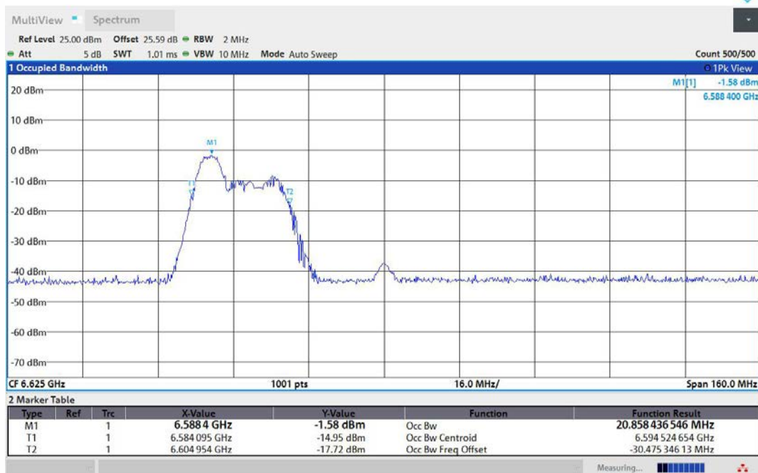
11AX80MIMO-Ant1-6625-52Tone-RU37-PASS
