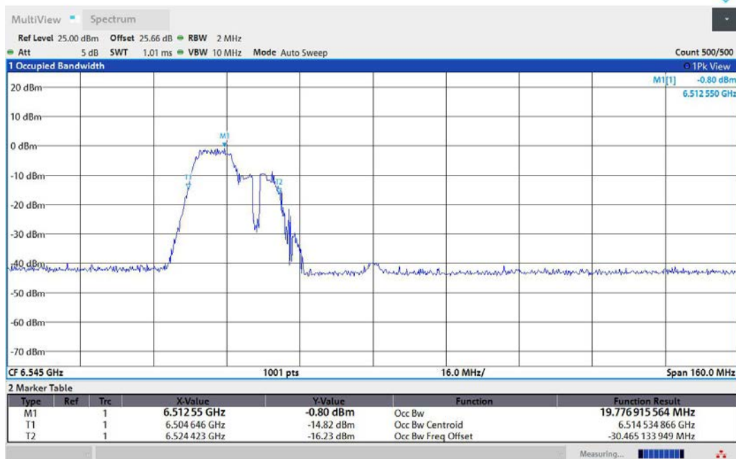
11AX80MIMO-Ant1-6545-106Tone-RU53-PASS
