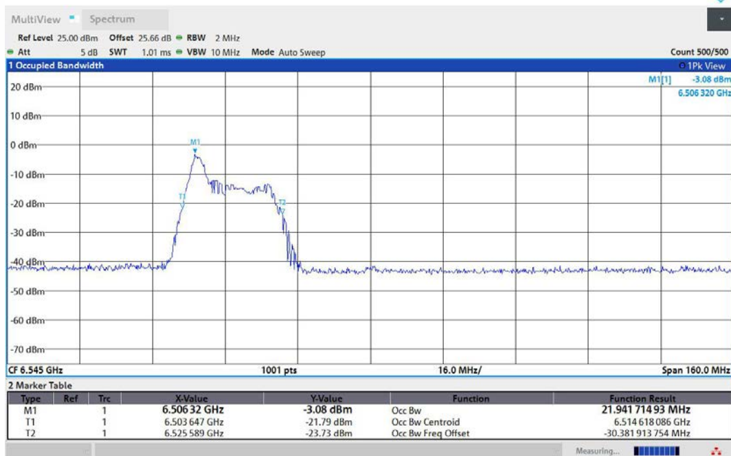
11AX80MIMO-Ant1-6545-26Tone-RU0-PASS
