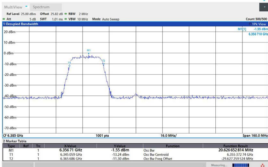
11AX80MIMO-Ant1-6385-242Tone-RU61-PASS
