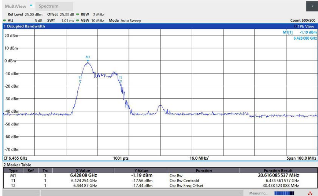
11AX80MIMO-Ant1-6465-52Tone-RU37-PASS
