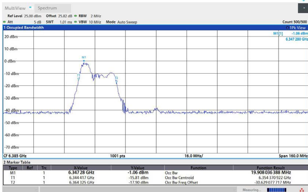
11AX80MIMO-Ant1-6385-52Tone-RU37-PASS
