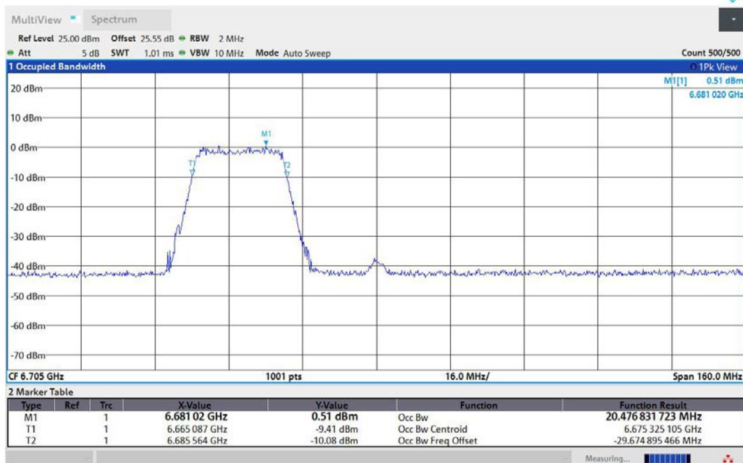
11AX80MIMO-Ant2-6705-242Tone-RU61-PASS
