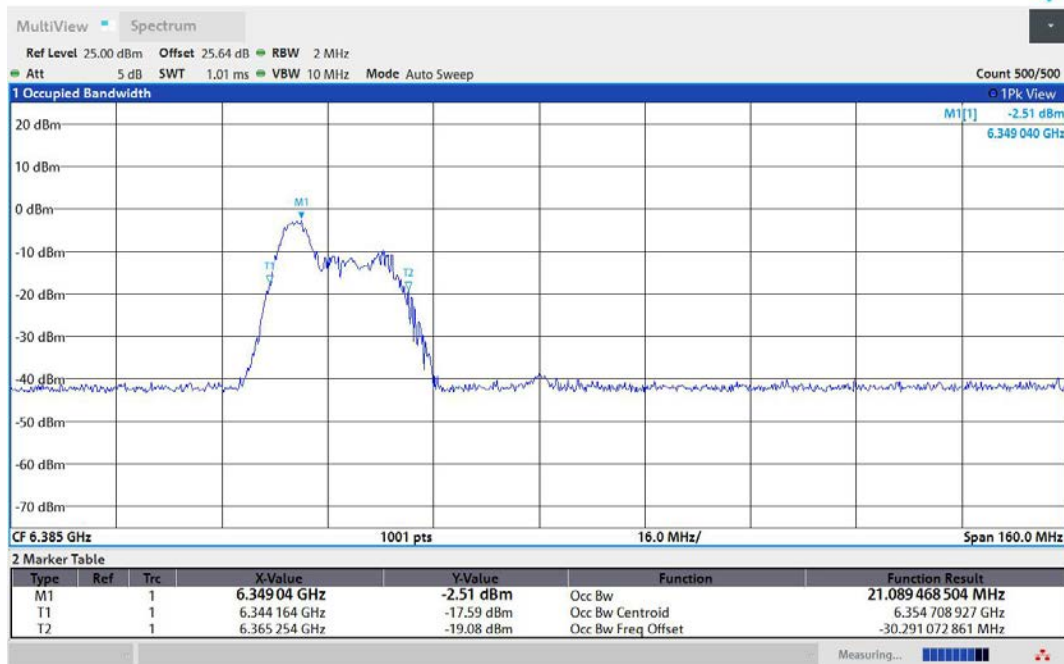
11AX80MIMO-Ant2-6385-52Tone-RU37-PASS
