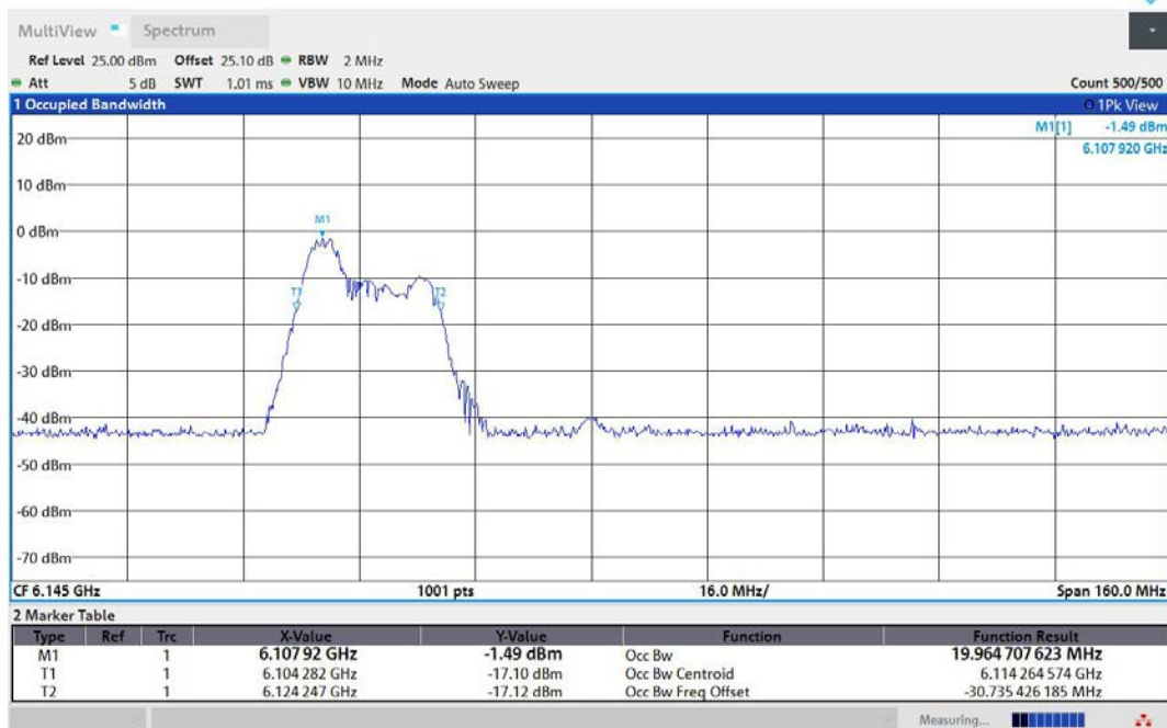
11AX80MIMO-Ant1-6145-52Tone-RU37-PASS
