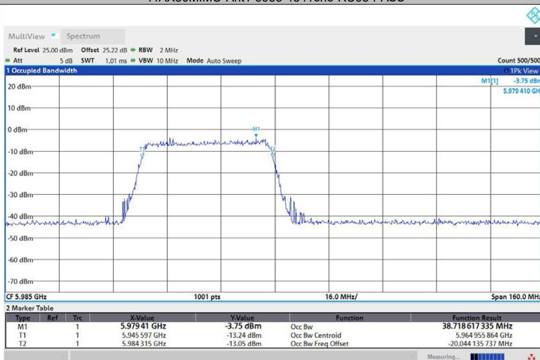
11AX80MIMO-Ant2-5985-484Tone-RU65-PASS
