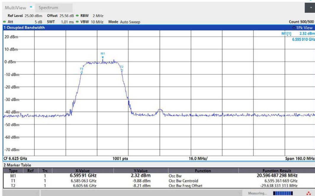
11AX80MIMO-Ant2-6625-242Tone-RU61-PASS
