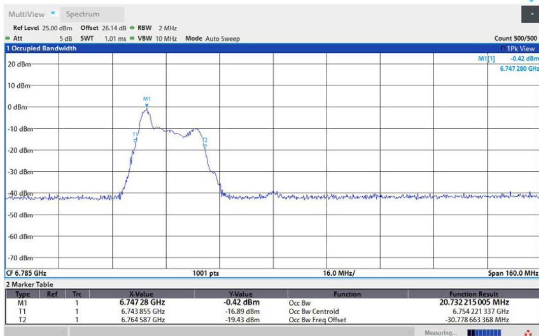
11AX80MIMO-Ant2-6785-26Tone-RU0-PASS
