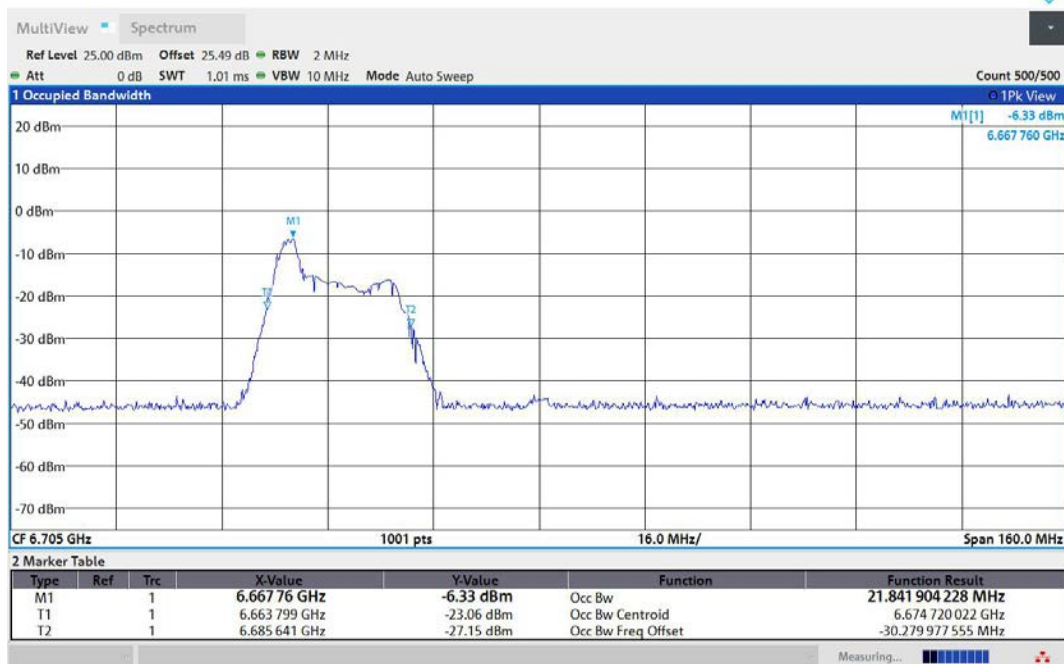
11AX80MIMO-Ant1-6705-26Tone-RU0-PASS
