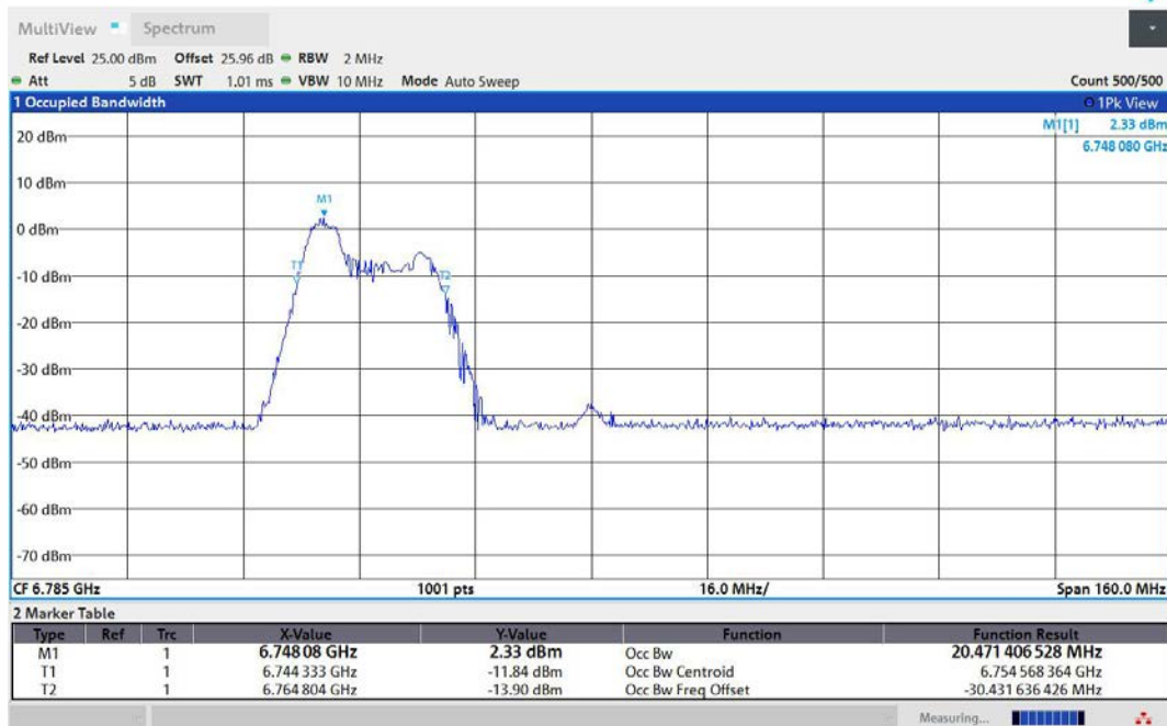
11AX80MIMO-Ant1-6785-52Tone-RU37-PASS
