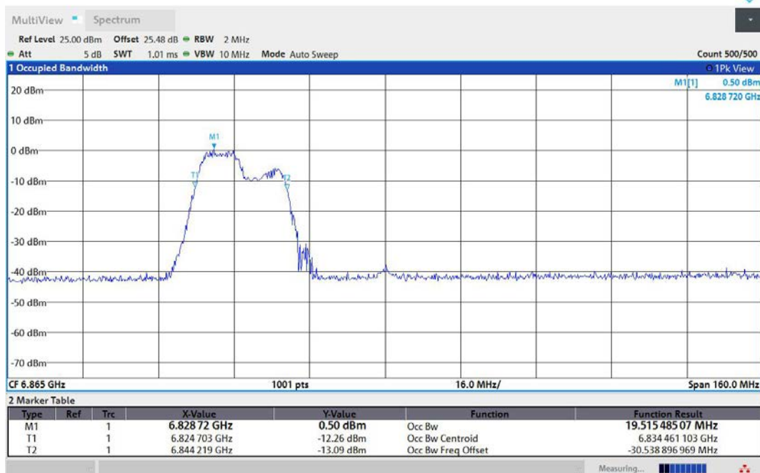
11AX80MIMO-Ant2-6865-106Tone-RU53-PASS
