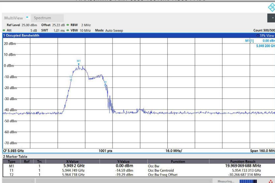
11AX80MIMO-Ant2-5985-106Tone-RU53-PASS
