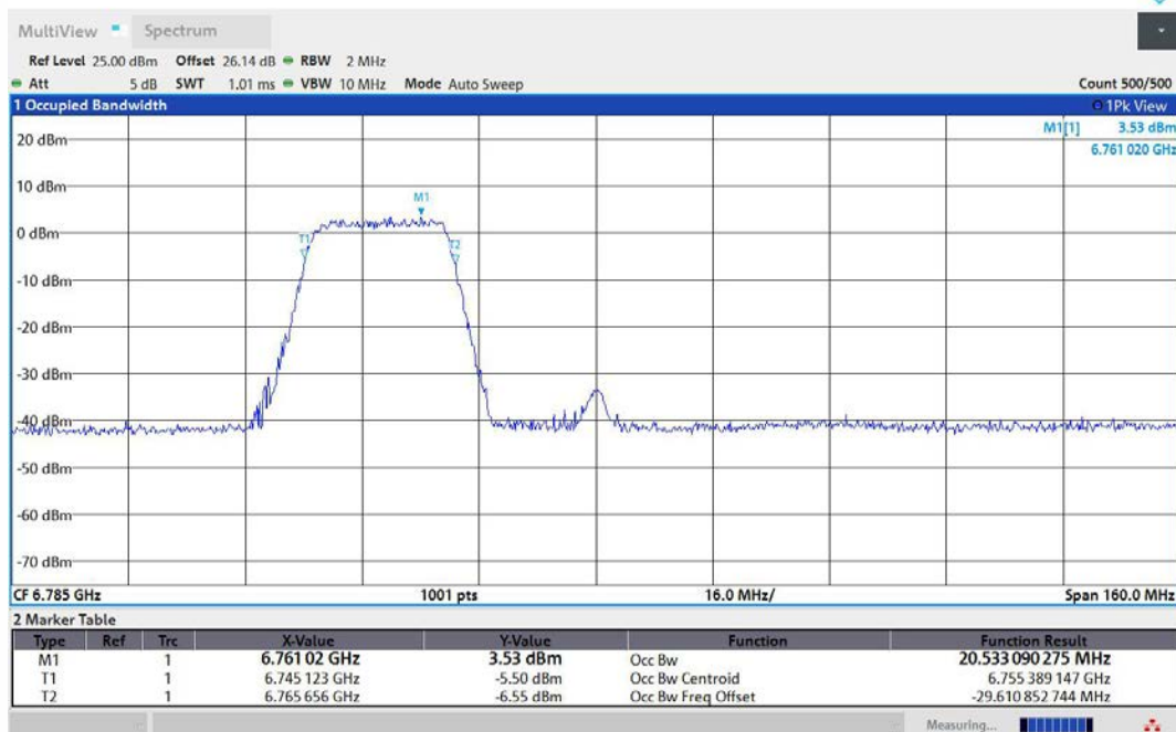
11AX80MIMO-Ant2-6785-242Tone-RU61-PASS
