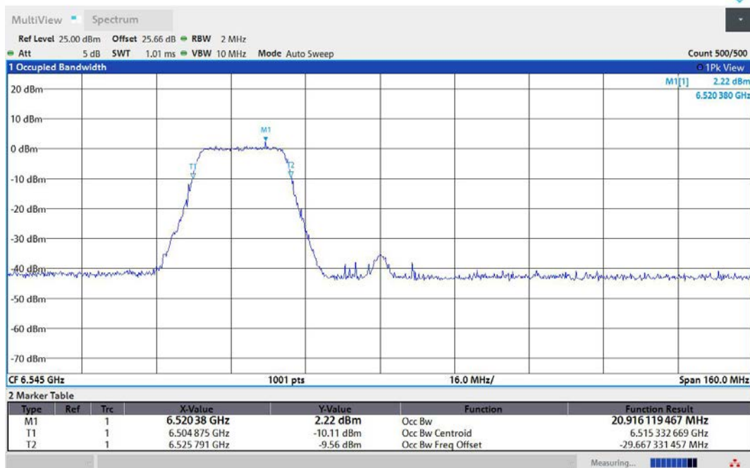
11AX80MIMO-Ant1-6545-242Tone-RU61-PASS
