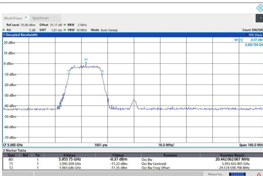
11AX80MIMO-Ant1-5985-242Tone-RU61-PASS
