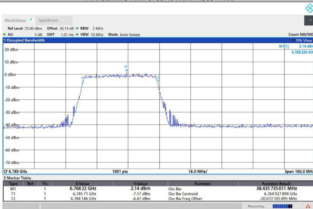
11AX80MIMO-Ant2-6785-484Tone-RU65-PASS
