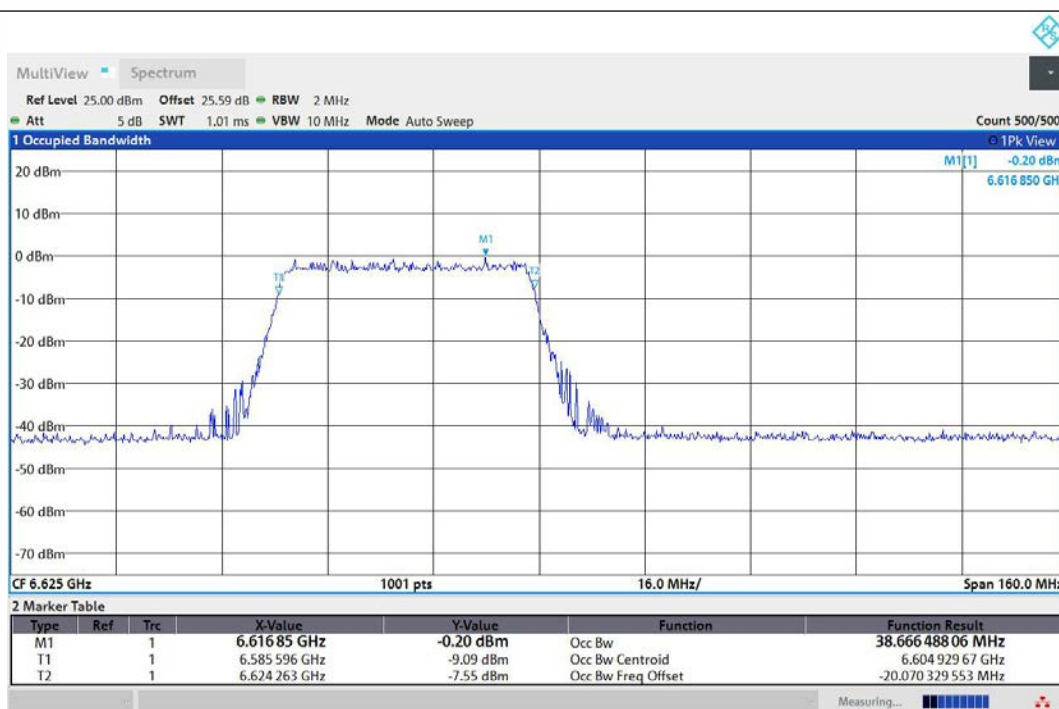
11AX80MIMO-Ant1-6625-484Tone-RU65-PASS
