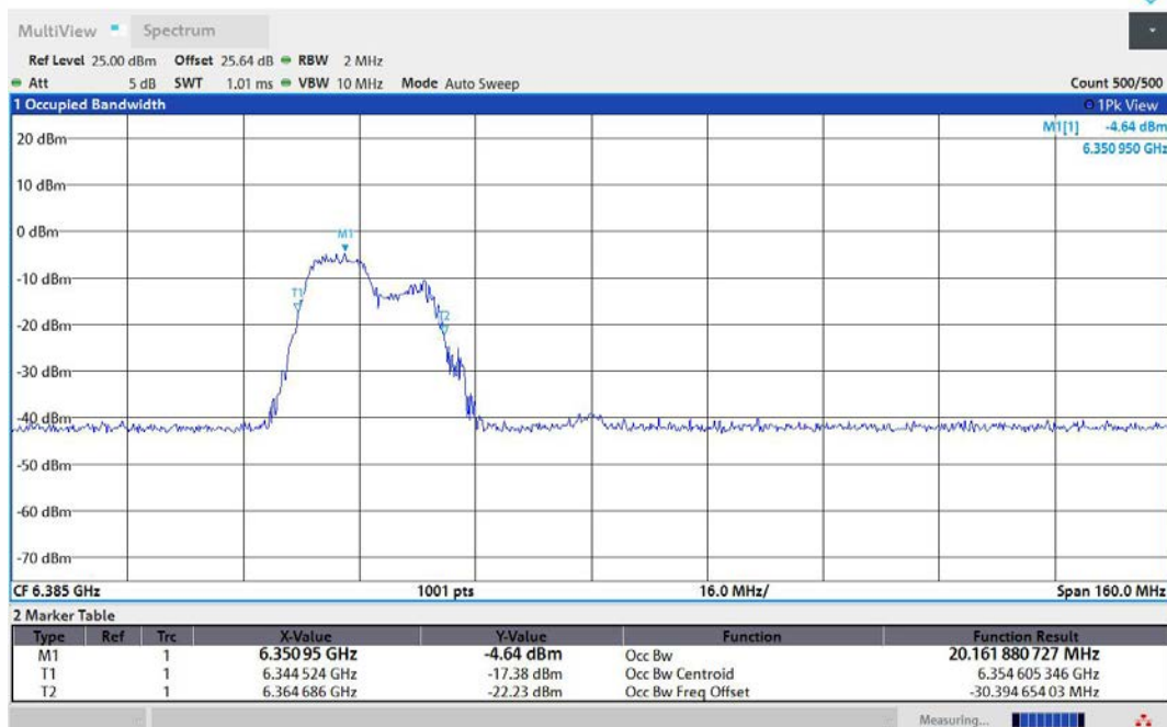
11AX80MIMO-Ant2-6385-106Tone-RU53-PASS
