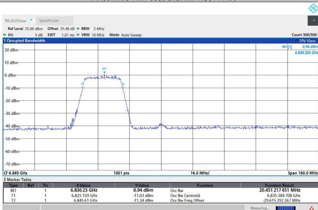
11AX80MIMO-Ant2-6865-242Tone-RU61-PASS
