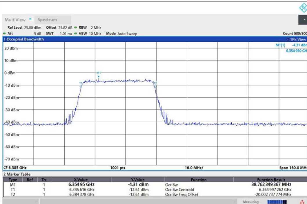
11AX80MIMO-Ant1-6385-484Tone-RU65-PASS
