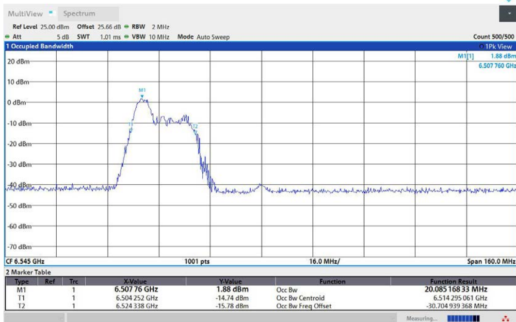
11AX80MIMO-Ant1-6545-52Tone-RU37-PASS
