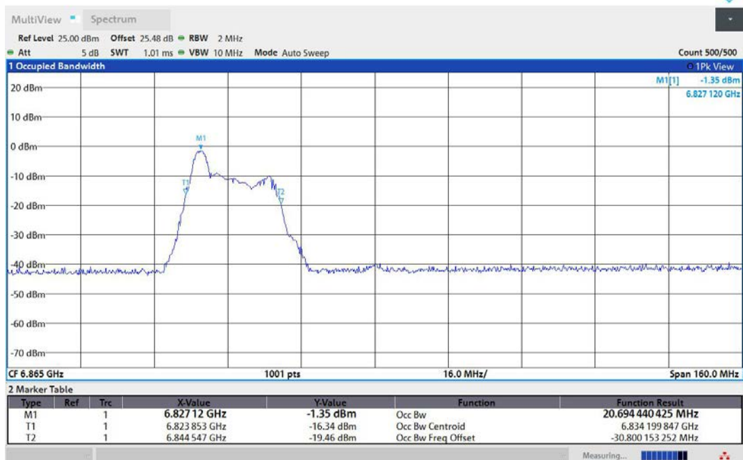
11AX80MIMO-Ant2-6865-26Tone-RU0-PASS
