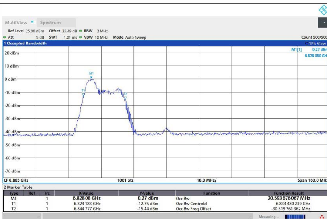
11AX80MIMO-Ant1-6865-52Tone-RU37-PASS
