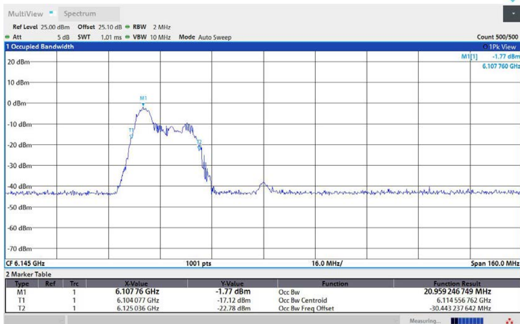
11AX80MIMO-Ant2-6145-52Tone-RU37-PASS
