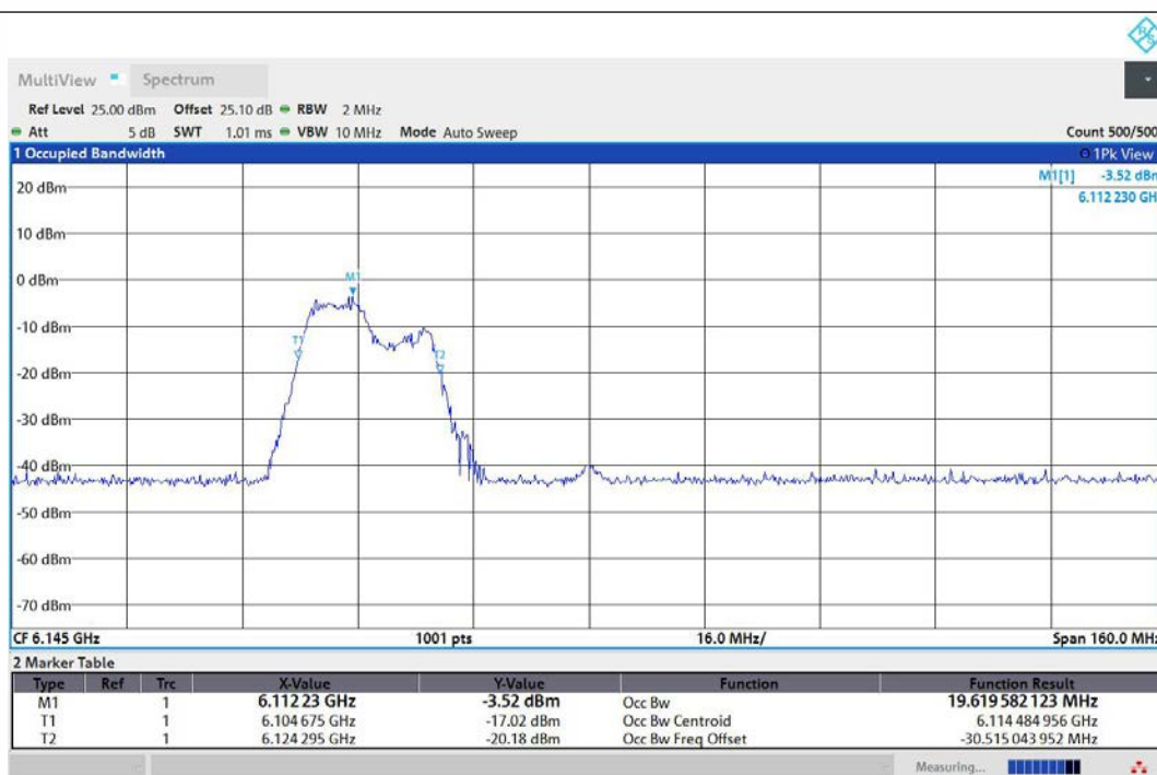
11AX80MIMO-Ant1-6145-106Tone-RU53-PASS
