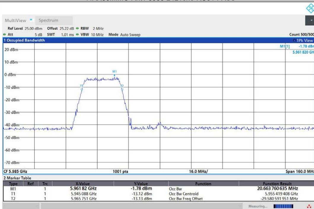
11AX80MIMO-Ant2-5985-242Tone-RU61-PASS
