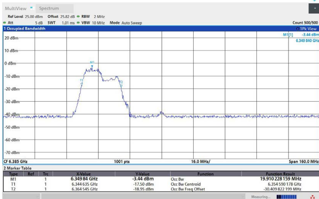
11AX80MIMO-Ant1-6385-106Tone-RU53-PASS
