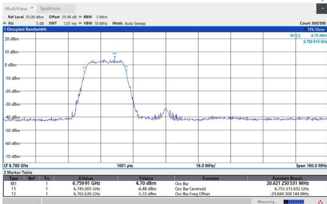
11AX80MIMO-Ant1-6785-242Tone-RU61-PASS
