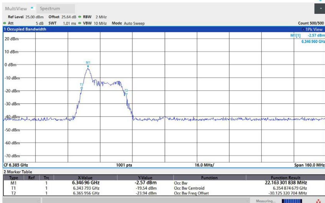
11AX80MIMO-Ant2-6385-26Tone-RU0-PASS
