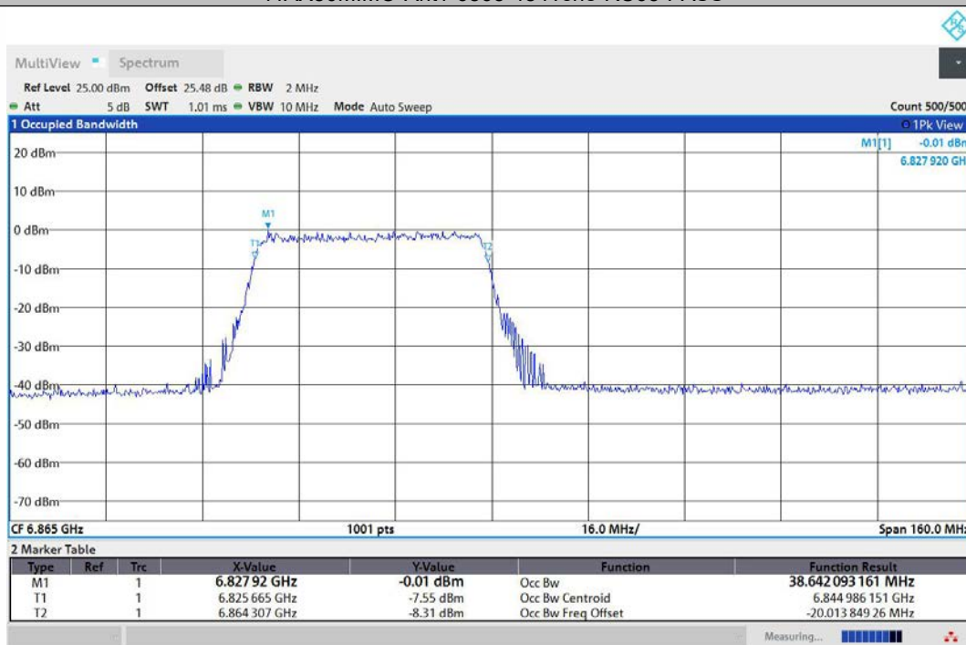
11AX80MIMO-Ant2-6865-484Tone-RU65-PASS
