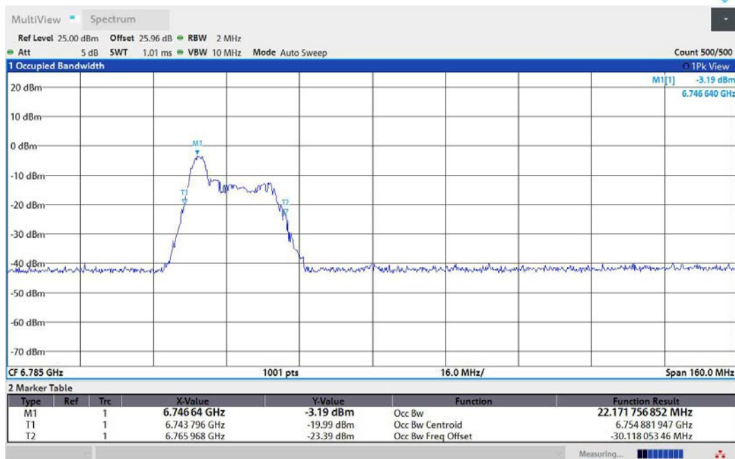
11AX80MIMO-Ant1-6785-26Tone-RU0-PASS
