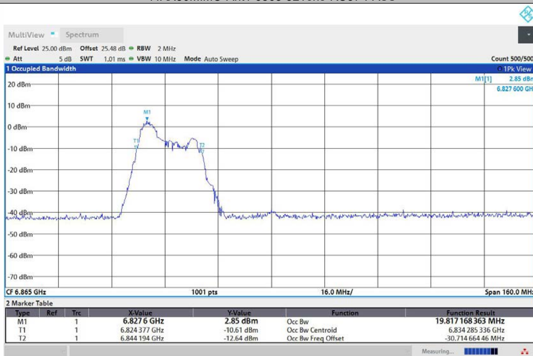
11AX80MIMO-Ant2-6865-52Tone-RU37-PASS
