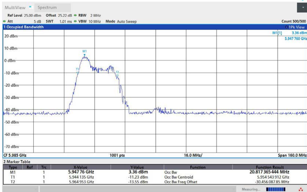
11AX80MIMO-Ant2-5985-52Tone-RU37-PASS
