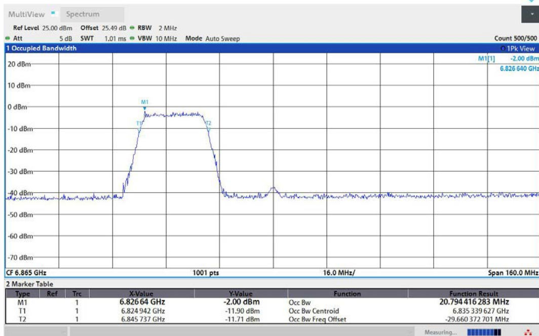
11AX80MIMO-Ant1-6865-242Tone-RU61-PASS
