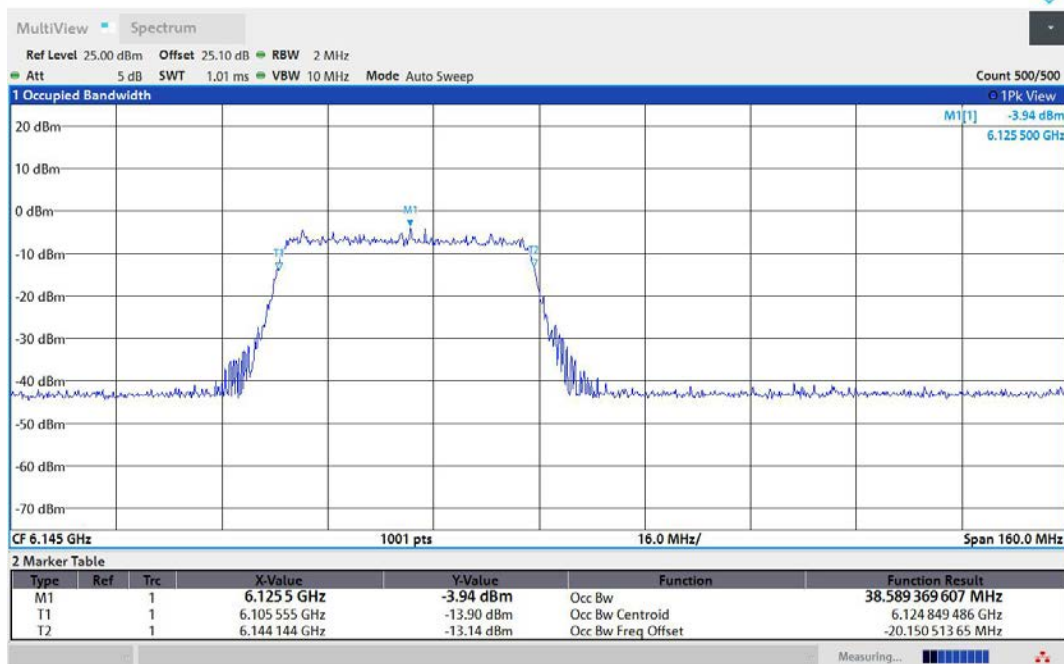
11AX80MIMO-Ant1-6145-484Tone-RU65-PASS
