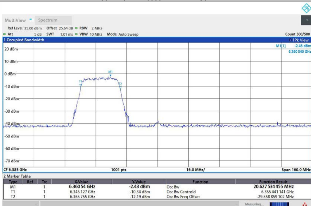
11AX80MIMO-Ant2-6385-242Tone-RU61-PASS
