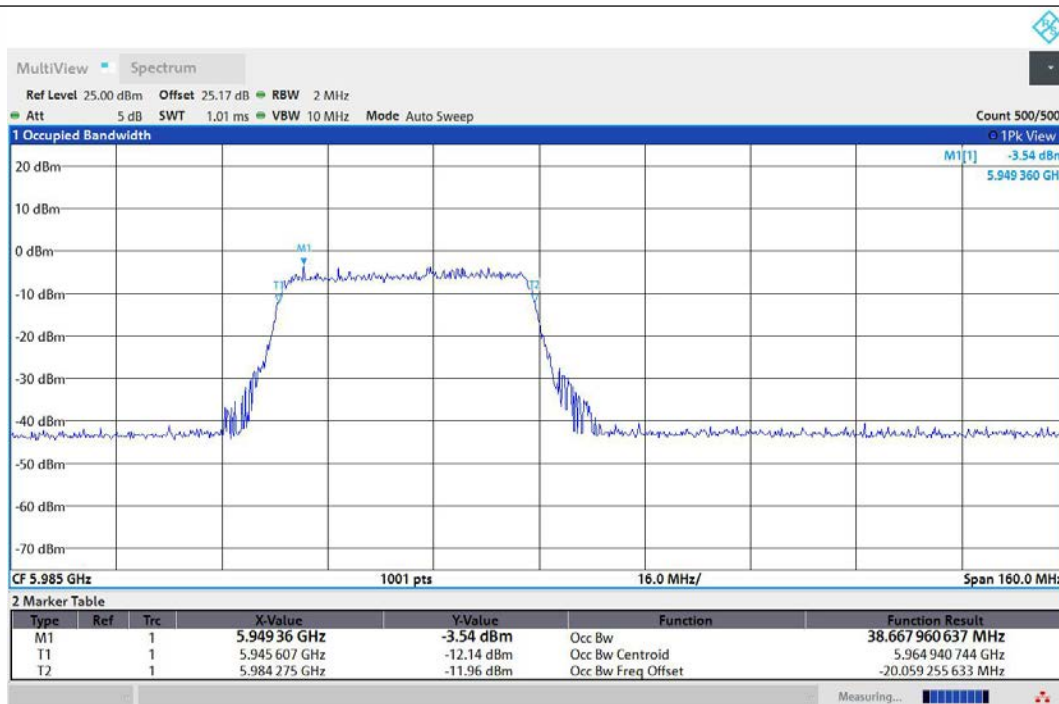
11AX80MIMO-Ant1-5985-484Tone-RU65-PASS
