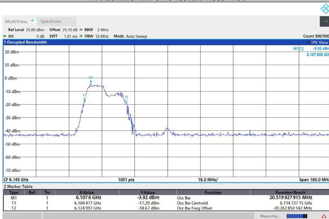
11AX80MIMO-Ant2-6145-106Tone-RU53-PASS
