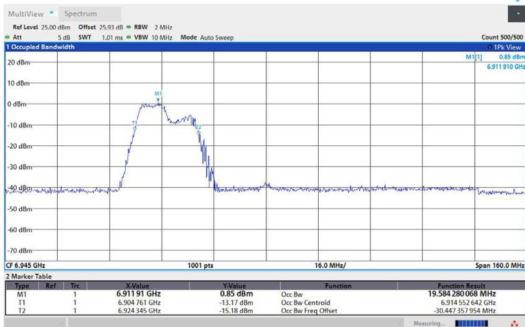
11AX80MIMO-Ant1-6945-106Tone-RU53-PASS
