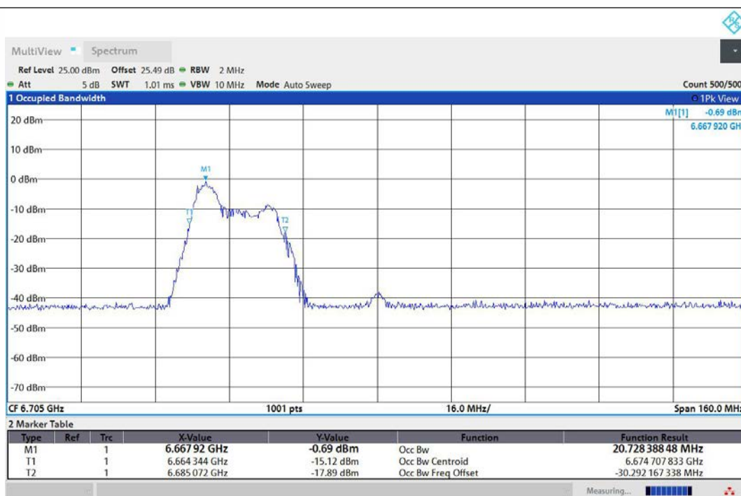
11AX80MIMO-Ant1-6705-52Tone-RU37-PASS
