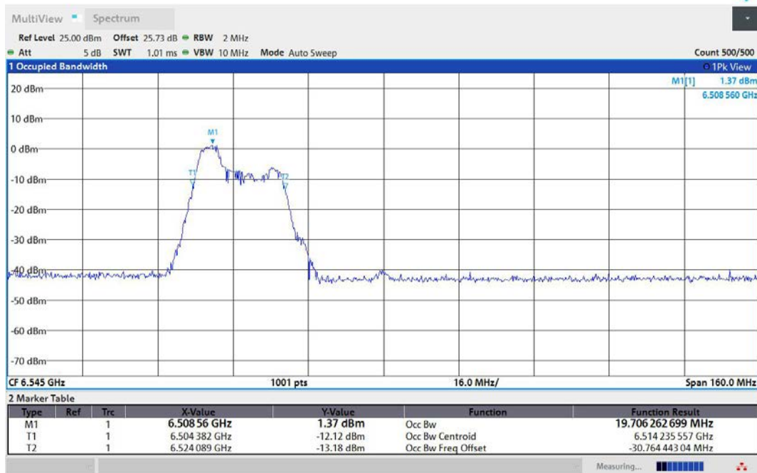
11AX80MIMO-Ant2-6545-52Tone-RU37-PASS
