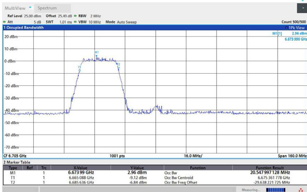
11AX80MIMO-Ant1-6705-242Tone-RU61-PASS
