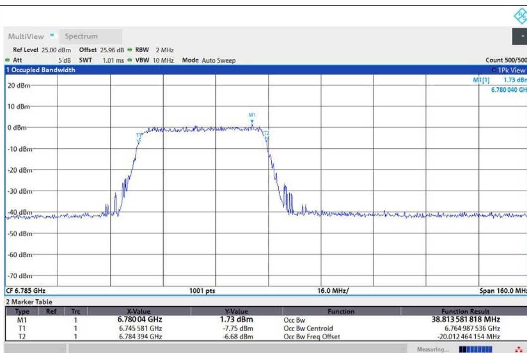
11AX80MIMO-Ant1-6785-484Tone-RU65-PASS
