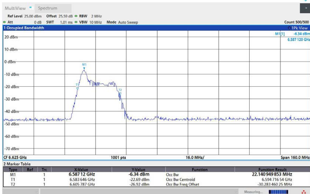
11AX80MIMO-Ant1-6625-26Tone-RU0-PASS
