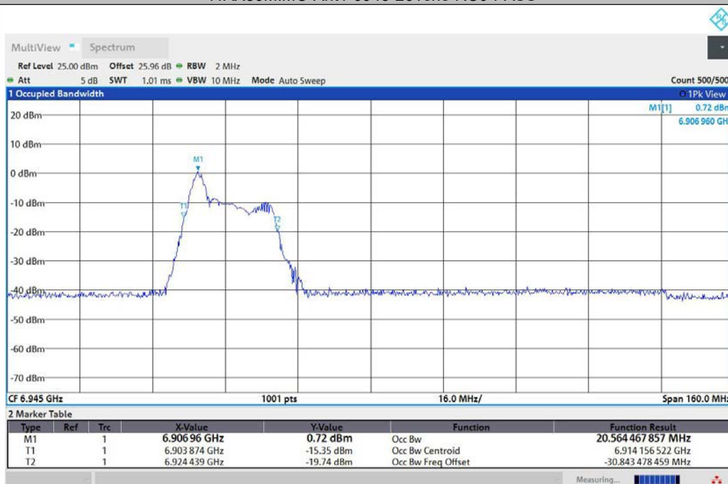
11AX80MIMO-Ant2-6945-26Tone-RU0-PASS
