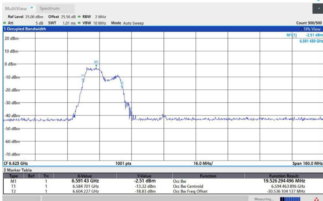
11AX80MIMO-Ant2-6625-106Tone-RU53-PASS
