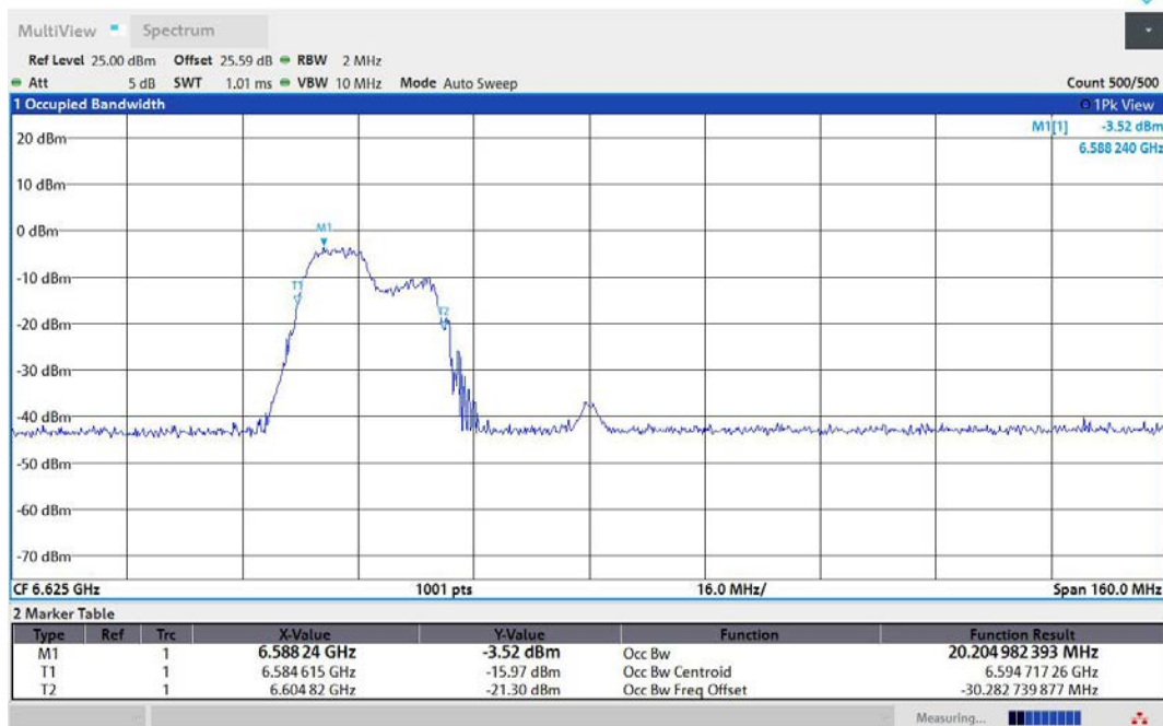
11AX80MIMO-Ant1-6625-106Tone-RU53-PASS
