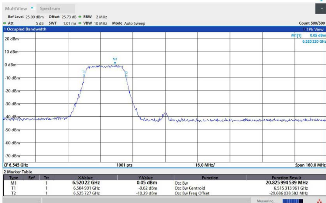
11AX80MIMO-Ant2-6545-242Tone-RU61-PASS
