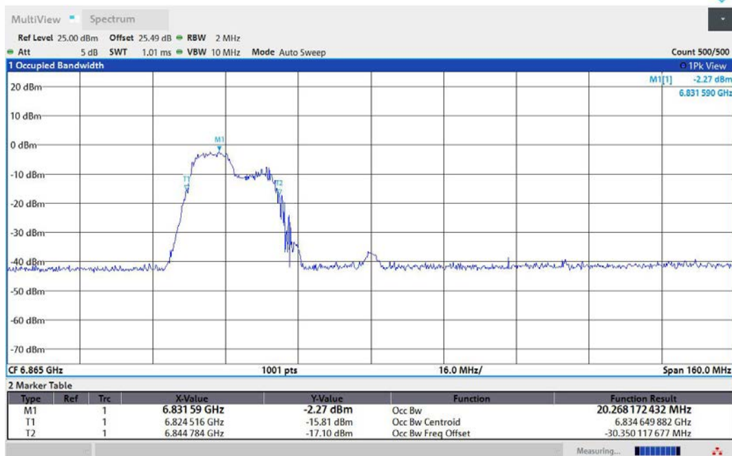
11AX80MIMO-Ant1-6865-106Tone-RU53-PASS
