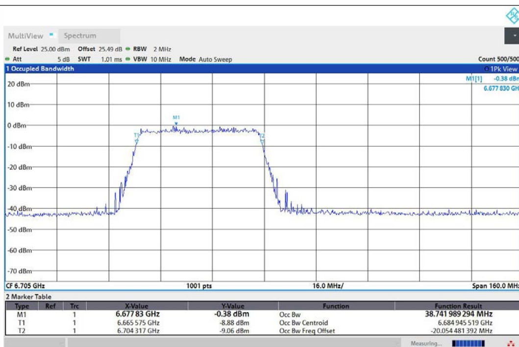
11AX80MIMO-Ant1-6705-484Tone-RU65-PASS
