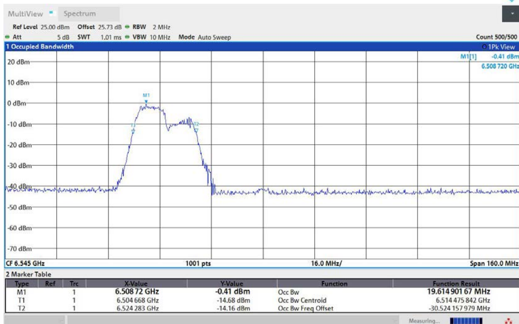
11AX80MIMO-Ant2-6545-106Tone-RU53-PASS
