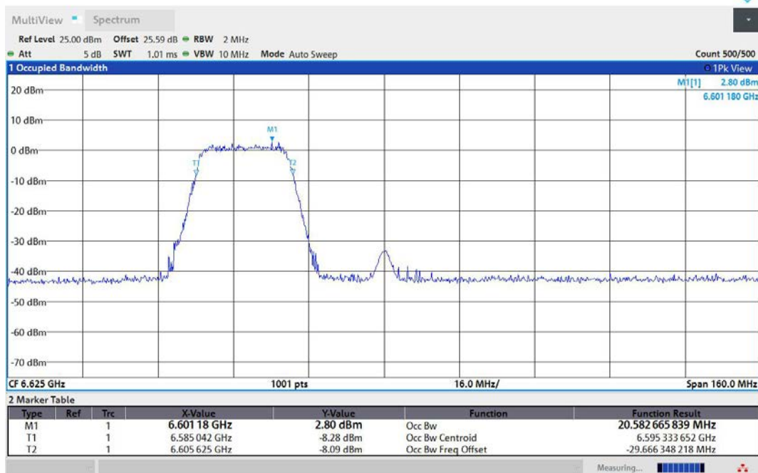
11AX80MIMO-Ant1-6625-242Tone-RU61-PASS
