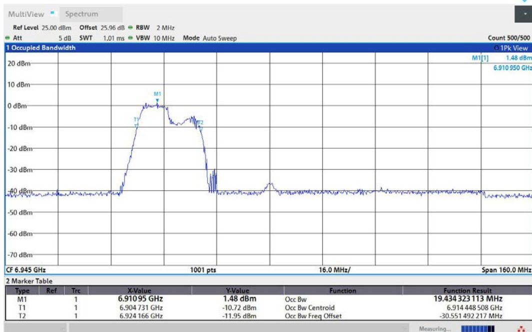
11AX80MIMO-Ant2-6945-106Tone-RU53-PASS
