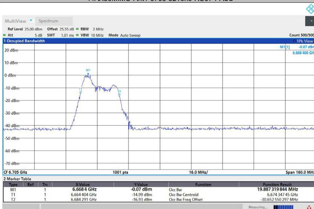
11AX80MIMO-Ant2-6705-52Tone-RU37-PASS
