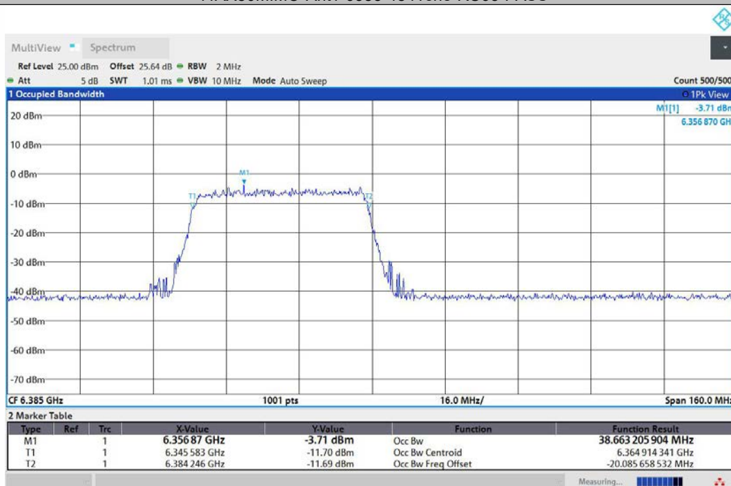
11AX80MIMO-Ant2-6385-484Tone-RU65-PASS
