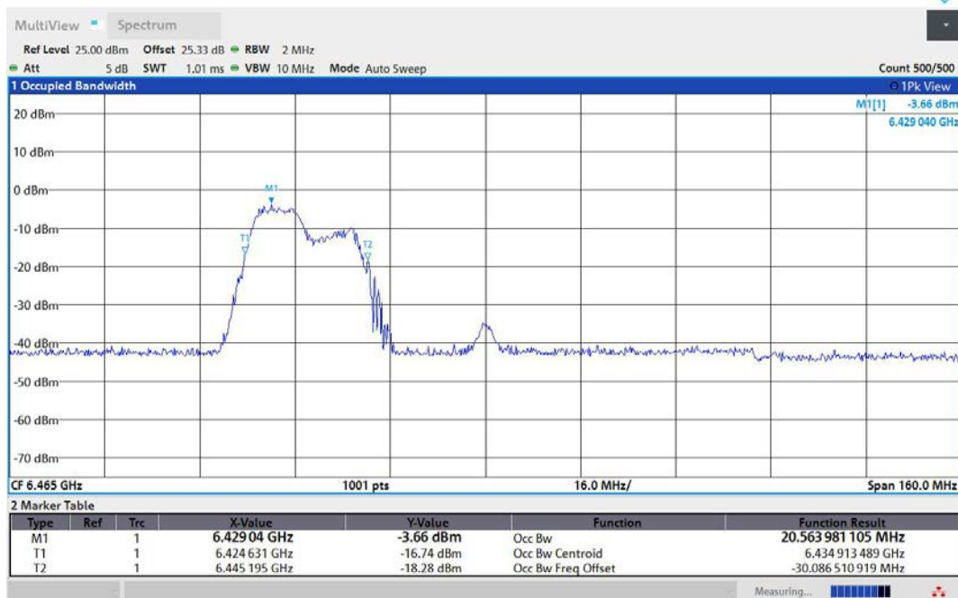
11AX80MIMO-Ant1-6465-106Tone-RU53-PASS
