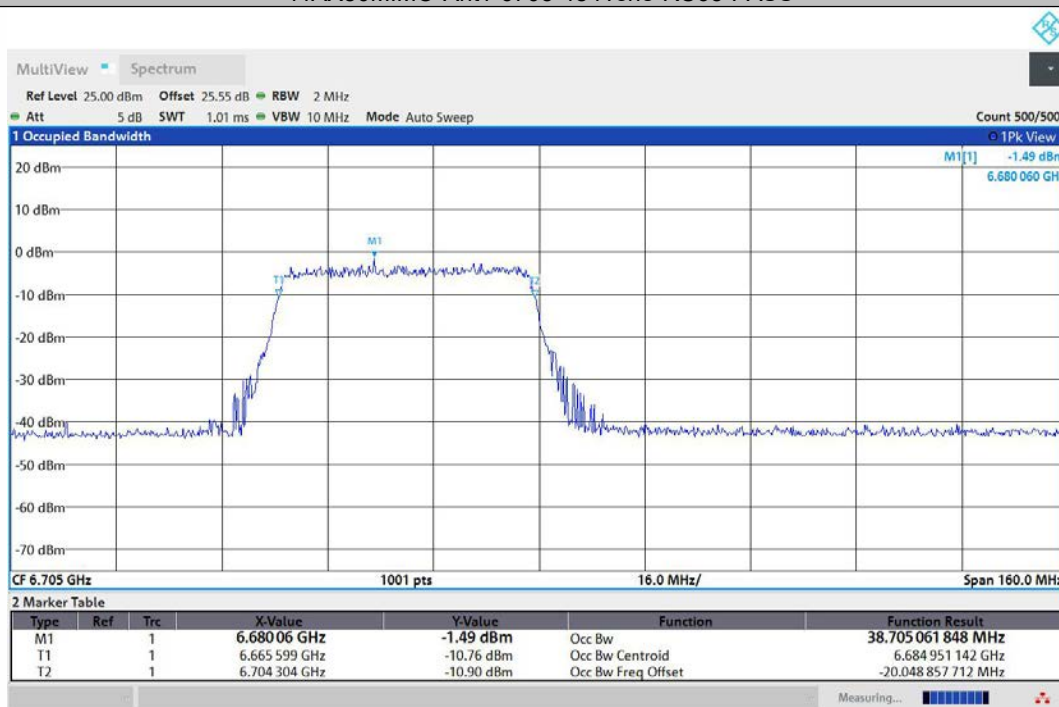
11AX80MIMO-Ant2-6705-484Tone-RU65-PASS
