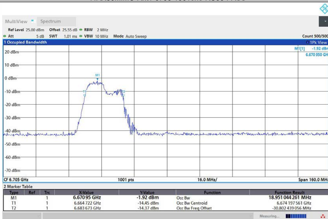
11AX80MIMO-Ant2-6705-106Tone-RU53-PASS
