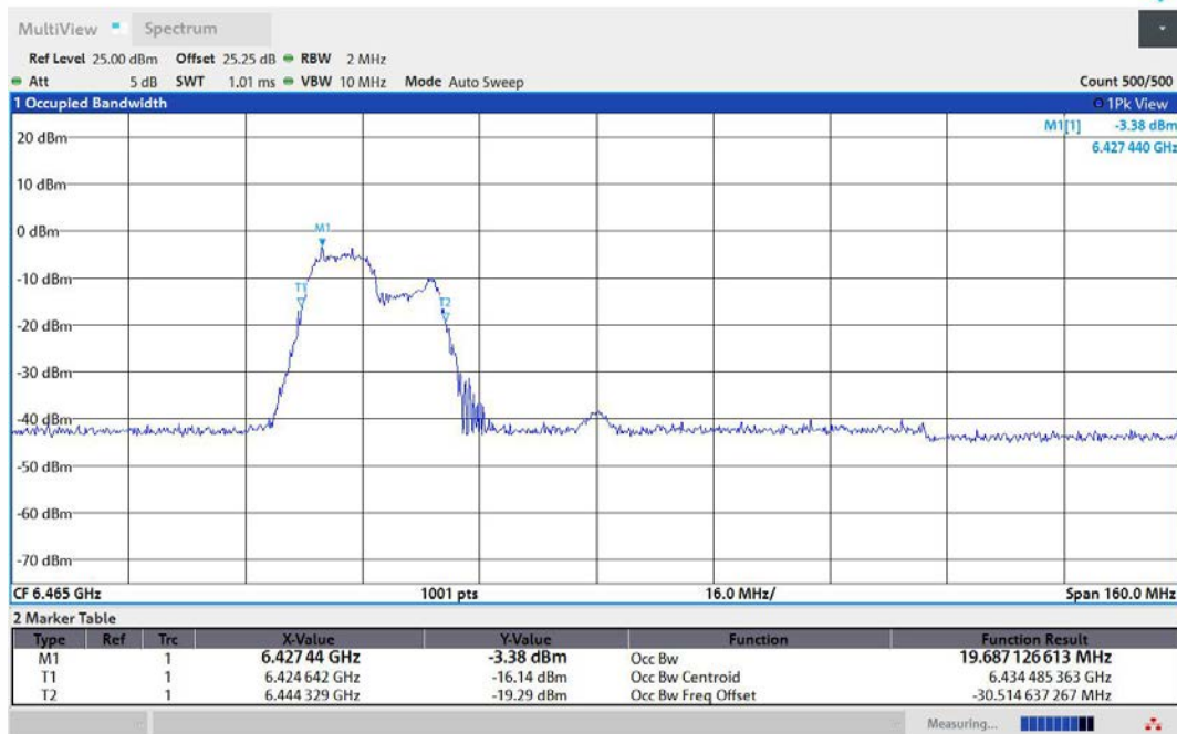
11AX80MIMO-Ant2-6465-106Tone-RU53-PASS
