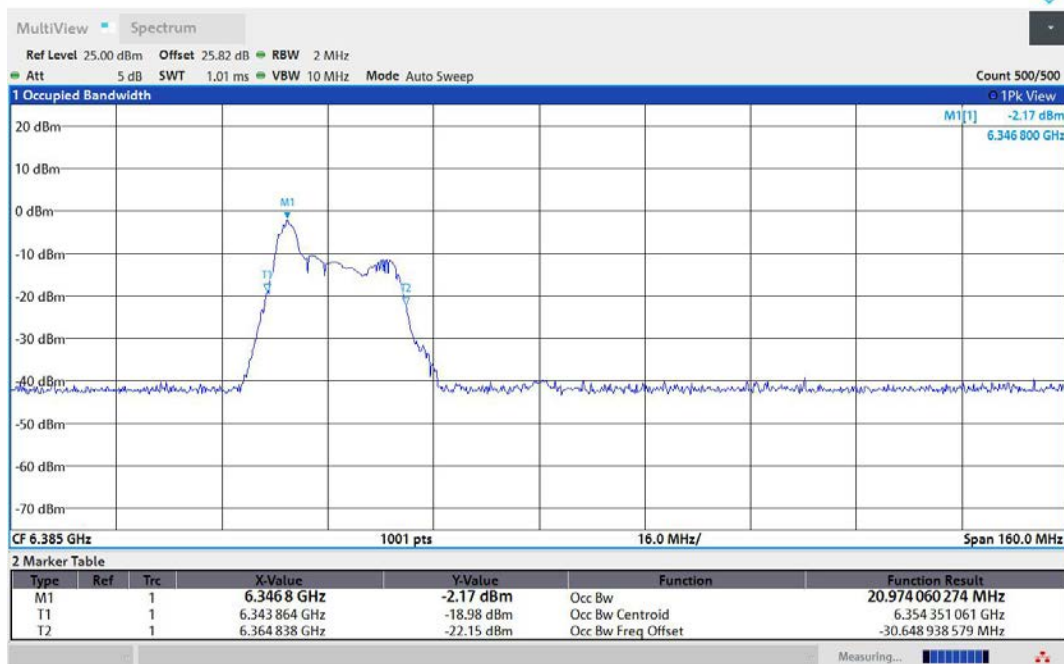
11AX80MIMO-Ant1-6385-26Tone-RU0-PASS
