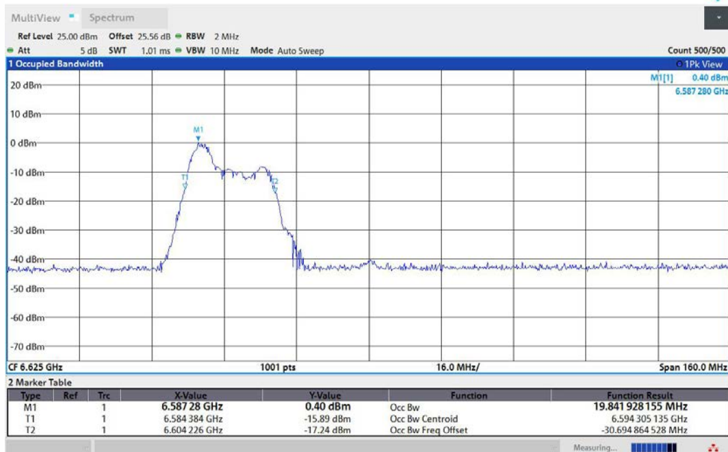
11AX80MIMO-Ant2-6625-52Tone-RU37-PASS
