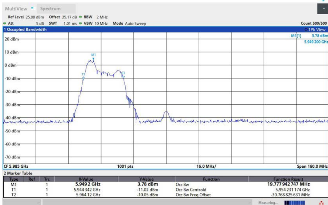
11AX80MIMO-Ant1-5985-52Tone-RU37-PASS
