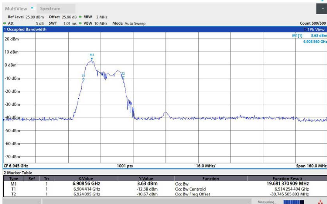
11AX80MIMO-Ant2-6945-52Tone-RU37-PASS
