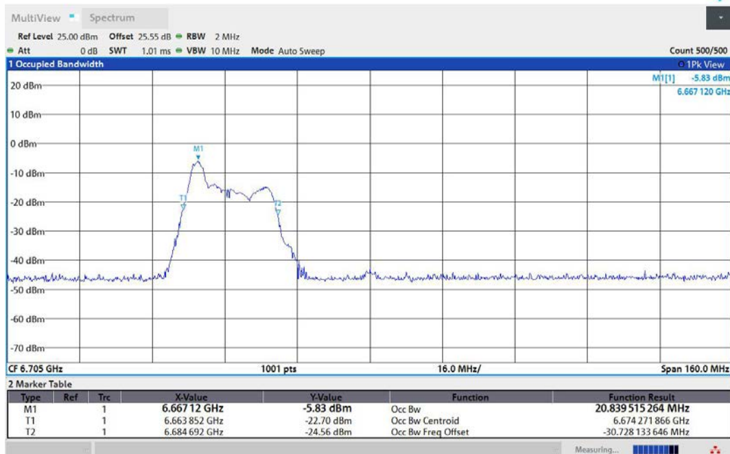
11AX80MIMO-Ant2-6705-26Tone-RU0-PASS
