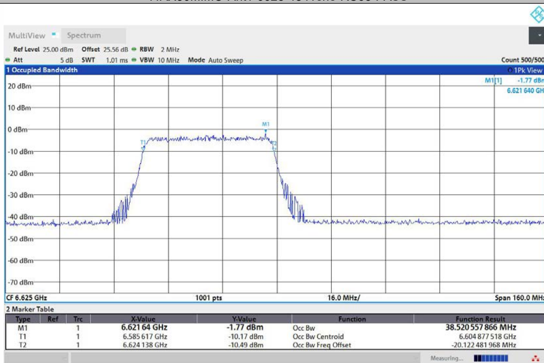
11AX80MIMO-Ant2-6625-484Tone-RU65-PASS
