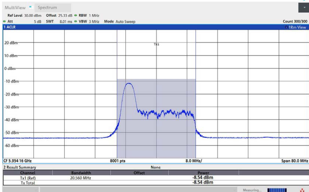
11AX40MIMO-Ant2-5965-26Tone-RU0-PASS
