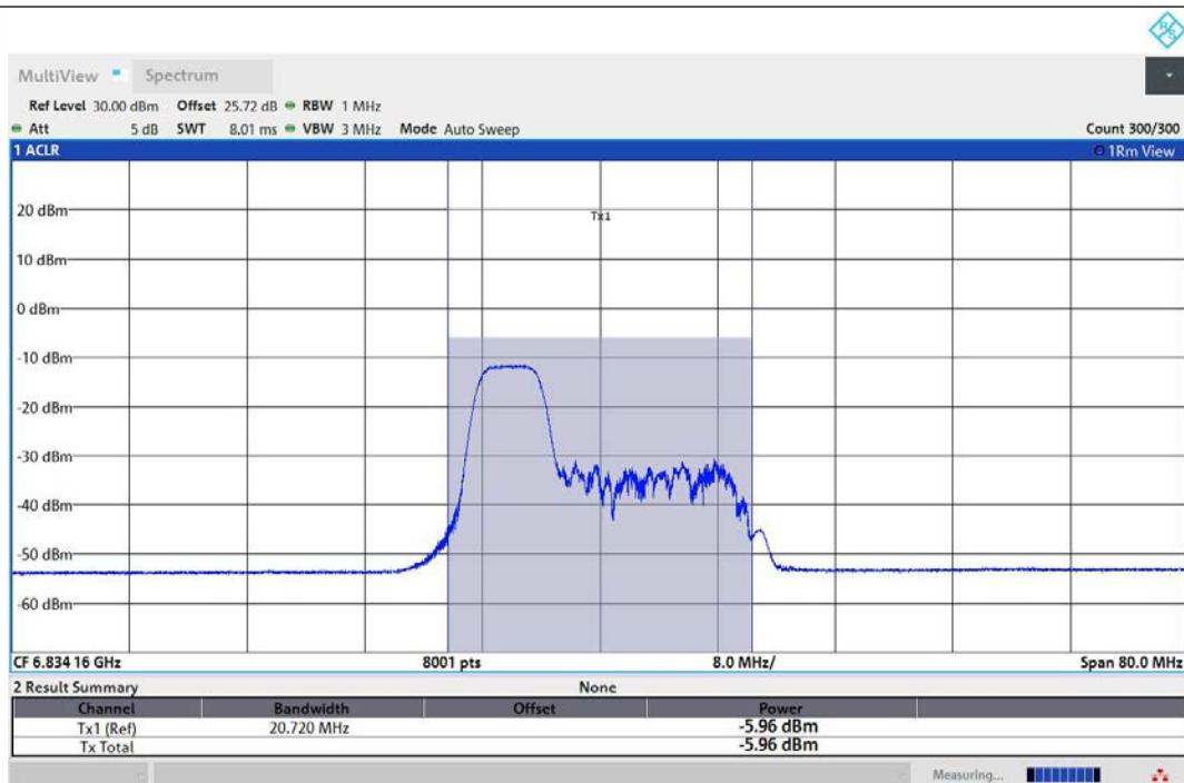
11AX40MIMO-Ant1-6845-52Tone-RU37-PASS
