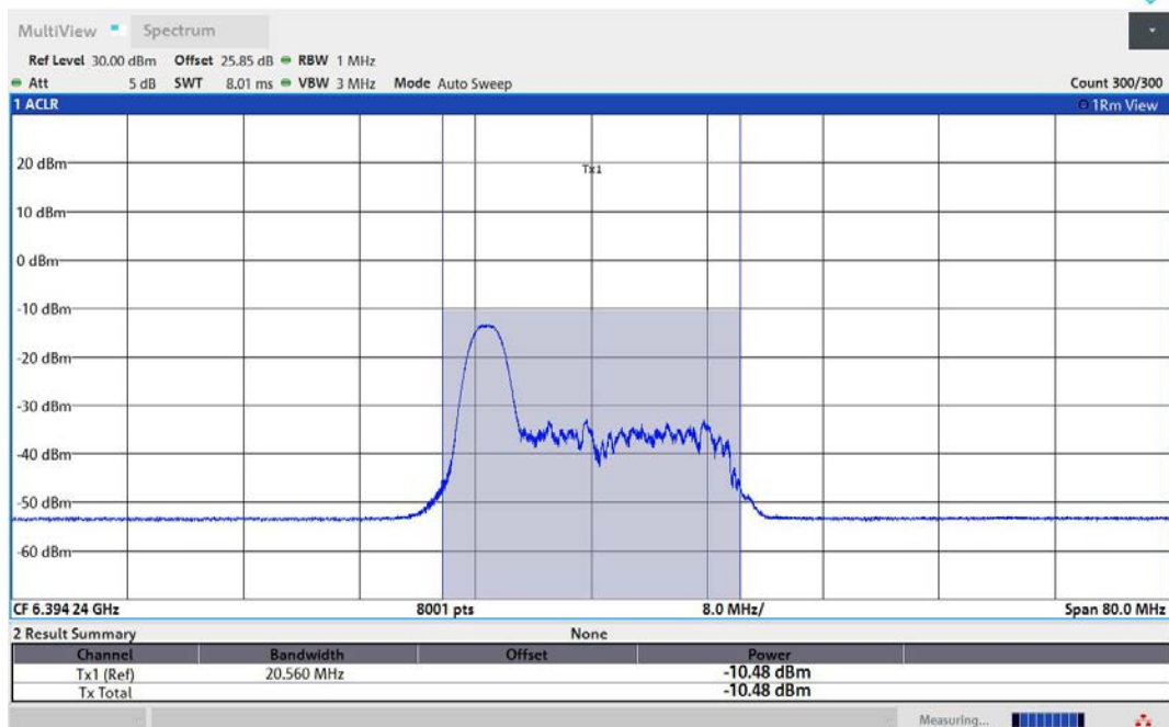
11AX40MIMO-Ant2-6405-26Tone-RU0-PASS
