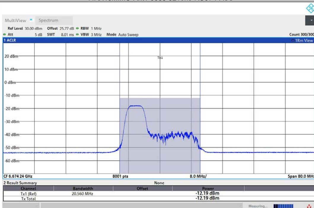
11AX40MIMO-Ant2-6685-52Tone-RU37-PASS
