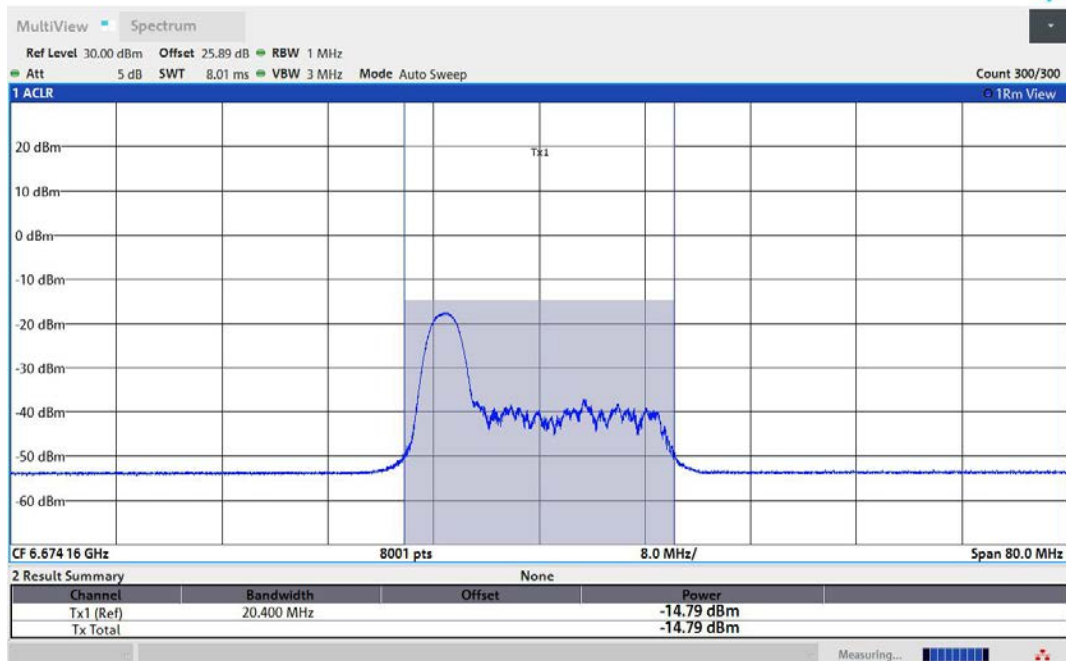
11AX40MIMO-Ant2-6685-26Tone-RU0-PASS
