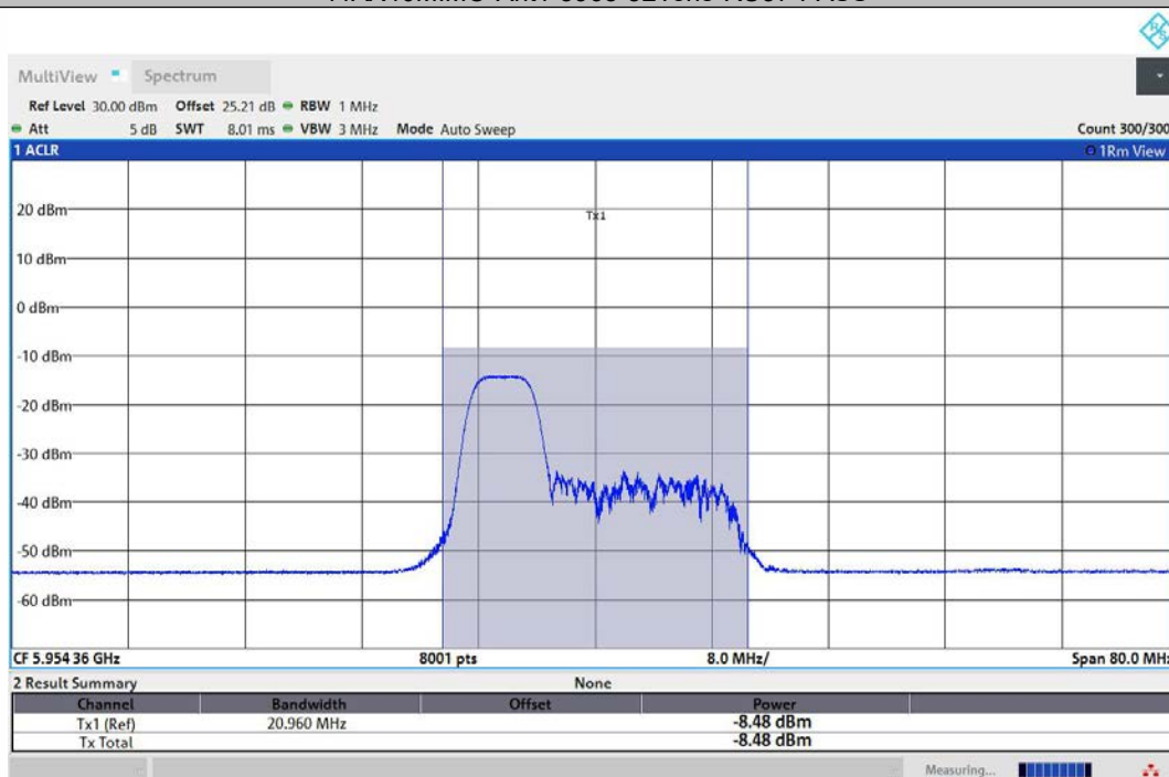
11AX40MIMO-Ant2-5965-52Tone-RU37-PASS
