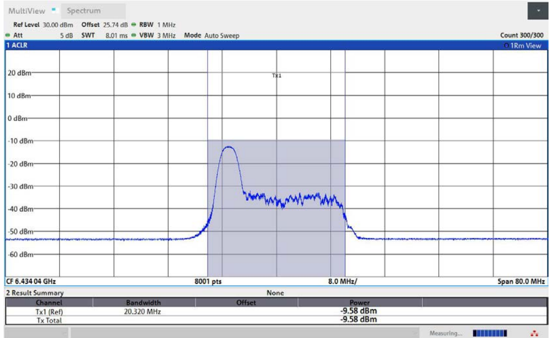
11AX40MIMO-Ant1-6445-26Tone-RU0-PASS
