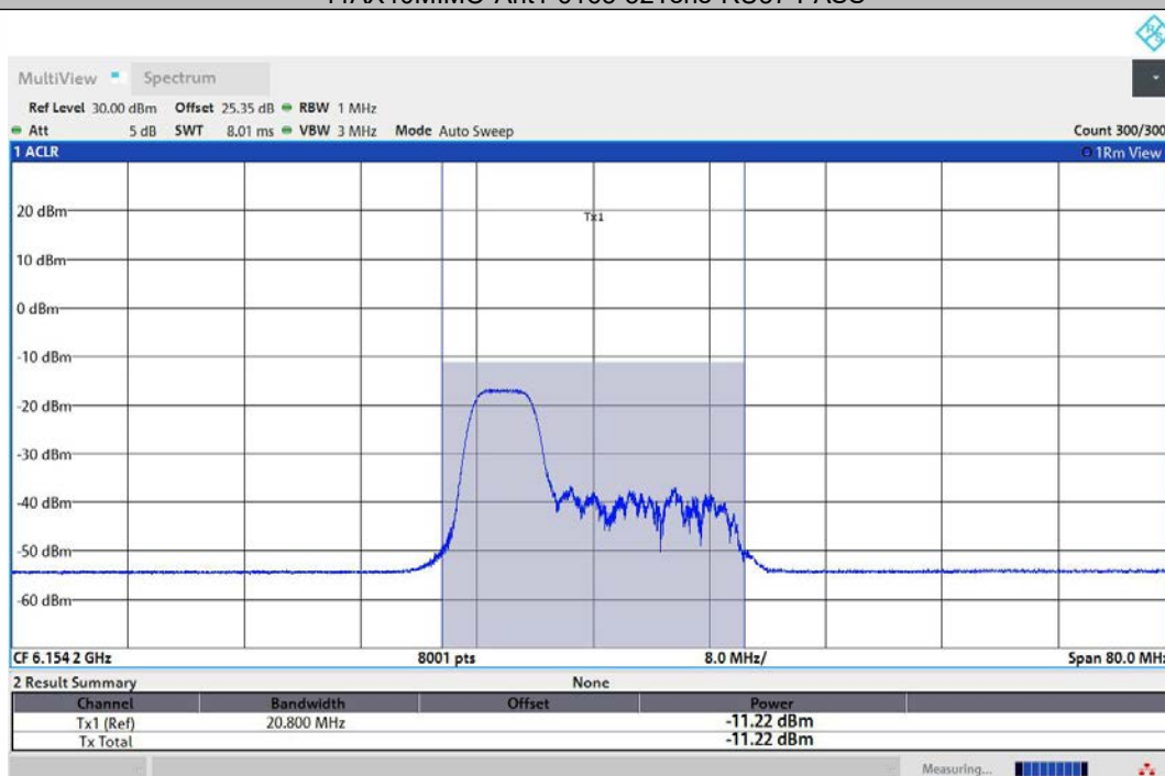
11AX40MIMO-Ant2-6165-52Tone-RU37-PASS
