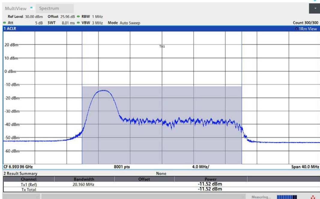
11AX20MIMO-Ant2-6995-26Tone-RU0-PASS
