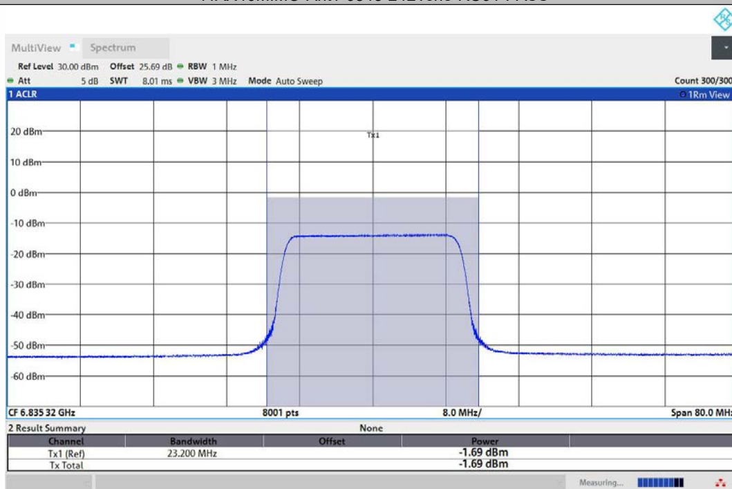
11AX40MIMO-Ant2-6845-242Tone-RU61-PASS
