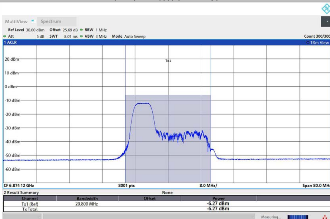
11AX40MIMO-Ant2-6885-52Tone-RU37-PASS
