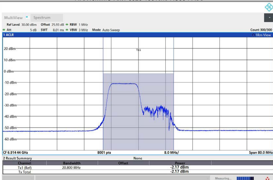
11AX40MIMO-Ant2-6925-106Tone-RU53-PASS
