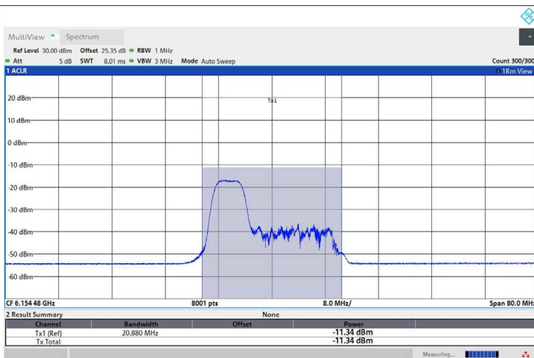
11AX40MIMO-Ant1-6165-52Tone-RU37-PASS
