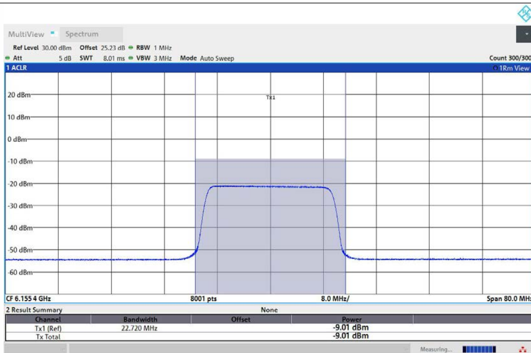
11AX40MIMO-Ant1-6165-242Tone-RU61-PASS
