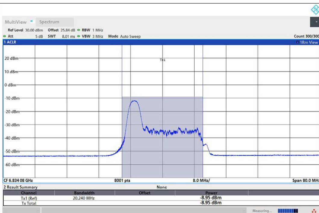
11AX40MIMO-Ant1-6845-26Tone-RU0-PASS
