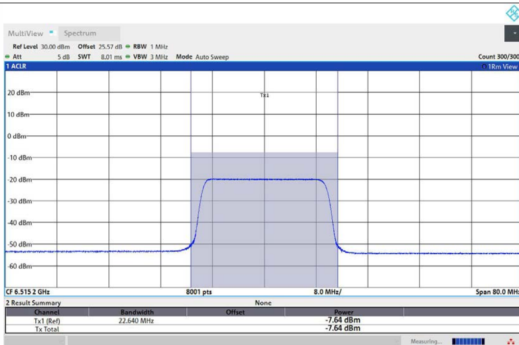
11AX40MIMO-Ant1-6525-242Tone-RU61-PASS
