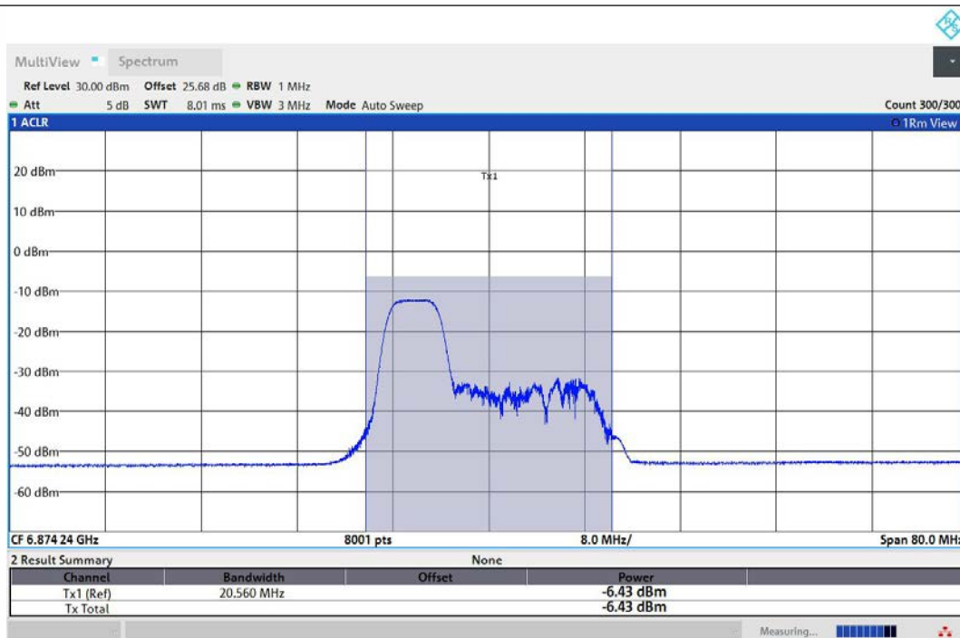
11AX40MIMO-Ant1-6885-52Tone-RU37-PASS
