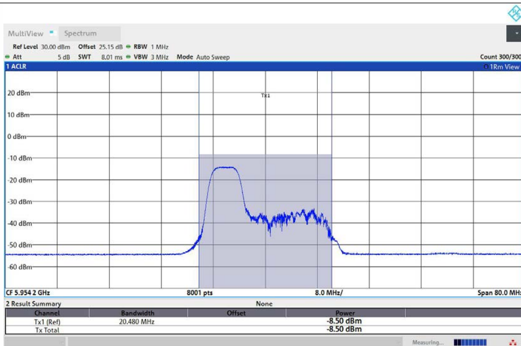
11AX40MIMO-Ant1-5965-52Tone-RU37-PASS
