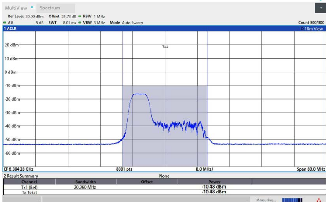
11AX40MIMO-Ant2-6405-52Tone-RU37-PASS
