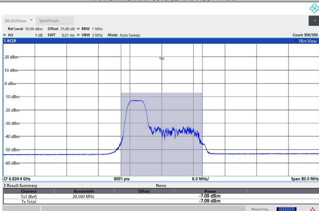
11AX40MIMO-Ant2-6845-52Tone-RU37-PASS
