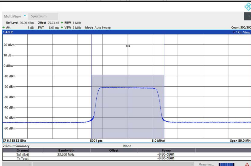
11AX40MIMO-Ant2-6165-242Tone-RU61-PASS
