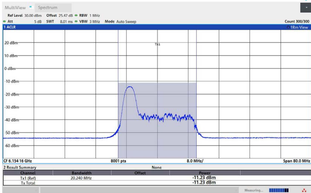
11AX40MIMO-Ant2-6165-26Tone-RU0-PASS
