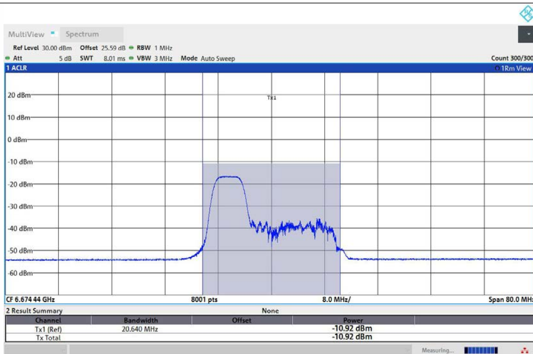
11AX40MIMO-Ant1-6685-52Tone-RU37-PASS
