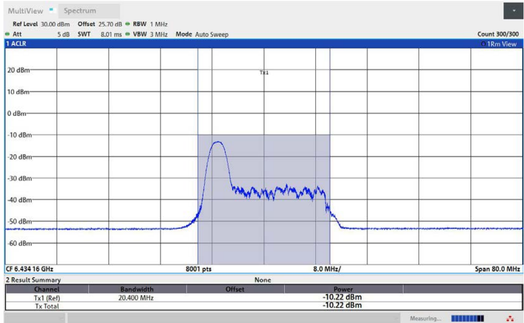
11AX40MIMO-Ant2-6445-26Tone-RU0-PASS
