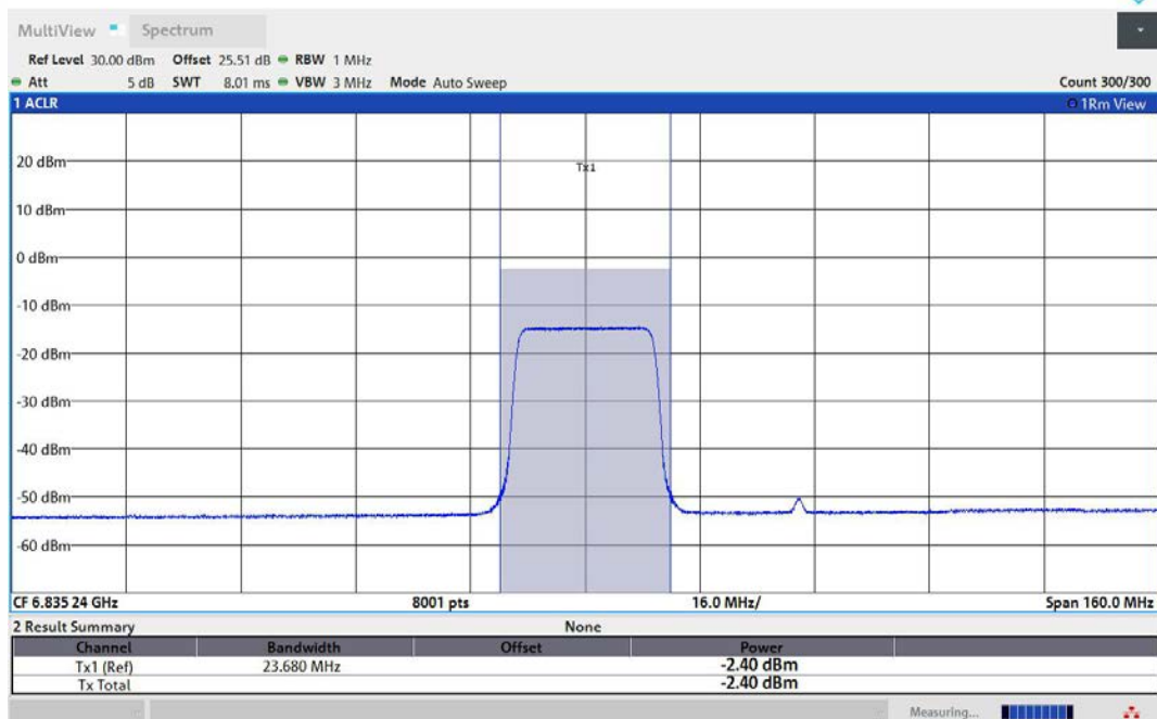
11AX80MIMO-Ant2-6865-242Tone-RU61-PASS
