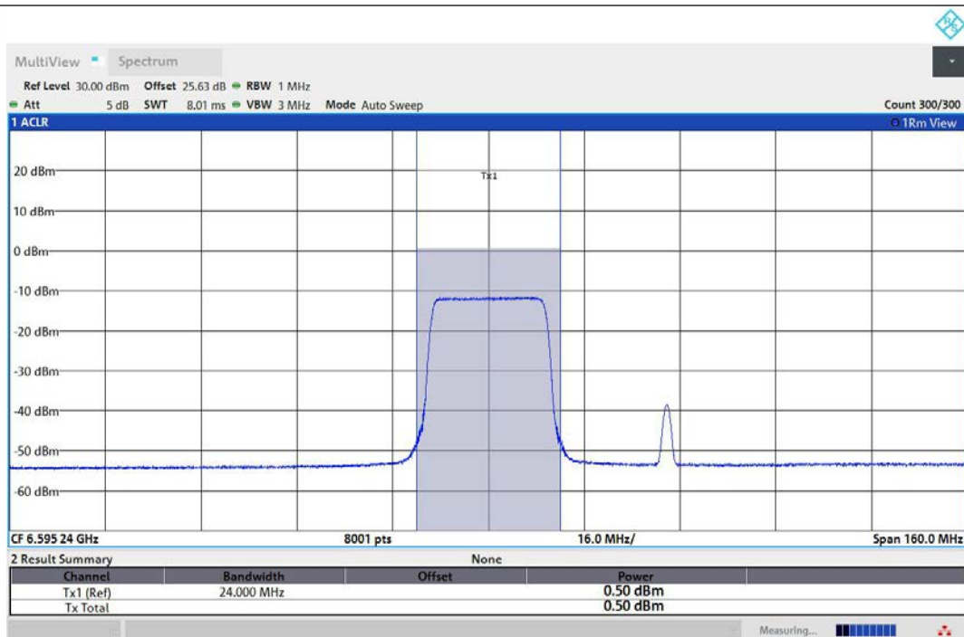
11AX80MIMO-Ant1-6625-242Tone-RU61-PASS
