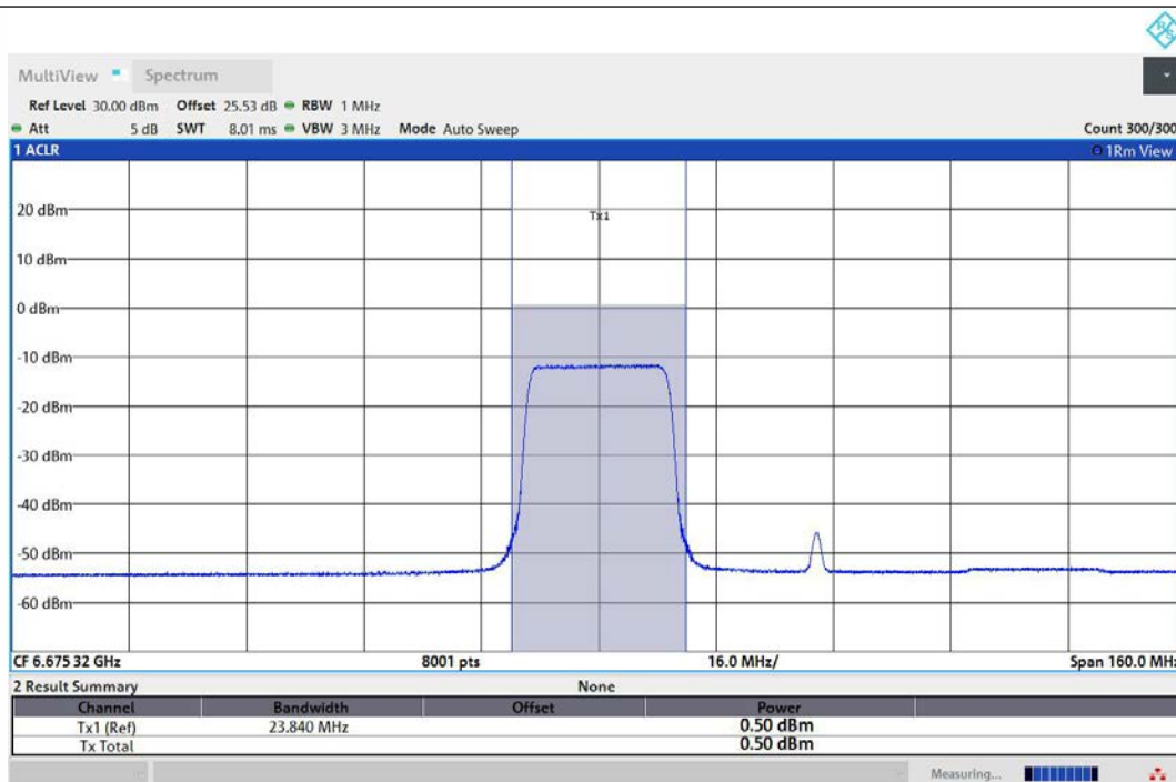
11AX80MIMO-Ant1-6705-242Tone-RU61-PASS
