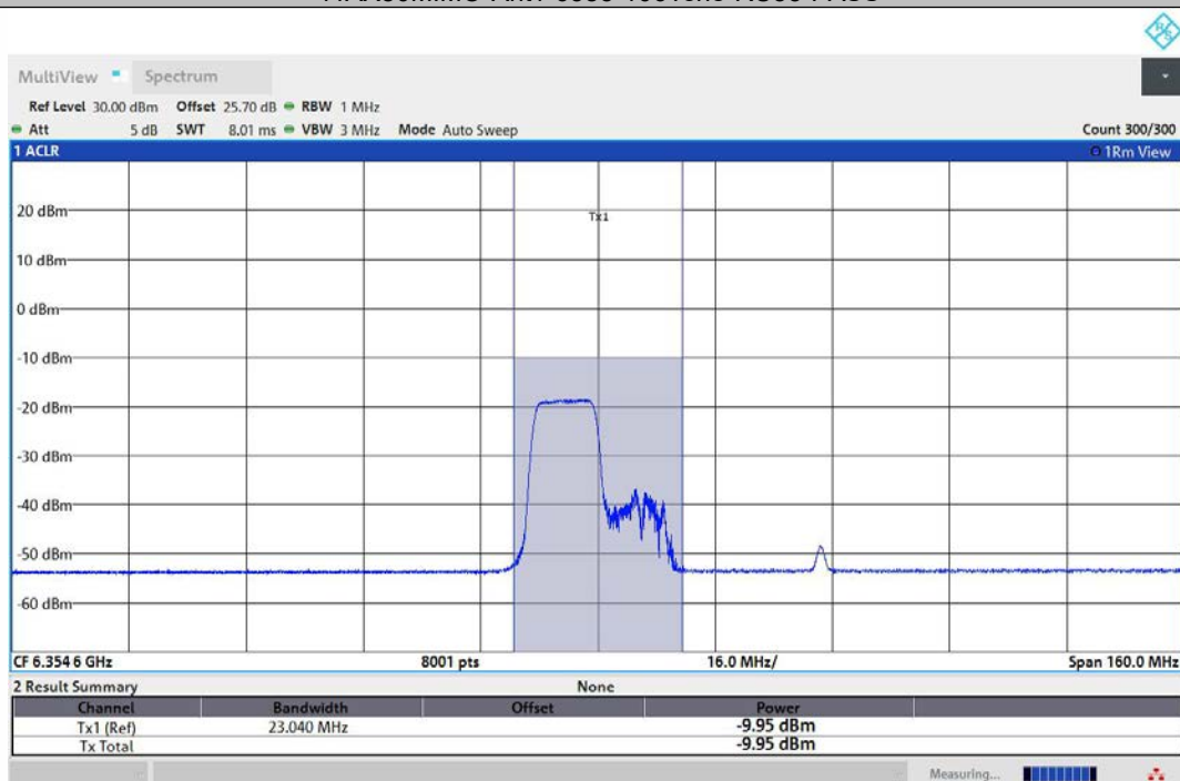
11AX80MIMO-Ant2-6385-106Tone-RU53-PASS
