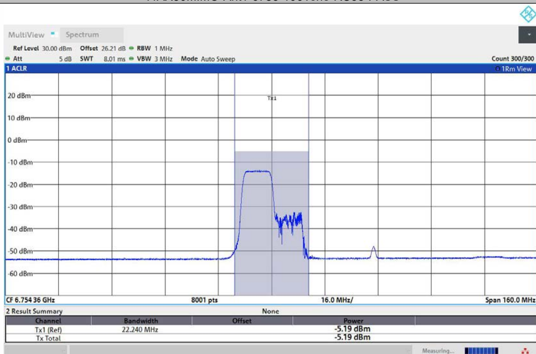
11AX80MIMO-Ant2-6785-106Tone-RU53-PASS
