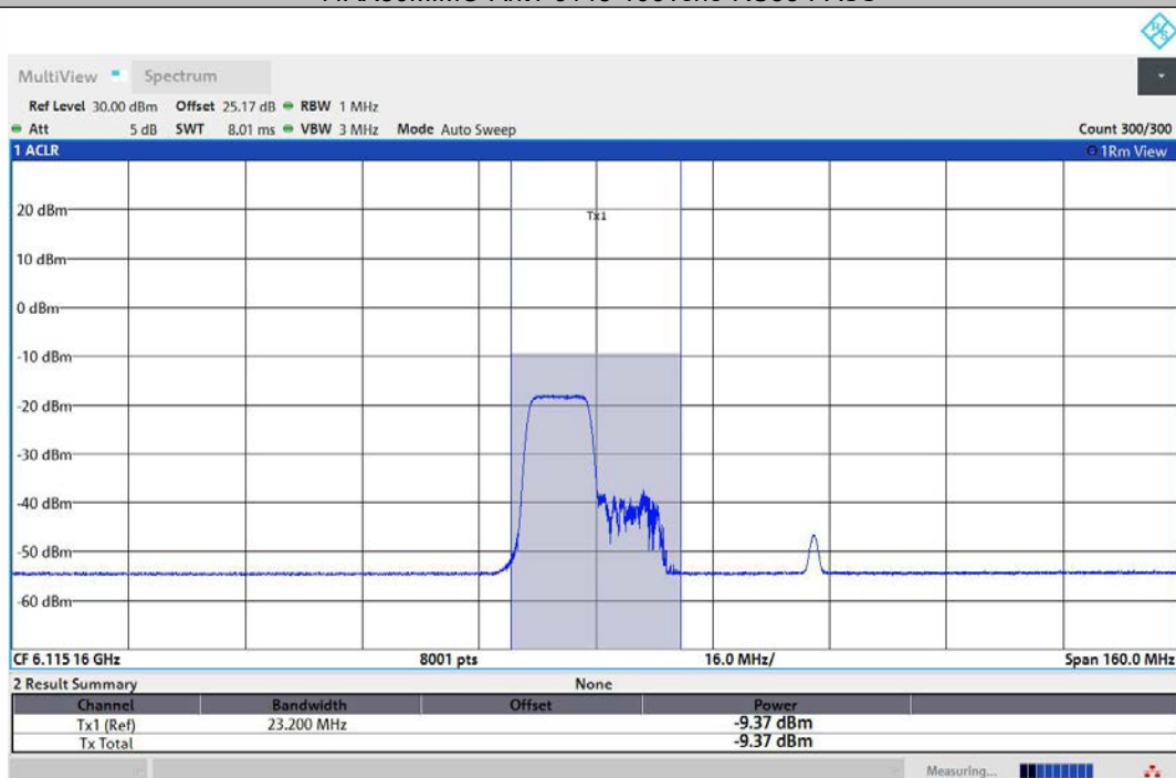
11AX80MIMO-Ant2-6145-106Tone-RU53-PASS
