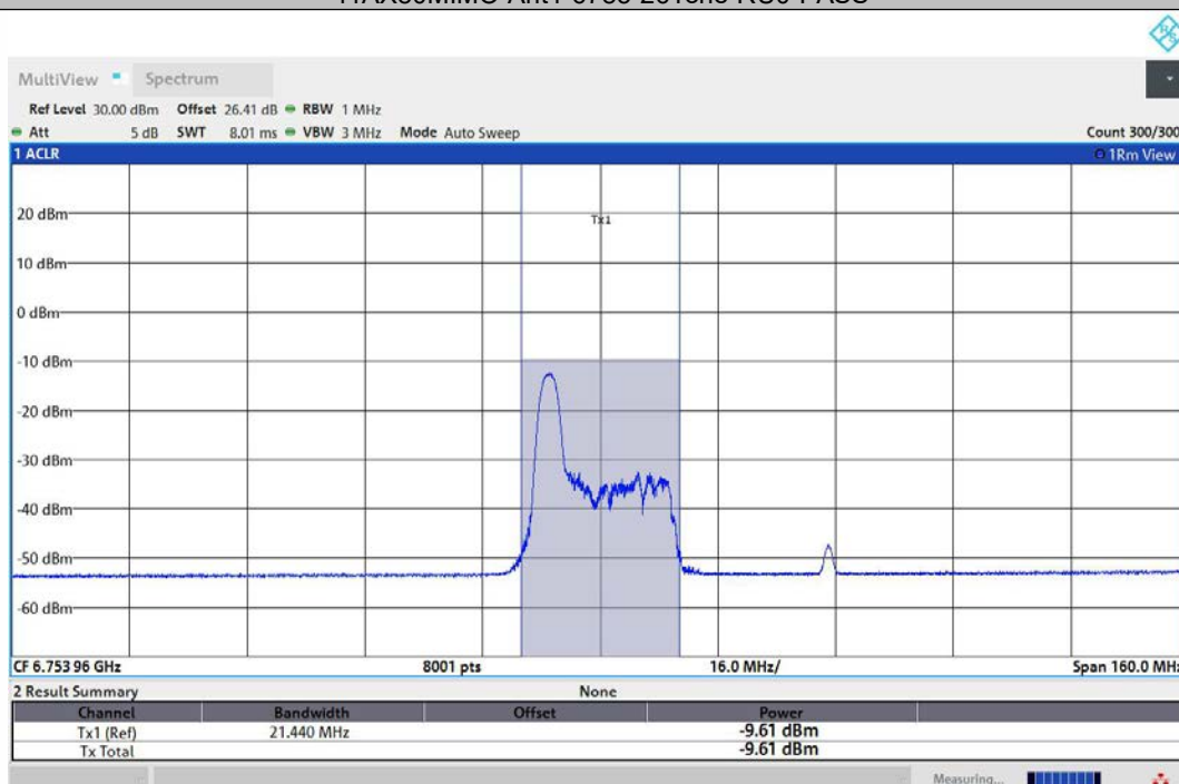
11AX80MIMO-Ant2-6785-26Tone-RU0-PASS
