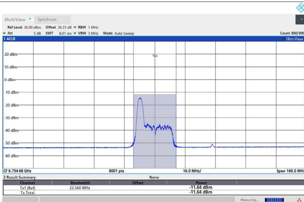
11AX80MIMO-Ant1-6785-26Tone-RU0-PASS
