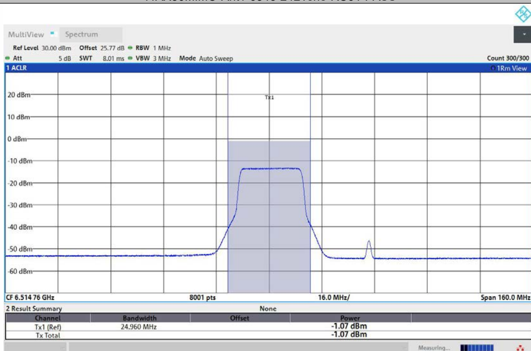
11AX80MIMO-Ant2-6545-242Tone-RU61-PASS
