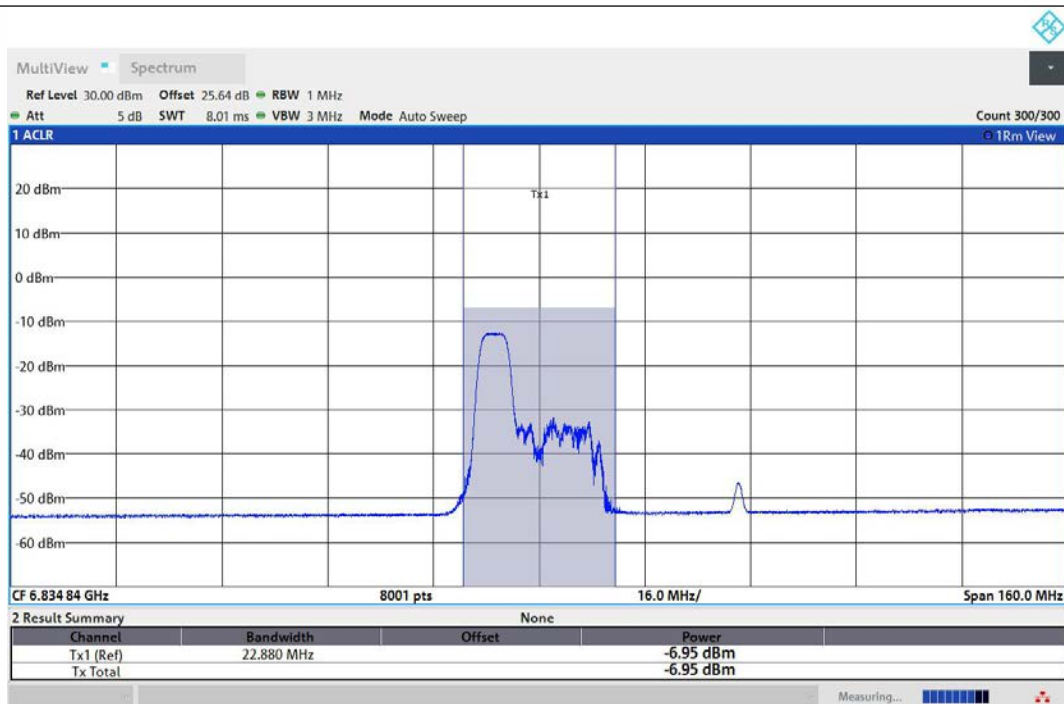
11AX80MIMO-Ant1-6865-52Tone-RU37-PASS
