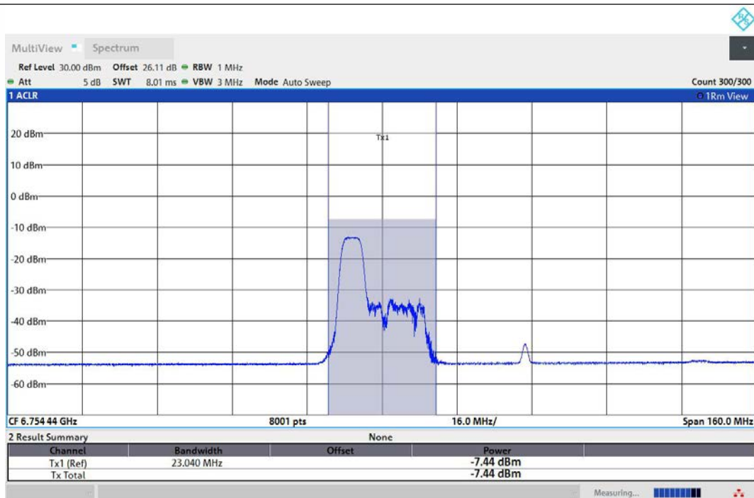
11AX80MIMO-Ant1-6785-52Tone-RU37-PASS
