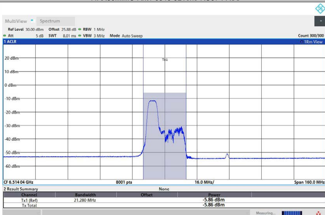
11AX80MIMO-Ant2-6545-52Tone-RU37-PASS
