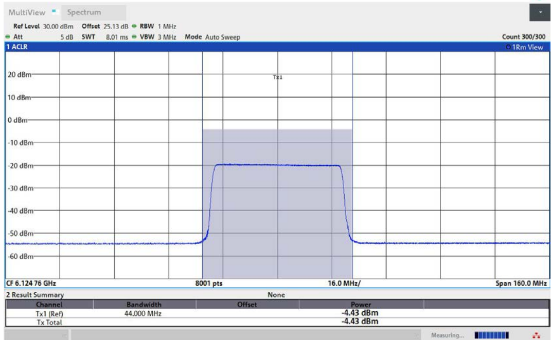
11AX80MIMO-Ant2-6145-484Tone-RU65-PASS
