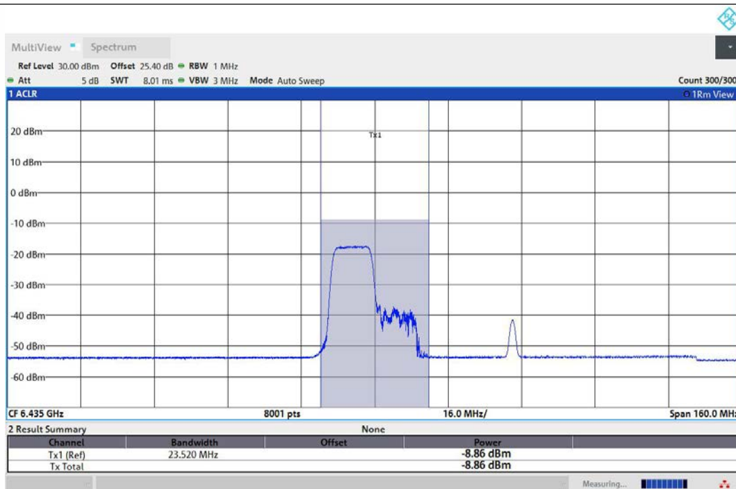
11AX80MIMO-Ant1-6465-106Tone-RU53-PASS
