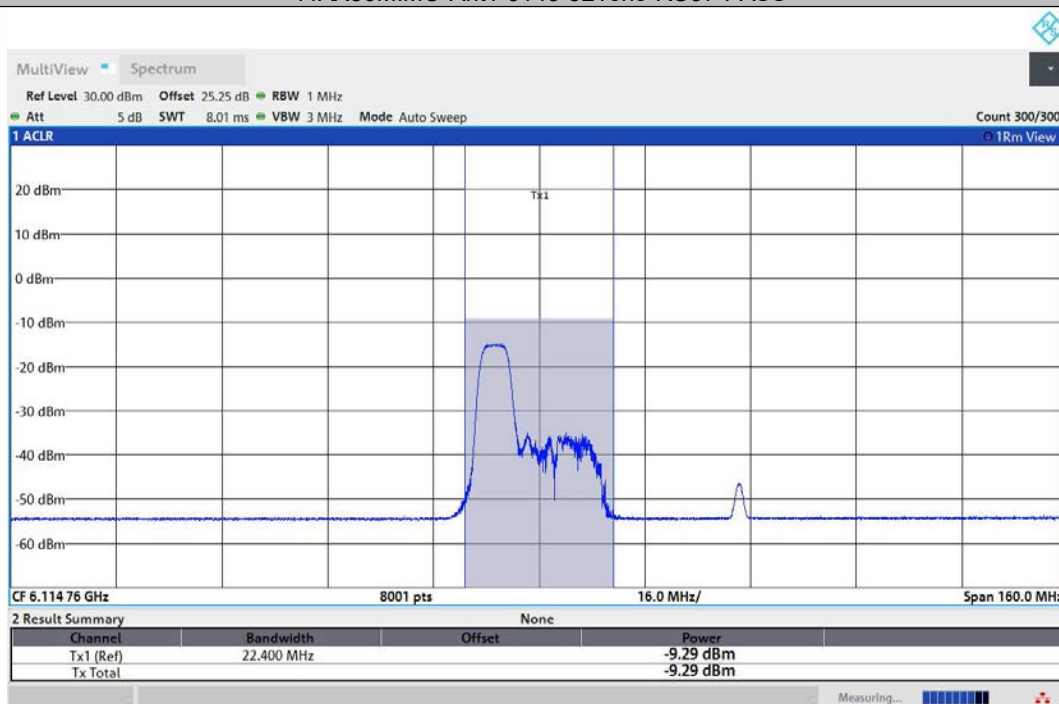
11AX80MIMO-Ant2-6145-52Tone-RU37-PASS
