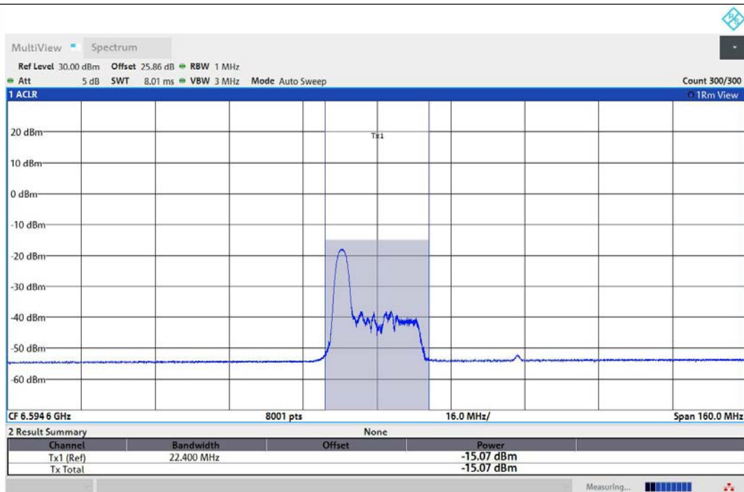
11AX80MIMO-Ant1-6625-26Tone-RU0-PASS
