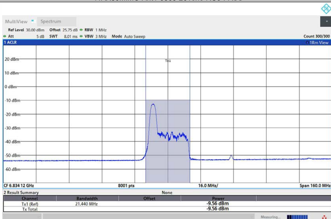
11AX80MIMO-Ant2-6865-26Tone-RU0-PASS
