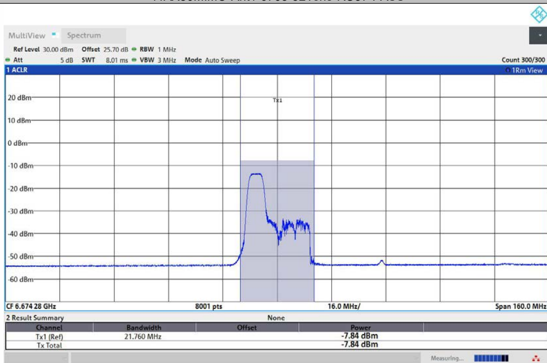
11AX80MIMO-Ant2-6705-52Tone-RU37-PASS
