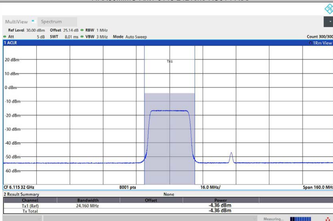
11AX80MIMO-Ant2-6145-242Tone-RU61-PASS
