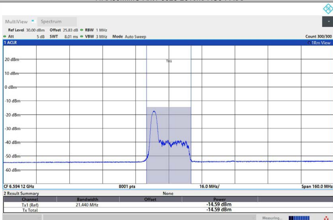
11AX80MIMO-Ant2-6625-26Tone-RU0-PASS
