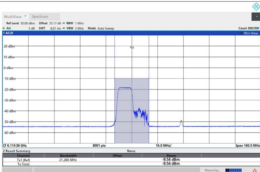
11AX80MIMO-Ant1-6145-106Tone-RU53-PASS
