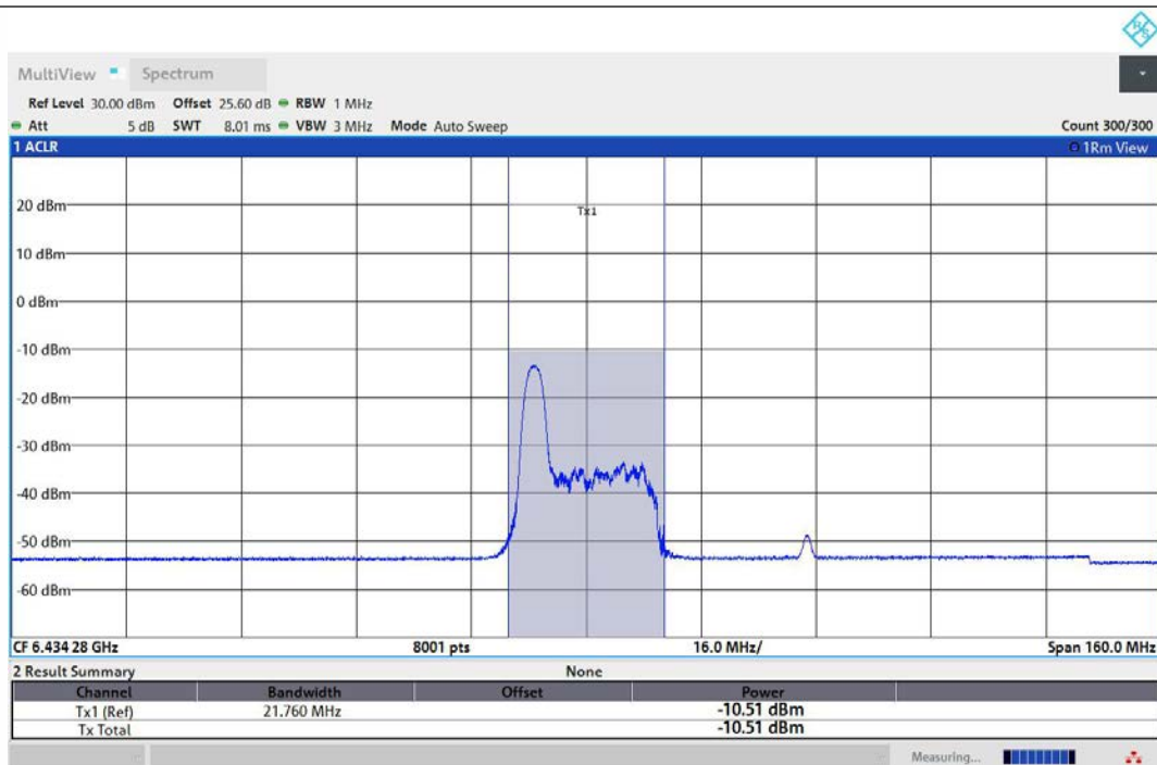
11AX80MIMO-Ant1-6465-26Tone-RU0-PASS
