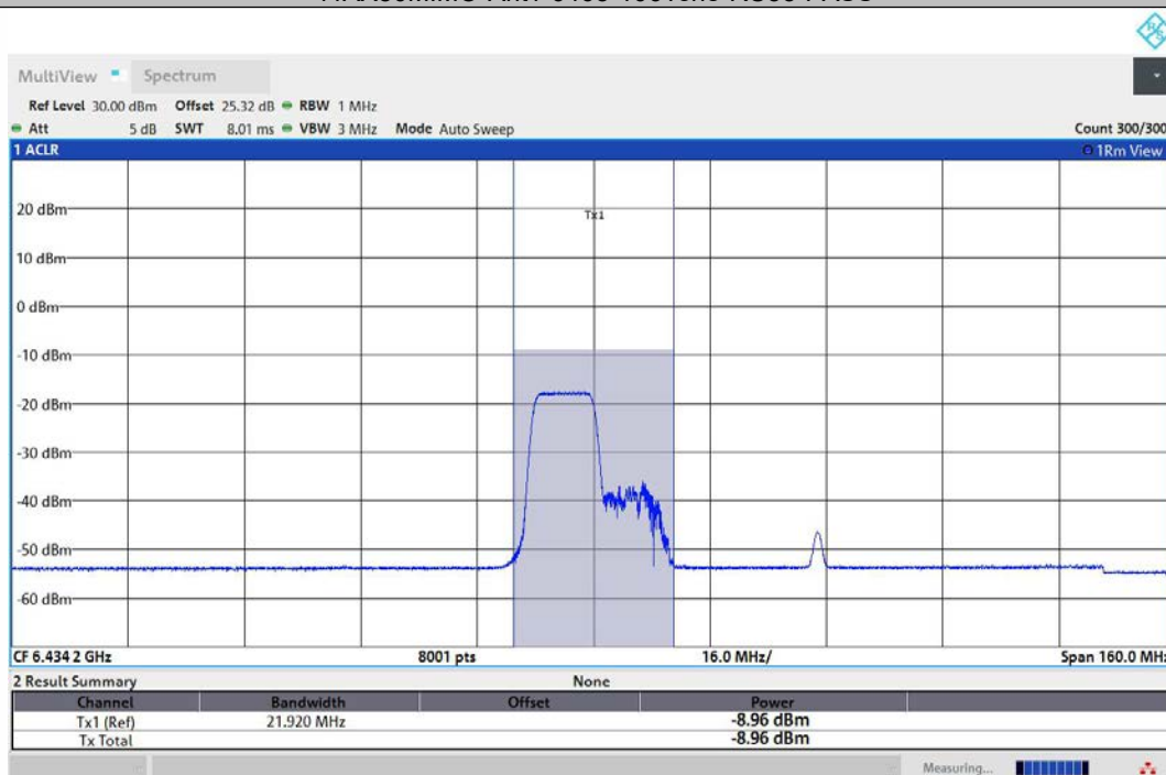
11AX80MIMO-Ant2-6465-106Tone-RU53-PASS
