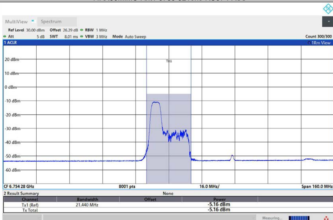
11AX80MIMO-Ant2-6785-52Tone-RU37-PASS
