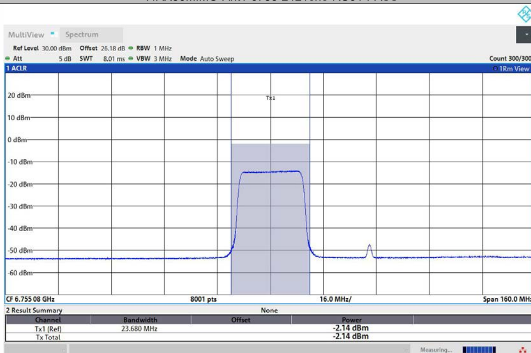
11AX80MIMO-Ant2-6785-242Tone-RU61-PASS
