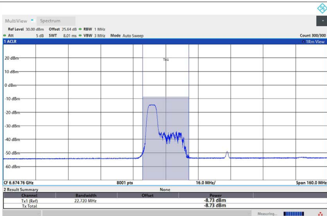
11AX80MIMO-Ant1-6705-52Tone-RU37-PASS
