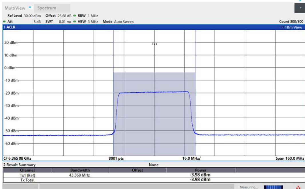
11AX80MIMO-Ant2-6385-484Tone-RU65-PASS
