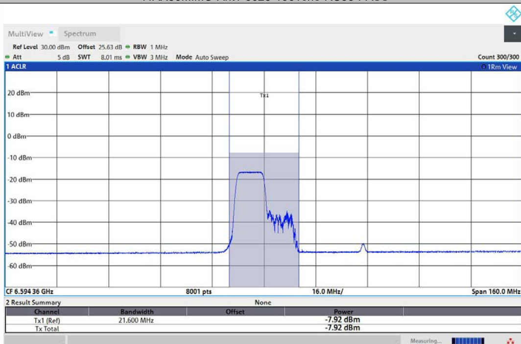
11AX80MIMO-Ant2-6625-106Tone-RU53-PASS
