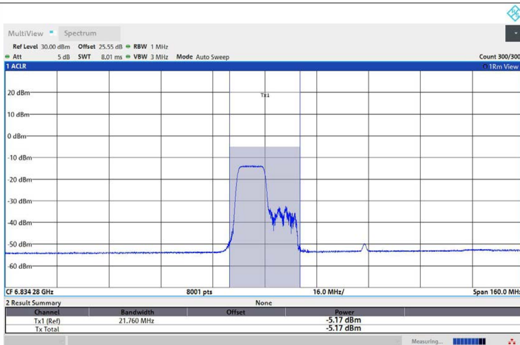
11AX80MIMO-Ant2-6865-106Tone-RU53-PASS
