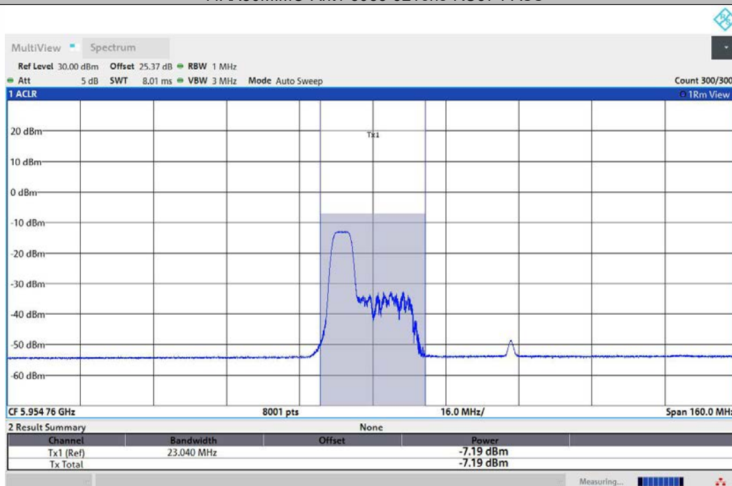
11AX80MIMO-Ant2-5985-52Tone-RU37-PASS
