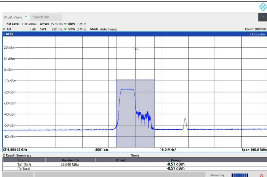
11AX80MIMO-Ant1-6625-106Tone-RU53-PASS
