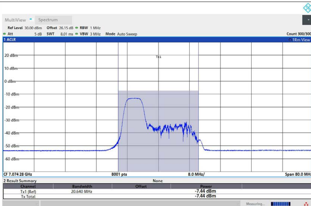
11AX40MIMO-Ant1-7085-52Tone-RU37-PASS
