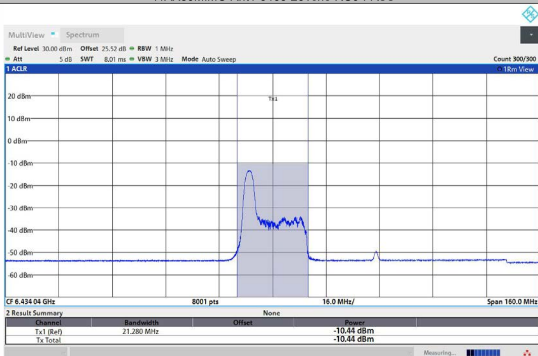
11AX80MIMO-Ant2-6465-26Tone-RU0-PASS
