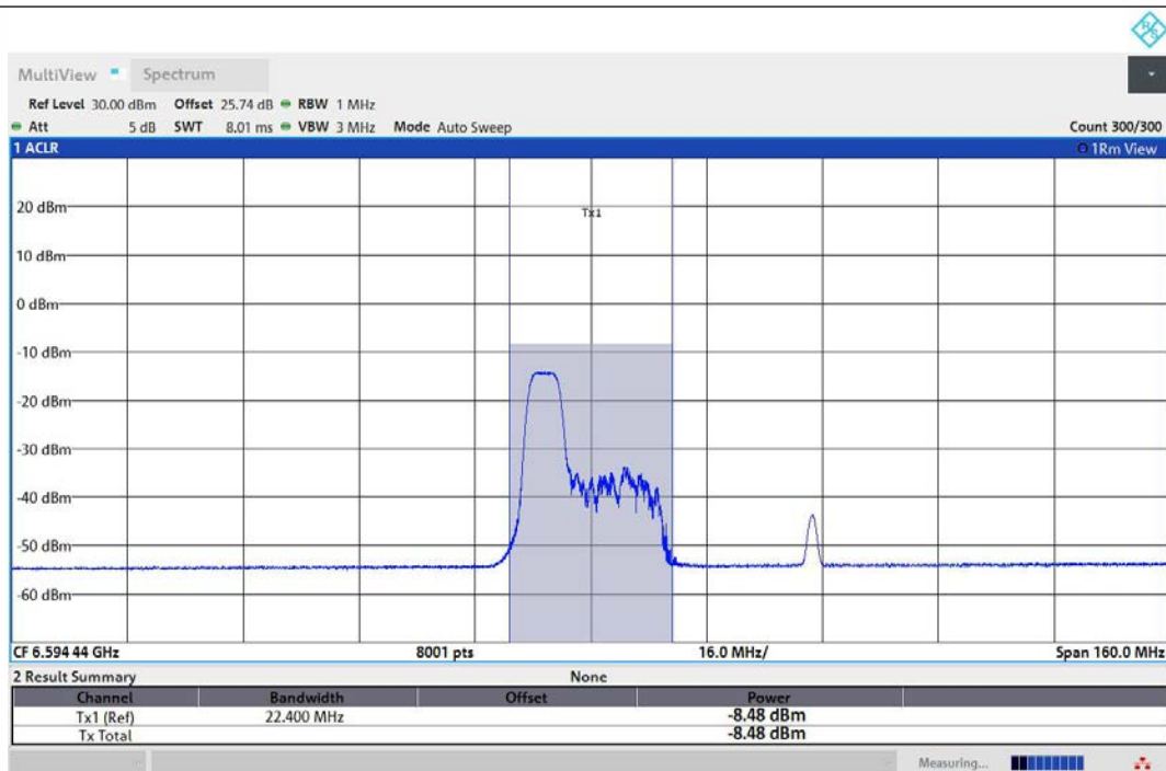
11AX80MIMO-Ant1-6625-52Tone-RU37-PASS
