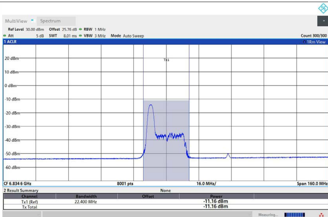
11AX80MIMO-Ant1-6865-26Tone-RU0-PASS
