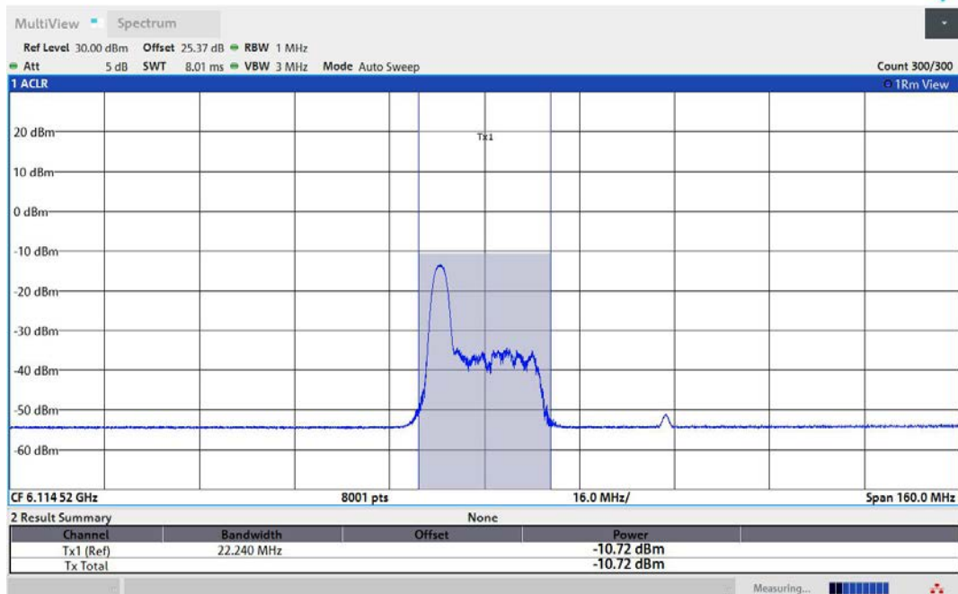
11AX80MIMO-Ant2-6145-26Tone-RU0-PASS
