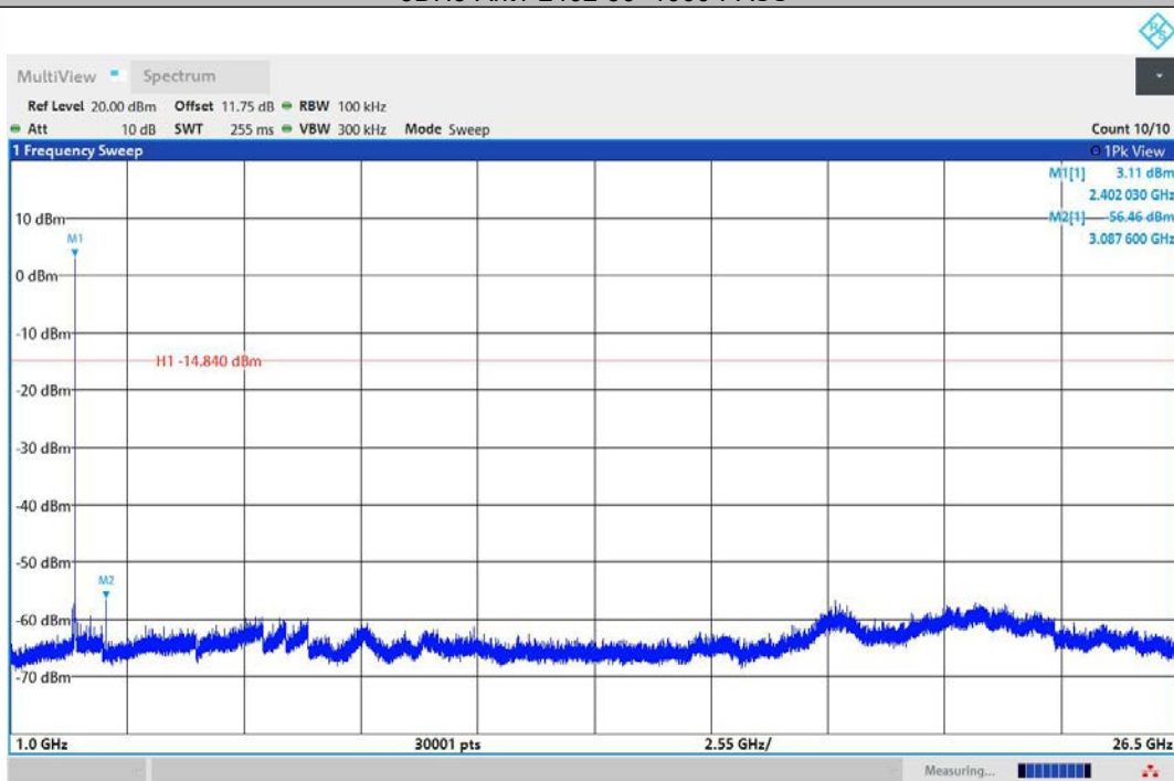
3DH5-Ant1-2402-1000~26500-PASS
