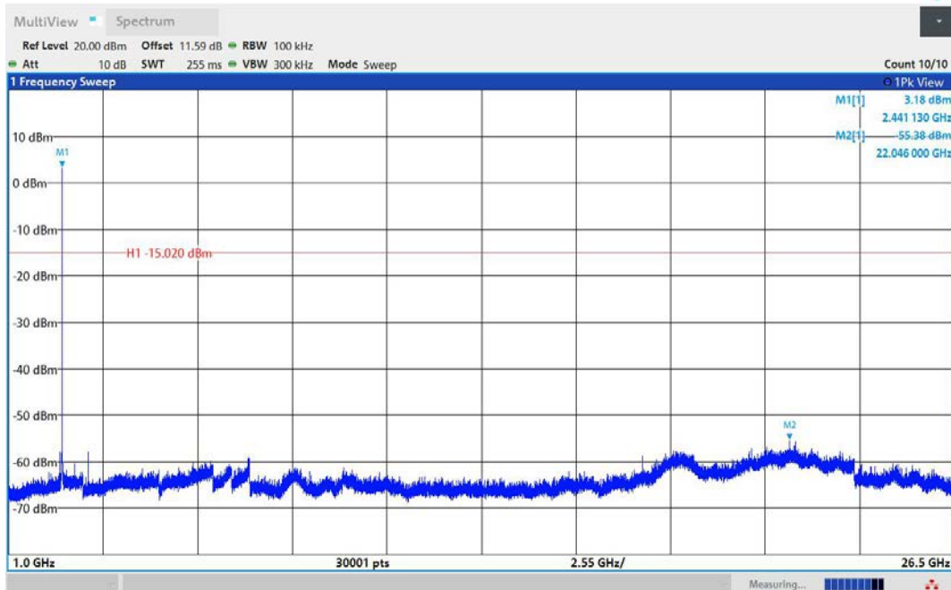
3DH5-Ant1-2441-1000~26500-PASS
