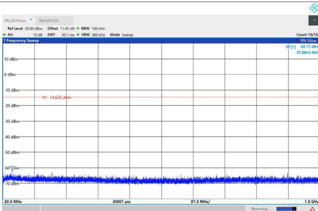
3DH5-Ant1-2480-30~1000-PASS
