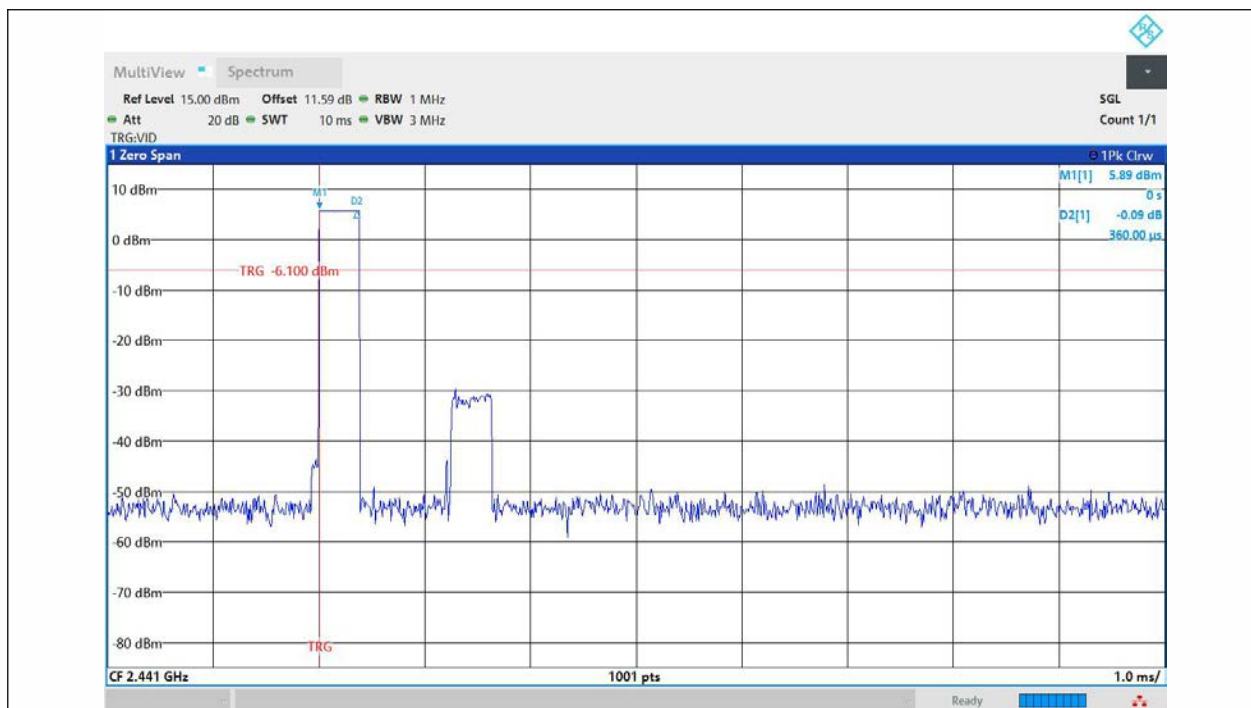
DH1-Ant1-Hop-PASS
