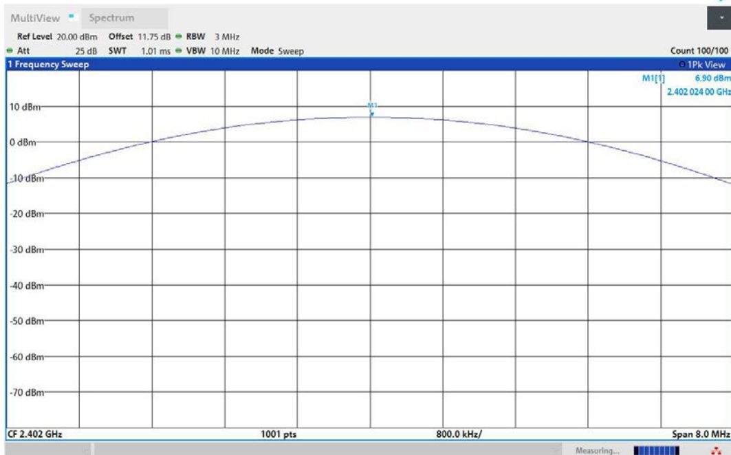
2DH5-Ant1-2402-PASS
