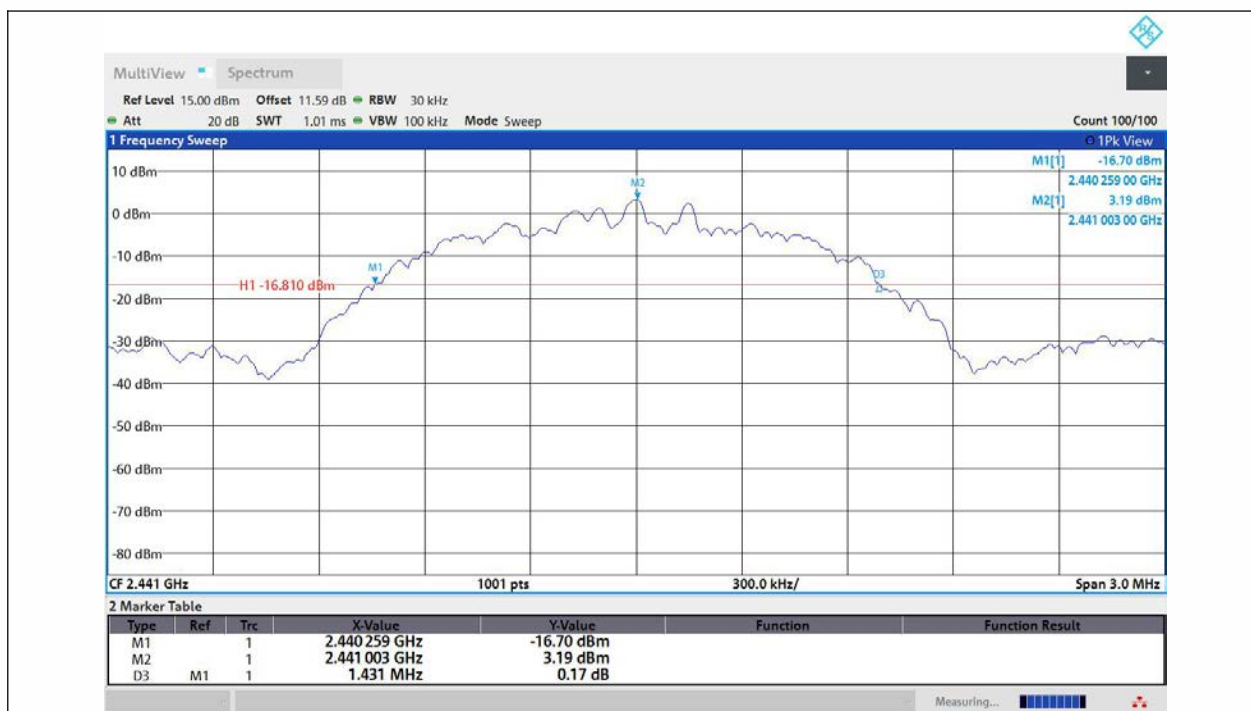
2DH5-Ant1-2441
