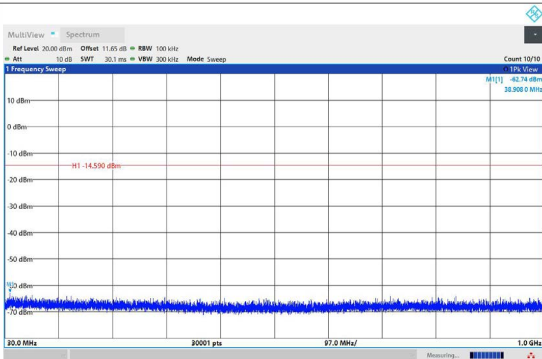
2DH5-Ant1-2480-30~1000-PASS
