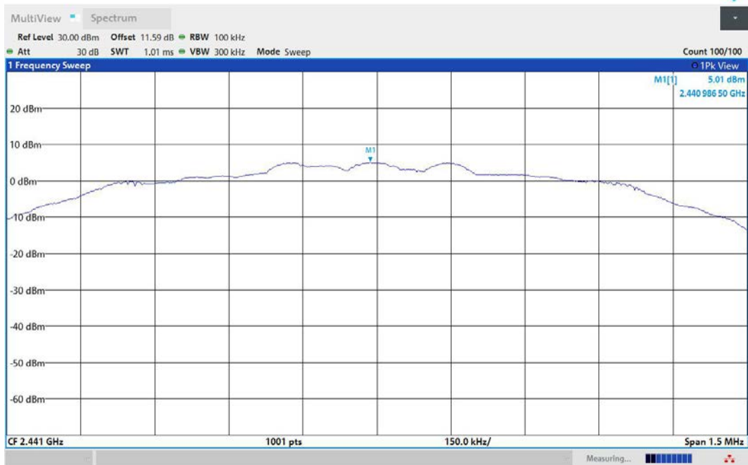
2DH5-Ant1-2441-PASS
