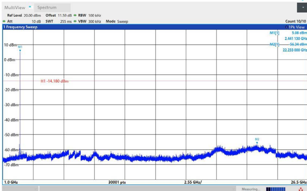
DH5-Ant1-2441-1000~26500-PASS
