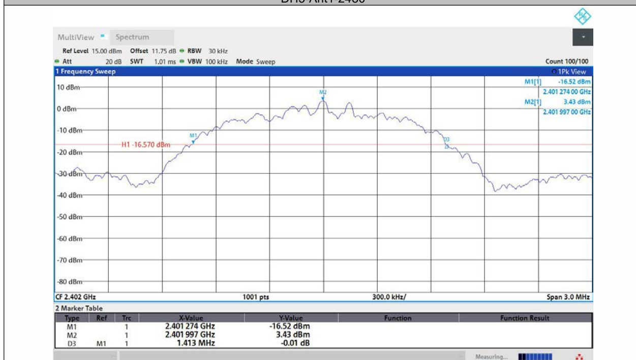
2DH5-Ant1-2402
