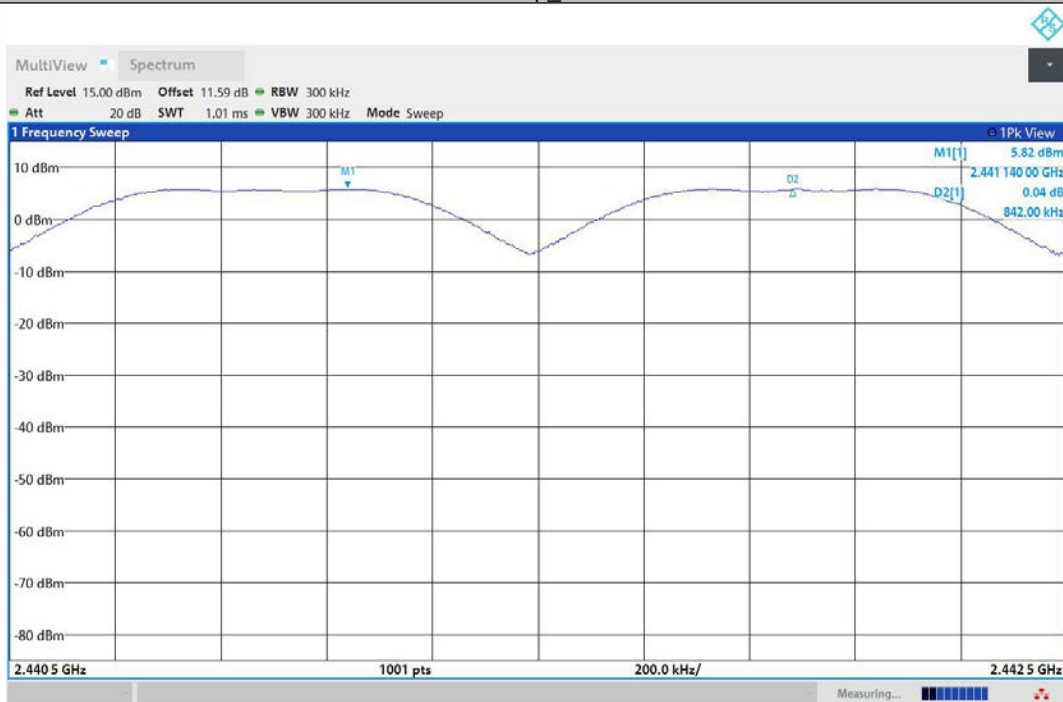
DH5-Ant1-Hop_2441-PASS
