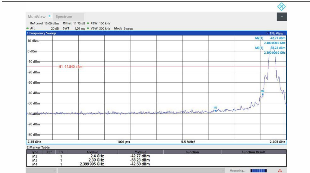
3DH5-Ant1-2402-PASS
