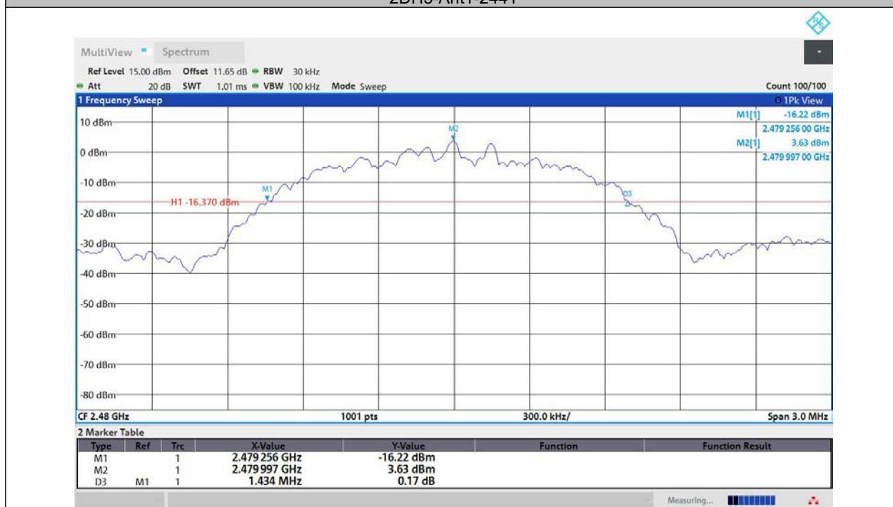
2DH5-Ant1-2480
