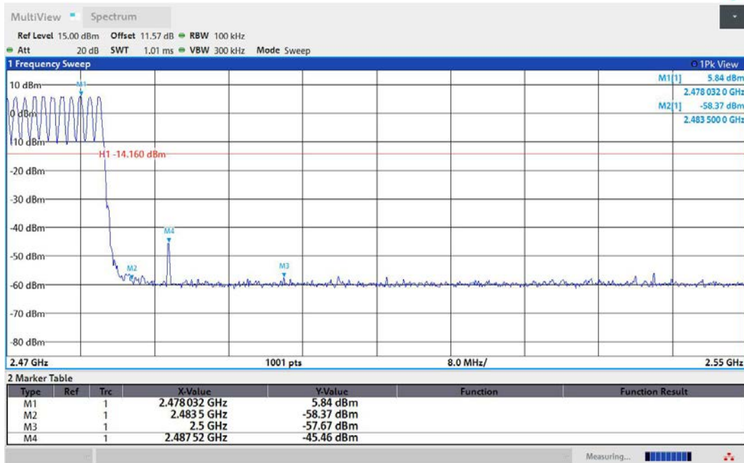
DH5-Ant1-Hop_2480-PASS
