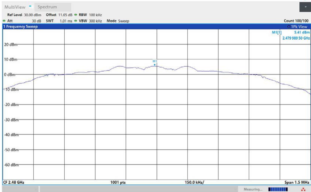
2DH5-Ant1-2480-PASS
