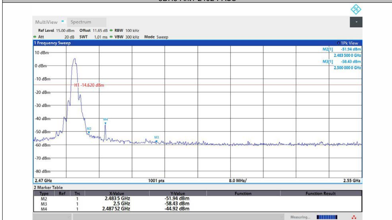
3DH5-Ant1-2480-PASS
