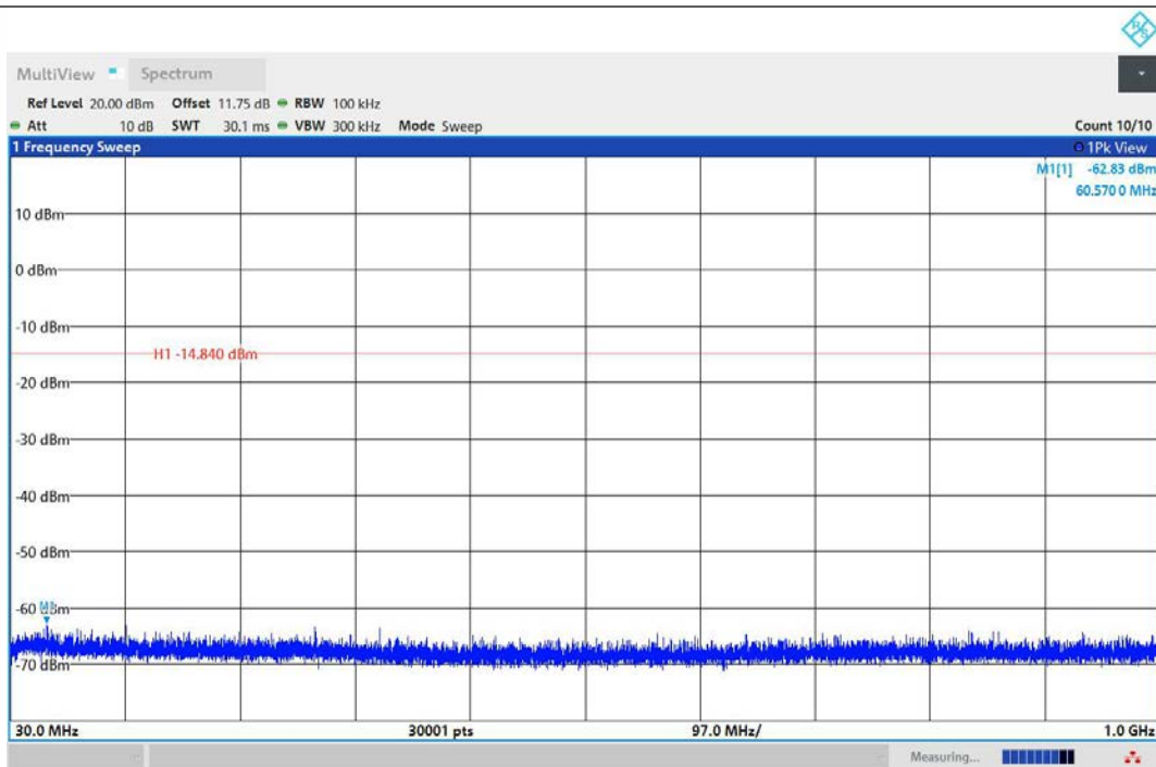
3DH5-Ant1-2402-30~1000-PASS
