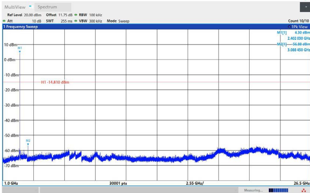
2DH5-Ant1-2402-1000~26500-PASS
