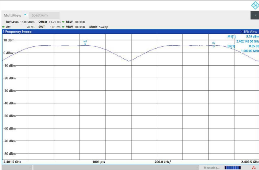
DH5-Ant1-Hop_2402-PASS
