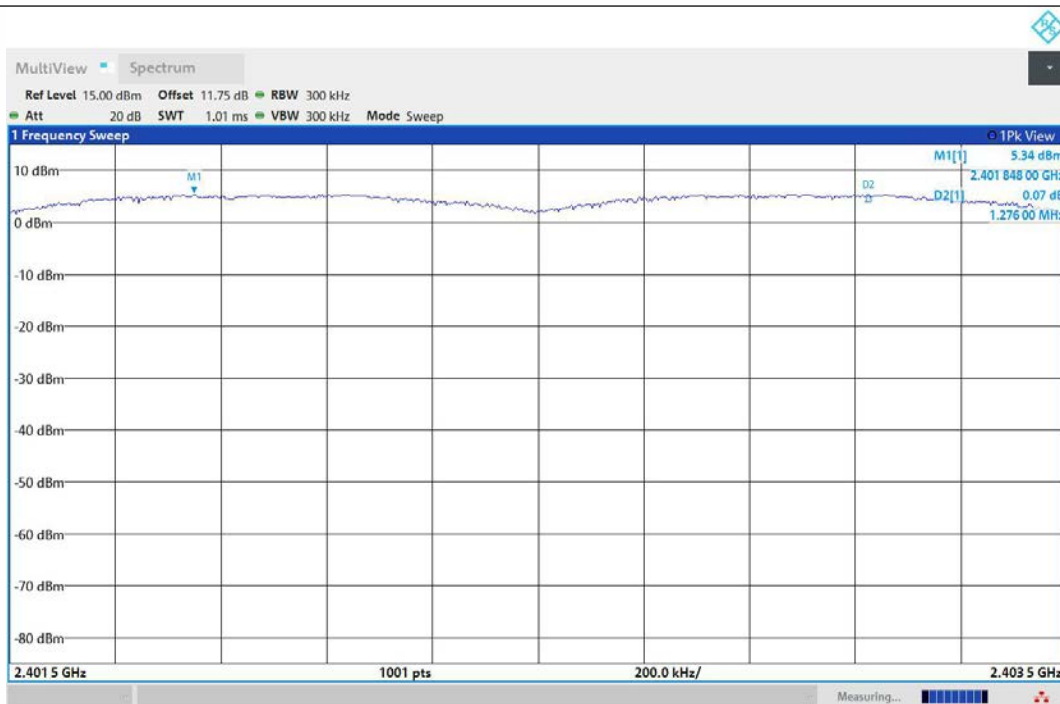
3DH5-Ant1-Hop_2402-PASS
