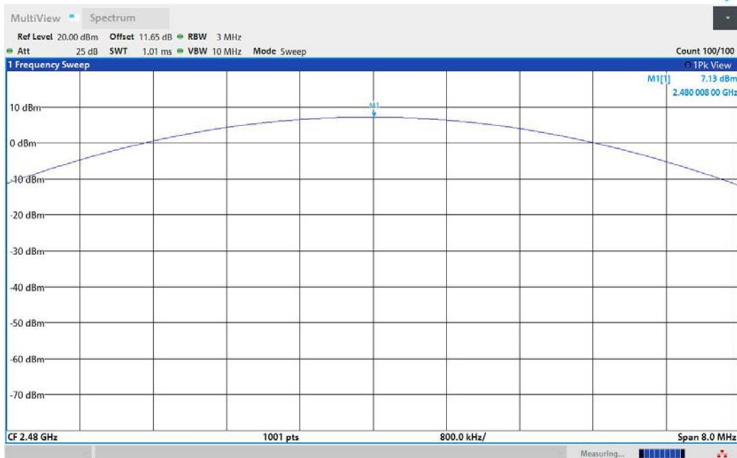
2DH5-Ant1-2480-PASS
