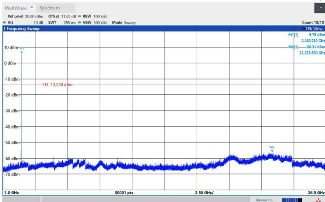
DH5-Ant1-2480-1000~26500-PASS
