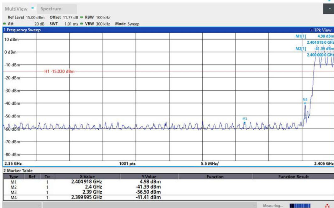
DH5-Ant1-Hop_2402-PASS
