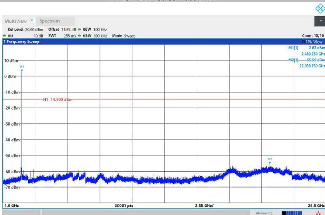
2DH5-Ant1-2480-1000~26500-PASS
