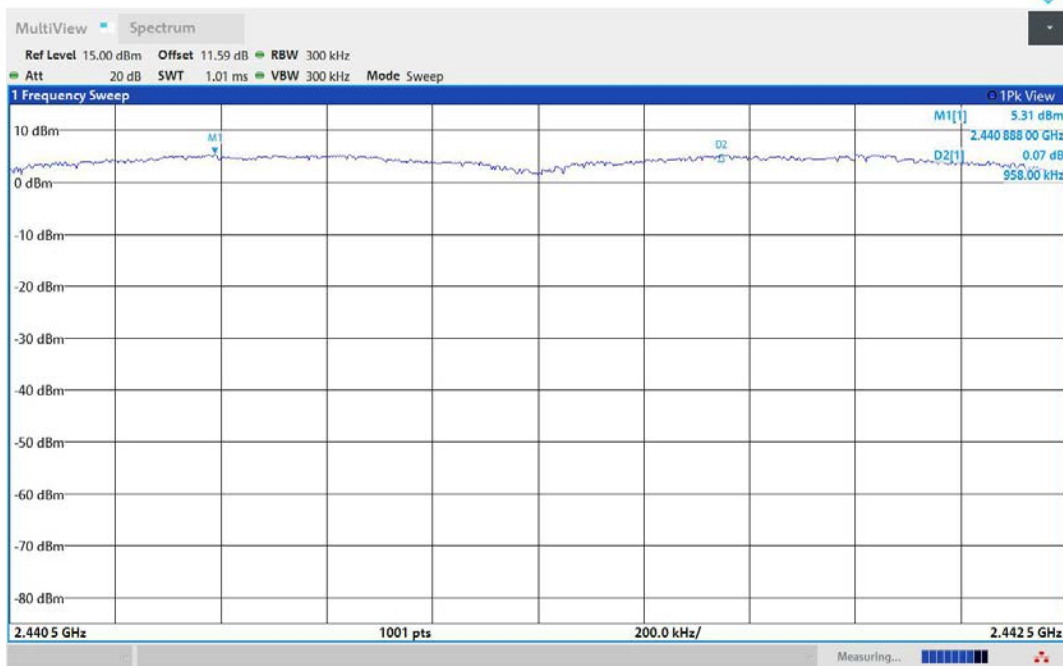
2DH5-Ant1-Hop_2441-PASS
