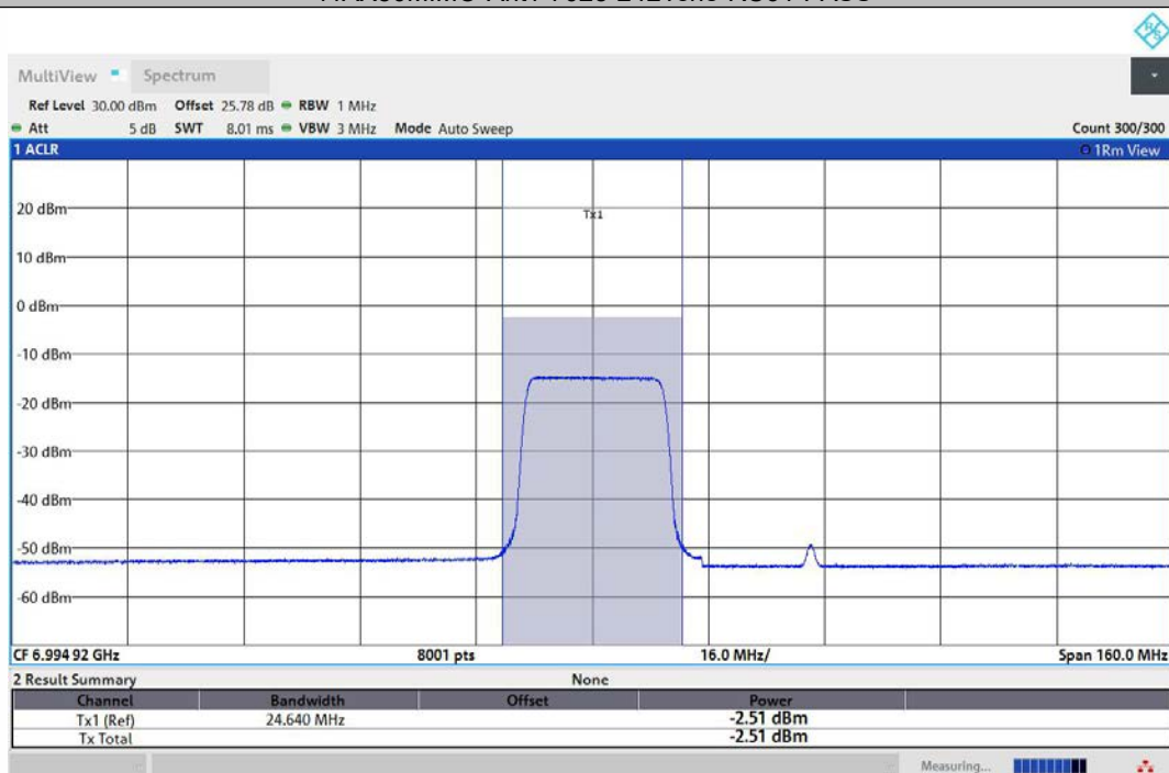
11AX80MIMO-Ant2-7025-242Tone-RU61-PASS
