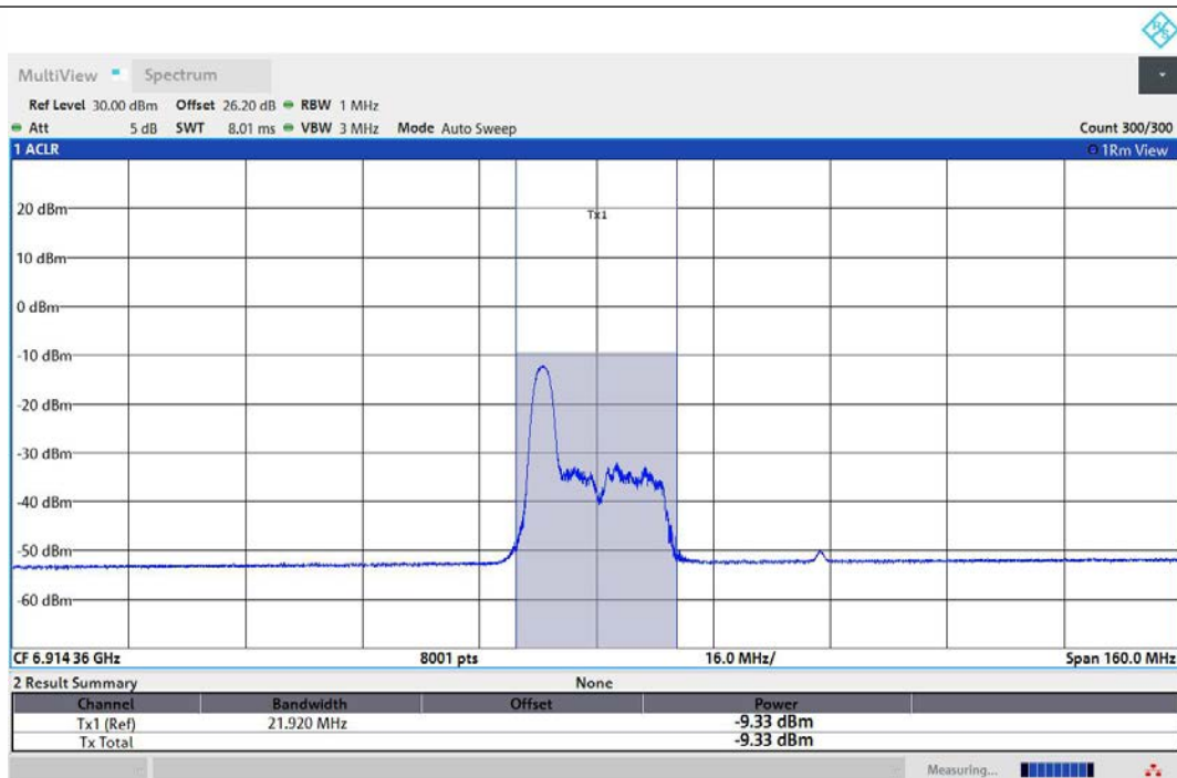
11AX80MIMO-Ant1-6945-26Tone-RU0-PASS
