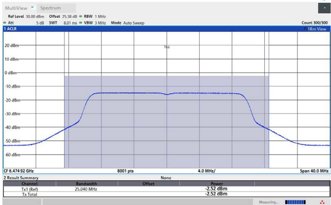
11AX20MIMO-Ant1-6475-PASS
