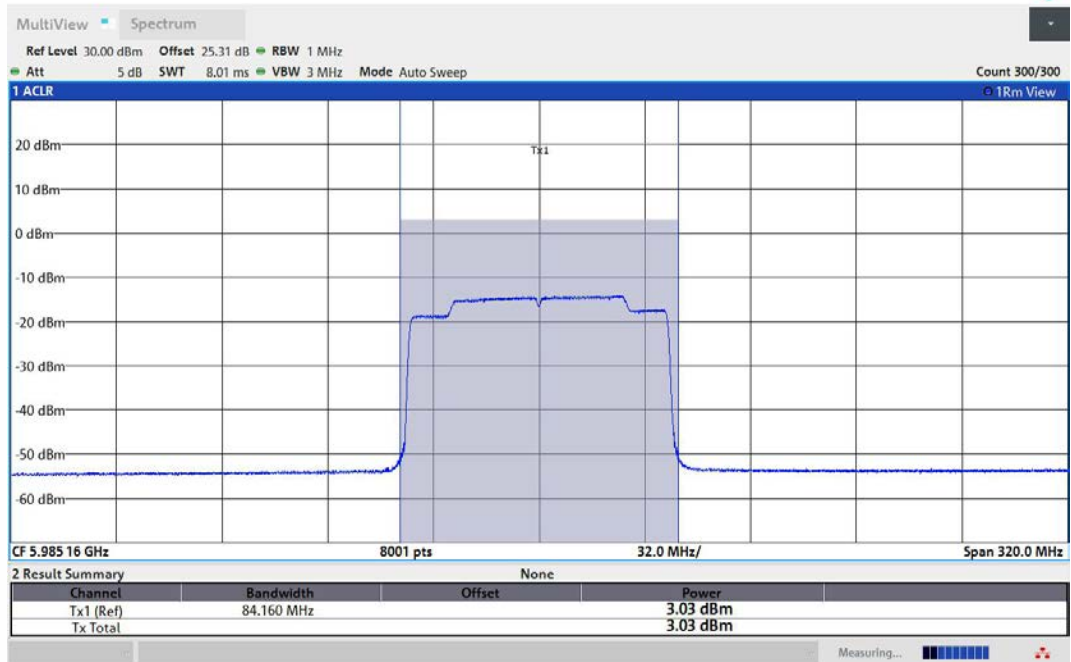
11AX160MIMO-Ant2-6025-996Tone-RU67-PASS
