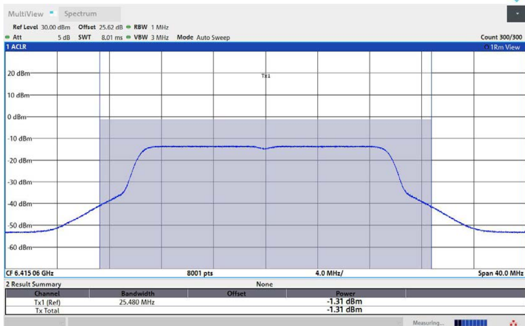
11AX20MIMO-Ant2-6415-PASS
