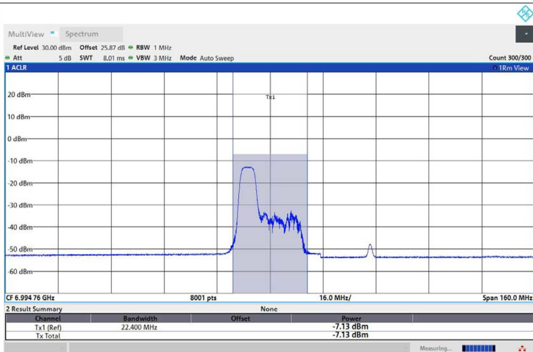
11AX80MIMO-Ant1-7025-52Tone-RU37-PASS
