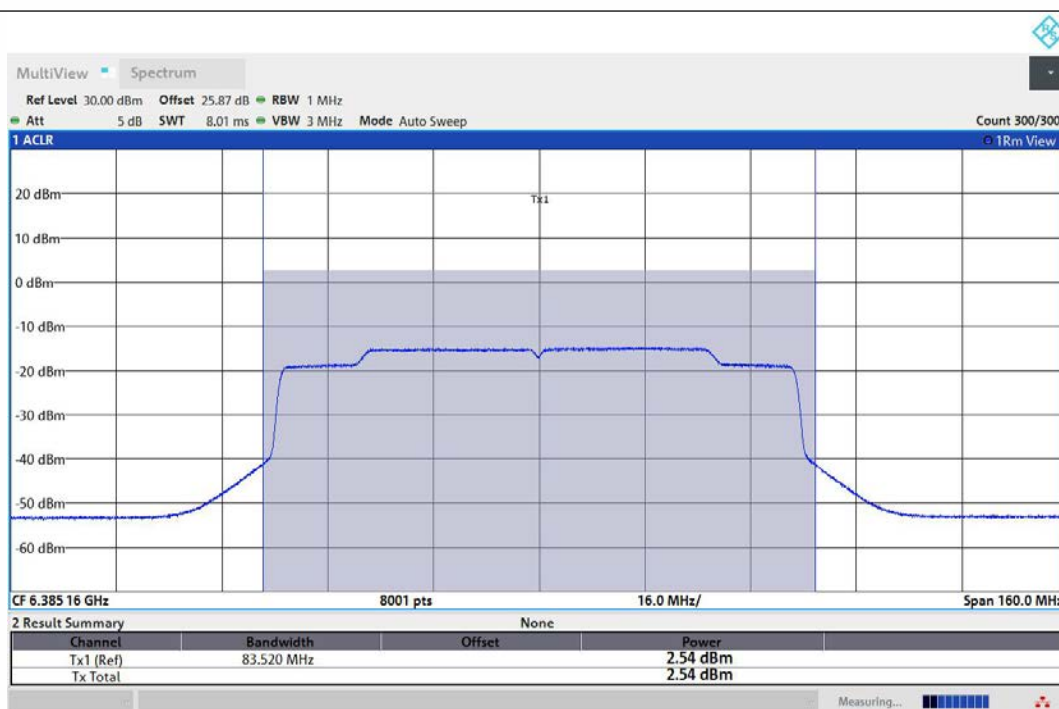
11AX80MIMO-Ant1-6385-PASS
