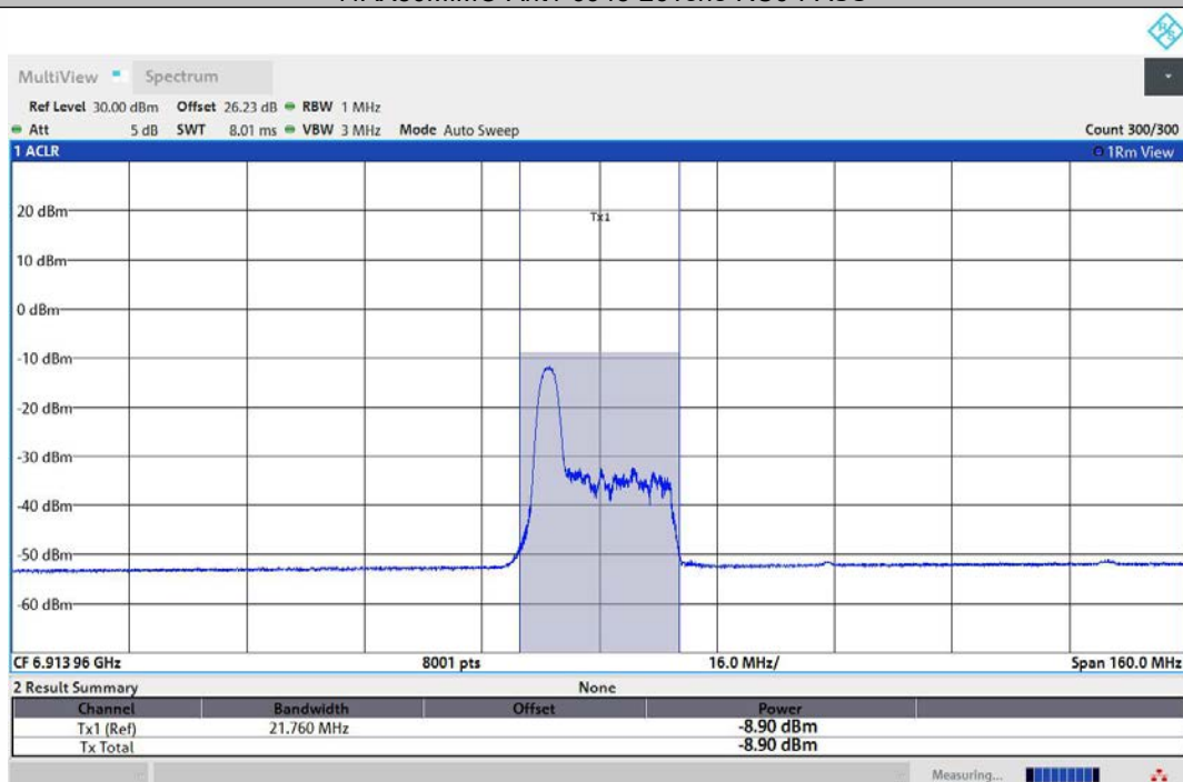
11AX80MIMO-Ant2-6945-26Tone-RU0-PASS
