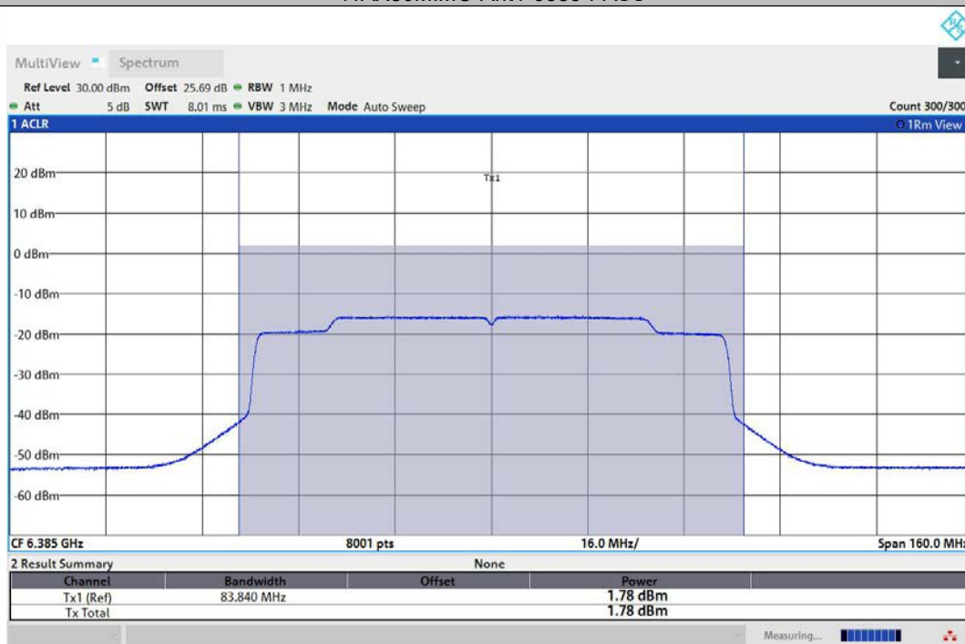
11AX80MIMO-Ant2-6385-PASS
