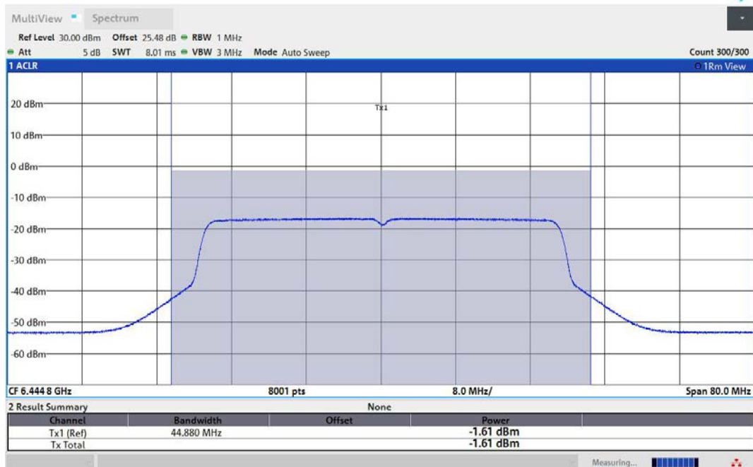
11AX40MIMO-Ant2-6445-PASS
