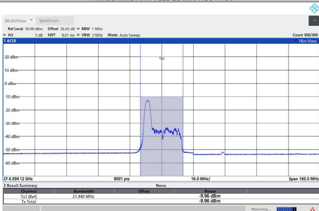
11AX80MIMO-Ant2-7025-26Tone-RU0-PASS
