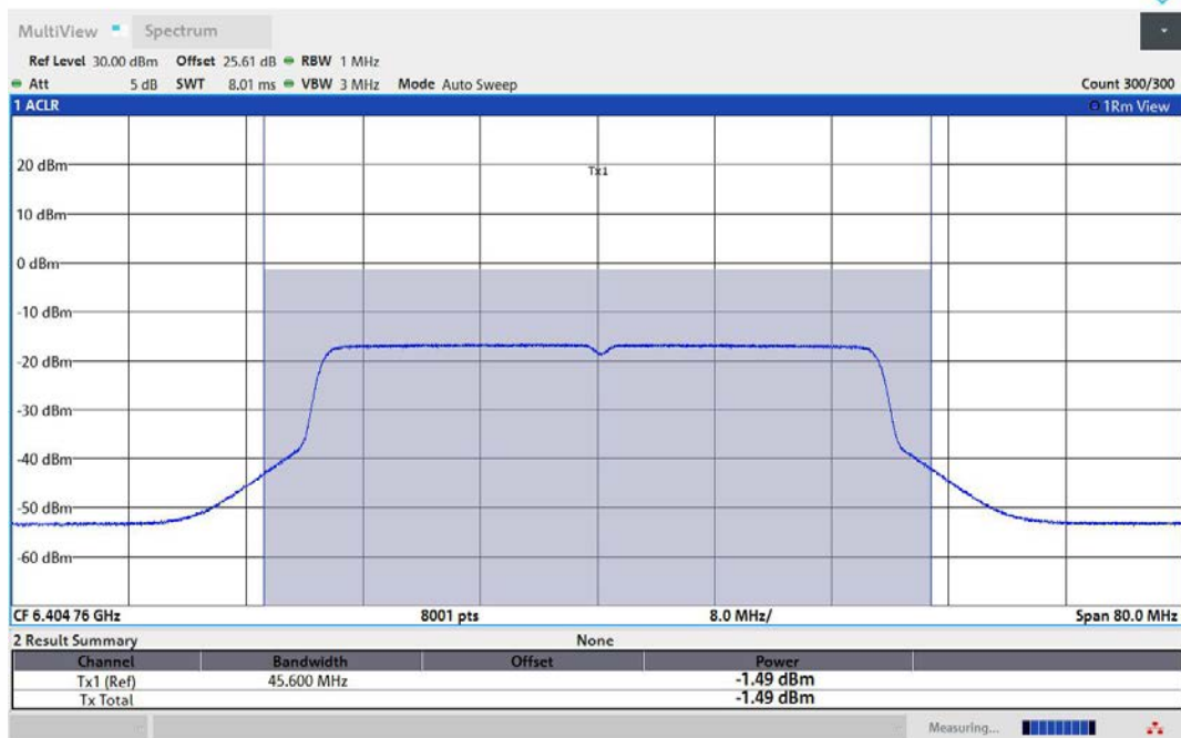
11AX40MIMO-Ant2-6405-PASS
