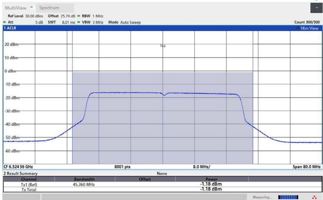
11AX40MIMO-Ant2-6525-PASS
