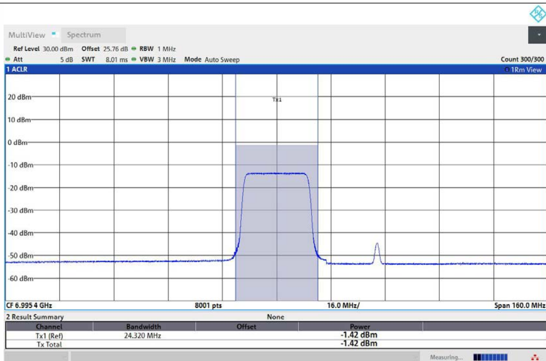
11AX80MIMO-Ant1-7025-242Tone-RU61-PASS
