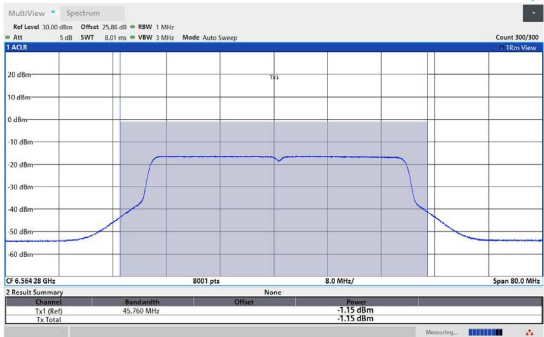
11AX40MIMO-Ant1-6565-PASS
