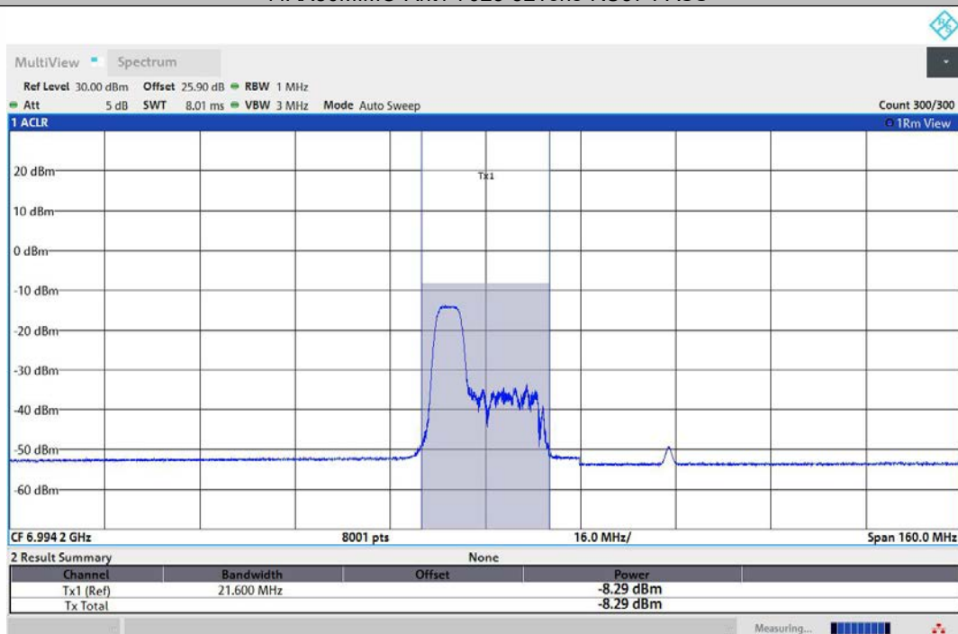
11AX80MIMO-Ant2-7025-52Tone-RU37-PASS
