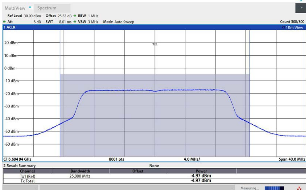
11AX20MIMO-Ant2-6695-PASS
