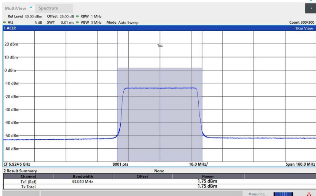
11AX80MIMO-Ant2-6945-484Tone-RU65-PASS
