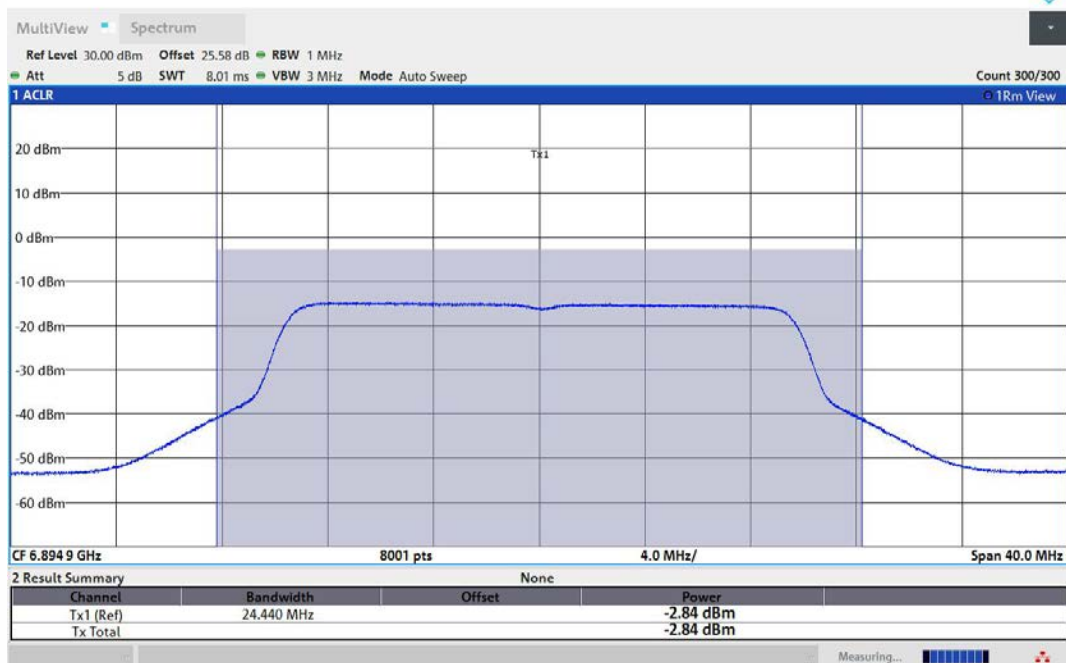
11AX20MIMO-Ant2-6895-PASS
