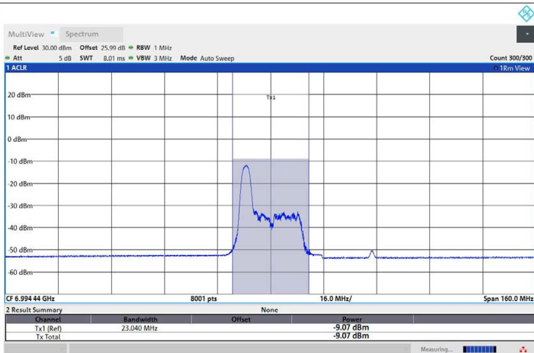
11AX80MIMO-Ant1-7025-26Tone-RU0-PASS
