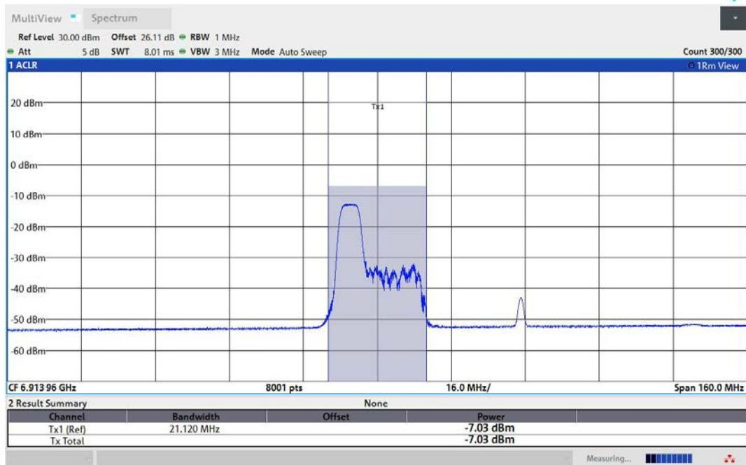
11AX80MIMO-Ant2-6945-52Tone-RU37-PASS
