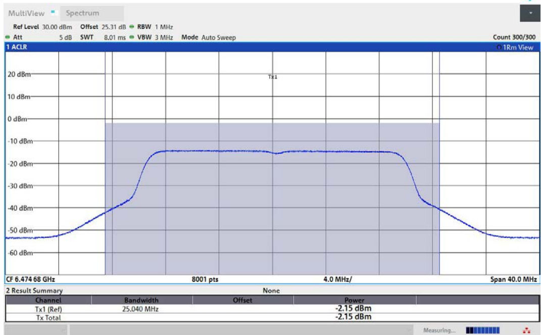
11AX20MIMO-Ant2-6475-PASS
