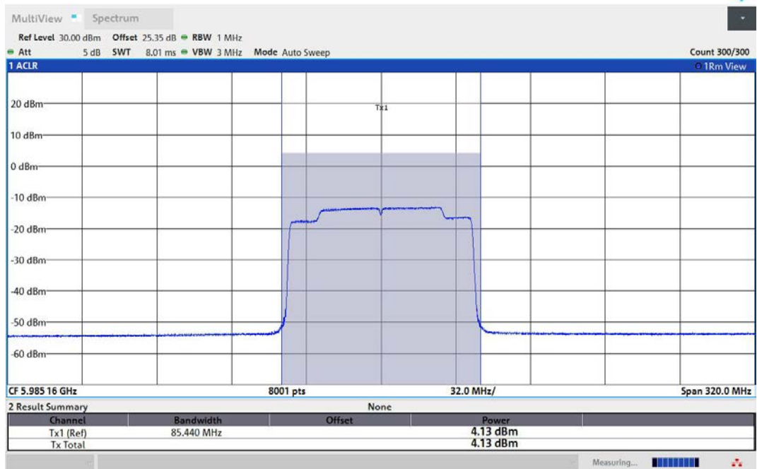
11AX160MIMO-Ant1-6025-996Tone-RU67-PASS
