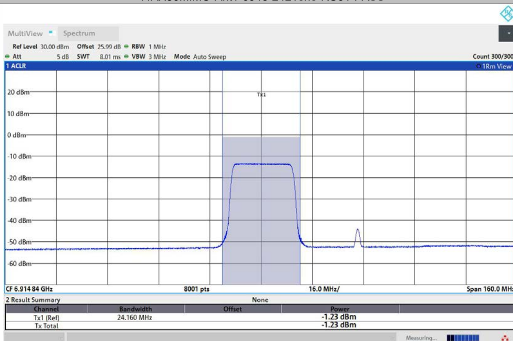
11AX80MIMO-Ant2-6945-242Tone-RU61-PASS
