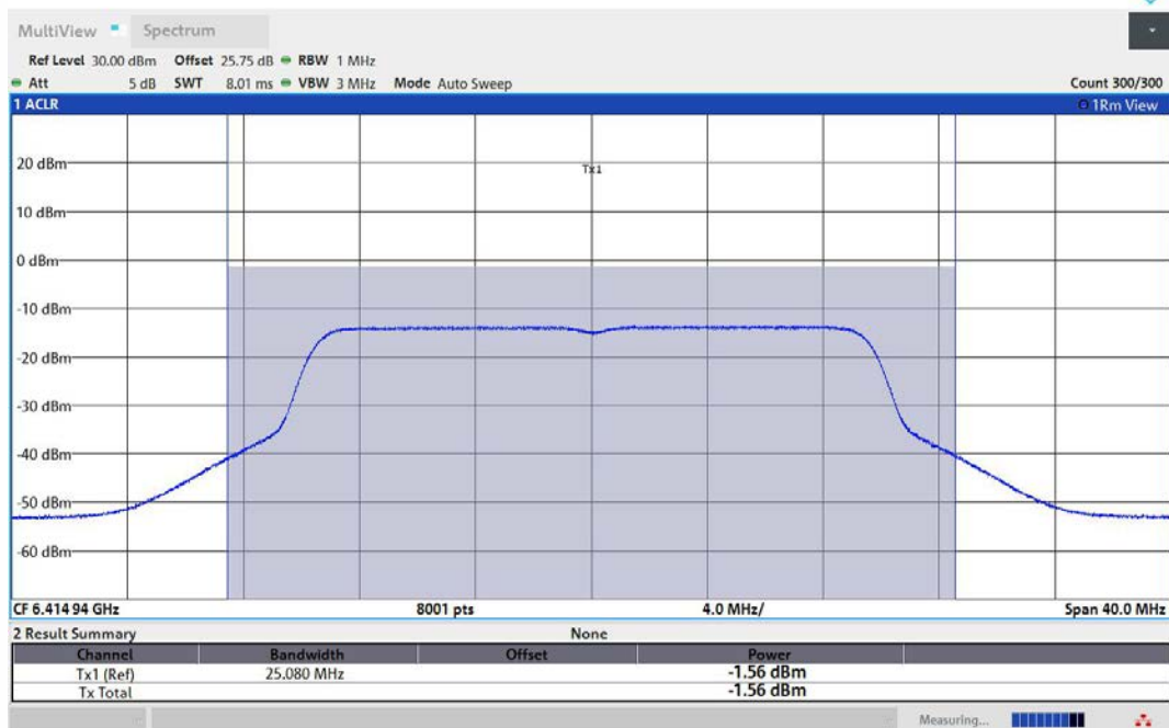
11AX20MIMO-Ant1-6415-PASS
