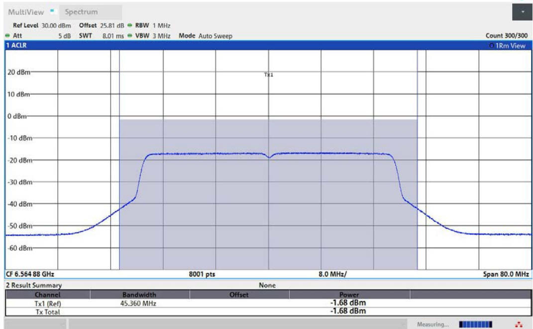
11AX40MIMO-Ant2-6565-PASS
