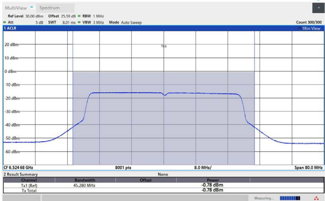
11AX40MIMO-Ant1-6525-PASS
