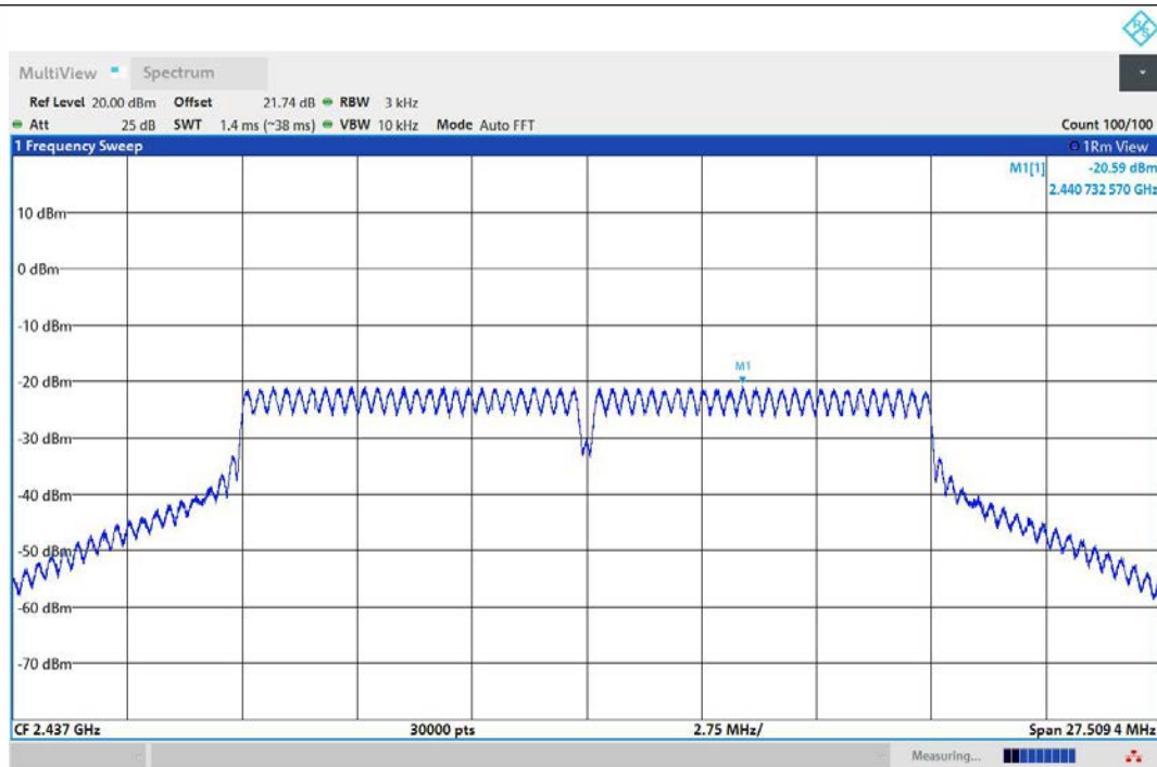
11G-Ant1-2437-PASS
