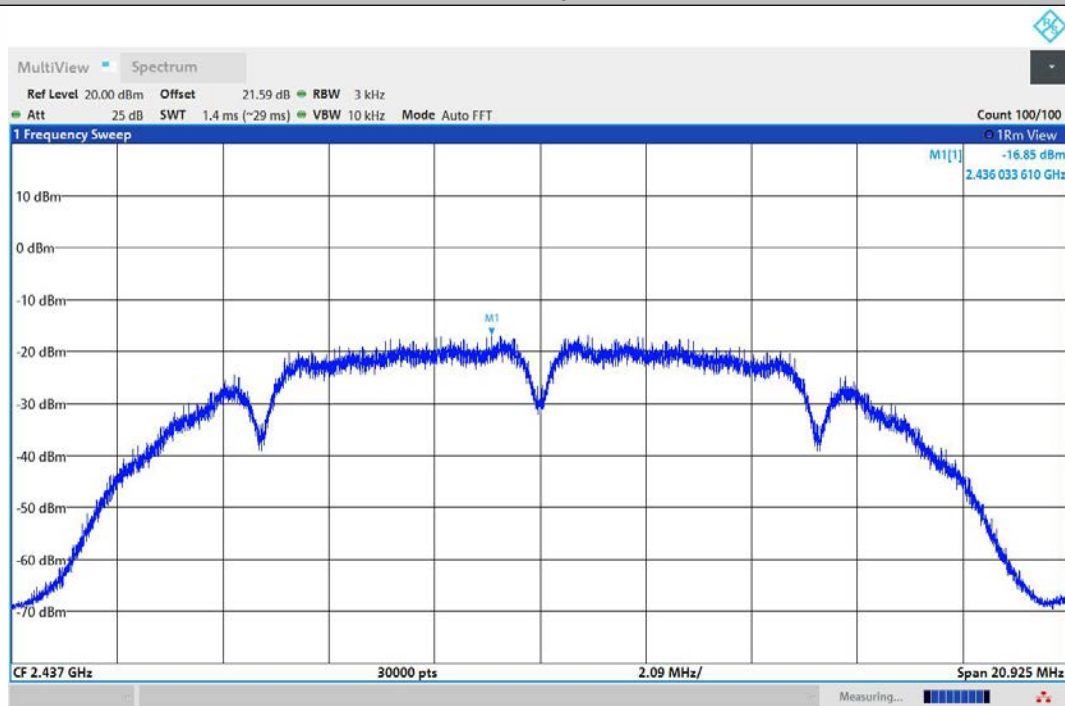
11B-Ant2-2437-PASS
