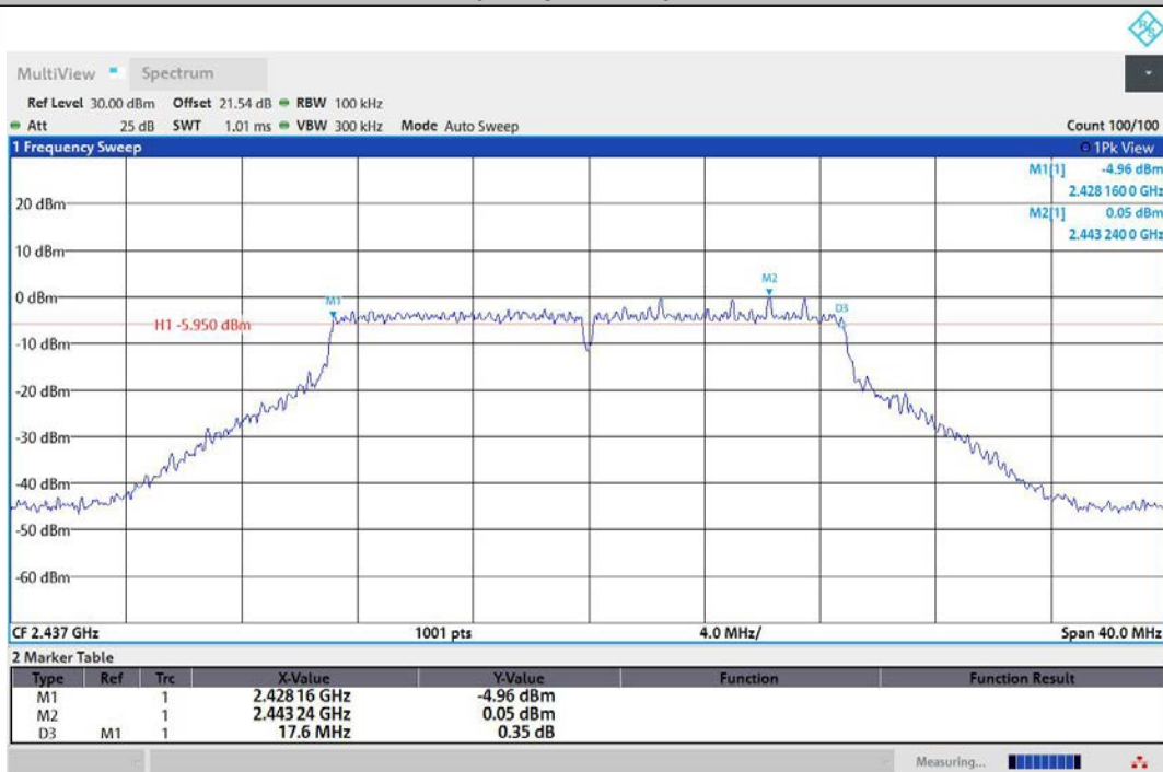
11N20MIMO-Ant2-2437-PASS
