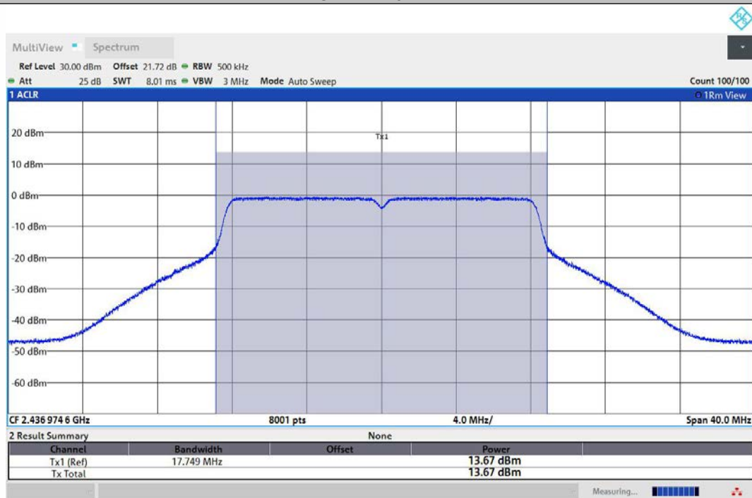
11G-Ant2-2437-PASS
