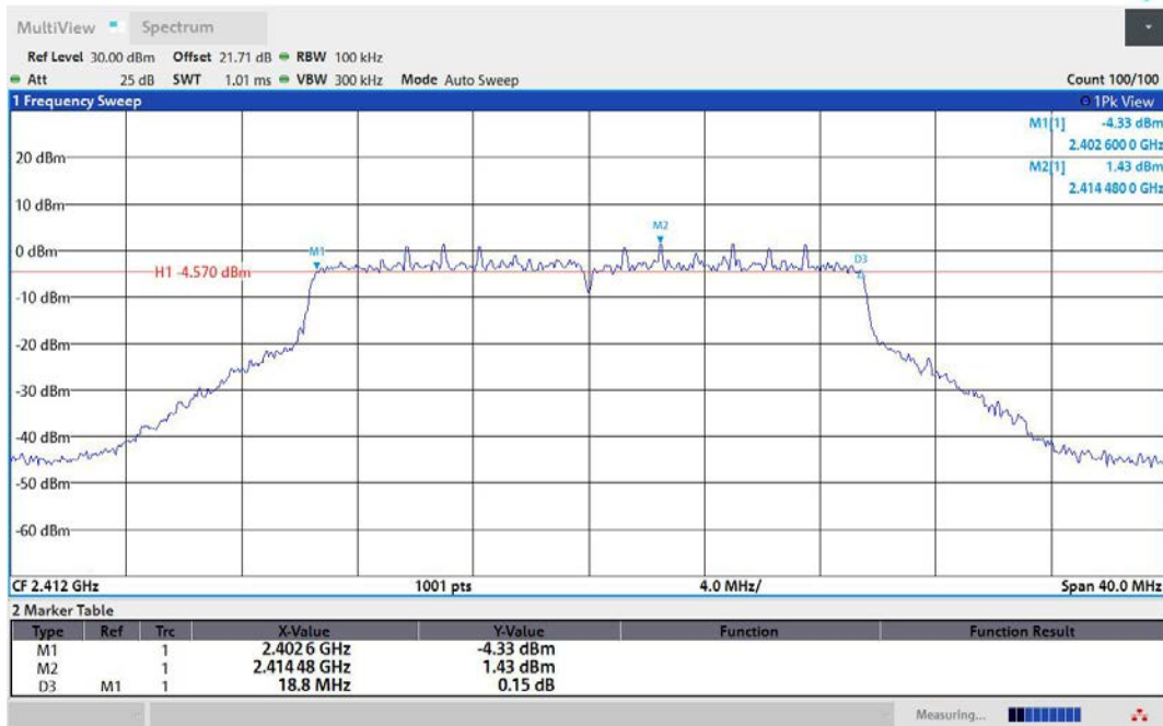
11AX20MIMO-Ant1-2412-PASS
