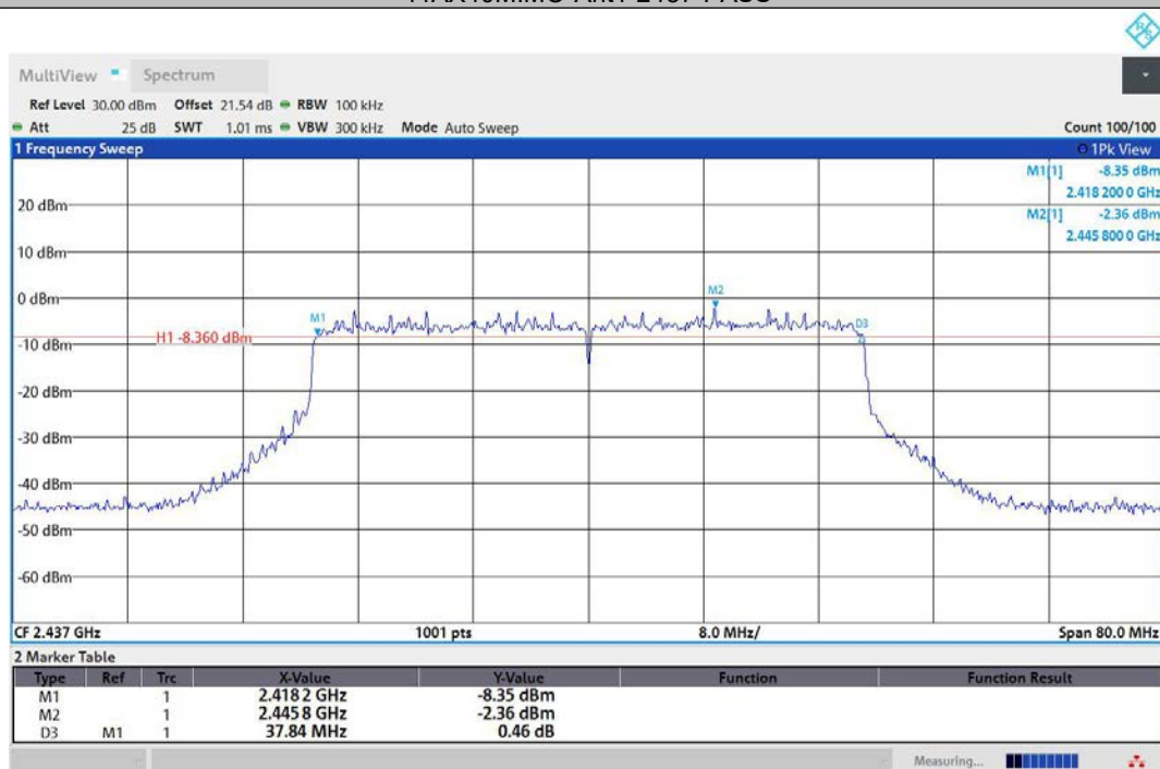
11AX40MIMO-Ant2-2437-PASS
