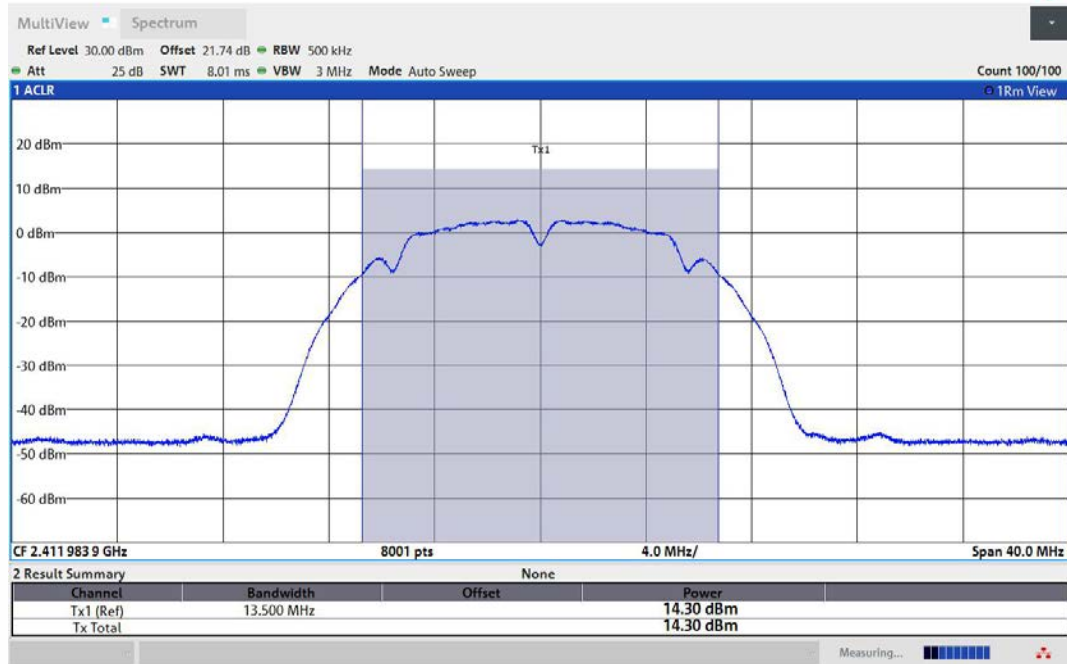
11B-Ant2-2412-PASS
