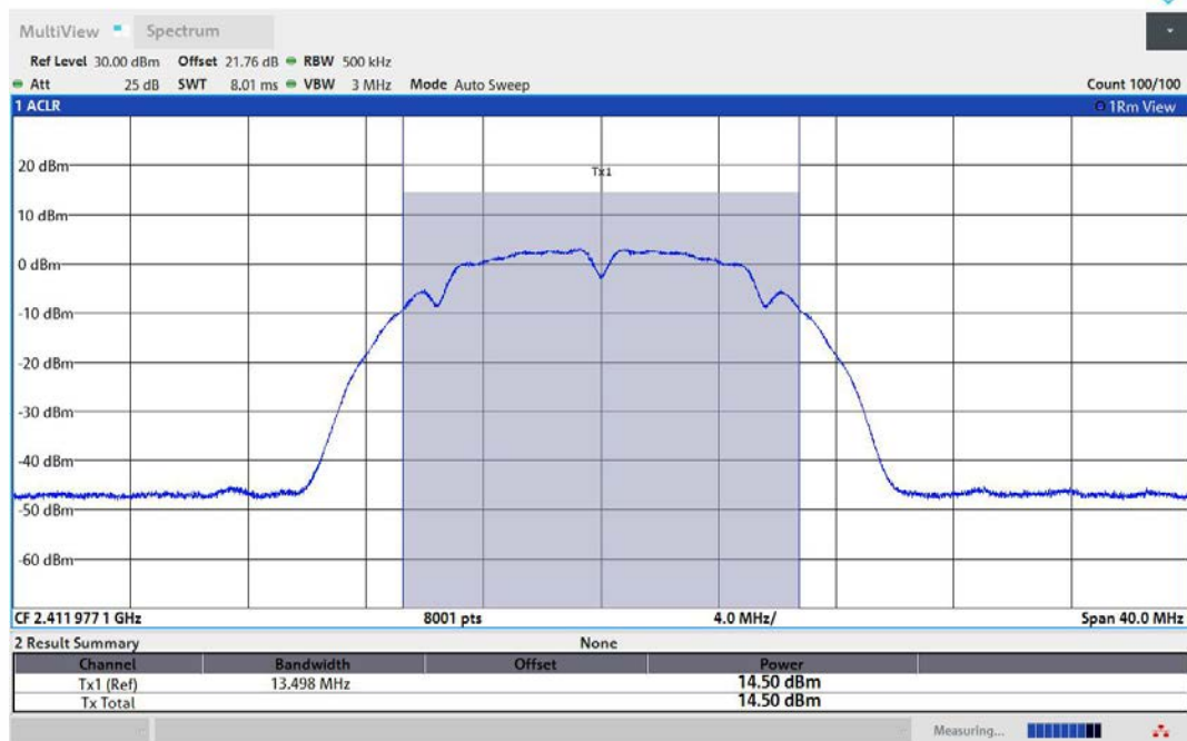
11B-Ant1-2412-PASS
