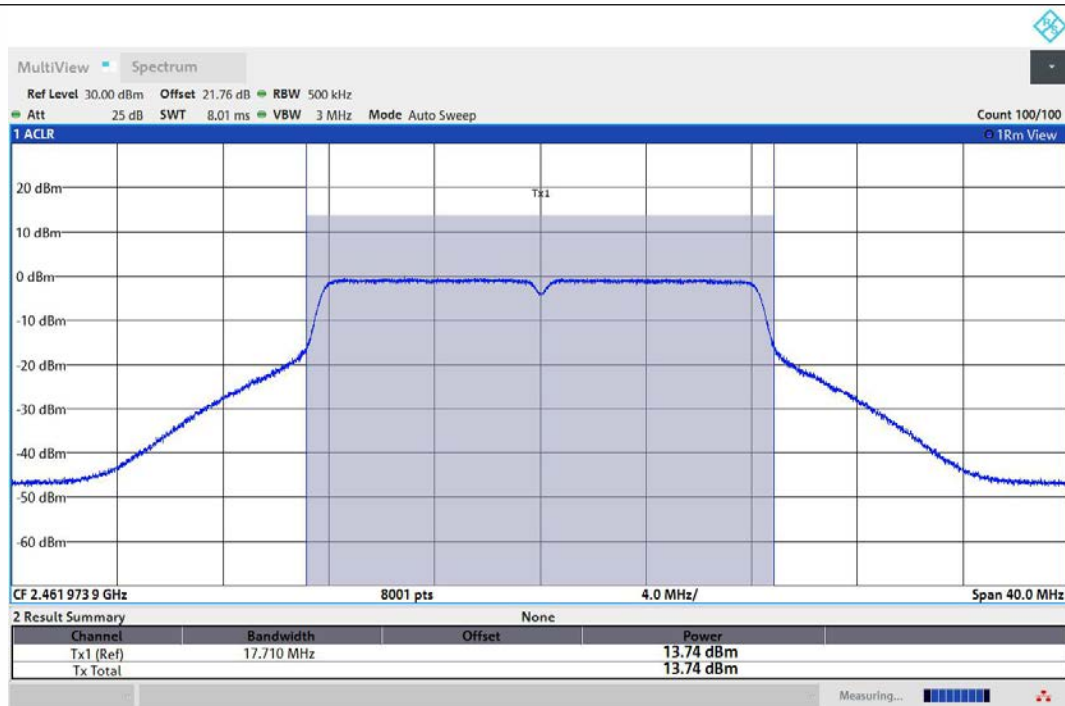
11G-Ant1-2462-PASS
