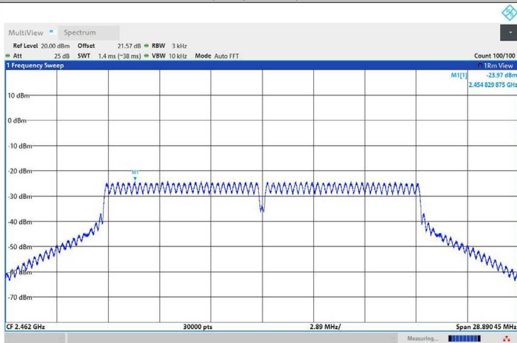
11N20MIMO-Ant2-2462-PASS
