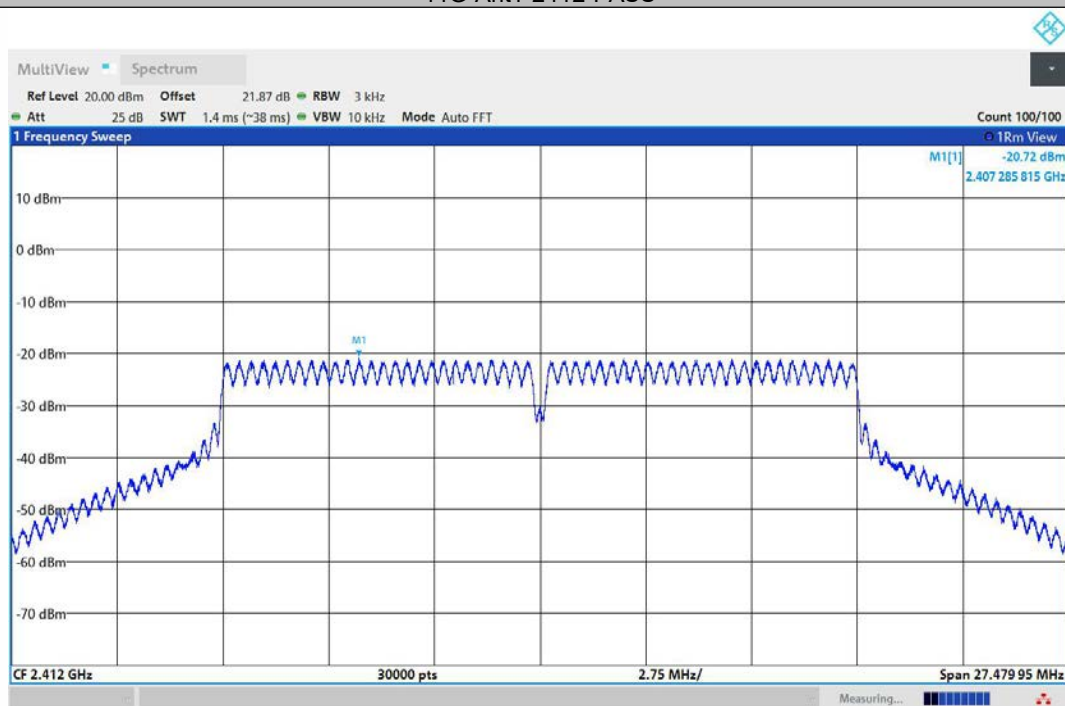
11G-Ant2-2412-PASS
