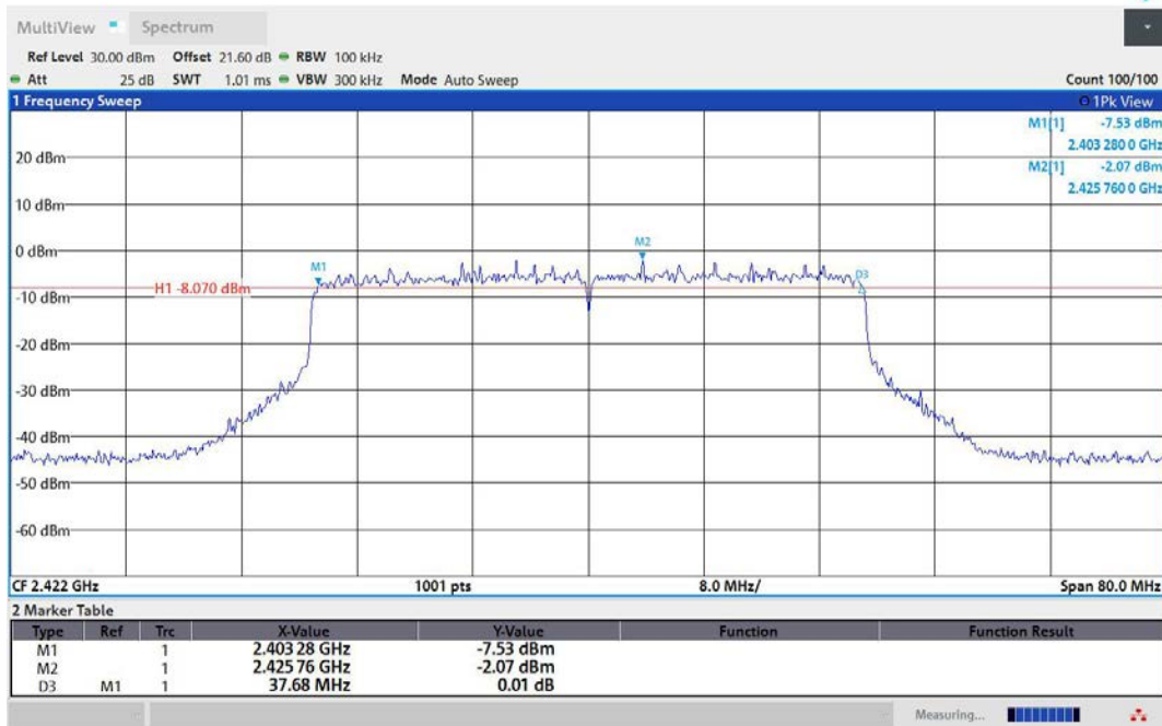
11AX40MIMO-Ant1-2422-PASS
