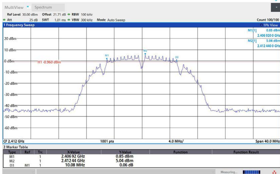
11B-Ant1-2412-PASS
