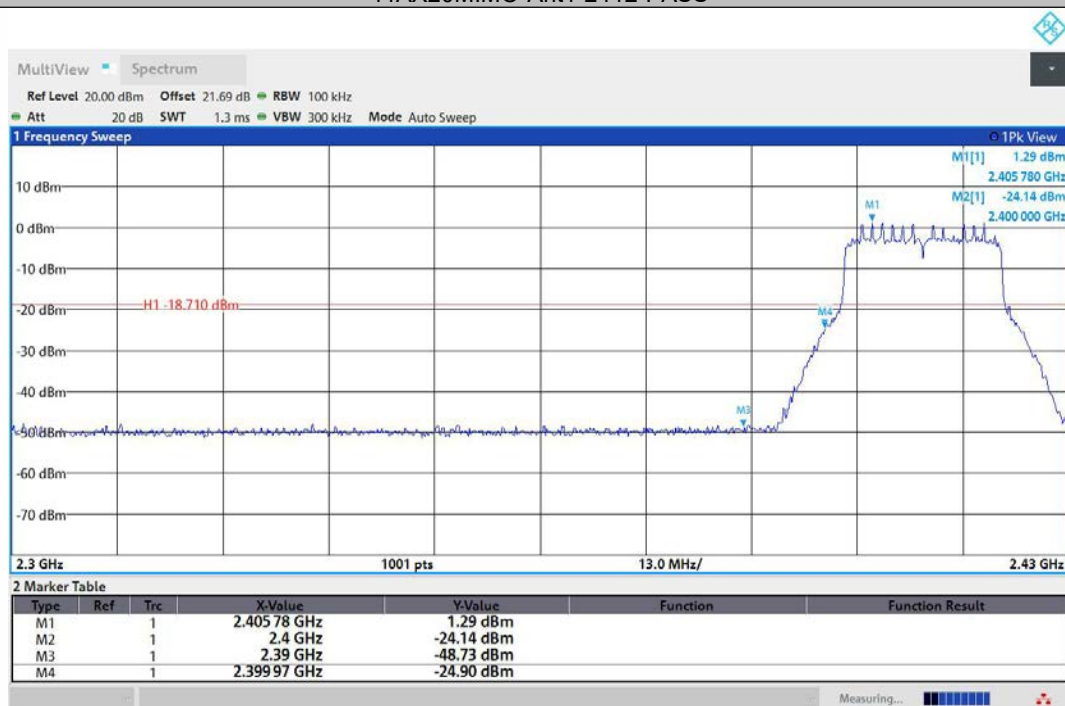
11AX20MIMO-Ant2-2412-PASS
