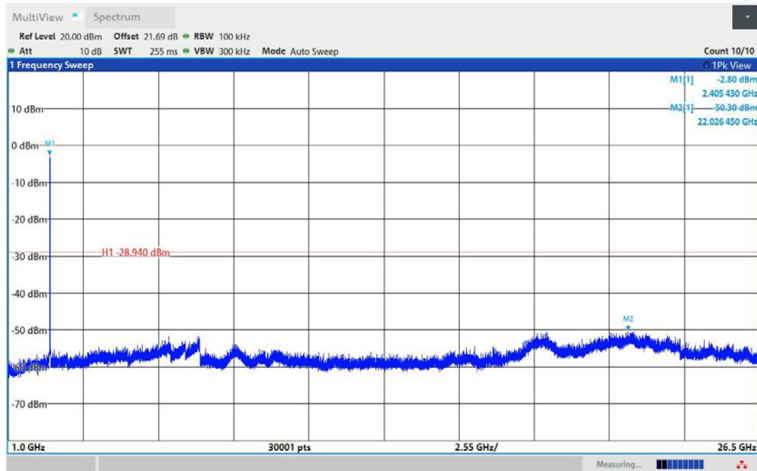
11N20MIMO-Ant2-2412-1000~26500-PASS
