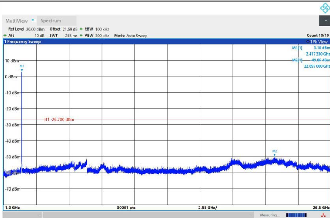
11G-Ant2-2412-1000~26500-PASS
