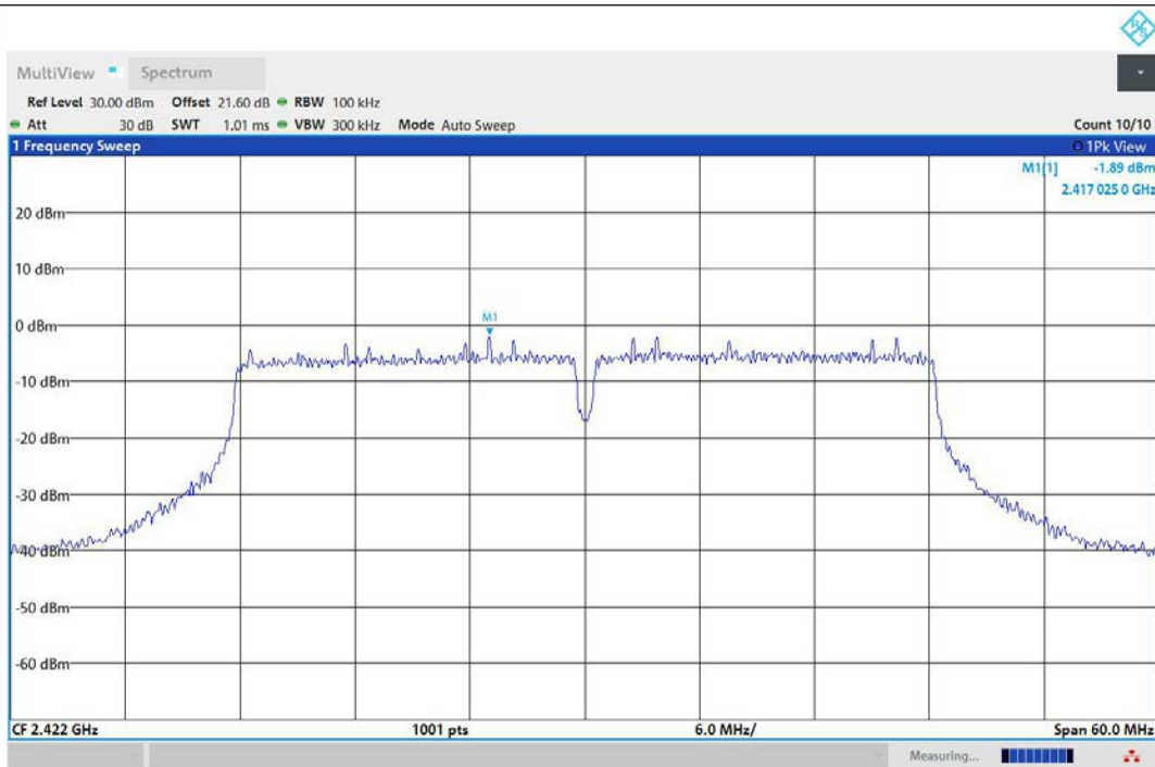
11N40MIMO-Ant1-2422-0~Reference-PASS
