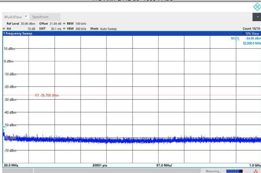
11G-Ant2-2412-30~1000-PASS
