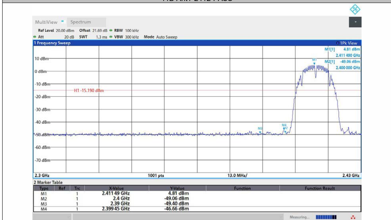
11B-Ant2-2412-PASS
