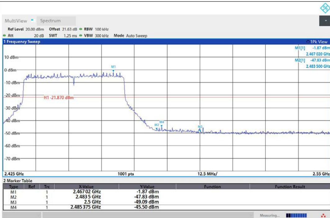
11AX40MIMO-Ant1-2452-PASS
