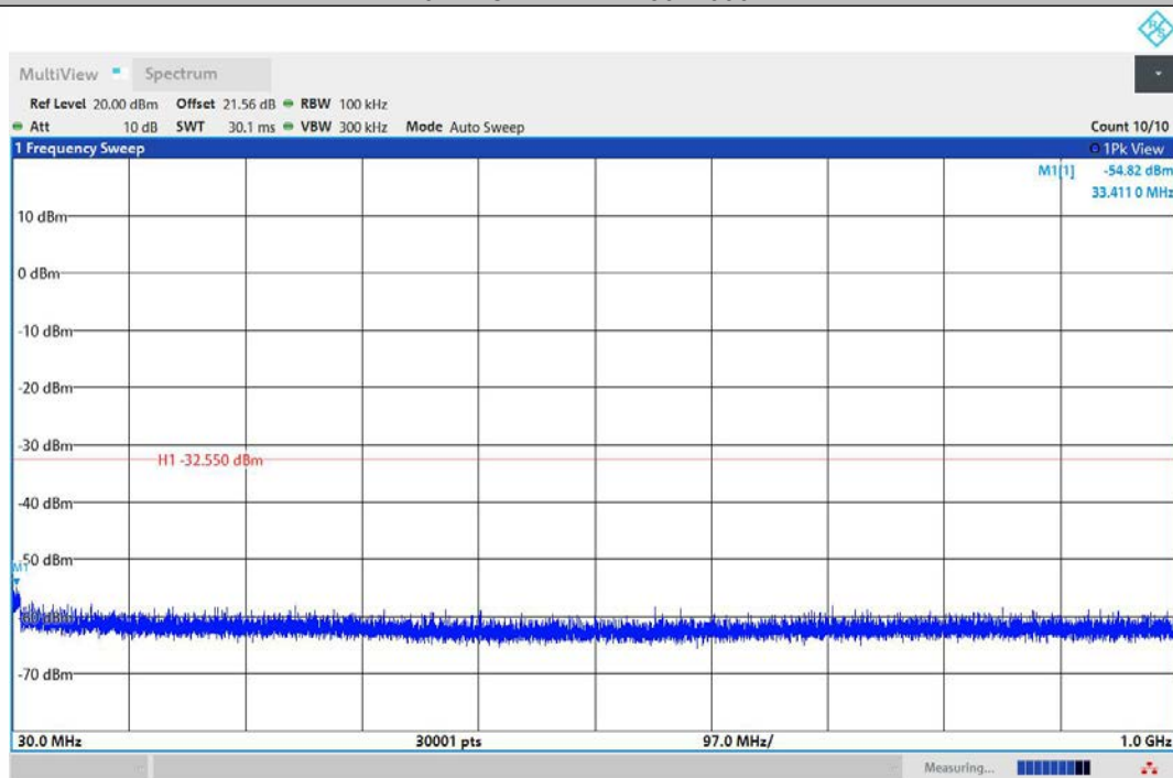
11N40MIMO-Ant2-2422-30~1000-PASS
