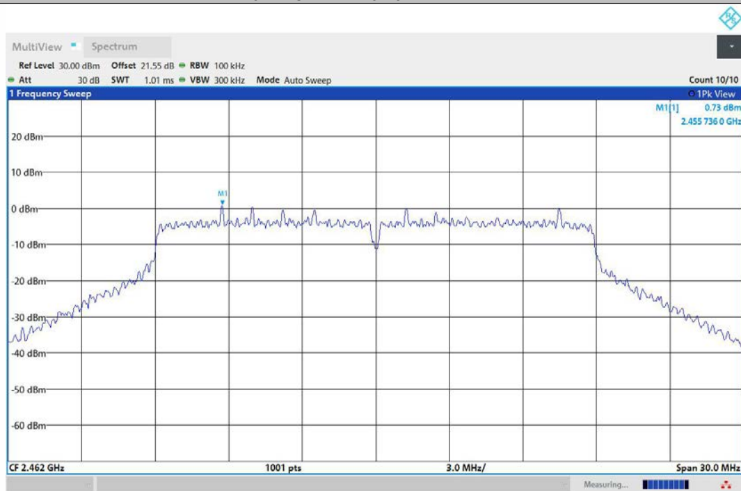
11N20MIMO-Ant2-2462-0~Reference-PASS
