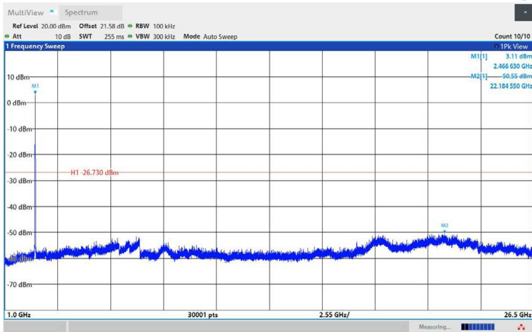
11G-Ant1-2462-1000~26500-PASS
