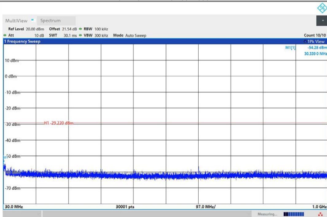
11N20MIMO-Ant2-2437-30~1000-PASS
