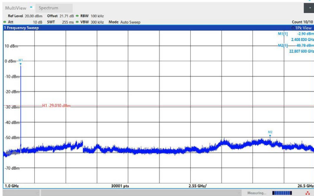
11N20MIMO-Ant1-2412-1000~26500-PASS
