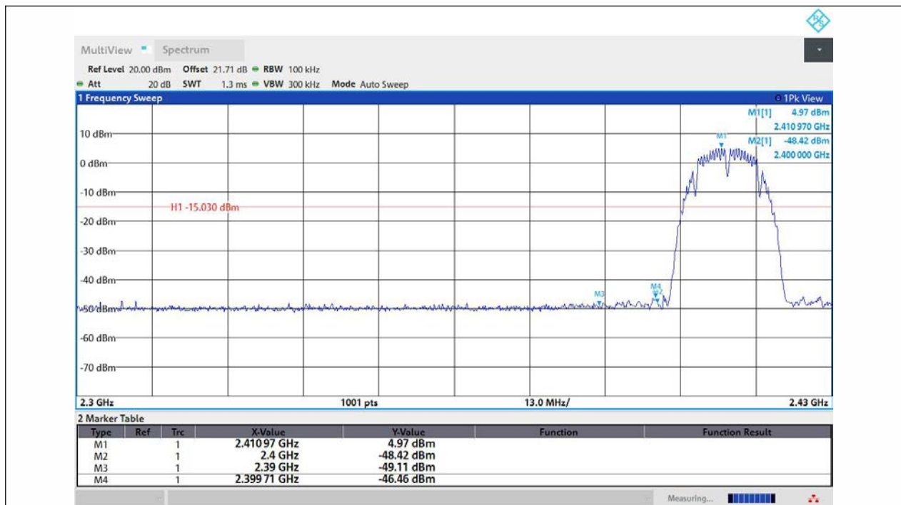
11B-Ant1-2412-PASS
