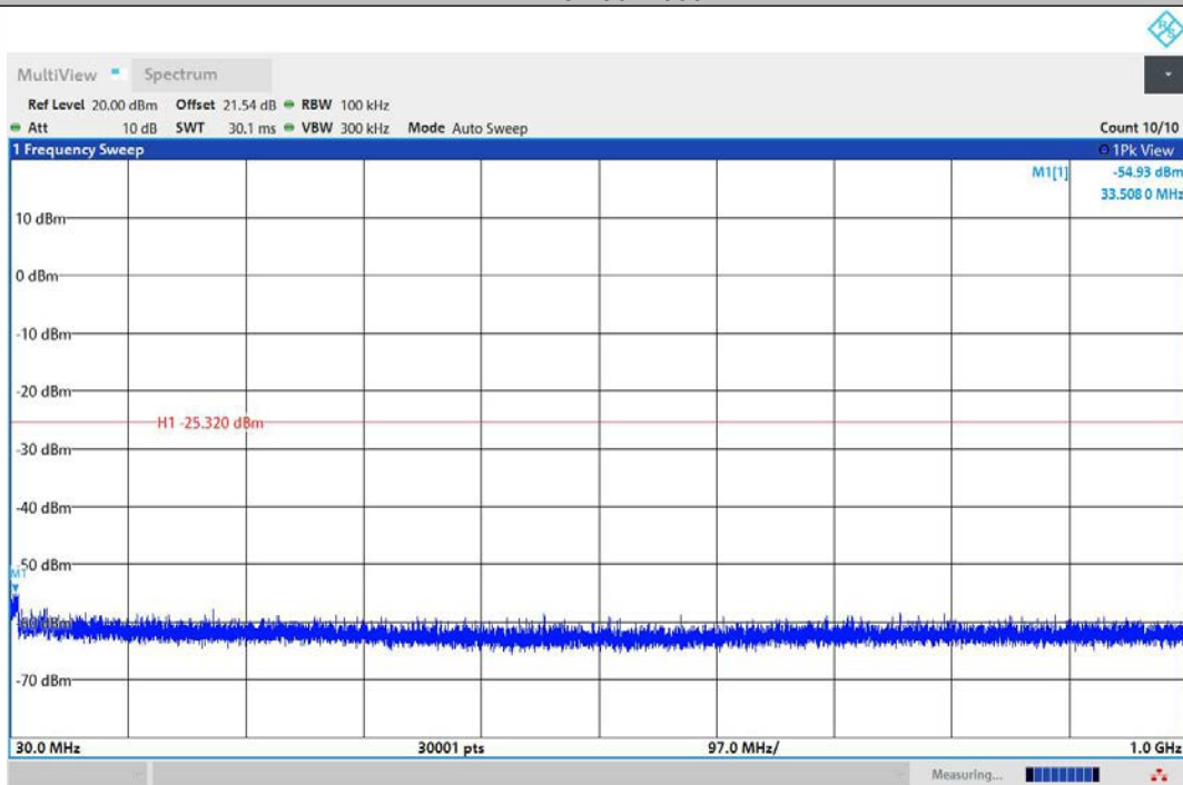
11B-Ant2-2437-30~1000-PASS
