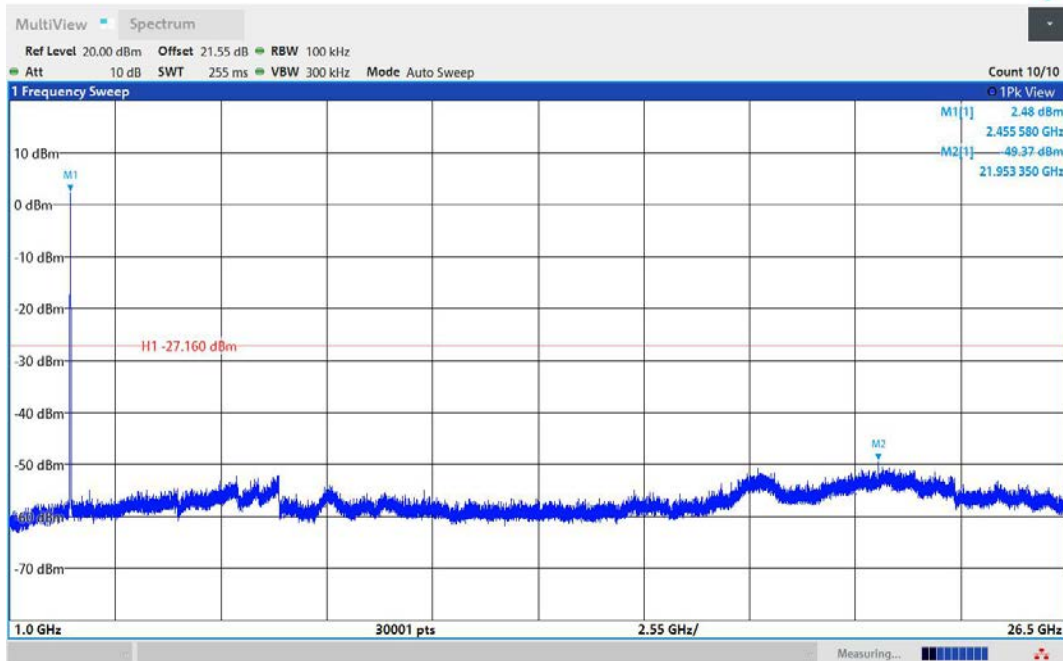
11G-Ant2-2462-1000~26500-PASS
