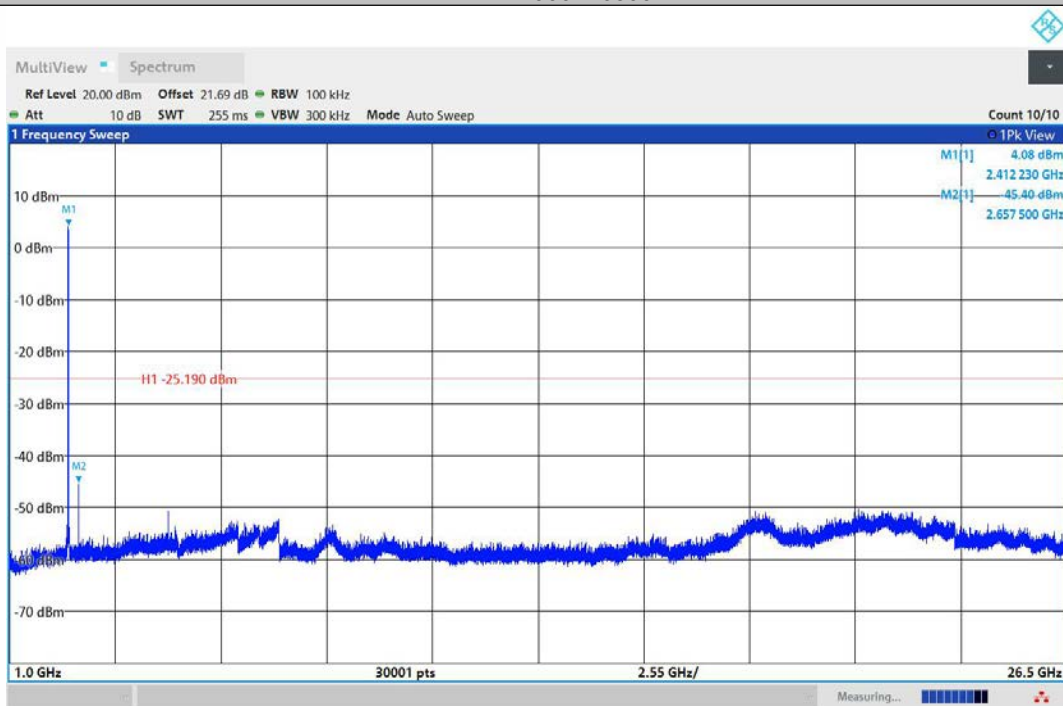
11B-Ant2-2412-1000~26500-PASS
