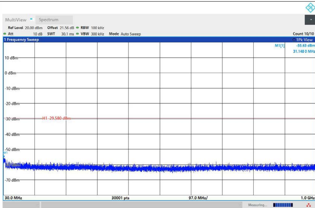
11N20MIMO-Ant1-2437-30~1000-PASS
