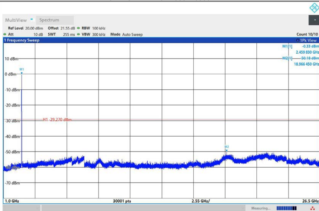
11N20MIMO-Ant2-2462-1000~26500-PASS
