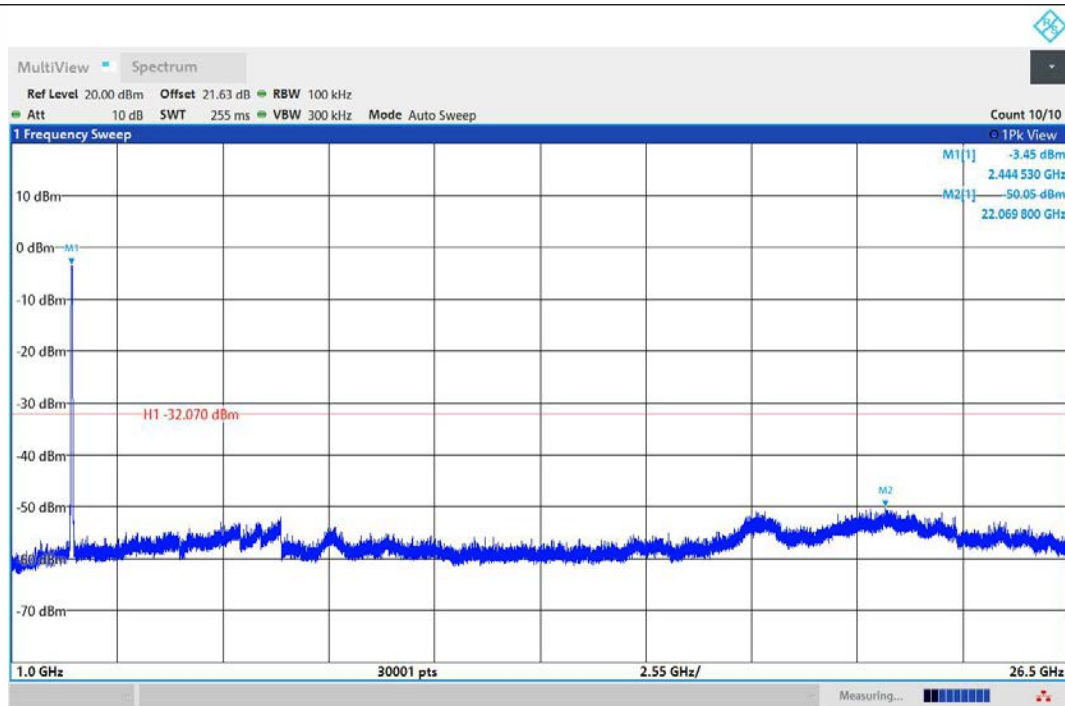
11AX40MIMO-Ant1-2452-1000~26500-PASS
