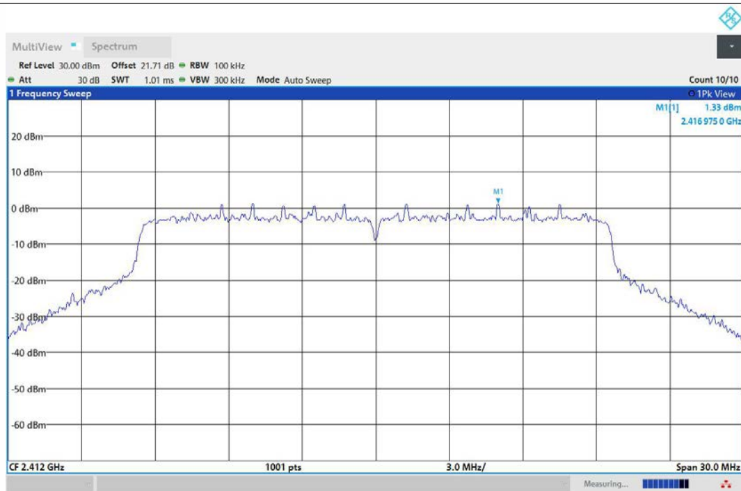
11AX20MIMO-Ant1-2412-0~Reference-PASS
