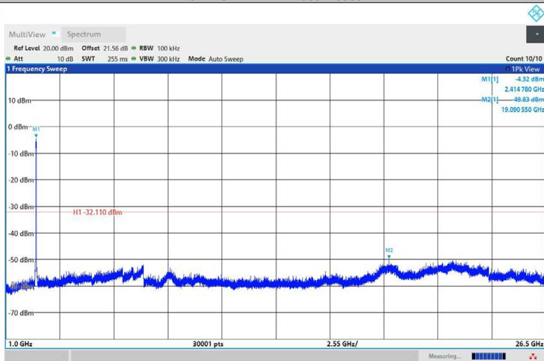
11AX40MIMO-Ant2-2422-1000~26500-PASS
