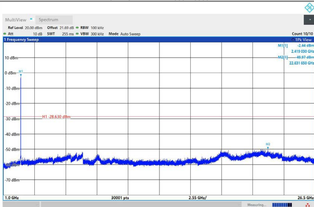
11AX20MIMO-Ant2-2412-1000~26500-PASS
