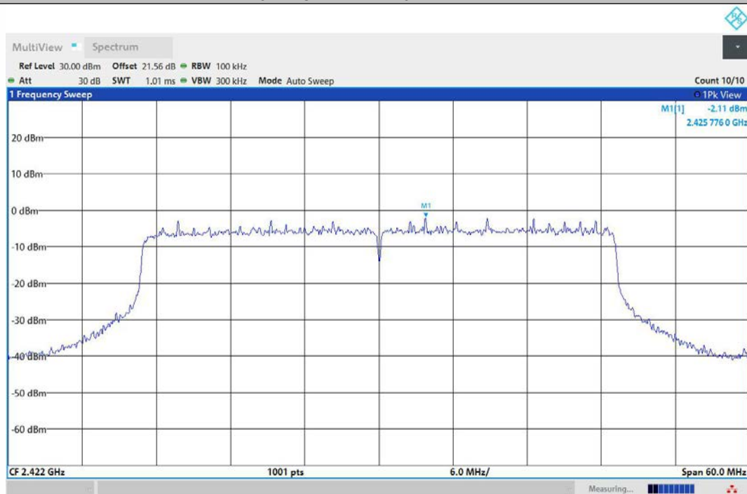
11AX40MIMO-Ant2-2422-0~Reference-PASS
