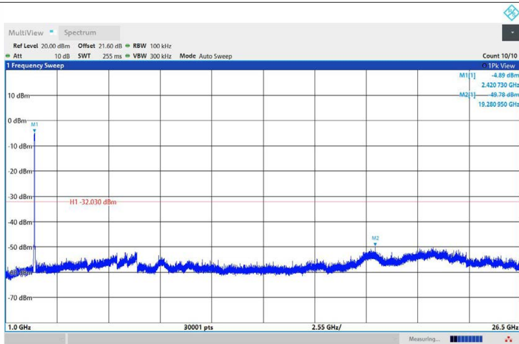
11AX40MIMO-Ant1-2422-1000~26500-PASS
