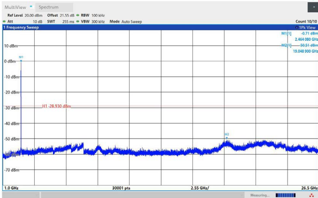
11AX20MIMO-Ant2-2462-1000~26500-PASS
