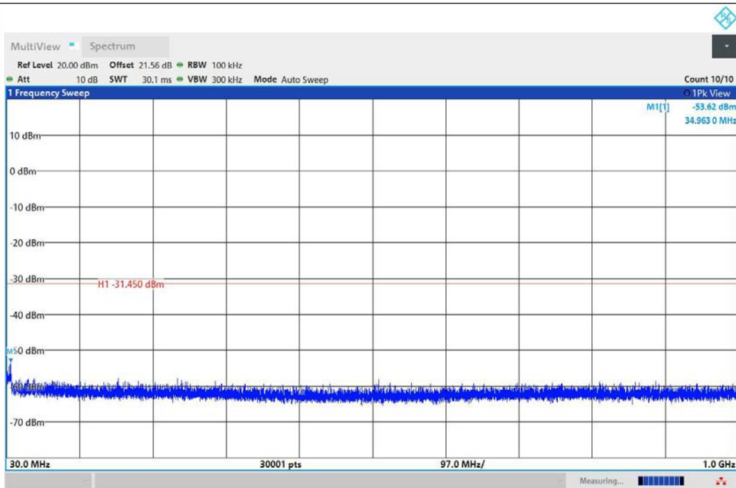
11N40MIMO-Ant1-2437-30~1000-PASS
