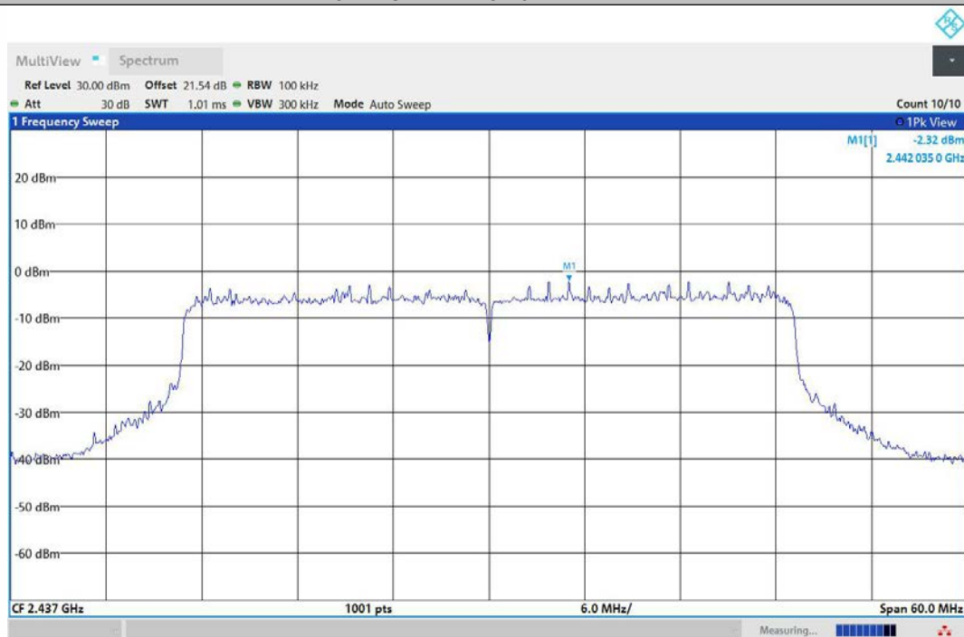
11AX40MIMO-Ant2-2437-0~Reference-PASS
