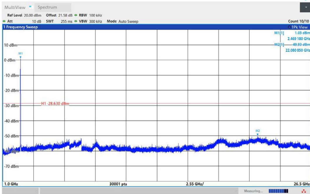
11AX20MIMO-Ant1-2462-1000~26500-PASS
