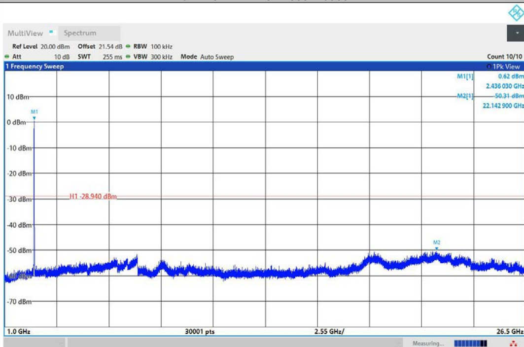
11AX20MIMO-Ant2-2437-1000~26500-PASS
