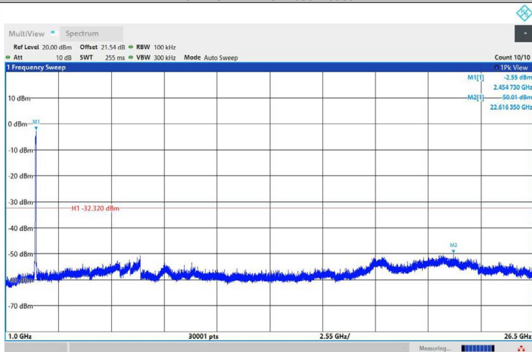
11AX40MIMO-Ant2-2437-1000~26500-PASS
