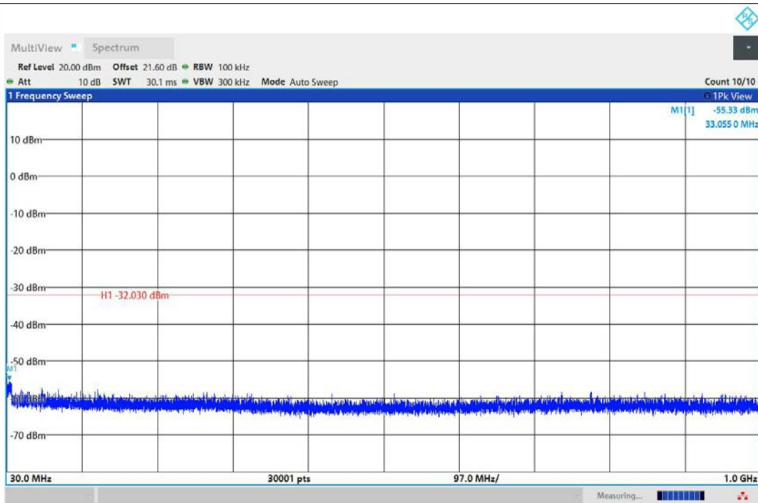
11AX40MIMO-Ant1-2422-30~1000-PASS
