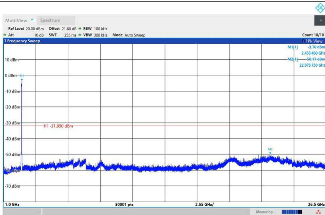
11N40MIMO-Ant1-2422-1000~26500-PASS
