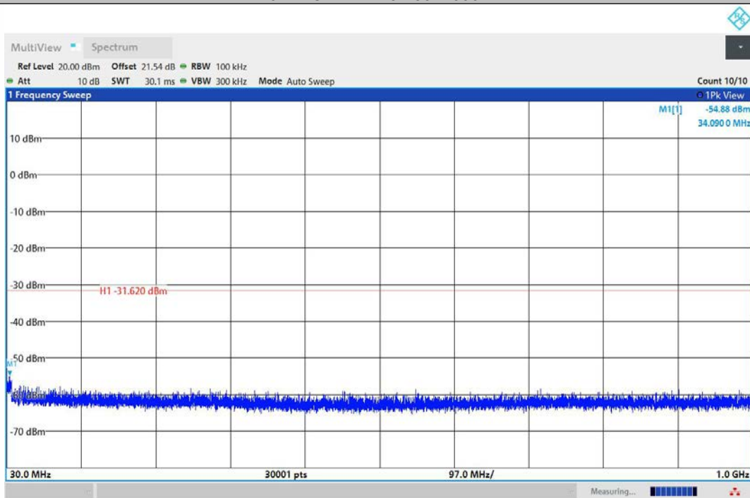
11N40MIMO-Ant2-2437-30~1000-PASS
