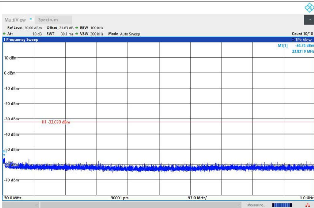
11AX40MIMO-Ant1-2452-30~1000-PASS
