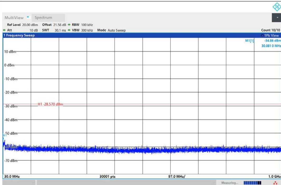
11AX20MIMO-Ant1-2437-30~1000-PASS
