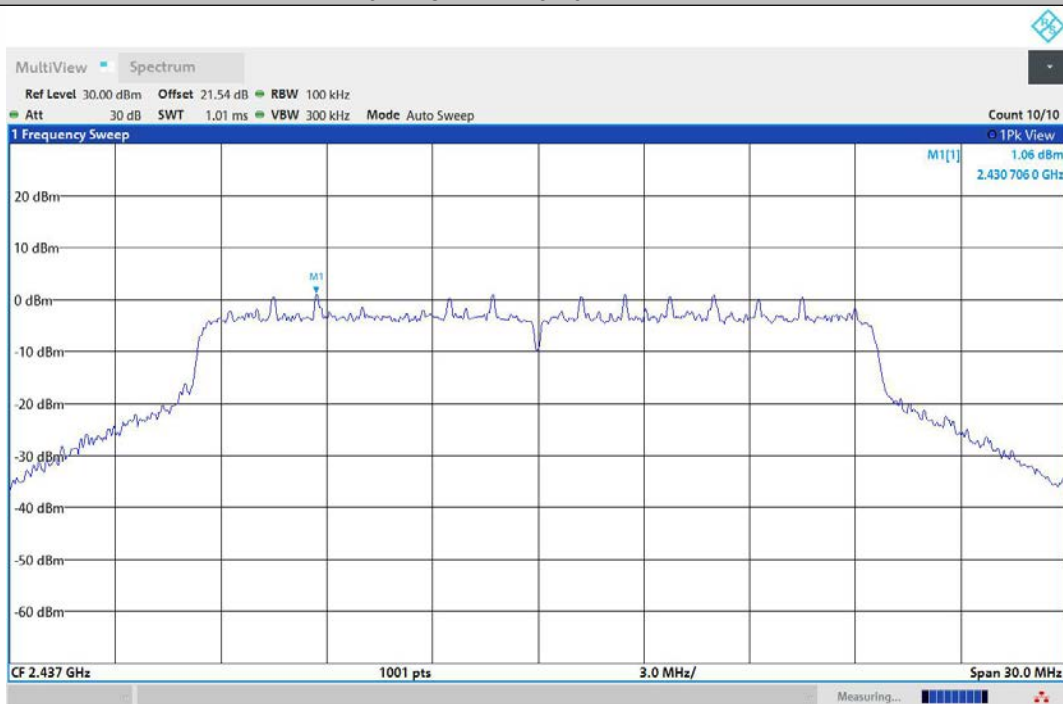
11AX20MIMO-Ant2-2437-0~Reference-PASS
