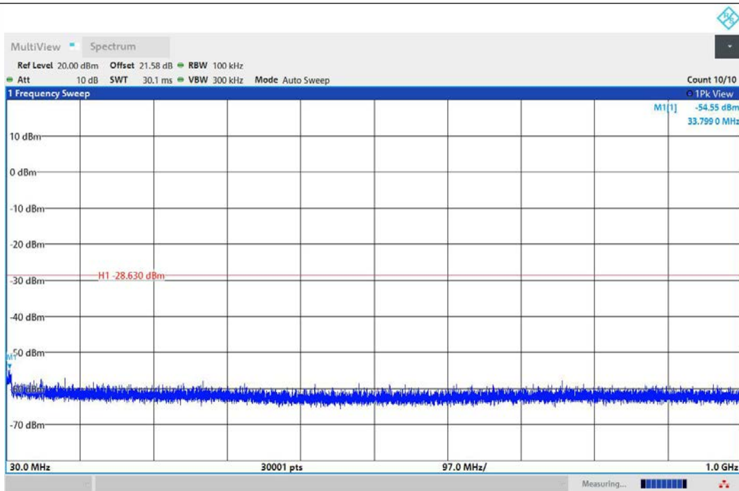
11AX20MIMO-Ant1-2462-30~1000-PASS
