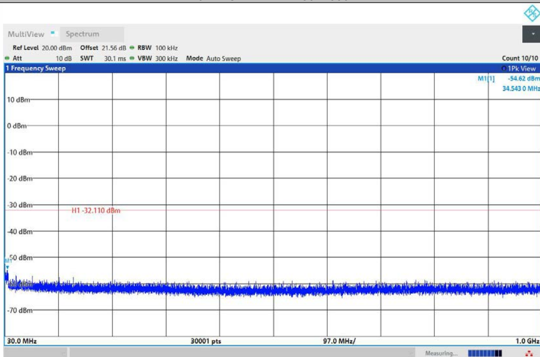
11AX40MIMO-Ant2-2422-30~1000-PASS
