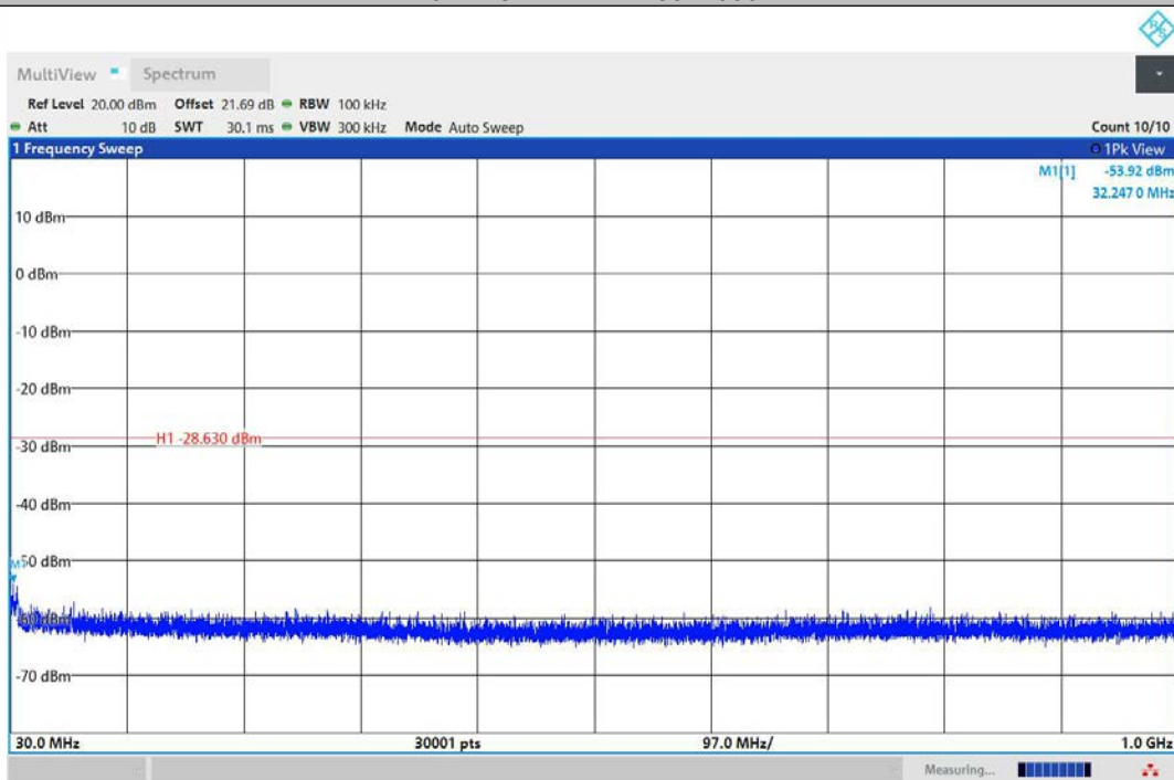
11AX20MIMO-Ant2-2412-30~1000-PASS
