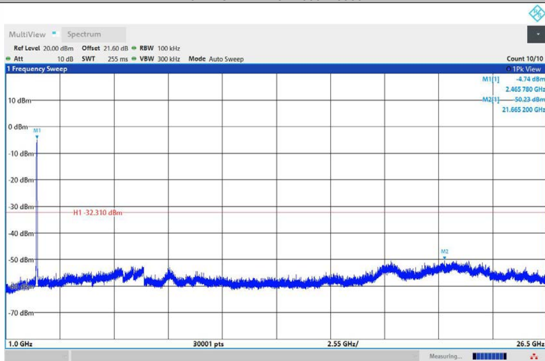
11AX40MIMO-Ant2-2452-1000~26500-PASS
