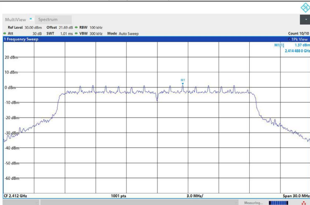
11AX20MIMO-Ant2-2412-0~Reference-PASS
