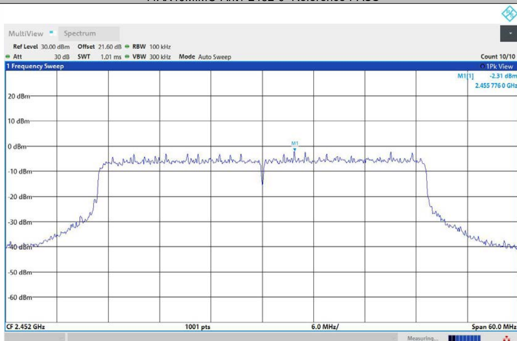
11AX40MIMO-Ant2-2452-0~Reference-PASS
