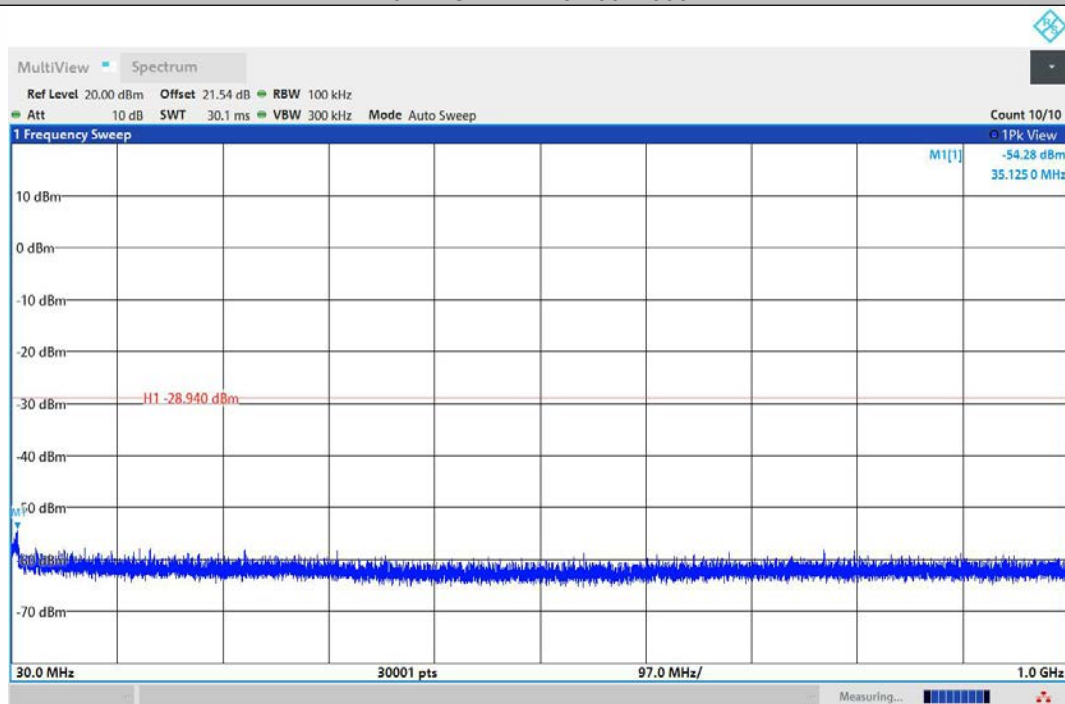
11AX20MIMO-Ant2-2437-30~1000-PASS
