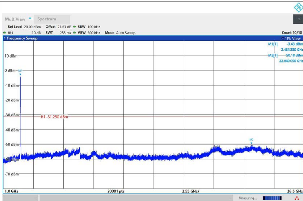
11N40MIMO-Ant1-2452-1000~26500-PASS
