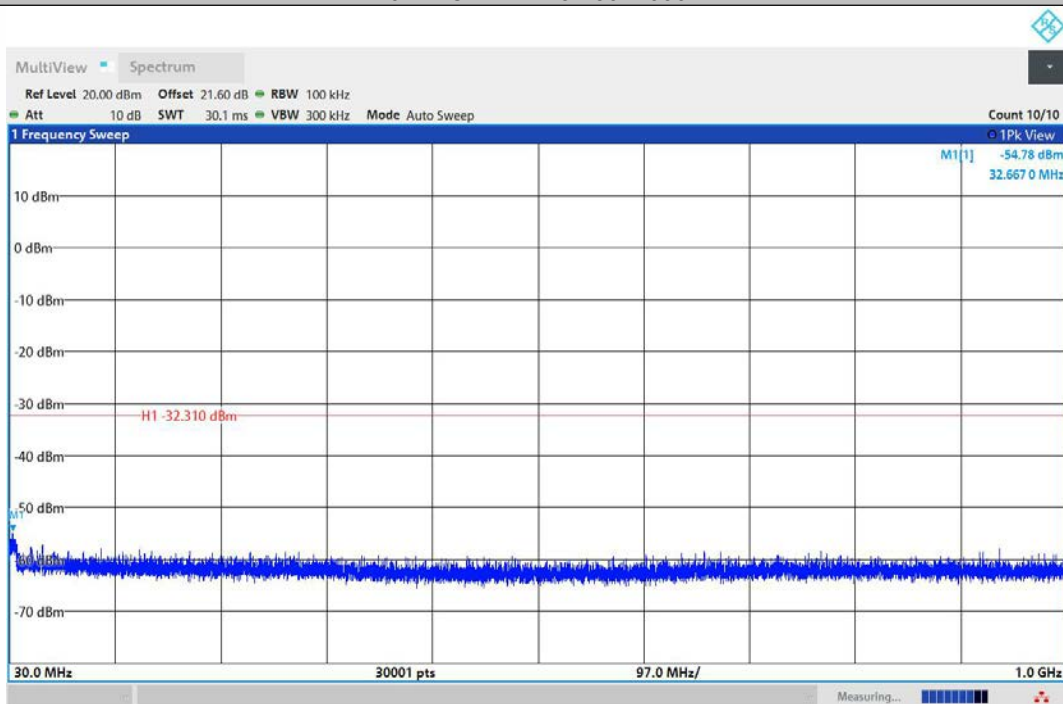
11AX40MIMO-Ant2-2452-30~1000-PASS
