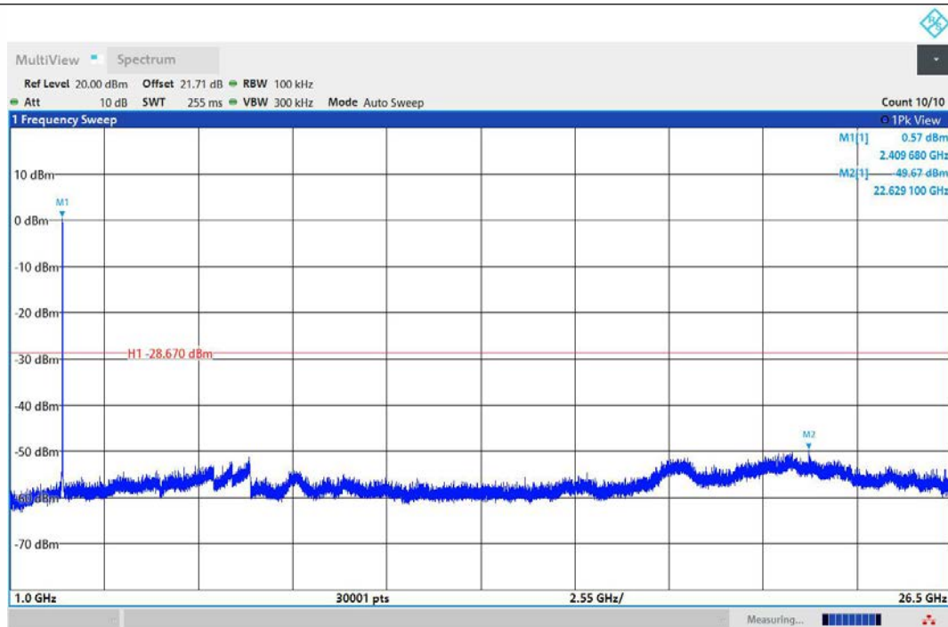
11AX20MIMO-Ant1-2412-1000~26500-PASS
