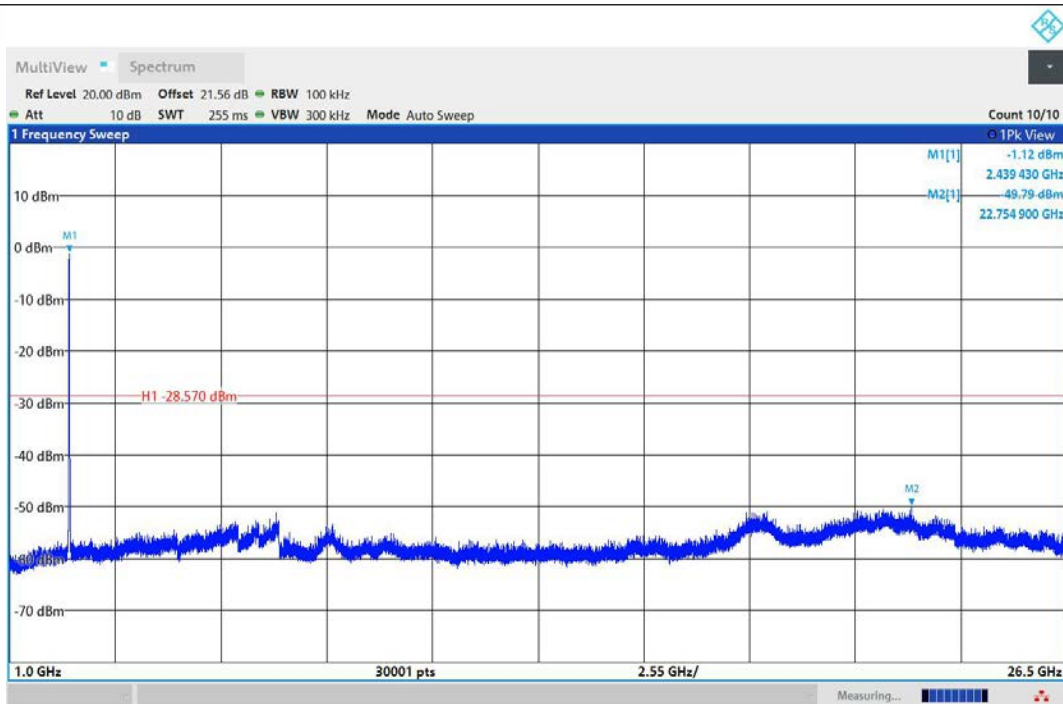
11AX20MIMO-Ant1-2437-1000~26500-PASS
