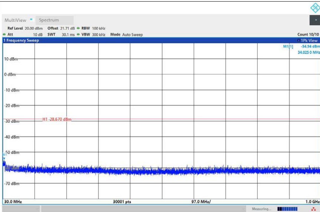
11AX20MIMO-Ant1-2412-30~1000-PASS
