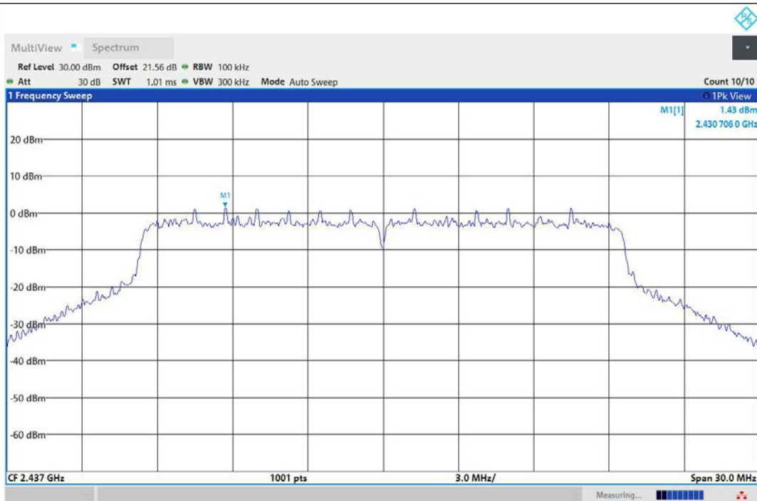
11AX20MIMO-Ant1-2437-0~Reference-PASS
