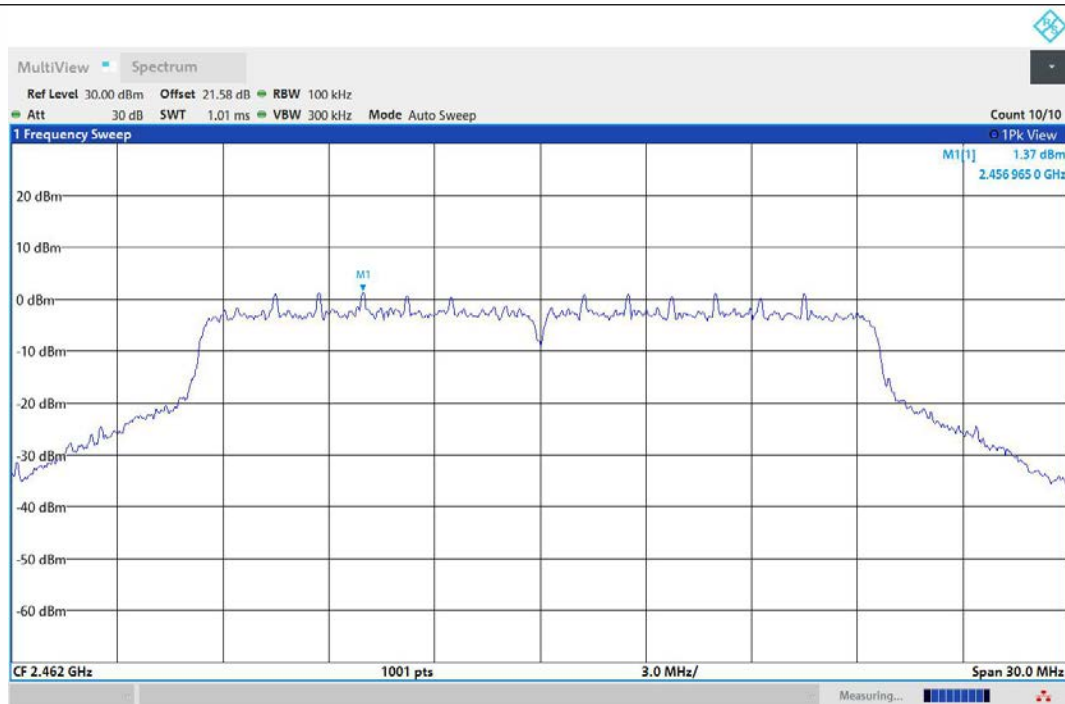
11AX20MIMO-Ant1-2462-0~Reference-PASS
