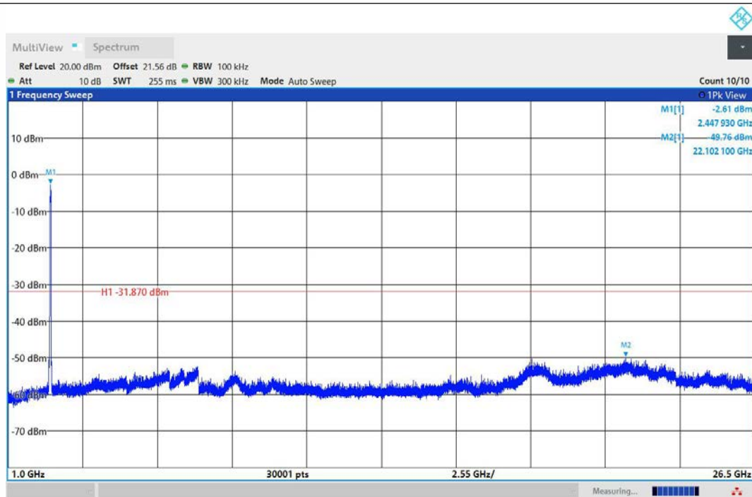
11AX40MIMO-Ant1-2437-1000~26500-PASS
