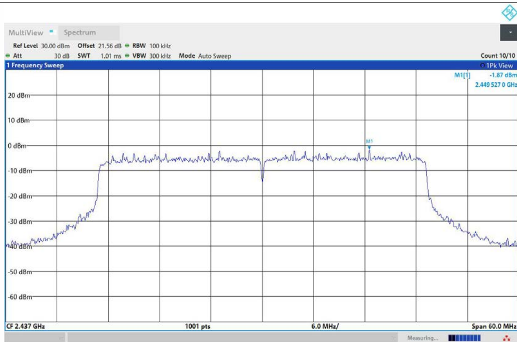
11AX40MIMO-Ant1-2437-0~Reference-PASS
