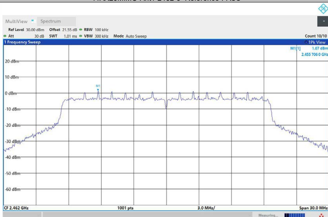
11AX20MIMO-Ant2-2462-0~Reference-PASS
