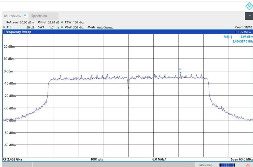
11AX40MIMO-Ant1-2452-0~Reference-PASS
