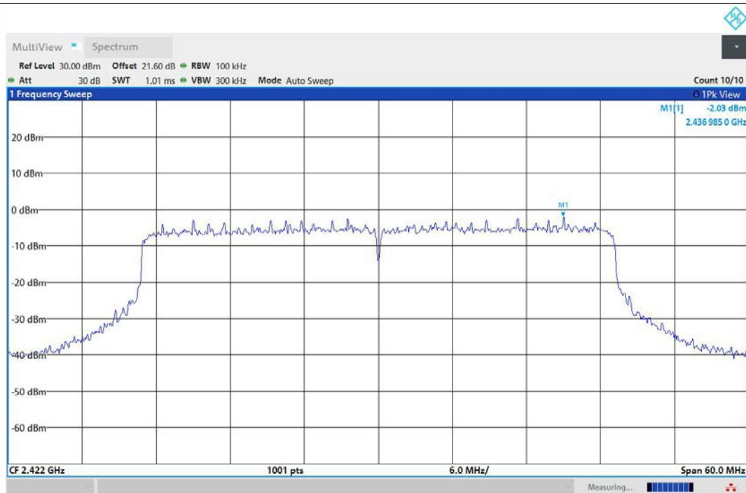
11AX40MIMO-Ant1-2422-0~Reference-PASS
