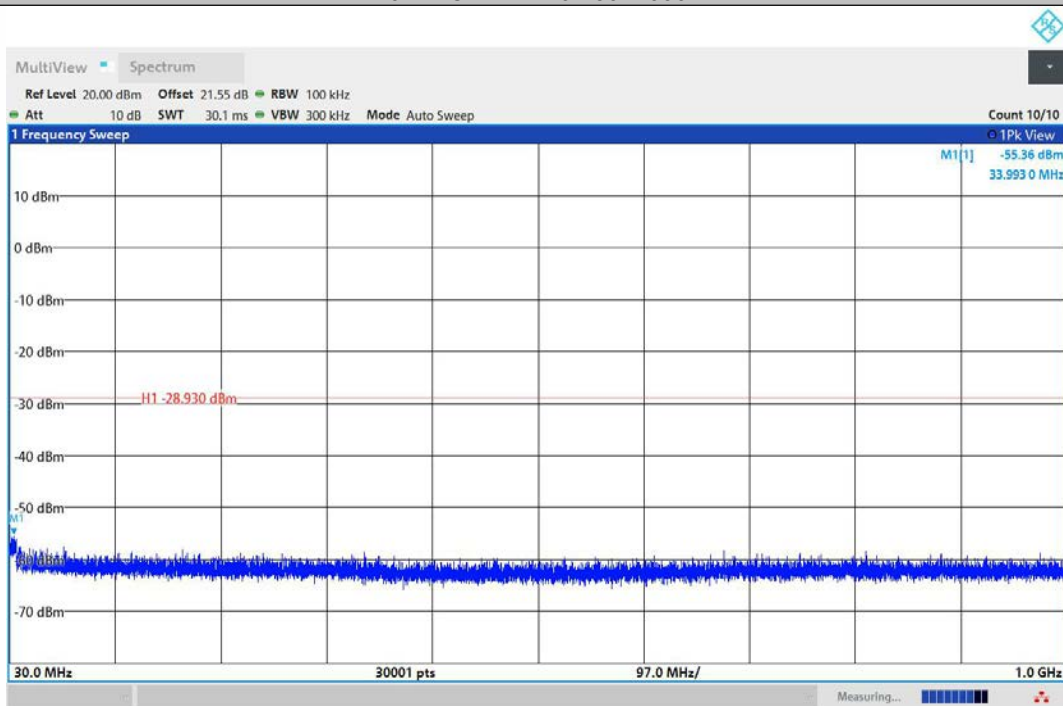
11AX20MIMO-Ant2-2462-30~1000-PASS
