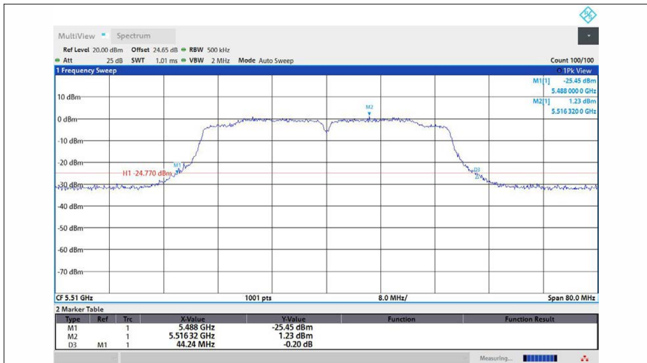
11AC40MIMO-Ant1-5510
