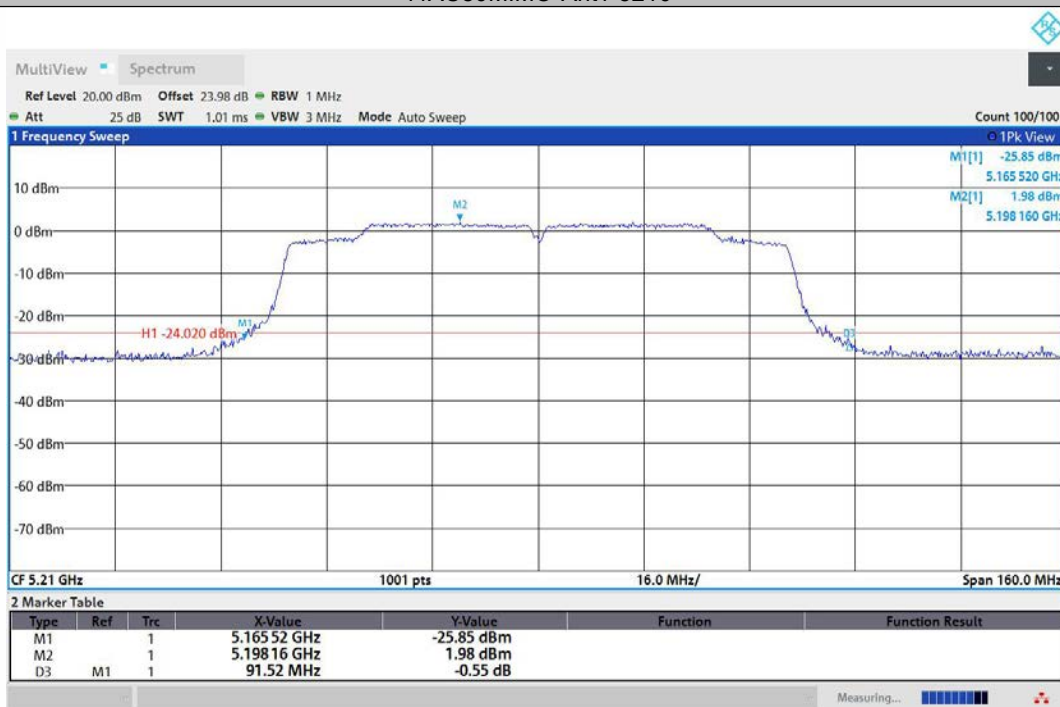
11AC80MIMO-Ant2-5210
