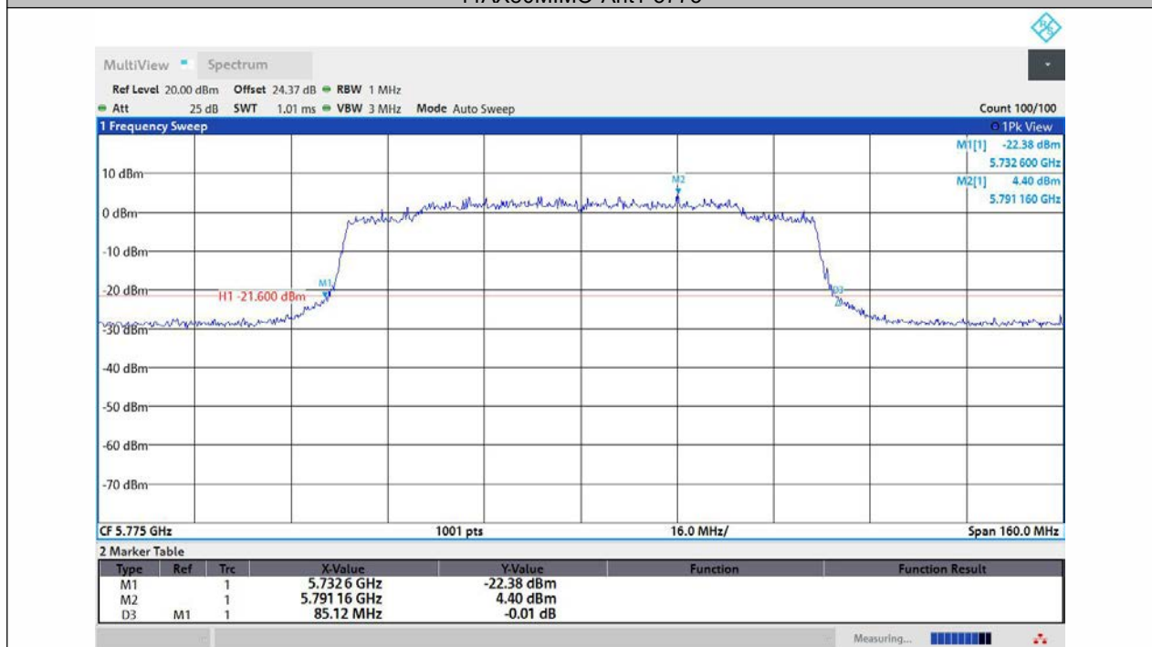
11AX80MIMO-Ant2-5775
