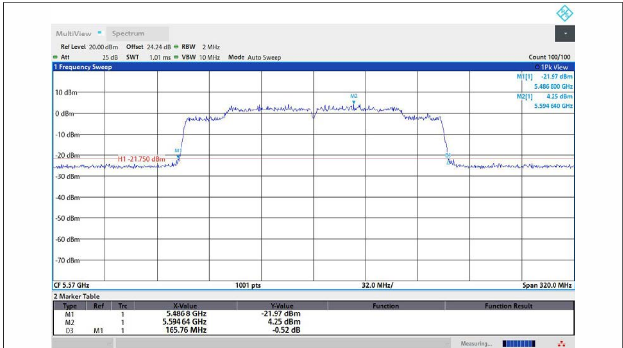
11AX160MIMO-Ant1-5570
