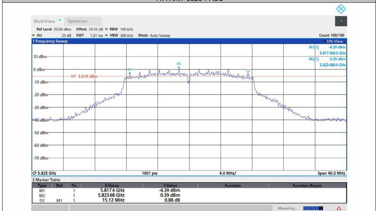
11A-Ant2-5825-PASS
