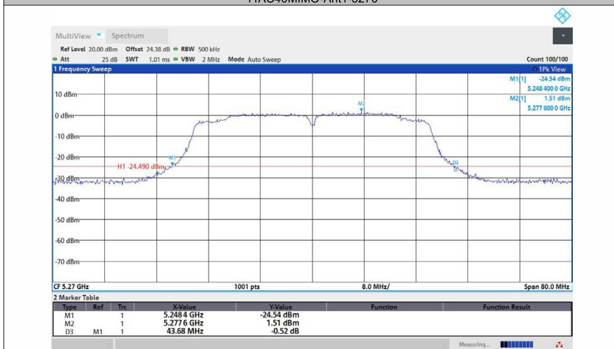
11AC40MIMO-Ant2-5270
