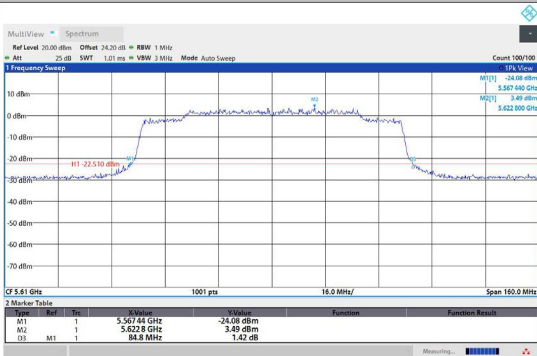
11AX80MIMO-Ant2-5610
