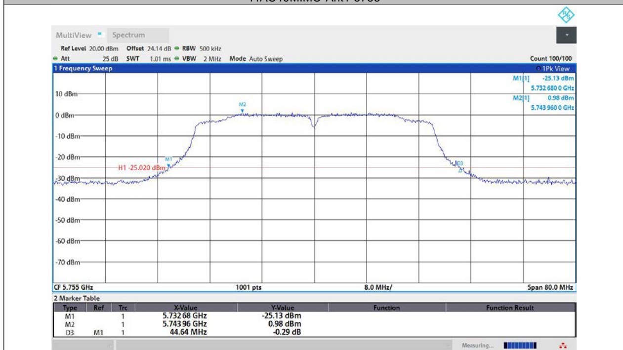
11AC40MIMO-Ant2-5755
