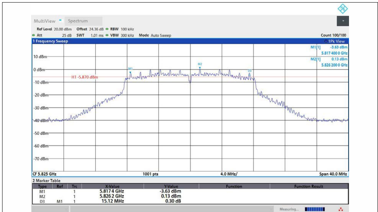
11A-Ant1-5825-PASS
