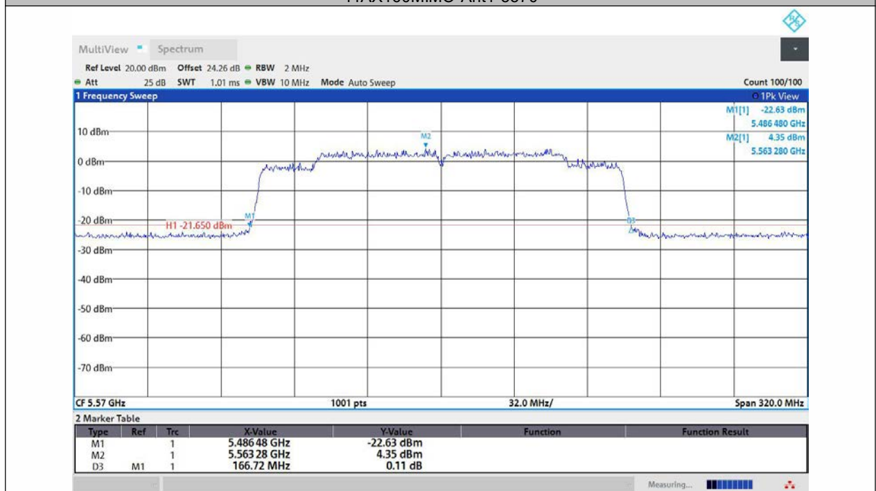
11AX160MIMO-Ant2-5570
