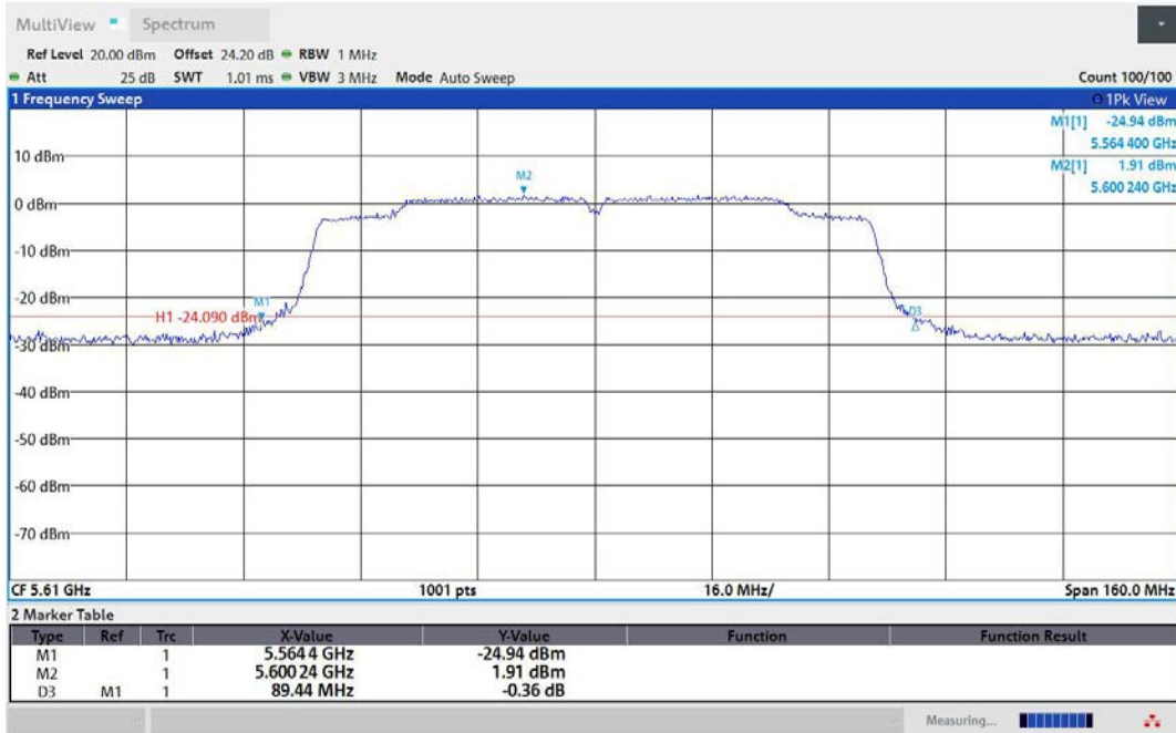
11AC80MIMO-Ant2-5610
