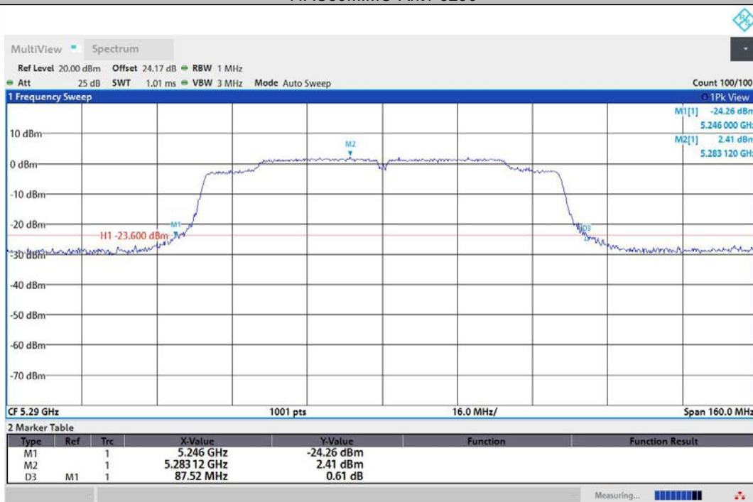
11AC80MIMO-Ant2-5290
