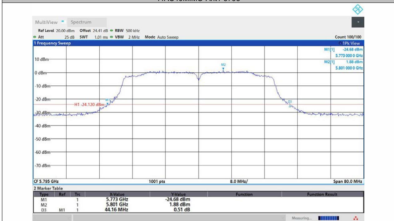
11AC40MIMO-Ant2-5795
