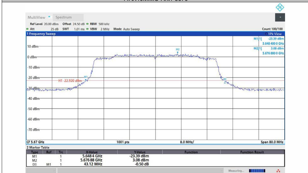
11AX40MIMO-Ant2-5670
