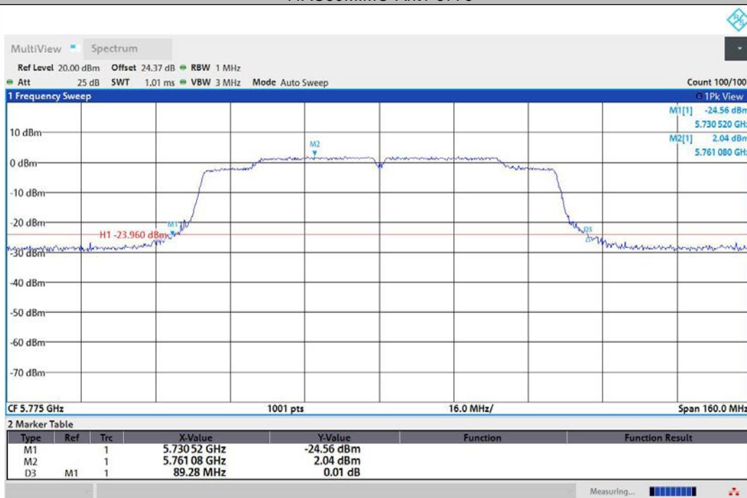
11AC80MIMO-Ant2-5775
