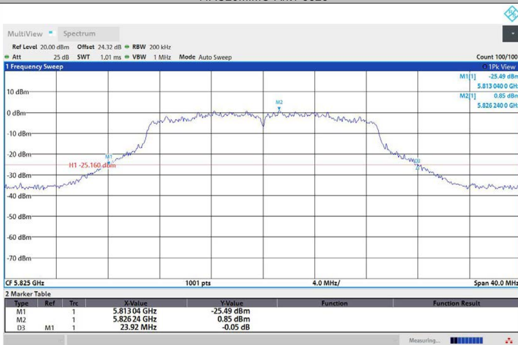
11AC20MIMO-Ant2-5825
