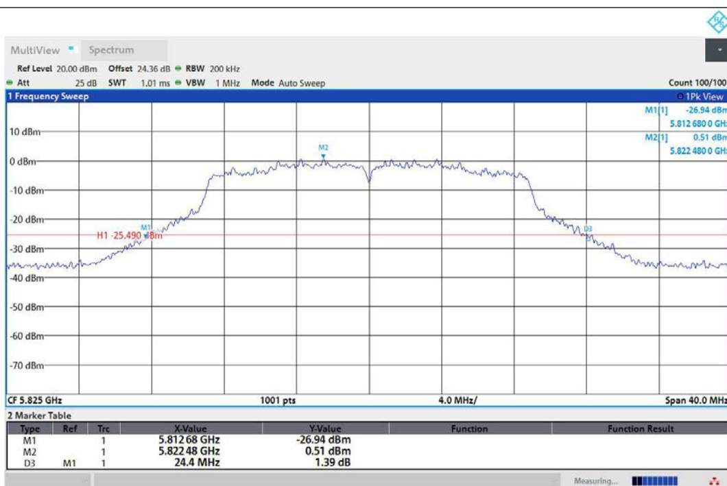
11AC20MIMO-Ant1-5825
