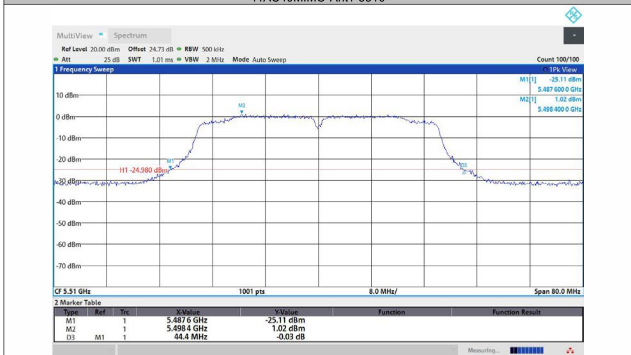
11AC40MIMO-Ant2-5510
