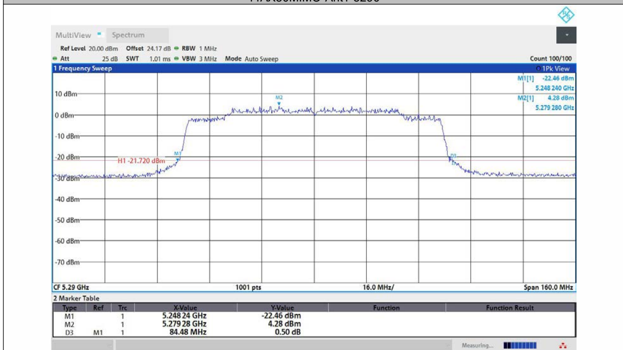
11AX80MIMO-Ant2-5290
